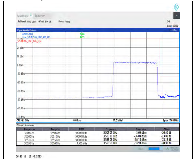
1-N78-3450-3550-30-50-H-3-DFT-PI2BPSK-Outer_Full-128@0-Ant1-1--PASS-see graph
