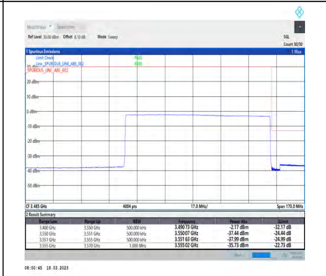
1-N78-3450-3550-30-90-H-6-CP-QPSK-Outer_Full-245@0-Ant1-1--PASS-see graph
