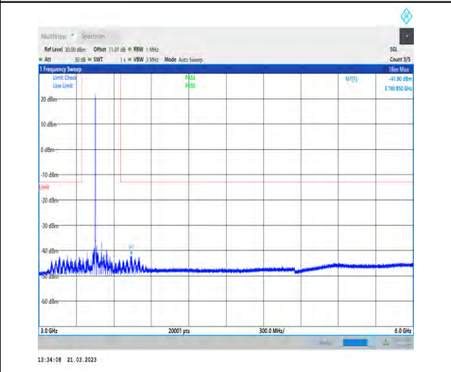
1-N77-3450-3550-30-100-M-1-DFT-QPSK-Edge_1R B_Left-1@0-3000-6000-Ant1-3740.85--41.90--13-PA SS
