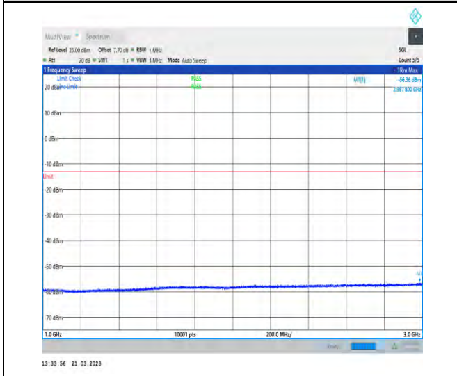
1-N77-3450-3550-30-100-M-1-DFT-QPSK-Edge_1R B_Left-1@0-1000-3000-Ant1-2987.80--56.36--13-PA SS
