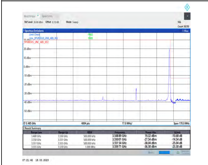
1-N78-3450-3550-30-70-H-5-CP-QPSK-Edge_1RB_Right-1@188-Ant1-1--PASS-see graph
