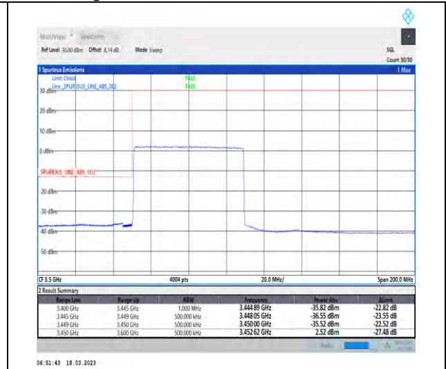
1-N78-3450-3550-30-60-L-3-DFT-PI2BPSK-Outer_Full-162@0-Ant1-1--PASS-see graph
