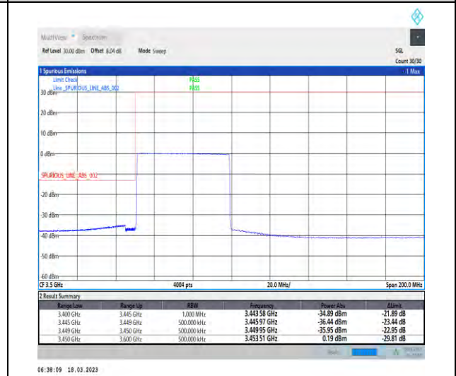
1-N78-3450-3550-30-50-L-6-CP-QPSK-Outer_Full -133@0-Ant1-1--PASS-see graph
