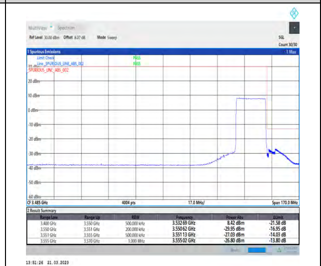
1-N77-3450-3550-30-20-H-6-CP-QPSK-Outer_Full -51@0-Ant1-1--PASS-see graph
