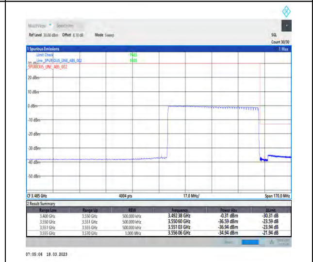
1-N78-3450-3550-30-60-H-6-CP-QPSK-Outer_Full-162@0-Ant1-1--PASS-see graph
