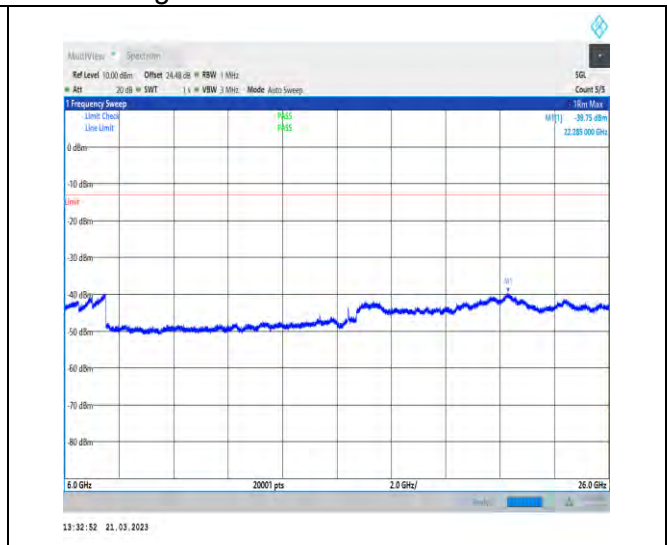
1-N77-3450-3550-30-100-L-1-DFT-QPSK-Edge_1R B_Left-1@0-6000-26000-Ant1-22285.00--39.75--13- PASS
