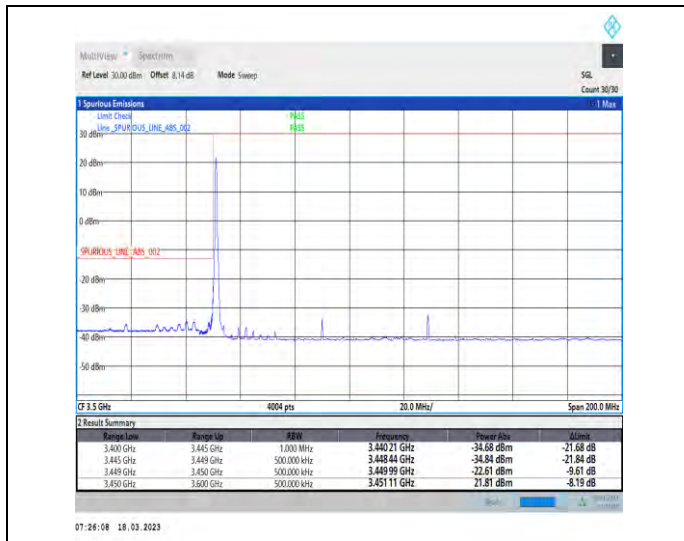
1-N78-3450-3550-30-80-L-1-DFT-PI2BPSK-Edge_1RB_Left-1@0-Ant1-1--PASS-see graph
