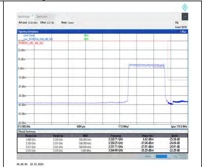
1-N78-3450-3550-30-40-H-3-DFT-PI2BPSK-Outer_Full-100@0-Ant1-1--PASS-see graph
