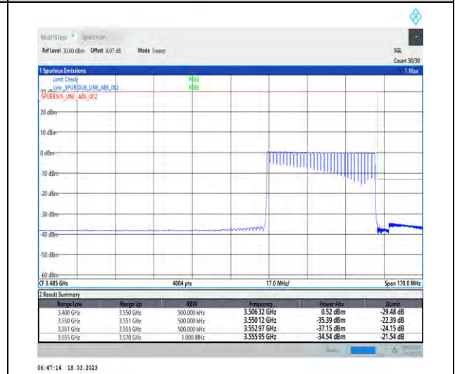
1-N78-3450-3550-30-50-H-6-CP-QPSK-Outer_Full-133@0-Ant1-1--PASS-see graph
