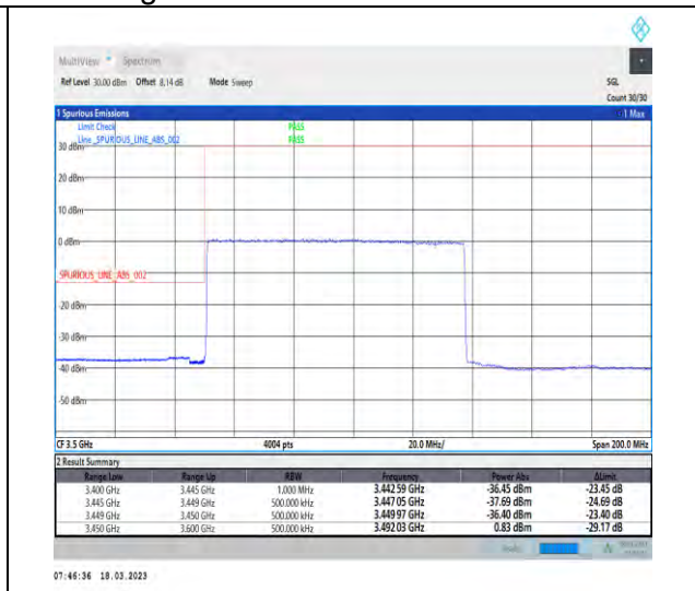
1-N78-3450-3550-30-90-L-3-DFT-PI2BPSK-Outer_Full-240@0-Ant1-1--PASS-see graph
