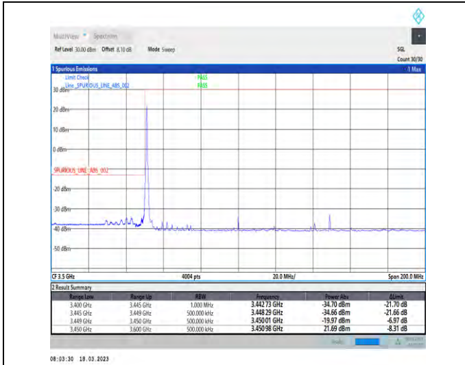
1-N78-3450-3550-30-100-L-1-DFT-PI2BPSK-Edge_1R_B_Left-1@0-Ant1-1--PASS-see graph
