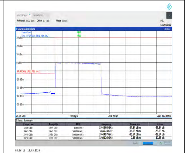
1-N78-3450-3550-30-60-L-6-CP-QPSK-Outer_Full -162@0-Ant1-1--PASS-see graph
