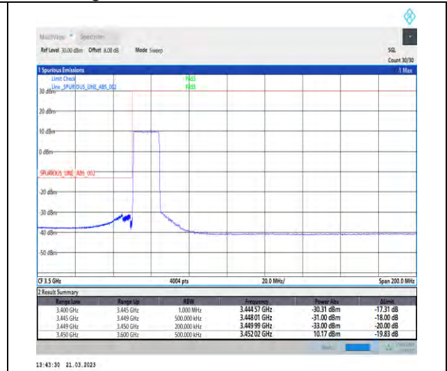
1-N77-3450-3550-30-15-L-6-CP-QPSK-Outer_Full -38@0-Ant1-1--PASS-see graph
