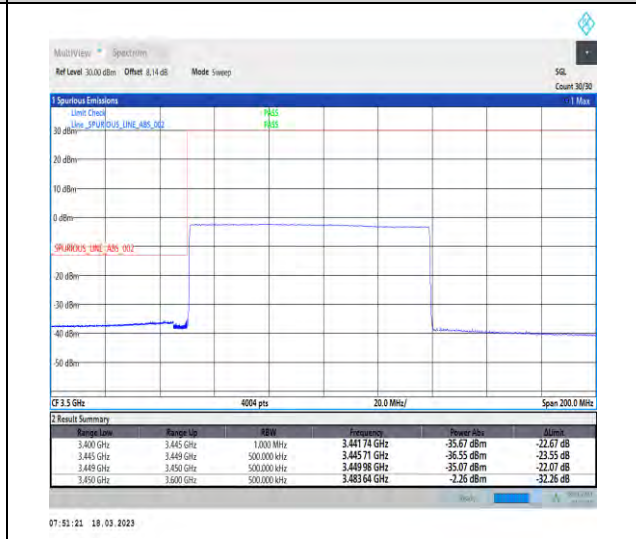
1-N78-3450-3550-30-90-L-6-CP-QPSK-Outer_Full -245@0-Ant1-1--PASS-see graph
