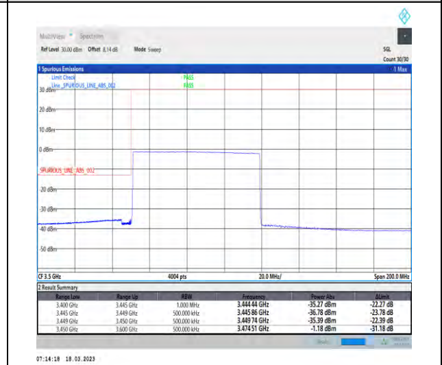
1-N78-3450-3550-30-70-L-6-CP-QPSK-Outer_Full -189@0-Ant1-1--PASS-see graph
