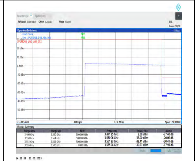
1-N77-3450-3550-30-80-H-6-CP-QPSK-Outer_Full -217@0-Ant1-1--PASS-see graph
