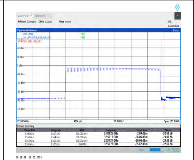
1-N78-3450-3550-30-100-H-6-CP-QPSK-Outer_Full-273@0-Ant1-1--PASS-see graph
