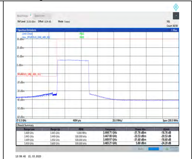
1-N77-3450-3550-30-40-L-6-CP-QPSK-Outer_Full -106@0-Ant1-1--PASS-see graph
