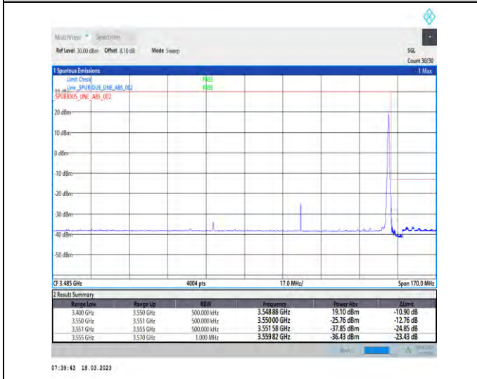
1-N78-3450-3550-30-80-H-5-CP-QPSK-Edge_1RB_Right-1@216-Ant1-1--PASS-see graph
