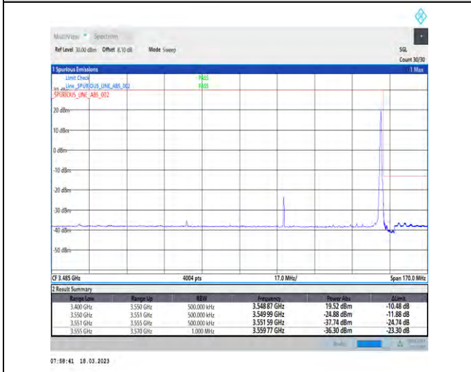
1-N78-3450-3550-30-90-H-5-CP-QPSK-Edge_1RB_Right-1@244-Ant1-1--PASS-see graph
