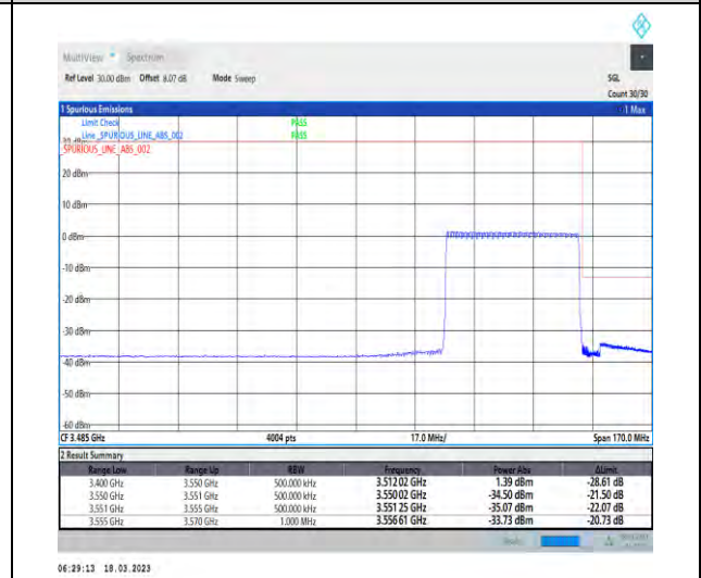
1-N78-3450-3550-30-40-H-6-CP-QPSK-Outer_Full-106@0-Ant1-1--PASS-see graph
