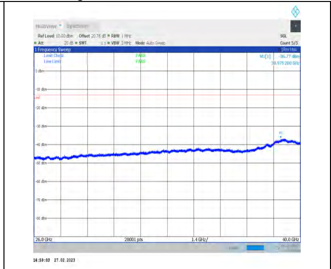
1-N77-3450-3550-30-100-M-1-DFT-QPSK-Edge_1R B_Left-1@0-26000-40000-Ant1-26000.00--45.11--13 -PASS
