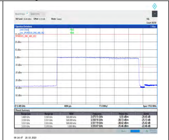
1-N78-3450-3550-30-100-H-3-DFT-PI2BPSK-Outer_Full-270@0-Ant1-1--PASS-see graph
