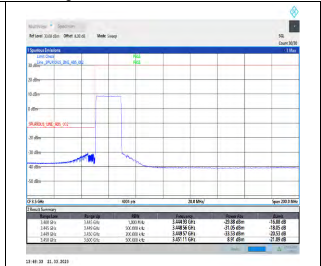
1-N77-3450-3550-30-20-L-6-CP-QPSK-Outer_Full -51@0-Ant1-1--PASS-see graph
