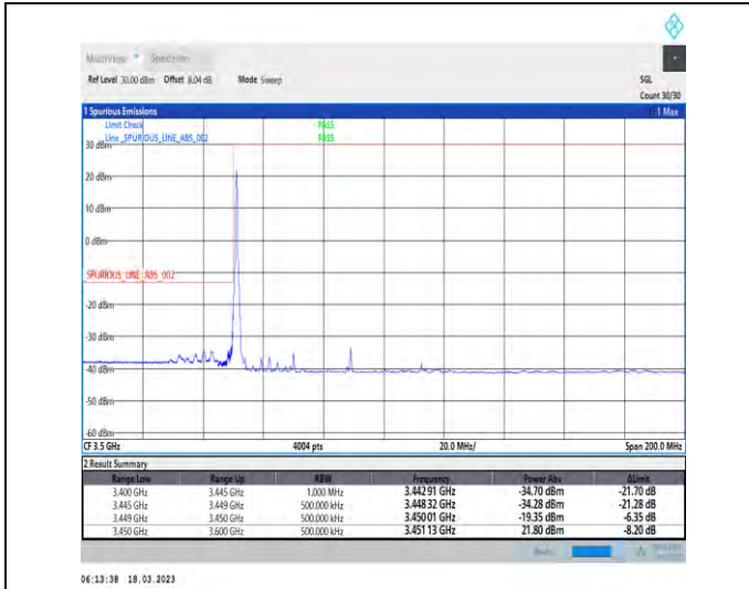
1-N78-3450-3550-30-40-L-1-DFT-PI2BPSK-Edge_1RB_Left-1@0-Ant1-1--PASS-see graph
