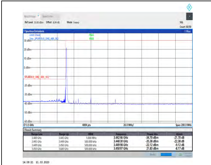
1-N77-3450-3550-30-60-L-4-CP-QPSK-Edge_1RB_Lef t-1@0-Ant1-1--PASS-see graph
