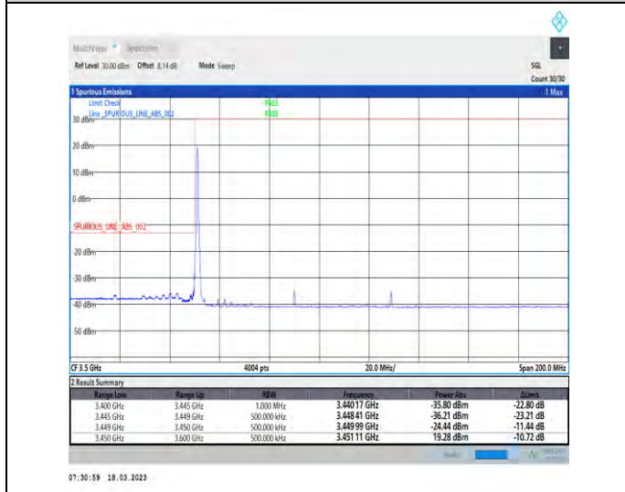
1-N78-3450-3550-30-80-L-4-CP-QPSK-Edge_1RB_Lef t-1@0-Ant1-1--PASS-see graph
