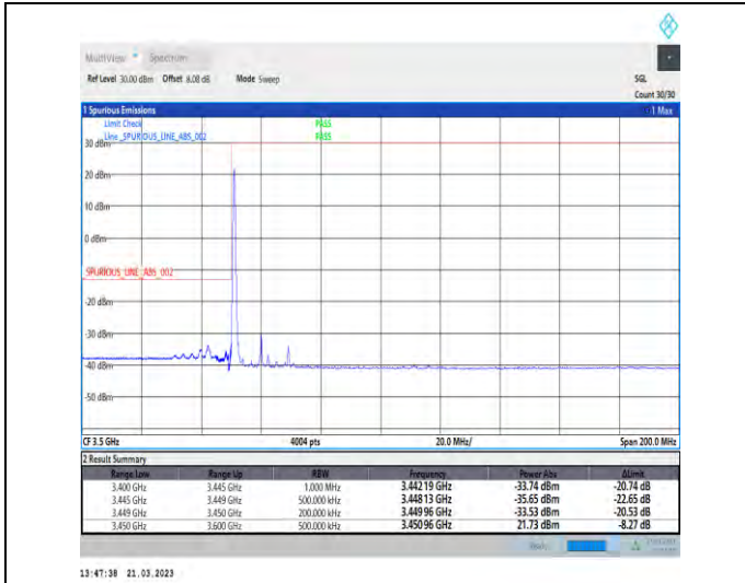
1-N77-3450-3550-30-20-L-4-CP-QPSK-Edge_1RB_Lef t-1@0-Ant1-1--PASS-see graph
