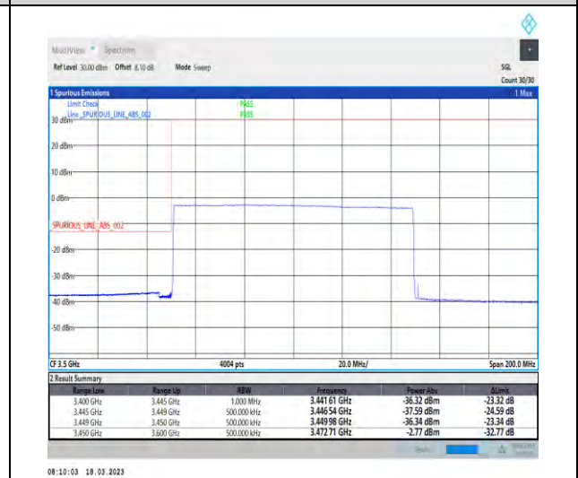
1-N78-3450-3550-30-100-L-6-CP-QPSK-Outer_Full-273@0-Ant1-1--PASS-see graph
