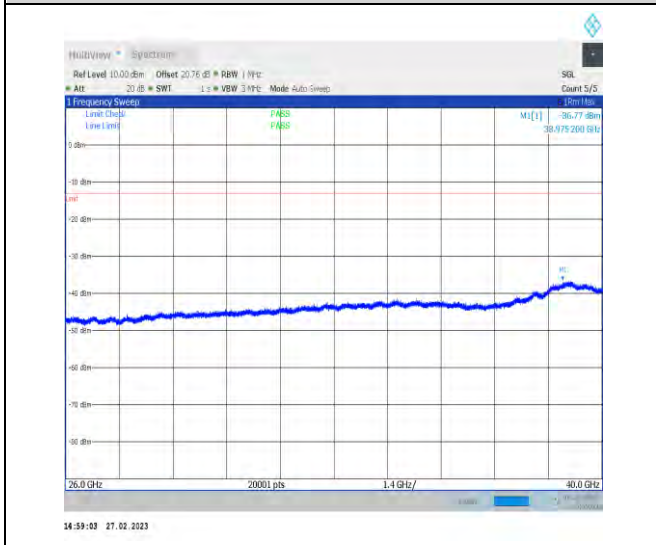
1-N77-3450-3550-30-100-L-1-DFT-QPSK-Edge_1R B_Left-1@0-26000-40000-Ant1-26000.00--45.34--13 -PASS
