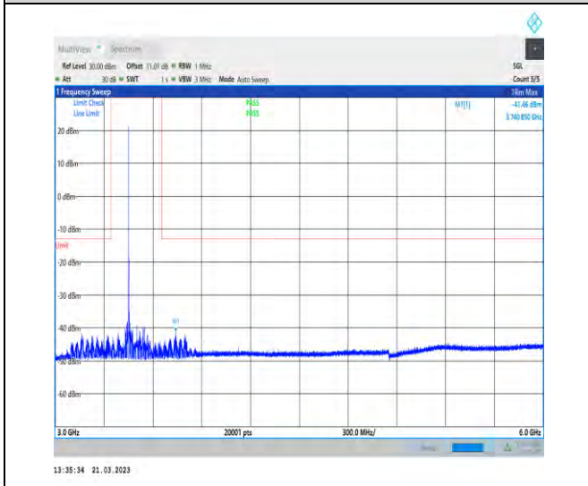
1-N77-3450-3550-30-100-H-1-DFT-QPSK-Edge_1R B_Left-1@0-3000-6000-Ant1-3740.85--41.46--13-PA SS
