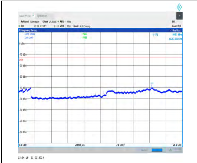
1-N77-3450-3550-30-100-M-1-DFT-QPSK-Edge_1R B_Left-1@0-6000-26000-Ant1-22282.00--39.51--13- PASS
