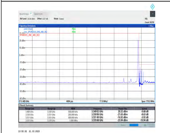
1-N77-3450-3550-30-20-H-5-CP-QPSK-Edge_1RB_Ri ght-1@50-Ant1-1--PASS-see graph
