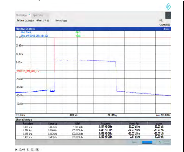
1-N77-3450-3550-30-80-L-6-CP-QPSK-Outer_Full -217@0-Ant1-1--PASS-see graph
