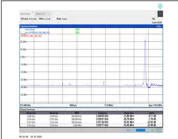
1-N78-3450-3550-30-100-H-2-DFT-PI2BPSK-Edge_1R_B_Right-1@272-Ant1-1--PASS-see graph
