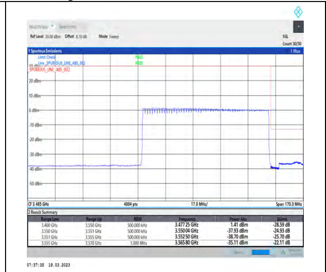
1-N78-3450-3550-30-80-H-3-DFT-PI2BPSK-Outer_Full-216@0-Ant1-1--PASS-see graph
