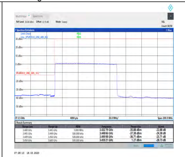
1-N78-3450-3550-30-80-L-3-DFT-PI2BPSK-Outer_Full-216@0-Ant1-1--PASS-see graph
