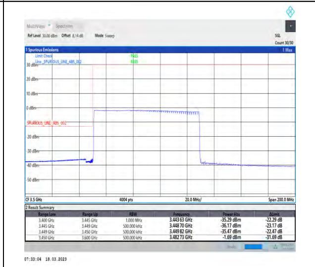
1-N78-3450-3550-30-80-L-6-CP-QPSK-Outer_Full -217@0-Ant1-1--PASS-see graph
