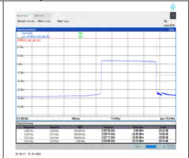
1-N78-3450-3550-30-60-H-3-DFT-PI2BPSK-Outer_Full-162@0-Ant1-1--PASS-see graph
