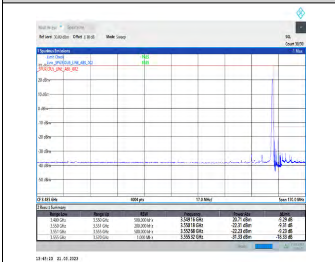
1-N77-3450-3550-30-15-H-5-CP-QPSK-Edge_1RB_Ri ght-1@37-Ant1-1--PASS-see graph
