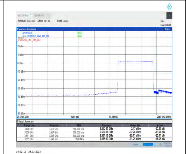
1-N77-3450-3550-30-40-H-6-CP-QPSK-Outer_Full -106@0-Ant1-1--PASS-see graph
