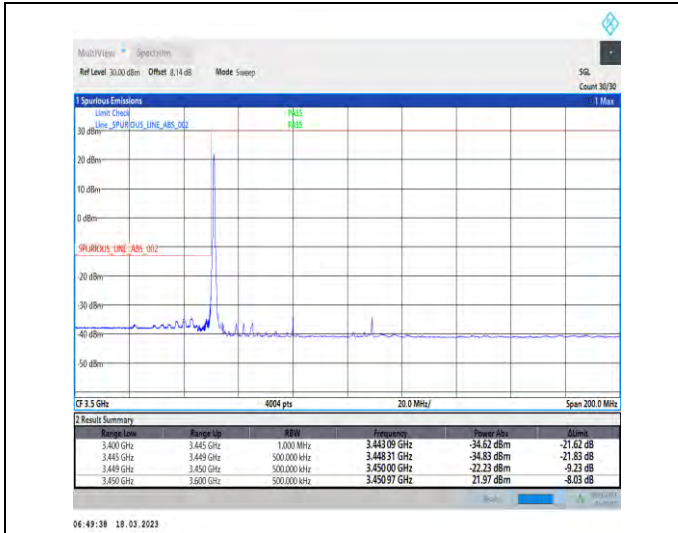
1-N78-3450-3550-30-60-L-1-DFT-PI2BPSK-Edge_1RB_Left-1@0-Ant1-1--PASS-see graph
