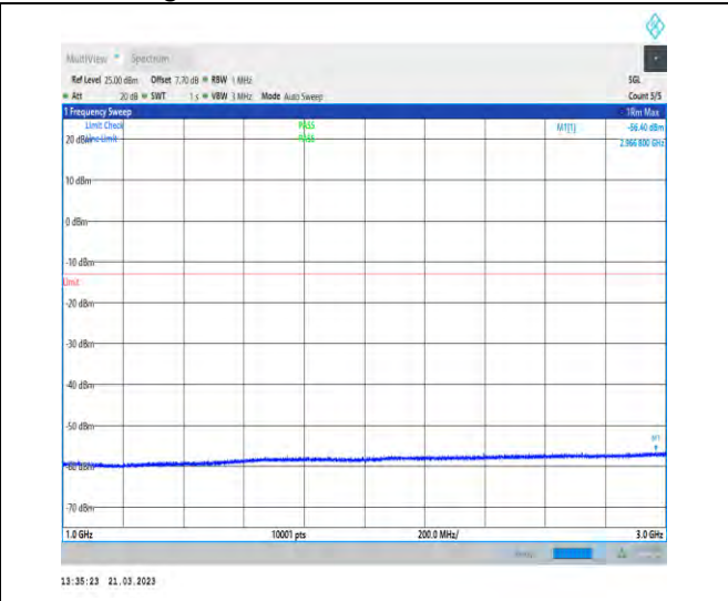
1-N77-3450-3550-30-100-H-1-DFT-QPSK-Edge_1R B_Left-1@0-1000-3000-Ant1-2966.80--56.40--13-PA SS
