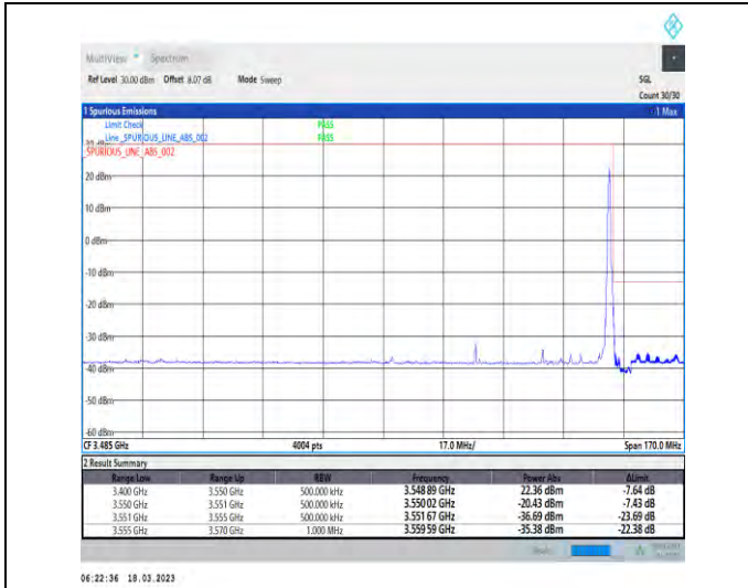
1-N78-3450-3550-30-40-H-2-DFT-PI2BPSK-Edge_1R_B_Right-1@105-Ant1-1--PASS-see graph
