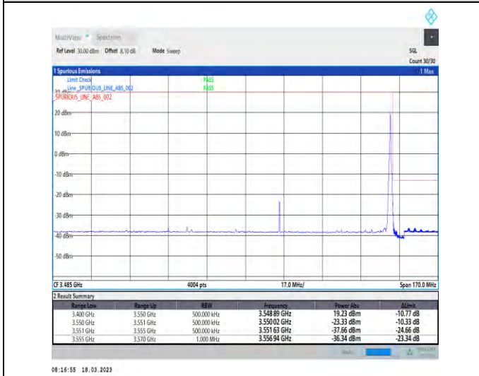
1-N78-3450-3550-30-100-H-5-CP-QPSK-Edge_1RB_Right-1@272-Ant1-1--PASS-see graph
