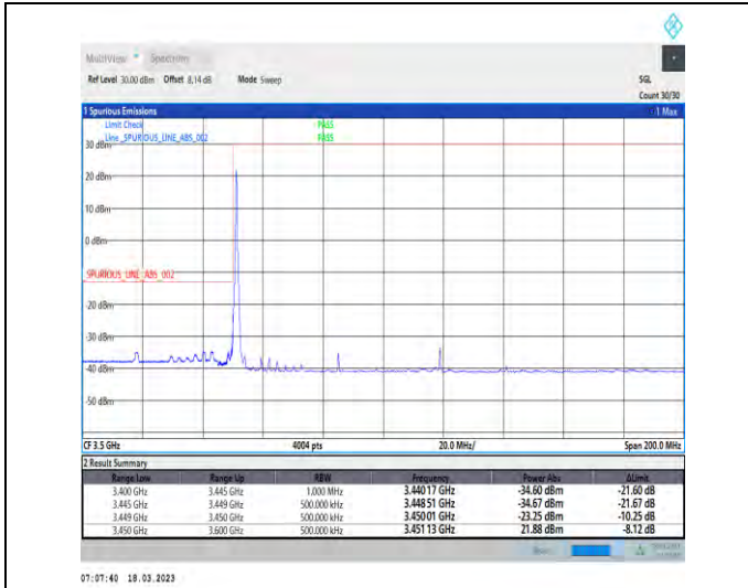
1-N78-3450-3550-30-70-L-1-DFT-PI2BPSK-Edge_1RB_Left-1@0-Ant1-1--PASS-see graph
