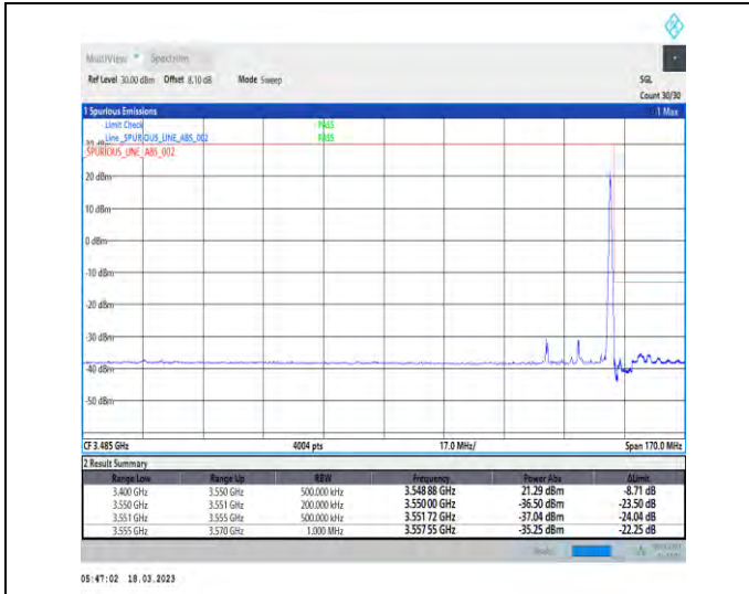
1-N78-3450-3550-30-20-H-2-DFT-PI2BPSK-Edge_1R_B_Right-1@50-Ant1-1--PASS-see graph
