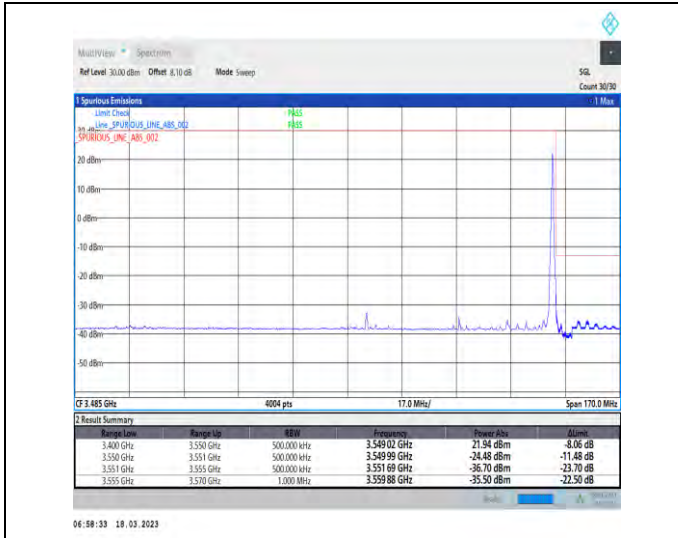
1-N78-3450-3550-30-60-H-2-DFT-PI2BPSK-Edge_1R_B_Right-1@161-Ant1-1--PASS-see graph
