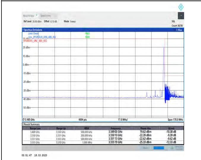
1-N78-3450-3550-30-20-H-5-CP-QPSK-Edge_1RB_Right-1@50-Ant1-1--PASS-see graph
