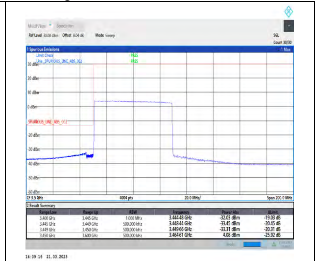
1-N77-3450-3550-30-60-L-6-CP-QPSK-Outer_Full -162@0-Ant1-1--PASS-see graph
