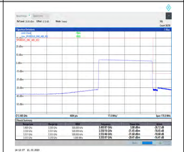
1-N77-3450-3550-30-60-H-6-CP-QPSK-Outer_Full -162@0-Ant1-1--PASS-see graph
