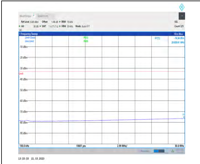
1-N77-3450-3550-30-100-M-1-DFT-QPSK-Edge_1R B_Left-1@0-0.15-30-Ant1-29.84--76.34--33-PASS
