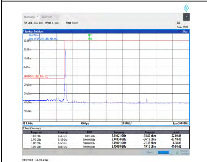
1-N78-3450-3550-30-100-L-4-CP-QPSK-Edge_1RB_Left-1@0-Ant1-1--PASS-see graph
