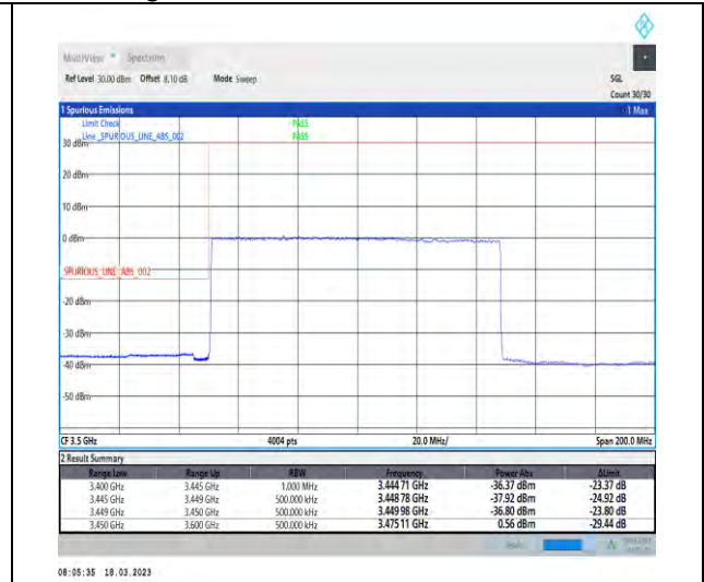
1-N78-3450-3550-30-100-L-3-DFT-PI2BPSK-Outer_Full-270@0-Ant1-1--PASS-see graph
