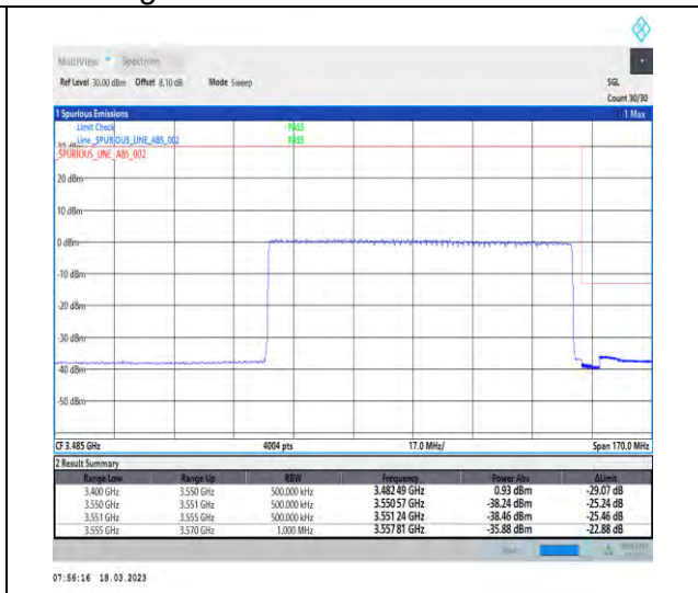
1-N78-3450-3550-30-90-H-3-DFT-PI2BPSK-Outer_Full-240@0-Ant1-1--PASS-see graph
