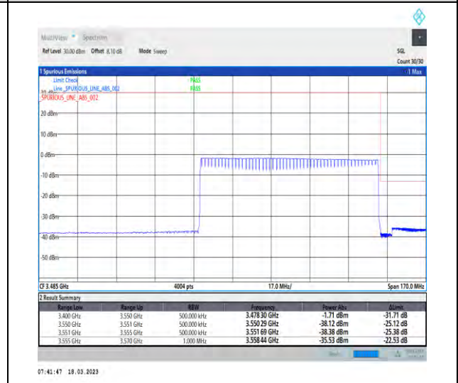
1-N78-3450-3550-30-80-H-6-CP-QPSK-Outer_Full-217@0-Ant1-1--PASS-see graph
