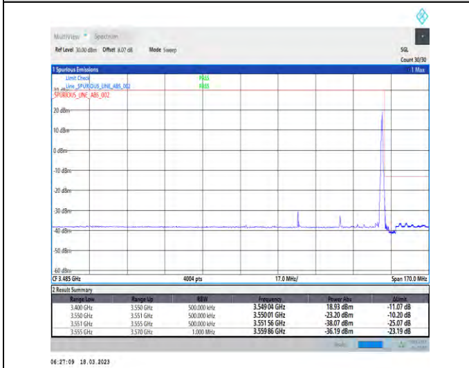
1-N78-3450-3550-30-40-H-5-CP-QPSK-Edge_1RB_Right-1@105-Ant1-1--PASS-see graph
