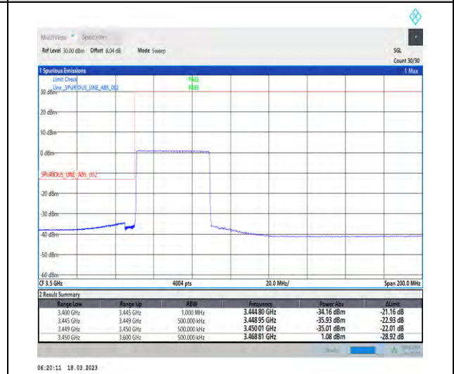
1-N78-3450-3550-30-40-L-6-CP-QPSK-Outer_Full -106@0-Ant1-1--PASS-see graph
