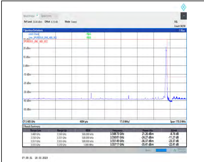
1-N78-3450-3550-30-80-H-2-DFT-PI2BPSK-Edge_1R_B_Right-1@216-Ant1-1--PASS-see graph
