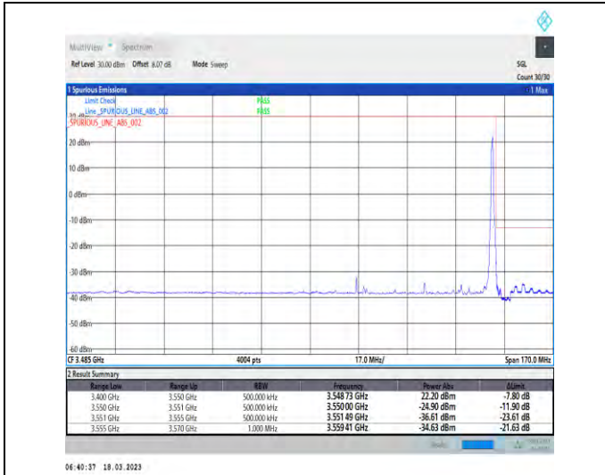
1-N78-3450-3550-30-50-H-2-DFT-PI2BPSK-Edge_1R_B_Right-1@132-Ant1-1--PASS-see graph
