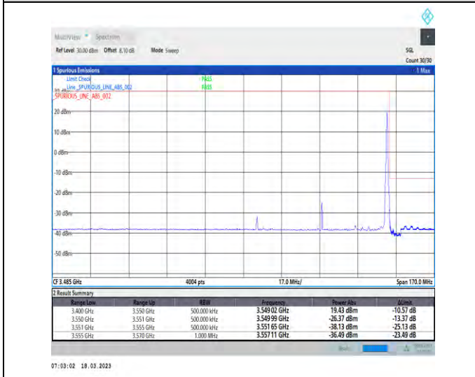
1-N78-3450-3550-30-60-H-5-CP-QPSK-Edge_1RB_Right-1@161-Ant1-1--PASS-see graph
