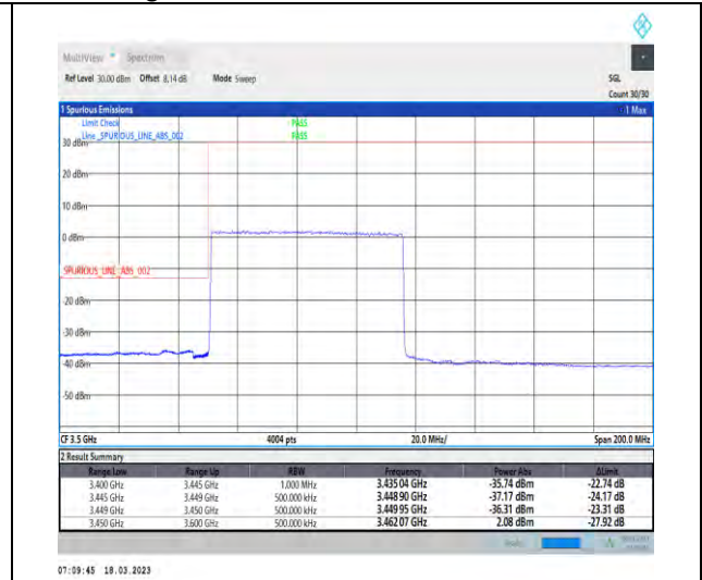
1-N78-3450-3550-30-70-L-3-DFT-PI2BPSK-Outer_Full-180@0-Ant1-1--PASS-see graph
