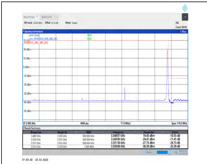
1-N78-3450-3550-30-90-H-2-DFT-PI2BPSK-Edge_1R_B_Right-1@244-Ant1-1--PASS-see graph
