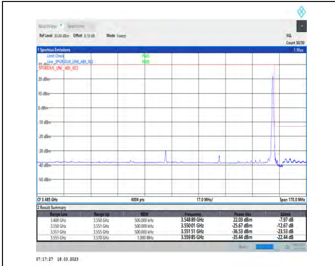
1-N78-3450-3550-30-70-H-2-DFT-PI2BPSK-Edge_1R_B_Right-1@188-Ant1-1--PASS-see graph
