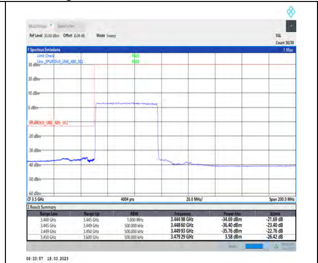
1-N78-3450-3550-30-50-L-3-DFT-PI2BPSK-Outer_Full-128@0-Ant1-1--PASS-see graph
