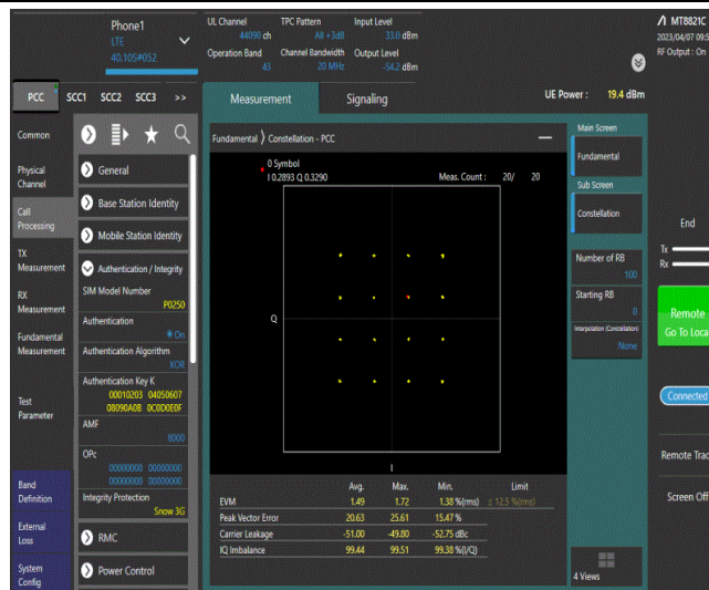
Band43-20MHz-16QAM-44090-100RB#0
