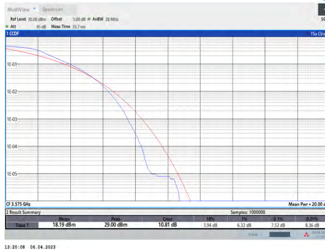
Band42-20MHz-QPSK-43340-100RB#0
