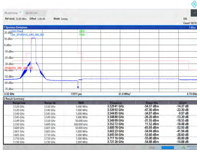
Band42-5MHz-QPSK-43115-25RB#0
