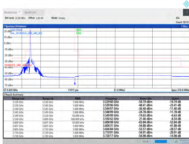
Band42-5MHz-QPSK-43115-1RB#0
