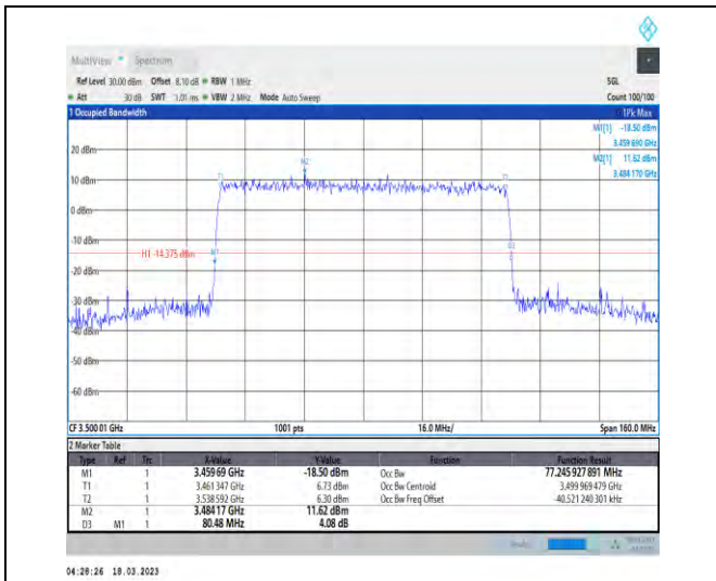
1-N78-3450-3550-30-80-M-6-CP-QPSK-Outer_Full-2 17@0-Ant1-77.246-80.480-≤80-PASS
