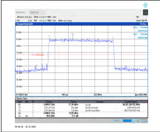
1-N78-3450-3550-30-100-L-3-DFT-16QAM-Outer_Fu ll-270@0-Ant1-96.291-99.600-≤100-PASS
