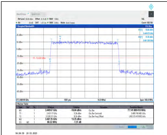
1-N78-3450-3550-30-80-L-3-DFT-16QAM-Outer_Full -216@0-Ant1-77.142-80.320-≤80-PASS
