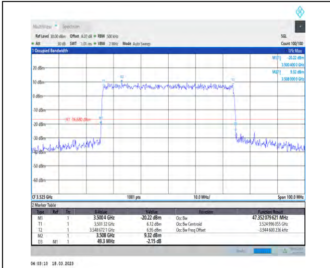
1-N78-3450-3550-30-50-H-6-CP-QPSK-Outer_Full-1 33@0-Ant1-47.352-49.300-≤50-PASS
