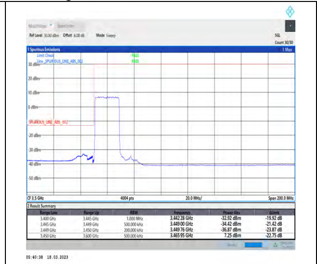
1-N78-3450-3550-30-20-L-3-DFT-PI2BPSK-Outer_Full-50@0-Ant1-1--PASS-see graph
