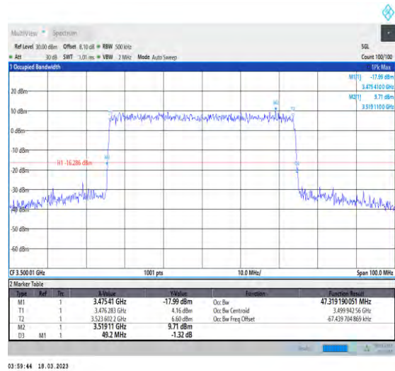
1-N78-3450-3550-30-50-M-6-CP-QPSK-Outer_Full-1 33@0-Ant1-47.319-49.200-≤50-PASS
