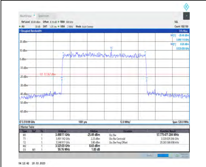
1-N78-3450-3550-30-60-H-5-DFT-256QAM-Outer_F ull-162@0-Ant1-57.775-59.760-≤60-PASS
