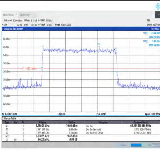
1-N78-3450-3550-30-70-H-4-DFT-64QAM-Outer_Ful I-180@0-Ant1-64.285-66.220-≤70-PASS
