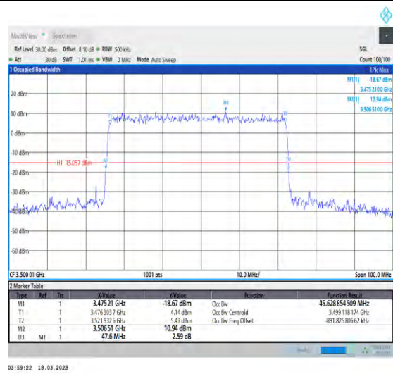
1-N78-3450-3550-30-50-M-4-DFT-64QAM-Outer_Ful I-128@0-Ant1-45.629-47.600-≤50-PASS
