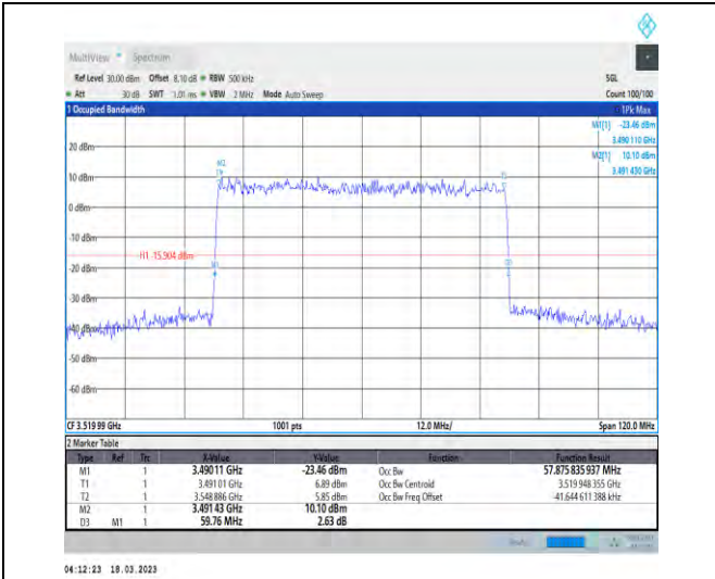
1-N78-3450-3550-30-60-H-3-DFT-16QAM-Outer_Ful I-162@0-Ant1-57.876-59.760-≤60-PASS
