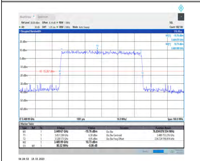
1-N78-3450-3550-30-80-L-5-DFT-256QAM-Outer_Fu ll-216@0-Ant1-76.835-80.320-≤80-PASS
