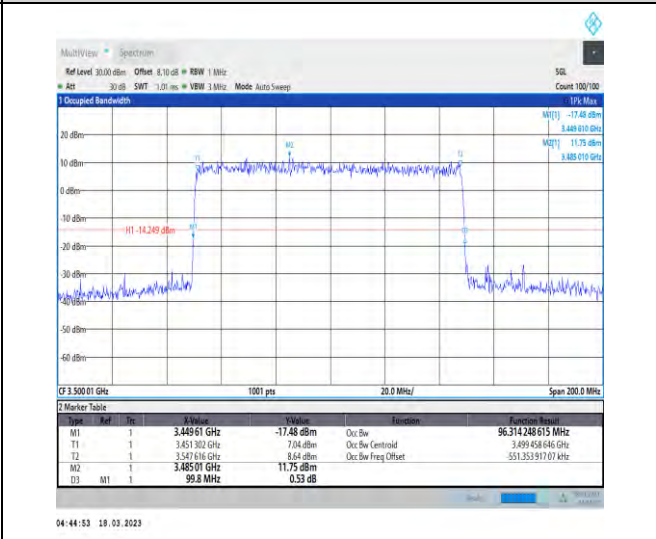
1-N78-3450-3550-30-100-M-3-DFT-16QAM-Outer_F ull-270@0-Ant1-96.314-99.800-≤100-PASS
