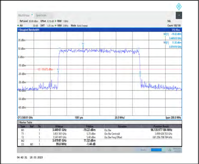
1-N78-3450-3550-30-100-L-4-DFT-64QAM-Outer_F ull-270@0-Ant1-96.136-99.800-≤100-PASS
