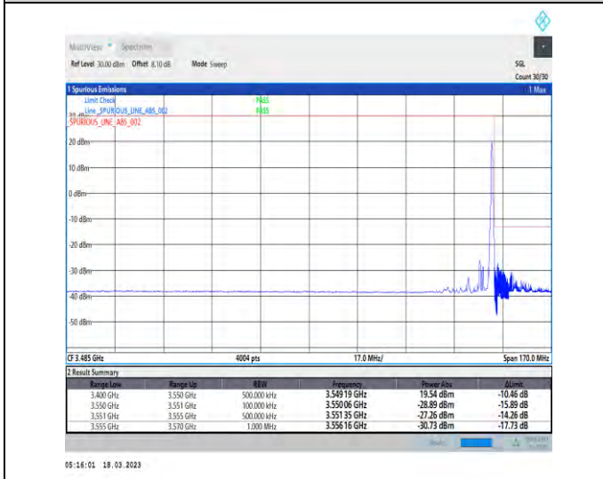
1-N78-3450-3550-30-10-H-5-CP-QPSK-Edge_1RB_Right-1@23-Ant1-1--PASS-see graph
