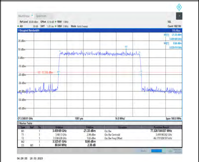
1-N78-3450-3550-30-80-M-9-CP-256QAM-Outer_Fu ll-217@0-Ant1-77.328-80.640-≤80-PASS
