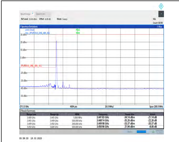
1-N78-3450-3550-30-20-L-1-DFT-PI2BPSK-Edge_1RB_Left-1@0-Ant1-1--PASS-see graph
