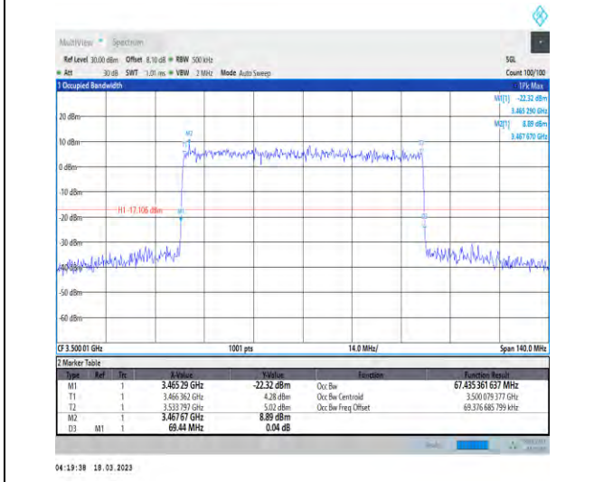
1-N78-3450-3550-30-70-M-7-CP-16QAM-Outer_Full-189@0-Ant1-67.435-69.440-≤70-PASS
