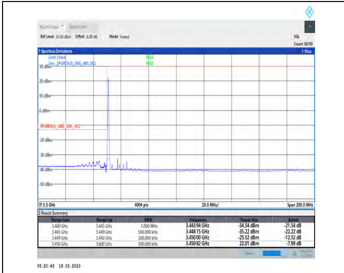
1-N78-3450-3550-30-15-L-1-DFT-PI2BPSK-Edge_1RB_Left-1@0-Ant1-1--PASS-see graph
