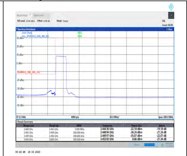
1-N78-3450-3550-30-15-L-3-DFT-PI2BPSK-Outer_Full-36@0-Ant1-1--PASS-see graph
