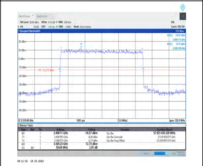
1-N78-3450-3550-30-60-H-2-DFT-PI2BPSK-Outer_Full-162@0-Ant1-57.921-59.640-≤60-PASS
