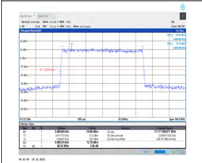
1-N78-3450-3550-30-80-H-3-DFT-16QAM-Outer_Full-216@0-Ant1-77.118-80.320-≤80-PASS
