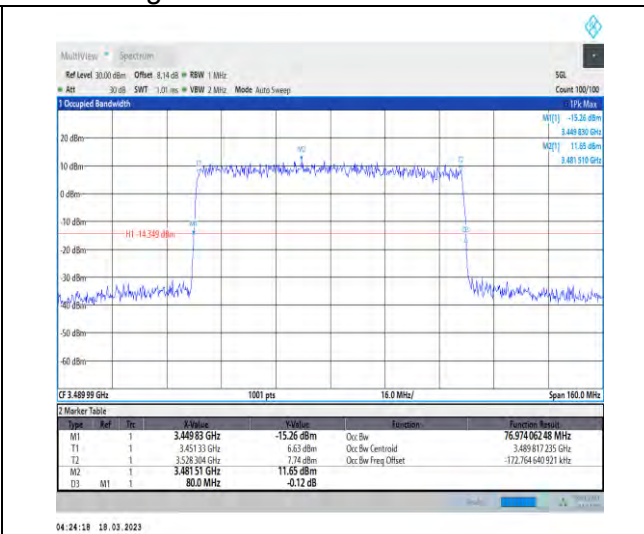
1-N78-3450-3550-30-80-L-4-DFT-64QAM-Outer_Full -216@0-Ant1-76.974-80.000-≤80-PASS
