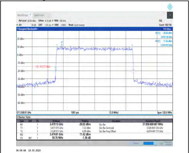
1-N78-3450-3550-30-60-M-1-DFT-QPSK-Outer_Full -162@0-Ant1-57.857-59.760-≤60-PASS
