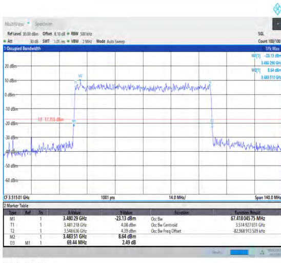
1-N78-3450-3550-30-70-H-6-CP-QPSK-Outer_Full-1 89@0-Ant1-67.418-69.440-≤70-PASS
