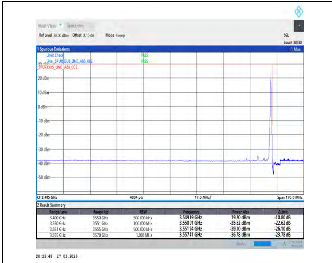
1-N78-3450-3550-30-10-H-2-DFT-PI2BPSK-Edge_1R_B_Right-1@23-Ant1-1--PASS-see graph
