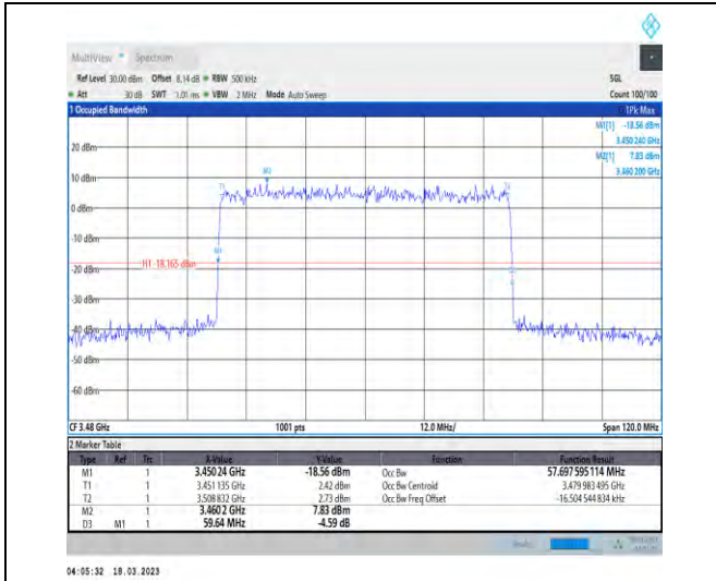
1-N78-3450-3550-30-60-L-5-DFT-256QAM-Outer_Fu II-162@0-Ant1-57.698-59.640-≤60-PASS
