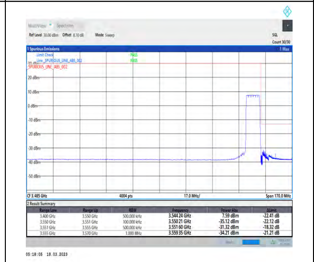
1-N78-3450-3550-30-10-H-6-CP-QPSK-Outer_Full-24@0-Ant1-1--PASS-see graph
