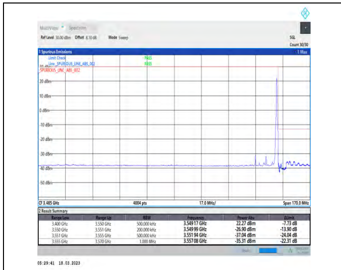
1-N78-3450-3550-30-15-H-2-DFT-PI2BPSK-Edge_1R_B_Right-1@37-Ant1-1--PASS-see graph
