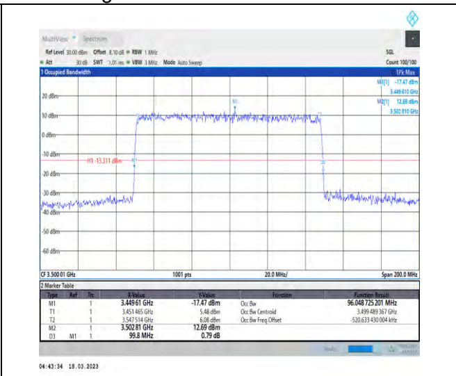
1-N78-3450-3550-30-100-M-1-DFT-QPSK-Outer_Ful l-270@0-Ant1-96.049-99.800-≤100-PASS
