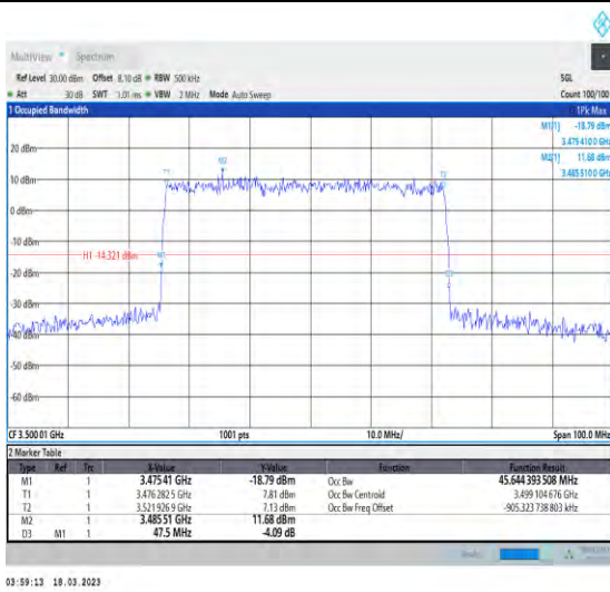
1-N78-3450-3550-30-50-M-3-DFT-16QAM-Outer_Ful I-128@0-Ant1-45.644-47.500-≤50-PASS
