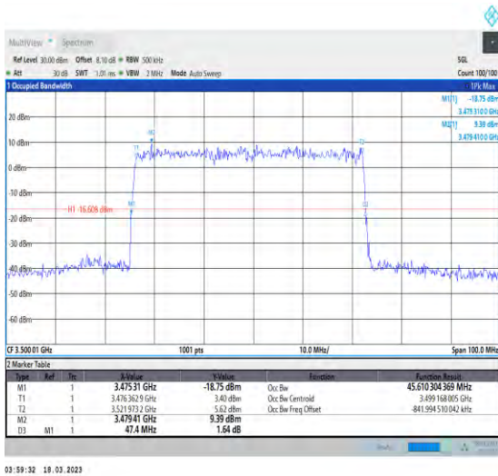
1-N78-3450-3550-30-50-M-5-DFT-256QAM-Outer_F ull-128@0-Ant1-45.61-47.400-≤50-PASS
