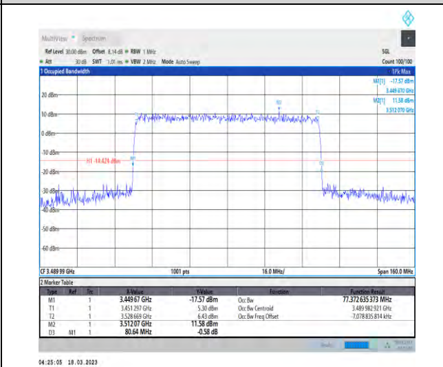
1-N78-3450-3550-30-80-L-6-CP-QPSK-Outer_Full-2 17@0-Ant1-77.373-80.640-≤80-PASS
