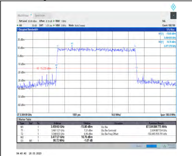
1-N78-3450-3550-30-90-H-7-CP-16QAM-Outer_Full-245@0-Ant1-87.534-90.720-≤90-PASS
