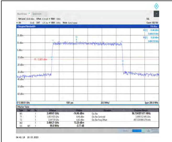
1-N78-3450-3550-30-100-L-1-DFT-QPSK-Outer_Full -270@0-Ant1-96.155-99.800-≤100-PASS
