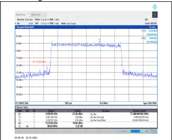
1-N78-3450-3550-30-80-M-7-CP-16QAM-Outer_Full -217@0-Ant1-77.288-80.640-≤80-PASS
