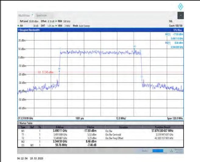
1-N78-3450-3550-30-60-H-6-CP-QPSK-Outer_Full-1 62@0-Ant1-57.879-59.760-≤60-PASS
