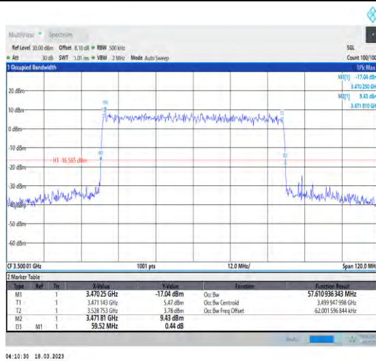
1-N78-3450-3550-30-60-M-7-CP-16QAM-Outer_Full-162@0-Ant1-57.611-59.520-≤60-PASS
