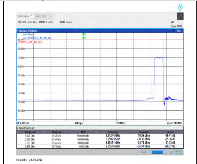
1-N78-3450-3550-30-10-H-3-DFT-PI2BPSK-Outer_Full-24@0-Ant1-1--PASS-see graph
