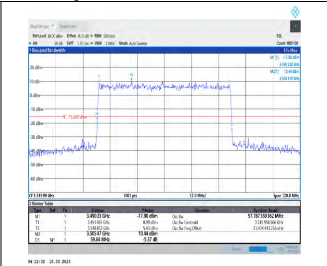
1-N78-3450-3550-30-60-H-4-DFT-64QAM-Outer_Ful I-162@0-Ant1-57.787-59.640-≤60-PASS
