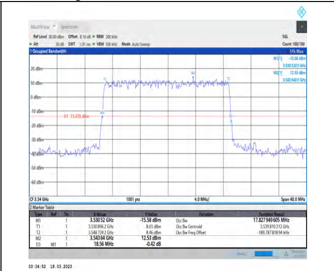
1-N78-3450-3550-30-20-H-2-DFT-PI2BPSK-Outer_Full-50@0-Ant1-17.828-18.560-≤20-PASS
