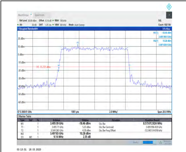
1-N78-3450-3550-30-10-M-4-DFT-64QAM-Outer_Ful I-24@0-Ant1-8.573-9.140-≤10-PASS
