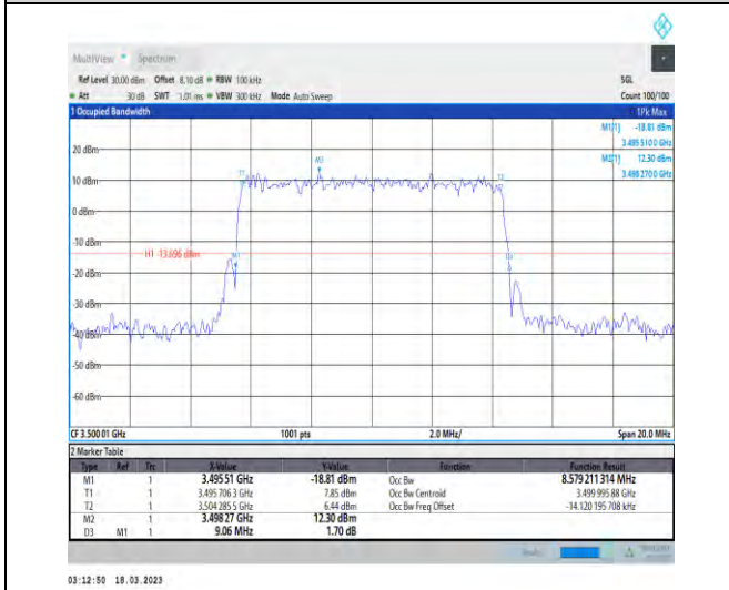
1-N78-3450-3550-30-10-M-2-DFT-PI2BPSK-Outer_Full -24@0-Ant1-8.579-9.060-≤10-PASS
