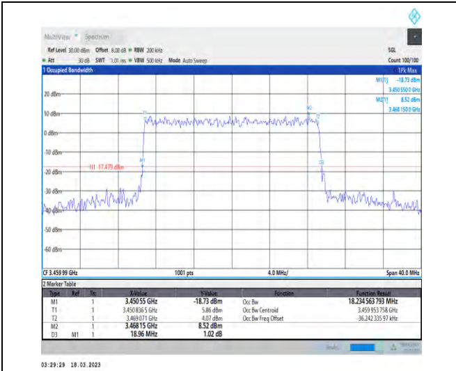
1-N78-3450-3550-30-20-L-7-CP-16QAM-Outer_Full_51@0-Ant1-18.235-18.960-≤20-PASS
