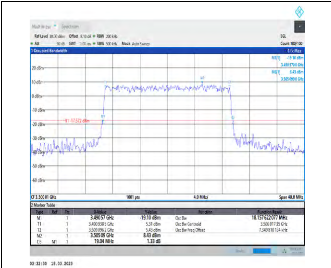
1-N78-3450-3550-30-20-M-6-CP-QPSK-Outer_Full-5 1@0-Ant1-18.158-19.040-≤20-PASS
