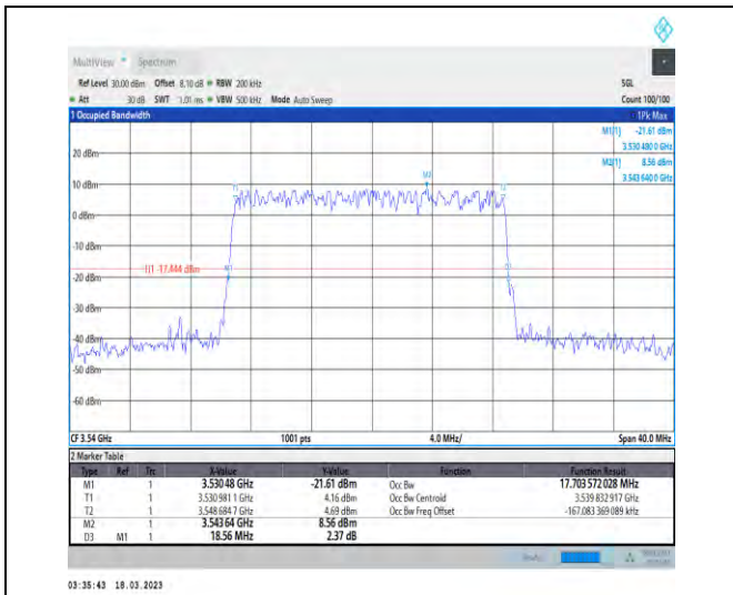
1-N78-3450-3550-30-20-H-5-DFT-256QAM-Outer_Full-50@0-Ant1-17.704-18.560-≤20-PASS
