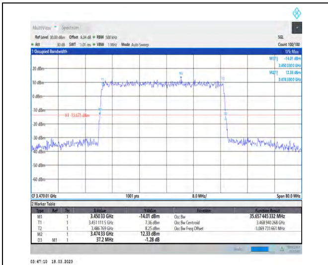
1-N78-3450-3550-30-40-L-3-DFT-16QAM-Outer_Full -100@0-Ant1-35.657-37.200-≤40-PASS
