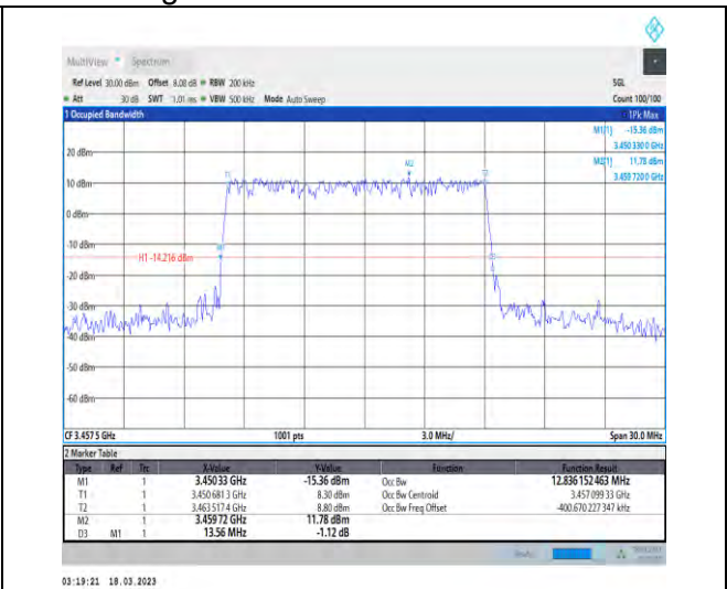
1-N78-3450-3550-30-15-L-3-DFT-16QAM-Outer_Full-36@0-Ant1-12.836-13.560-≤15-PASS
