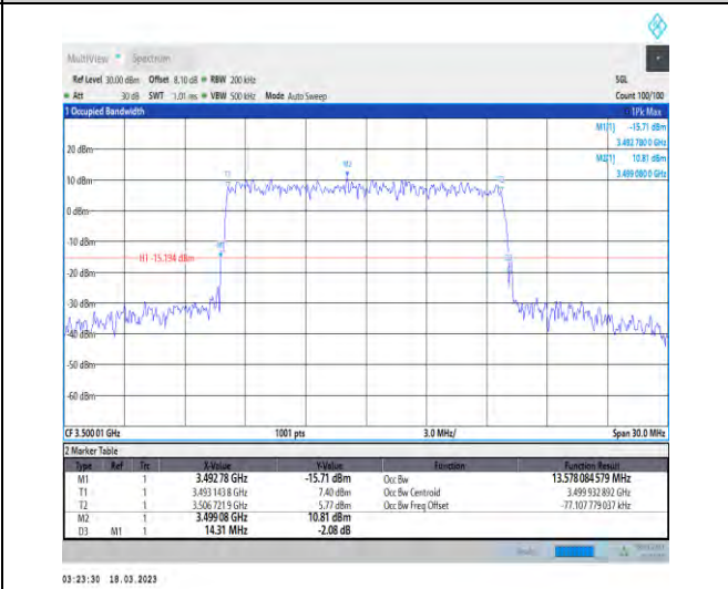
1-N78-3450-3550-30-15-M-8-CP-64QAM-Outer_Full-38@0-Ant1-13.578-14.310-≤15-PASS
