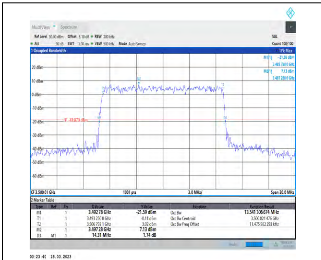
1-N78-3450-3550-30-15-M-9-CP-256QAM-Outer_Ful I-38@0-Ant1-13.541-14.310-≤15-PASS
