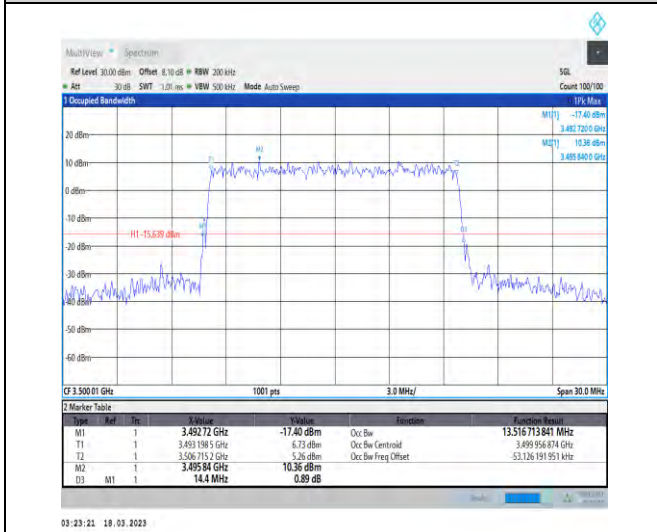
1-N78-3450-3550-30-15-M-7-CP-16QAM-Outer_Full-38@0-Ant1-13.517-14.400-≤15-PASS
