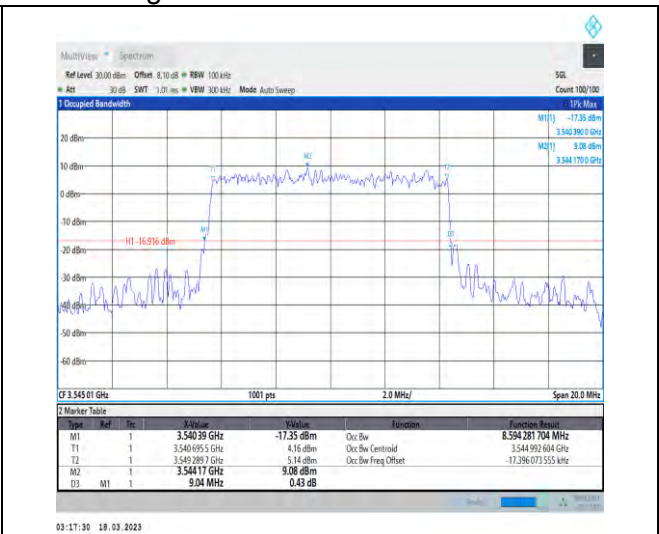
1-N78-3450-3550-30-10-H-8-CP-64QAM-Outer_Full-24@0-Ant1-8.594-9.040-≤10-PASS
