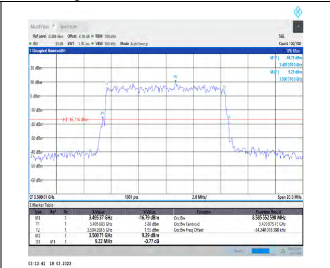
1-N78-3450-3550-30-10-M-5-DFT-256QAM-Outer_Full-24@0-Ant1-8.586-9.220-≤10-PASS
