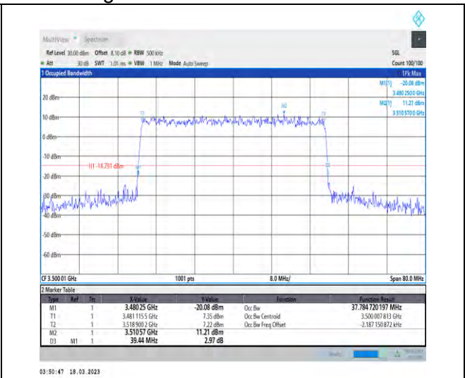
1-N78-3450-3550-30-40-M-7-CP-16QAM-Outer_Full-106@0-Ant1-37.785-39.440-≤40-PASS
