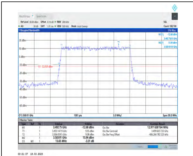
1-N78-3450-3550-30-15-M-1-DFT-QPSK-Outer_Full-36@0-Ant1-12.912-13.650-≤15-PASS
