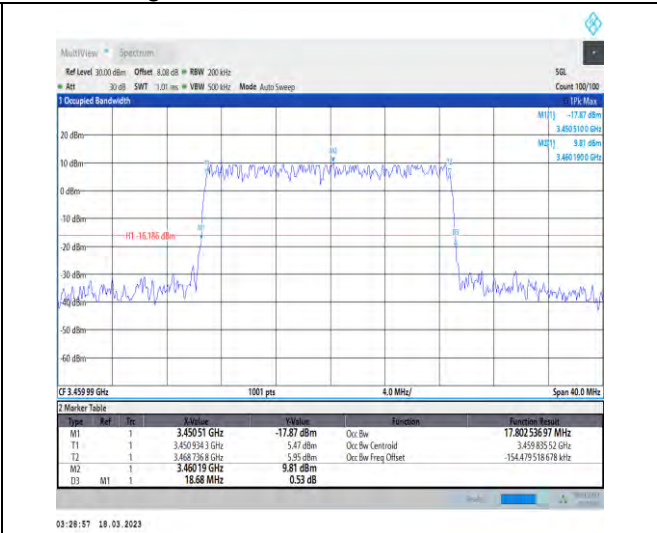
1-N78-3450-3550-30-20-L-4-DFT-64QAM-Outer_Full -50@0-Ant1-17.803-18.680-≤20-PASS
