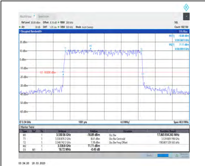
1-N78-3450-3550-30-20-H-1-DFT-QPSK-Outer_Full-50@0-Ant1-17.866-18.720-≤20-PASS
