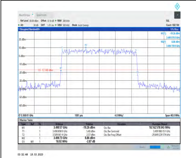
1-N78-3450-3550-30-20-M-8-CP-64QAM-Outer_Full-51@0-Ant1-18.163-18.920-≤20-PASS
