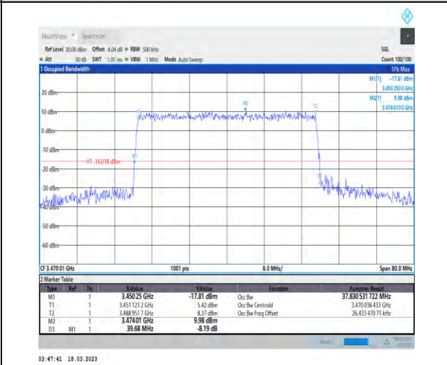
1-N78-3450-3550-30-40-L-6-CP-QPSK-Outer_Full-1 06@0-Ant1-37.831-39.680-≤40-PASS
