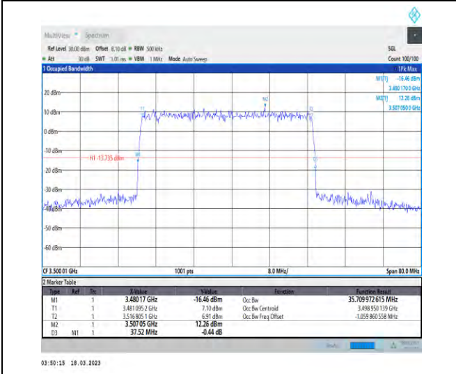
1-N78-3450-3550-30-40-M-4-DFT-64QAM-Outer_Full-100@0-Ant1-35.71-37.520-≤40-PASS
