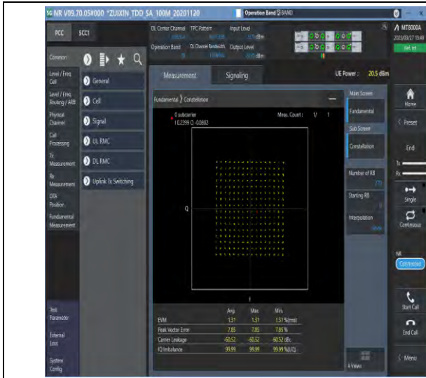
1-N78-3450-3550-30-100-M-5-DFT-256QAM-Outer_Full-270@0-Ant1-see graph-PASS
