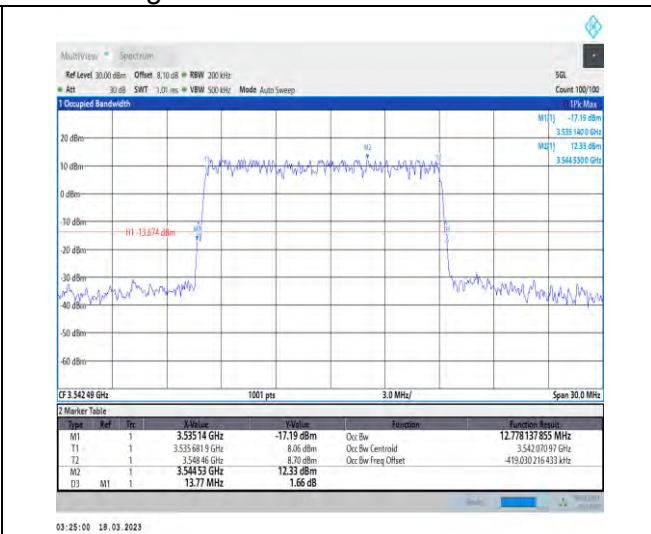
1-N78-3450-3550-30-15-H-1-DFT-QPSK-Outer_Full-36@0-Ant1-12.778-13.770-≤15-PASS
