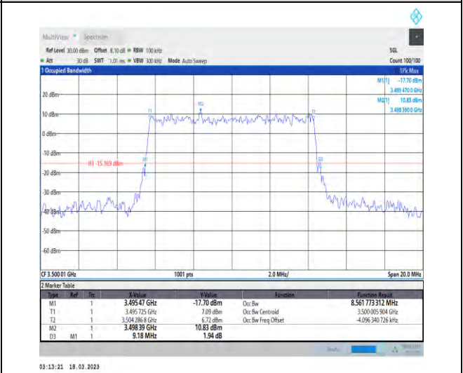
1-N78-3450-3550-30-10-M-3-DFT-16QAM-Outer_Full -24@0-Ant1-8.562-9.180-≤10-PASS
