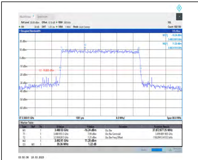
1-N78-3450-3550-30-40-M-6-CP-QPSK-Outer_Full-106@0-Ant1-37.873-39.360-≤40-PASS
