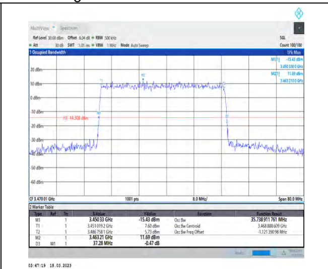
1-N78-3450-3550-30-40-L-4-DFT-64QAM-Outer_Full -100@0-Ant1-35.739-37.280-≤40-PASS
