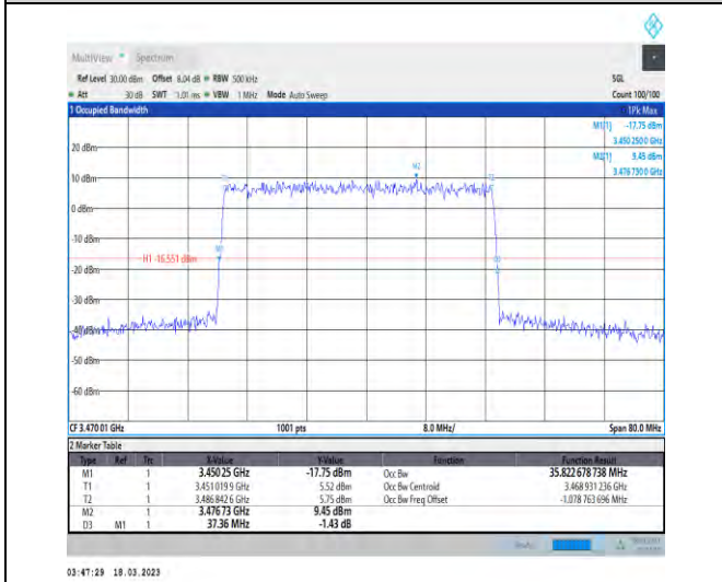
1-N78-3450-3550-30-40-L-5-DFT-256QAM-Outer_Fu ll-100@0-Ant1-35.823-37.360-≤40-PASS
