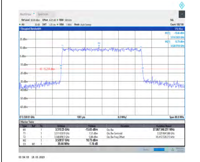
1-N78-3450-3550-30-40-H-7-CP-16QAM-Outer_Full-106@0-Ant1-37.867-39.440-≤40-PASS
