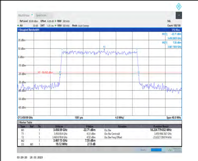
1-N78-3450-3550-30-20-L-6-CP-QPSK-Outer_Full-5 1@0-Ant1-18.225-19.120-≤20-PASS
