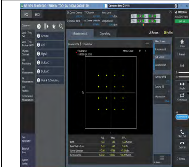
1-N78-3450-3550-30-100-M-7-CP-16QAM-Outer_Full-273@0-Ant1-see graph-PASS
