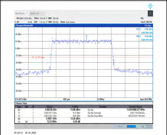
1-N78-3450-3550-30-15-L-1-DFT-QPSK-Outer_Full-36@0-Ant1-12.818-13.530-≤15-PASS
