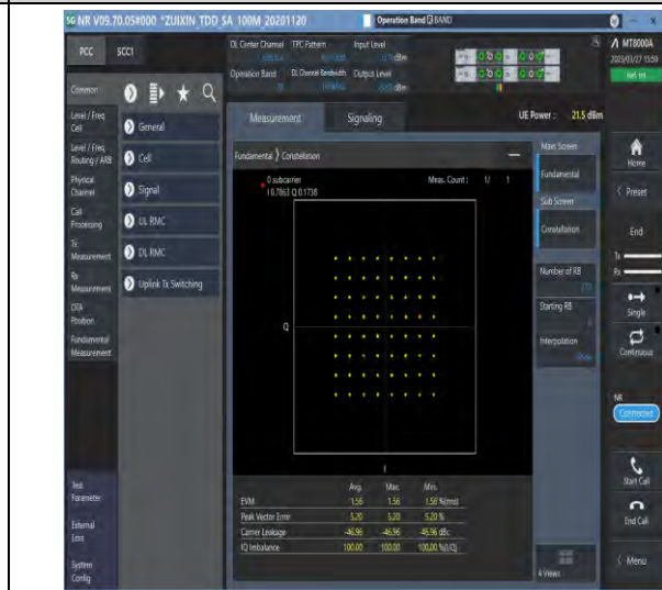
1-N78-3450-3550-30-100-M-8-CP-64QAM-Outer_Full-273@0-Ant1-see graph-PASS
