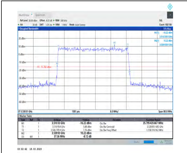
1-N78-3450-3550-30-40-H-5-DFT-256QAM-Outer_Full-100@0-Ant1-35.795-37.360-≤40-PASS
