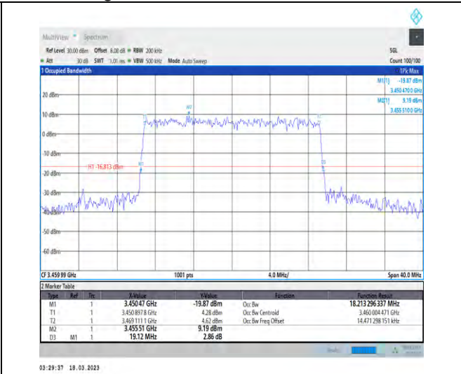
1-N78-3450-3550-30-20-L-8-CP-64QAM-Outer_Full_51@0-Ant1-18.213-19.120-≤20-PASS
