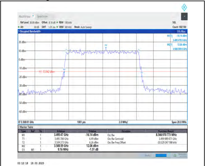
1-N78-3450-3550-30-10-M-1-DFT-QPSK-Outer_Full -24@0-Ant1-8.567-9.160-≤10-PASS
