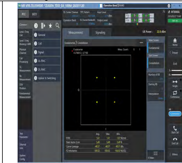
1-N78-3450-3550-30-100-M-6-CP-QPSK-Outer_Full-273@0-Ant1-see graph-PASS
