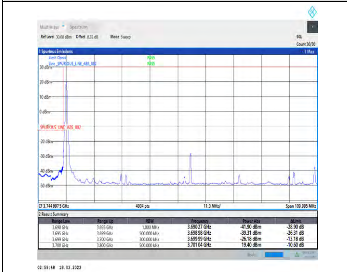
1-N77-3700-3980-30-100-L-4-CP-QPSK-Edge_1RB_Left-1@0-Ant1-1--PASS-see graph
