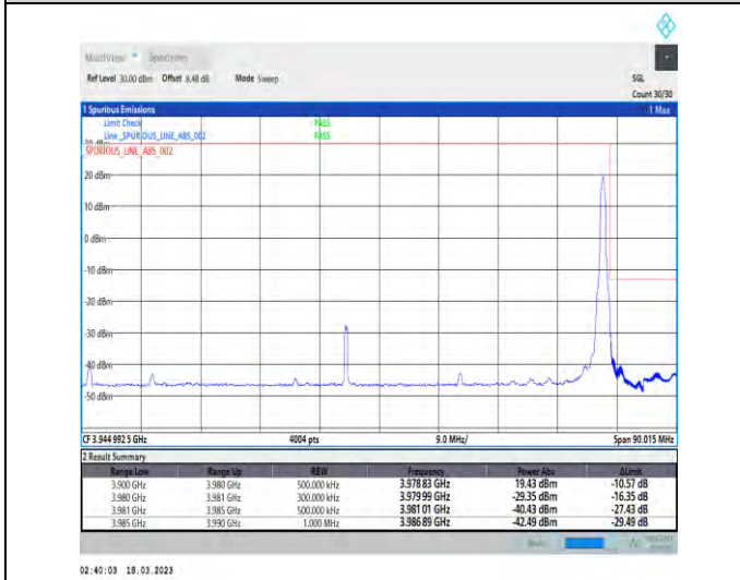
1-N77-3700-3980-30-80-H-5-CP-QPSK-Edge_1RB_Right-1@216-Ant1-1--PASS-see graph
