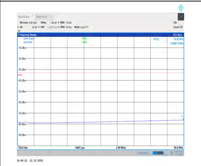
1-N77-3700-3980-30-100-H-1-DFT-QPSK-Edge_1R B_Left-1@0-0.15-30-Ant1-29.86--76.29--33-PASS
