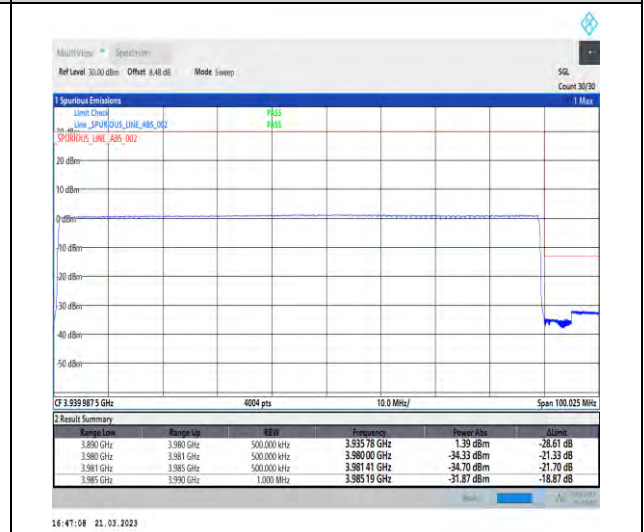
1-N77-3700-3980-30-90-H-6-CP-QPSK-Outer_Full -245@0-Ant1-1--PASS-see graph
