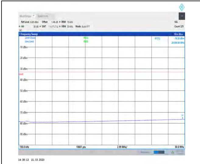
1-N77-3700-3980-30-100-M-1-DFT-QPSK-Edge_1R B_Left-1@0-0.15-30-Ant1-29.59--76.33--33-PASS
