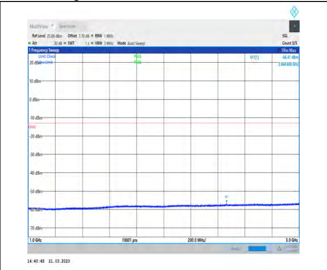
1-N77-3700-3980-30-100-H-1-DFT-QPSK-Edge_1R B_Left-1@0-1000-3000-Ant1-2464.60--56.41--13-PA SS
