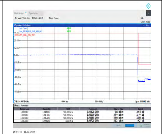
1-N77-3700-3980-30-100-H-6-CP-QPSK-Outer_F ull-273@0-Ant1-1--PASS-see graph
