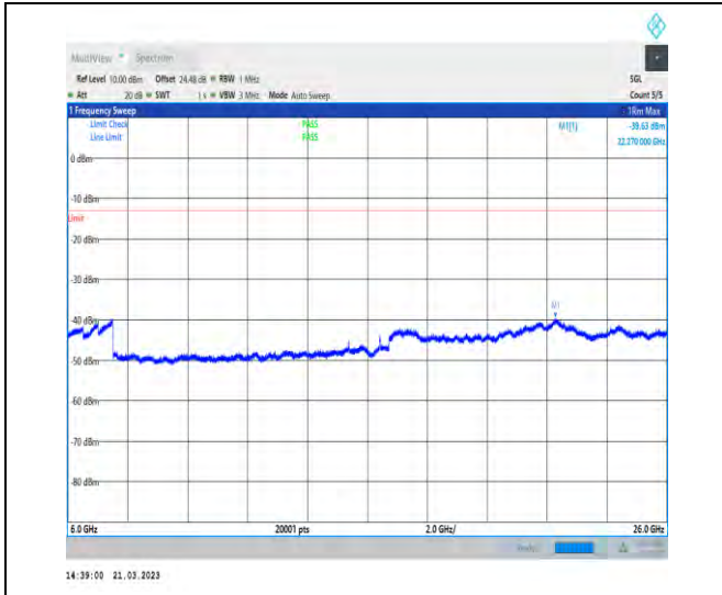
1-N77-3700-3980-30-100-M-1-DFT-QPSK-Edge_1R B_Left-1@0-6000-26000-Ant1-22270.00--39.63--13- PASS
