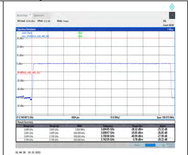
1-N77-3700-3980-30-90-L-3-DFT-PI2BPSK-Outer_Full-240@0-Ant1-1--PASS-see graph
