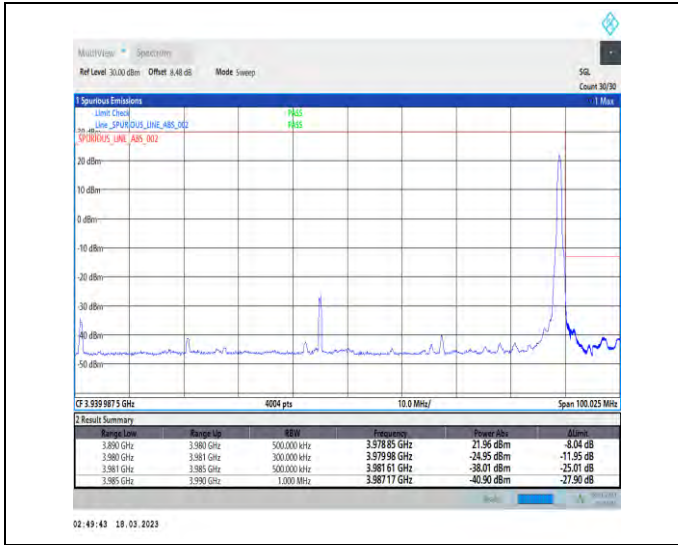
1-N77-3700-3980-30-90-H-2-DFT-PI2BPSK-Edge_1R_B_Right-1@244-Ant1-1--PASS-see graph
