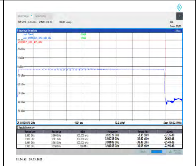
1-N77-3700-3980-30-90-H-6-CP-QPSK-Outer_Full-245@0-Ant1-1--PASS-see graph
