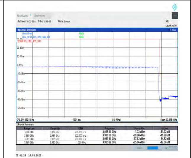
1-N77-3700-3980-30-80-H-6-CP-QPSK-Outer_Full-217@0-Ant1-1--PASS-see graph
