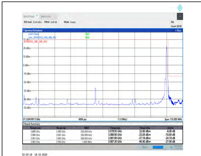
1-N77-3700-3980-30-100-H-2-DFT-PI2BPSK-Edge_1R_B_Right-1@272-Ant1-1--PASS-see graph
