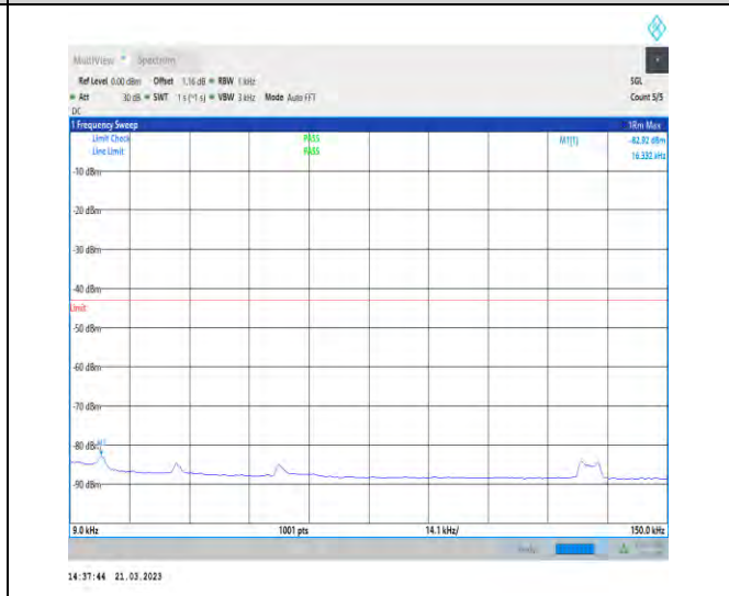
1-N77-3700-3980-30-100-M-1-DFT-QPSK-Edge_1R B_Left-1@0-0.009-0.15-Ant1-0.02--82.92--43-PASS
