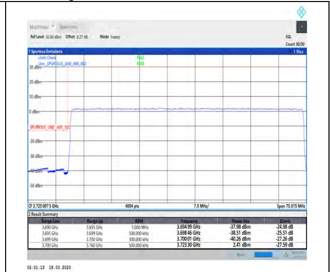
1-N77-3700-3980-30-60-L-3-DFT-PI2BPSK-Outer_Full-162@0-Ant1-1--PASS-see graph
