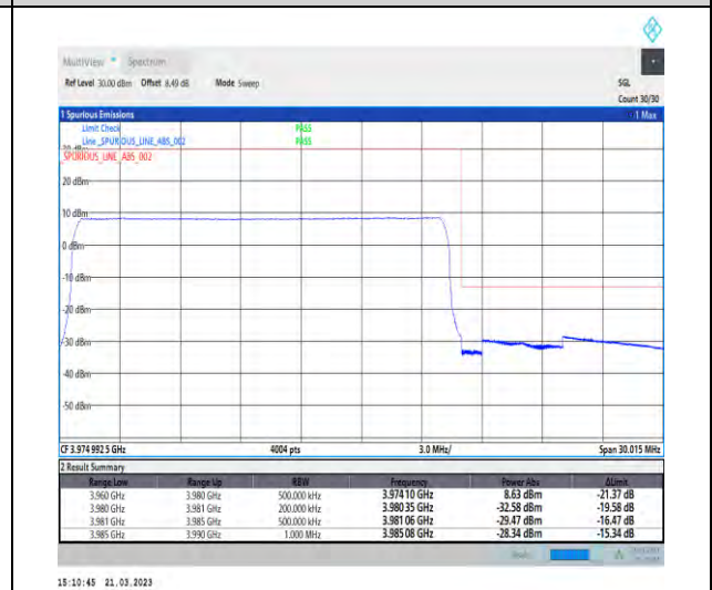
1-N77-3700-3980-30-20-H-6-CP-QPSK-Outer_Full -51@0-Ant1-1--PASS-see graph
