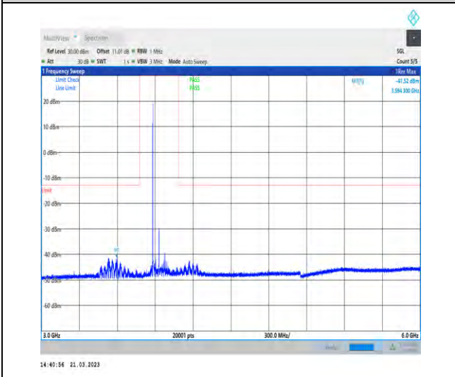
1-N77-3700-3980-30-100-H-1-DFT-QPSK-Edge_1R B_Left-1@0-3000-6000-Ant1-3594.30--41.52--13-PA SS
