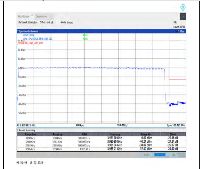
1-N77-3700-3980-30-90-H-3-DFT-PI2BPSK-Outer_Full-240@0-Ant1-1--PASS-see graph
