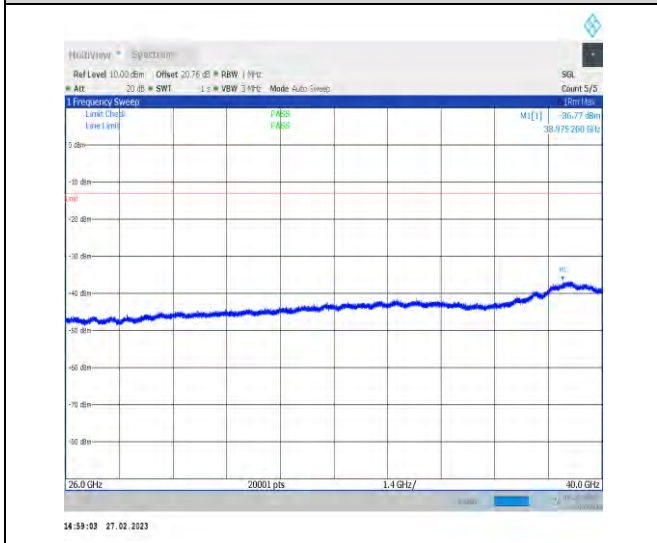
1-N77-3700-3980-30-100-L-1-DFT-QPSK-Edge_1R B_Left-1@0-26000-40000-Ant1-26000.00--45.23--13 -PASS
