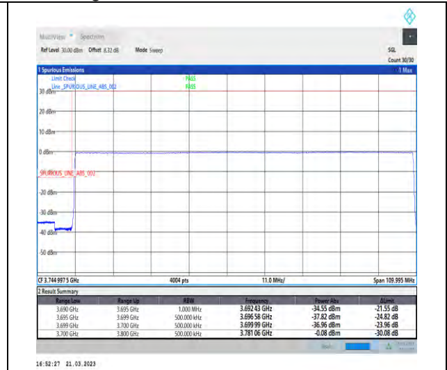
1-N77-3700-3980-30-100-L-6-CP-QPSK-Outer_Fu II-273@0-Ant1-1--PASS-see graph
