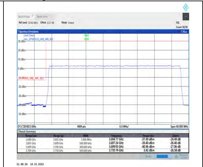
1-N77-3700-3980-30-50-L-3-DFT-PI2BPSK-Outer _Full-128@0-Ant1-1--PASS-see graph
