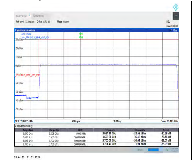
1-N77-3700-3980-30-60-L-6-CP-QPSK-Outer_Full -162@0-Ant1-1--PASS-see graph
