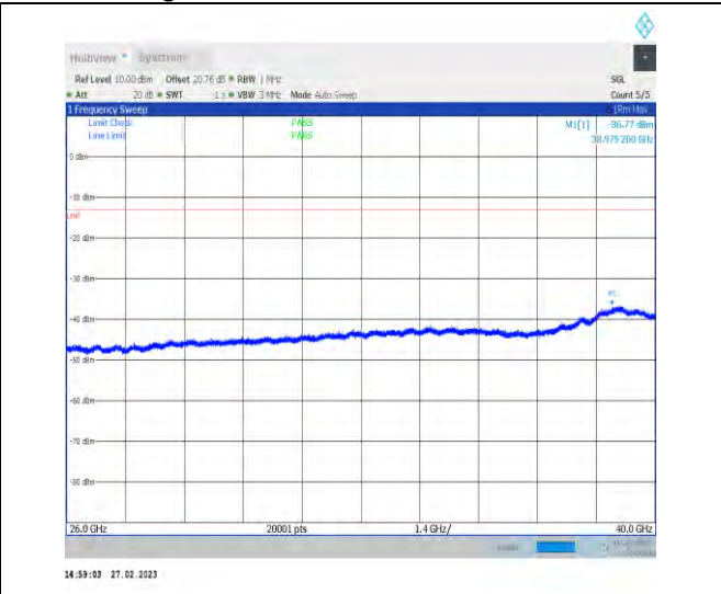
1-N77-3700-3980-30-100-M-1-DFT-QPSK-Edge_1R B_Left-1@0-26000-40000-Ant1-26000.00--45.07--13 -PASS
