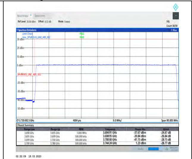
1-N77-3700-3980-30-80-L-3-DFT-PI2BPSK-Outer_Full-216@0-Ant1-1--PASS-see graph
