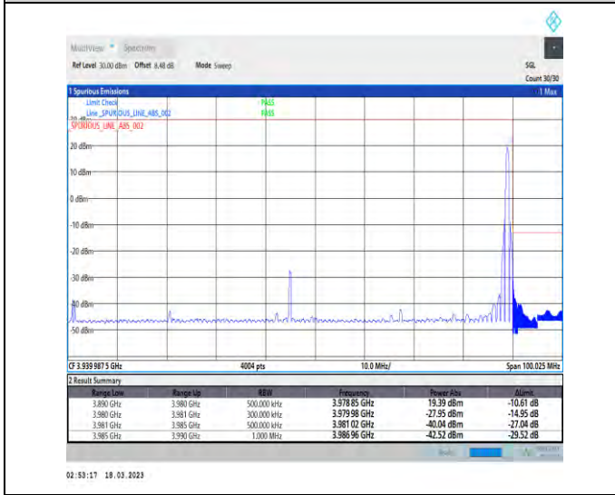
1-N77-3700-3980-30-90-H-5-CP-QPSK-Edge_1RB_Right-1@244-Ant1-1--PASS-see graph
