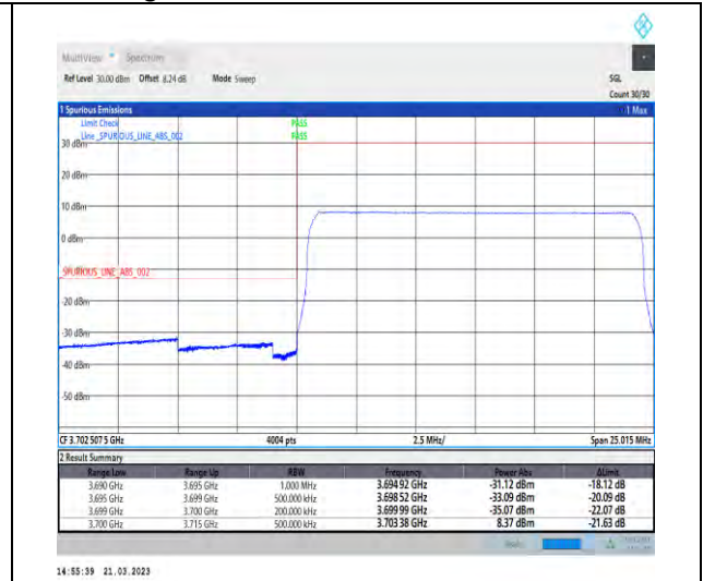
1-N77-3700-3980-30-15-L-6-CP-QPSK-Outer_Full -38@0-Ant1-1--PASS-see graph
