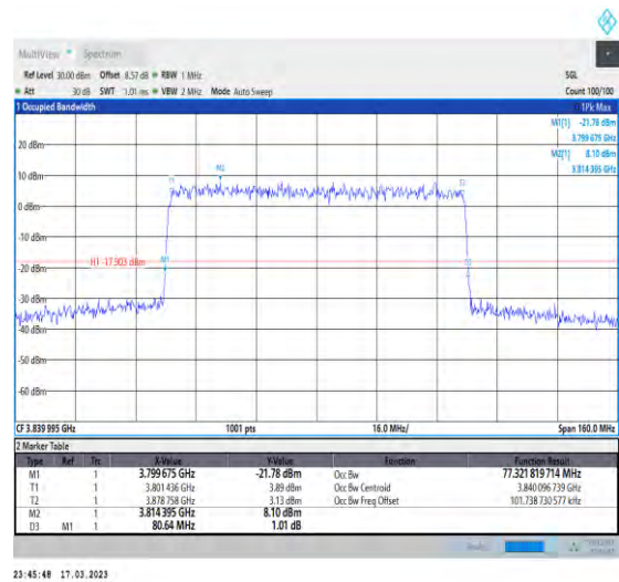
1-N77-3700-3980-30-80-M-9-CP-256QAM-Outer_Fu ll-217@0-Ant1-77.322-80.640-≤80-PASS
