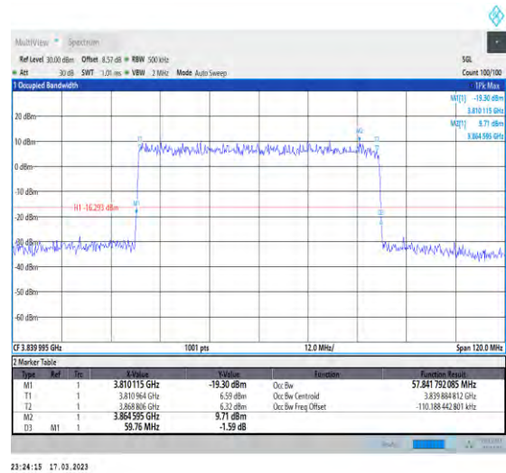
1-N77-3700-3980-30-60-M-3-DFT-16QAM-Outer_Full -162@0-Ant1-57.842-59.760-≤60-PASS
