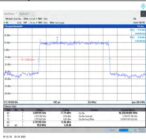
1-N77-3700-3980-30-100-L-2-DFT-PI2BPSK-Outer_Full-270@0-Ant1-96.259-99.800-≤100-PASS
