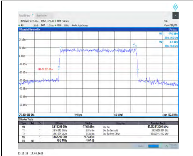
1-N77-3700-3980-30-50-M-7-CP-16QAM-Outer_Full-133@0-Ant1-47.292-49.300-≤50-PASS
