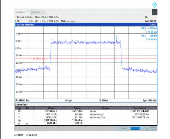
1-N77-3700-3980-30-80-M-1-DFT-QPSK-Outer_Full-216@0-Ant1-77.202-80.160-≤80-PASS
