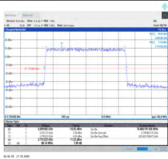
1-N77-3700-3980-30-80-L-4-DFT-64QAM-Outer_Full -216@0-Ant1-76.86-80.160-≤80-PASS
