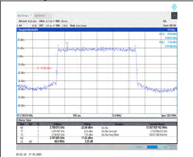
1-N77-3700-3980-30-60-L-2-DFT-PI2BPSK-Outer_Full-162@0-Ant1-57.858-60.000-≤60-PASS
