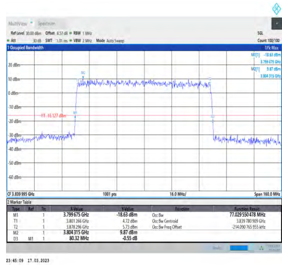
1-N77-3700-3980-30-80-M-5-DFT-256QAM-Outer_Full-216@0-Ant1-77.03-80.320-≤80-PASS
