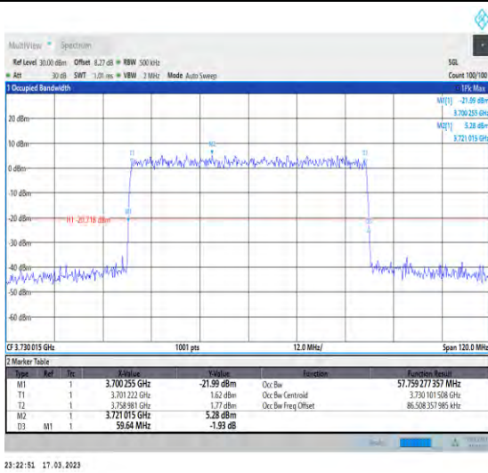
1-N77-3700-3980-30-60-L-9-CP-256QAM-Outer_Full -162@0-Ant1-57.759-59.640-≤60-PASS
