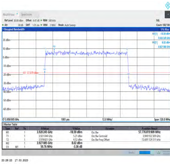
1-N77-3700-3980-30-60-H-5-DFT-256QAM-Outer_Full-162@0-Ant1-57.777-59.760-≤60-PASS
