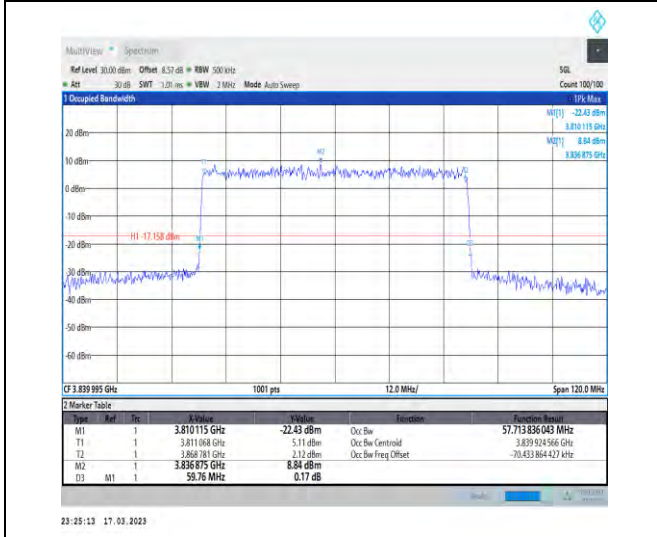
1-N77-3700-3980-30-60-M-6-CP-QPSK-Outer_Full-162@0-Ant1-57.714-59.760-≤60-PASS
