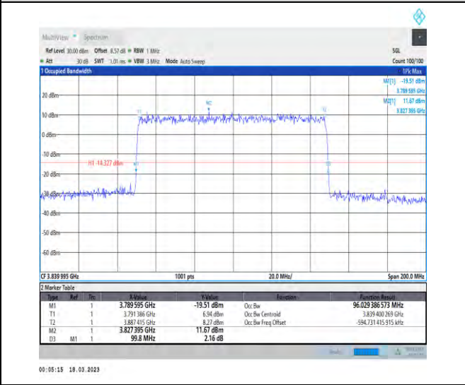
1-N77-3700-3980-30-100-M-3-DFT-16QAM-Outer_F ull-270@0-Ant1-96.029-99.800-≤100-PASS
