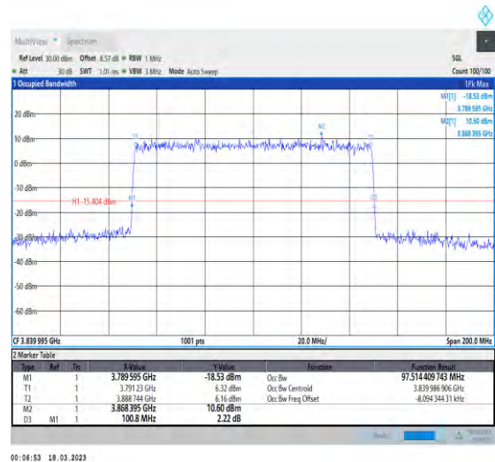
1-N77-3700-3980-30-100-M-7-CP-16QAM-Outer_Full-273@0-Ant1-97.514-100.800-≤100-PASS
