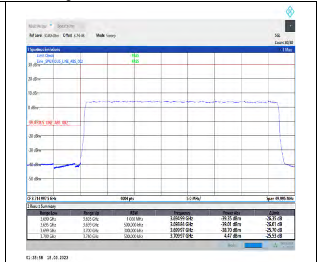
1-N77-3700-3980-30-40-L-3-DFT-PI2BPSK-Outer _Full-100@0-Ant1-1--PASS-see graph
