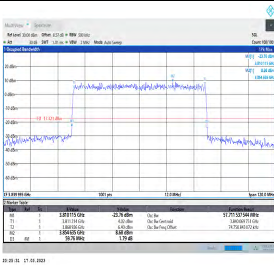
1-N77-3700-3980-30-60-M-8-CP-64QAM-Outer_Full-162@0-Ant1-57.712-59.760-≤60-PASS
