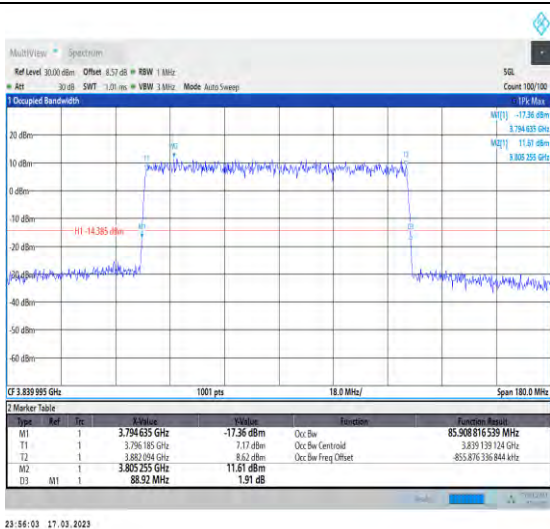
1-N77-3700-3980-30-90-M-3-DFT-16QAM-Outer_Full-240@0-Ant1-85.909-88.920-≤90-PASS
