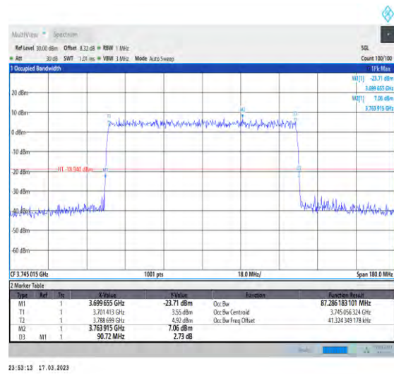
1-N77-3700-3980-30-90-L-9-CP-256QAM-Outer_Full-245@0-Ant1-87.286-90.720-<math>\leq 90</math>-PASS
