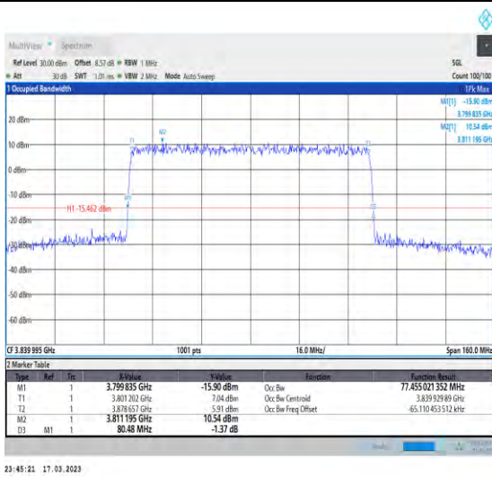
1-N77-3700-3980-30-80-M-6-CP-QPSK-Outer_Full-2 17@0-Ant1-77.455-80.480-≤80-PASS
