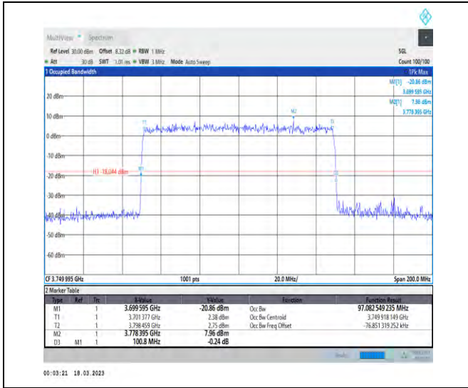
1-N77-3700-3980-30-100-L-9-CP-256QAM-Outer_F ull-273@0-Ant1-97.083-100.800-≤100-PASS
