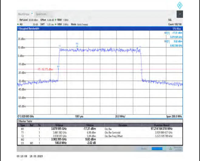
1-N77-3700-3980-30-100-H-6-CP-QPSK-Outer_Full-273@0-Ant1-97.214-100.800-≤100-PASS
