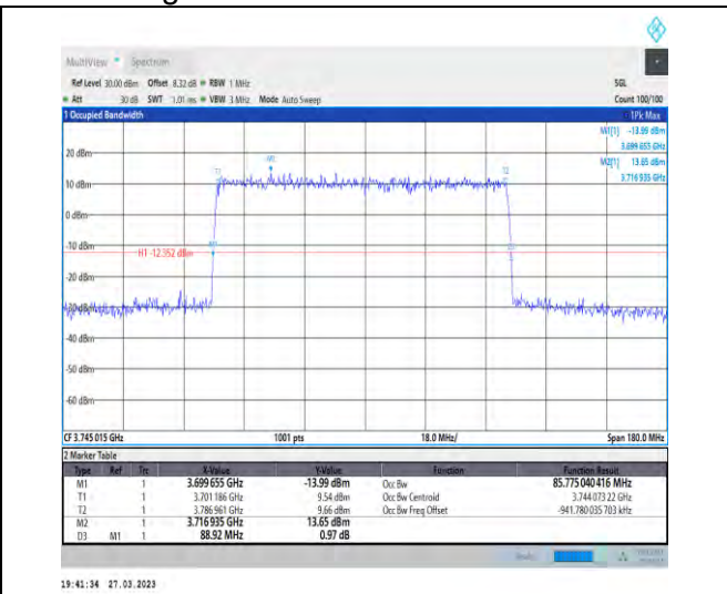
1-N77-3700-3980-30-90-L-1-DFT-QPSK-Outer_Full-240@0-Ant1-85.775-88.920-≤90-PASS
