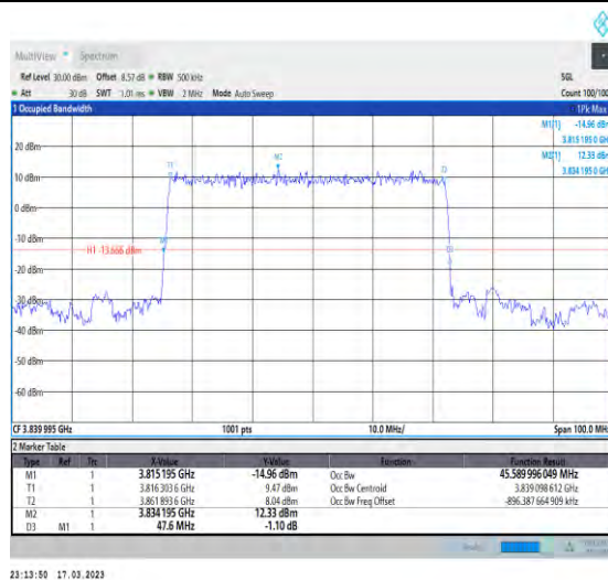
1-N77-3700-3980-30-50-M-2-DFT-PI2BPSK-Outer_Full-128@0-Ant1-45.59-47.600-<math>\leq 50</math>-PASS
