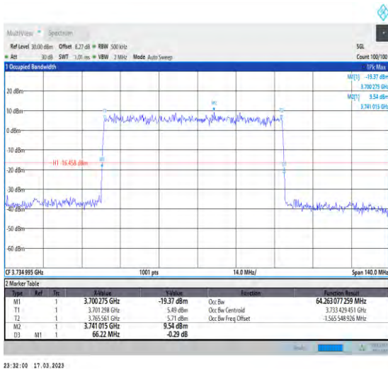
1-N77-3700-3980-30-70-L-4-DFT-64QAM-Outer_Full-180@0-Ant1-64.263-66.220-≤70-PASS
