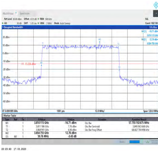
1-N77-3700-3980-30-60-M-2-DFT-PI2BPSK-Outer_Full -162@0-Ant1-57.755-59.760-≤60-PASS
