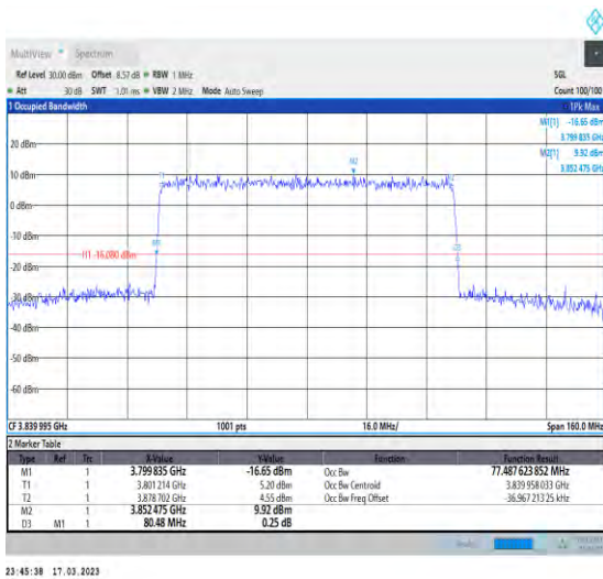
1-N77-3700-3980-30-80-M-8-CP-64QAM-Outer_Full- 217@0-Ant1-77.488-80.480-≤80-PASS
