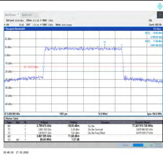
1-N77-3700-3980-30-80-M-7-CP-16QAM-Outer_Full -217@0-Ant1-77.368-80.640-≤80-PASS
