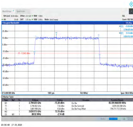
1-N77-3700-3980-30-90-M-1-DFT-QPSK-Outer_Full-240@0-Ant1-85.596-88.920-<math>\leq 90</math>-PASS
