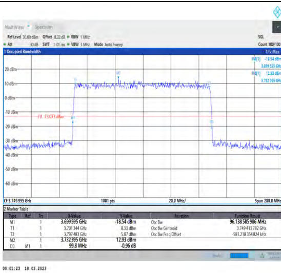
1-N77-3700-3980-30-100-L-1-DFT-QPSK-Outer_Full -270@0-Ant1-96.139-99.800-≤100-PASS
