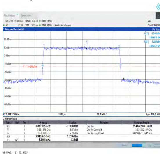
1-N77-3700-3980-30-90-H-3-DFT-16QAM-Outer_Full-240@0-Ant1-85.488-88.920-≤90-PASS
