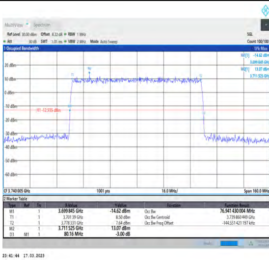
1-N77-3700-3980-30-80-L-3-DFT-16QAM-Outer_Full -216@0-Ant1-76.941-80.160-≤80-PASS
