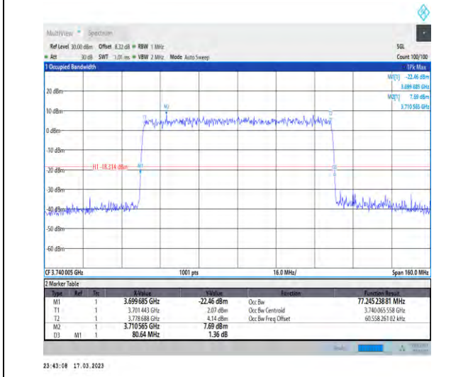
1-N77-3700-3980-30-80-L-9-CP-256QAM-Outer_Full-217@0-Ant1-77.245-80.640-≤80-PASS
