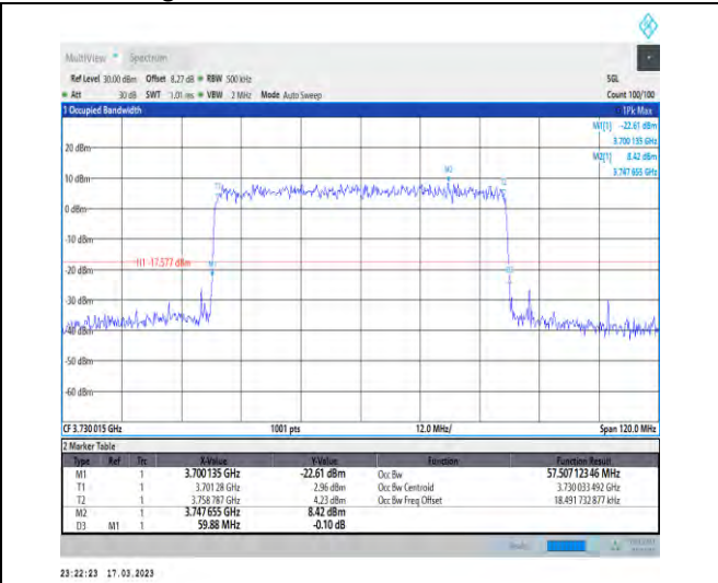
1-N77-3700-3980-30-60-L-6-CP-QPSK-Outer_Full-1 62@0-Ant1-57.507-59.880-≤60-PASS
