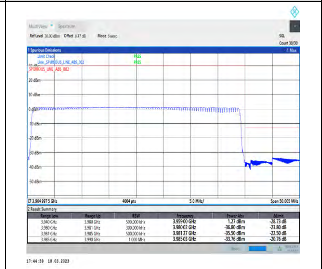
1-N77-3700-3980-30-40-H-6-CP-QPSK-Outer_Full-106@0-Ant1-1--PASS-see graph
