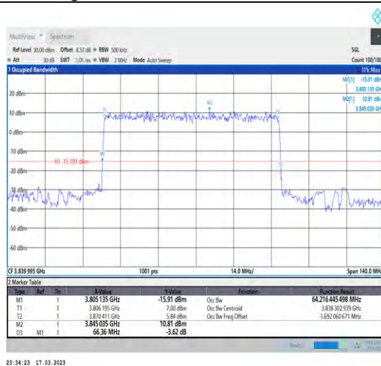
1-N77-3700-3980-30-70-M-2-DFT-PI2BPSK-Outer_Full-180@0-Ant1-64.216-66.360-≤70-PASS
