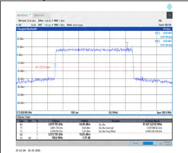
1-N77-3700-3980-30-100-H-8-CP-64QAM-Outer_Ful I-273@0-Ant1-97.421-100.600-≤100-PASS
