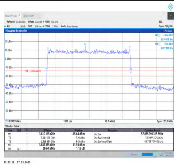
1-N77-3700-3980-30-60-M-1-DFT-QPSK-Outer_Full -162@0-Ant1-57.886-59.640-≤60-PASS
