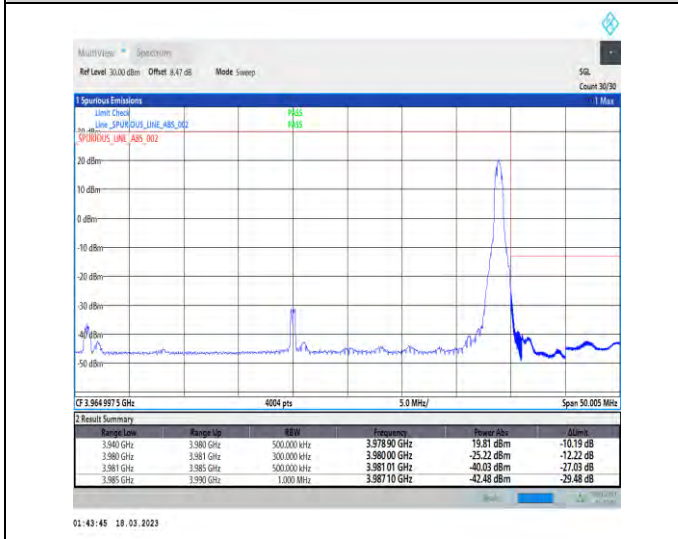
1-N77-3700-3980-30-40-H-5-CP-QPSK-Edge_1RB_Right-1@105-Ant1-1--PASS-see graph
