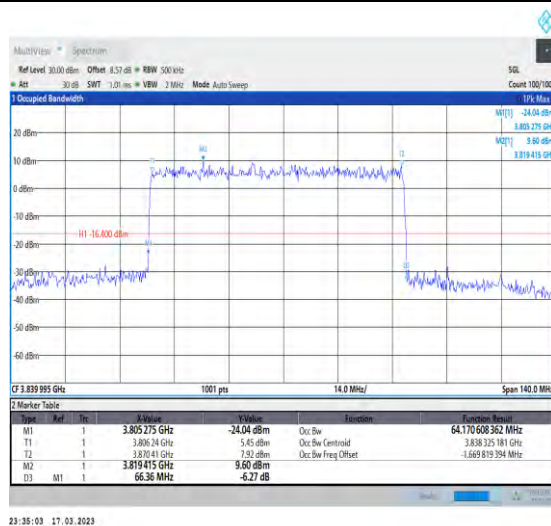
1-N77-3700-3980-30-70-M-4-DFT-64QAM-Outer_Full-180@0-Ant1-64.171-66.360-≤70-PASS
