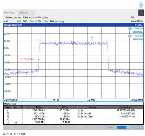
1-N77-3700-3980-30-60-H-4-DFT-64QAM-Outer_Ful I-162@0-Ant1-57.702-59.760-≤60-PASS
