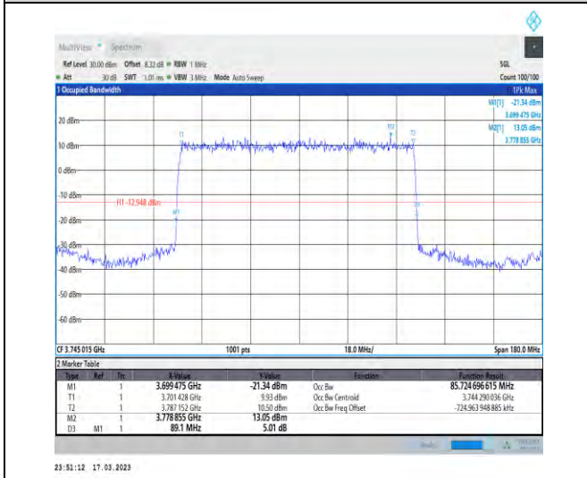
1-N77-3700-3980-30-90-L-2-DFT-PI2BPSK-Outer_Full-240@0-Ant1-85.725-89.100-≤90-PASS
