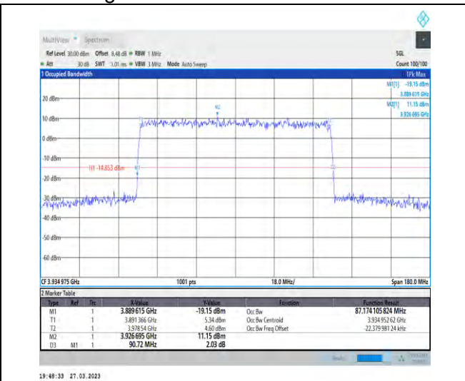
1-N77-3700-3980-30-90-H-7-CP-16QAM-Outer_Full-245@0-Ant1-87.174-90.720-≤90-PASS
