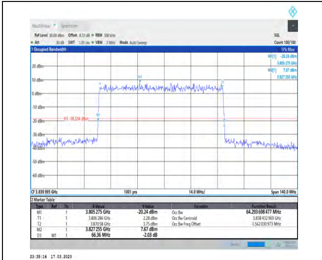
1-N77-3700-3980-30-70-M-5-DFT-256QAM-Outer_Full-180@0-Ant1-64.294-66.360-≤70-PASS
