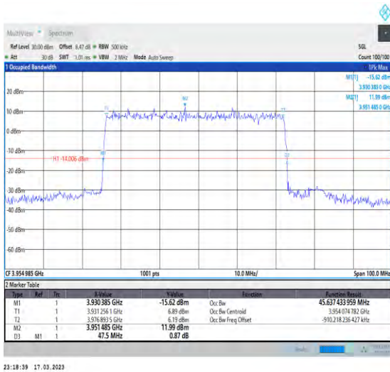
1-N77-3700-3980-30-50-H-4-DFT-64QAM-Outer_Full-128@0-Ant1-45.637-47.500-≤50-PASS
