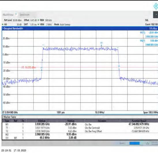
1-N77-3700-3980-30-50-H-6-CP-QPSK-Outer_Full-1 33@0-Ant1-47.547-49.300-≤50-PASS
