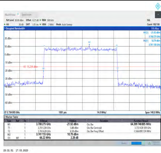
1-N77-3700-3980-30-70-L-3-DFT-16QAM-Outer_Full-180@0-Ant1-64.4-66.220-≤70-PASS
