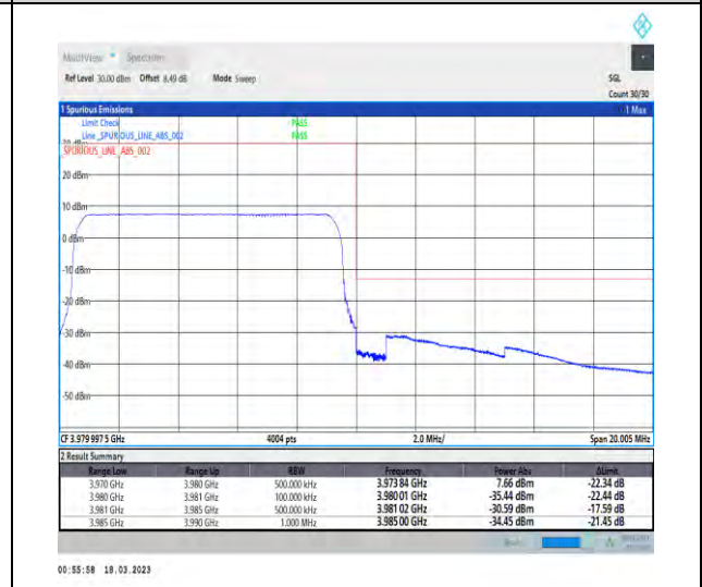
1-N77-3700-3980-30-10-H-6-CP-QPSK-Outer_Full-24@0-Ant1-1--PASS-see graph
