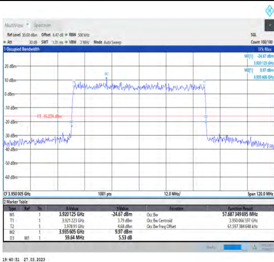
1-N77-3700-3980-30-60-H-9-CP-256QAM-Outer_Ful-162@0-Ant1-57.687-59.640-≤60-PASS
