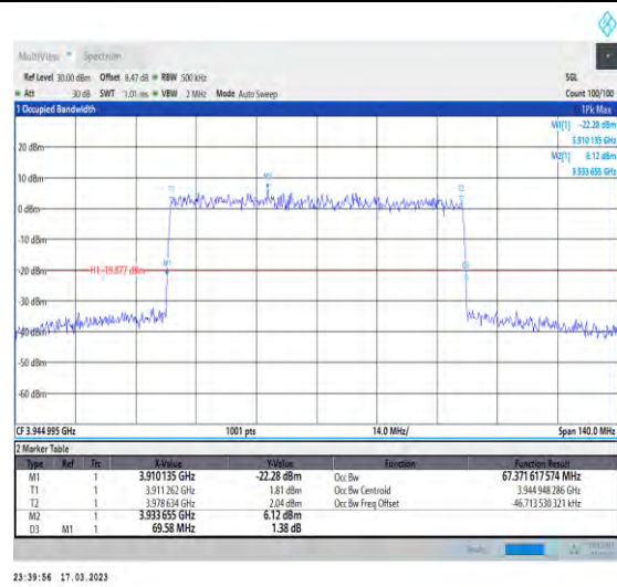
1-N77-3700-3980-30-70-H-9-CP-256QAM-Outer_Ful I-189@0-Ant1-67.372-69.580-≤70-PASS
