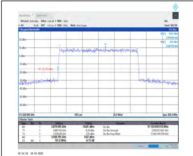
1-N77-3700-3980-30-100-H-7-CP-16QAM-Outer_Ful I-273@0-Ant1-97.193-101.000-≤100-PASS
