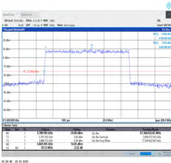
1-N77-3700-3980-30-100-M-6-CP-QPSK-Outer_Full-273@0-Ant1-97.361-101.000-≤100-PASS
