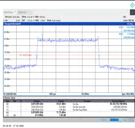
1-N77-3700-3980-30-50-M-4-DFT-64QAM-Outer_Full-128@0-Ant1-45.763-47.400-≤50-PASS
