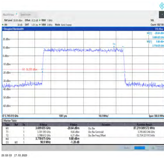
1-N77-3700-3980-30-90-L-8-CP-64QAM-Outer_Full-245@0-Ant1-87.219-90.900-<math>\leq 90</math>-PASS
