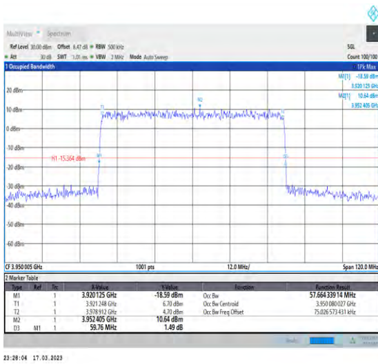
1-N77-3700-3980-30-60-H-3-DFT-16QAM-Outer_Ful I-162@0-Ant1-57.664-59.760-≤60-PASS
