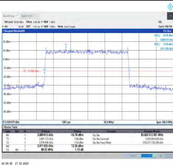
1-N77-3700-3980-30-90-H-4-DFT-64QAM-Outer_Full-240@0-Ant1-85.864-88.920-≤90-PASS
