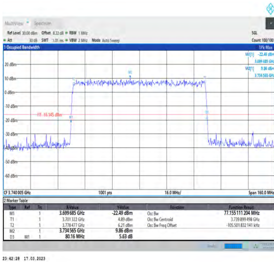
1-N77-3700-3980-30-80-L-5-DFT-256QAM-Outer_Fu ll-216@0-Ant1-77.155-80.160-≤80-PASS
