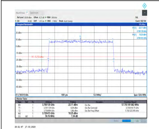
1-N77-3700-3980-30-60-L-3-DFT-16QAM-Outer_Full-162@0-Ant1-57.755-59.760-≤60-PASS
