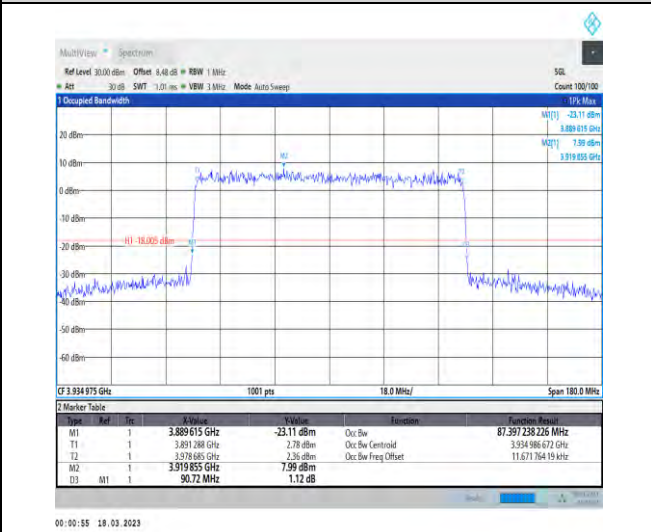
1-N77-3700-3980-30-90-H-9-CP-256QAM-Outer_Full-245@0-Ant1-87.397-90.720-≤90-PASS
