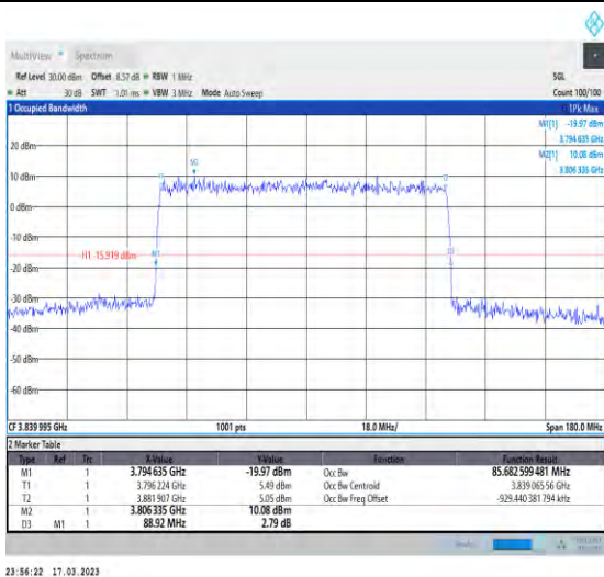
1-N77-3700-3980-30-90-M-5-DFT-256QAM-Outer_Full-240@0-Ant1-85.683-88.920-≤90-PASS
