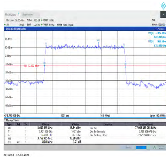
1-N77-3700-3980-30-80-L-2-DFT-PI2BPSK-Outer_Full-216@0-Ant1-77.003-80.000-≤80-PASS
