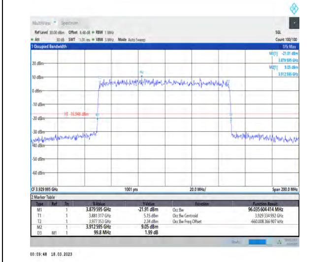
1-N77-3700-3980-30-100-H-5-DFT-256QAM-Outer_Full-270@0-Ant1-96.036-99.800-≤100-PASS
