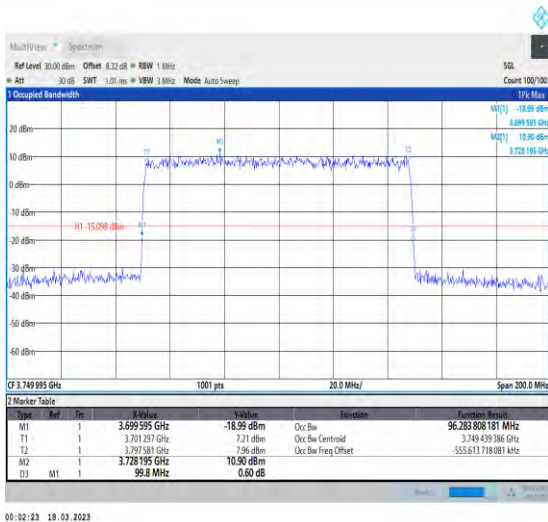
1-N77-3700-3980-30-100-L-3-DFT-16QAM-Outer_Fu ll-270@0-Ant1-96.284-99.800-≤100-PASS
