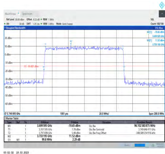
1-N77-3700-3980-30-100-L-4-DFT-64QAM-Outer_F ull-270@0-Ant1-96.103-99.800-≤100-PASS
