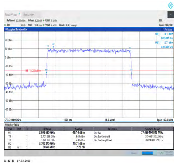
1-N77-3700-3980-30-80-L-6-CP-QPSK-Outer_Full-2 17@0-Ant1-77.489-80.480-≤80-PASS
