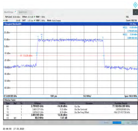
1-N77-3700-3980-30-80-M-3-DFT-16QAM-Outer_Full-216@0-Ant1-77.184-80.000-≤80-PASS
