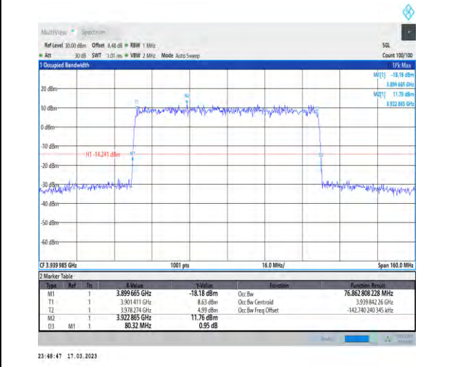
1-N77-3700-3980-30-80-H-4-DFT-64QAM-Outer_Full-216@0-Ant1-76.863-80.320-≤80-PASS
