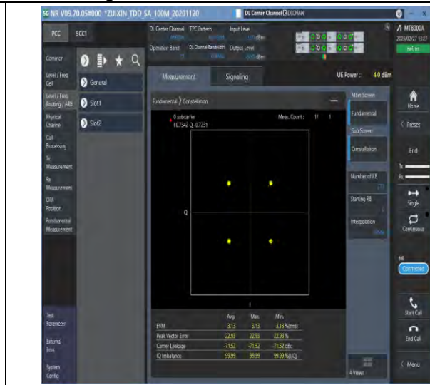
1-N77-3700-3980-30-100-M-6-CP-QPSK-Outer_Full-273@0-Ant1-see graph-PASS
