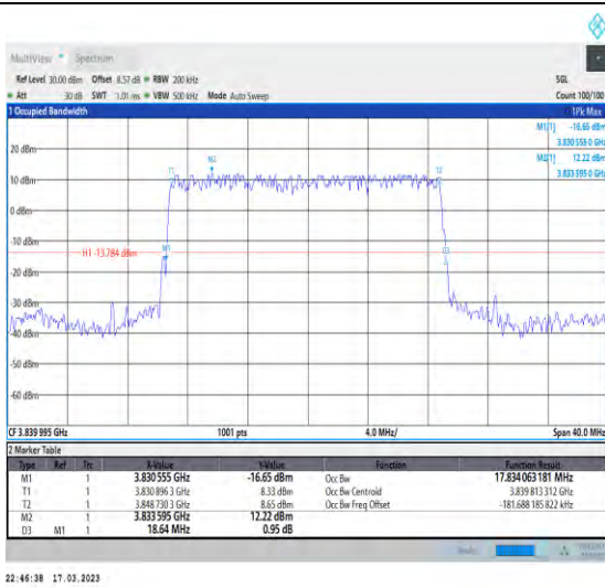
1-N77-3700-3980-30-20-M-2-DFT-PI2BPSK-Outer_Full-50@0-Ant1-17.834-18.640-≤20-PASS
