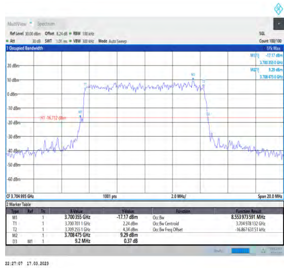
1-N77-3700-3980-30-10-L-8-CP-64QAM-Outer_Full-24@0-Ant1-8.554-9.200-≤10-PASS
