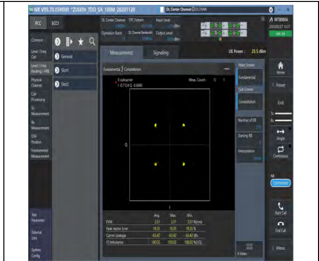
1-N77-3700-3980-30-100-M-2-DFT-QPSK-Outer_Full-270@0-Ant1-see graph-PASS
