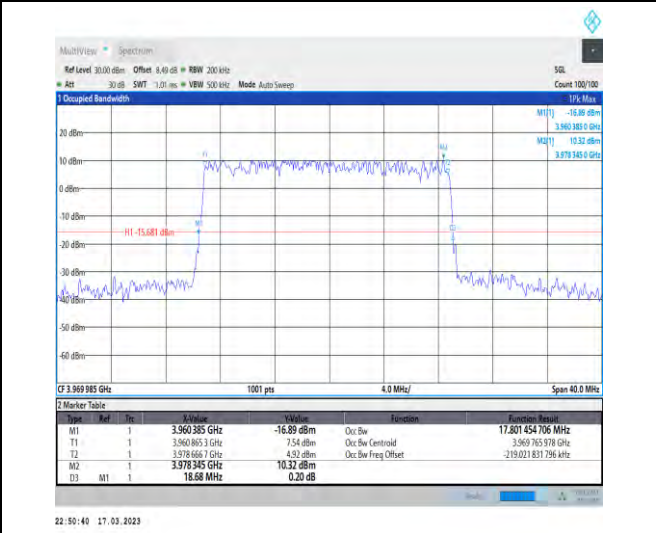
1-N77-3700-3980-30-20-H-4-DFT-64QAM-Outer_Full-50@0-Ant1-17.801-18.680-≤20-PASS
