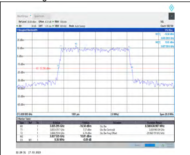
1-N77-3700-3980-30-10-M-1-DFT-QPSK-Outer_Full -24@0-Ant1-8.589-9.360-≤10-PASS
