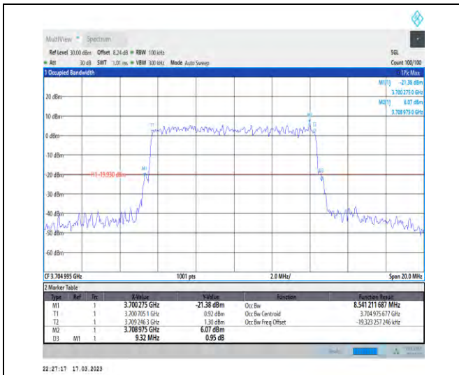
1-N77-3700-3980-30-10-L-9-CP-256QAM-Outer_Full -24@0-Ant1-8.541-9.320-≤10-PASS
