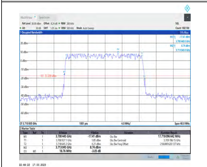
1-N77-3700-3980-30-20-L-5-DFT-256QAM-Outer_Fu II-50@0-Ant1-17.718-18.760-≤20-PASS
