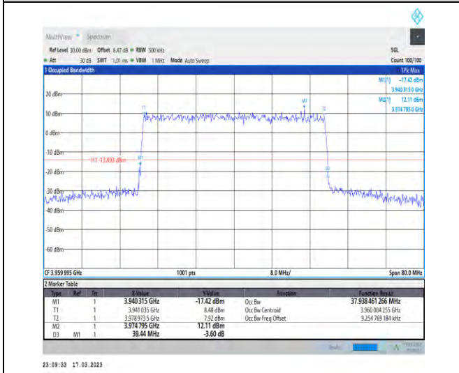
1-N77-3700-3980-30-40-H-7-CP-16QAM-Outer_Full-106@0-Ant1-37.938-39.440-≤40-PASS
