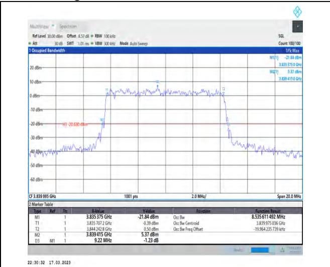
1-N77-3700-3980-30-10-M-9-CP-256QAM-Outer_Fu II-24@0-Ant1-8.536-9.220-≤10-PASS
