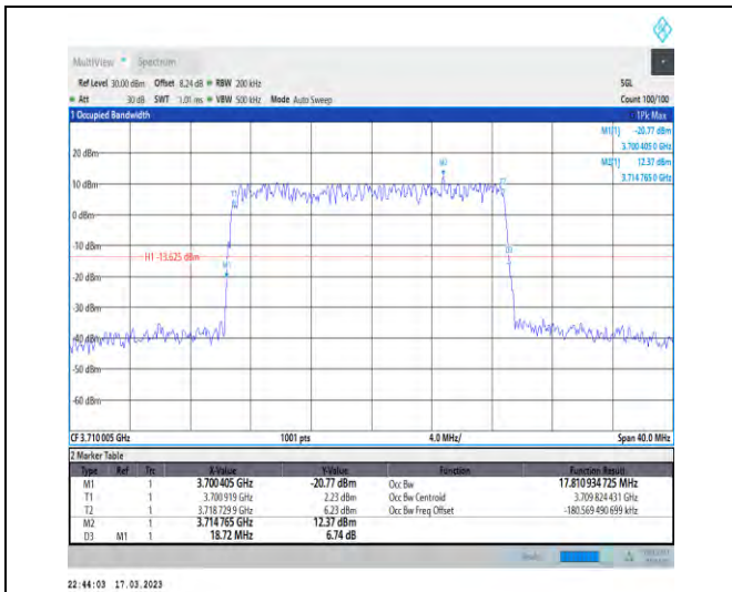
1-N77-3700-3980-30-20-L-3-DFT-16QAM-Outer_Full -50@0-Ant1-17.811-18.720-≤20-PASS
