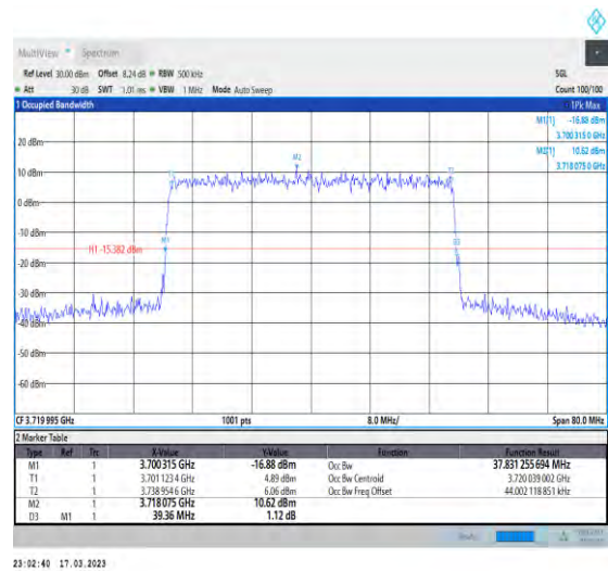
1-N77-3700-3980-30-40-L-6-CP-QPSK-Outer_Full-1 06@0-Ant1-37.831-39.360-≤40-PASS
