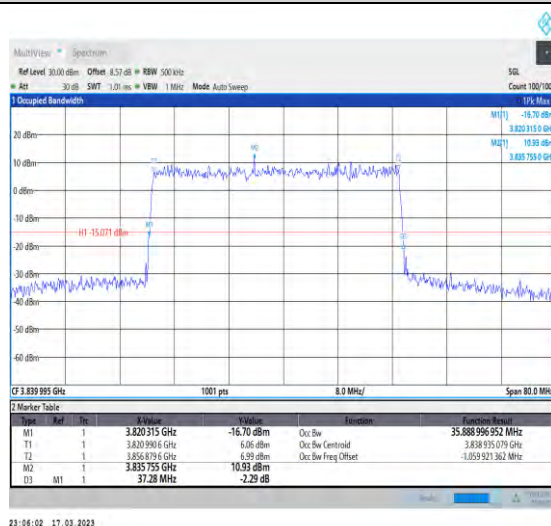
1-N77-3700-3980-30-40-M-5-DFT-256QAM-Outer_Full-100@0-Ant1-35.889-37.280-≤40-PASS
