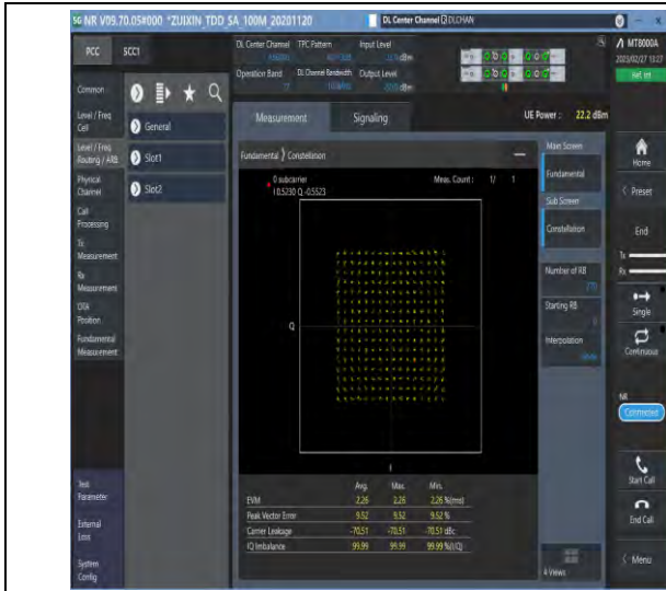
1-N77-3700-3980-30-100-M-5-DFT-256QAM-Outer_Full-270@0-Ant1-see graph-PASS
