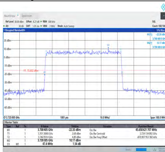
1-N77-3700-3980-30-50-L-5-DFT-256QAM-Outer_Full-128@0-Ant1-45.651-47.400-≤50-PASS
