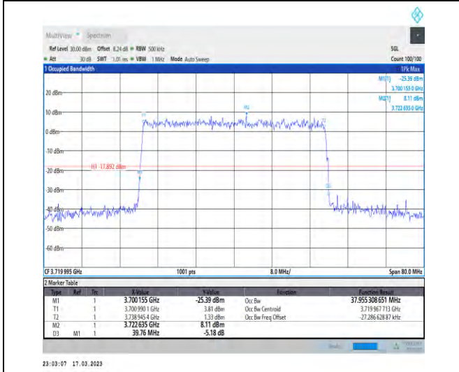
1-N77-3700-3980-30-40-L-9-CP-256QAM-Outer_Full-106@0-Ant1-37.955-39.760-≤40-PASS
