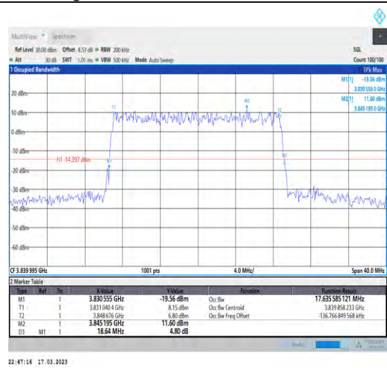
1-N77-3700-3980-30-20-M-3-DFT-16QAM-Outer_Full-50@0-Ant1-17.636-18.640-≤20-PASS
