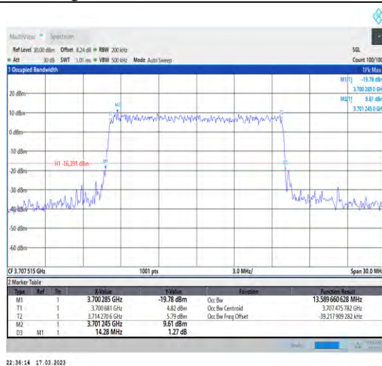
1-N77-3700-3980-30-15-L-7-CP-16QAM-Outer_Full-38@0-Ant1-13.59-14.280-≤15-PASS
