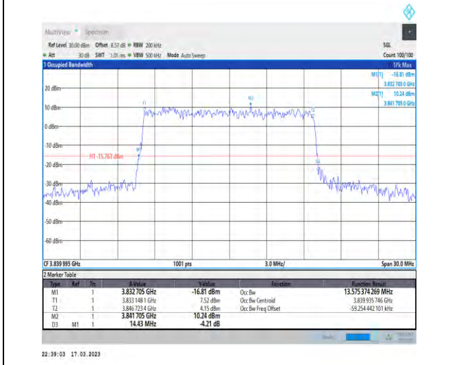
1-N77-3700-3980-30-15-M-7-CP-16QAM-Outer_Full-38@0-Ant1-13.575-14.430-≤15-PASS
