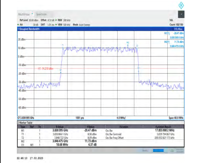
1-N77-3700-3980-30-20-M-1-DFT-QPSK-Outer_Full-50@0-Ant1-17.856-18.680-≤20-PASS
