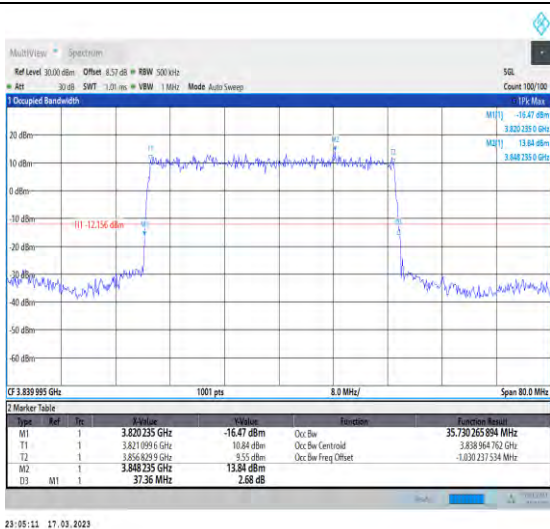
1-N77-3700-3980-30-40-M-2-DFT-PI2BPSK-Outer_Full-100@0-Ant1-35.73-37.360-≤40-PASS
