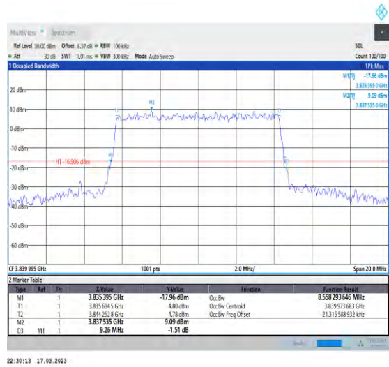
1-N77-3700-3980-30-10-M-7-CP-16QAM-Outer_Full-24@0-Ant1-8.558-9.260-≤10-PASS
