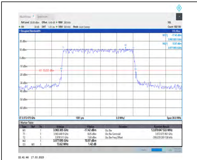
1-N77-3700-3980-30-15-H-4-DFT-64QAM-Outer_Full-36@0-Ant1-12.87-13.620-≤15-PASS
