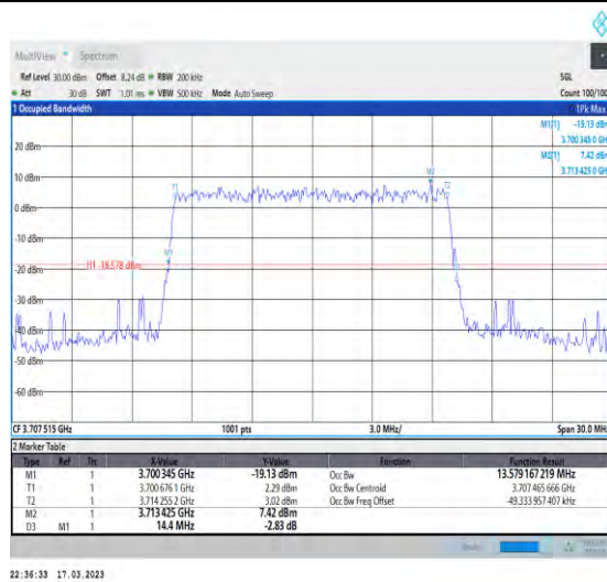
1-N77-3700-3980-30-15-L-9-CP-256QAM-Outer_Full-38@0-Ant1-13.579-14.400-≤15-PASS
