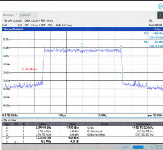
1-N77-3700-3980-30-50-L-4-DFT-64QAM-Outer_Full -128@0-Ant1-45.643-47.400-≤50-PASS
