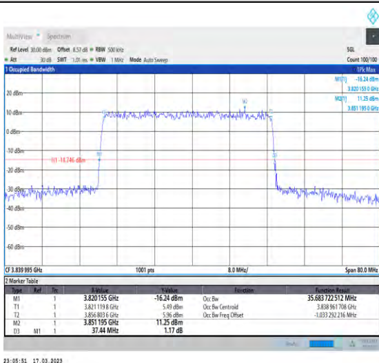
1-N77-3700-3980-30-40-M-4-DFT-64QAM-Outer_Full-100@0-Ant1-35.684-37.440-≤40-PASS
