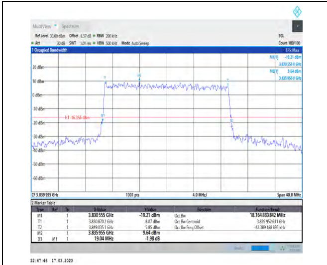
1-N77-3700-3980-30-20-M-6-CP-QPSK-Outer_Full-5 1@0-Ant1-18.165-19.040-≤20-PASS
