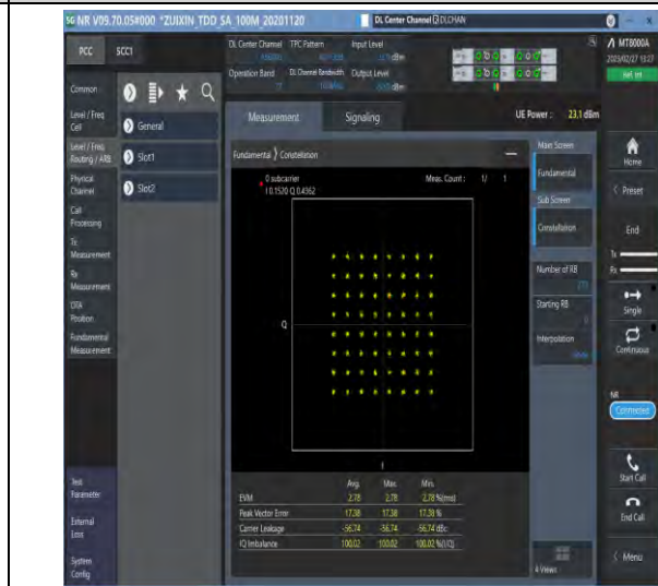
1-N77-3700-3980-30-100-M-8-CP-64QAM-Outer_Full-273@0-Ant1-see graph-PASS
