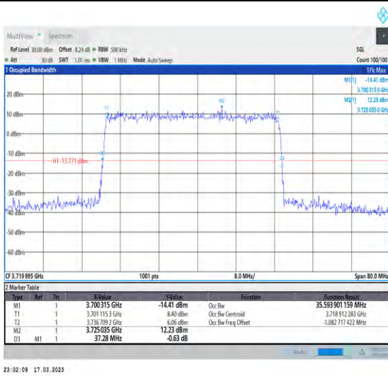
1-N77-3700-3980-30-40-L-3-DFT-16QAM-Outer_Full -100@0-Ant1-35.594-37.280-≤40-PASS
