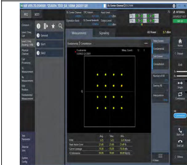
1-N77-3700-3980-30-100-M-7-CP-16QAM-Outer_Full-273@0-Ant1-see graph-PASS
