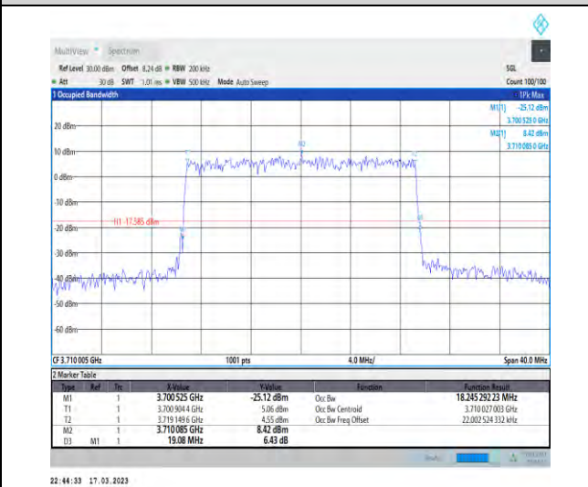
1-N77-3700-3980-30-20-L-6-CP-QPSK-Outer_Full-5 1@0-Ant1-18.245-19.080-≤20-PASS
