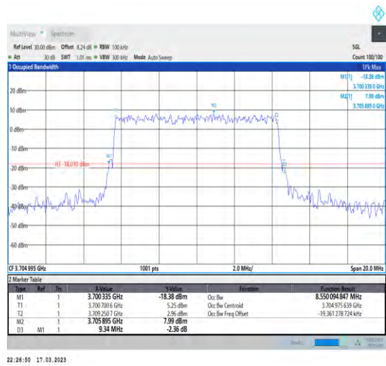
1-N77-3700-3980-30-10-L-6-CP-QPSK-Outer_Full-2 4@0-Ant1-8.55-9.340-≤10-PASS
