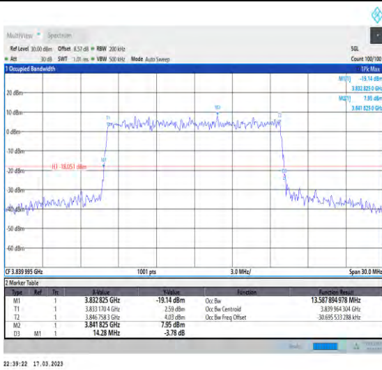
1-N77-3700-3980-30-15-M-9-CP-256QAM-Outer_Ful I-38@0-Ant1-13.588-14.280-≤15-PASS
