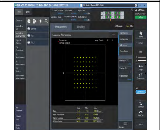
1-N77-3700-3980-30-100-M-4-DFT-64QAM-Outer_Full-270@0-Ant1-see graph-PASS
