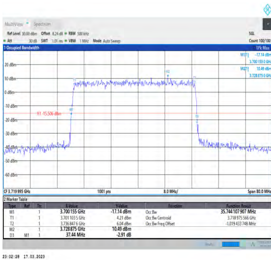
1-N77-3700-3980-30-40-L-5-DFT-256QAM-Outer_Fu II-100@0-Ant1-35.744-37.440-≤40-PASS
