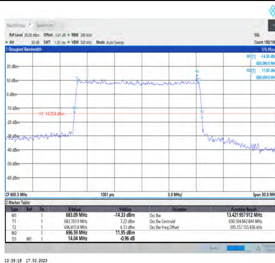
1-N71-PC3-15-15-H-5-DFT-256QAM-Outer_Full-75 @0-Ant1-13.422-14.040-≤15-PASS
