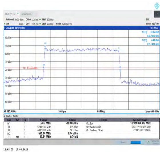
1-N71-PC3-15-20-M-9-CP-256QAM-Outer_Full-106 @0-Ant1-18.925-19.640-≤20-PASS
