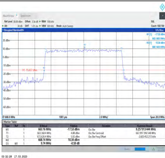
1-N71-PC3-15-10-L-6-CP-QPSK-Outer_Full-52@0-A Ant1-9.258-9.740-≤10-PASS
