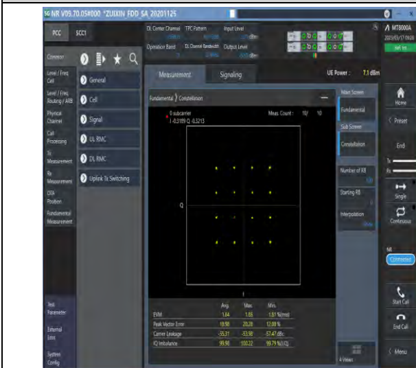
1-N71-PC3-15-20-M-3-DFT-16QAM-Outer_Full-100 @0-Ant1-see graph-PASS
