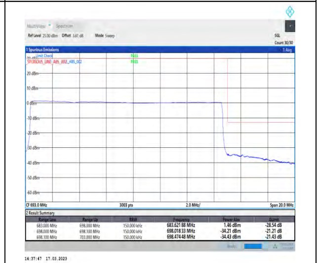
1-N71-PC3-15-15-H-6-CP-QPSK-Outer_Full-79@0-Ant1-1--PASS-see graph
