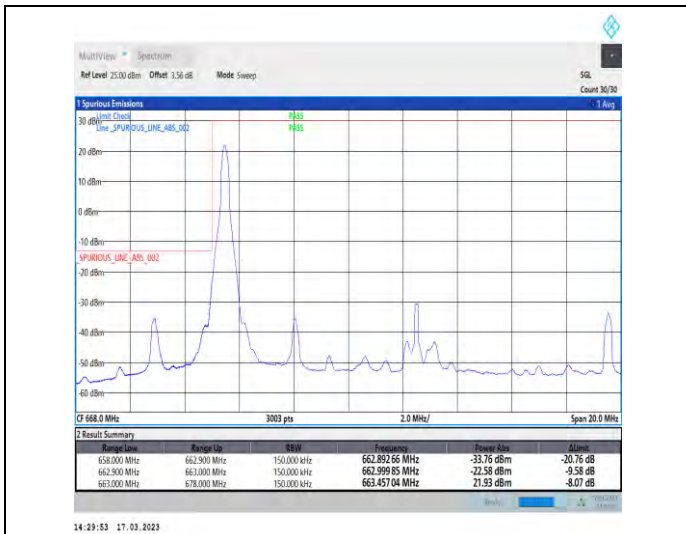
1-N71-PC3-15-15-L-1-DFT-PI2BPSK-Edge_1RB_Left-1@0-Ant1-1--PASS-see graph
