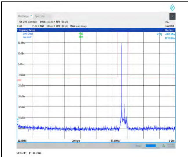
1-N71-PC3-15-20-M-1-DFT-PI2BPSK-Inner_1RB_L eft-1@1-30-1000-Ant1-35.34--55.02--13-PASS
