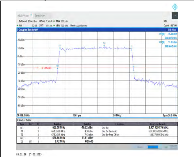
1-N71-PC3-15-10-L-3-DFT-16QAM-Outer_Full-50 @0-Ant1-8.902-9.420-≤10-PASS
