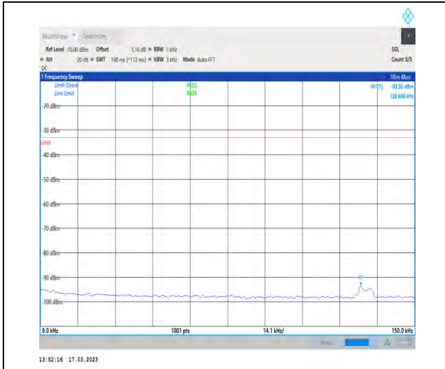
1-N71-PC3-15-20-H-1-DFT-PI2BPSK-Inner_1RB_L eft-1@1-0.009-0.15-Ant1-0.13--93.55--33-PASS
