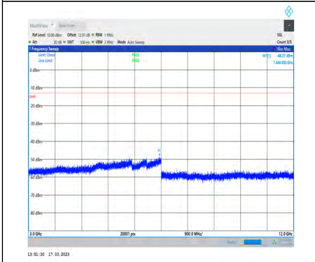
1-N71-PC3-15-20-M-1-DFT-PI2BPSK-Inner_1RB_L eft-1@1-3000-12000-Ant1-7446.45--48.37--13-PASS
