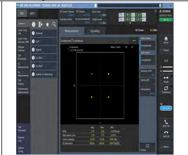
1-N71-PC3-15-20-M-6-CP-QPSK-Outer_Full-106 @0-Ant1-see graph-PASS
