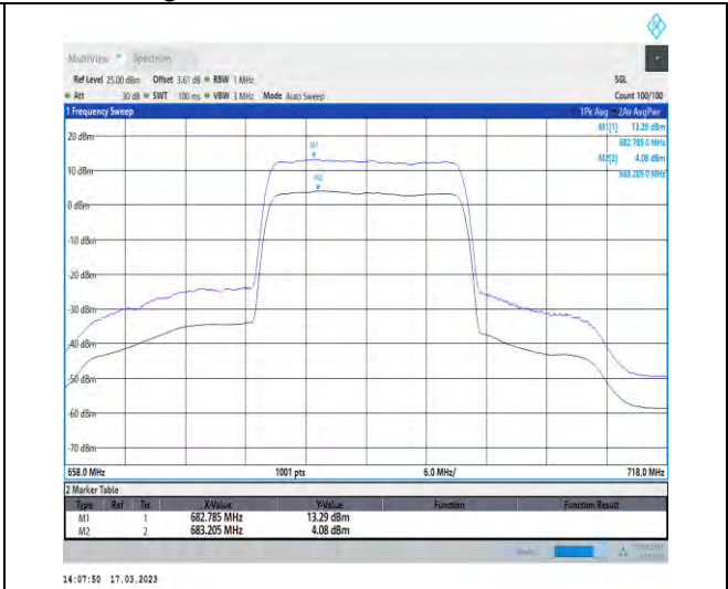
1-N71-PC3-15-20-H-2-CP-256QAM-Outer_Full-106 @0-Ant1-9.21-100%-0.00-9.21-PASS-≤13
