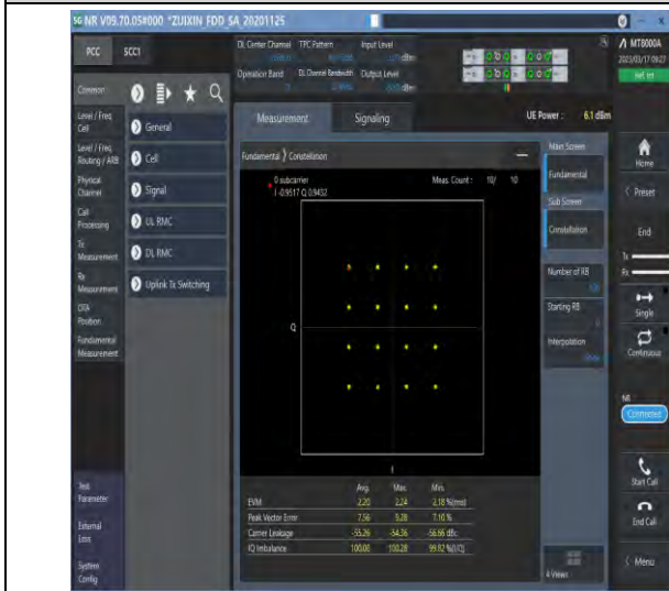
1-N71-PC3-15-20-M-7-CP-16QAM-Outer_Full-106 @0-Ant1-see graph-PASS
