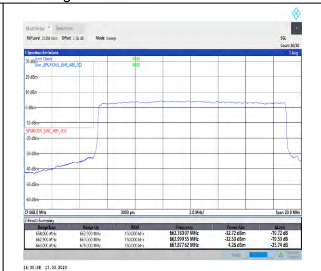
1-N71-PC3-15-15-L-3-DFT-PI2BPSK-Outer_Full-75@0-Ant1-1--PASS-see graph
