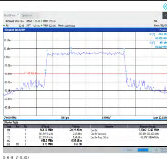
1-N71-PC3-15-10-L-9-CP-256QAM-Outer_Full-52@ 0-Ant1-9.27-9.760-≤10-PASS
