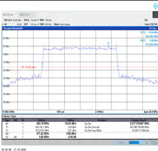
1-N71-PC3-15-10-L-8-CP-64QAM-Outer_Full-52@0- Ant1-9.277-9.660-≤10-PASS
