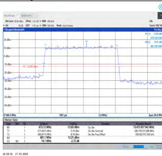
1-N71-PC3-15-15-M-8-CP-64QAM-Outer_Full-79@0 -Ant1-13.416-14.100-≤15-PASS
