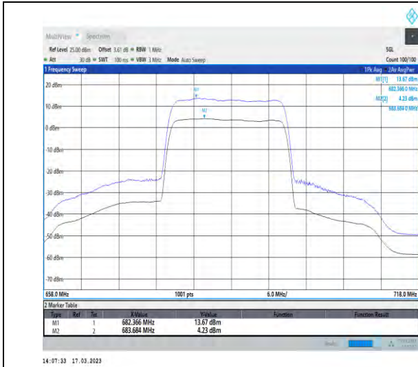
1-N71-PC3-15-20-H-1-DFT-256QAM-Outer_Full-100 @0-Ant1-9.44-100%-0.00-9.44-PASS-≤13
