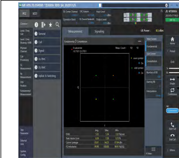
1-N71-PC3-15-20-M-1-DFT-PI2BPSK-Outer_Full-100 @0-Ant1-see graph-PASS
