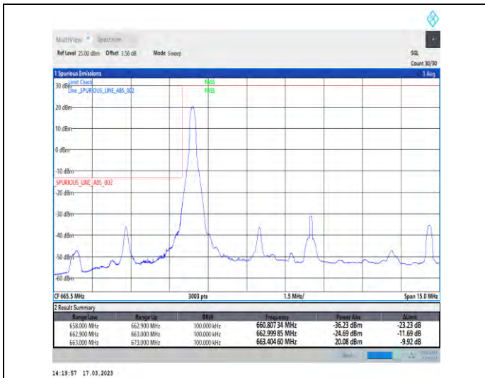
1-N71-PC3-15-10-L-1-DFT-PI2BPSK-Edge_1RB_Left-1@0-Ant1-1--PASS-see graph
