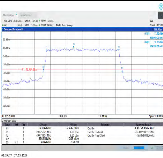
1-N71-PC3-15-5-H-7-CP-16QAM-Outer_Full-25@0-Ant1-4.467-4.860-≤5-PASS
