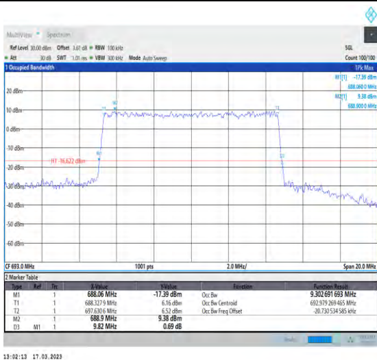
1-N71-PC3-15-10-H-6-CP-QPSK-Outer_Full-52@0- Ant1-9.303-9.820-≤10-PASS
