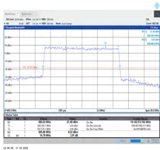
1-N71-PC3-15-15-H-9-CP-256QAM-Outer_Full-79@0-Ant1-14.142-14.790-≤15-PASS
