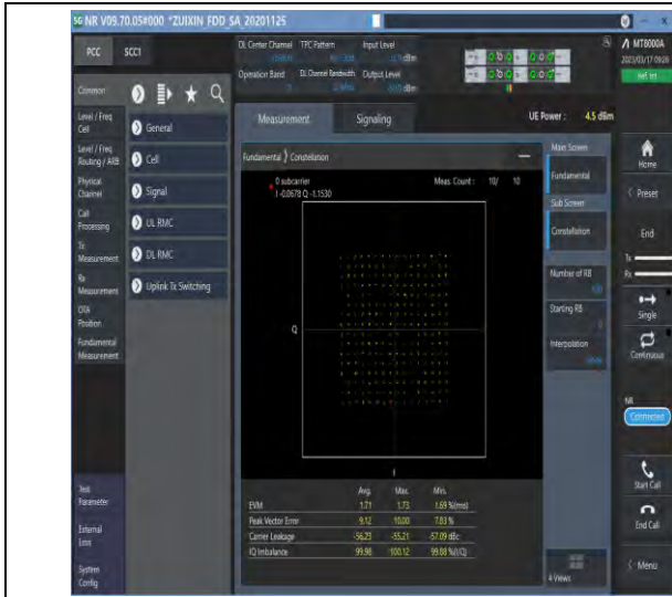
1-N71-PC3-15-20-M-5-DFT-256QAM-Outer_Full-100 @0-Ant1-see graph-PASS
