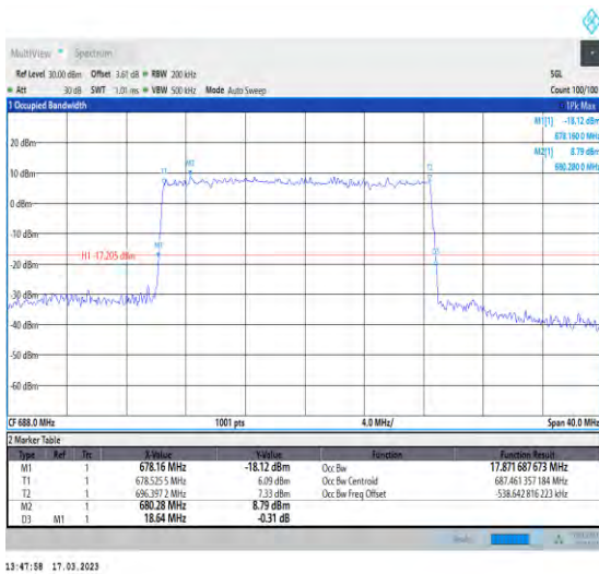
1-N71-PC3-15-20-H-5-DFT-256QAM-Outer_Full-100 @0-Ant1-17.872-18.640-≤20-PASS
