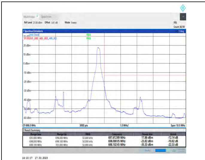
1-N71-PC3-15-5-H-2-DFT-PI2BPSK-Edge_1RB_Right-1@24-Ant1-1--PASS-see graph
