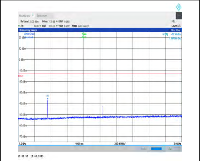
1-N71-PC3-15-20-H-1-DFT-PI2BPSK-Inner_1RB_Lef t-1@1-1000-3000-Ant1-1357.50--36.53--13-PASS
