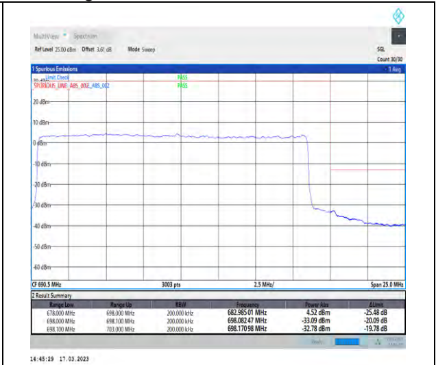
1-N71-PC3-15-20-H-3-DFT-PI2BPSK-Outer_Full-1 00@0-Ant1-1--PASS-see graph
