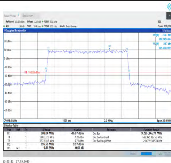
1-N71-PC3-15-10-H-7-CP-16QAM-Outer_Full-52@0- -Ant1-9.286-9.840-≤10-PASS
