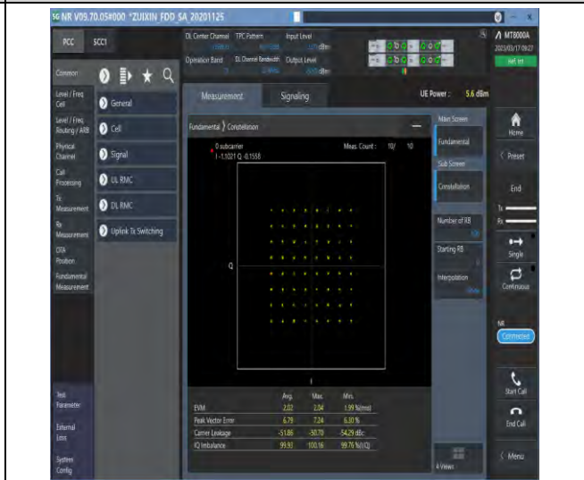
1-N71-PC3-15-20-M-8-CP-64QAM-Outer_Full-106 @0-Ant1-see graph-PASS
