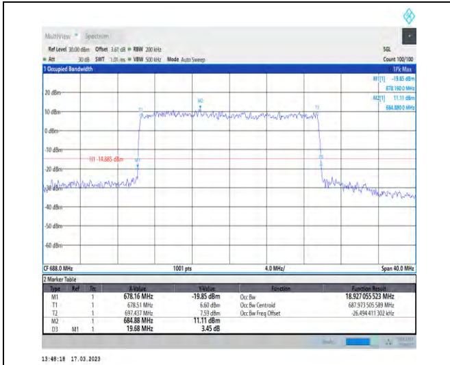
1-N71-PC3-15-20-H-7-CP-16QAM-Outer_Full-106@ 0-Ant1-18.927-19.680-≤20-PASS
