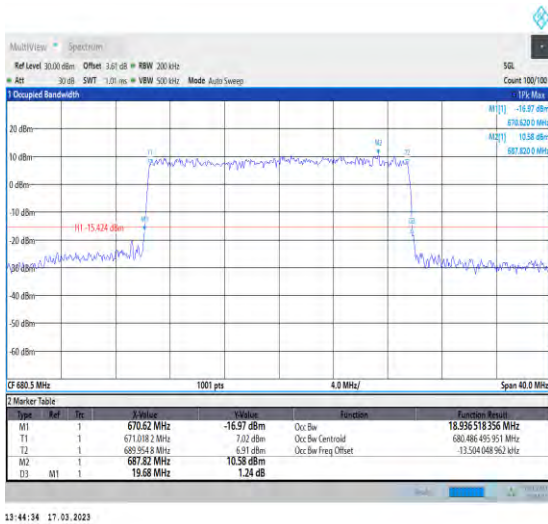
1-N71-PC3-15-20-M-6-CP-QPSK-Outer_Full-106@0-Ant1-18.937-19.680-<=20-PASS
