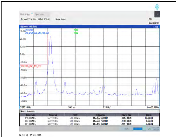
1-N71-PC3-15-20-L-1-DFT-PI2BPSK-Edge_1RB_Left-1@0-Ant1-1--PASS-see graph
