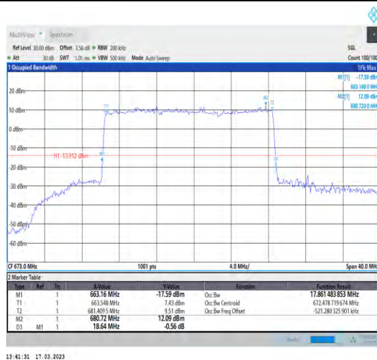
1-N71-PC3-15-20-L-4-DFT-64QAM-Outer_Full-100@0-Ant1-17.861-18.640-≤20-PASS
