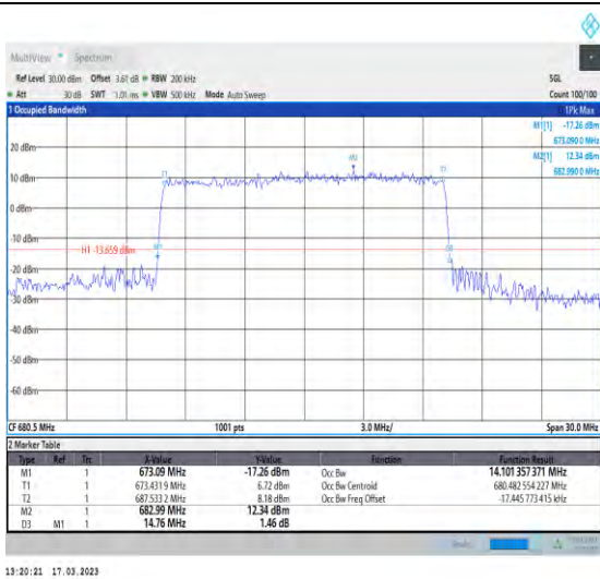
1-N71-PC3-15-15-M-7-CP-16QAM-Outer_Full-79@0 -Ant1-14.101-14.760-≤15-PASS
