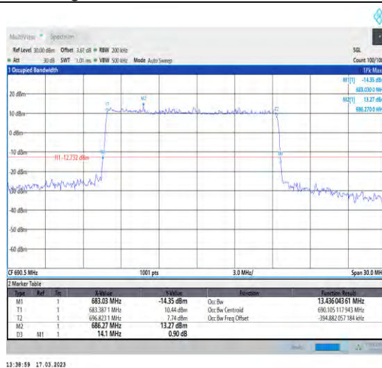
1-N71-PC3-15-15-H-3-DFT-16QAM-Outer_Full-75 @0-Ant1-13.436-14.100-≤15-PASS
