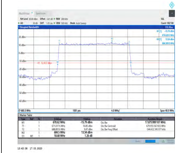
1-N71-PC3-15-20-M-2-DFT-PI2BPSK-Outer_Full-100 @0-Ant1-17.876-18.680-≤20-PASS
