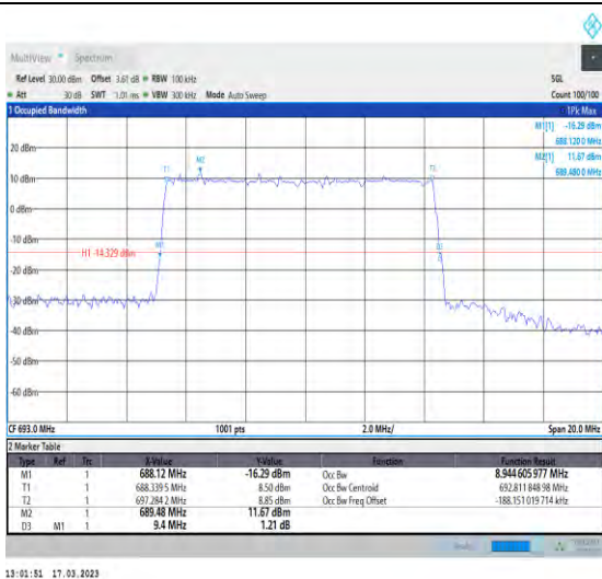
1-N71-PC3-15-10-H-4-DFT-64QAM-Outer_Full-50@ 0-Ant1-8.945-9.400-≤10-PASS
