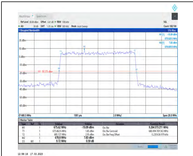
1-N71-PC3-15-10-M-9-CP-256QAM-Outer_Full-52@ 0-Ant1-9.264-9.720-≤10-PASS
