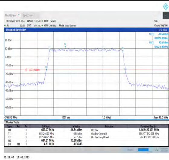
1-N71-PC3-15-5-H-4-DFT-64QAM-Outer_Full-25@0-Ant1-4.462-4.810-≤5-PASS
