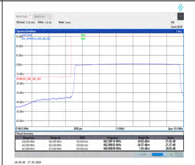
1-N71-PC3-15-10-L-6-CP-QPSK-Outer_Full-52@0-Ant1-1--PASS-see graph
