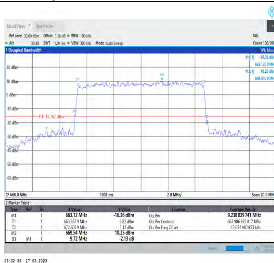
1-N71-PC3-15-10-L-7-CP-16QAM-Outer_Full-52@0- Ant1-9.238-9.720-≤10-PASS
