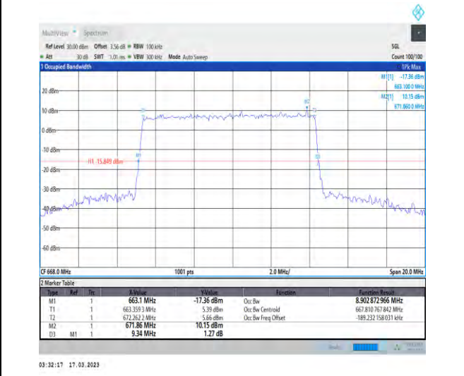
1-N71-PC3-15-10-L-5-DFT-256QAM-Outer_Full-50 @0-Ant1-8.903-9.340-≤10-PASS
