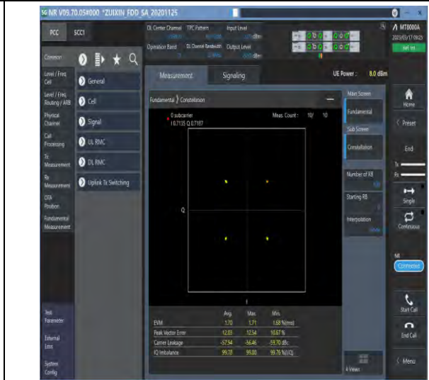
1-N71-PC3-15-20-M-2-DFT-QPSK-Outer_Full-100 @0-Ant1-see graph-PASS
