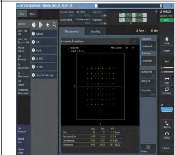
1-N71-PC3-15-20-M-4-DFT-64QAM-Outer_Full-100 @0-Ant1-see graph-PASS
