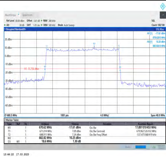
1-N71-PC3-15-20-M-5-DFT-256QAM-Outer_Full-100 @0-Ant1-17.897-18.600-<=20-PASS
