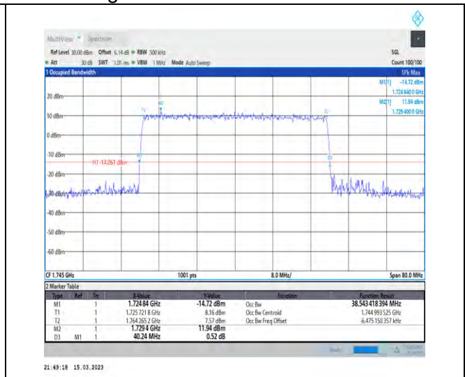
1-N66-PC3-15-40-M-7-CP-16QAM-Outer_Full-216@0 -Ant1-38.543-40.240-≤40-PASS
