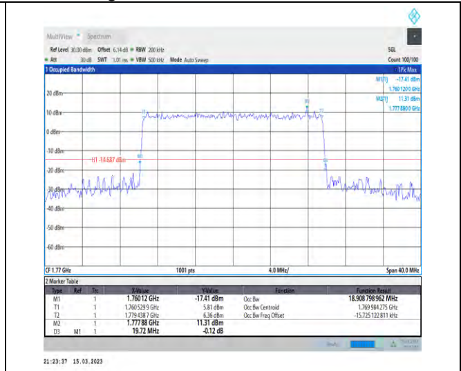
1-N66-PC3-15-20-H-7-CP-16QAM-Outer_Full-106@0 -Ant1-18.909-19.720-≤20-PASS
