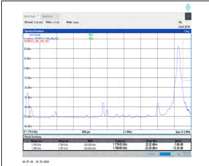
1-N66-PC3-15-20-H-2-DFT-PI2BPSK-Edge_1RB_Right-t-1@105-Ant1-1-seegraph-PASS-see graph
