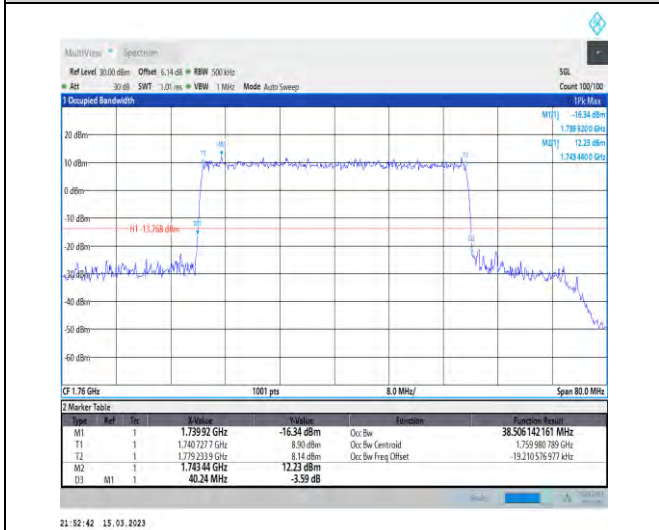
1-N66-PC3-15-40-H-7-CP-16QAM-Outer_Full-216@0-Ant1-38.506-40.240-≤40-PASS
