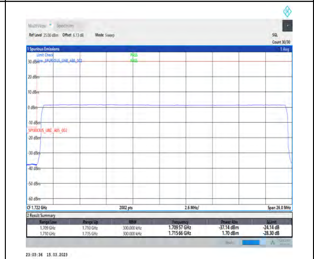
1-N66-PC3-15-25-L-6-CP-QPSK-Outer_Full-133@0-Ant1-1-seegraph-PASS-see graph
