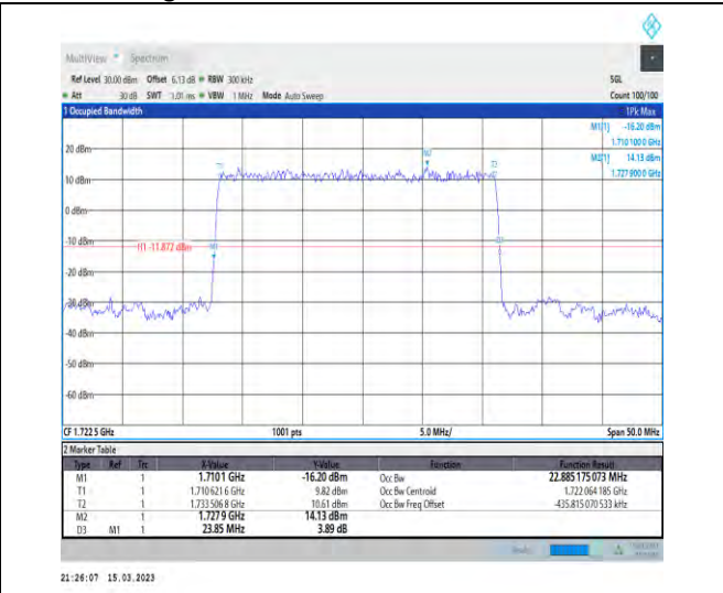
1-N66-PC3-15-25-L-2-DFT-PI2BPSK-Outer_Full-128 @0-Ant1-22.885-23.850-≤25-PASS
