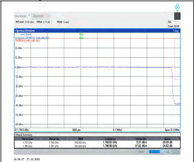
1-N66-PC3-15-30-H-3-DFT-PI2BPSK-Outer_Full-160@0-Ant1-1-seegraph-PASS-see graph
