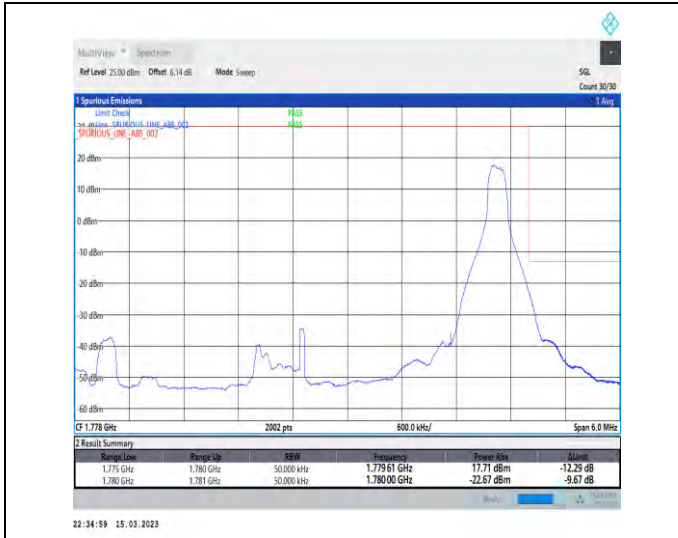
1-N66-PC3-15-5-H-2-DFT-PI2BPSK-Edge_1RB_Right-1@24-Ant1-1-seegraph-PASS-see graph
