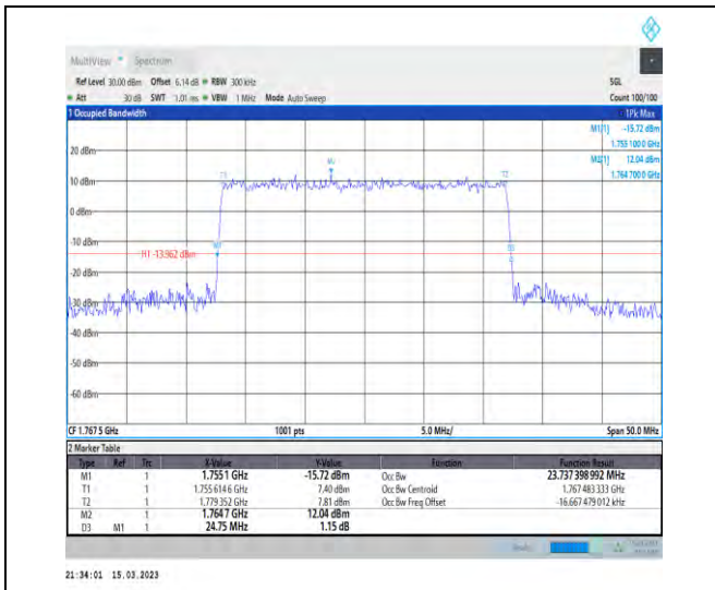
1-N66-PC3-15-25-H-7-CP-16QAM-Outer_Full-133@ 0-Ant1-23.737-24.750-≤25-PASS
