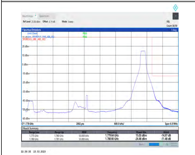
1-N66-PC3-15-5-H-5-CP-QPSK-Edge_1RB_Right-1@24-Ant1-1-seegraph-PASS-see graph
