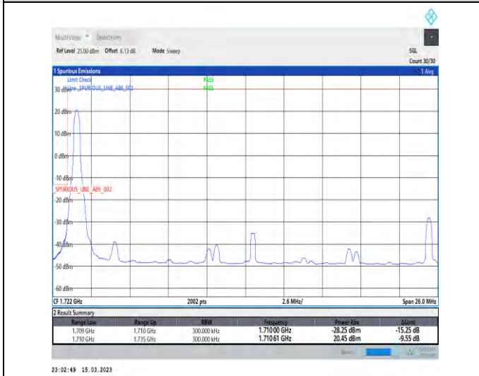
1-N66-PC3-15-25-L-4-CP-QPSK-Edge_1RB_Left-1@0-Ant1-1-seegraph-PASS-see graph
