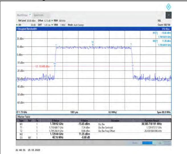
1-N66-PC3-15-40-L-8-CP-64QAM-Outer_Full-216@0-Ant1-38.586-40.160-≤40-PASS
