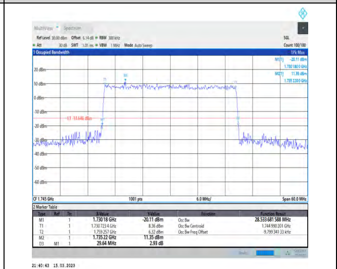
1-N66-PC3-15-30-M-8-CP-64QAM-Outer_Full-160@0-Ant1-28.534-29.640-≤30-PASS
