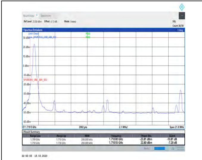
1-N66-PC3-15-20-L-1-DFT-PI2BPSK-Edge_1RB_Left-1@0-Ant1-1-seegraph-PASS-see graph
