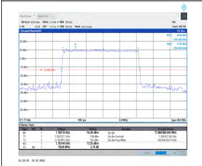
1-N66-PC3-15-20-H-4-DFT-64QAM-Outer_Full-100@0-Ant1-17.86-18.640-≤20-PASS
