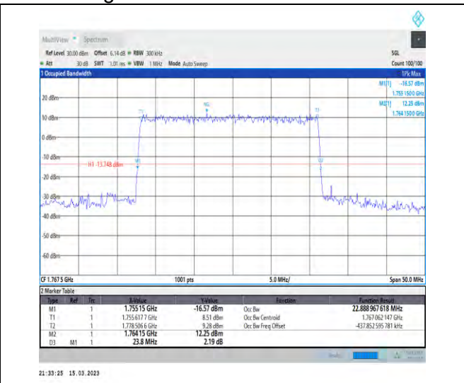
1-N66-PC3-15-25-H-4-DFT-64QAM-Outer_Full-128 @0-Ant1-22.889-23.800-≤25-PASS
