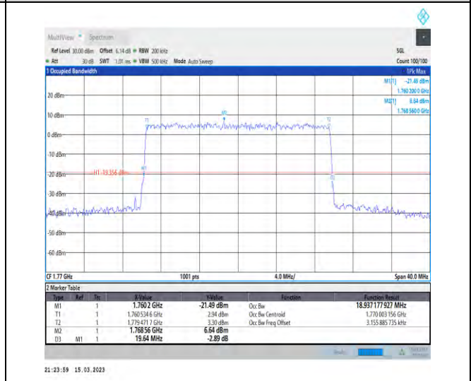
1-N66-PC3-15-20-H-9-CP-256QAM-Outer_Full-106@0 -Ant1-18.937-19.640-≤20-PASS
