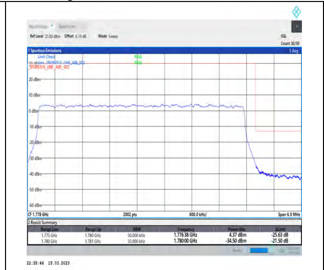
1-N66-PC3-15-5-H-3-DFT-PI2BPSK-Outer_Full-25@0-Ant1-1-seegraph-PASS-see graph
