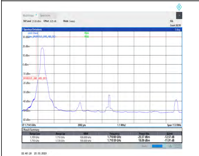
1-N66-PC3-15-10-L-4-CP-QPSK-Edge_1RB_Left-1@0-Ant1-1-seegraph-PASS-see graph
