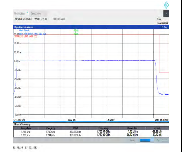
1-N66-PC3-15-15-H-6-CP-QPSK-Outer_Full-79@0-Ant1-1-seegraph-PASS-see graph
