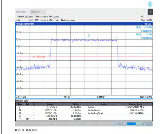
1-N66-PC3-15-25-M-6-CP-QPSK-Outer_Full-133@0 -Ant1-23.73-24.800-≤25-PASS
