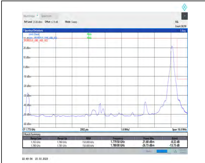
1-N66-PC3-15-15-H-2-DFT-PI2BPSK-Edge_1RB_Right-t@78-Ant1-1-seegraph-PASS-see graph
