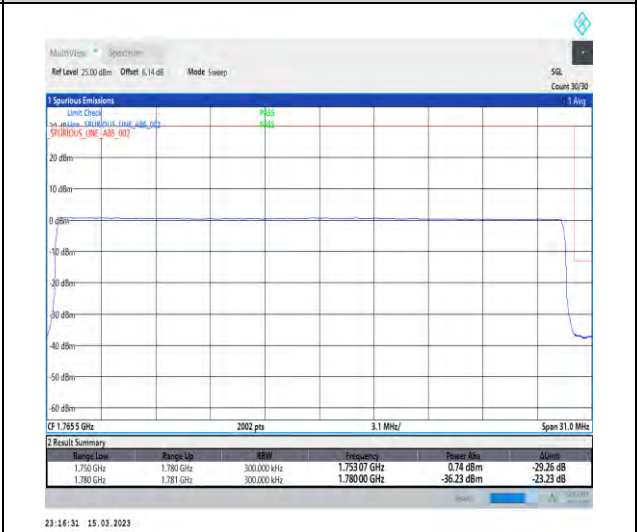
1-N66-PC3-15-30-H-6-CP-QPSK-Outer_Full-160@0-Ant1-1-seegraph-PASS-see graph
