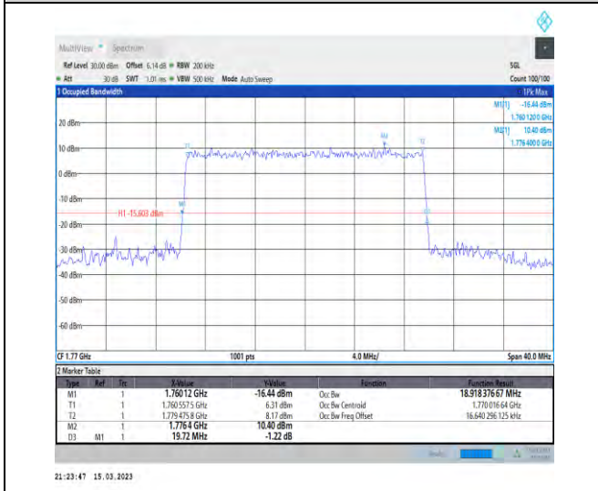
1-N66-PC3-15-20-H-8-CP-64QAM-Outer_Full-106@0 -Ant1-18.918-19.720-≤20-PASS
