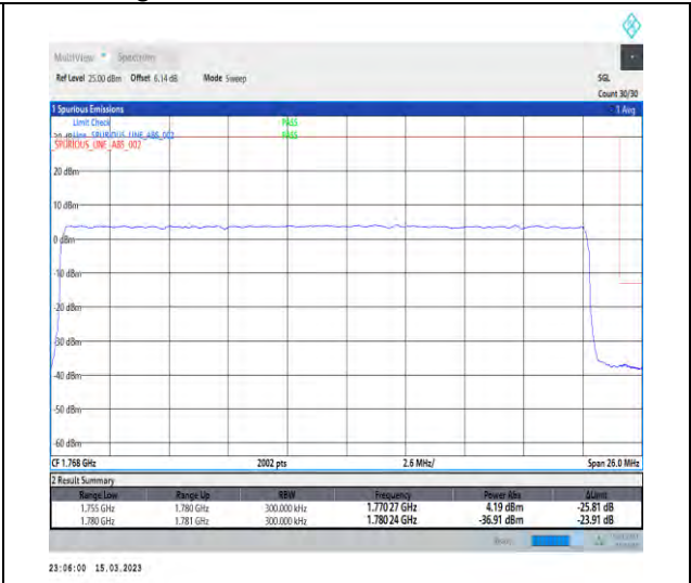
1-N66-PC3-15-25-H-3-DFT-PI2BPSK-Outer_Full-1-28@0-Ant1-1-seegraph-PASS-see graph
