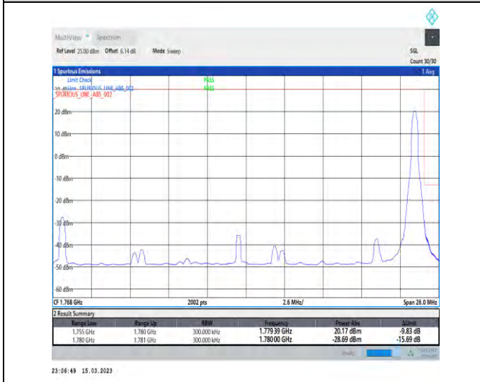
1-N66-PC3-15-25-H-5-CP-QPSK-Edge_1RB_Right-1@132-Ant1-1-seegraph-PASS-see graph
