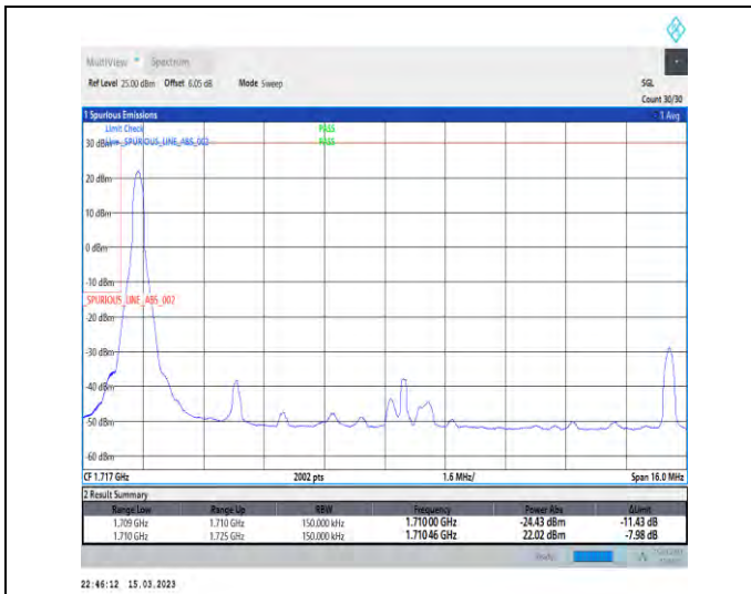
1-N66-PC3-15-15-L-1-DFT-PI2BPSK-Edge_1RB_Left-1@0-Ant1-1-seegraph-PASS-see graph
