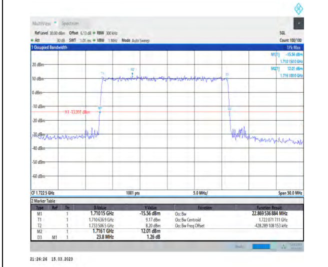
1-N66-PC3-15-25-L-3-DFT-16QAM-Outer_Full-128 @0-Ant1-22.87-23.800-≤25-PASS
