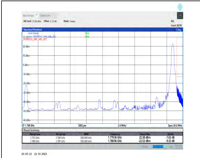
1-N66-PC3-15-25-H-2-DFT-PI2BPSK-Edge_1RB_Right-t-1@132-Ant1-1-seegraph-PASS-see graph
