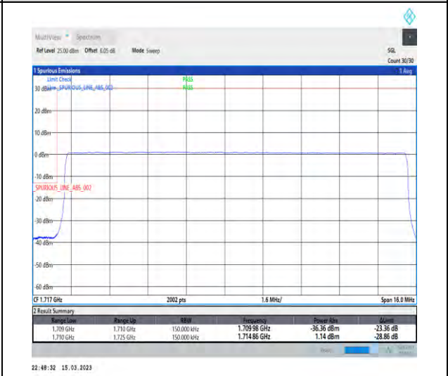
1-N66-PC3-15-15-L-6-CP-QPSK-Outer_Full-79@0-Ant1-1-seegraph-PASS-see graph
