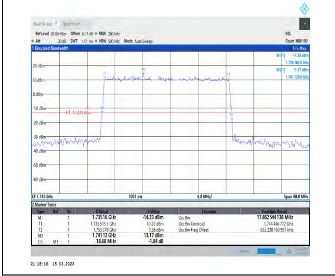
1-N66-PC3-15-20-M-1-DFT-QPSK-Outer_Full-100@0-Ant1-17.863-18.680-≤20-PASS
