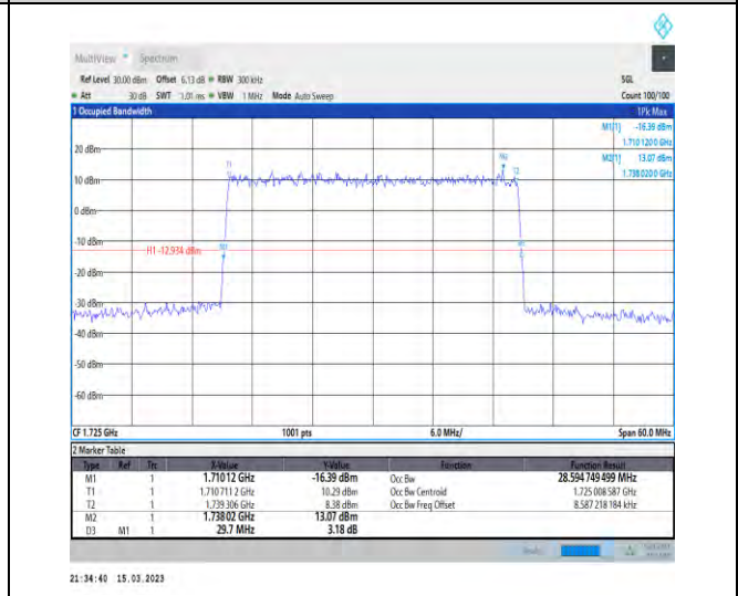
1-N66-PC3-15-30-L-1-DFT-QPSK-Outer_Full-160@ 0-Ant1-28.595-29.700-≤30-PASS
