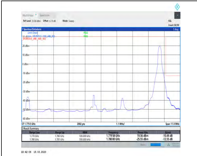
1-N66-PC3-15-10-H-2-DFT-PI2BPSK-Edge_1RB_Right-t@51-Ant1-1-seegraph-PASS-see graph
