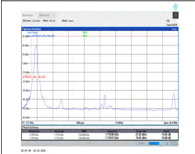
1-N66-PC3-15-15-L-4-CP-QPSK-Edge_1RB_Left-1@0-Ant1-1-seegraph-PASS-see graph
