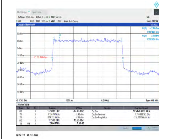
1-N66-PC3-15-30-H-2-DFT-PI2BPSK-Outer_Full-160 @0-Ant1-28.506-29.640-≤30-PASS
