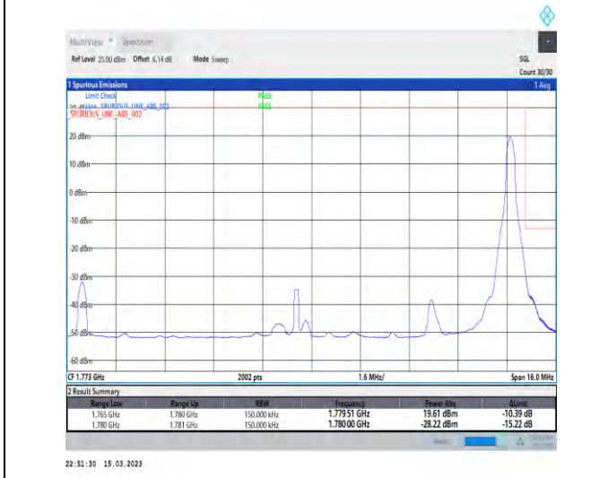
1-N66-PC3-15-15-H-5-CP-QPSK-Edge_1RB_Right-1@78-Ant1-1-seegraph-PASS-see graph
