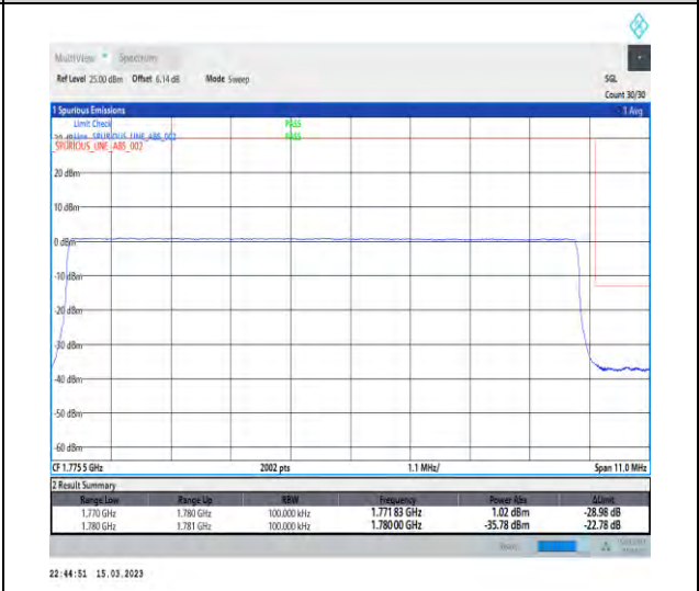
1-N66-PC3-15-10-H-6-CP-QPSK-Outer_Full-52@0-Ant1-1-seegraph-PASS-see graph
