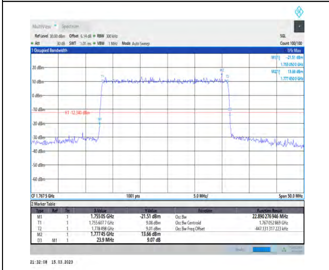
1-N66-PC3-15-25-H-1-DFT-QPSK-Outer_Full-128@ 0-Ant1-22.89-23.900-<25-PASS
