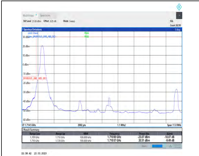
1-N66-PC3-15-10-L-1-DFT-PI2BPSK-Edge_1RB_Left-1@0-Ant1-1-seegraph-PASS-see graph
