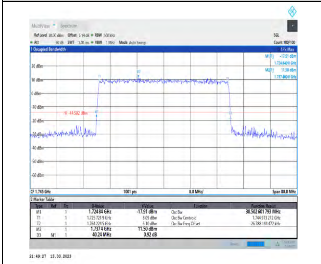
1-N66-PC3-15-40-M-8-CP-64QAM-Outer_Full-216@0 -Ant1-38.503-40.240-≤40-PASS
