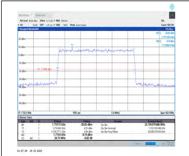
1-N66-PC3-15-25-L-9-CP-256QAM-Outer_Full-133 @0-Ant1-23.734-24.750-≤25-PASS
