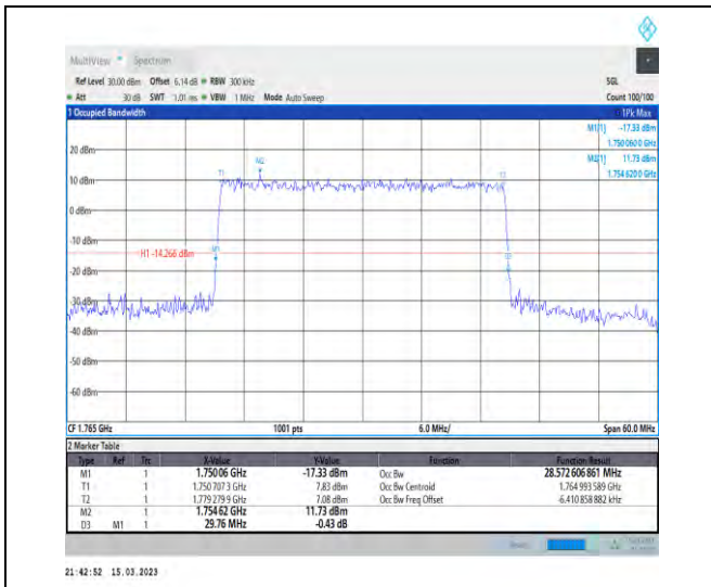
1-N66-PC3-15-30-H-4-DFT-64QAM-Outer_Full-160 @0-Ant1-28.573-29.760-≤30-PASS
