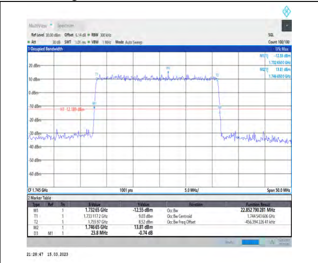
1-N66-PC3-15-25-M-1-DFT-QPSK-Outer_Full-128 @0-Ant1-22.853-23.800-≤25-PASS
