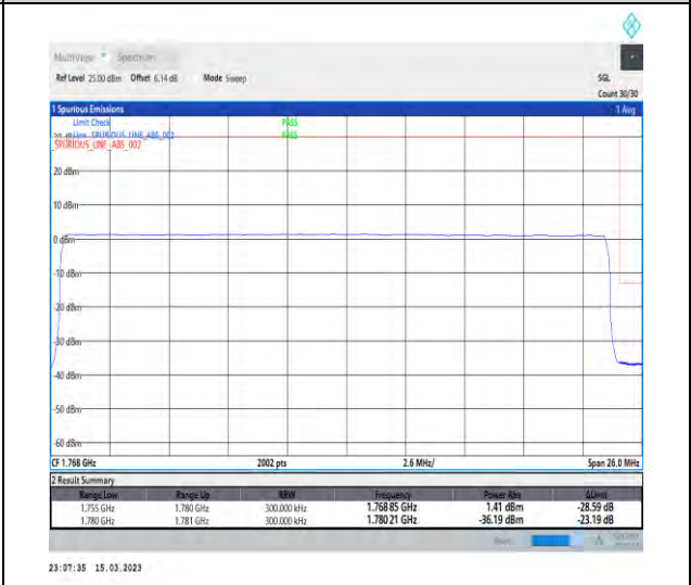
1-N66-PC3-15-25-H-6-CP-QPSK-Outer_Full-133@0-Ant1-1-seegraph-PASS-see graph
