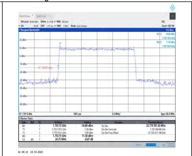
1-N66-PC3-15-25-H-8-CP-64QAM-Outer_Full-133@ 0-Ant1-23.775-24.750-≤25-PASS
