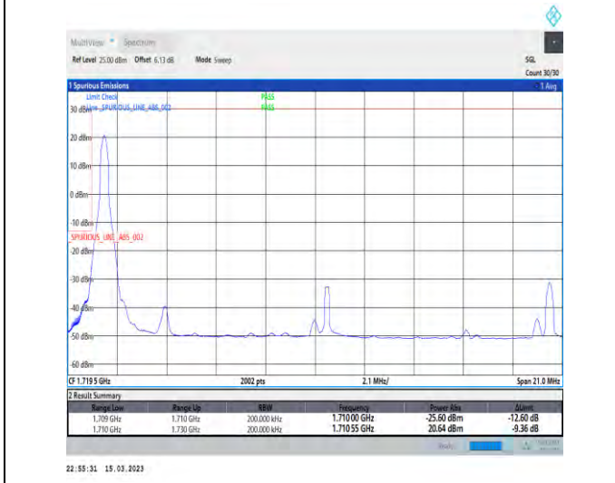
1-N66-PC3-15-20-L-4-CP-QPSK-Edge_1RB_Left-1@0-Ant1-1-seegraph-PASS-see graph
