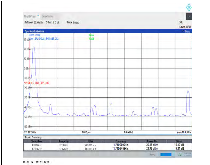
1-N66-PC3-15-25-L-1-DFT-PI2BPSK-Edge_1RB_Left-1@0-Ant1-1-seegraph-PASS-see graph
