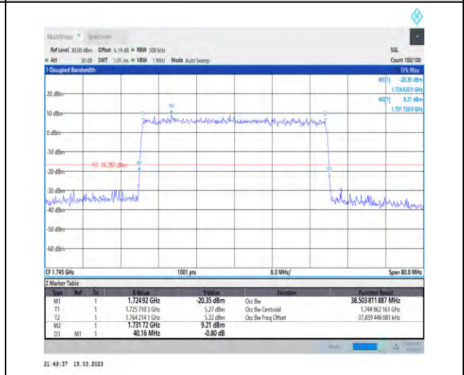
1-N66-PC3-15-40-M-9-CP-256QAM-Outer_Full-216@0 -Ant1-38.504-40.160-≤40-PASS
