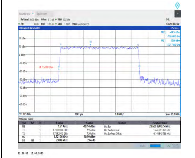
1-N66-PC3-15-30-L-4-DFT-64QAM-Outer_Full-160 @0-Ant1-28.601-29.880-≤30-PASS
