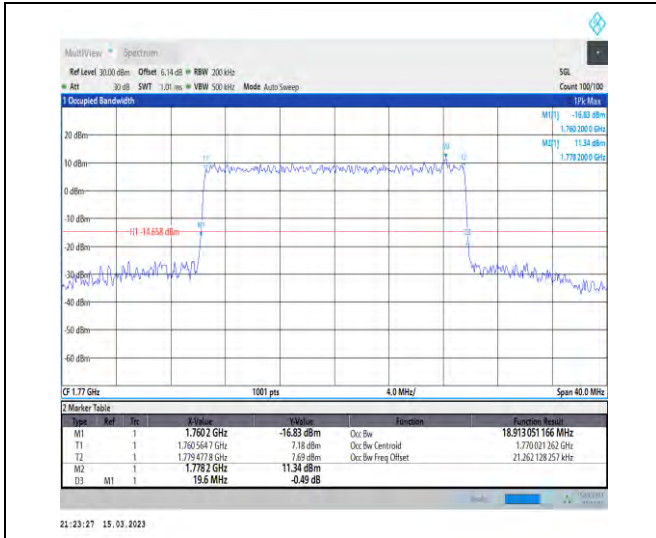
1-N66-PC3-15-20-H-6-CP-QPSK-Outer_Full-106@0 -Ant1-18.913-19.600-≤20-PASS
