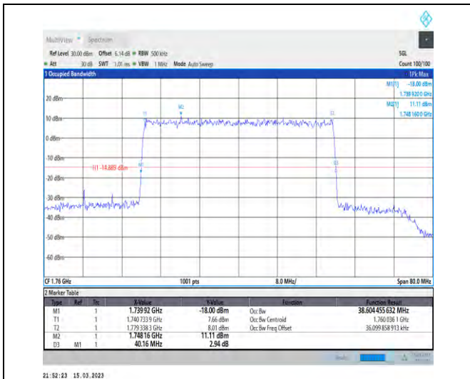
1-N66-PC3-15-40-H-5-DFT-256QAM-Outer_Full-216 @0-Ant1-38.604-40.160-≤40-PASS
