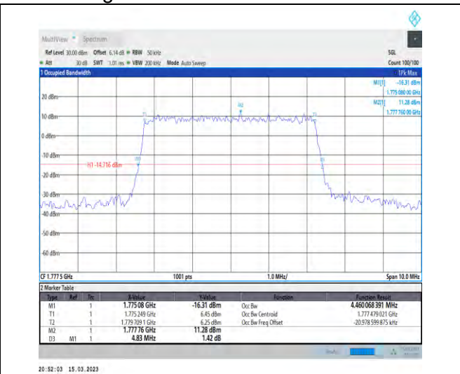
1-N66-PC3-15-5-H-4-DFT-64QAM-Outer_Full-25@0 -Ant1-4.46-4.830-≤5-PASS
