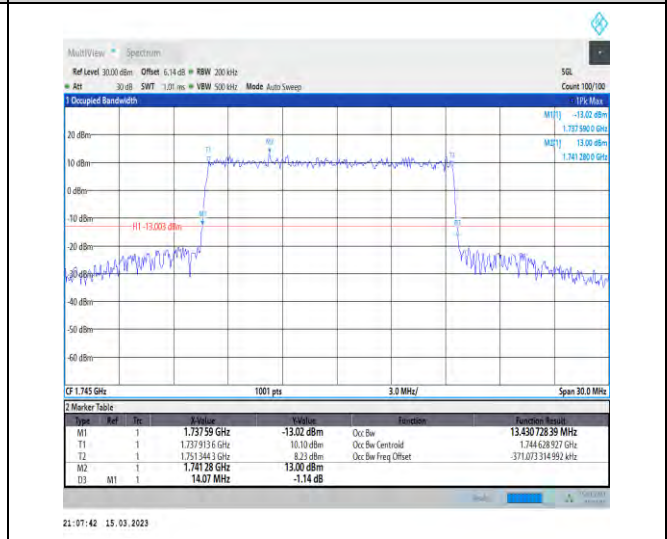
1-N66-PC3-15-15-M-1-DFT-QPSK-Outer_Full-75@0-Ant1-13.431-14.070-≤15-PASS
