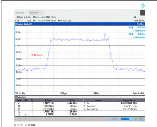
1-N66-PC3-15-5-M-4-DFT-64QAM-Outer_Full-25@0 -Ant1-4.46-4.780-≤5-PASS
