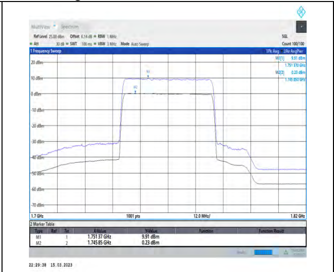
1-N66-PC3-15-40-H-2-CP-256QAM-Outer_Full-216 @0-Ant1-9.68-100%-0.00-9.68-PASS-≤13
