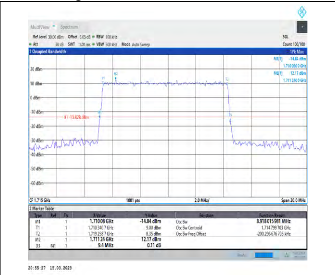
1-N66-PC3-15-10-L-3-DFT-16QAM-Outer_Full-50 @0-Ant1-8.918-9.400-≤10-PASS
