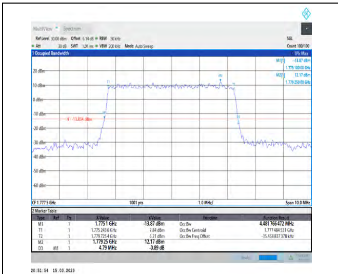
1-N66-PC3-15-5-H-3-DFT-16QAM-Outer_Full-25@0 -Ant1-4.482-4.790-≤5-PASS
