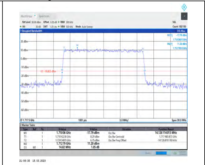
1-N66-PC3-15-15-L-8-CP-64QAM-Outer_Full-79@0-Ant1-14.126-14.820-≤15-PASS
