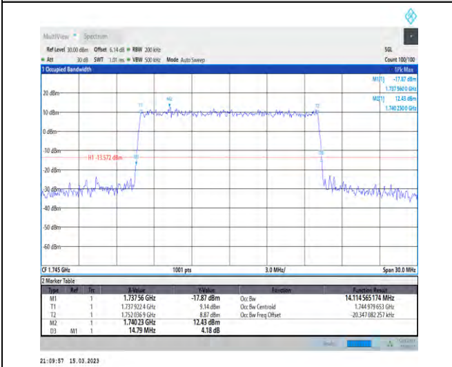
1-N66-PC3-15-15-M-8-CP-64QAM-Outer_Full-79@0-Ant1-14.115-14.790-≤15-PASS
