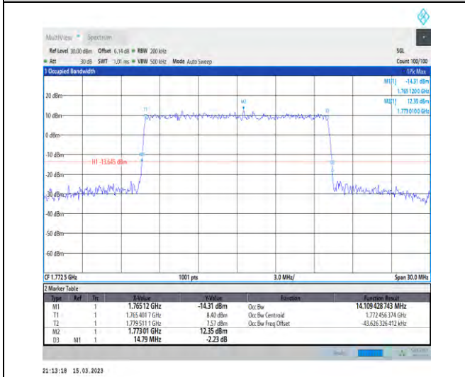
1-N66-PC3-15-15-H-7-CP-16QAM-Outer_Full-79@0 -Ant1-14.109-14.790-≤15-PASS
