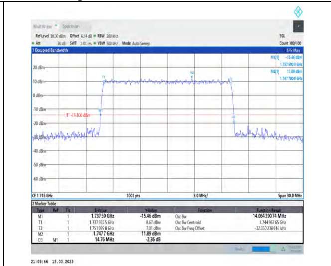
1-N66-PC3-15-15-M-7-CP-16QAM-Outer_Full-79@0-Ant1-14.064-14.760-≤15-PASS
