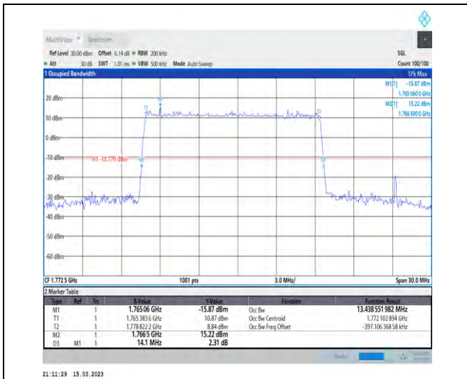
1-N66-PC3-15-15-H-1-DFT-QPSK-Outer_Full-75@0-Ant1-13.439-14.100-≤15-PASS
