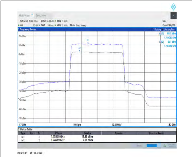
1-N66-PC3-15-40-H-1-DFT-256QAM-Outer_Full-216 @0-Ant1-9.02-100%-0.00-9.02-PASS-≤13
