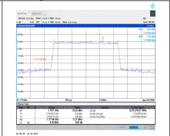
1-N66-PC3-15-10-L-7-CP-16QAM-Outer_Full-52@0- Ant1-9.272-9.780-≤10-PASS
