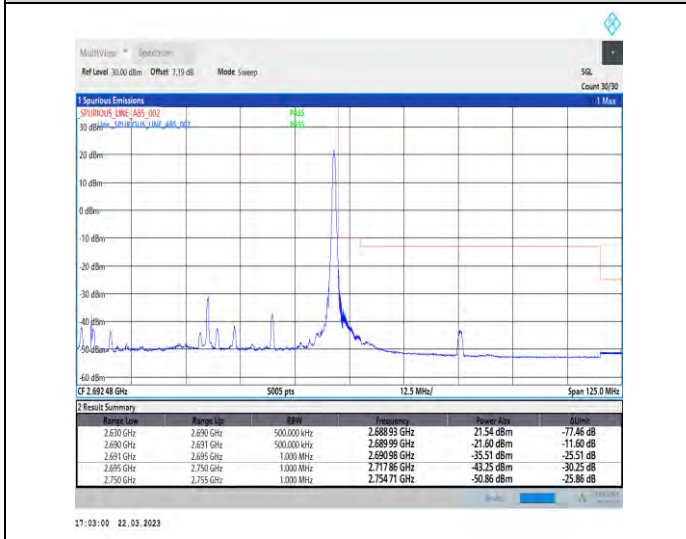
1-N41-30-60-H-5-CP-QPSK-Edge_1RB_Right-1@161-Ant1-1--PASS-see graph
