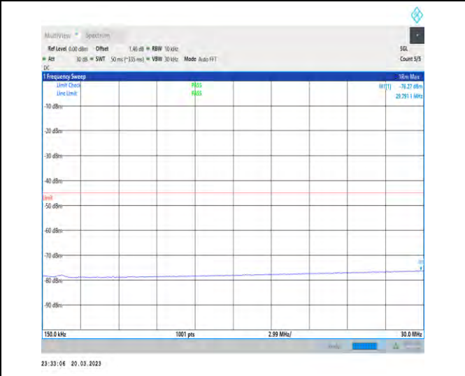
1-N41-30-100-M-1-DFT-PI2BPSK-Inner_1RB_Left-1 @1-0.15-30-Ant1-29.79--76.27--45-PASS
