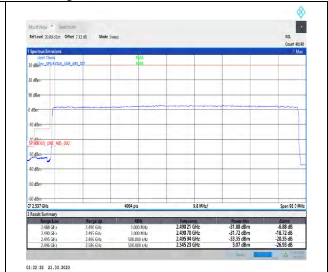
1-N41-30-90-L-3-DFT-PI2BPSK-Outer_Full-240@0-Ant1-1--PASS-see graph
