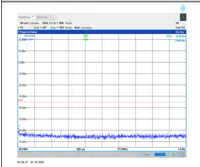
1-N41-30-100-H-1-DFT-PI2BPSK-Inner_1RB_Left-1 @1-30-1000-Ant1-33.88--59.38--35-PASS
