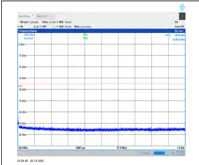
1-N41-30-100-M-1-DFT-QPSK-Edge_1RB_Left-1@ 0-30-1000-Ant1-33.49--68.39--35-PASS
