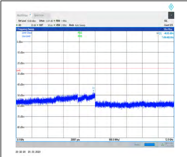
1-N41-30-100-L-1-DFT-PI2BPSK-Inner_1RB_Left-1 @1-3000-12000-Ant1-7406.40--46.82--25-PASS
