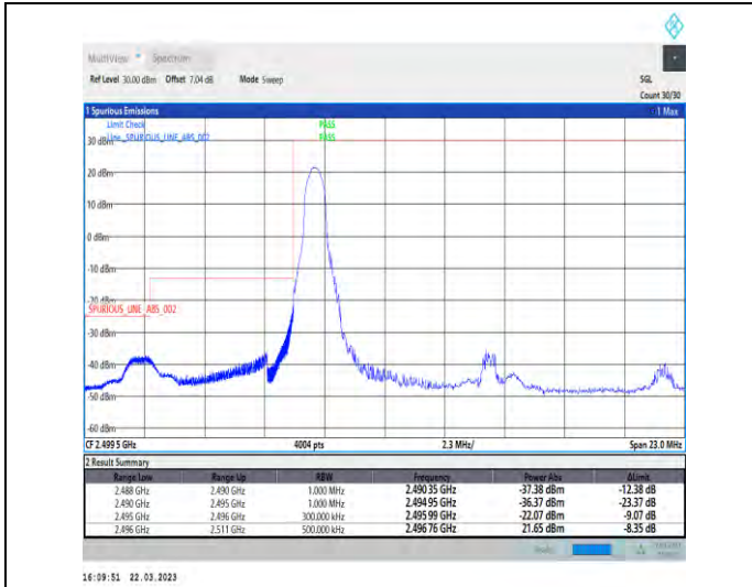
1-N41-30-15-L-4-CP-QPSK-Edge_1RB_Left-1@0-Ant1 1-1--PASS-see graph
