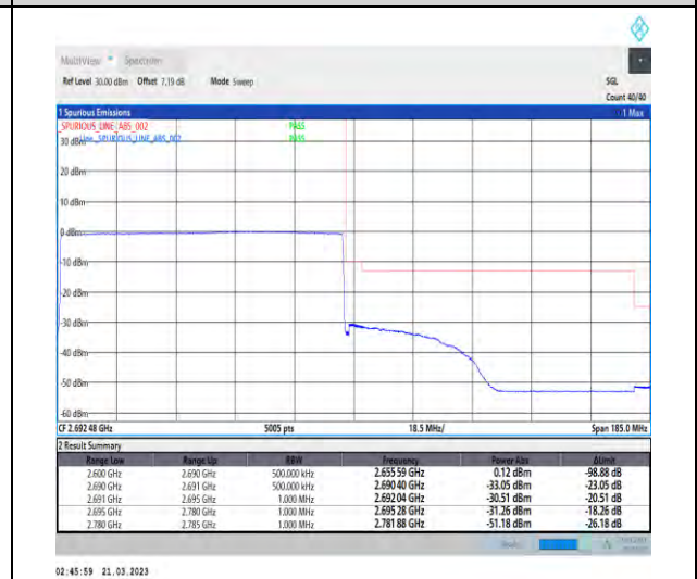
1-N41-30-90-H-6-CP-QPSK-Outer_Full-245@0-Ant1-1--PASS-see graph
