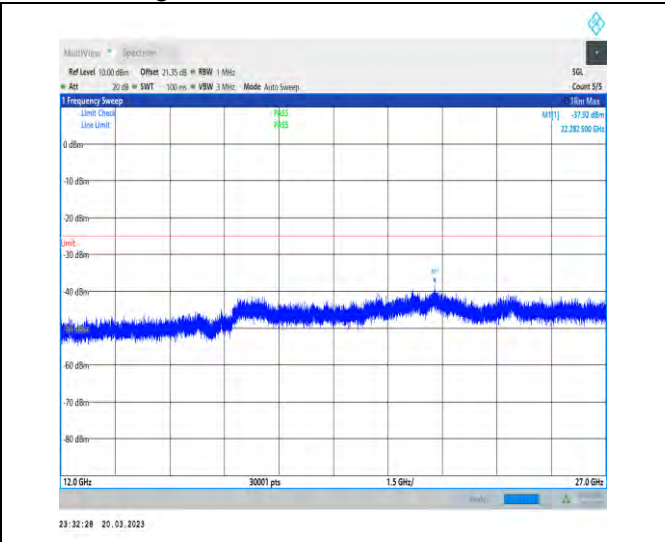
1-N41-30-100-L-1-DFT-PI2BPSK-Inner_1RB_Left-1 @1-12000-27000-Ant1-22282.50--37.92--25-PASS
