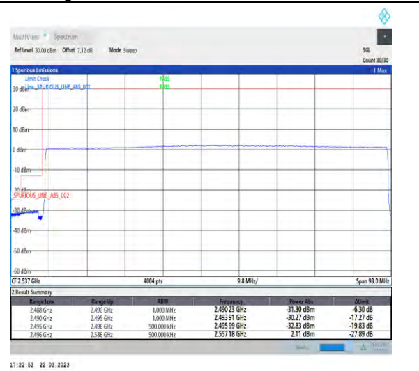
1-N41-30-90-L-6-CP-QPSK-Outer_Full-245@0-Ant1-1--PASS-see graph
