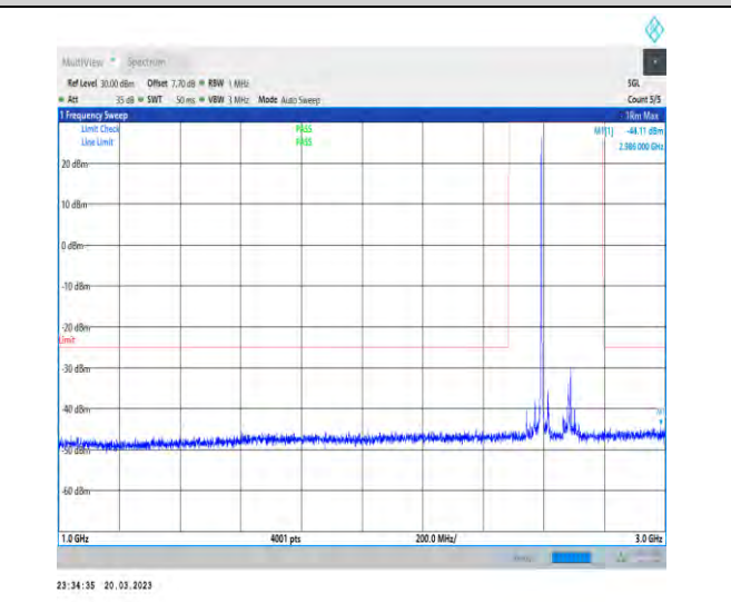
1-N41-30-100-H-1-DFT-PI2BPSK-Inner_1RB_Left-1 @1-1000-3000-Ant1-2986.00--44.11--25-PASS
