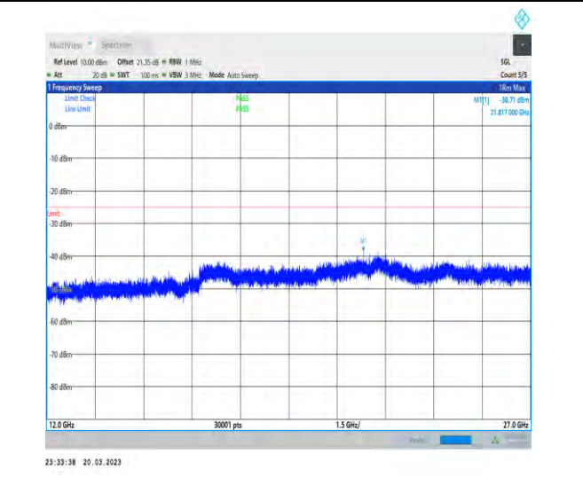
1-N41-30-100-M-1-DFT-PI2BPSK-Inner_1RB_Left-1 @1-12000-27000-Ant1-21817.00--38.71--25-PASS
