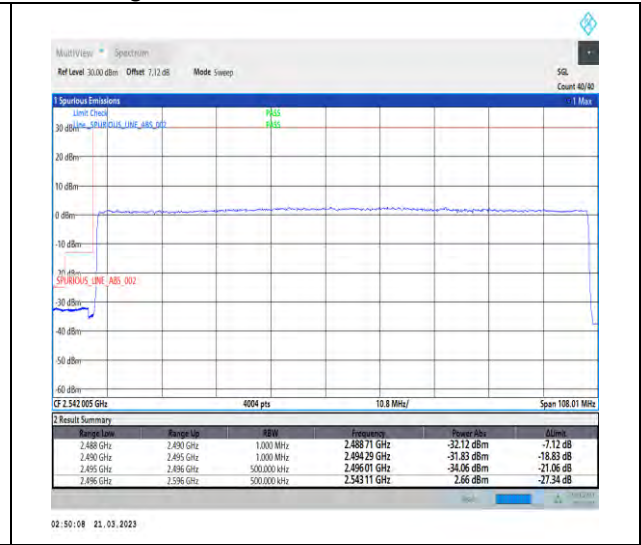
1-N41-30-100-L-3-DFT-PI2BPSK-Outer_Full-270@0-Ant1-1--PASS-see graph
