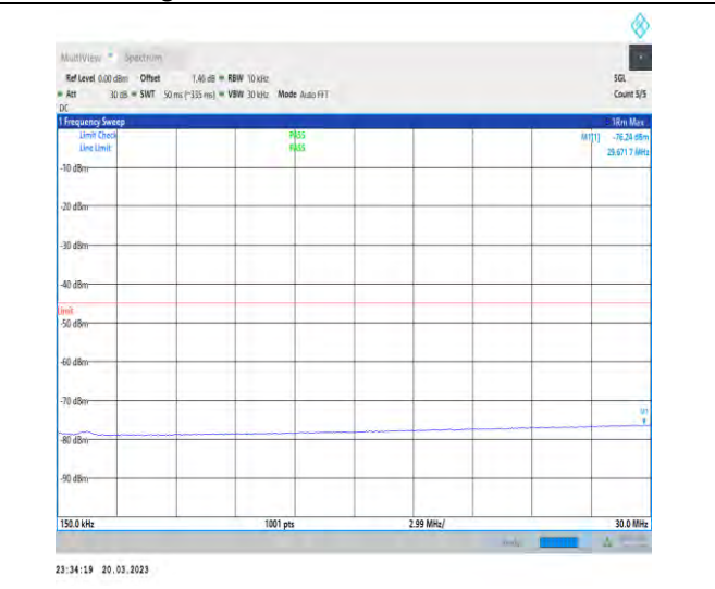
1-N41-30-100-H-1-DFT-PI2BPSK-Inner_1RB_Left-1 @1-0.15-30-Ant1-29.67--76.24--45-PASS
