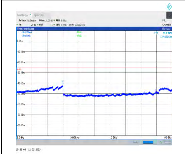
1-N41-30-100-M-1-DFT-QPSK-Edge_1RB_Left-1@ 0-3000-18000-Ant1-7476.00--41.79--25-PASS
