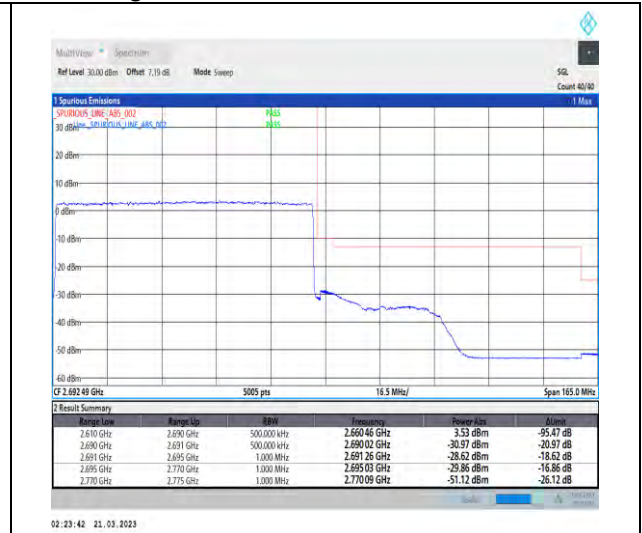
1-N41-30-80-H-3-DFT-PI2BPSK-Outer_Full-216@0-Ant1-1--PASS-see graph
