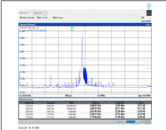
1-N41-30-80-H-2-DFT-PI2BPSK-Edge_1RB_Right-1@216-Ant1-1--PASS-see graph
