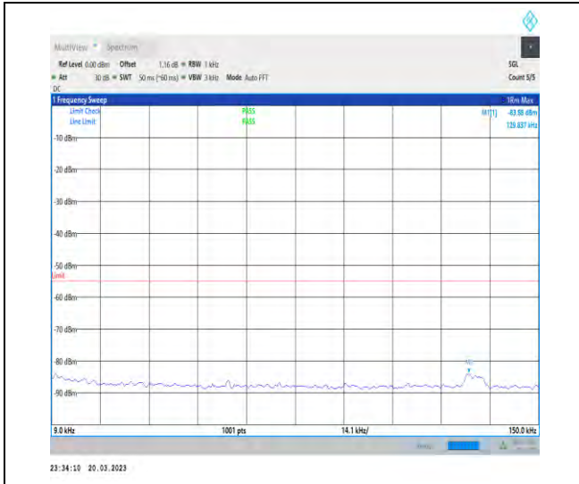
1-N41-30-100-H-1-DFT-PI2BPSK-Inner_1RB_Left-1 @1-0.009-0.15-Ant1-0.13--83.88--55-PASS
