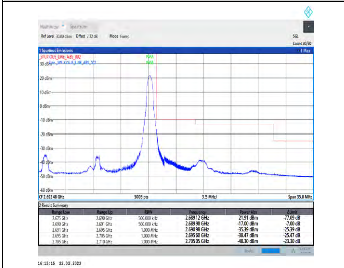
1-N41-30-15-H-5-CP-QPSK-Edge_1RB_Right-1@37-Ant1 1-1--PASS-see graph
