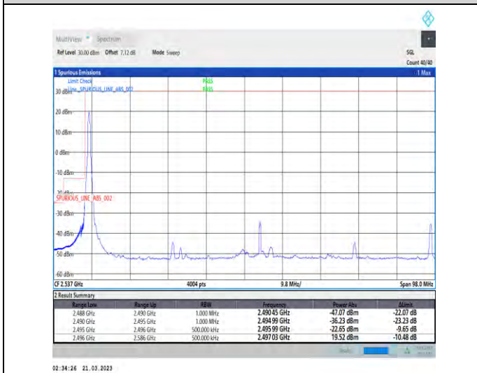
1-N41-30-90-L-4-CP-QPSK-Edge_1RB_Left-1@0-Ant1-1--PASS-see graph
