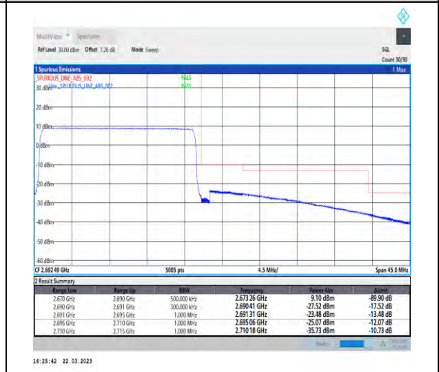
1-N41-30-20-H-6-CP-QPSK-Outer_Full-51@0-Ant1 1--PASS-see graph
