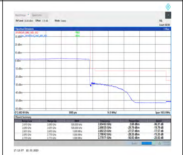
1-N41-30-80-H-6-CP-QPSK-Outer_Full-217@0-Ant1-1--PASS-see graph
