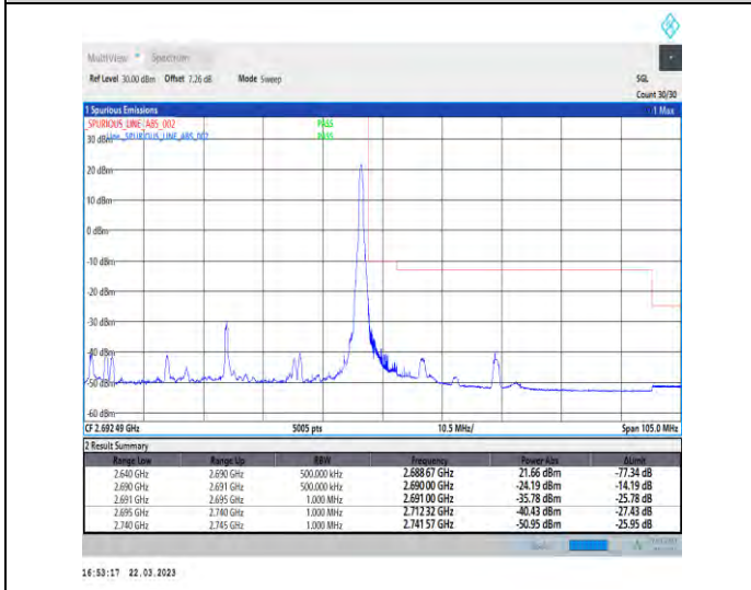
1-N41-30-50-H-5-CP-QPSK-Edge_1RB_Right-1@132-Ant1-1--PASS-see graph
