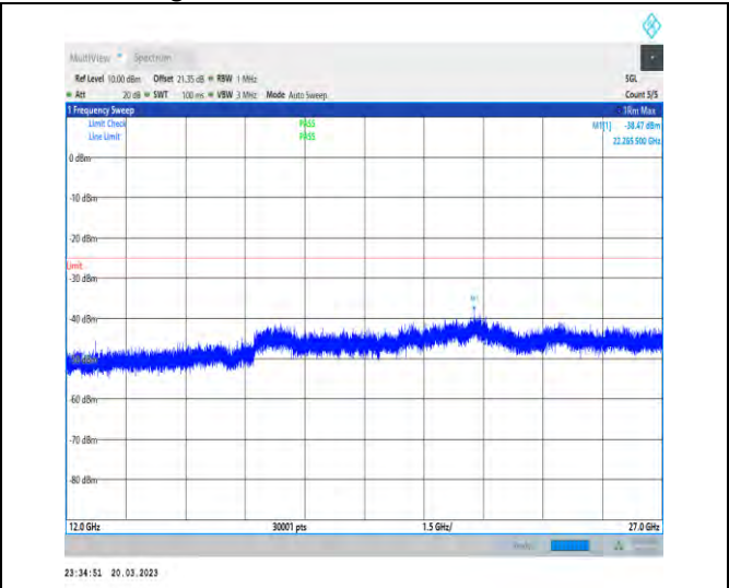
1-N41-30-100-H-1-DFT-PI2BPSK-Inner_1RB_Left-1 @1-12000-27000-Ant1-22265.50--38.47--25-PASS
