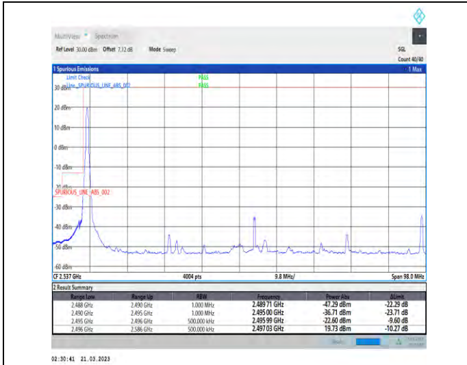
1-N41-30-90-L-1-DFT-PI2BPSK-Edge_1RB_Left-1@0-Ant1-1--PASS-see graph
