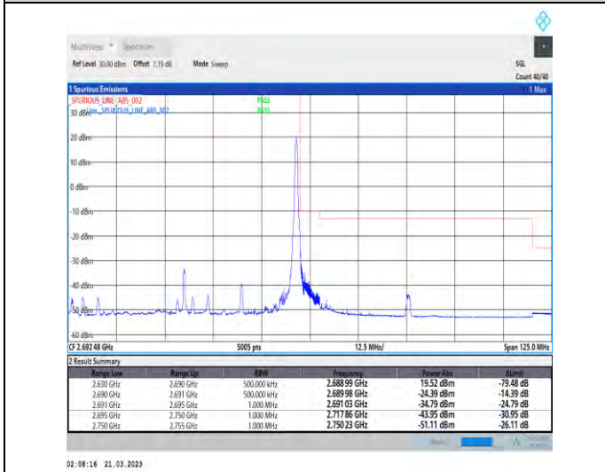
1-N41-30-60-H-5-CP-QPSK-Edge_1RB_Right-1@161-Ant1-1--PASS-see graph
