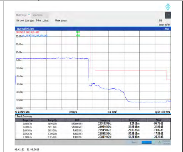
1-N41-30-90-H-3-DFT-PI2BPSK-Outer_Full-240@0-Ant1-1--PASS-see graph
