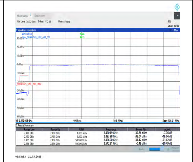
1-N41-30-100-L-6-CP-QPSK-Outer_Full-273@0-Ant1-1--PASS-see graph
