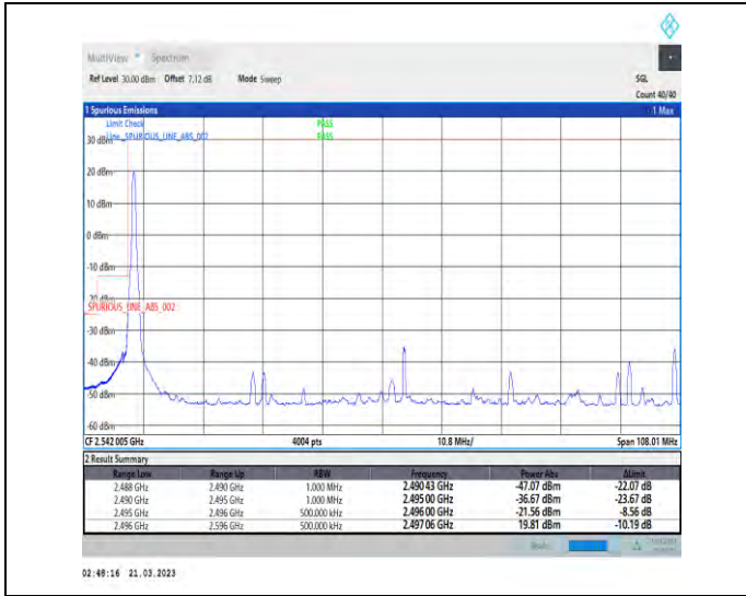
1-N41-30-100-L-1-DFT-PI2BPSK-Edge_1RB_Left-1@0-Ant1-1--PASS-see graph
