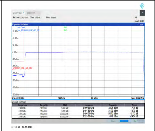
1-N41-30-80-L-6-CP-QPSK-Outer_Full-217@0-Ant1-1--PASS-see graph
