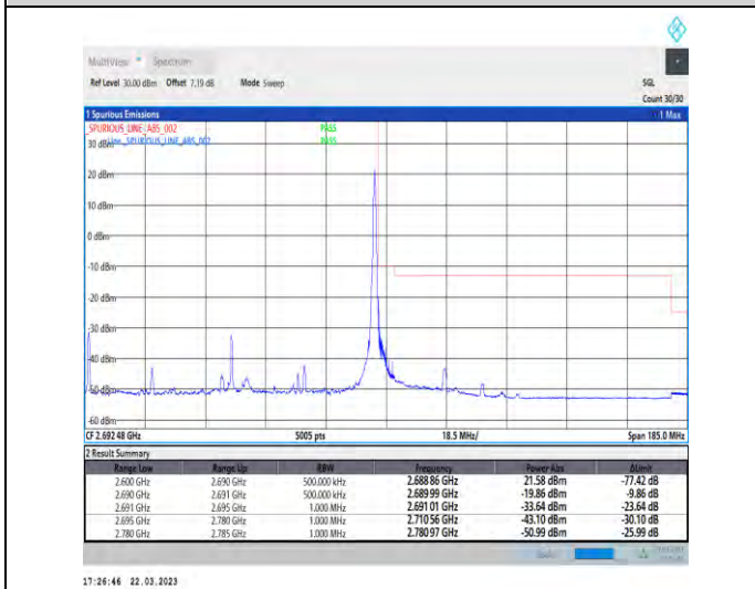
1-N41-30-90-H-5-CP-QPSK-Edge_1RB_Right-1@244-Ant1-1--PASS-see graph
