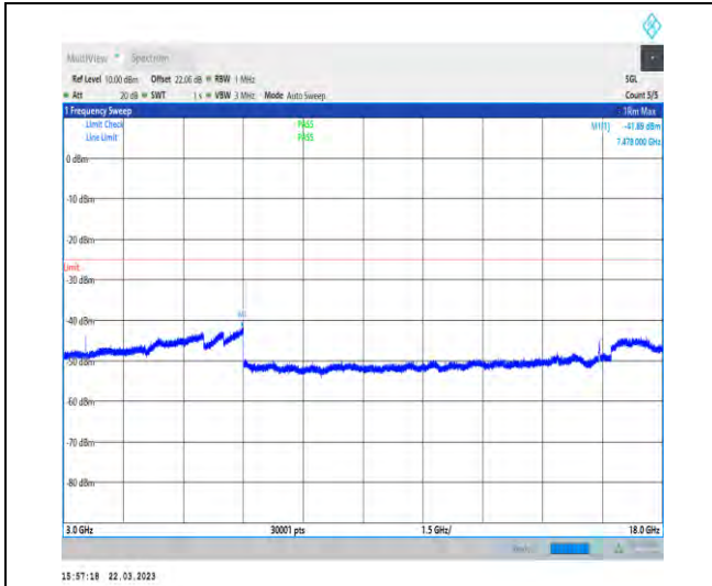
1-N41-30-100-H-1-DFT-QPSK-Edge_1RB_Left-1@ 0-3000-18000-Ant1-7478.00--41.89--25-PASS
