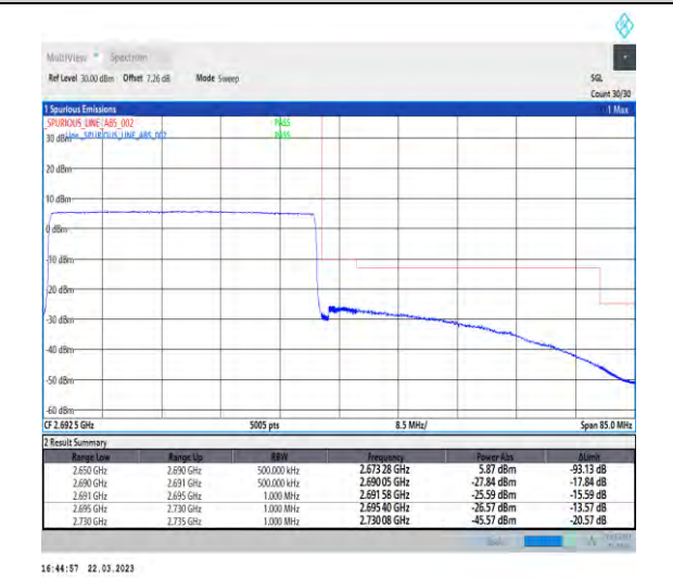
1-N41-30-40-H-6-CP-QPSK-Outer_Full-106@0-Ant1-1--PASS-see graph
