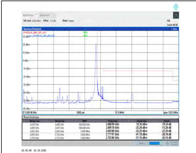
1-N41-30-60-H-2-DFT-PI2BPSK-Edge_1RB_Right-1@161-Ant1-1--PASS-see graph
