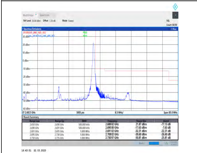
1-N41-30-40-H-5-CP-QPSK-Edge_1RB_Right-1@105-Ant1-1--PASS-see graph
