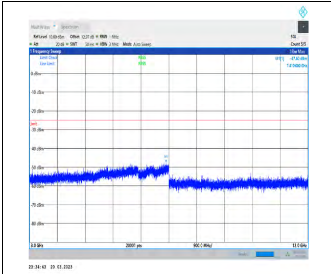
1-N41-30-100-H-1-DFT-PI2BPSK-Inner_1RB_Left-1 @1-3000-12000-Ant1-7410.00--47.60--25-PASS
