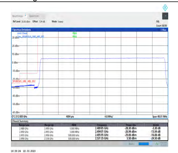
1-N41-30-40-L-6-CP-QPSK-Outer_Full-106@0-Ant1-1--PASS-see graph
