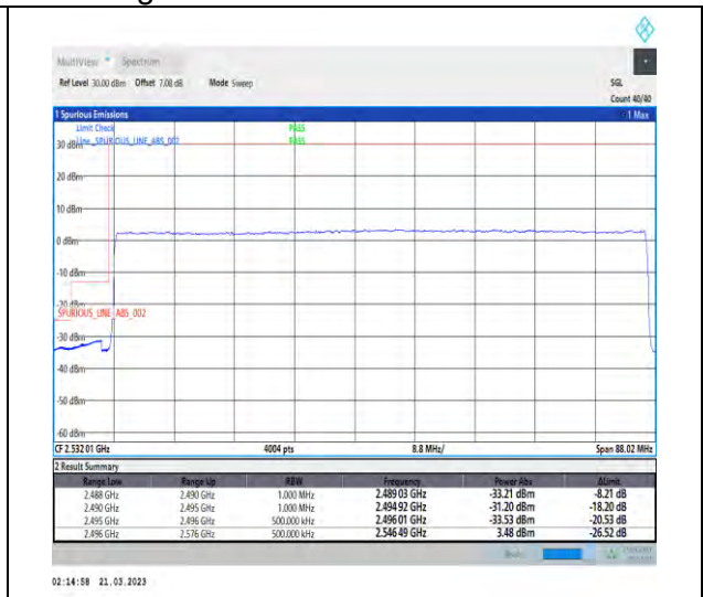
1-N41-30-80-L-3-DFT-PI2BPSK-Outer_Full-216@0-Ant1-1--PASS-see graph
