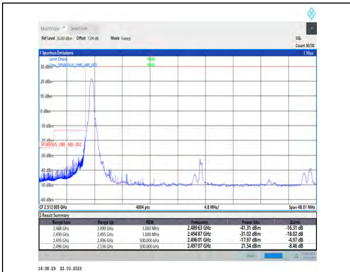
1-N41-30-40-L-4-CP-QPSK-Edge_1RB_Left-1@0-Ant1 -1--PASS-see graph
