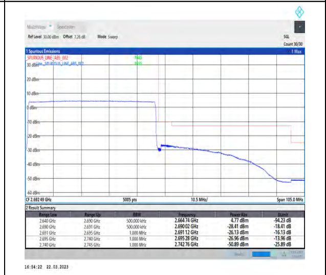
1-N41-30-50-H-6-CP-QPSK-Outer_Full-133@0-Ant1-1--PASS-see graph
