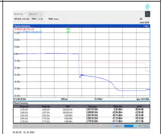
1-N41-30-80-H-6-CP-QPSK-Outer_Full-217@0-Ant1-1--PASS-see graph
