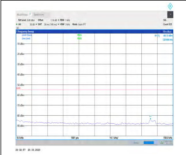
1-N41-30-100-M-1-DFT-PI2BPSK-Inner_1RB_Left-1 @1-0.009-0.15-Ant1-0.13--84.13--55-PASS
