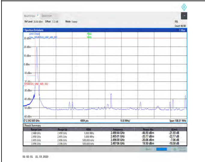
1-N41-30-100-L-4-CP-QPSK-Edge_1RB_Left-1@0-Ant1-1--PASS-see graph
