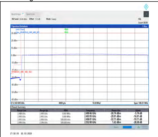
1-N41-30-100-L-6-CP-QPSK-Outer_Full-273@0-Ant 1-1--PASS-see graph
