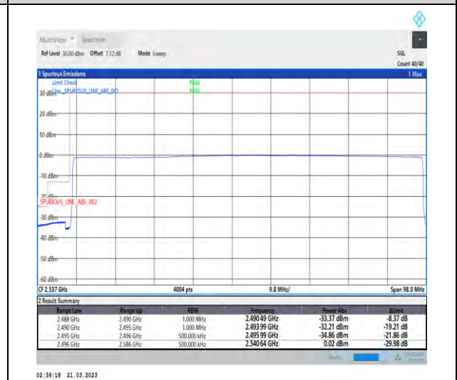
1-N41-30-90-L-6-CP-QPSK-Outer_Full-245@0-Ant1-1--PASS-see graph
