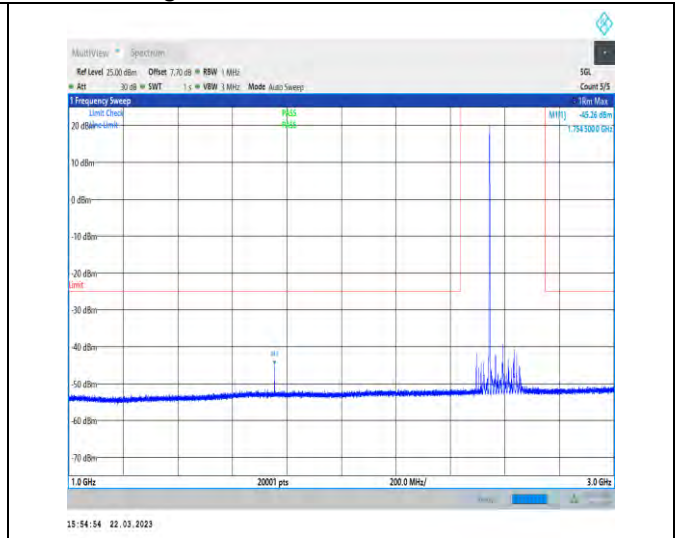
1-N41-30-100-M-1-DFT-QPSK-Edge_1RB_Left-1@0- 1000-3000-Ant1-1754.50--45.26--25-PASS
