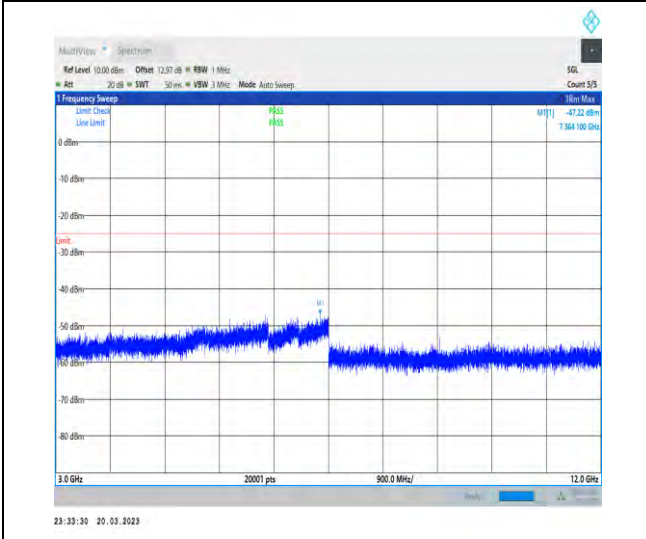
1-N41-30-100-M-1-DFT-PI2BPSK-Inner_1RB_Left-1 @1-3000-12000-Ant1-7364.10--47.22--25-PASS
