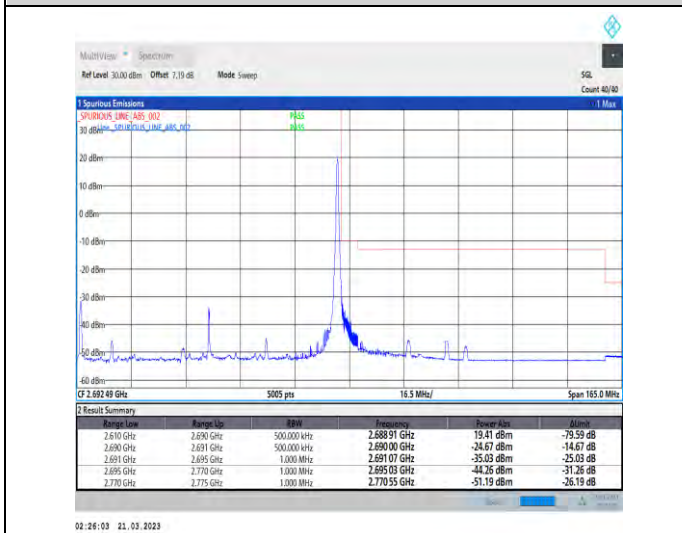
1-N41-30-80-H-5-CP-QPSK-Edge_1RB_Right-1@216-Ant1-1--PASS-see graph
