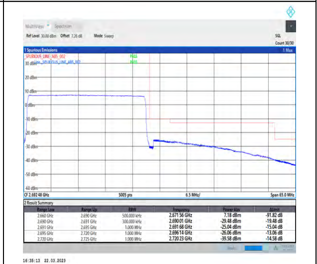
1-N41-30-30-H-6-CP-QPSK-Outer_Full-78@0-Ant1 1-1--PASS-see graph
