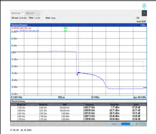
1-N41-30-100-H-6-CP-QPSK-Outer_Full-273@0-Ant 1-1--PASS-see graph
