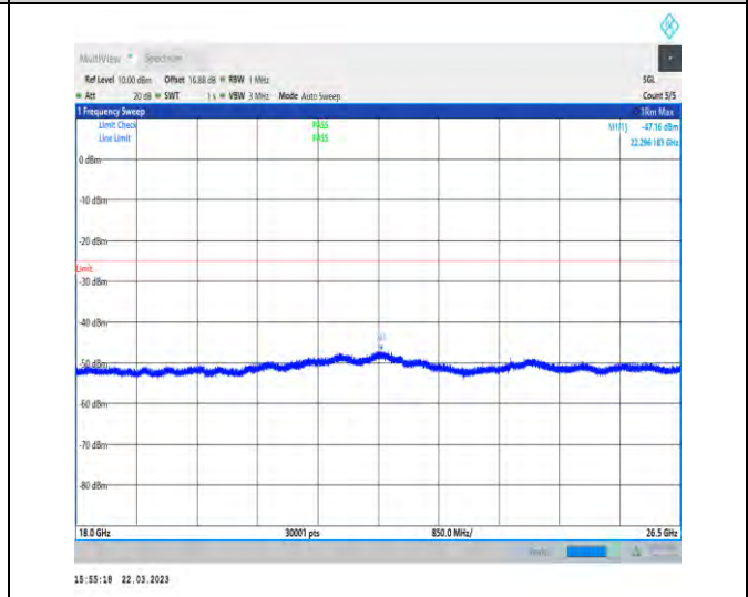
1-N41-30-100-M-1-DFT-QPSK-Edge_1RB_Left-1@0- 18000-26500-Ant1-22296.18--47.16--25-PASS
