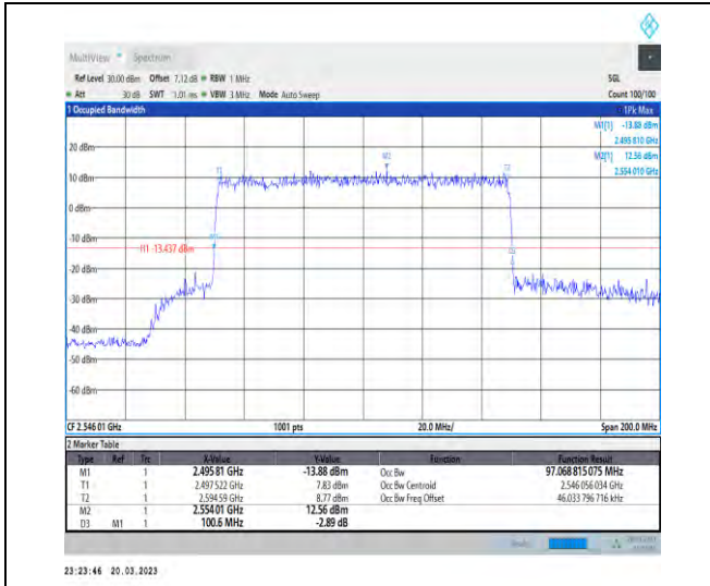
1-N41-30-100-L-6-CP-QPSK-Outer_Full-273@0-Ant 1-97.069-100.600-≤100-PASS
