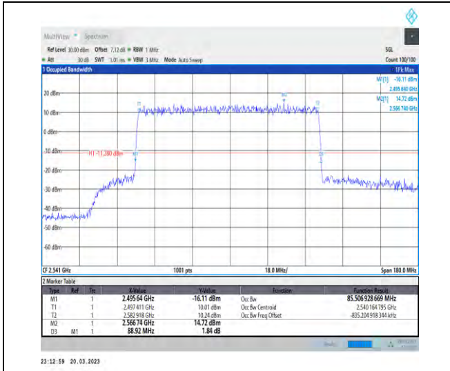
1-N41-30-90-L-1-DFT-QPSK-Outer_Full-240@0-Ant 1-85.507-88.920-≤90-PASS
