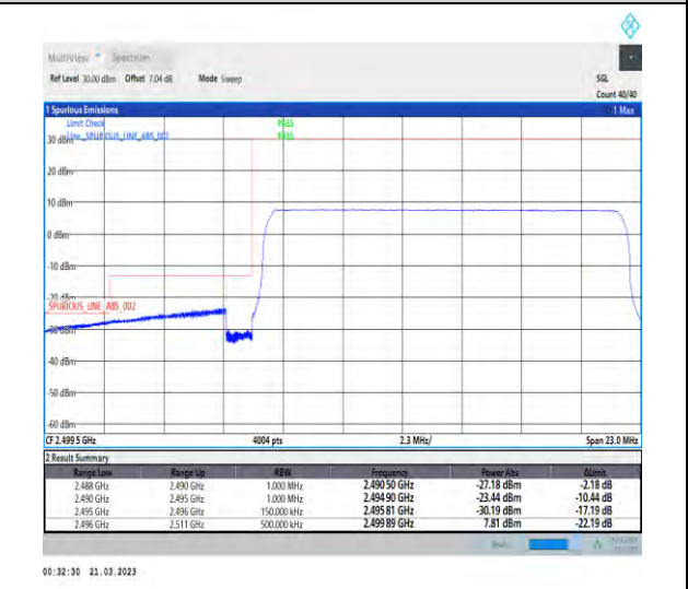
1-N41-30-15-L-6-CP-QPSK-Outer_Full-38@0-Ant1-1--PASS-see graph
