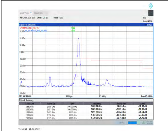
1-N41-30-30-H-5-CP-QPSK-Edge_1RB_Right-1@77-Ant1-1--PASS-see graph
