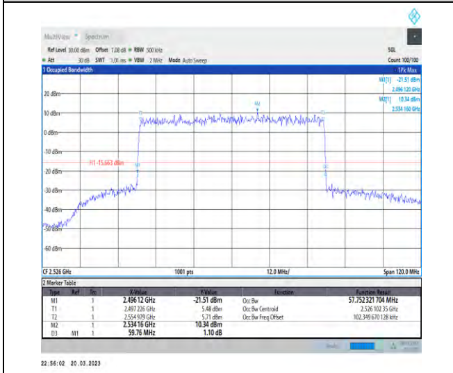
1-N41-30-60-L-5-DFT-256QAM-Outer_Full-162@0-A Ant1-57.752-59.760-≤60-PASS
