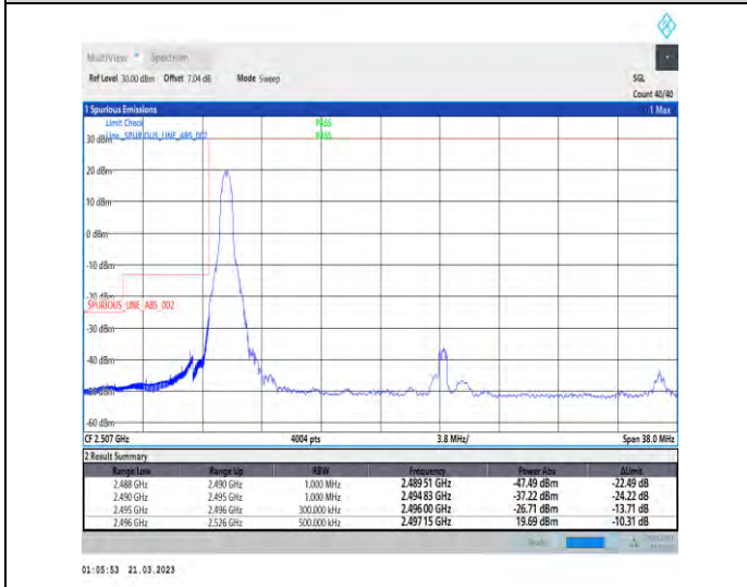
1-N41-30-30-L-4-CP-QPSK-Edge_1RB_Left-1@0-Ant1-1--PASS-see graph
