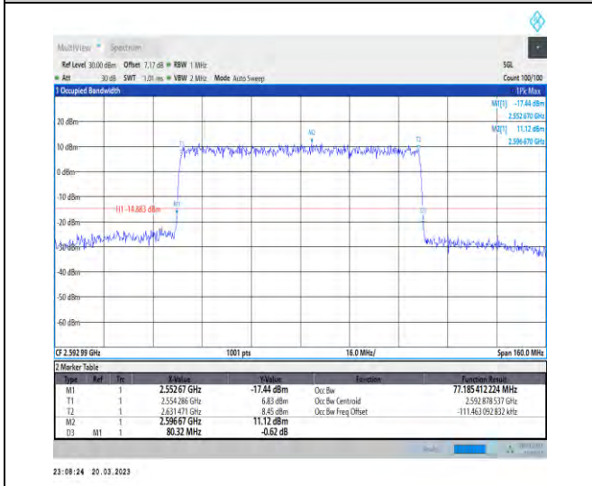
1-N41-30-80-M-5-DFT-256QAM-Outer_Full-216@0-A Ant1-77.185-80.320-≤80-PASS
