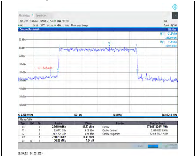
1-N41-30-60-M-7-CP-16QAM-Outer_Full-162@0-Ant 1-57.805-59.880-≤60-PASS
