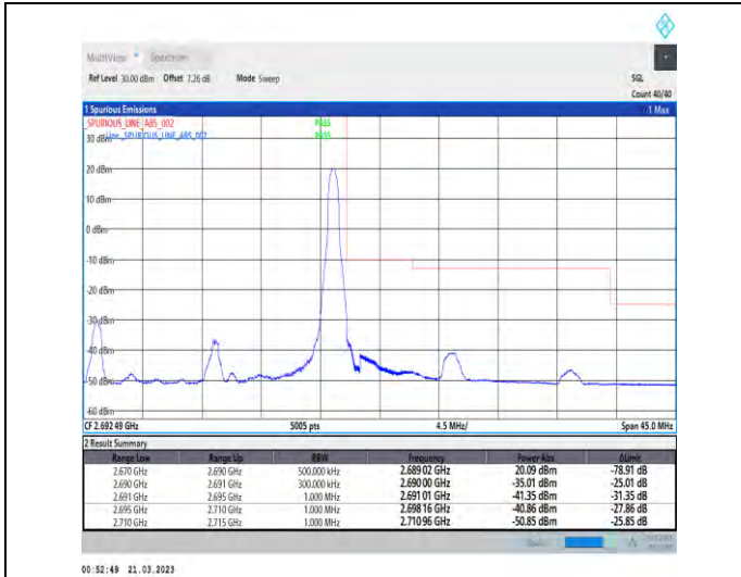
1-N41-30-20-H-2-DFT-PI2BPSK-Edge_1RB_Right-1@50-Ant1-1--PASS-see graph
