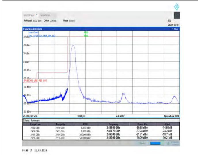
1-N41-30-20-L-4-CP-QPSK-Edge_1RB_Left-1@0-Ant1-1--PASS-see graph
