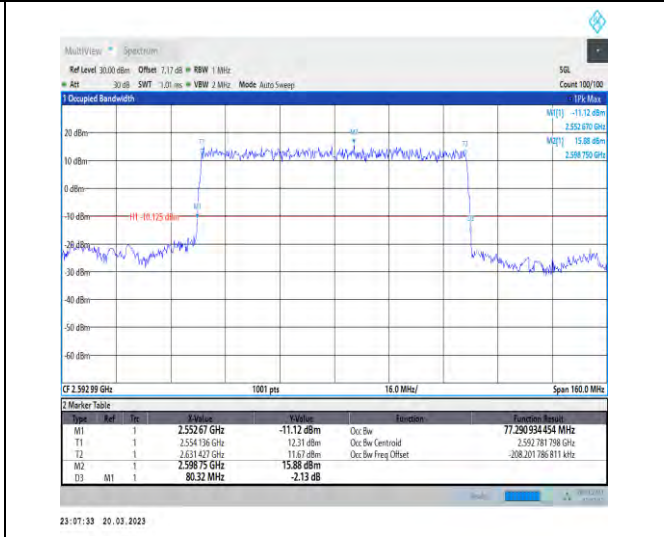
1-N41-30-80-M-2-DFT-PI2BPSK-Outer_Full-216@0-Ant 1-77.291-80.320-≤80-PASS
