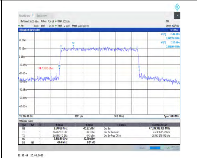
1-N41-30-50-H-7-CP-16QAM-Outer_Full-133@0-Ant 1-47.339-49.400-≤50-PASS
