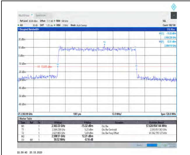
1-N41-30-60-M-6-CP-QPSK-Outer_Full-162@0-Ant 1-57.627-59.520-≤60-PASS
