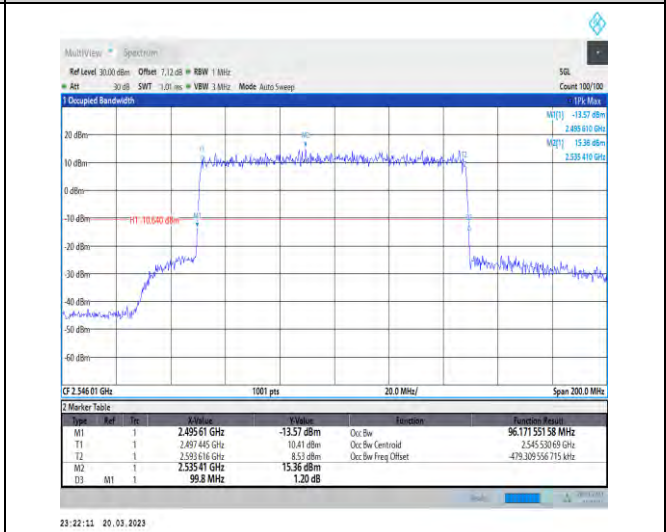
1-N41-30-100-L-1-DFT-QPSK-Outer_Full-270@0-An t1-96.172-99.800-≤100-PASS
