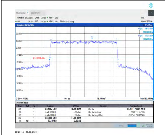
1-N41-30-90-H-5-DFT-256QAM-Outer_Full-240@0-A Ant1-85.591-89.100-≤90-PASS
