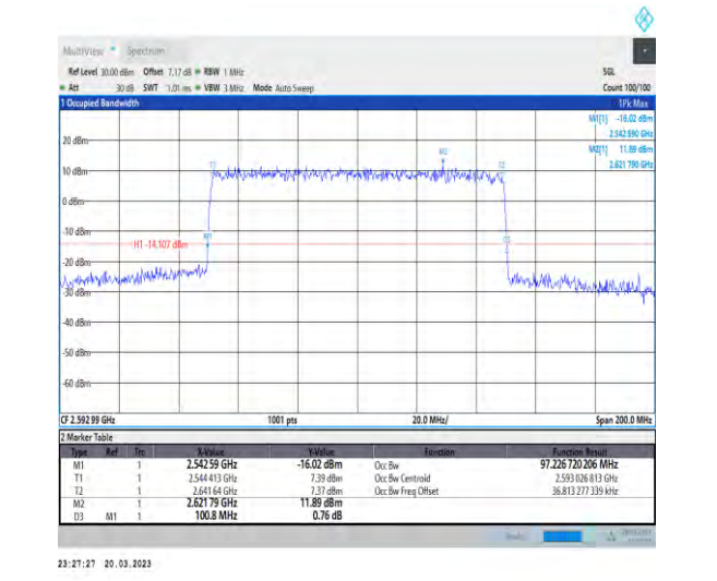
1-N41-30-100-M-8-CP-64QAM-Outer_Full-273@0-A nt1-97.227-100.800-≤100-PASS
