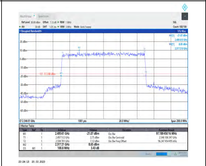
1-N41-30-100-L-9-CP-256QAM-Outer_Full-273@0-Ant nt1-97.189-100.800-≤100-PASS
