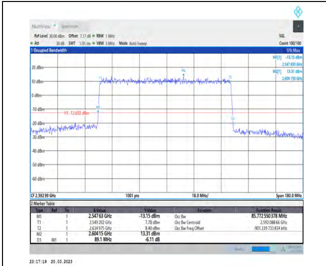
1-N41-30-90-M-4-DFT-64QAM-Outer_Full-240@0-A nt1-85.773-89.100-≤90-PASS
