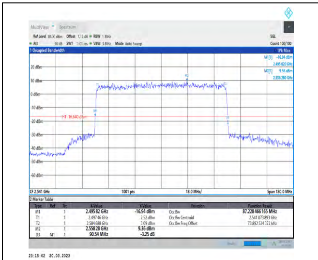
1-N41-30-90-L-9-CP-256QAM-Outer_Full-245@0-A nt1-87.228-90.540-≤90-PASS
