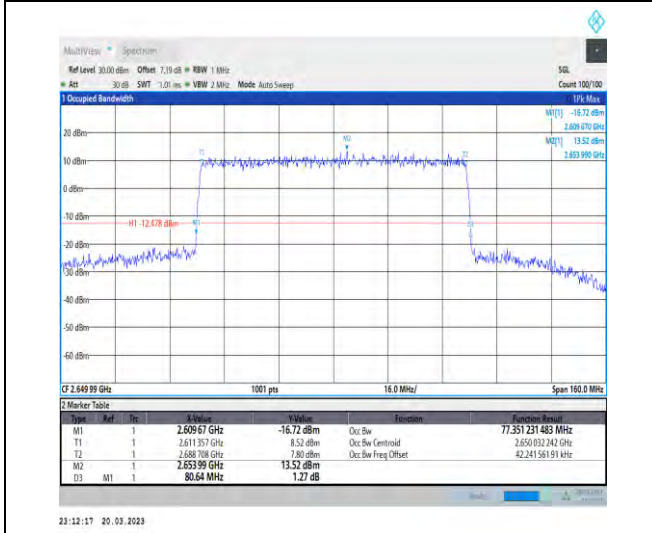
1-N41-30-80-H-8-CP-64QAM-Outer_Full-217@0-Ant 1-77.351-80.640-≤80-PASS
