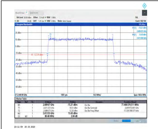
1-N41-30-80-H-6-CP-QPSK-Outer_Full-217@0-Ant1 -77.4-80.480-≤80-PASS
