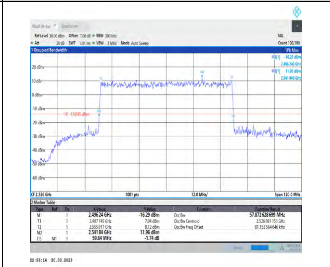
1-N41-30-60-L-6-CP-QPSK-Outer_Full-162@0-A Ant1-57.873-59.640-≤60-PASS
