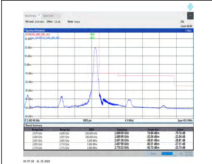
1-N41-30-20-H-5-CP-QPSK-Edge_1RB_Right-1@50-Ant1-1--PASS-see graph
