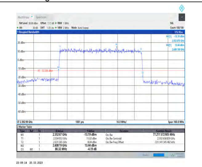
1-N41-30-80-M-4-DFT-64QAM-Outer_Full-216@0-A nt1-77.212-80.320-≤80-PASS
