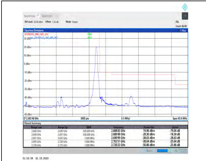
1-N41-30-30-H-2-DFT-PI2BPSK-Edge_1RB_Right-1@77-Ant1-1--PASS-see graph
