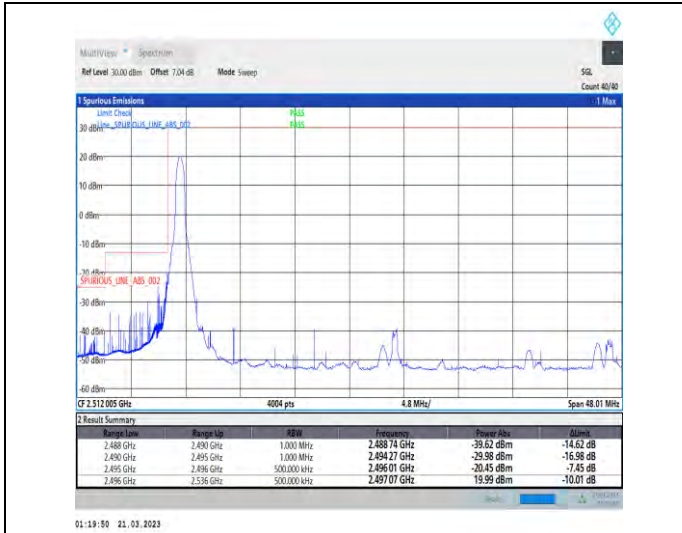
1-N41-30-40-L-1-DFT-PI2BPSK-Edge_1RB_Left-1@0-Ant1-1--PASS-see graph
