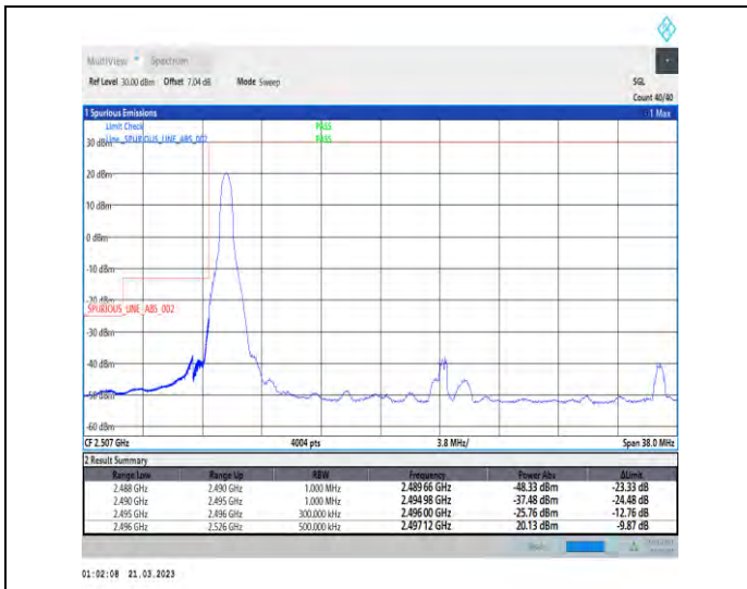
1-N41-30-30-L-1-DFT-PI2BPSK-Edge_1RB_Left-1@0-Ant1-1--PASS-see graph
