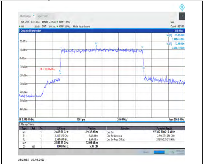
1-N41-30-100-L-7-CP-16QAM-Outer_Full-273@0-Ant t1-97.318-100.800-≤100-PASS
