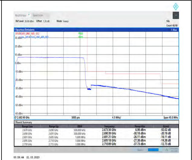
1-N41-30-20-H-6-CP-QPSK-Outer_Full-51@0-Ant1-1--PASS-see graph
