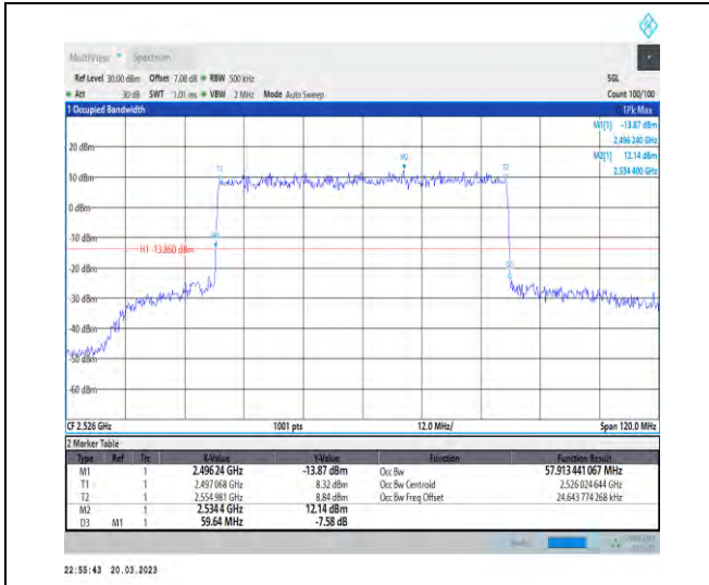
1-N41-30-60-L-3-DFT-16QAM-Outer_Full-162@0-A nt1-57.913-59.640-≤60-PASS
