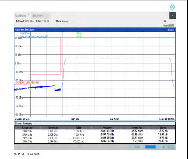
1-N41-30-20-L-6-CP-QPSK-Outer_Full-51@0-Ant1-1--PASS-see graph
