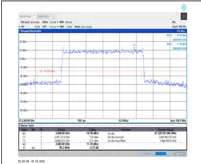
1-N41-30-50-H-8-CP-64QAM-Outer_Full-133@0-Ant 1-47.321-49.200-≤50-PASS
