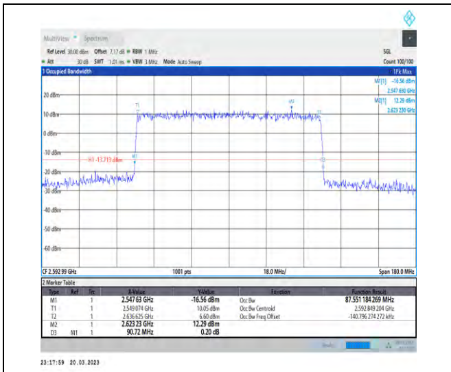
1-N41-30-90-M-8-CP-64QAM-Outer_Full-245@0-An t1-87.551-90.720-<90-PASS
