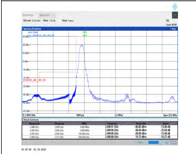
1-N41-30-15-L-4-CP-QPSK-Edge_1RB_Left-1@0-Ant1-1--PASS-see graph
