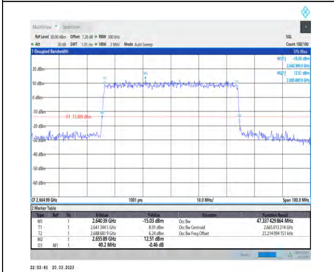
1-N41-30-50-H-6-CP-QPSK-Outer_Full-133@0-Ant1 -47.337-49.200-≤50-PASS
