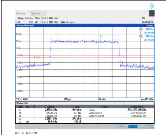
1-N41-30-90-M-6-CP-QPSK-Outer_Full-245@0-Ant 1-87.238-90.900-≤90-PASS
