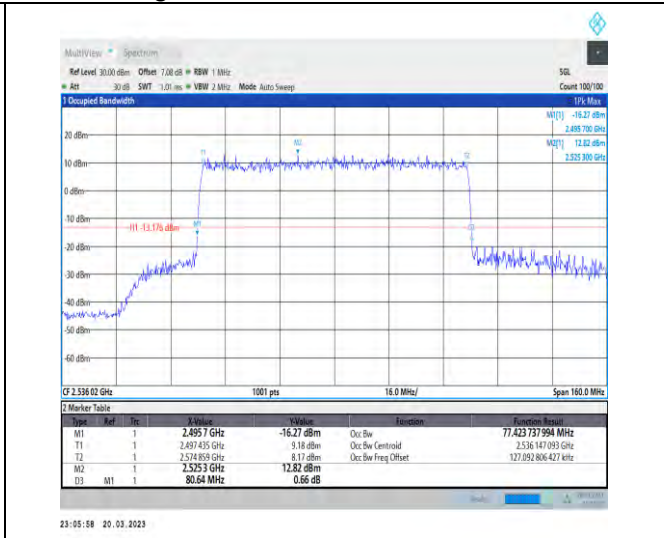
1-N41-30-80-L-9-CP-256QAM-Outer_Full-217@0-An t1-77.424-80.640-≤80-PASS
