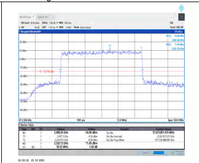
1-N41-30-60-L-8-CP-64QAM-Outer_Full-162@0-Ant 1-57.616-59.520-≤60-PASS
