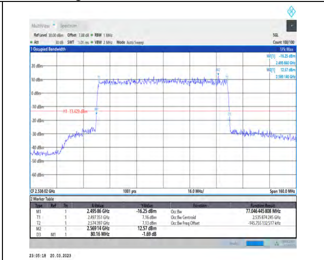
1-N41-30-80-L-5-DFT-256QAM-Outer_Full-216@0-A nt1-77.046-80.160-<80-PASS
