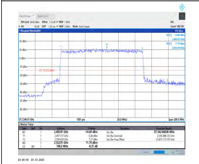
1-N41-30-100-L-8-CP-64QAM-Outer_Full-273@0-Ant nt1-97.343-100.600-≤100-PASS
