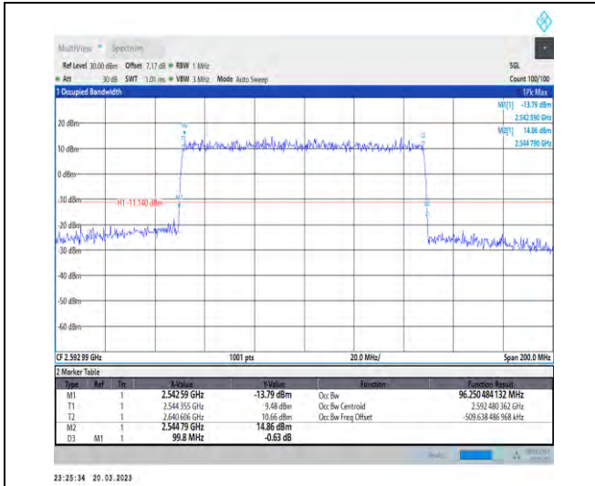
1-N41-30-100-M-1-DFT-QPSK-Outer_Full-270@0-A nt1-96.25-99.800-≤100-PASS
