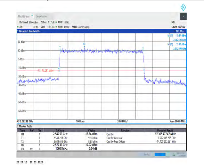
1-N41-30-100-M-6-CP-QPSK-Outer_Full-273@0-Ant 1-97.395-100.800-≤100-PASS
