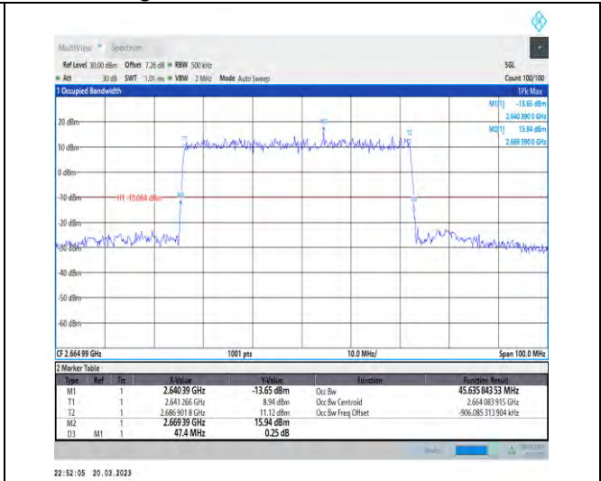
1-N41-30-50-H-1-DFT-QPSK-Outer_Full-128@0-Ant 1-45.636-47.400-≤50-PASS
