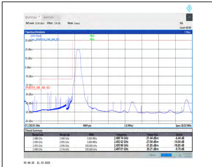
1-N41-30-20-L-1-DFT-PI2BPSK-Edge_1RB_Left-1@0-Ant1-1--PASS-see graph
