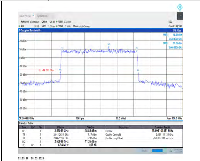
1-N41-30-50-H-5-DFT-256QAM-Outer_Full-128@0-A nt1-45.696-47.400-≤50-PASS
