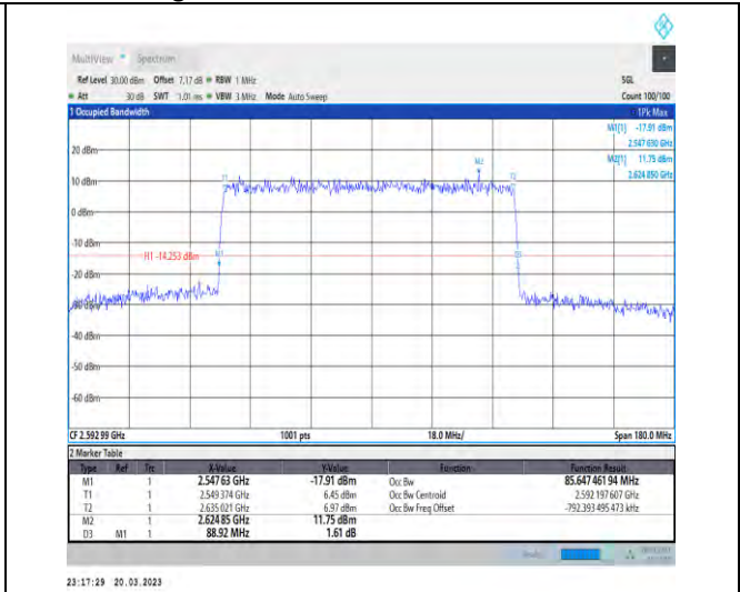
1-N41-30-90-M-5-DFT-256QAM-Outer_Full-240@0-A Ant1-85.647-88.920-≤90-PASS
