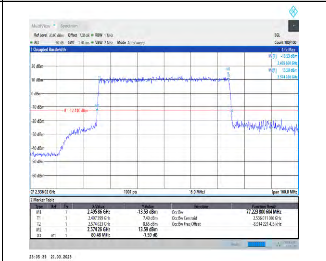
1-N41-30-80-L-7-CP-16QAM-Outer_Full-217@0-Ant 1-77.224-80.480-<80-PASS
