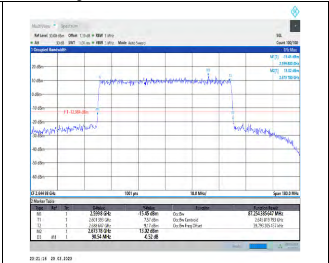
1-N41-30-90-H-8-CP-64QAM-Outer_Full-245@0-Ant 1-87.254-90.540-≤90-PASS
