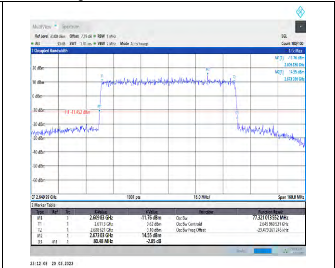
1-N41-30-80-H-7-CP-16QAM-Outer_Full-217@0-Ant 1-77.321-80.480-≤80-PASS
