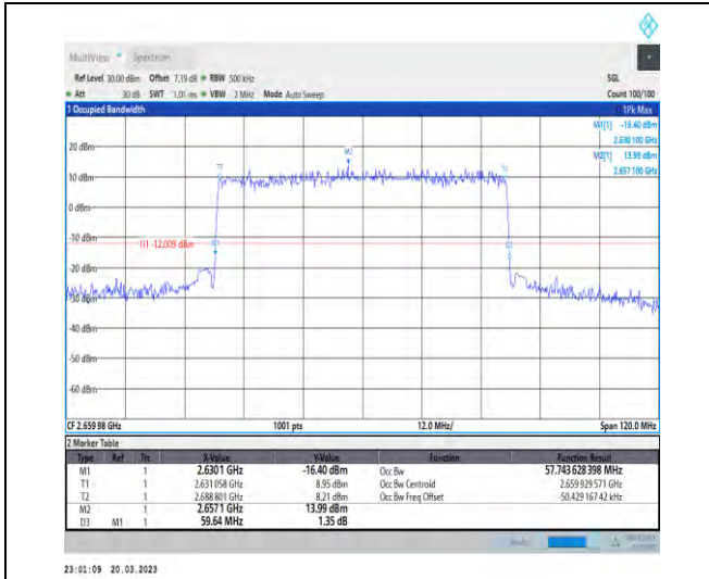
1-N41-30-60-H-1-DFT-QPSK-Outer_Full-162@0-Ant 1-57.744-59.640-≤60-PASS
