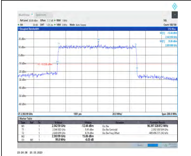
1-N41-30-100-M-3-DFT-16QAM-Outer_Full-270@0-A Ant1-96.397-99.800-≤100-PASS
