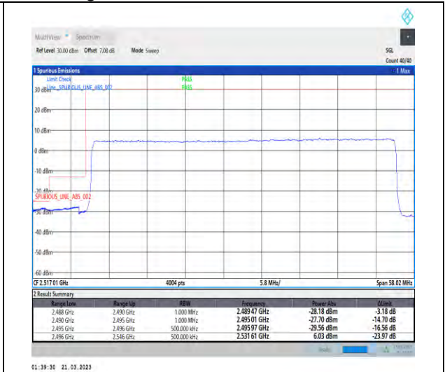
1-N41-30-50-L-3-DFT-PI2BPSK-Outer_Full-128@0-Ant1-1--PASS-see graph
