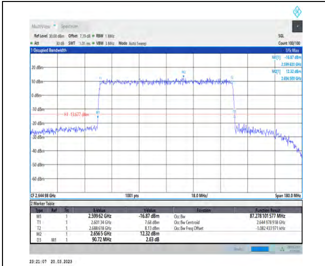
1-N41-30-90-H-7-CP-16QAM-Outer_Full-245@0-Ant 1-87.278-90.720-≤90-PASS
