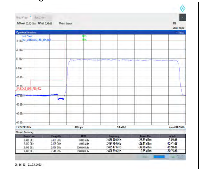
1-N41-30-20-L-3-DFT-PI2BPSK-Outer_Full-50@0-Ant1-1--PASS-see graph
