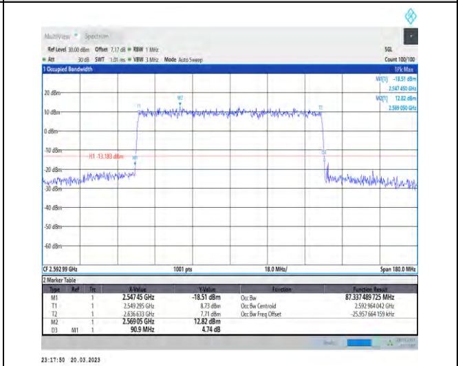
1-N41-30-90-M-7-CP-16QAM-Outer_Full-245@0-Ant 1-87.337-90.900-≤90-PASS
