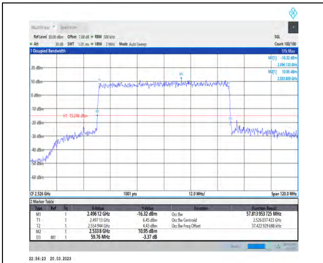
1-N41-30-60-L-7-CP-16QAM-Outer_Full-162@0-Ant 1-57.814-59.760-≤60-PASS
