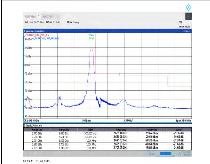
1-N41-30-15-H-5-CP-QPSK-Edge_1RB_Right-1@37-Ant1-1--PASS-see graph
