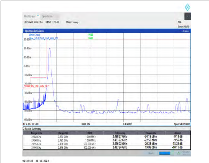
1-N41-30-50-L-1-DFT-PI2BPSK-Edge_1RB_Left-1@0-Ant1-1--PASS-see graph
