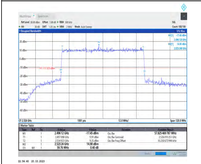
1-N41-30-60-L-1-DFT-QPSK-Outer_Full-162@0-Ant 1-57.825-59.760-≤60-PASS
