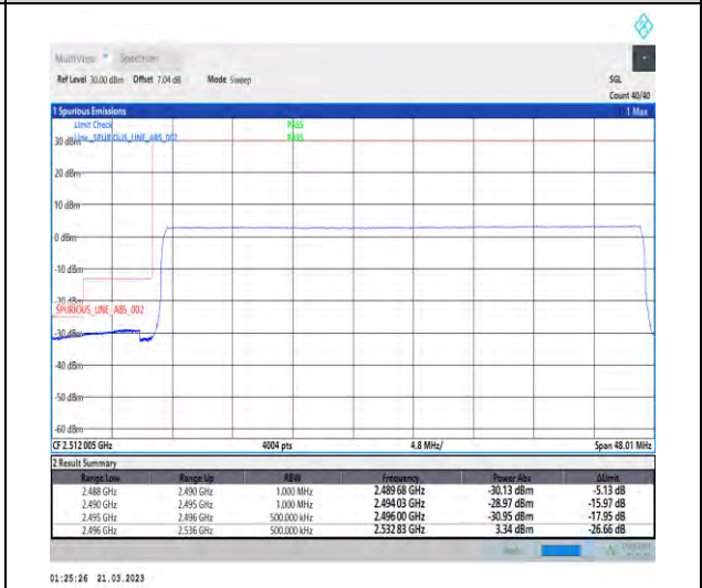
1-N41-30-40-L-6-CP-QPSK-Outer_Full-106@0-Ant1-1--PASS-see graph
