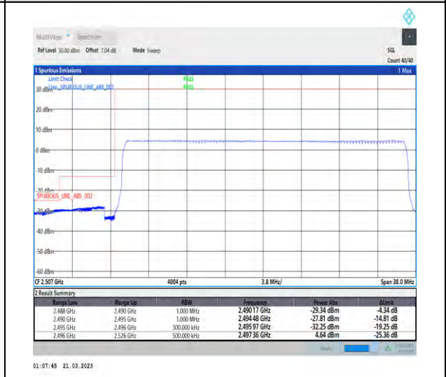
1-N41-30-30-L-6-CP-QPSK-Outer_Full-78@0-Ant1-1--PASS-see graph
