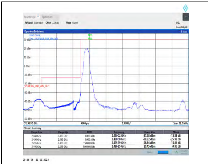
1-N41-30-15-L-1-DFT-PI2BPSK-Edge_1RB_Left-1@0-Ant1-1--PASS-see graph
