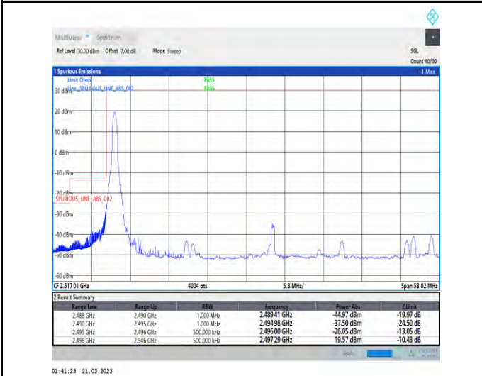
1-N41-30-50-L-4-CP-QPSK-Edge_1RB_Left-1@0-Ant1-1--PASS-see graph
