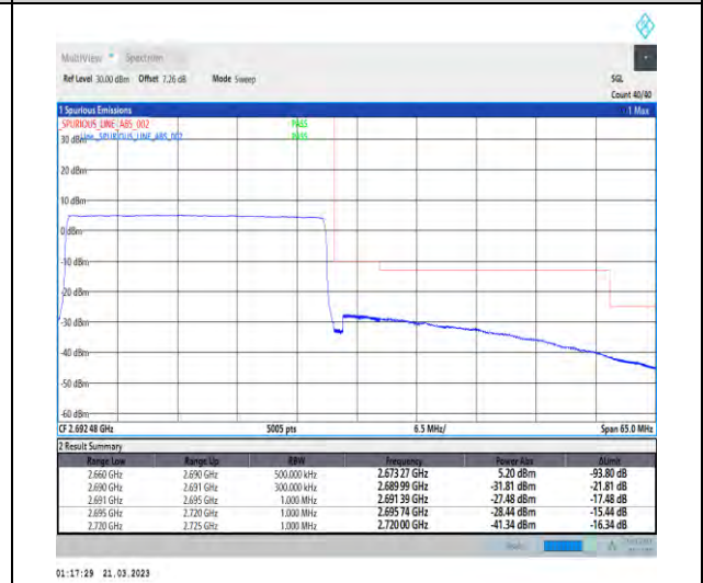
1-N41-30-30-H-6-CP-QPSK-Outer_Full-78@0-Ant1-1--PASS-see graph
