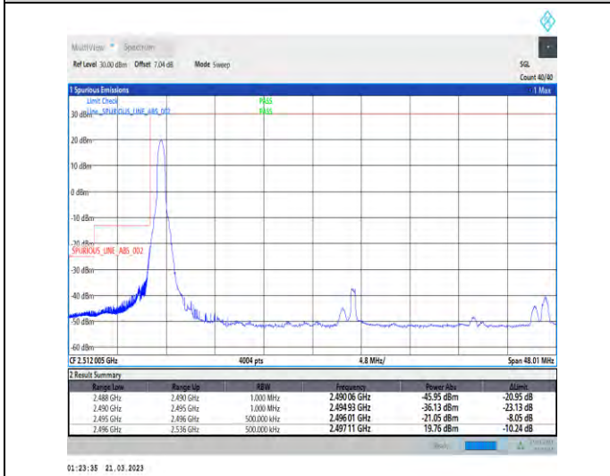
1-N41-30-40-L-4-CP-QPSK-Edge_1RB_Left-1@0-Ant1-1--PASS-see graph
