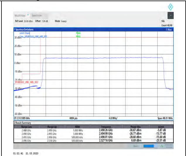
1-N41-30-40-L-3-DFT-PI2BPSK-Outer_Full-100@0-Ant1-1--PASS-see graph
