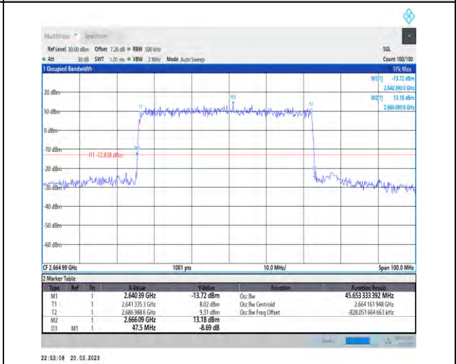
1-N41-30-50-H-3-DFT-16QAM-Outer_Full-128@0-Ant t1-45.653-47.500-≤50-PASS
