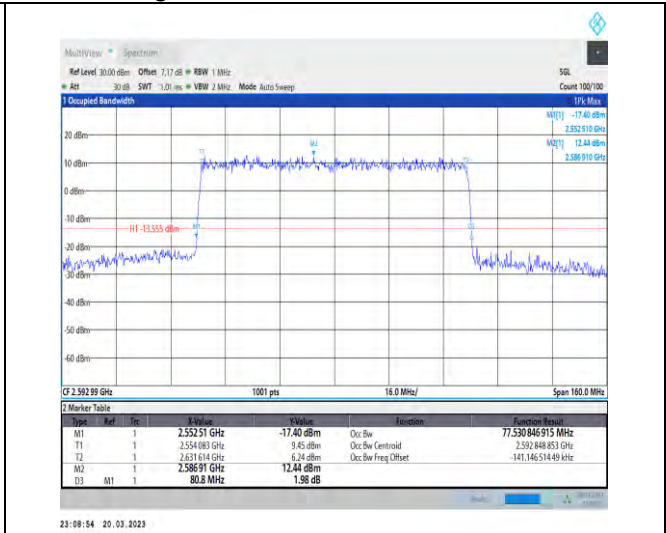
1-N41-30-80-M-8-CP-64QAM-Outer_Full-217@0-Ant 1-77.531-80.800-<80-PASS
