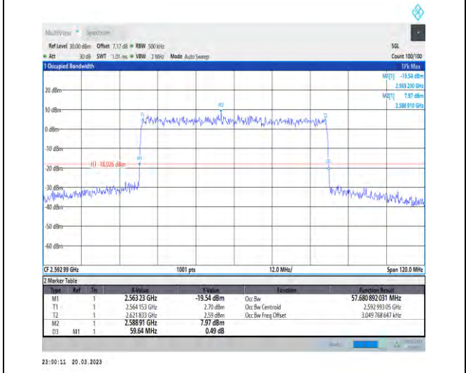
1-N41-30-60-M-9-CP-256QAM-Outer_Full-162@0-Ant nt1-57.681-59.640-≤60-PASS
