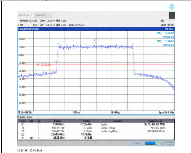
1-N41-30-90-H-4-DFT-64QAM-Outer_Full-240@0-A t1-85.703-88.560-≤90-PASS
