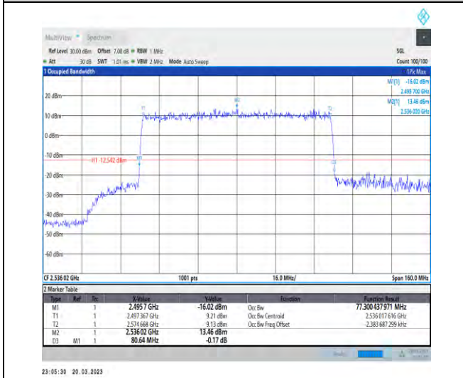
1-N41-30-80-L-6-CP-QPSK-Outer_Full-217@0-Ant1 -77.3-80.640-<80-PASS
