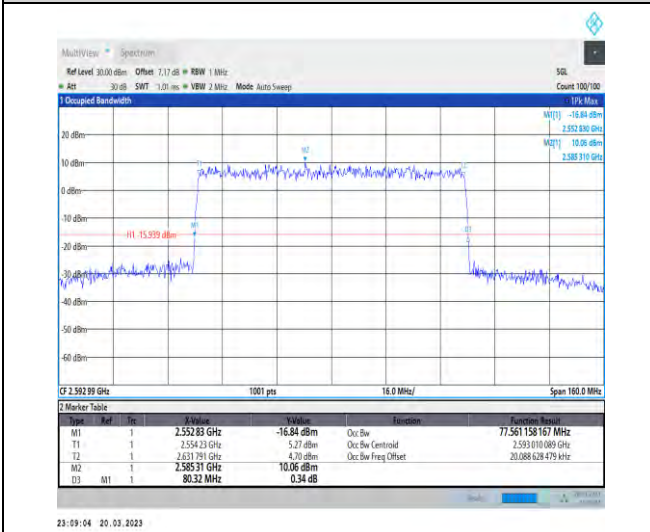
1-N41-30-80-M-9-CP-256QAM-Outer_Full-217@0-A nt1-77.561-80.320-<80-PASS
