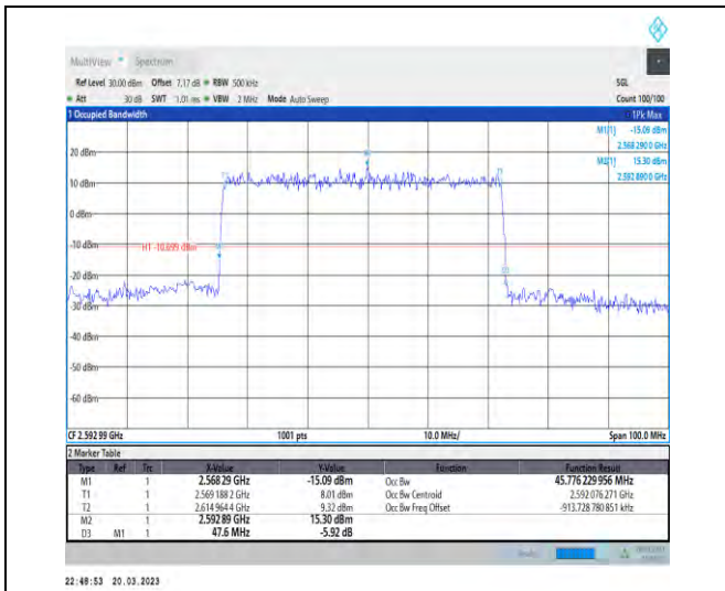
1-N41-30-50-M-1-DFT-QPSK-Outer_Full-128@0-Ant 1-45.776-47.600-≤50-PASS
