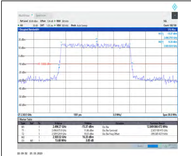
1-N41-30-15-L-2-DFT-PI2BPSK-Outer_Full-36@0-Ant1-12.849-13.680-≤15-PASS
