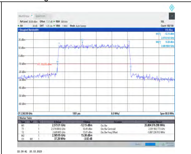
1-N41-30-40-M-1-DFT-QPSK-Outer_Full-100@0-Ant 1-35.804-37.280-≤40-PASS
