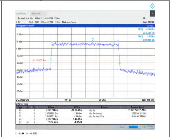
1-N41-30-40-M-9-CP-256QAM-Outer_Full-106@0-A nt1-37.973-39.520-<40-PASS
