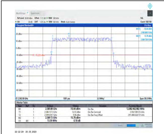
1-N41-30-15-M-1-DFT-QPSK-Outer_Full-36@0-Ant1 -12.882-13.590-≤15-PASS
