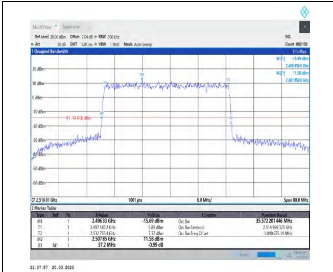
1-N41-30-40-L-5-DFT-256QAM-Outer_Full-100@0-Ant1-35.572-37.200-<=40-PASS
