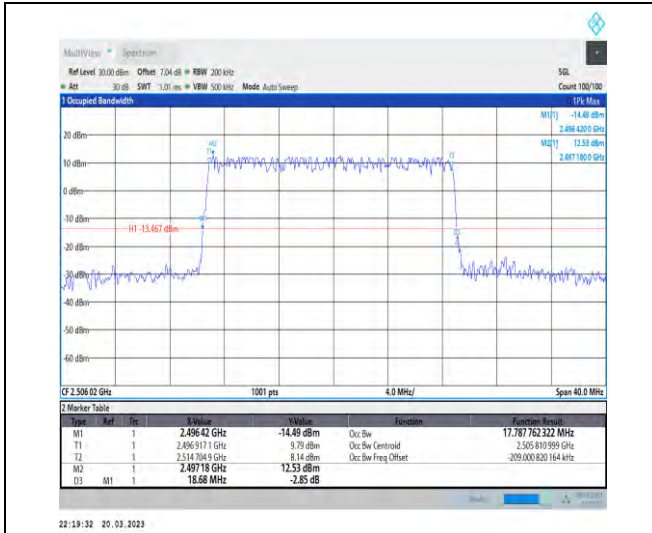
1-N41-30-20-L-3-DFT-16QAM-Outer_Full-50@0-Ant 1-17.788-18.680-≤20-PASS
