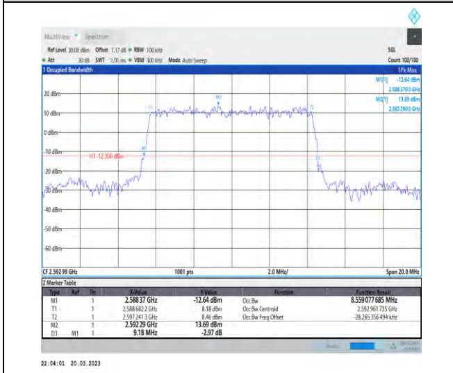
1-N41-30-10-M-2-DFT-16QAM-Outer_Full-24@0-A nt1-8.559-9.180-≤10-PASS
