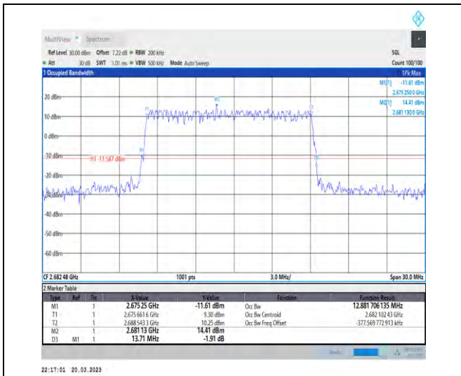
1-N41-30-15-H-4-DFT-64QAM-Outer_Full-36@0-Ant 1-12.882-13.710-≤15-PASS
