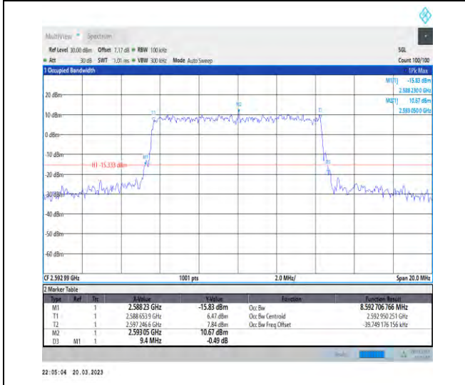
1-N41-30-10-M-6-CP-QPSK-Outer_Full-24@0-Ant1- 8.593-9.400-≤10-PASS
