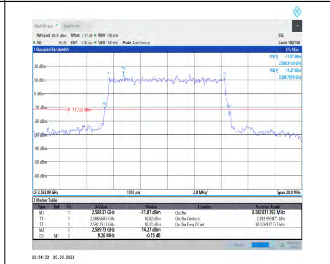
1-N41-30-10-M-3-DFT-16QAM-Outer_Full-24@0-Ant 1-8.583-9.260-≤10-PASS
