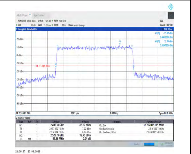
1-N41-30-40-L-8-CP-64QAM-Outer_Full-106@0-Ant1-37.762-39.360-<=40-PASS
