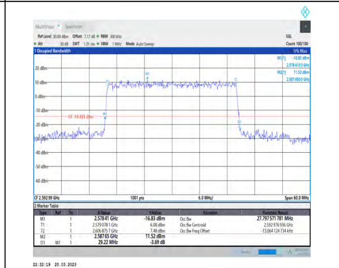
1-N41-30-30-M-6-CP-QPSK-Outer_Full-78@0-Ant1- 27.798-29.220-<30-PASS
