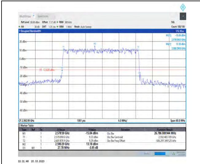
1-N41-30-30-M-3-DFT-16QAM-Outer_Full-75@0-An t1-26.786-27.780-<30-PASS
