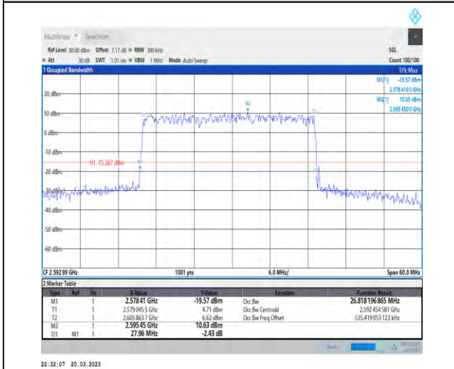
1-N41-30-30-M-5-DFT-256QAM-Outer_Full-75@0-A nt1-26.818-27.960-<30-PASS
