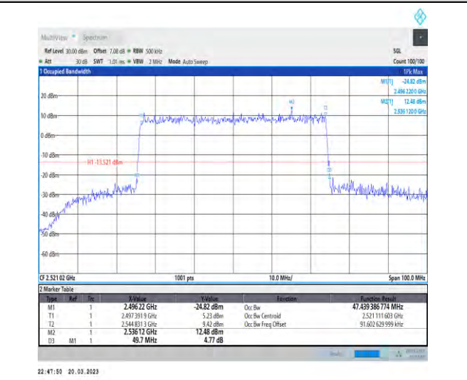
1-N41-30-50-L-9-CP-256QAM-Outer_Full-133@0-Ant 1-47.439-49.700-≤50-PASS
