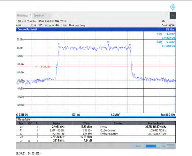
1-N41-30-30-L-3-DFT-16QAM-Outer_Full-75@0-Ant 1-26.75-28.140-≤30-PASS
