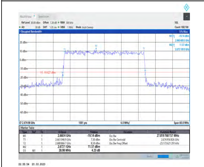
1-N41-30-30-H-8-CP-64QAM-Outer_Full-78@0-Ant1-27.82-28.980-<=30-PASS
