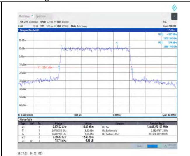
1-N41-30-15-H-5-DFT-256QAM-Outer_Full-36@0-Ant t1-12.846-13.710-≤15-PASS
