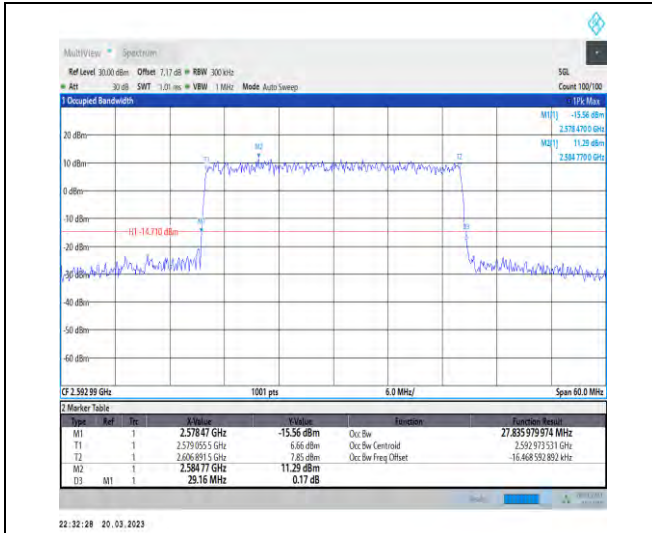
1-N41-30-30-M-7-CP-16QAM-Outer_Full-78@0-Ant 1-27.836-29.160-≤30-PASS
