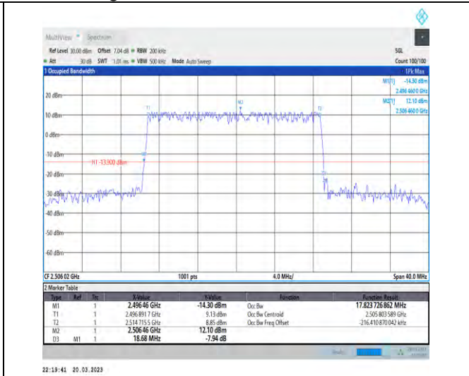
1-N41-30-20-L-4-DFT-64QAM-Outer_Full-50@0-Ant 1-17.824-18.680-≤20-PASS
