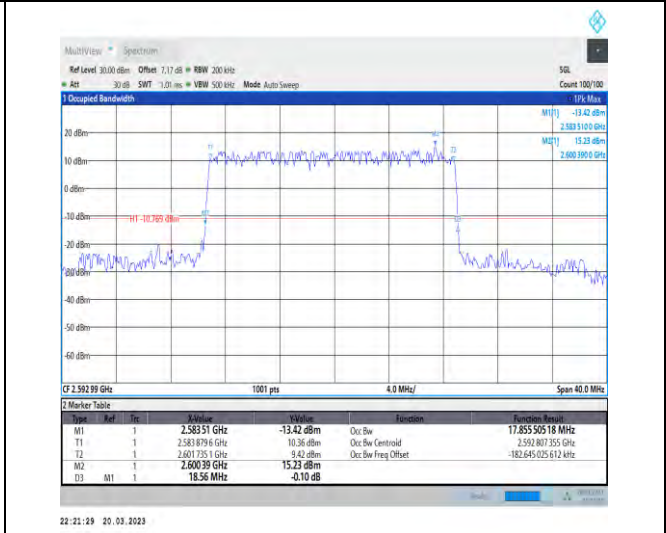
1-N41-30-20-M-1-DFT-QPSK-Outer_Full-50@0-Ant1 -17.856-18.560-≤20-PASS
