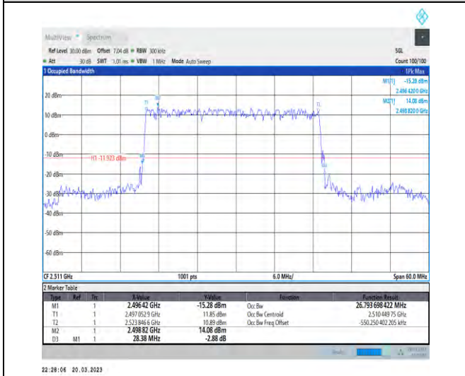
1-N41-30-30-L-2-DFT-PI2BPSK-Outer_Full-75@0-A nt1-26.794-28.380-≤30-PASS
