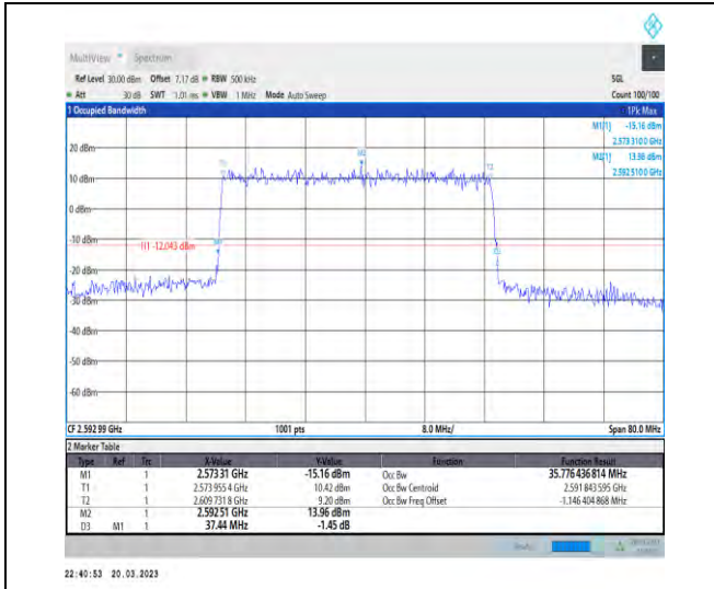
1-N41-30-40-M-4-DFT-64QAM-Outer_Full-100@0-A nt1-35.776-37.440-≤40-PASS
