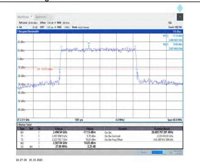
1-N41-30-30-L-1-DFT-QPSK-Outer_Full-75@0-Ant1 26.694-27.840-≤30-PASS
