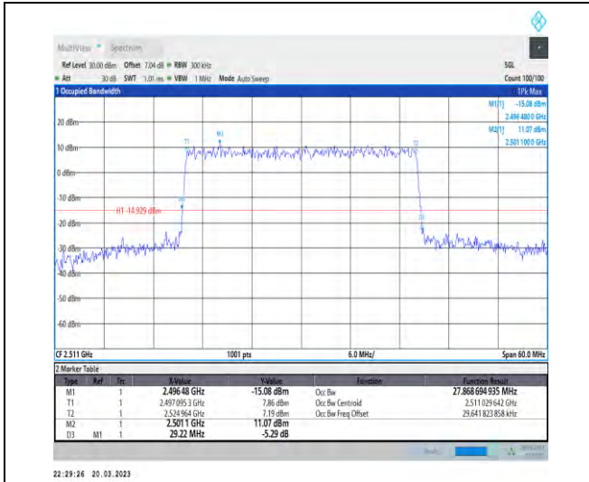
1-N41-30-30-L-8-CP-64QAM-Outer_Full-78@0-Ant1 -27.869-29.220-≤30-PASS
