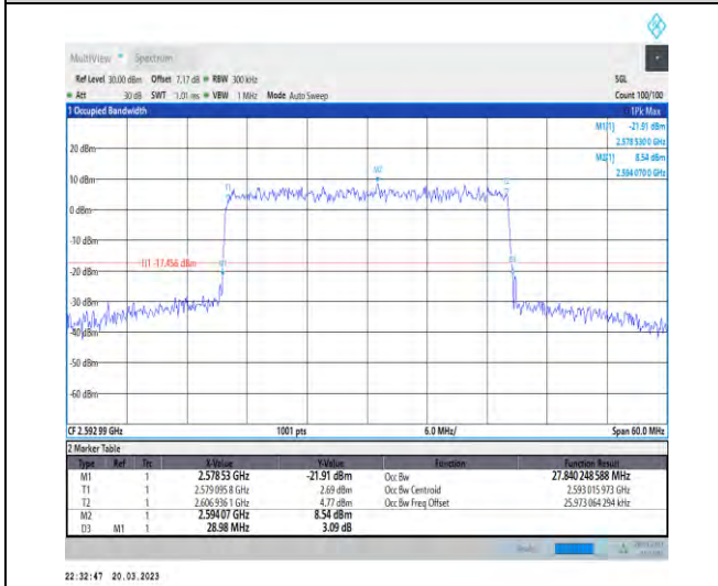
1-N41-30-30-M-9-CP-256QAM-Outer_Full-78@0-Ant t1-27.84-28.980-≤30-PASS
