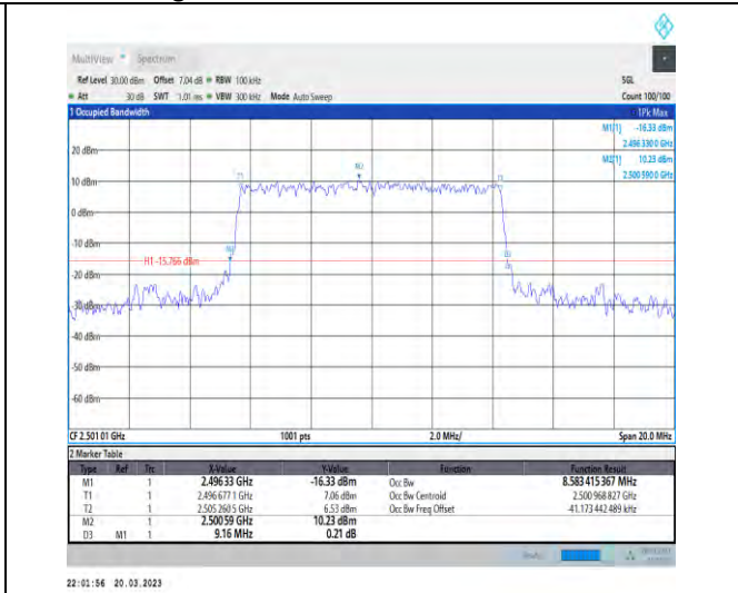
1-N41-30-10-L-6-CP-QPSK-Outer_Full-24@0-Ant1-8 .583-9.160-≤10-PASS
