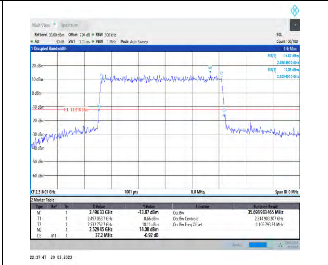
1-N41-30-40-L-4-DFT-64QAM-Outer_Full-100@0-Ant 1-35.699-37.200-≤40-PASS
