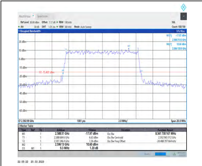
1-N41-30-10-M-8-CP-64QAM-Outer_Full-24@0-Ant 1-8.562-9.300-≤10-PASS
