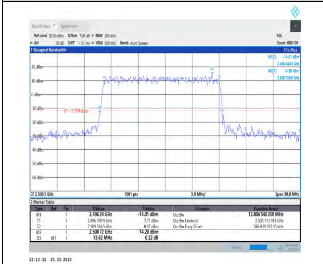
1-N41-30-15-L-4-DFT-64QAM-Outer_Full-36@0-Ant1-12.807-13.620-≤15-PASS
