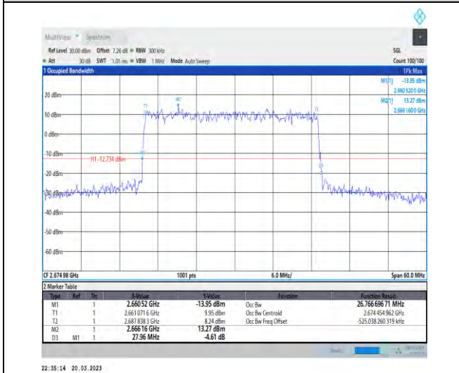
1-N41-30-30-H-4-DFT-64QAM-Outer_Full-75@0-Ant 1-26.767-27.960-≤30-PASS
