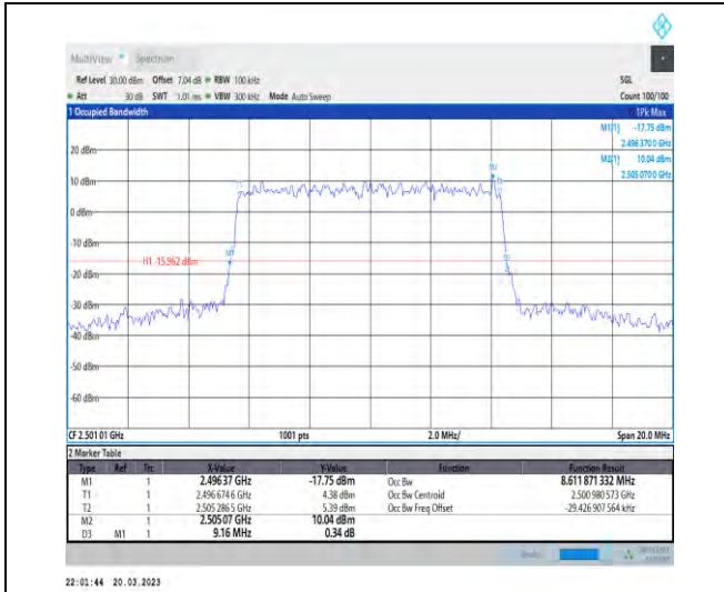
1-N41-30-10-L-5-DFT-256QAM-Outer_Full-24@0-A nt1-8.612-9.160-≤10-PASS
