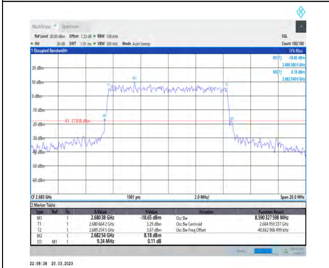
1-N41-30-10-H-9-CP-256QAM-Outer_Full-24@0-Ant 1-8.59-9.240≤10-PASS
