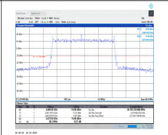
1-N41-30-30-H-1-DFT-QPSK-Outer_Full-75@0-Ant1 26.706-28.200-≤30-PASS
