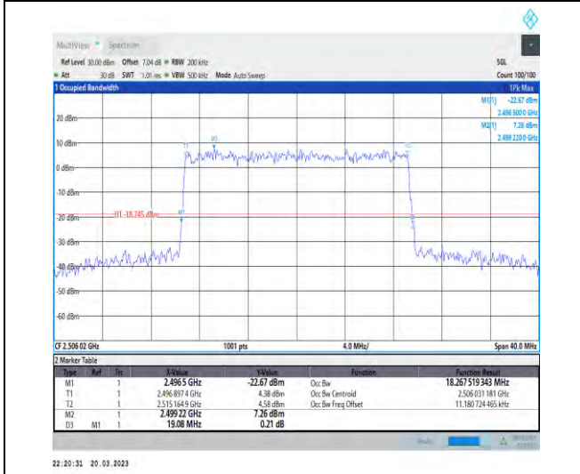
1-N41-30-20-L-9-CP-256QAM-Outer_Full-51@0-Ant 1-18.268-19.080-≤20-PASS
