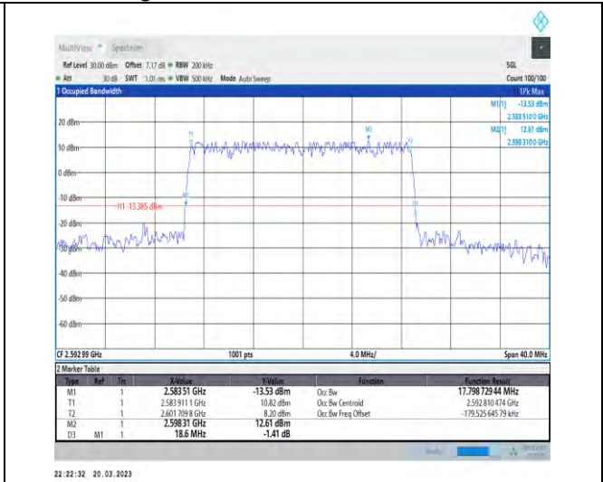
1-N41-30-20-M-3-DFT-16QAM-Outer_Full-50@0-Ant 1-17.799-18.600-≤20-PASS
