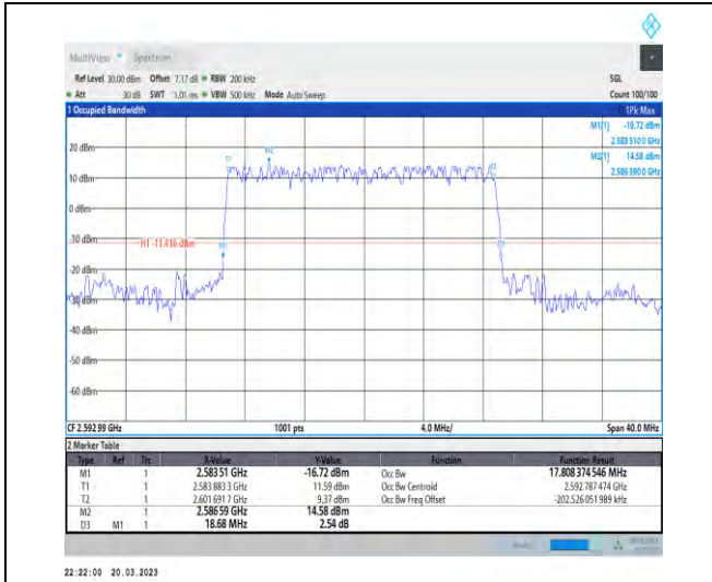
1-N41-30-20-M-2-DFT-PI2BPSK-Outer_Full-50@0-A nt1-17.808-18.680-≤20-PASS
