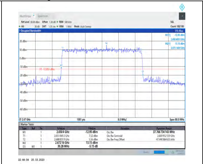
1-N41-30-40-H-8-CP-64QAM-Outer_Full-106@0-Ant 1-37.767-39.280-≤40-PASS
