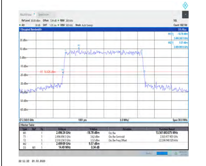
1-N41-30-15-L-9-CP-256QAM-Outer_Full-38@0-Ant1-1-13.562-14.490-≤15-PASS
