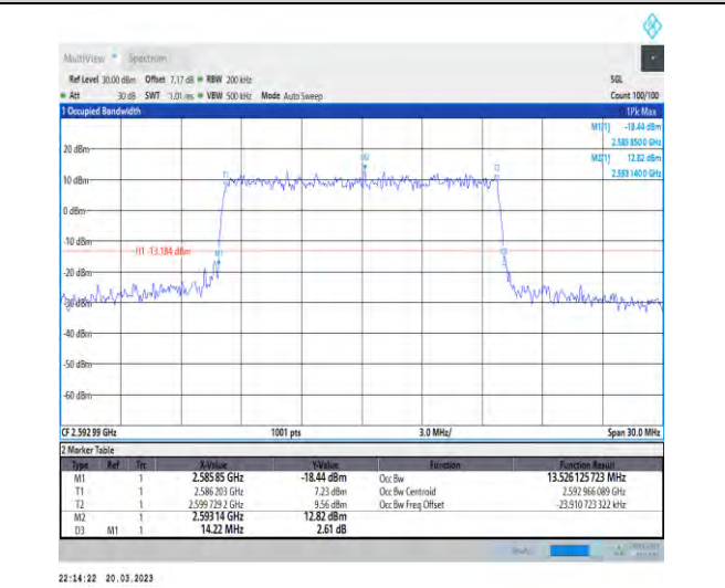
1-N41-30-15-M-8-CP-64QAM-Outer_Full-38@0-Ant1 -13.526-14.220-≤15-PASS
