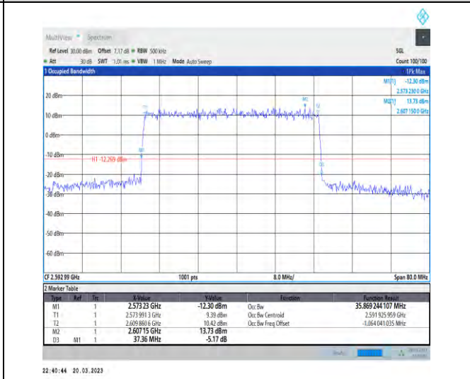
1-N41-30-40-M-3-DFT-16QAM-Outer_Full-100@0-A nt1-35.869-37.360-≤40-PASS
