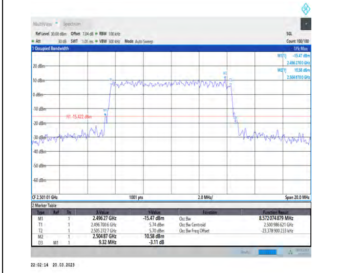
1-N41-30-10-L-8-CP-64QAM-Outer_Full-24@0-Ant1- 8.572-9.320-≤10-PASS
