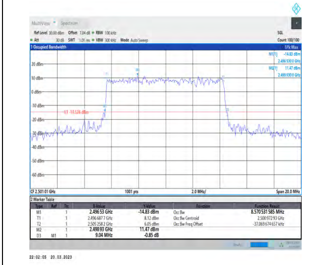
1-N41-30-10-L-7-CP-16QAM-Outer_Full-24@0-Ant1 -8.571-9.040-≤10-PASS
