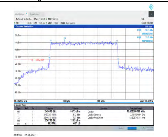
1-N41-30-50-L-7-CP-16QAM-Outer_Full-133@0-Ant 1-47.422-49.300-≤50-PASS
