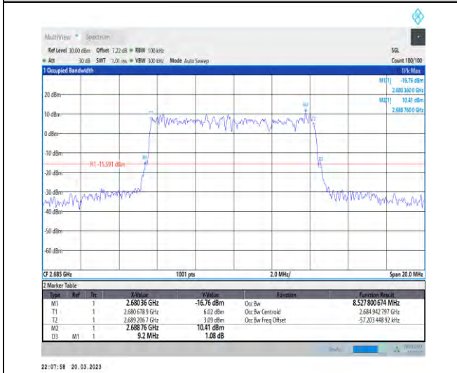
1-N41-30-10-H-5-DFT-256QAM-Outer_Full-24@0-A nt1-8.528-9.200-≤10-PASS
