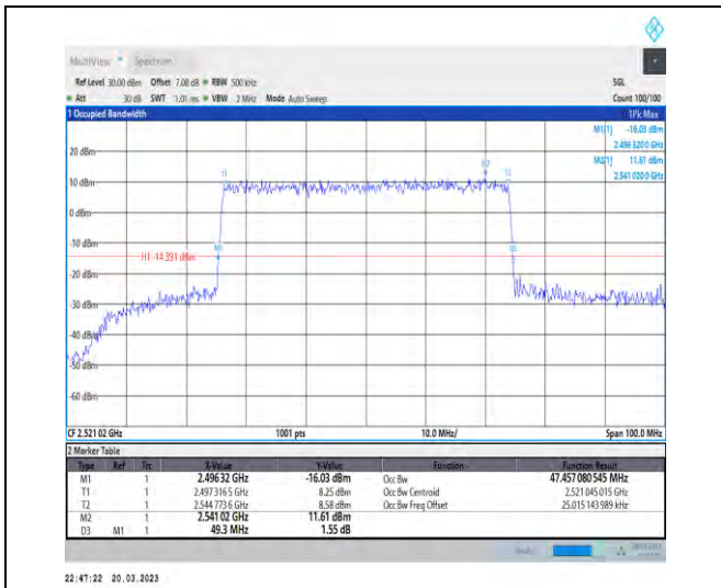
1-N41-30-50-L-6-CP-QPSK-Outer_Full-133@0-Ant1 -47.457-49.300-≤50-PASS
