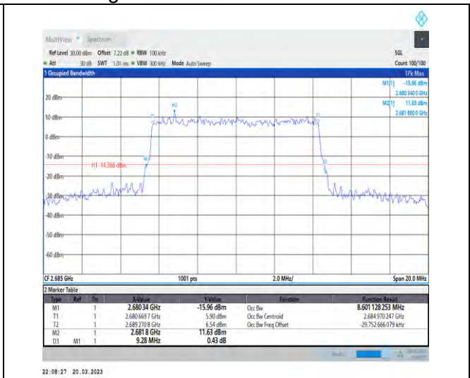
1-N41-30-10-H-8-CP-64QAM-Outer_Full-24@0-Ant1 -8.601-9.280≤10-PASS
