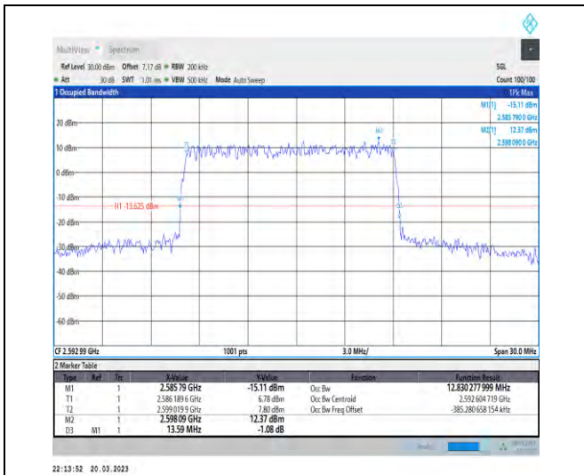
1-N41-30-15-M-5-DFT-256QAM-Outer_Full-36@0-A nt1-12.83-13.590-≤15-PASS
