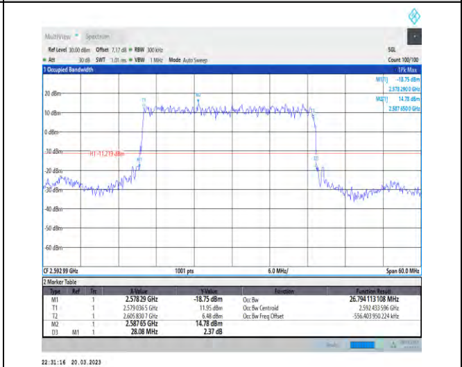
1-N41-30-30-M-2-DFT-PI2BPSK-Outer_Full-75@0-Ant1 -26.794-28.080-≤30-PASS
