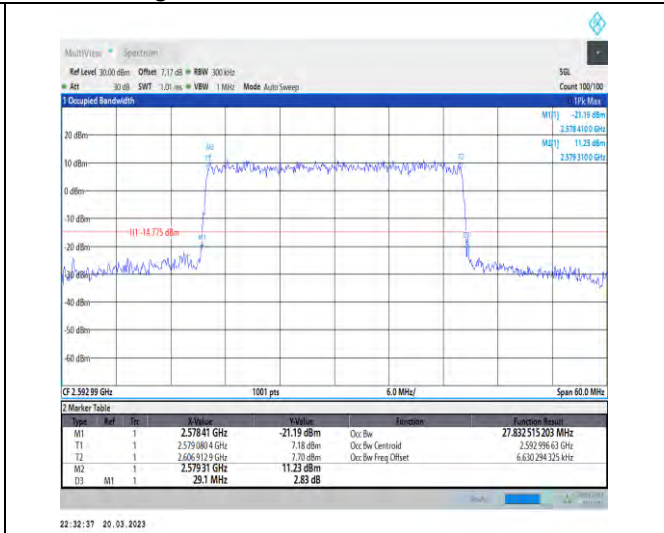
1-N41-30-30-M-8-CP-64QAM-Outer_Full-78@0-Ant1 -27.833-29.100-≤30-PASS
