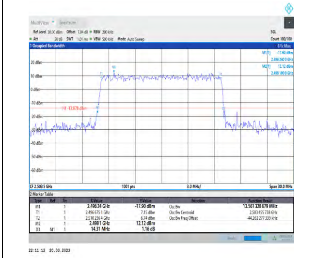
1-N41-30-15-L-8-CP-64QAM-Outer_Full-38@0-Ant1-13.561-14.310-≤15-PASS
