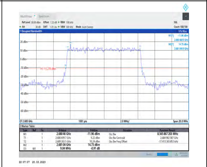
1-N41-30-10-H-2-DFT-PI2BPSK-Outer_Full-24@0-A nt1-8.566-9.040-≤10-PASS
