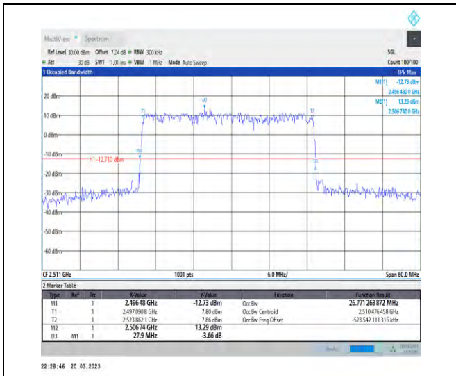
1-N41-30-30-L-4-DFT-64QAM-Outer_Full-75@0-Ant 1-26.771-27.900-≤30-PASS
