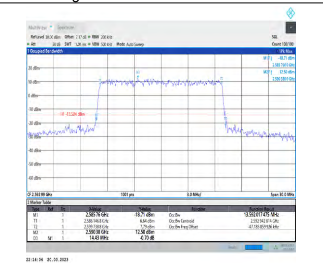
1-N41-30-15-M-6-CP-QPSK-Outer_Full-38@0-Ant1- 13.592-14.430-≤15-PASS
