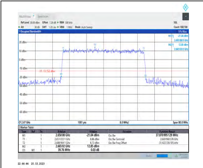
1-N41-30-40-H-7-CP-16QAM-Outer_Full-106@0-Ant 1-37.871-39.760-≤40-PASS
