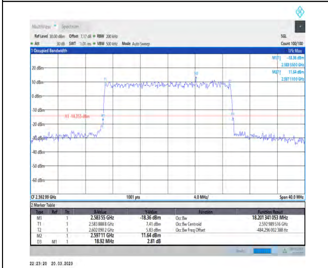
1-N41-30-20-M-8-CP-64QAM-Outer_Full-51@0-Ant1-18.201-18.920-≤20-PASS
