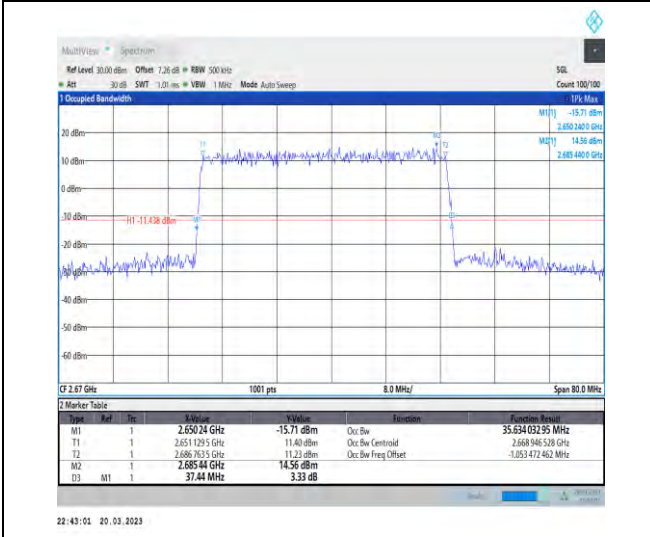
1-N41-30-40-H-1-DFT-QPSK-Outer_Full-100@0-Ant 1-35.634-37.440-<40-PASS
