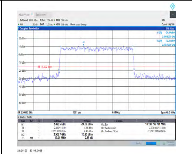
1-N41-30-20-L-6-CP-QPSK-Outer_Full-51@0-Ant1-1 8.194-19.040-≤20-PASS
