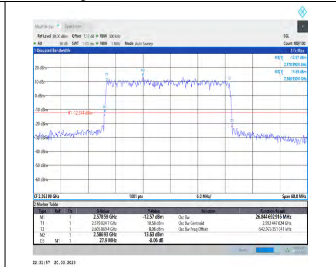
1-N41-30-30-M-4-DFT-64QAM-Outer_Full-75@0-Ant 1-26.845-27.900-<30-PASS
