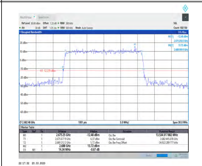
1-N41-30-15-H-7-CP-16QAM-Outer_Full-38@0-Ant1 -13.534-14.340-≤15-PASS
