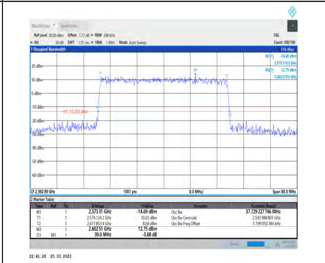
1-N41-30-40-M-7-CP-16QAM-Outer_Full-106@0-Ant 1-37.729-39.600-≤40-PASS
