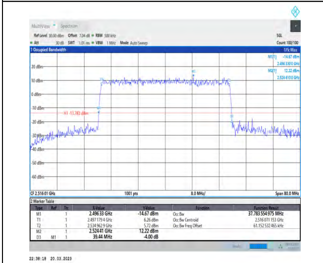
1-N41-30-40-L-7-CP-16QAM-Outer_Full-106@0-Ant1-37.784-39.440-<=40-PASS
