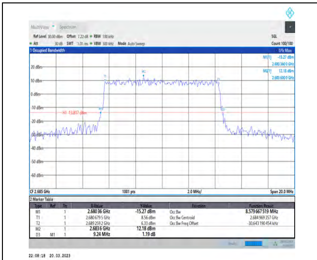
1-N41-30-10-H-7-CP-16QAM-Outer_Full-24@0-Ant1 -8.58-9.240≤10-PASS
