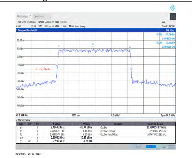
1-N41-30-30-L-5-DFT-256QAM-Outer_Full-75@0-An t1-26.79-27.960-≤30-PASS
