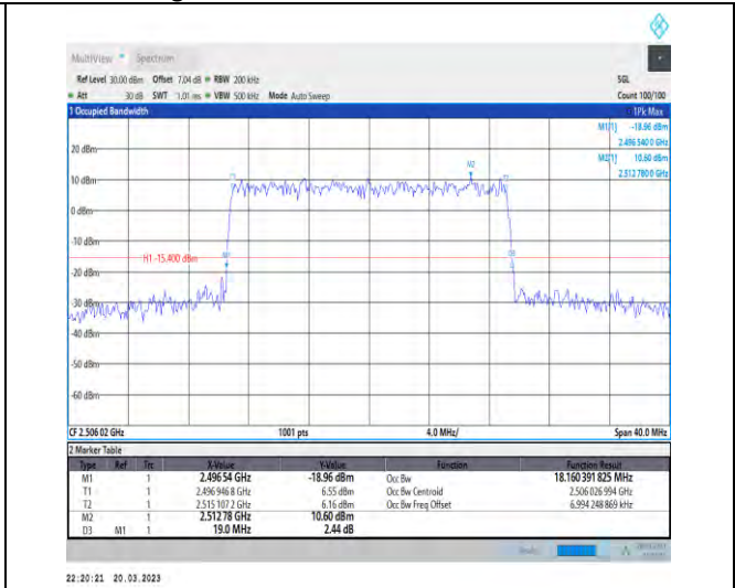
1-N41-30-20-L-8-CP-64QAM-Outer_Full-51@0-Ant1 18.16-19.000-≤20-PASS
