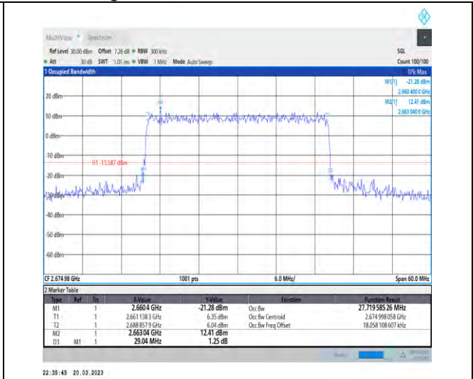
1-N41-30-30-H-7-CP-16QAM-Outer_Full-78@0-Ant1-27.72-29.040-<=30-PASS
