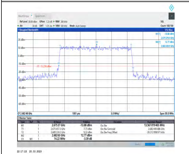
1-N41-30-15-H-6-CP-QPSK-Outer_Full-38@0-Ant1 13.567-14.220-≤15-PASS
