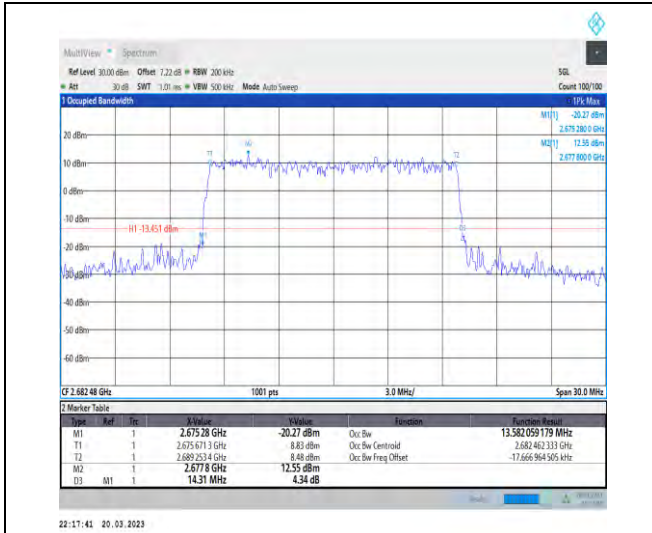
1-N41-30-15-H-8-CP-64QAM-Outer_Full-38@0-Ant1 -13.582-14.310-≤15-PASS
