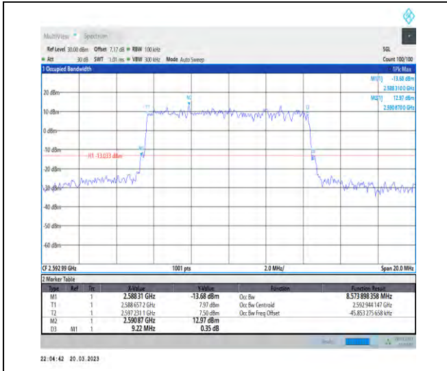
1-N41-30-10-M-4-DFT-64QAM-Outer_Full-24@0-An t1-8.574-9.220-≤10-PASS
