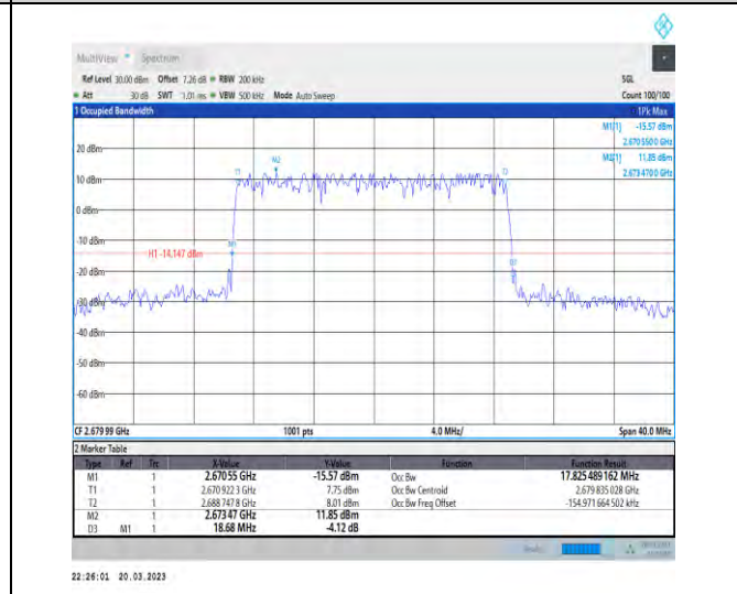
1-N41-30-20-H-4-DFT-64QAM-Outer_Full-50@0-Ant1 1-17.825-18.680-≤20-PASS
