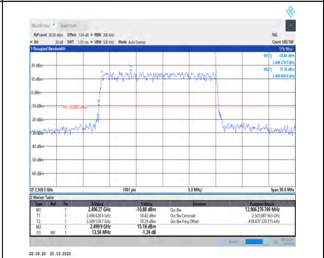
1-N41-30-15-L-1-DFT-QPSK-Outer_Full-36@0-Ant1 12.906-13.560≤15-PASS
