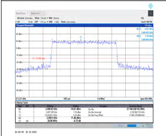
1-N41-30-30-L-6-CP-QPSK-Outer_Full-78@0-Ant1- 27.746-28.980-≤30-PASS
