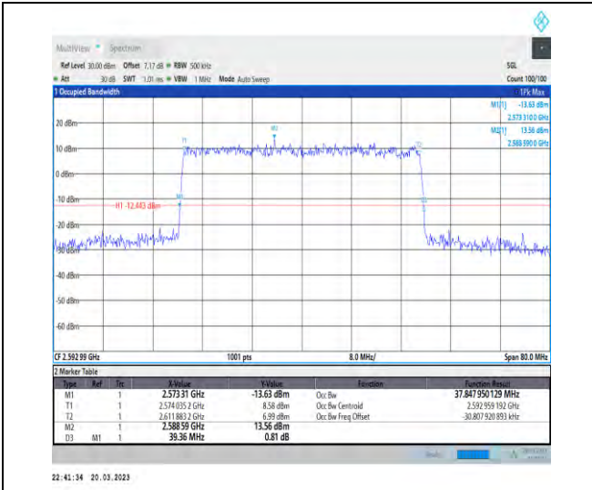
1-N41-30-40-M-8-CP-64QAM-Outer_Full-106@0-An t1-37.848-39.360-<40-PASS
