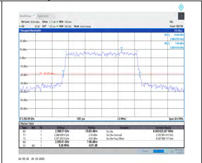
1-N41-30-10-M-9-CP-256QAM-Outer_Full-24@0-Ant 1-8.565-9.260-≤10-PASS
