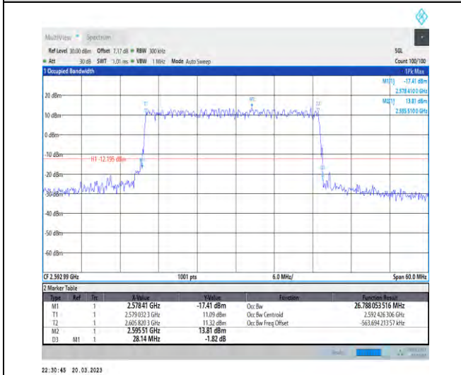
1-N41-30-30-M-1-DFT-QPSK-Outer_Full-75@0-Ant1 -26.788-28.140-≤30-PASS
