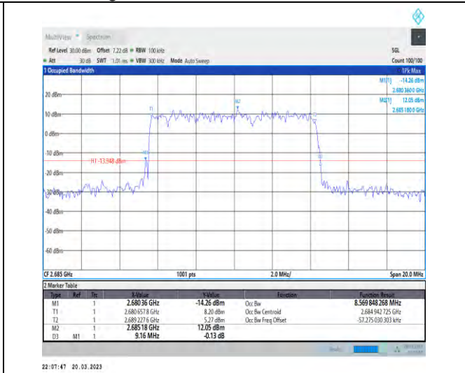
1-N41-30-10-H-4-DFT-64QAM-Outer_Full-24@0-Ant 1-8.57-9.160-≤10-PASS
