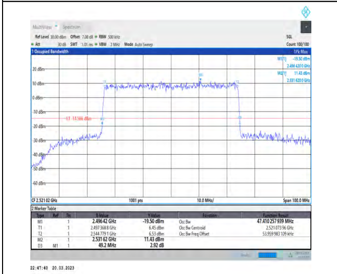
1-N41-30-50-L-8-CP-64QAM-Outer_Full-133@0-Ant 1-47.41-49.200-≤50-PASS
