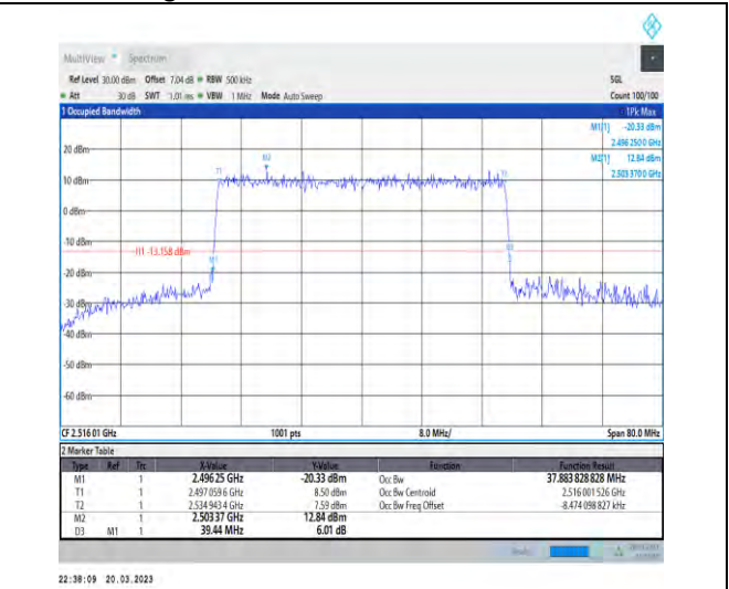
1-N41-30-40-L-6-CP-QPSK-Outer_Full-106@0-Ant1-37.884-39.440-<=40-PASS
