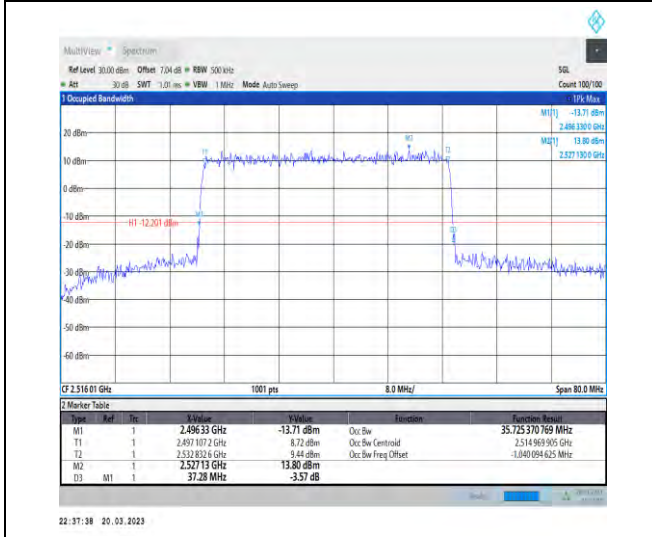
1-N41-30-40-L-3-DFT-16QAM-Outer_Full-100@0-Ant 1-35.725-37.280-≤40-PASS
