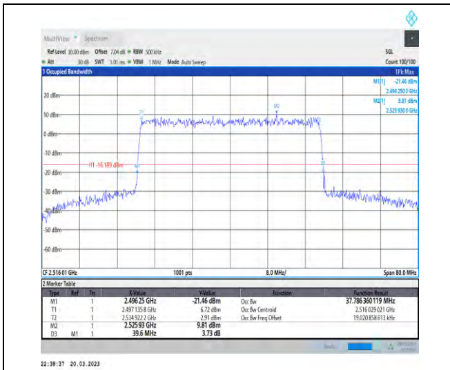
1-N41-30-40-L-9-CP-256QAM-Outer_Full-106@0-A nt1-37.786-39.600-≤40-PASS
