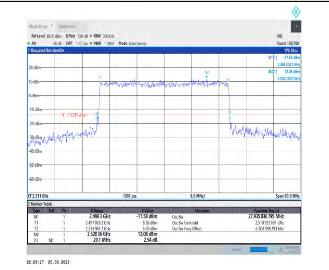
1-N41-30-30-L-7-CP-16QAM-Outer_Full-78@0-Ant1- 27.935-29.100-≤30-PASS
