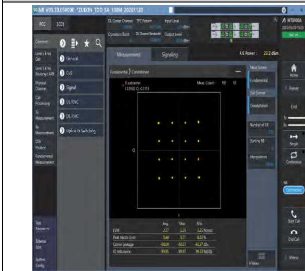
1-N41-30-100-M-3-DFT-16QAM-Outer_Full-270@0-Ant1-see graph-PASS
