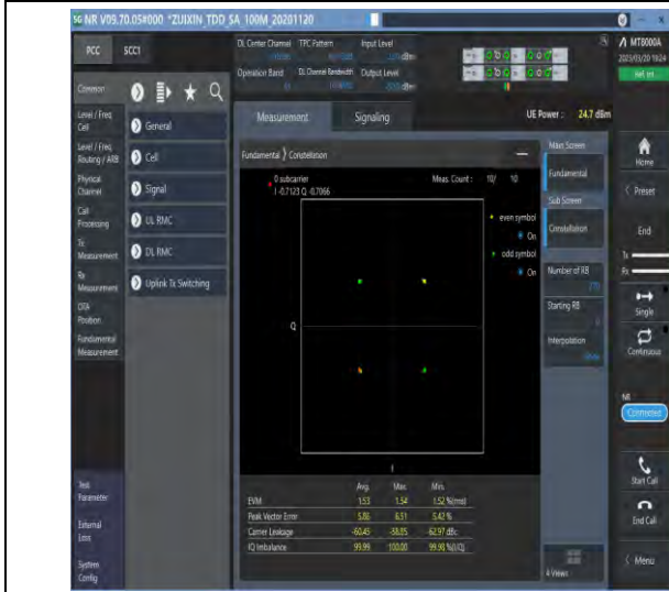
1-N41-30-100-M-1-DFT-PI2BPSK-Outer_Full-270@0-Ant1-see graph-PASS
