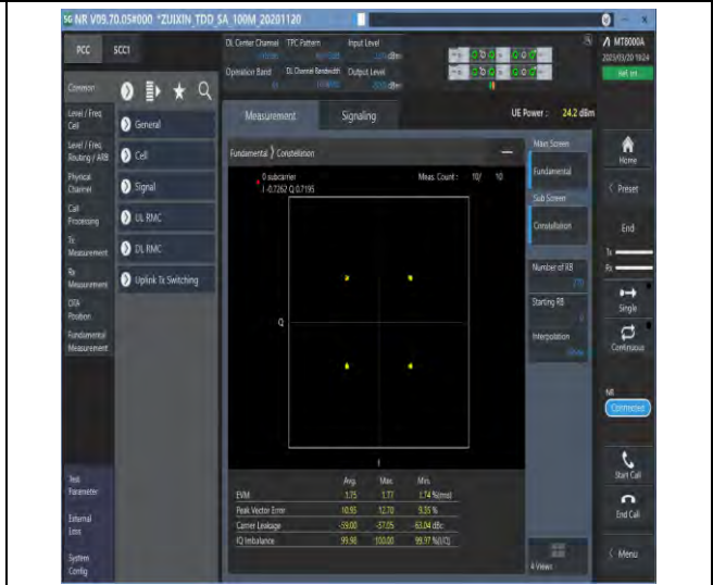
1-N41-30-100-M-2-DFT-QPSK-Outer_Full-270@0-Ant1-see graph-PASS
