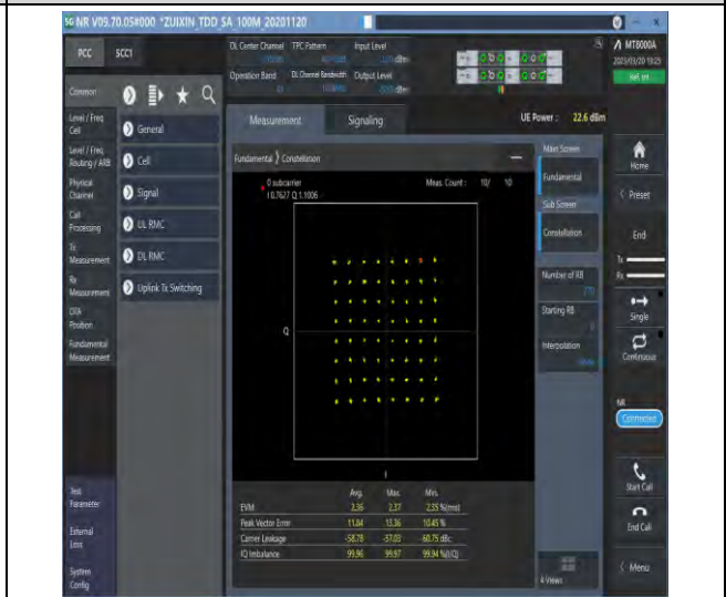
1-N41-30-100-M-4-DFT-64QAM-Outer_Full-270@0-Ant1-see graph-PASS
