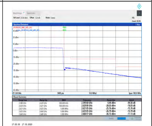
1-N38-30-40-H-6-CP-QPSK-Outer_Full-106@0-Ant1-1--PASS-see graph
