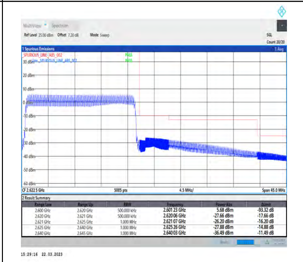
1-N38-30-20-H-6-CP-QPSK-Outer_Full-51@0-Ant1 1-1--PASS-see graph
