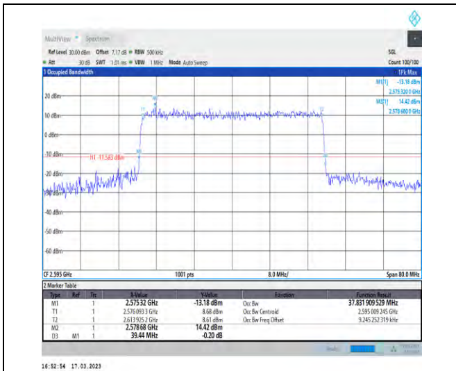
1-N38-30-40-M-7-CP-16QAM-Outer_Full-106@0-Ant t1-37.832-39.440-≤40-PASS
