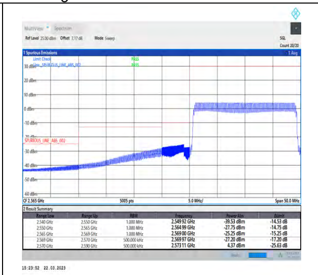
1-N38-30-20-L-6-CP-QPSK-Outer_Full-51@0-Ant1 1-1--PASS-see graph
