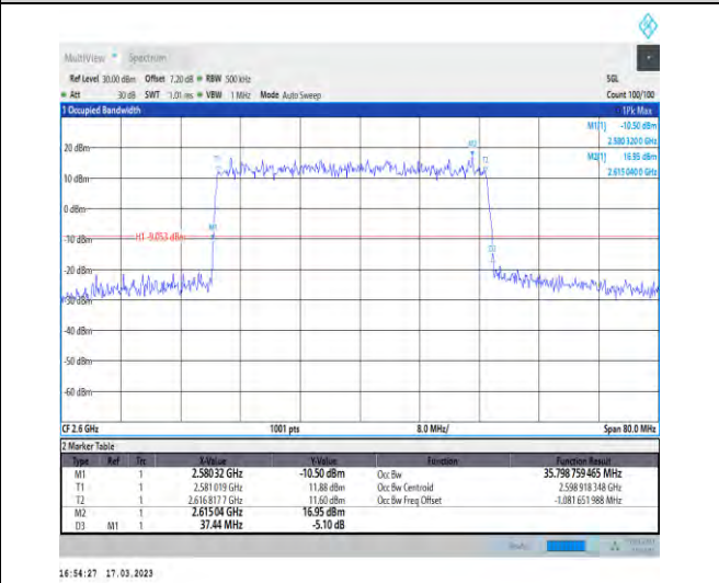
1-N38-30-40-H-1-DFT-QPSK-Outer_Full-100@0-Ant 1-35.799-37.440-≤40-PASS
