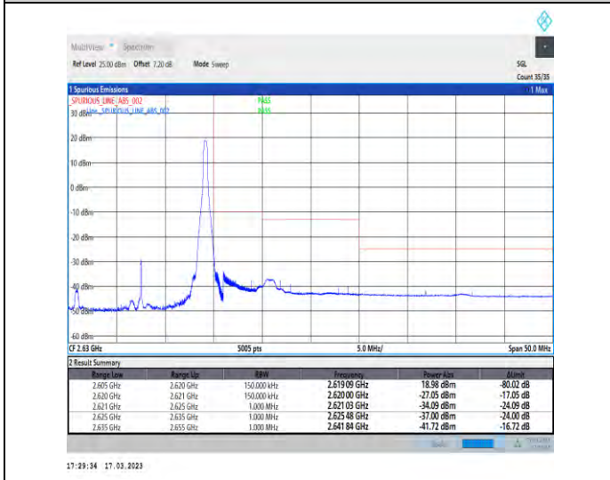
1-N38-30-15-H-5-CP-QPSK-Edge_1RB_Right-1@37-Ant1-1--PASS-see graph
