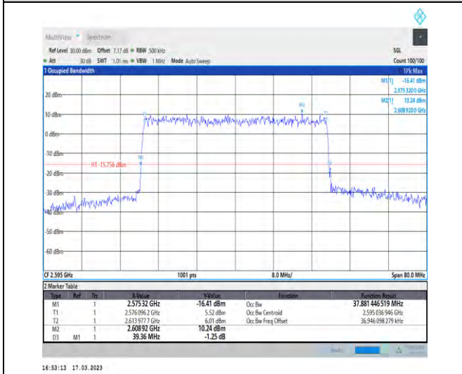
1-N38-30-40-M-9-CP-256QAM-Outer_Full-106@0-Ant nt1-37.881-39.360-≤40-PASS
