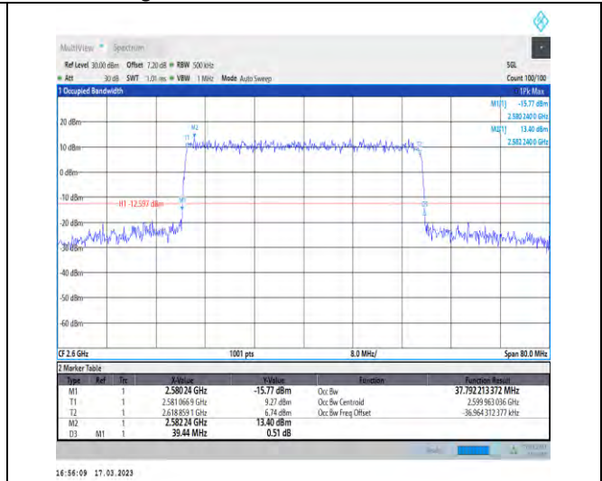
1-N38-30-40-H-7-CP-16QAM-Outer_Full-106@0-Ant1 -37.792-39.440-≤40-PASS
