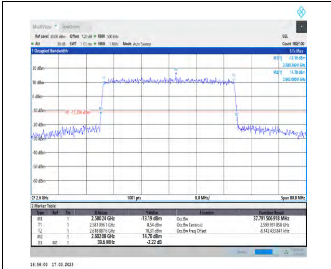
1-N38-30-40-H-6-CP-QPSK-Outer_Full-106@0-Ant1 -37.792-39.600-≤40-PASS
