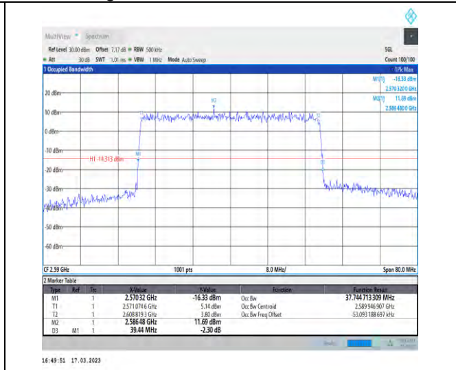
1-N38-30-40-L-9-CP-256QAM-Outer_Full-106@0-An t1-37.745-39.440-≤40-PASS
