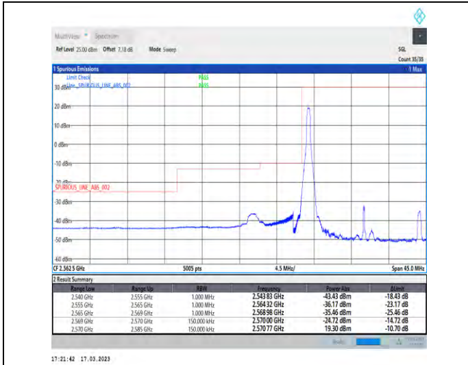
1-N38-30-15-L-1-DFT-PI2BPSK-Edge_1RB_Left-1@0-Ant1-1--PASS-see graph
