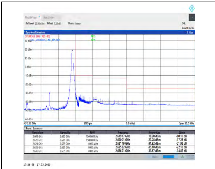
1-N38-30-15-H-2-DFT-PI2BPSK-Edge_1RB_Right-1@37-Ant1-1--PASS-see graph
