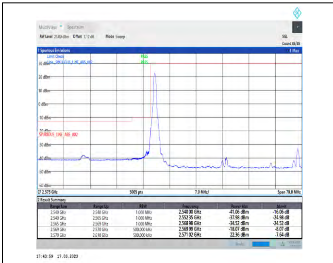
1-N38-30-40-L-1-DFT-PI2BPSK-Edge_1RB_Left-1@0-Ant1-1--PASS-see graph
