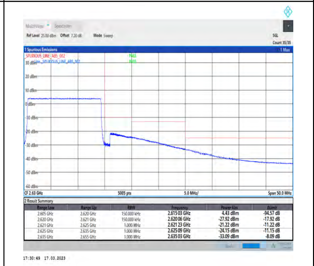
1-N38-30-15-H-6-CP-QPSK-Outer_Full-38@0-Ant1-1--PASS-see graph
