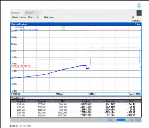
1-N38-30-20-L-6-CP-QPSK-Outer_Full-51@0-Ant1-1--PASS-see graph
