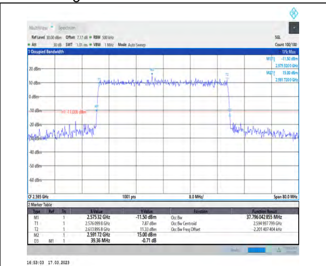
1-N38-30-40-M-8-CP-64QAM-Outer_Full-106@0-Ant 1-37.796-39.360-≤40-PASS
