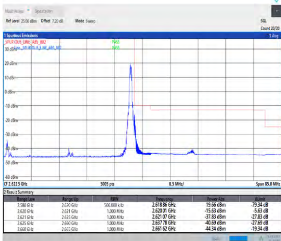
1-N38-30-40-H-5-CP-QPSK-Edge_1RB_Right-1@105-Ant1 -1--PASS-see graph
