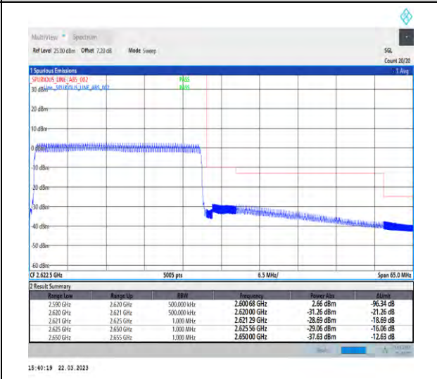
1-N38-30-30-H-6-CP-QPSK-Outer_Full-78@0-Ant1 1-1--PASS-see graph
