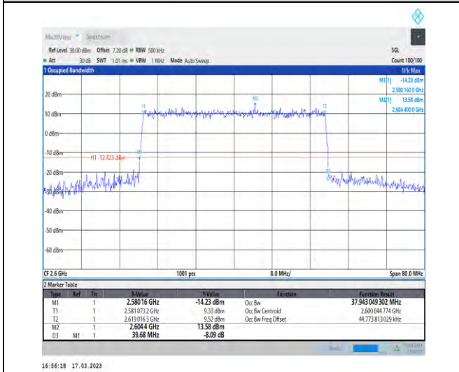
1-N38-30-40-H-8-CP-64QAM-Outer_Full-106@0-Ant1 -37.943-39.680-≤40-PASS
