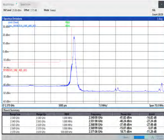
1-N38-30-40-L-4-CP-QPSK-Edge_1RB_Left-1@0-Ant1 -1--PASS-see graph
