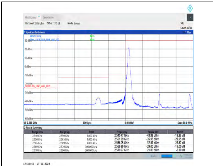
1-N38-30-20-L-1-DFT-PI2BPSK-Edge_1RB_Left-1@0-Ant1-1--PASS-see graph
