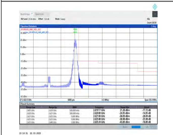
1-N38-30-15-H-5-CP-QPSK-Edge_1RB_Right-1@37-Ant1 -1--PASS-see graph
