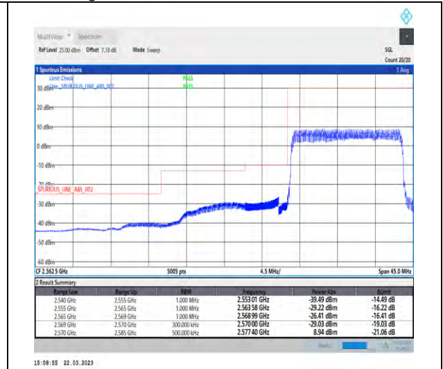
1-N38-30-15-L-6-CP-QPSK-Outer_Full-38@0-Ant1 -1--PASS-see graph
