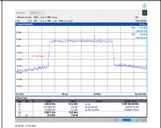
1-N38-30-40-H-9-CP-256QAM-Outer_Full-106@0-Ant1 -37.801-39.600-≤40-PASS
