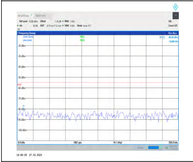
1-N38-30-40-M-1-DFT-PI2BPSK-Inner_1RB_Left-1 @ 1-0.009-0.15-Ant1-0.09--80.64--55-PASS
