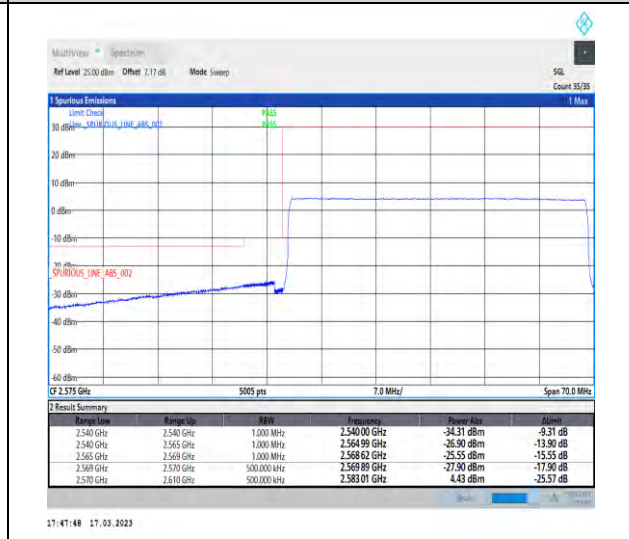
1-N38-30-40-L-6-CP-QPSK-Outer_Full-106@0-Ant1-1--PASS-see graph
