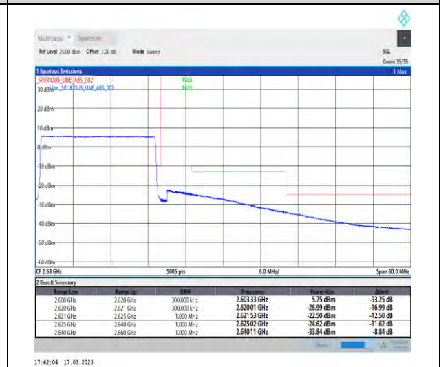
1-N38-30-20-H-6-CP-QPSK-Outer_Full-51@0-Ant1-1--PASS-see graph
