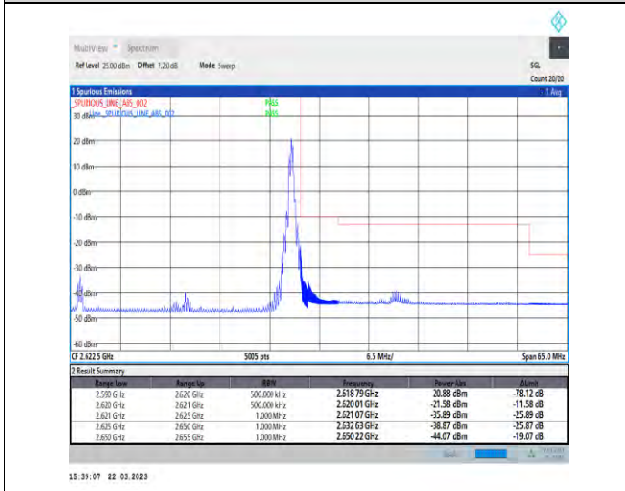
1-N38-30-30-H-5-CP-QPSK-Edge_1RB_Right-1@77-Ant1 nt1-1--PASS-see graph
