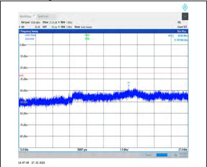
1-N38-30-40-H-1-DFT-PI2BPSK-Inner_1RB_Left-1@ 1-12000-27000-Ant1-21767.50--36.69--25-PASS
