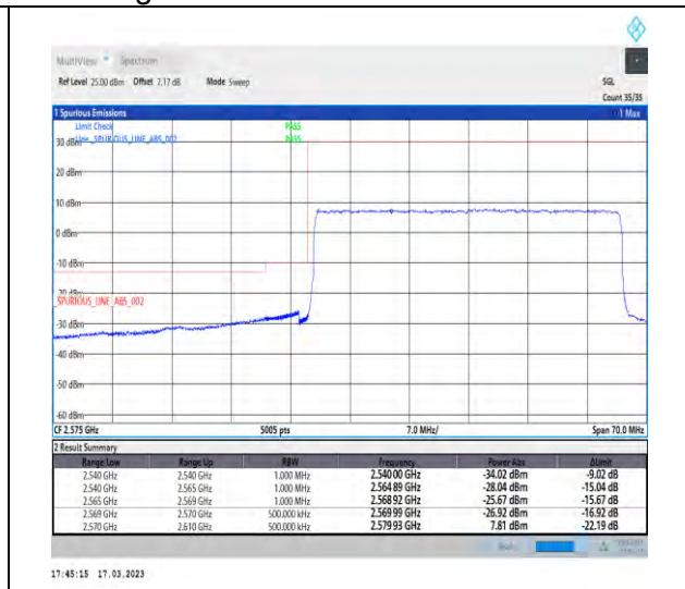
1-N38-30-40-L-3-DFT-PI2BPSK-Outer_Full-100@0-Ant1-1--PASS-see graph
