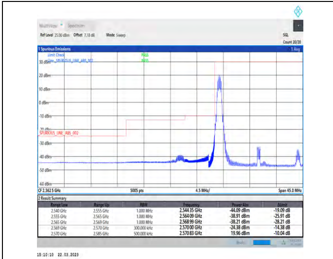
1-N38-30-15-L-4-CP-QPSK-Edge_1RB_Left-1@0-Ant1 -1--PASS-see graph
