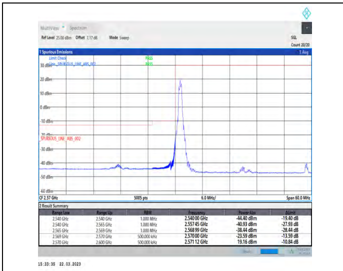
1-N38-30-30-L-4-CP-QPSK-Edge_1RB_Left-1@0-Ant1 -1--PASS-see graph
