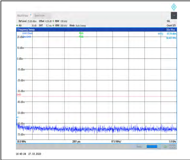
1-N38-30-40-M-1-DFT-PI2BPSK-Inner_1RB_Left-1 @ 1-30-1000-Ant1-32.43--57.74--35-PASS
