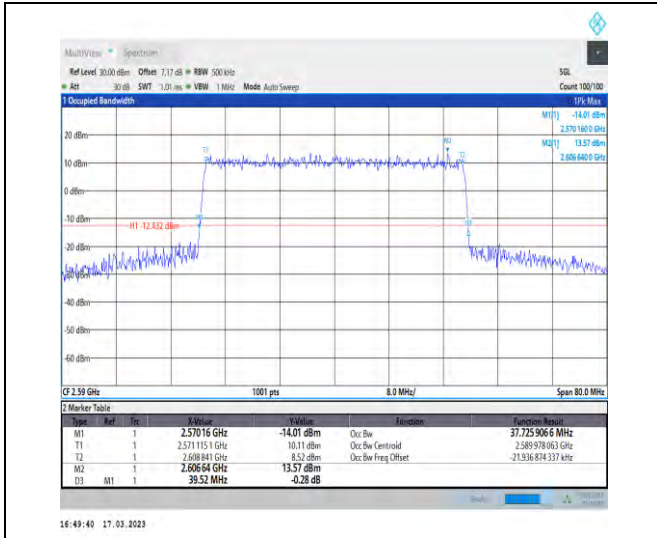
1-N38-30-40-L-8-CP-64QAM-Outer_Full-106@0-Ant 1-37.726-39.520-≤40-PASS
