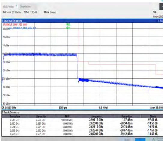
1-N38-30-40-H-6-CP-QPSK-Outer_Full-106@0-Ant1 -1--PASS-see graph
