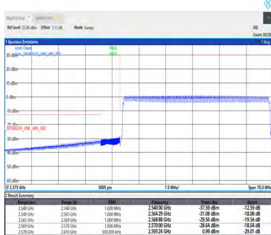
1-N38-30-40-L-6-CP-QPSK-Outer_Full-106@0-Ant1 -1--PASS-see graph
