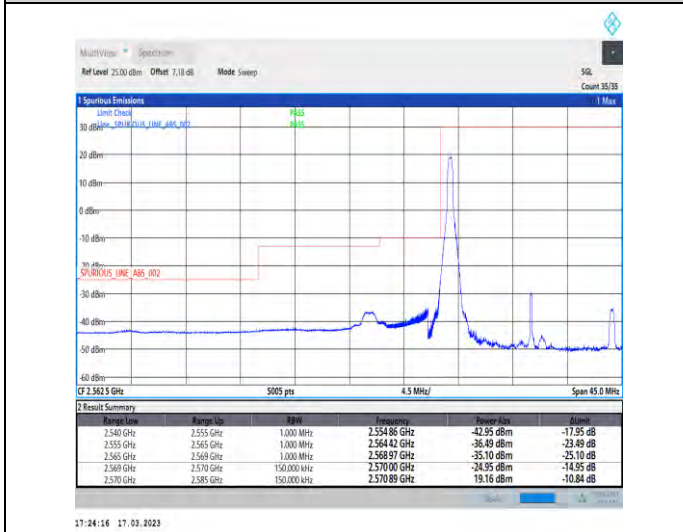
1-N38-30-15-L-4-CP-QPSK-Edge_1RB_Left-1@0-Ant1-1--PASS-see graph
