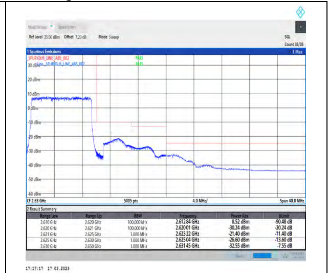
1-N38-30-10-H-3-DFT-PI2BPSK-Outer_Full-24@0-Ant1-1--PASS-see graph
