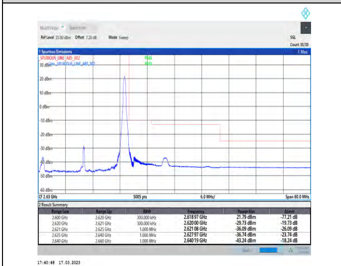
1-N38-30-20-H-5-CP-QPSK-Edge_1RB_Right-1@50-Ant1-1--PASS-see graph
