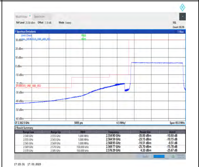
1-N38-30-15-L-6-CP-QPSK-Outer_Full-38@0-Ant1-1--PASS-see graph
