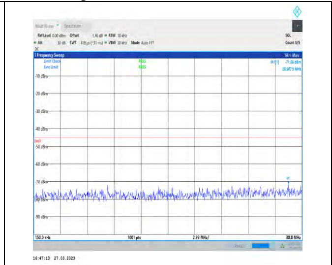
1-N38-30-40-H-1-DFT-PI2BPSK-Inner_1RB_Left-1 @ 1-0.15-30-Ant1-29.94--71.66--45-PASS
