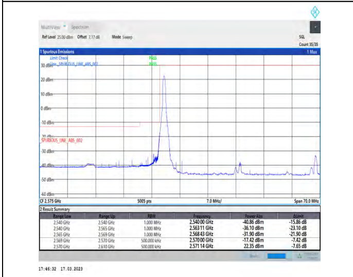
1-N38-30-40-L-4-CP-QPSK-Edge_1RB_Left-1@0-Ant1-1--PASS-see graph
