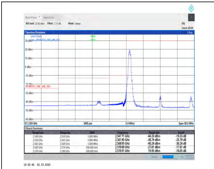
1-N38-30-20-L-4-CP-QPSK-Edge_1RB_Left-1@0-Ant1 -1--PASS-see graph
