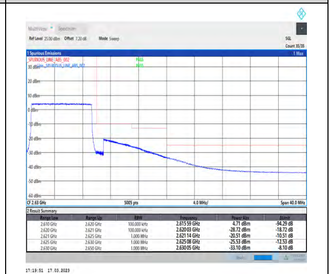
1-N38-30-10-H-6-CP-QPSK-Outer_Full-24@0-Ant1-1--PASS-see graph
