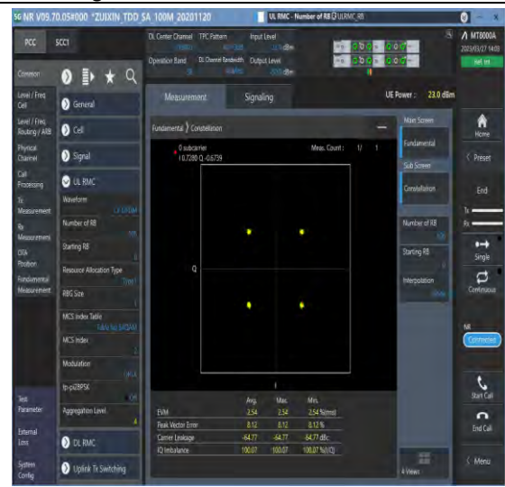
1-N38-30-40-M-6-CP-QPSK-Outer_Full-106@0-Ant 1-see graph-PASS
