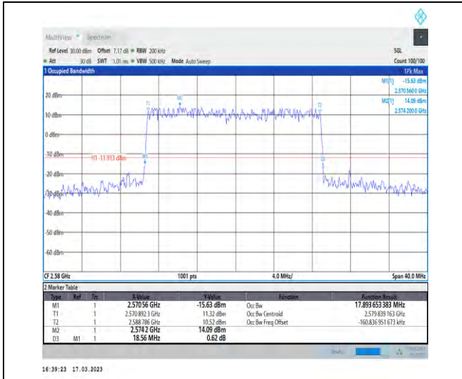
1-N38-30-20-L-3-DFT-16QAM-Outer_Full-50@0-Ant 1-17.894-18.560-≤20-PASS
