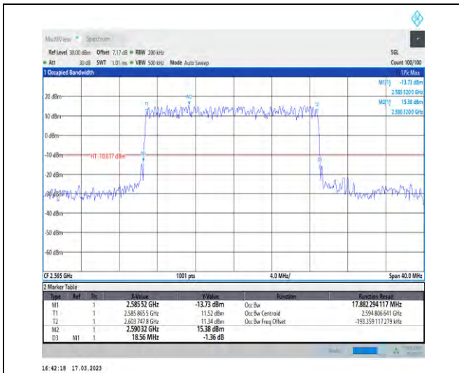
1-N38-30-20-M-2-DFT-PI2BPSK-Outer_Full-50@0-A nt1-17.882-18.560-≤20-PASS
