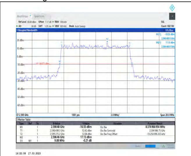
1-N38-30-10-M-1-DFT-QPSK-Outer_Full-24@0-Ant1 -8.577-9.080≤10-PASS
