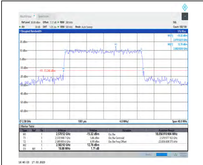
1-N38-30-20-L-7-CP-16QAM-Outer_Full-51@0-Ant1 -18.057-18.880-≤20-PASS
