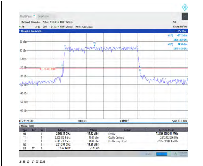
1-N38-30-15-H-4-DFT-64QAM-Outer_Full-36@0-Ant 1-12.859-13.770≤15-PASS
