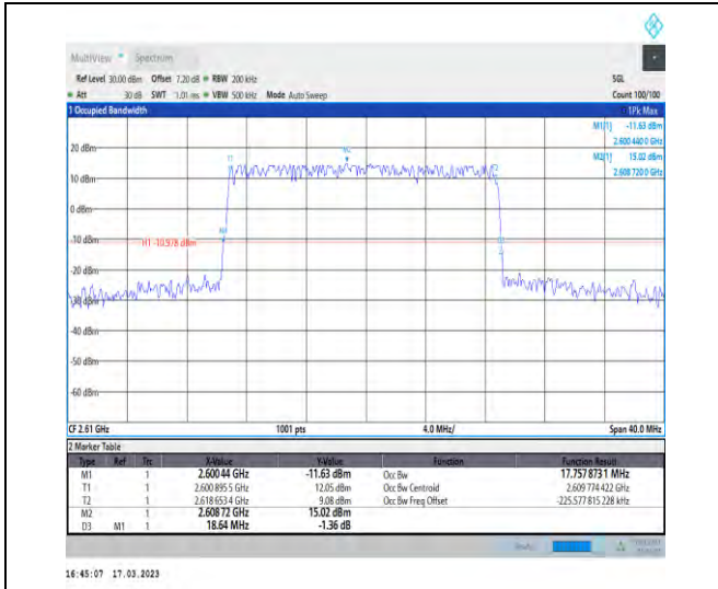
1-N38-30-20-H-1-DFT-QPSK-Outer_Full-50@0-Ant1 -17.758-18.640-≤20-PASS
