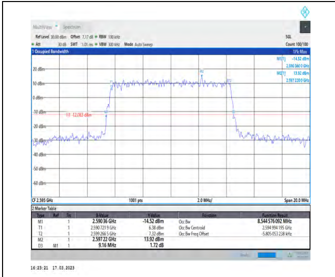
1-N38-30-10-M-4-DFT-64QAM-Outer_Full-24@0-Ant 1-8.545-9.160-≤10-PASS
