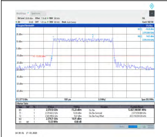
1-N38-30-15-L-4-DFT-64QAM-Outer_Full-36@0-Ant t1-12.827-13.530-≤15-PASS
