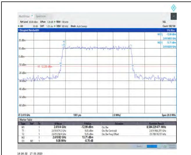
1-N38-30-10-H-3-DFT-16QAM-Outer_Full-24@0-Ant 1-8.584-9.080-≤10-PASS
