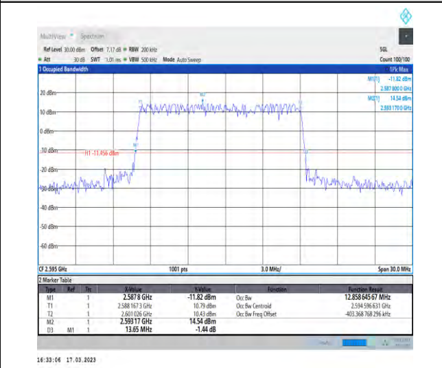
1-N38-30-15-M-4-DFT-64QAM-Outer_Full-36@0-Ant1 1-12.859-13.650≤15-PASS
