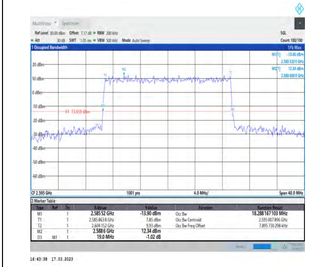
1-N38-30-20-M-8-CP-64QAM-Outer_Full-51@0-Ant1-18.288-19.000-<=20-PASS
