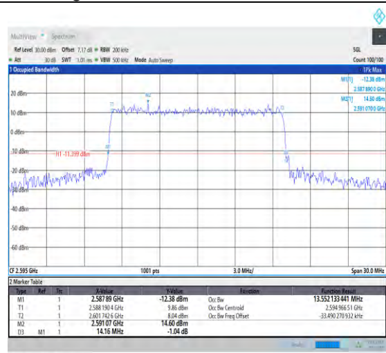
1-N38-30-15-M-6-CP-QPSK-Outer_Full-38@0-Ant1 13.552-14.160-≤15-PASS
