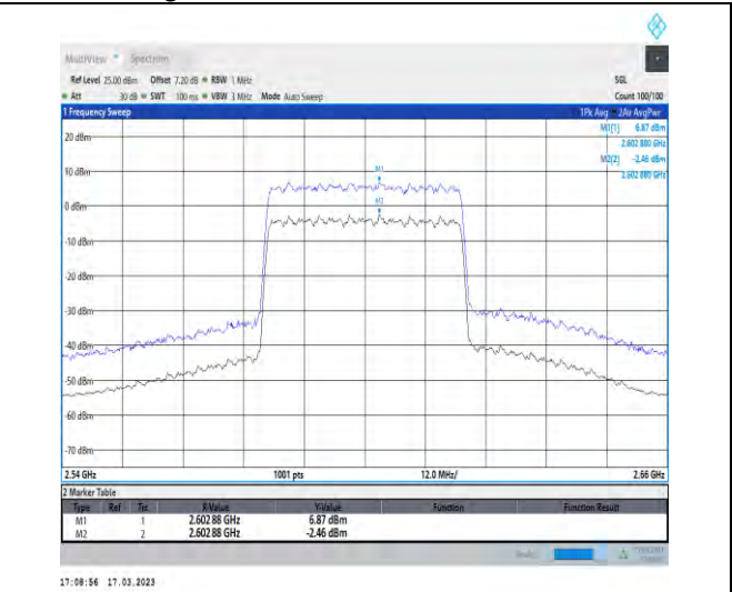
1-N38-30-40-H-2-CP-256QAM-Outer_Full-106@0-Ant1-9.33-100%-0.00-9.33-PASS-≤13
