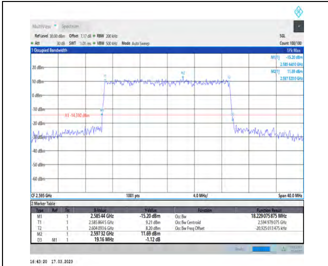
1-N38-30-20-M-6-CP-QPSK-Outer_Full-51@0-Ant1-18.229-19.160-<=20-PASS
