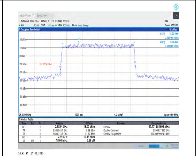
1-N38-30-20-M-1-DFT-QPSK-Outer_Full-50@0-Ant1 -17.772-18.640-≤20-PASS
