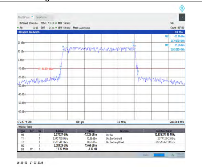
1-N38-30-15-L-3-DFT-16QAM-Outer_Full-36@0-Ant t1-12.835-13.770-≤15-PASS
