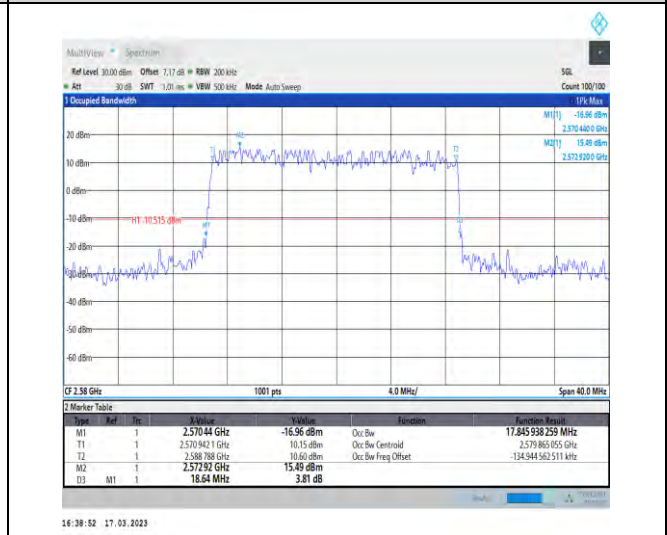
1-N38-30-20-L-2-DFT-PI2BPSK-Outer_Full-50@0-A nt1-17.846-18.640-≤20-PASS
