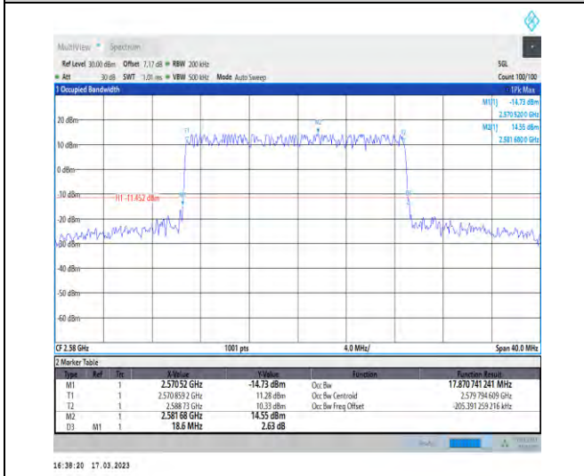
1-N38-30-20-L-1-DFT-QPSK-Outer_Full-50@0-Ant1 17.871-18.600-≤20-PASS
