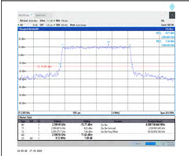
1-N38-30-10-M-6-CP-QPSK-Outer_Full-24@0-Ant1- 8.588-9.120-≤10-PASS
