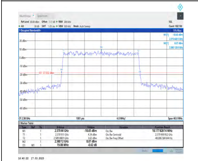
1-N38-30-20-L-9-CP-256QAM-Outer_Full-51@0-Ant 1-18.178-19.080-≤20-PASS
