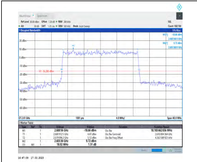
1-N38-30-20-H-9-CP-256QAM-Outer_Full-51@0-Ant 1-18.184-18.920-≤20-PASS
