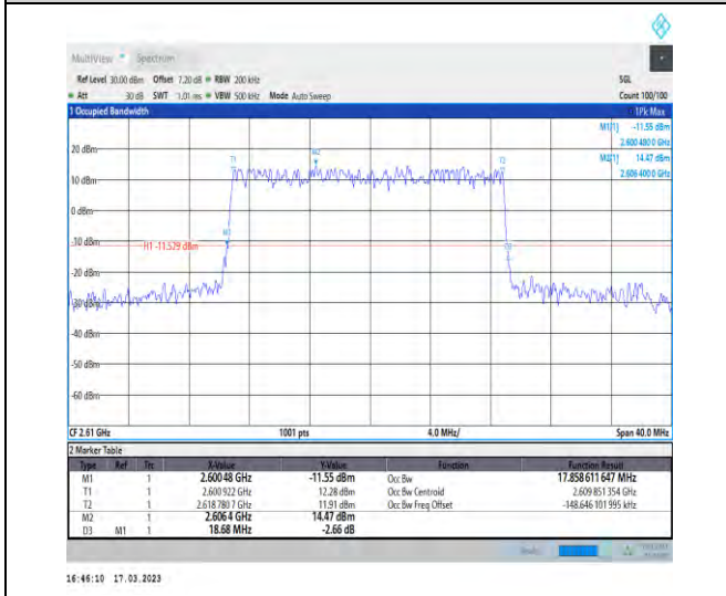
1-N38-30-20-H-3-DFT-16QAM-Outer_Full-50@0-Ant1 1-17.859-18.680-≤20-PASS
