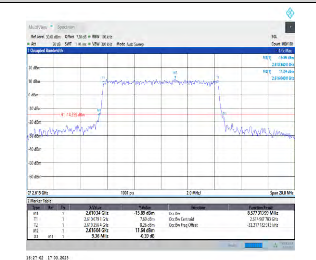
1-N38-30-10-H-6-CP-QPSK-Outer_Full-24@0-Ant1 8.577-9.360-≤10-PASS
