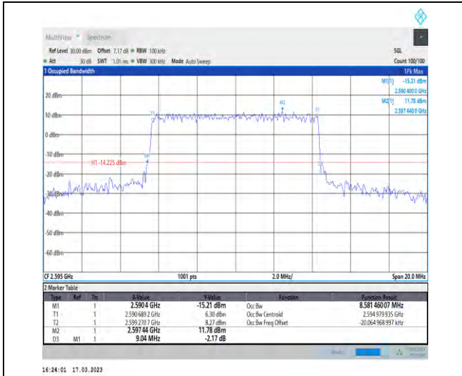
1-N38-30-10-M-8-CP-64QAM-Outer_Full-24@0-Ant 1-8.581-9.040-≤10-PASS
