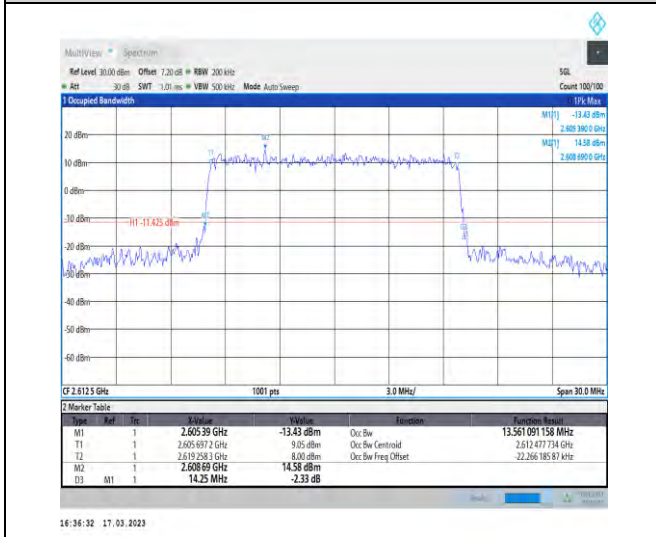
1-N38-30-15-H-6-CP-QPSK-Outer_Full-38@0-Ant1 13.561-14.250≤15-PASS
