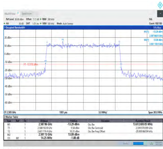
1-N38-30-15-M-8-CP-64QAM-Outer_Full-38@0-Ant1 -13.613-14.250-≤15-PASS
