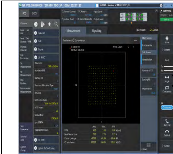
1-N38-30-40-M-5-DFT-256QAM-Outer_Full-100@0-A nt1-see graph-PASS
