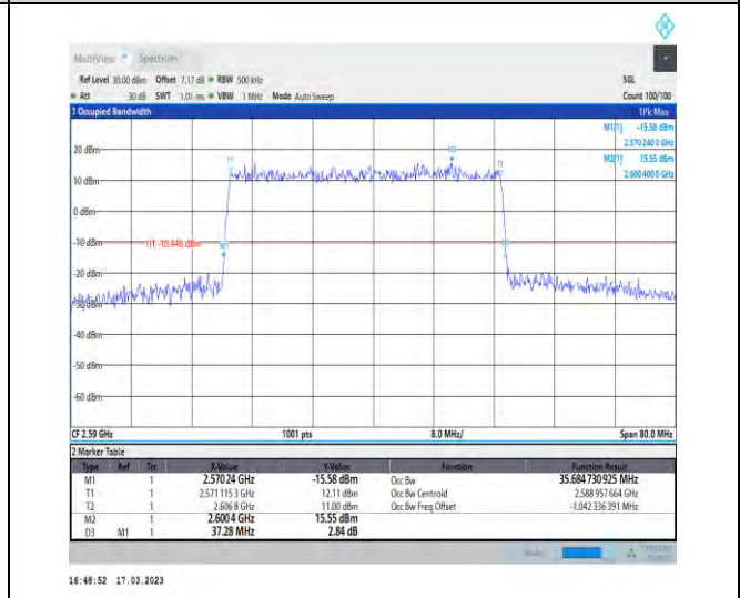
1-N38-30-40-L-3-DFT-16QAM-Outer_Full-100@0-Ant 1-35.685-37.280-≤40-PASS
