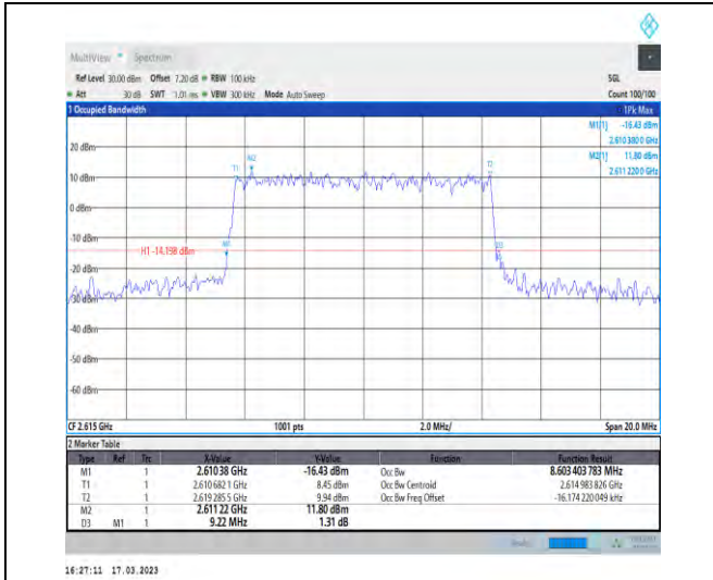
1-N38-30-10-H-7-CP-16QAM-Outer_Full-24@0-Ant1 -8.603-9.220-≤10-PASS
