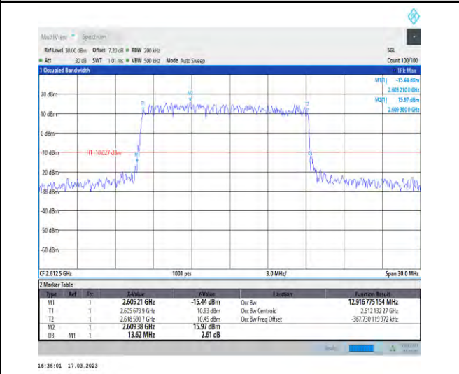
1-N38-30-15-H-3-DFT-16QAM-Outer_Full-36@0-Ant1-12.917-13.620-≤15-PASS
