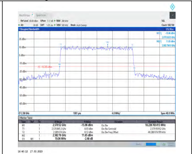
1-N38-30-20-L-8-CP-64QAM-Outer_Full-51@0-Ant1 18.229-19.040-≤20-PASS
