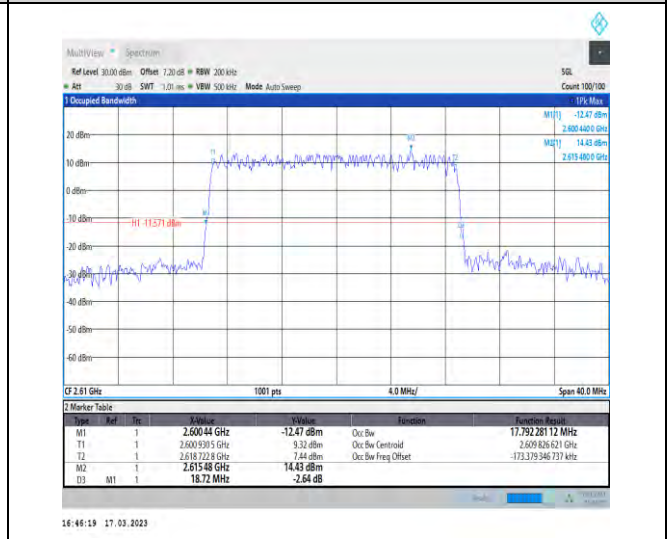
1-N38-30-20-H-4-DFT-64QAM-Outer_Full-50@0-Ant1 1-17.792-18.720-≤20-PASS
