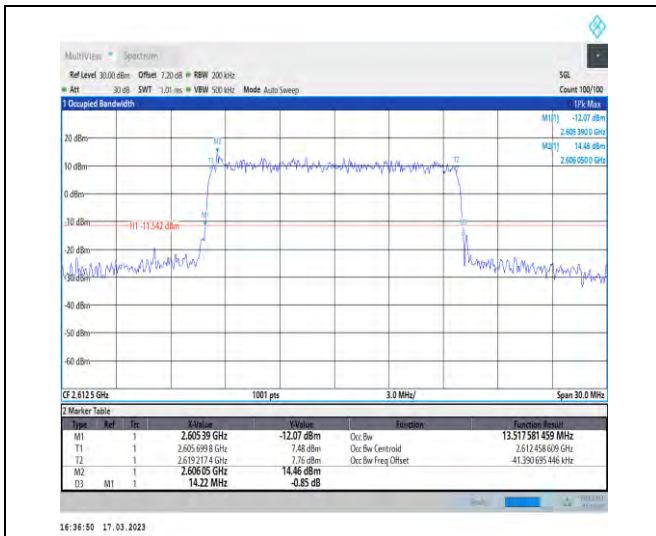
1-N38-30-15-H-8-CP-64QAM-Outer_Full-38@0-Ant1 -13.518-14.220-≤15-PASS
