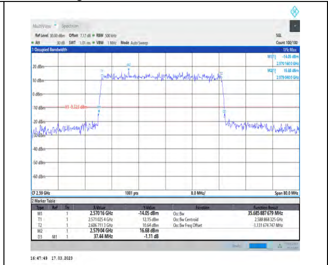
1-N38-30-40-L-1-DFT-QPSK-Outer_Full-100@0-Ant 1-35.686-37.440-≤40-PASS
