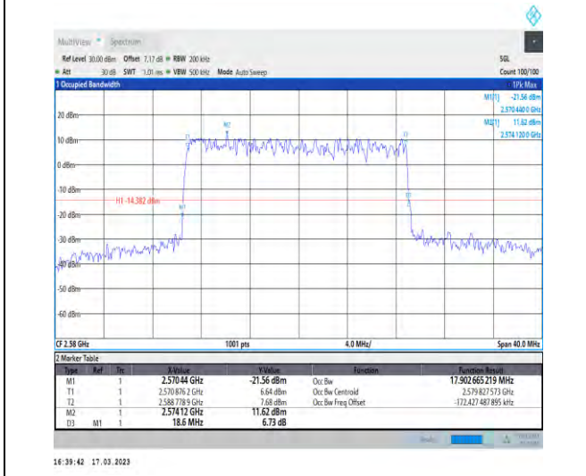
1-N38-30-20-L-5-DFT-256QAM-Outer_Full-50@0-Ant t1-17.903-18.600-≤20-PASS
