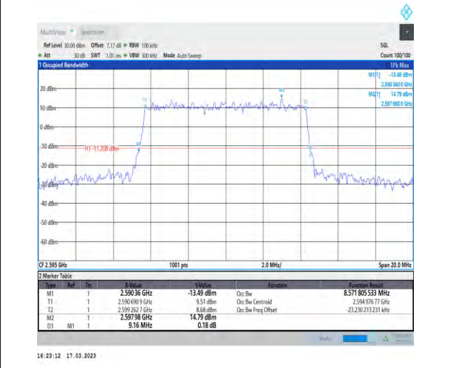
1-N38-30-10-M-3-DFT-16QAM-Outer_Full-24@0-Ant 1-8.572-9.160≤10-PASS
