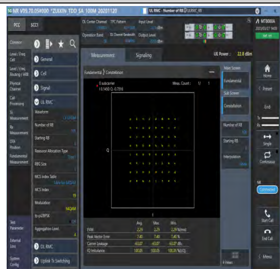
1-N38-30-40-M-8-CP-64QAM-Outer_Full-106@0-A nt1-see graph-PASS
