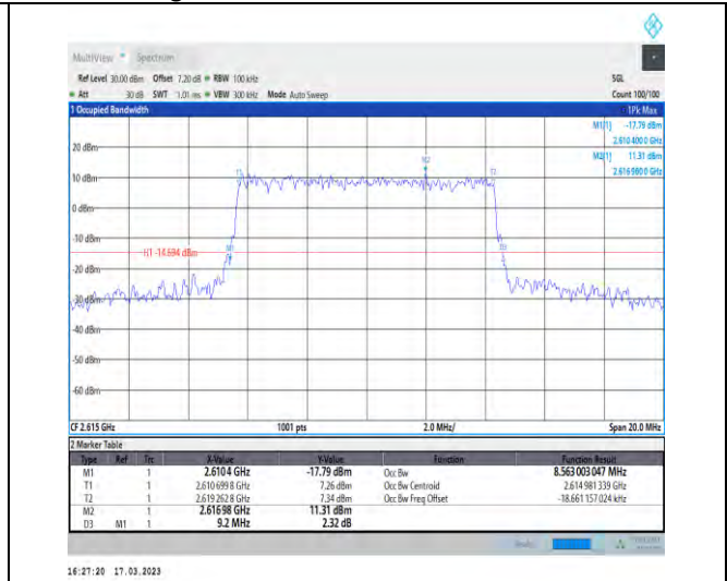
1-N38-30-10-H-8-CP-64QAM-Outer_Full-24@0-Ant1 -8.563-9.200-≤10-PASS
