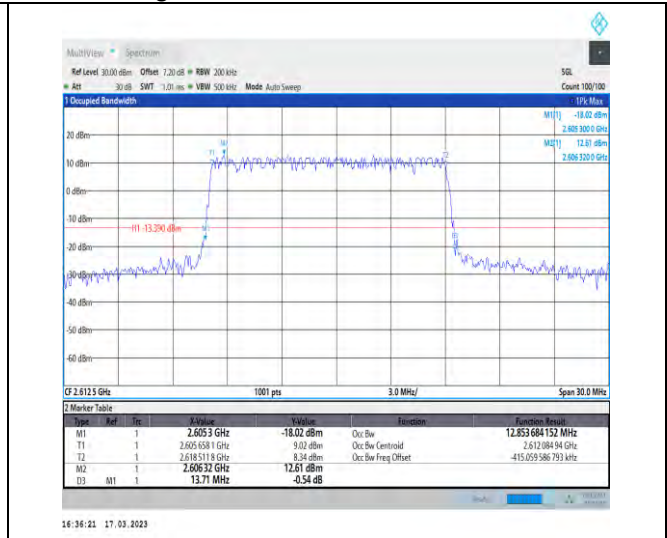
1-N38-30-15-H-5-DFT-256QAM-Outer_Full-36@0-A nt1-12.854-13.710≤15-PASS
