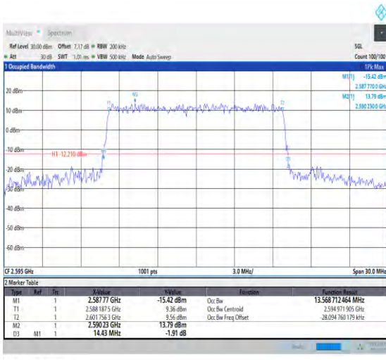
1-N38-30-15-M-7-CP-16QAM-Outer_Full-38@0-Ant 1-13.569-14.430-≤15-PASS
