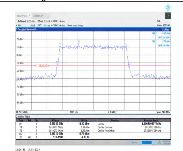
1-N38-30-10-H-4-DFT-64QAM-Outer_Full-24@0-Ant 1-8.601-9.360-≤10-PASS
