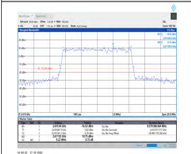
1-N38-30-10-H-5-DFT-256QAM-Outer_Full-24@0-A nt1-8.579-9.220-≤10-PASS
