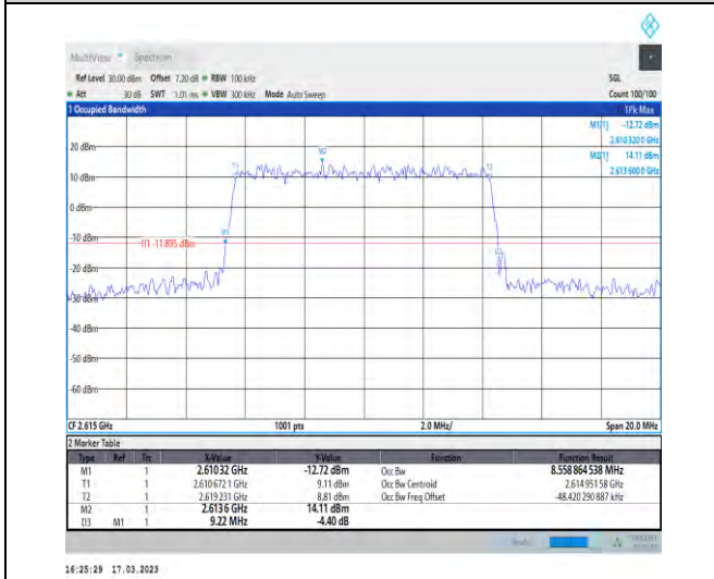
1-N38-30-10-H-1-DFT-QPSK-Outer_Full-24@0-Ant1 -8.559-9.220-≤10-PASS
