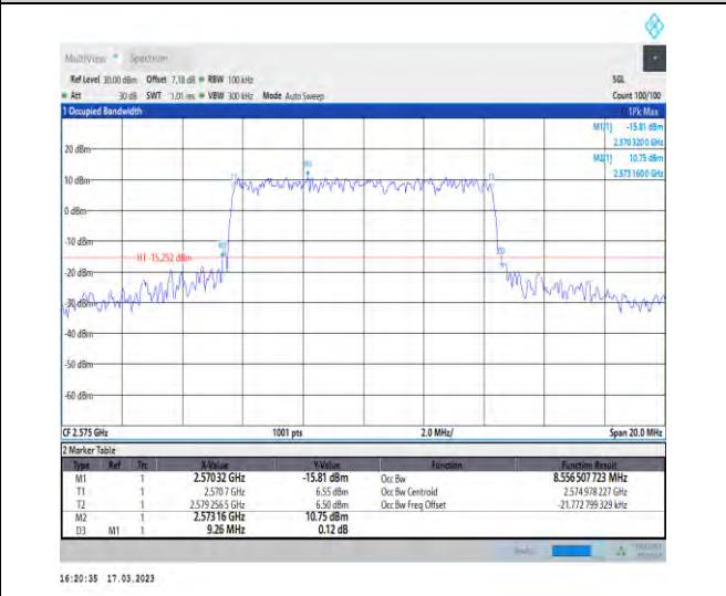
1-N38-30-10-L-8-CP-64QAM-Outer_Full-24@0-Ant1-8.557-9.260-≤10-PASS
