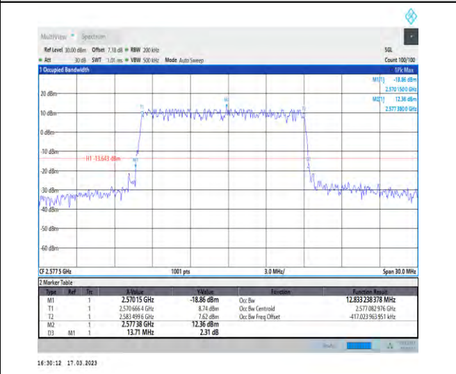
1-N38-30-15-L-5-DFT-256QAM-Outer_Full-36@0-Ant t1-12.833-13.710-≤15-PASS
