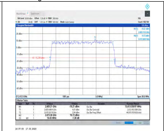
1-N38-30-15-H-9-CP-256QAM-Outer_Full-38@0-Ant 1-13.613-14.430-≤15-PASS
