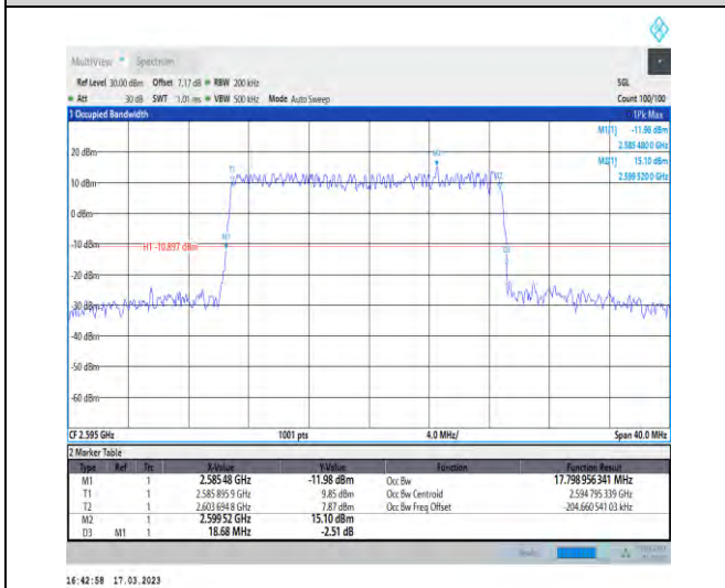
1-N38-30-20-M-4-DFT-64QAM-Outer_Full-50@0-Ant 1-17.799-18.680-≤20-PASS
