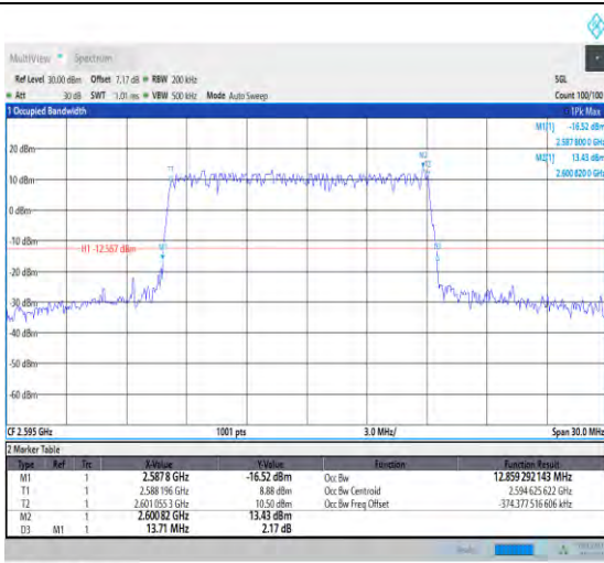
1-N38-30-15-M-5-DFT-256QAM-Outer_Full-36@0-A nt1-12.859-13.710-≤15-PASS
