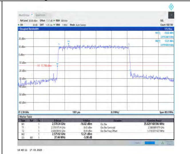
1-N38-30-40-L-5-DFT-256QAM-Outer_Full-100@0-Ant nt1-35.829-37.440-≤40-PASS
