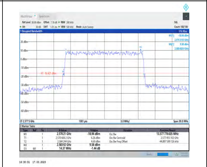
1-N38-30-15-L-9-CP-256QAM-Outer_Full-38@0-Ant1-13.578-14.370-≤15-PASS
