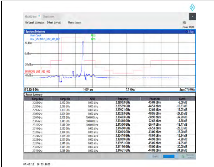
1-N30-PC3-15-10-H-2-DFT-PI2BPSK-Edge_1RB_Right-t-1@51-Ant1-1--PASS-see graph
