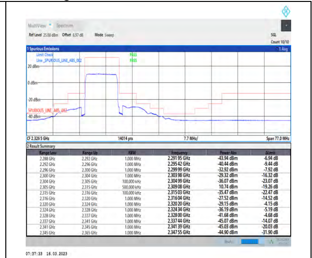
1-N30-PC3-15-10-L-3-DFT-PI2BPSK-Outer_Full-50@0-Ant1-1--PASS-see graph
