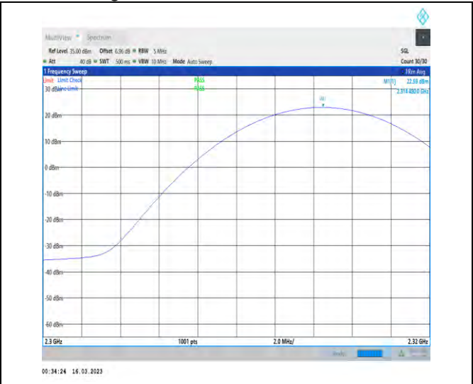
1-N30-PC3-15-10-M-2-DFT-PI2BPSK-Inner_1RB_Ri ght-1@50-2300-2320-Ant1-2314.48-22.93-99-PASS
