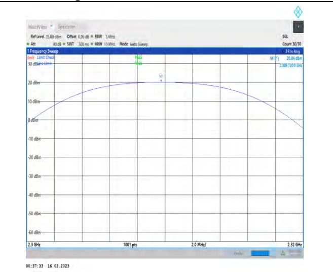
1-N30-PC3-15-10-H-3-DFT-PI2BPSK-Outer_Full-50 @0-2300-2320-Ant1-2309.72-20.04-99-PASS
