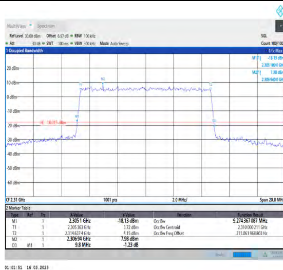
1-N30-PC3-15-10-L-9-CP-256QAM-Outer_Full-52@0- Ant1-9.274-9.800-≤10-PASS
