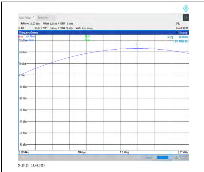
1-N30-PC3-15-5-M-2-DFT-PI2BPSK-Inner_1RB_Ri ght-1@23-2305-2315-Ant1-2311.96-23.00-99-PASS
