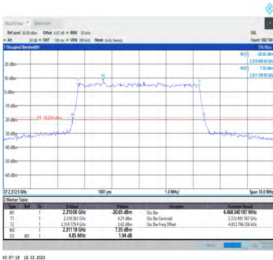
1-N30-PC3-15-5-H-9-CP-256QAM-Outer_Full-25@0-Ant1-4.468-4.850-≤5-PASS
