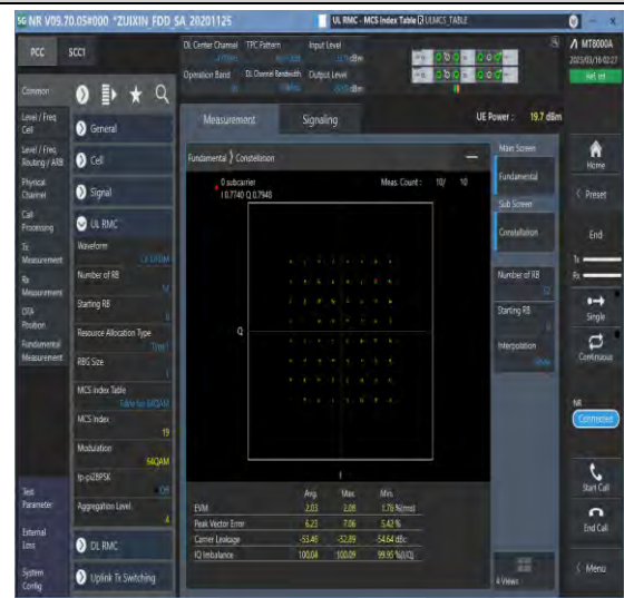
1-N30-PC3-15-10-M-8-CP-64QAM-Outer_Full-52@0-Ant1-see graph-PASS
