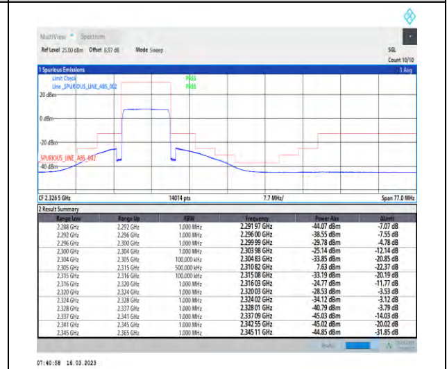
1-N30-PC3-15-10-L-6-CP-QPSK-Outer_Full-52@0-Ant1-1--PASS-see graph
