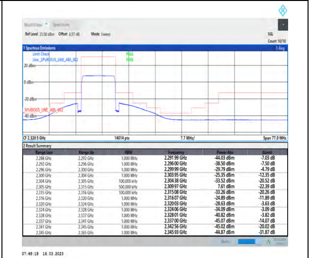
1-N30-PC3-15-10-H-6-CP-QPSK-Outer_Full-52@0-Ant1-1--PASS-see graph
