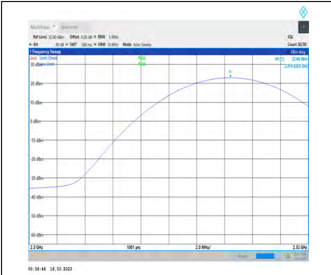
1-N30-PC3-15-10-H-2-DFT-PI2BPSK-Inner_1RB_Ri ght-1@50-2300-2320-Ant1-2314.42-22.94-99-PASS
