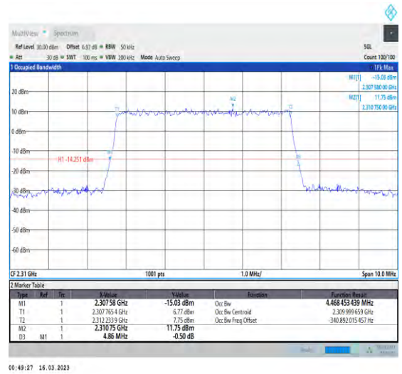
1-N30-PC3-15-5-M-3-DFT-16QAM-Outer_Full-25@0-Ant1-4.468-4.860-≤5-PASS
