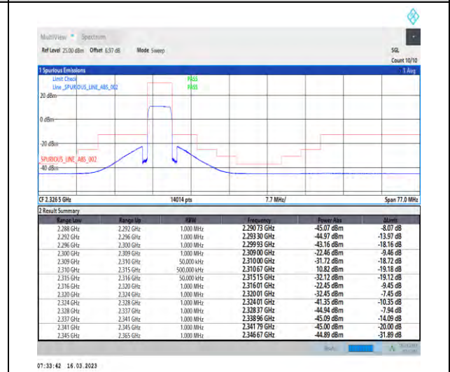
1-N30-PC3-15-5-H-6-CP-QPSK-Outer_Full-25@0-Ant1-1--PASS-see graph
