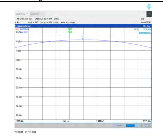
1-N30-PC3-15-5-M-3-DFT-PI2BPSK-Outer_Full-25@ 0-2305-2315-Ant1-2309.93-21.76-99-PASS
