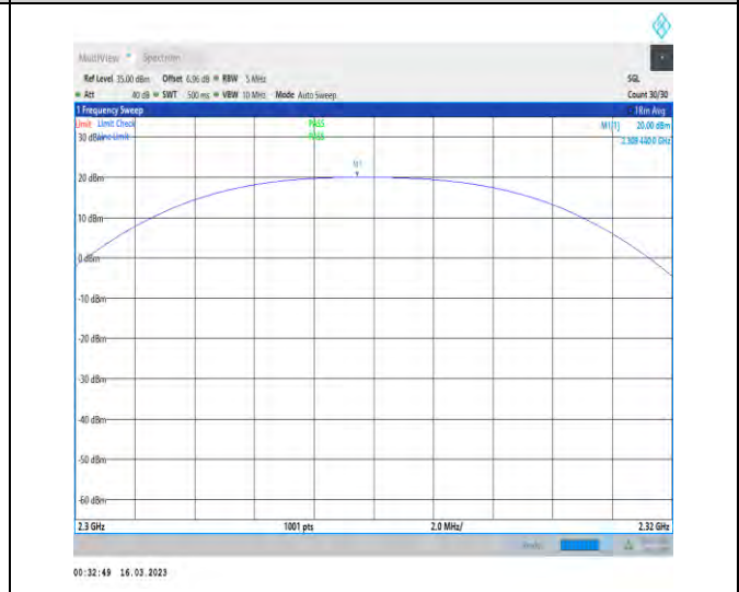
1-N30-PC3-15-10-L-3-DFT-PI2BPSK-Outer_Full-50 @0-2300-2320-Ant1-2309.44-20.00-99-PASS
