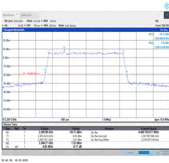
1-N30-PC3-15-5-L-9-CP-256QAM-Outer_Full-25@0-Ant1-4.47-4.850-≤5-PASS
