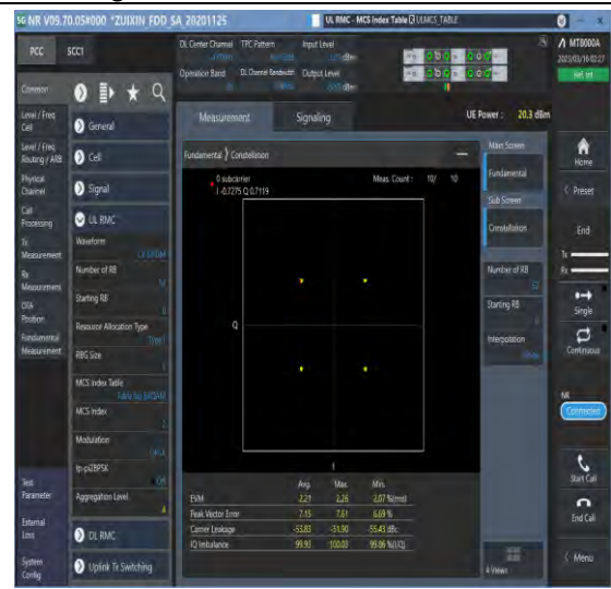
1-N30-PC3-15-10-M-6-CP-QPSK-Outer_Full-52@0-Ant1-see graph-PASS
