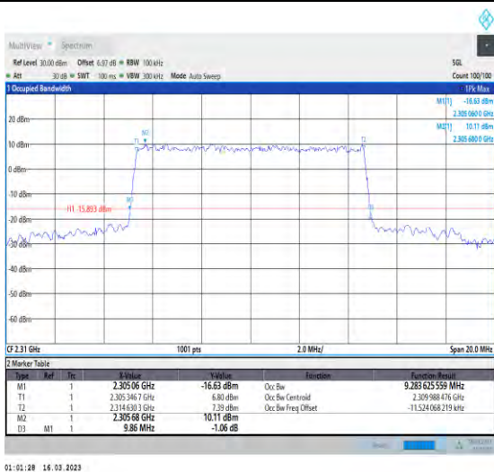
1-N30-PC3-15-10-L-8-CP-64QAM-Outer_Full-52@0- Ant1-9.284-9.860-≤10-PASS
