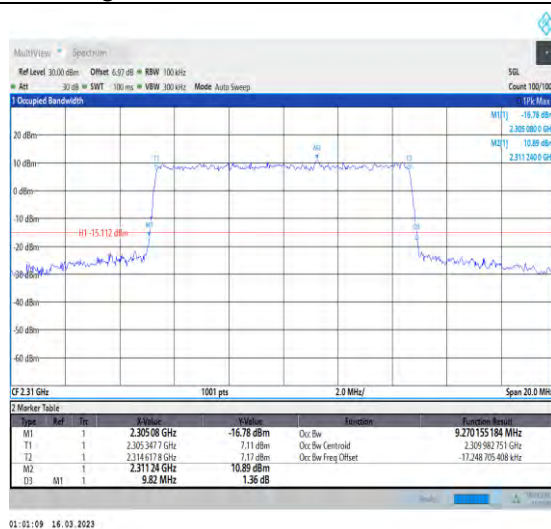
1-N30-PC3-15-10-L-7-CP-16QAM-Outer_Full-52@0- Ant1-9.27-9.820-≤10-PASS
