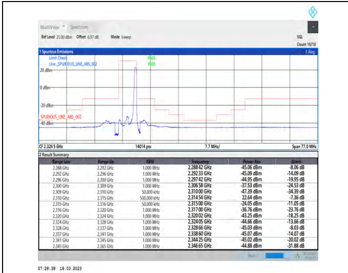
1-N30-PC3-15-5-H-2-DFT-PI2BPSK-Edge_1RB_Right-1@24-Ant1-1--PASS-see graph
