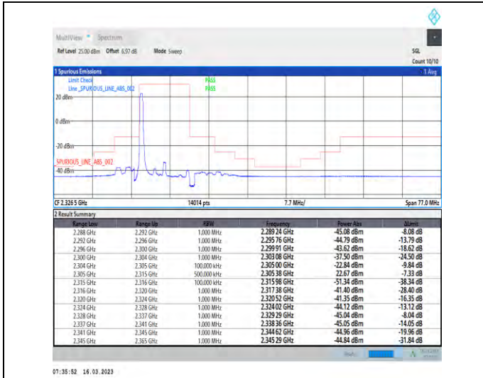
1-N30-PC3-15-10-L-1-DFT-PI2BPSK-Edge_1RB_Left-1@0-Ant1-1--PASS-see graph
