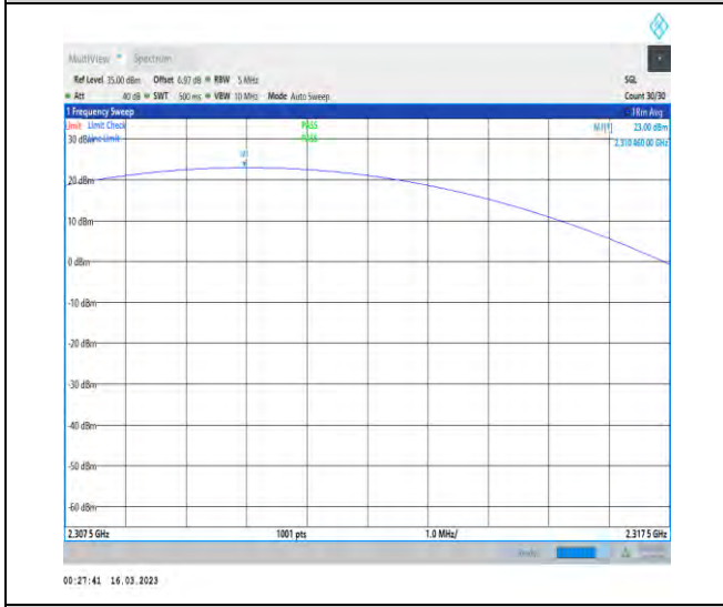
1-N30-PC3-15-5-H-1-DFT-PI2BPSK-Inner_1RB_Lef t-1@1-2307.5-2317.5-Ant1-2310.46-23.00-99-PASS
