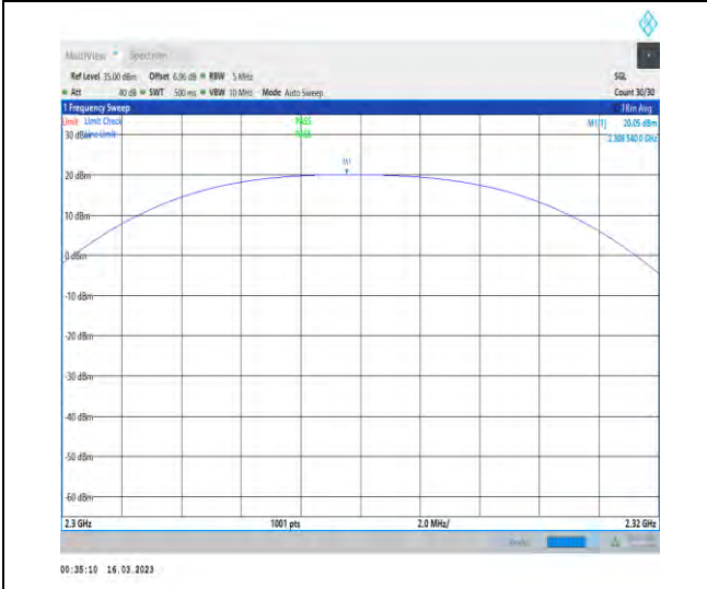
1-N30-PC3-15-10-M-3-DFT-PI2BPSK-Outer_Full-50 @0-2300-2320-Ant1-2309.54-20.05-99-PASS
