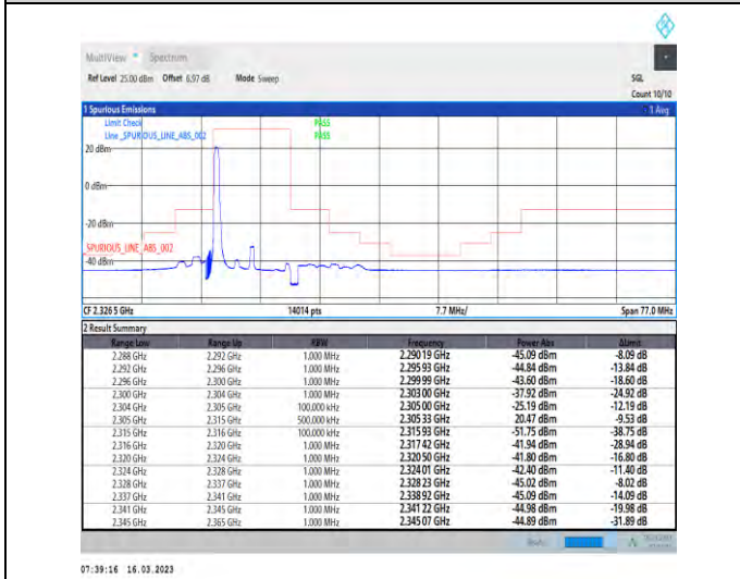
1-N30-PC3-15-10-L-4-CP-QPSK-Edge_1RB_Left-1@0-Ant1-1--PASS-see graph
