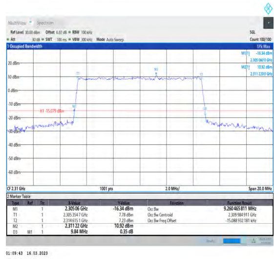
1-N30-PC3-15-10-H-7-CP-16QAM-Outer_Full-52@0 -Ant1-9.26-9.840-≤10-PASS
