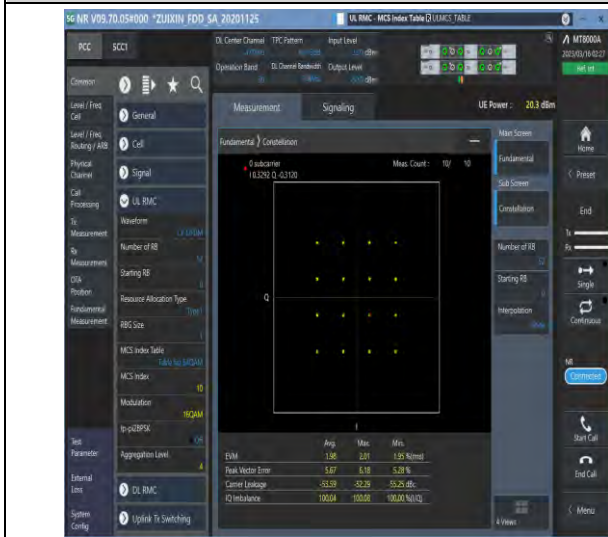
1-N30-PC3-15-10-M-7-CP-16QAM-Outer_Full-52@0-Ant1-see graph-PASS
