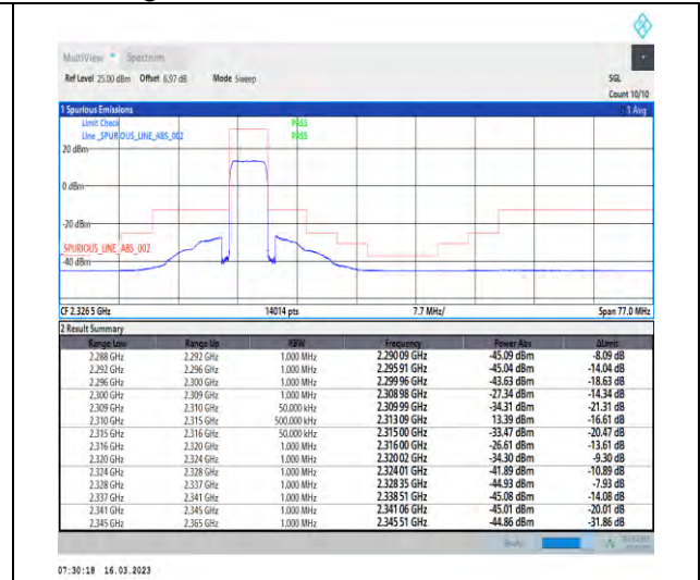
1-N30-PC3-15-5-H-3-DFT-PI2BPSK-Outer_Full-25@0-Ant1-1--PASS-see graph
