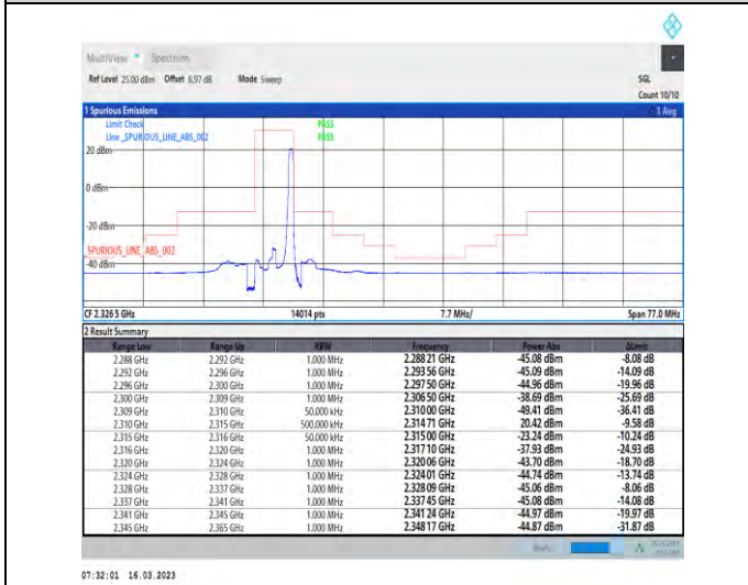
1-N30-PC3-15-5-H-5-CP-QPSK-Edge_1RB_Right-1@24-Ant1-1--PASS-see graph
