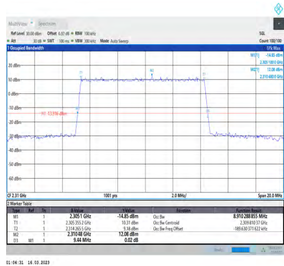
1-N30-PC3-15-10-M-4-DFT-64QAM-Outer_Full-50@0-Ant1-8.91-9.440-≤10-PASS
