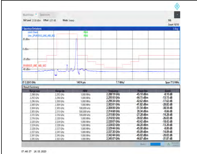
1-N30-PC3-15-10-H-5-CP-QPSK-Edge_1RB_Right-1@51-Ant1-1--PASS-see graph
