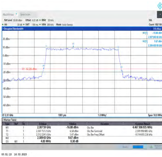
1-N30-PC3-15-5-M-8-CP-64QAM-Outer_Full-25@0-Ant1-4.467-4.830-≤5-PASS
