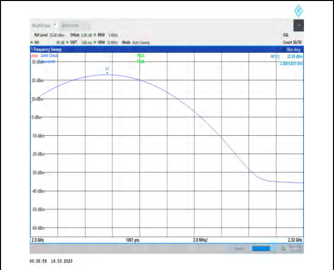
1-N30-PC3-15-10-H-1-DFT-PI2BPSK-Inner_1RB_Lef t-1@1-2300-2320-Ant1-2305.62-22.93-99-PASS
