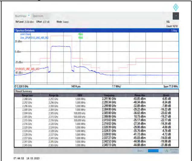
1-N30-PC3-15-10-H-3-DFT-PI2BPSK-Outer_Full-50@0-Ant1-1--PASS-see graph
