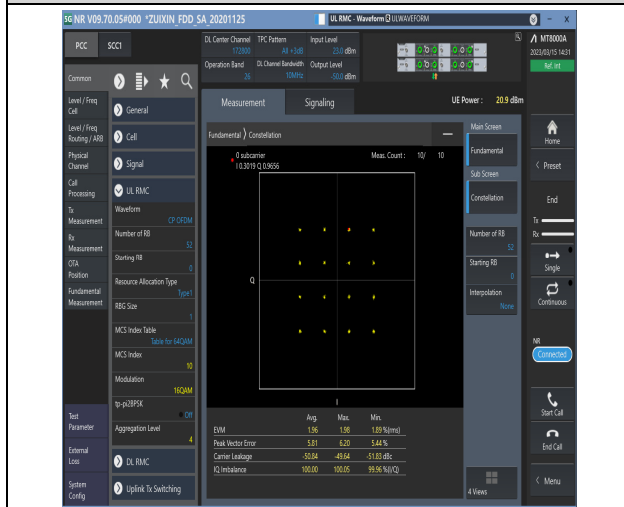
1-N26-814-824-PC3-15-10-M-7-CP-16QAM-Outer_Full-52@0-Ant1-see graph-PASS
