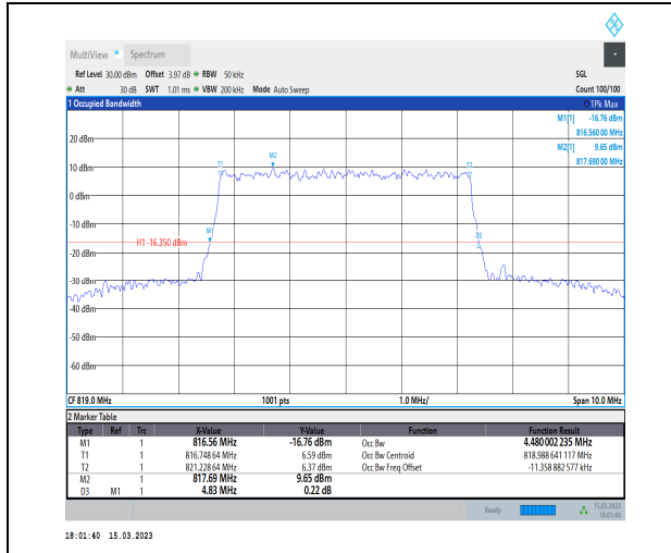
1-N26-814-824-PC3-15-5-M-8-CP-64QAM-Outer_Fu II-25@0-Ant1-4.48-4.830-<math>\leq 5</math>-PASS
