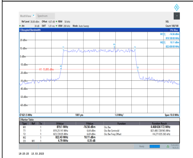
1-N26-814-824-PC3-15-5-H-5-DFT-256QAM-Outer_F ull-25@0-Ant1-4.469-4.790-<math>\leq</math>5-PASS
