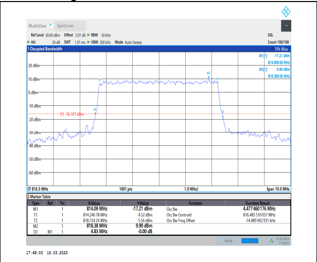
1-N26-814-824-PC3-15-5-L-6-CP-QPSK-Outer_Full-25@0-Ant1-4.477-4.830-≤5-PASS
