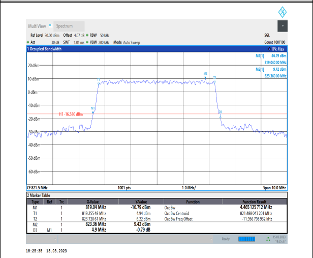
1-N26-814-824-PC3-15-5-H-6-CP-QPSK-Outer_F ull-25@0-Ant1-4.465-4.900-<math>\leq</math>5-PASS
