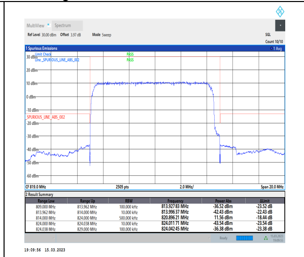
1-N26-814-824-PC3-15-10-L-3-DFT-PI2BPSK-Out_er_Full-50@0-Ant1-1--PASS-see graph
