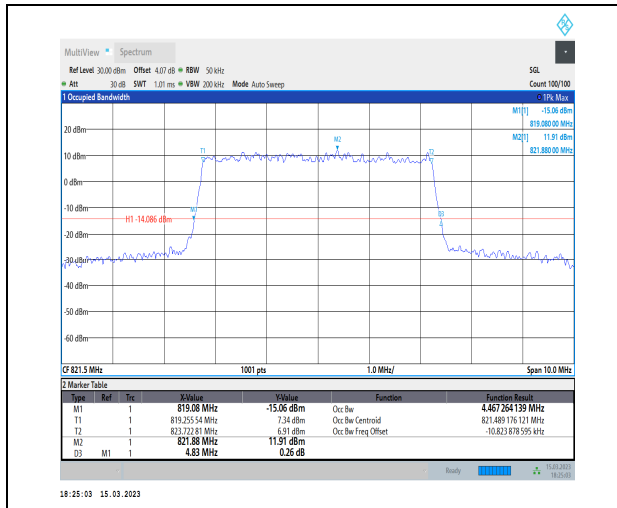
1-N26-814-824-PC3-15-5-H-3-DFT-16QAM-Outer_F ull-25@0-Ant1-4.467-4.830-<math>\leq</math>5-PASS
