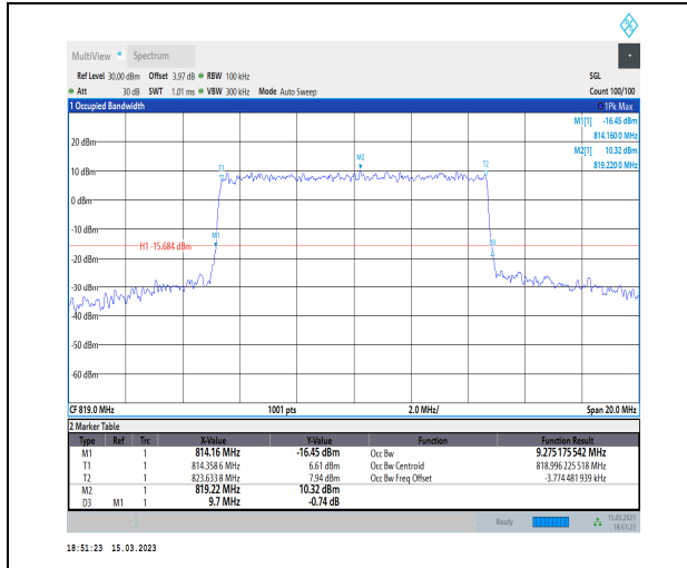
1-N26-814-824-PC3-15-10-M-6-CP-QPSK-Outer_Full I-52@0-Ant1-9.275-9.700-≤10-PASS
