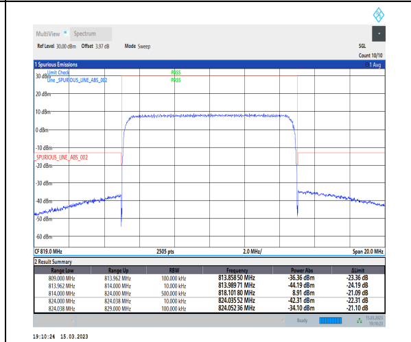
1-N26-814-824-PC3-15-10-L-6-CP-QPSK-Outer_Full-52@0-Ant1-1--PASS-see graph
