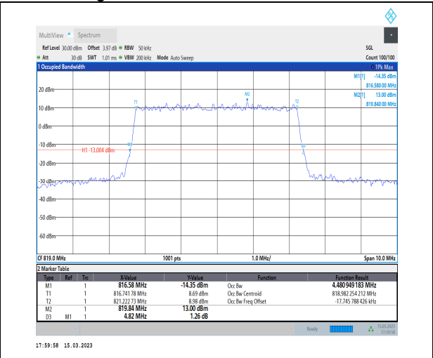
1-N26-814-824-PC3-15-5-M-1-DFT-QPSK-Outer_Fu ll-25@0-Ant1-4.481-4.820-≤5-PASS
