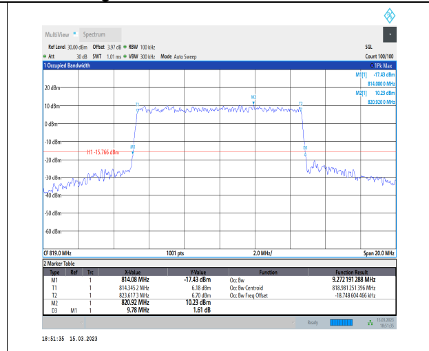
1-N26-814-824-PC3-15-10-M-7-CP-16QAM-Outer_Full ull-52@0-Ant1-9.272-9.780-≤10-PASS
