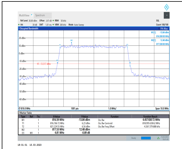
1-N26-814-824-PC3-15-5-M-4-DFT-64QAM-Outer_F ull-25@0-Ant1-4.458-4.810-<math>\leq 5</math>-PASS
