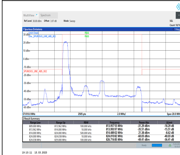
1-N26-814-824-PC3-15-10-L-4-CP-QPSK-Edge_1RB_Left-1@0-Ant1-1--PASS-see graph
