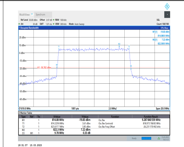
1-N26-814-824-PC3-15-10-M-9-CP-256QAM-Outer_Full Full-52@0-Ant1-9.288-9.780-≤10-PASS
