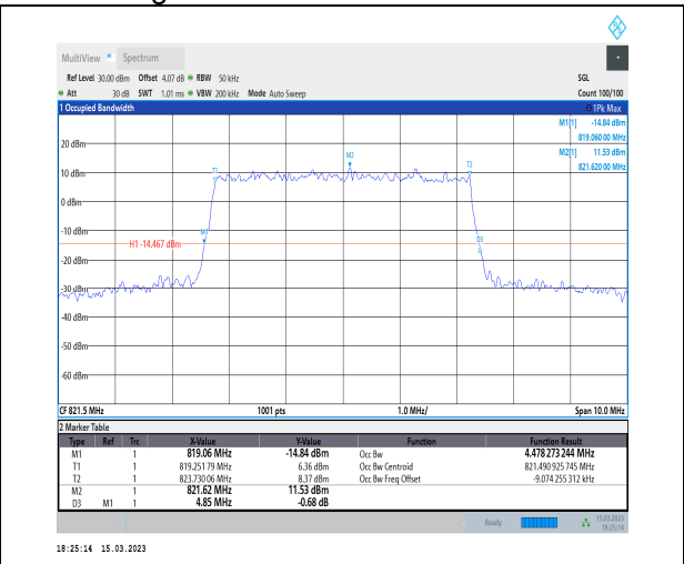
1-N26-814-824-PC3-15-5-H-4-DFT-64QAM-Outer_F ull-25@0-Ant1-4.478-4.850-<math>\leq</math>5-PASS
