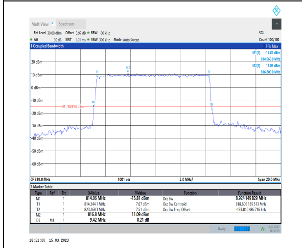
1-N26-814-824-PC3-15-10-M-4-DFT-64QAM-Outer_Full-50@0-Ant1-8.924-9.420-≤10-PASS
