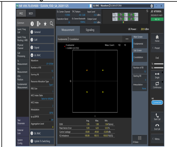
1-N26-814-824-PC3-15-10-M-6-CP-QPSK-Outer_Full-52@0-Ant1-see graph-PASS
