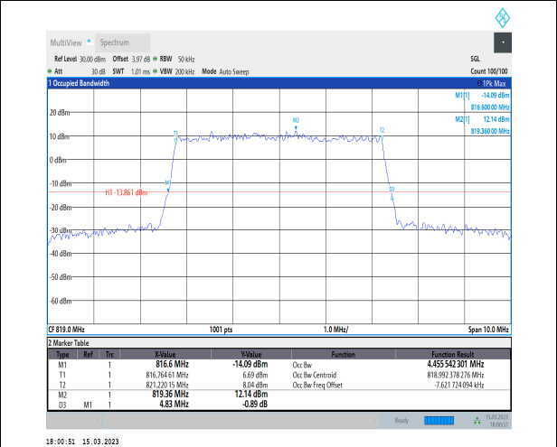
1-N26-814-824-PC3-15-5-M-3-DFT-16QAM-Outer_F ull-25@0-Ant1-4.456-4.830-≤5-PASS
