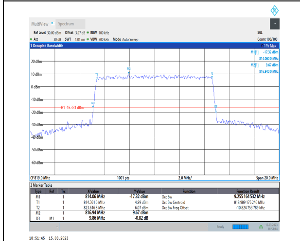
1-N26-814-824-PC3-15-10-M-8-CP-64QAM-Outer_Full ull-52@0-Ant1-9.255-9.860-≤10-PASS
