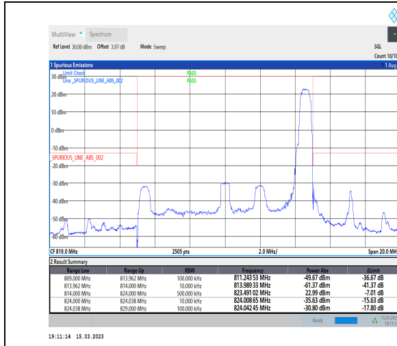
1-N26-814-824-PC3-15-10-H-2-DFT-PI2BPSK-Edge_1 RB_Right-1@51-Ant1-1--PASS-see graph
