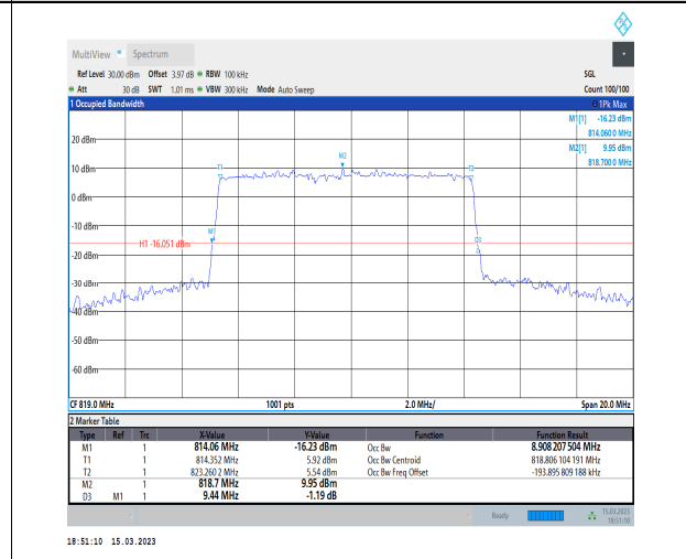
1-N26-814-824-PC3-15-10-M-5-DFT-256QAM-Outer_Full-50@0-Ant1-8.908-9.440-≤10-PASS
