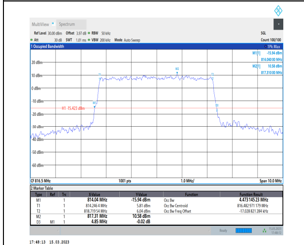
1-N26-814-824-PC3-15-5-L-7-CP-16QAM-Outer_Full-25@0-Ant1-4.473-4.850-≤5-PASS
