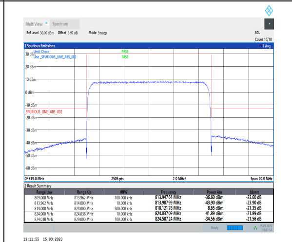
1-N26-814-824-PC3-15-10-H-6-CP-QPSK-Outer_Full-52@0-Ant1-1--PASS-see graph
