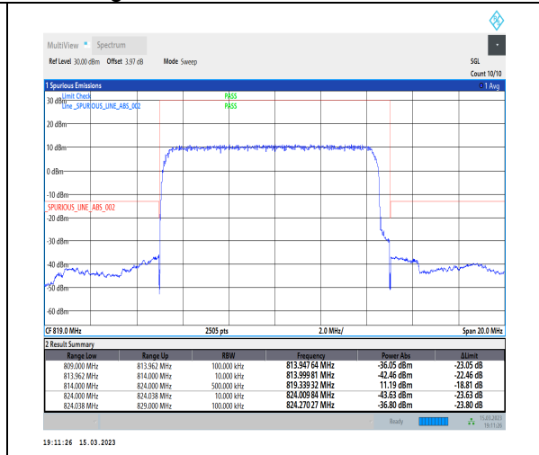
1-N26-814-824-PC3-15-10-H-3-DFT-PI2BPSK-Out_er_Full-50@0-Ant1-1--PASS-see graph
