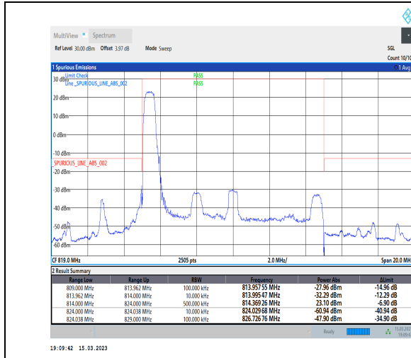
1-N26-814-824-PC3-15-10-L-1-DFT-PI2BPSK-Edge_1 RB_Left-1@0-Ant1-1--PASS-see graph
