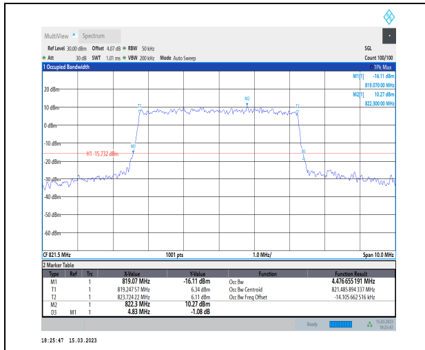
1-N26-814-824-PC3-15-5-H-7-CP-16QAM-Outer_Full-25@0-Ant1-4.477-4.830-≤5-PASS
