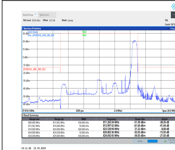
1-N26-814-824-PC3-15-10-H-5-CP-QPSK-Edge_1RB_Right-1@51-Ant1-1--PASS-see graph
