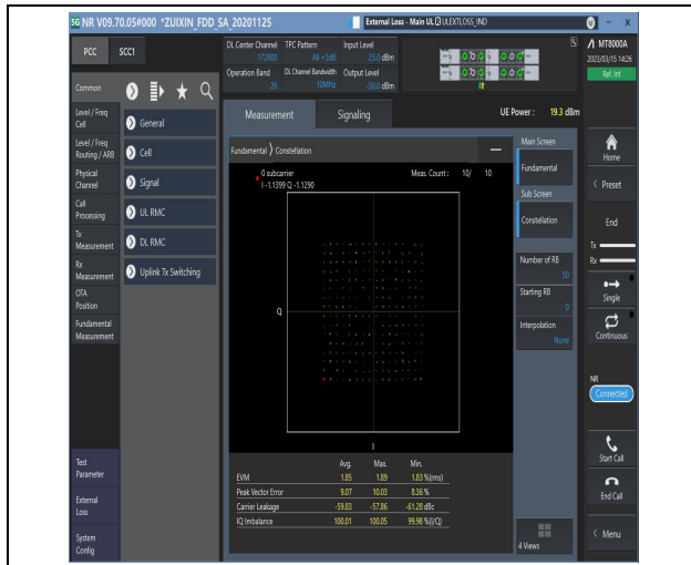
1-N26-814-824-PC3-15-10-M-5-DFT-256QAM-Outer_Full-50@0-Ant1-see graph-PASS
