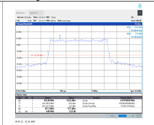
1-N26-814-824-PC3-15-5-M-5-DFT-256QAM-Outer_F ull-25@0-Ant1-4.475-4.840-<math>\leq 5</math>-PASS
