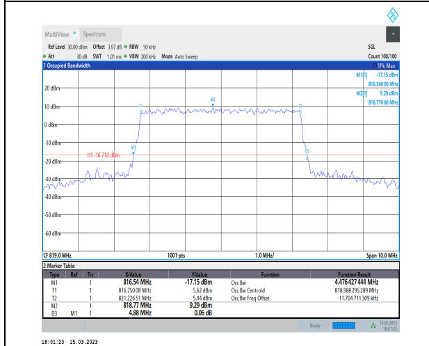
1-N26-814-824-PC3-15-5-M-6-CP-QPSK-Outer_F ull-25@0-Ant1-4.476-4.880-<math>\leq 5</math>-PASS
