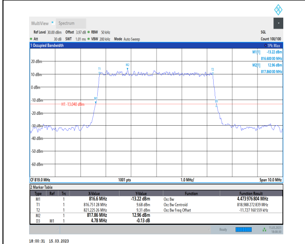
1-N26-814-824-PC3-15-5-M-2-DFT-PI2BPSK-Outer_ Full-25@0-Ant1-4.474-4.780-≤5-PASS
