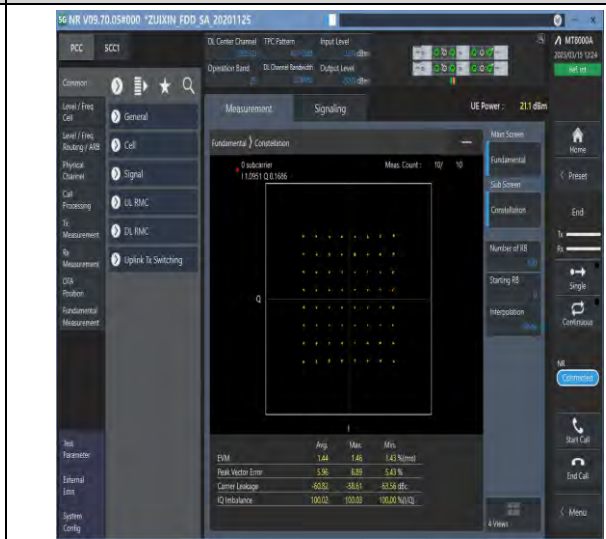
1-N25-PC3-15-20-M-4-DFT-64QAM-Outer_Full-100 @0-Ant1-see graph-PASS
