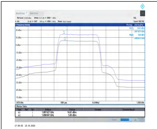
1-N25-PC3-15-20-H-1-DFT-256QAM-Outer_Full-100 @0-Ant1-8.78-100%-0.00-8.78-PASS-≤13
