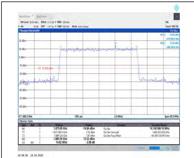
1-N25-PC3-15-15-M-6-CP-QPSK-Outer_Full-79@0-Ant1-14.141-14.820-≤15-PASS
