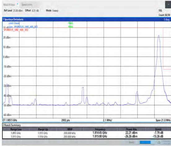
1-N25-PC3-15-20-H-2-DFT-PI2BPSK-Edge_1RB_Right-t-1@105-Ant1-1-seegraph-PASS-see graph
