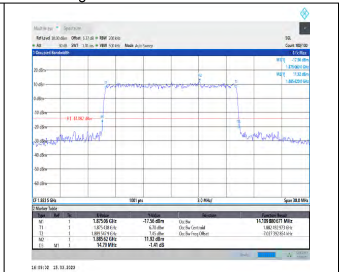
1-N25-PC3-15-15-M-7-CP-16QAM-Outer_Full-79@0-Ant1-14.11-14.790-≤15-PASS
