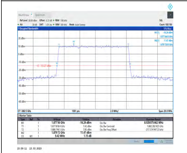
1-N25-PC3-15-10-M-3-DFT-16QAM-Outer_Full-50@0-Ant1-8.928-9.420-≤10-PASS
