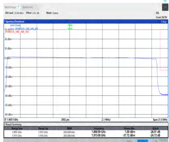
1-N25-PC3-15-20-H-6-CP-QPSK-Outer_Full-106@0-Ant1-1-seegraph-PASS-see graph
