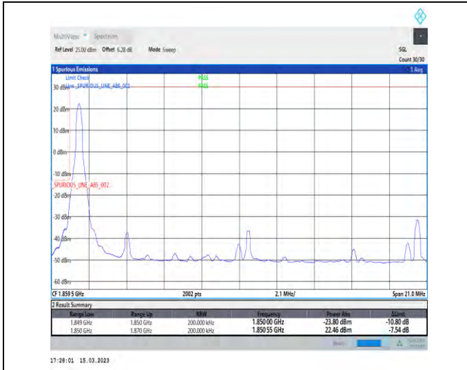
1-N25-PC3-15-20-L-1-DFT-PI2BPSK-Edge_1RB_Left-1@0-Ant1-1-seegraph-PASS-see graph
