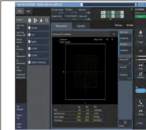
1-N25-PC3-15-20-M-5-DFT-256QAM-Outer_Full-100 @0-Ant1-see graph-PASS
