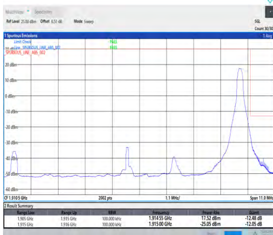
1-N25-PC3-15-10-H-5-CP-QPSK-Edge_1RB_Right-1@51-Ant1-1-seegraph-PASS-see graph
