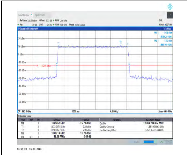
1-N25-PC3-15-20-M-3-DFT-16QAM-Outer_Full-100 @0-Ant1-17.895-18.680-≤20-PASS
