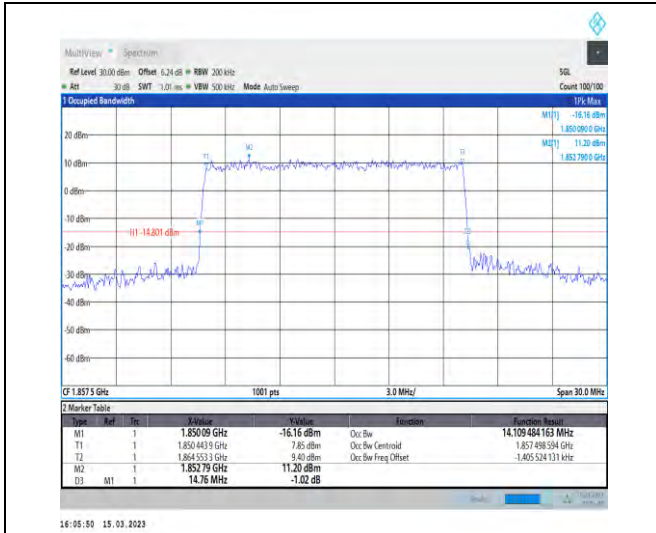
1-N25-PC3-15-15-L-7-CP-16QAM-Outer_Full-79@0-Ant1-14.109-14.760-≤15-PASS
