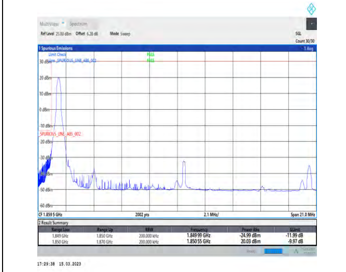
1-N25-PC3-15-20-L-4-CP-QPSK-Edge_1RB_Left-1@0-Ant1-1-seegraph-PASS-see graph
