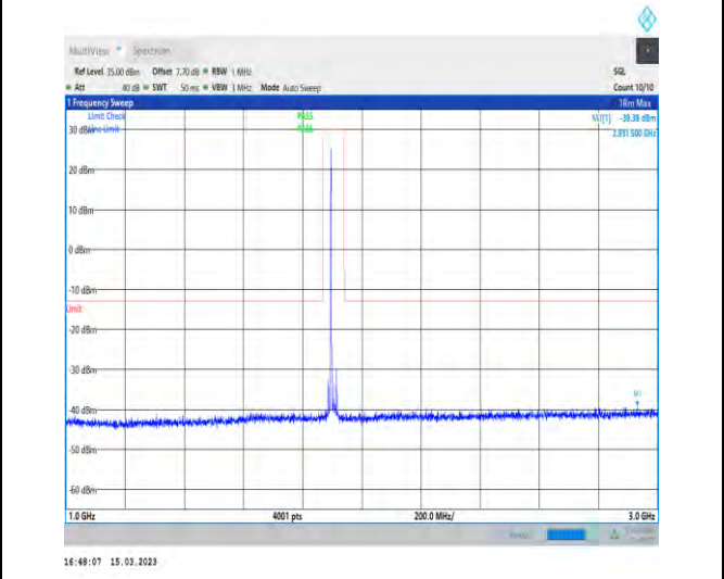
1-N25-PC3-15-20-H-1-DFT-PI2BPSK-Inner_1RB_Lef t-1@1-1000-3000-Ant1-2931.50--39.38--13-PASS
