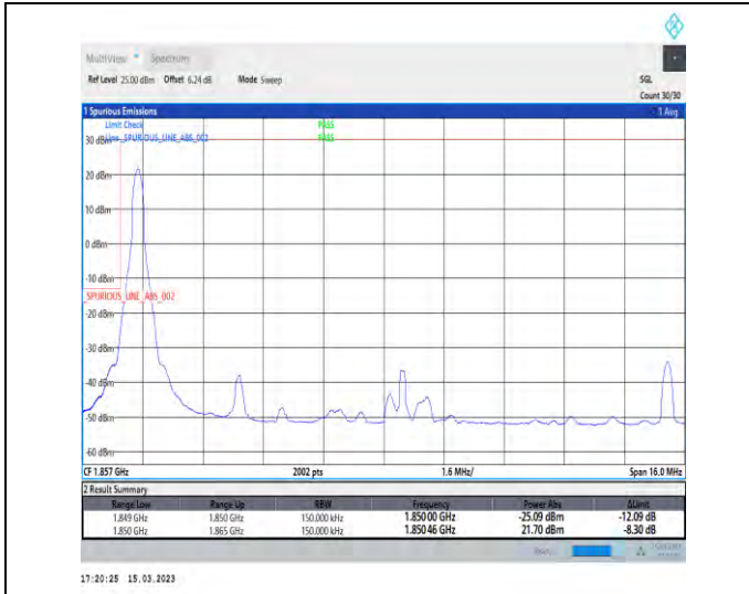
1-N25-PC3-15-15-L-1-DFT-PI2BPSK-Edge_1RB_Left-1@0-Ant1-1-seegraph-PASS-see graph
