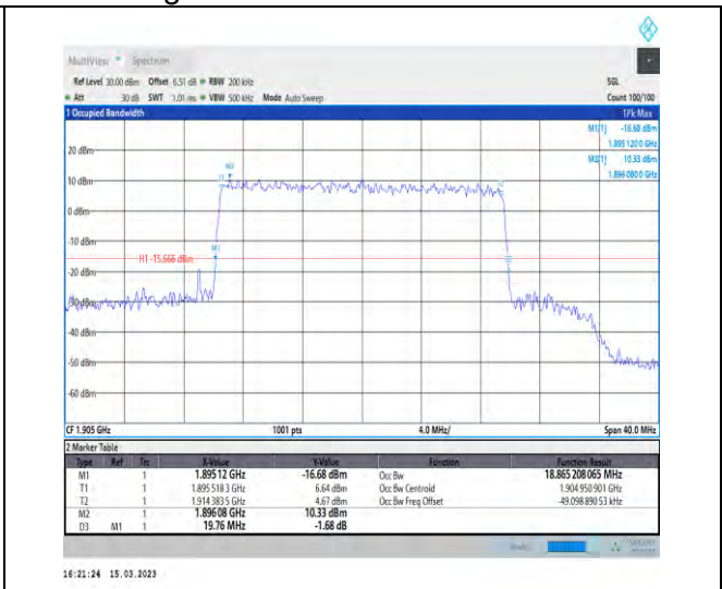
1-N25-PC3-15-20-H-7-CP-16QAM-Outer_Full-106@0 -Ant1-18.865-19.760-≤20-PASS
