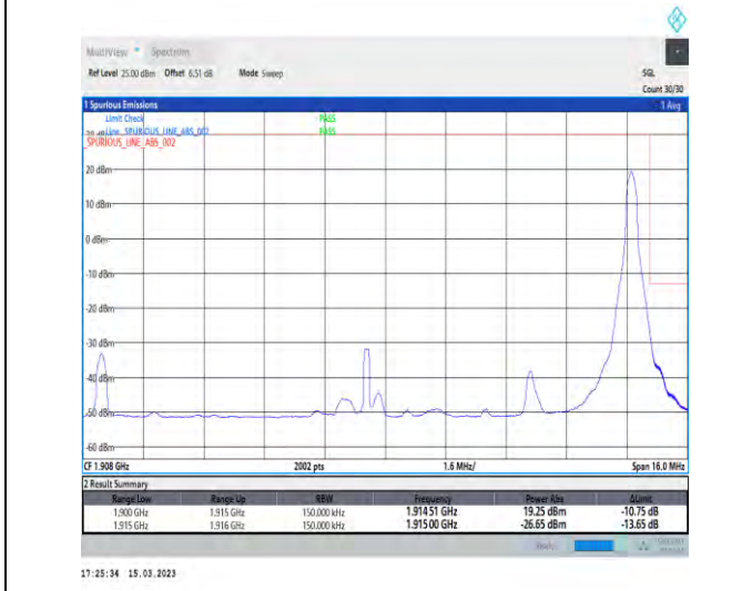
1-N25-PC3-15-15-H-5-CP-QPSK-Edge_1RB_Right-1@78-Ant1-1-seegraph-PASS-see graph
