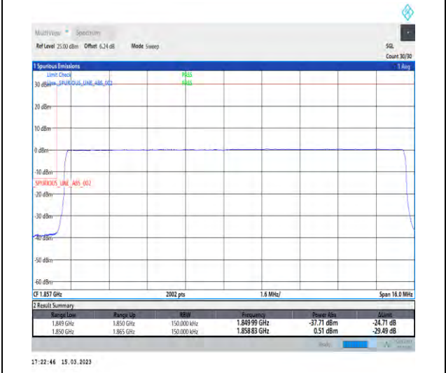
1-N25-PC3-15-15-L-6-CP-QPSK-Outer_Full-79@0-Ant1-1-seegraph-PASS-see graph
