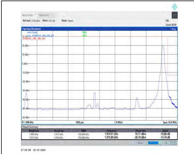
1-N25-PC3-15-15-H-2-DFT-PI2BPSK-Edge_1RB_Right-t1@78-Ant1-1-seegraph-PASS-see graph
