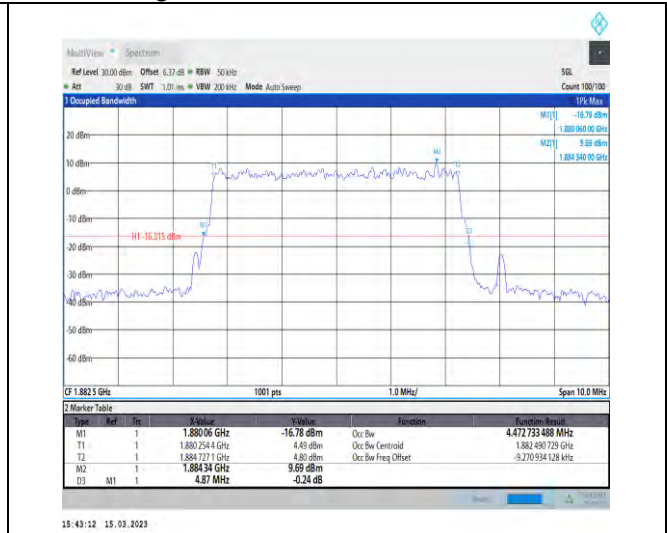
1-N25-PC3-15-5-M-5-DFT-256QAM-Outer_Full-25@0-Ant1-4.473-4.870-≤5-PASS
