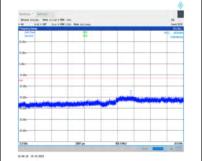
1-N25-PC3-15-20-M-1-DFT-PI2BPSK-Inner_1RB_Lef t-1@1-12000-20000-Ant1-17460.00--28.04--13-PASS
