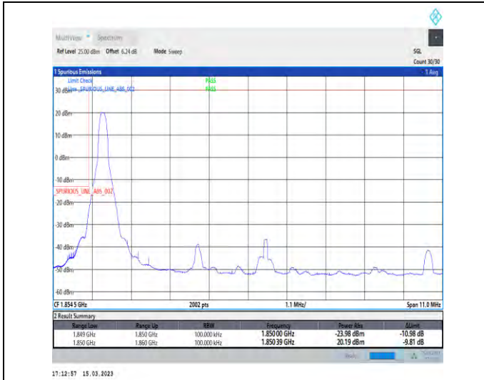
1-N25-PC3-15-10-L-1-DFT-PI2BPSK-Edge_1RB_Left-1@0-Ant1-1-seegraph-PASS-see graph
