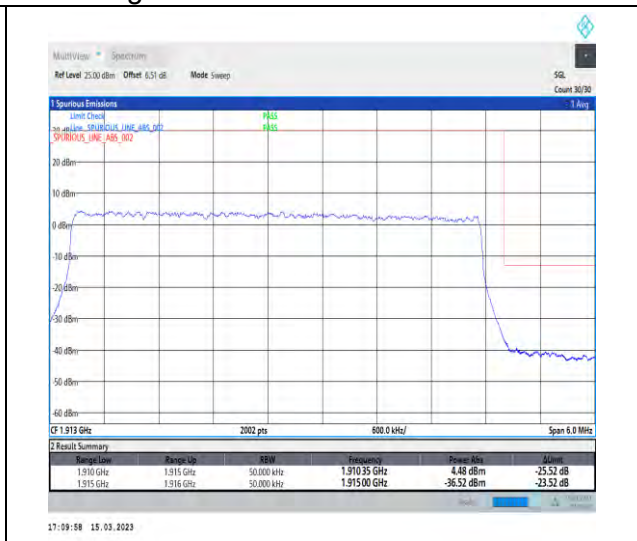
1-N25-PC3-15-5-H-3-DFT-PI2BPSK-Outer_Full-25@0-Ant1-1-seegraph-PASS-see graph
