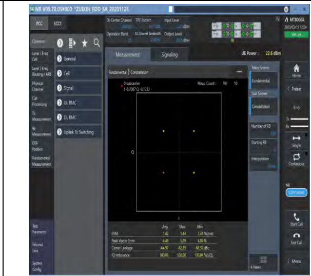
1-N25-PC3-15-20-M-2-DFT-QPSK-Outer_Full-100 @0-Ant1-see graph-PASS
