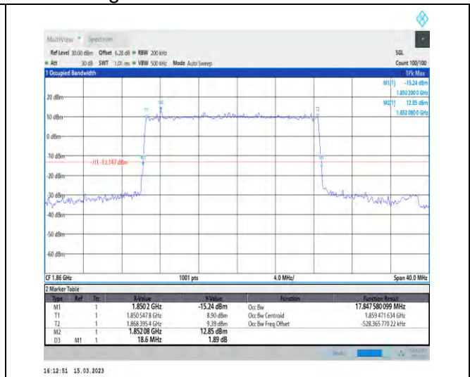
1-N25-PC3-15-20-L-1-DFT-QPSK-Outer_Full-100@0 -Ant1-17.848-18.600-≤20-PASS
