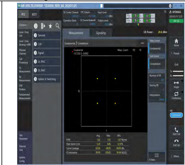
1-N25-PC3-15-20-M-6-CP-QPSK-Outer_Full-106 @0-Ant1-see graph-PASS
