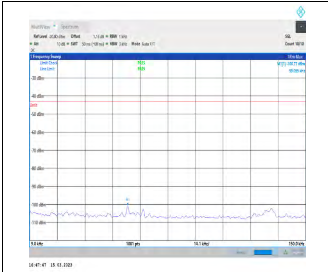
1-N25-PC3-15-20-H-1-DFT-PI2BPSK-Inner_1RB_L eft-1@1-0.009-0.15-Ant1-0.06--100.77--43-PASS
