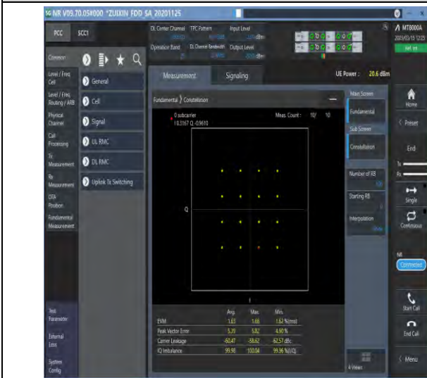
1-N25-PC3-15-20-M-7-CP-16QAM-Outer_Full-106 @0-Ant1-see graph-PASS
