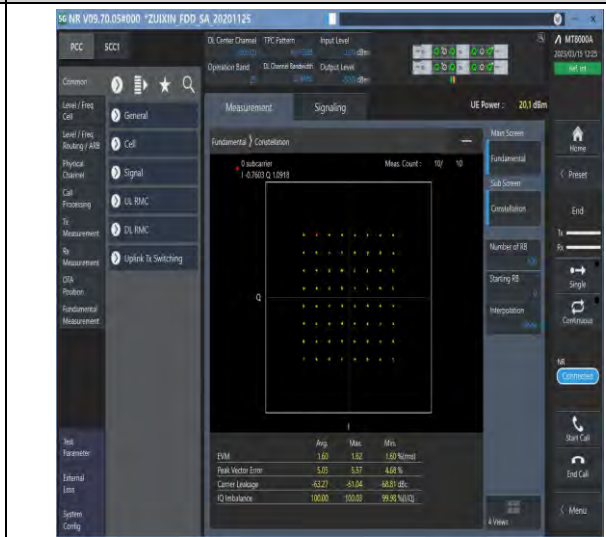
1-N25-PC3-15-20-M-8-CP-64QAM-Outer_Full-106 @0-Ant1-see graph-PASS
