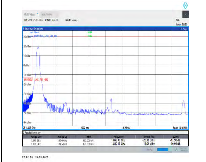
1-N25-PC3-15-15-L-4-CP-QPSK-Edge_1RB_Left-1@0-Ant1-1-seegraph-PASS-see graph
