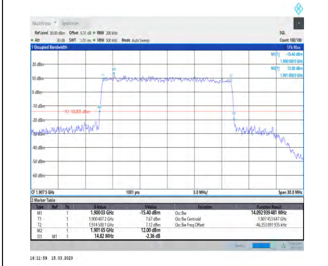
1-N25-PC3-15-15-H-7-CP-16QAM-Outer_Full-79@0 -Ant1-14.093-14.820-≤15-PASS
