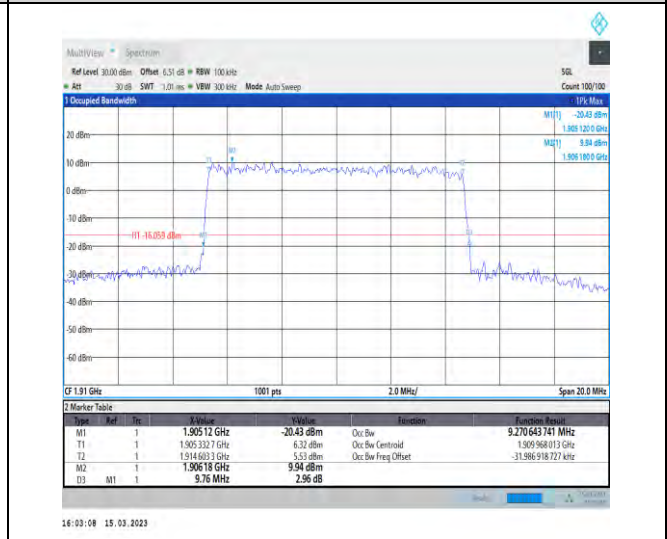
1-N25-PC3-15-10-H-7-CP-16QAM-Outer_Full-52@0 -Ant1-9.271-9.760-≤10-PASS
