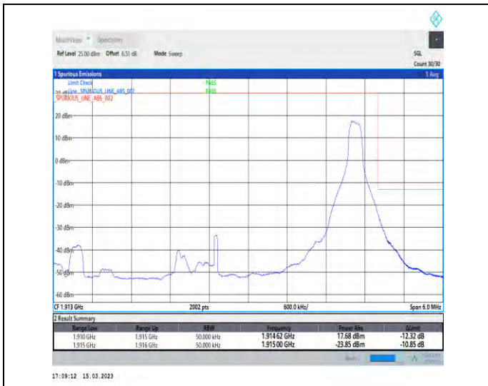
1-N25-PC3-15-5-H-2-DFT-PI2BPSK-Edge_1RB_Right-1@24-Ant1-1-seegraph-PASS-see graph
