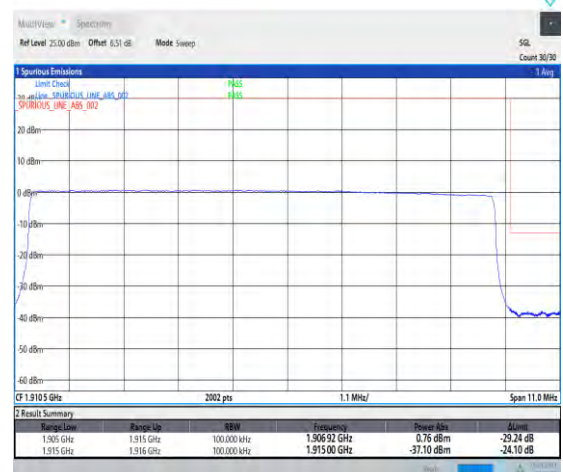
1-N25-PC3-15-10-H-6-CP-QPSK-Outer_Full-52@0-Ant1-1-seegraph-PASS-see graph
