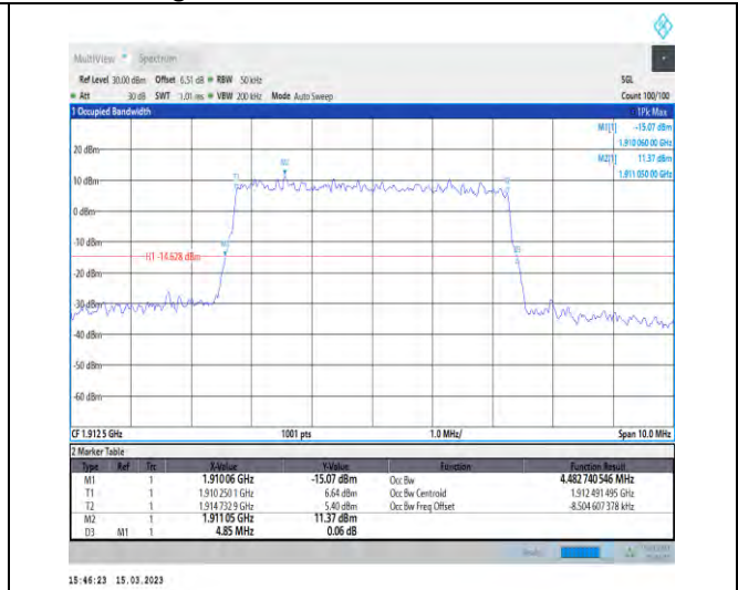
1-N25-PC3-15-5-H-4-DFT-64QAM-Outer_Full-25@0- Ant1-4.483-4.850-≤5-PASS
