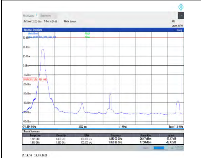
1-N25-PC3-15-10-L-4-CP-QPSK-Edge_1RB_Left-1@0-Ant1-1-seegraph-PASS-see graph
