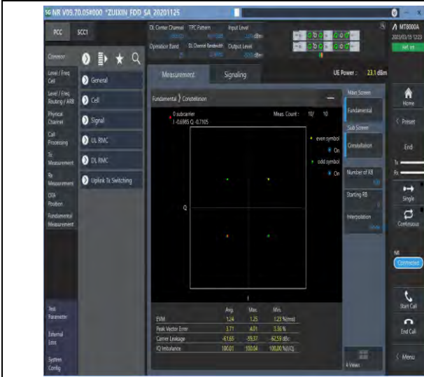
1-N25-PC3-15-20-M-1-DFT-PI2BPSK-Outer_Full-100 @0-Ant1-see graph-PASS
