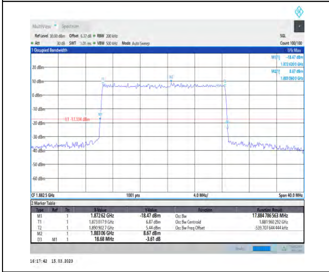
1-N25-PC3-15-20-M-5-DFT-256QAM-Outer_Full-100 @0-Ant1-17.885-18.680-≤20-PASS
