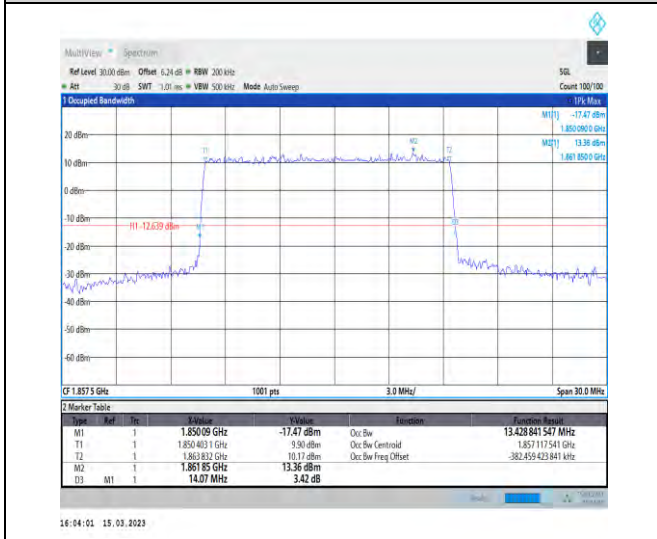
1-N25-PC3-15-15-L-1-DFT-QPSK-Outer_Full-75@0- Ant1-13.429-14.070-≤15-PASS
