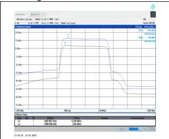
1-N25-PC3-15-20-H-2-CP-256QAM-Outer_Full-106 @0-Ant1-9.50-100%-0.00-9.50-PASS-≤13
