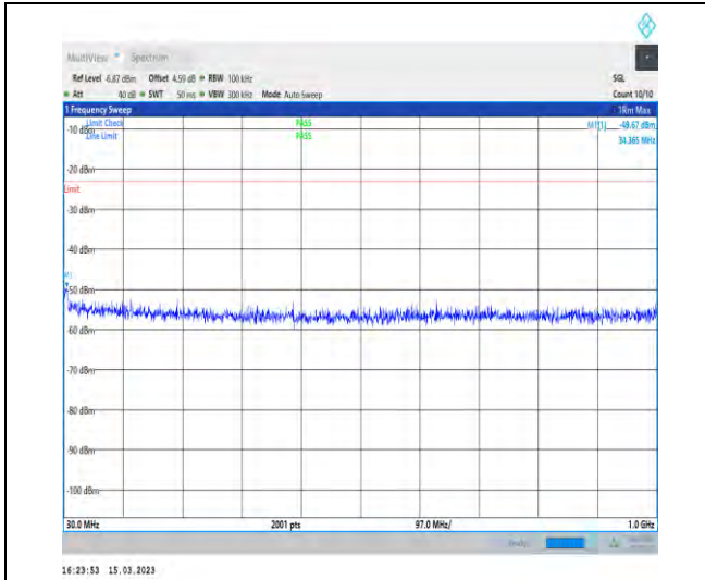
1-N25-PC3-15-20-M-1-DFT-PI2BPSK-Inner_1RB_L eft-1@1-30-1000-Ant1-34.37--49.67--23-PASS
