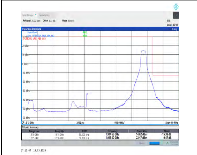
1-N25-PC3-15-5-H-5-CP-QPSK-Edge_1RB_Right-1@24-Ant1-1-seegraph-PASS-see graph
