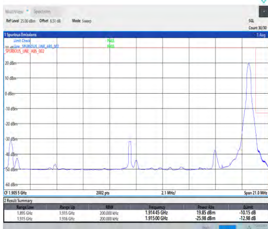
1-N25-PC3-15-20-H-5-CP-QPSK-Edge_1RB_Right-1@105-Ant1-1-seegraph-PASS-see graph
