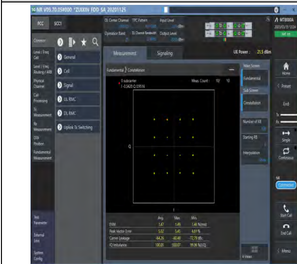
1-N25-PC3-15-20-M-3-DFT-16QAM-Outer_Full-100 @0-Ant1-see graph-PASS
