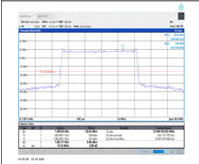
1-N25-PC3-15-15-L-5-DFT-256QAM-Outer_Full-75 @0-Ant1-13.44-14.160-≤15-PASS
