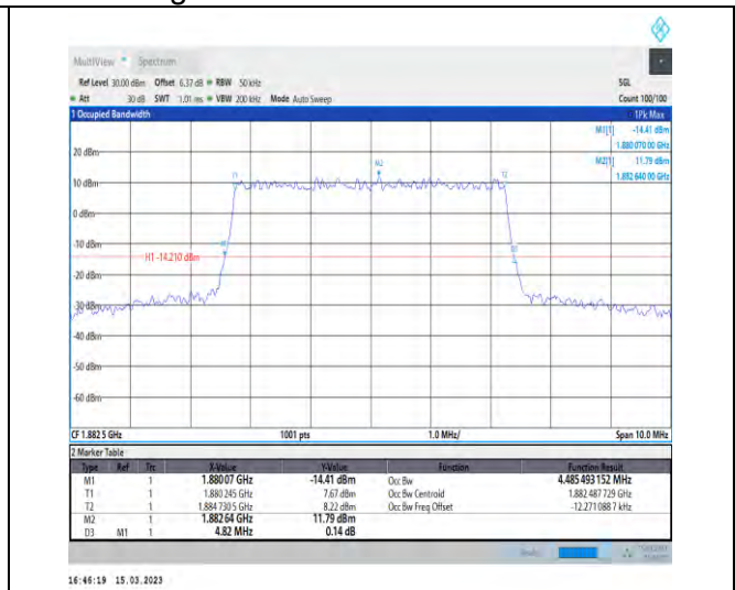
1-N25-PC3-15-5-M-1-DFT-QPSK-Outer_Full-25@0-Ant1-4.485-4.820-≤5-PASS
