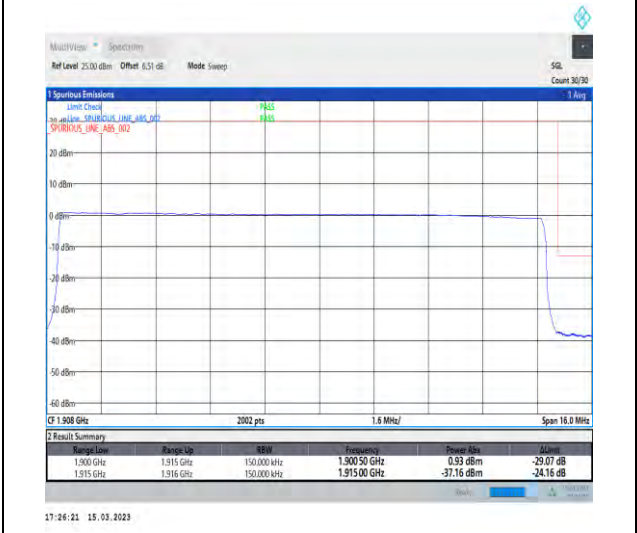
1-N25-PC3-15-15-H-6-CP-QPSK-Outer_Full-79@0-Ant1-1-seegraph-PASS-see graph
