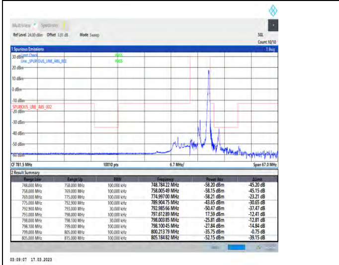
1-N14-PC3-15-5-H-5-CP-QPSK-Edge_1RB_Right-1@24-Ant1-1--PASS-see graph
