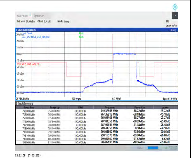
1-N14-PC3-15-10-H-6-CP-QPSK-Outer_Full-52@0-Ant1-1--PASS-see graph
