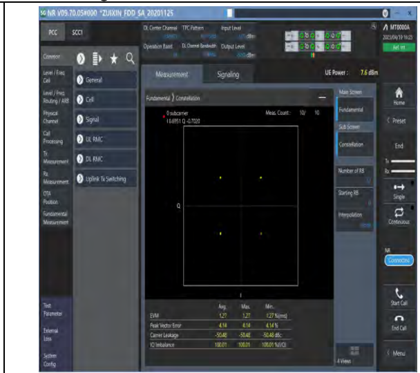
1-N14-PC3-15-10-M-6-CP-QPSK-Outer_Full-52@0-Ant1-see graph-PASS
