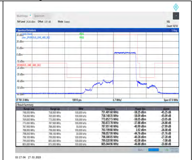
1-N14-PC3-15-10-L-3-DFT-PI2BPSK-Outer_Full-50@0-Ant1-1--PASS-see graph
