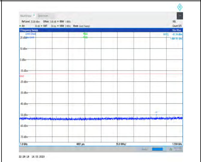
1-N14-PC3-15-10-M-1-DFT-PI2BPSK-Inner_1RB_Lef t-1@1-1000-1559-Ant1-1469.14--51.14--13-PASS
