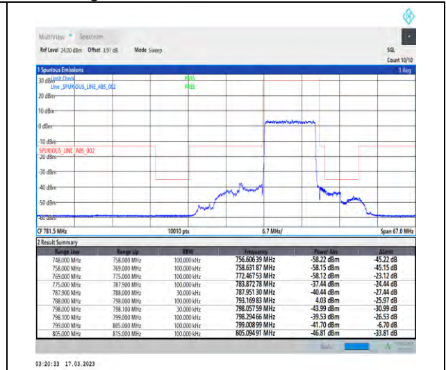
1-N14-PC3-15-10-H-3-DFT-PI2BPSK-Outer_Full-50@0-Ant1-1--PASS-see graph
