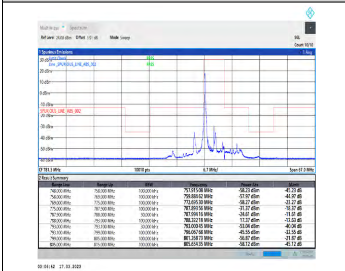
1-N14-PC3-15-5-L-4-CP-QPSK-Edge_1RB_Left-1@0-Ant1-1--PASS-see graph
