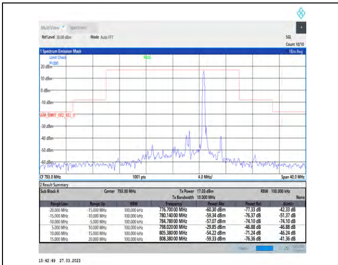
1-N14-PC3-15-5-H-2-DFT-PI2BPSK-Edge_1RB_Right-1@24-Ant1-1--PASS-see graph
