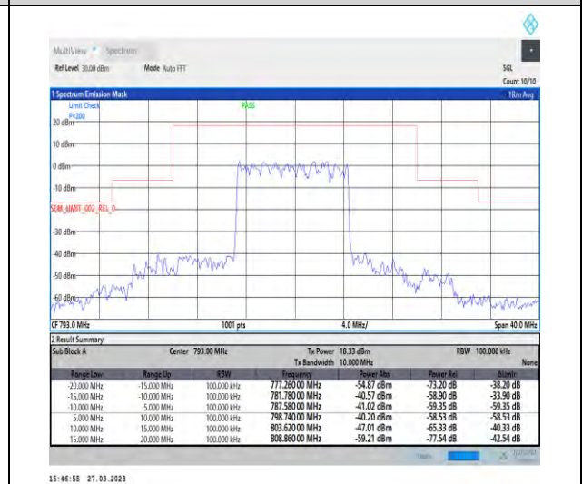
1-N14-PC3-15-10-H-6-CP-QPSK-Outer_Full-52@ 0-Ant1-1--PASS-see graph
