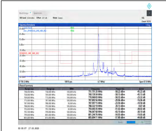
1-N14-PC3-15-5-L-1-DFT-PI2BPSK-Edge_1RB_Left-1 @0-Ant1-1--PASS-see graph
