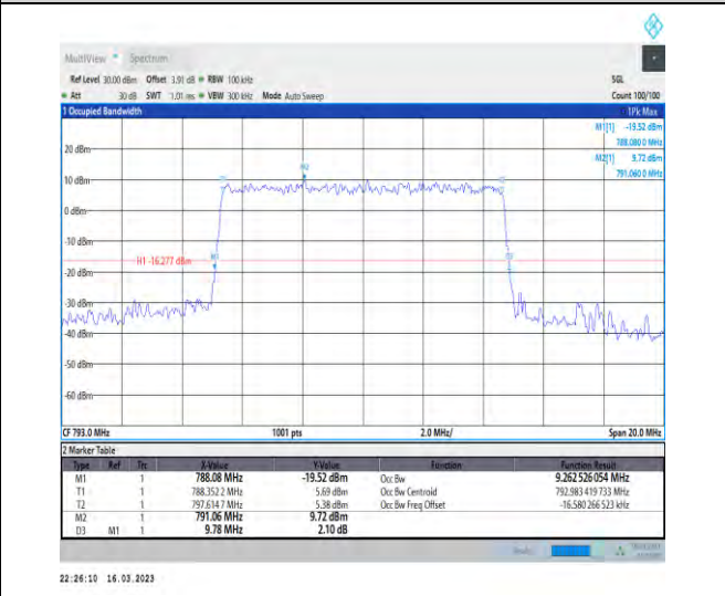
1-N14-PC3-15-10-H-7-CP-16QAM-Outer_Full-52@0 -Ant1-9.263-9.780-≤10-PASS
