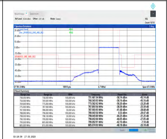
1-N14-PC3-15-10-L-6-CP-QPSK-Outer_Full-52@0-Ant1-1--PASS-see graph
