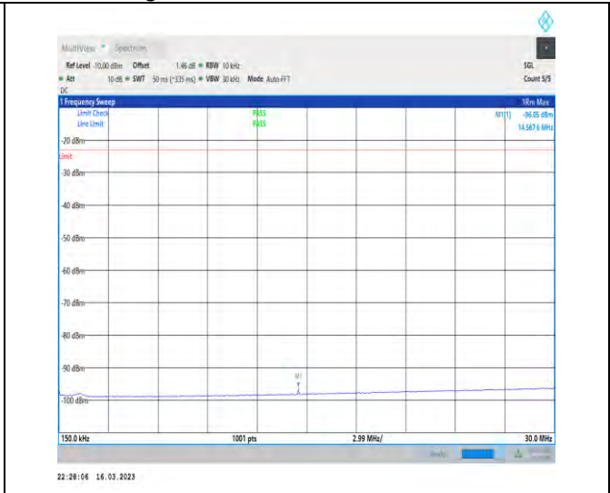
1-N14-PC3-15-10-M-1-DFT-PI2BPSK-Inner_1RB_Lef t-1@1-0.15-30-Ant1-14.57--96.05--23-PASS
