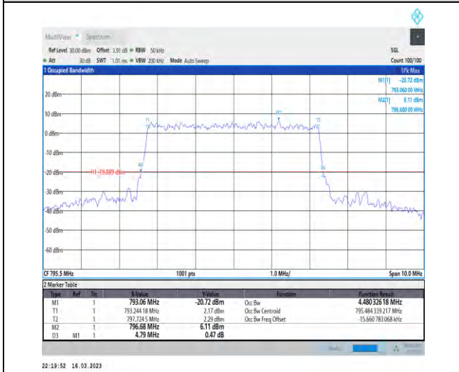
1-N14-PC3-15-5-H-9-CP-256QAM-Outer_Full-25@0-Ant1-4.48-4.790-≤5-PASS
