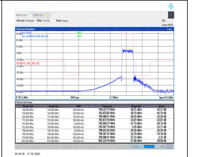
1-N14-PC3-15-5-H-6-CP-QPSK-Outer_Full-25@0-Ant1-1--PASS-see graph
