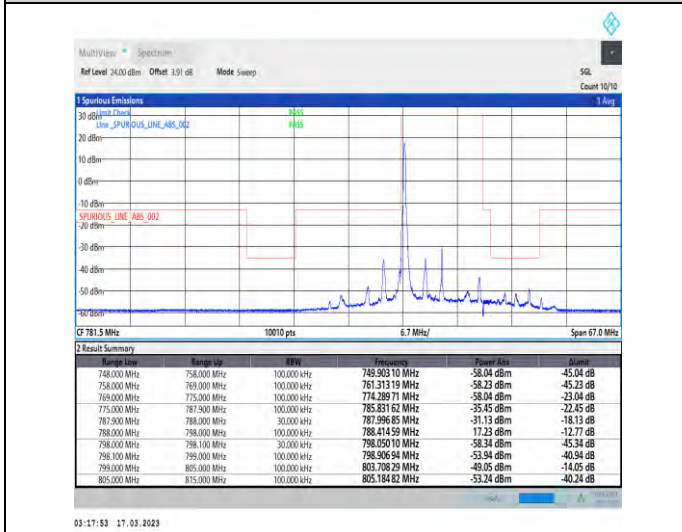
1-N14-PC3-15-10-L-4-CP-QPSK-Edge_1RB_Left-1@0-Ant1-1--PASS-see graph
