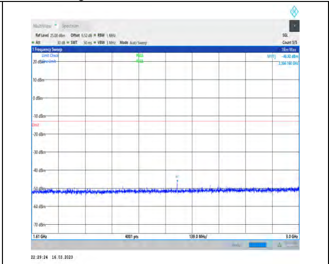
1-N14-PC3-15-10-H-1-DFT-PI2BPSK-Inner_1RB_L eft-1@1-1610-3000-Ant1-2366.16--46.92--13-PASS
