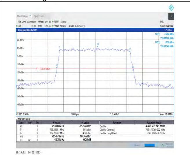
1-N14-PC3-15-5-H-4-DFT-64QAM-Outer_Full-25@0- Ant1-4.459-4.820-≤5-PASS
