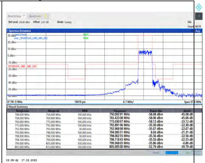
1-N14-PC3-15-5-H-3-DFT-PI2BPSK-Outer_Full-25@0-Ant1-1--PASS-see graph
