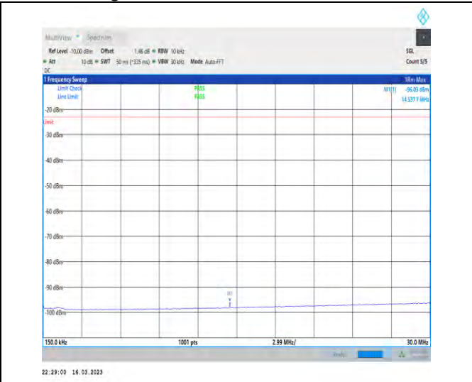
1-N14-PC3-15-10-H-1-DFT-PI2BPSK-Inner_1RB_Lef t-1@1-0.15-30-Ant1-14.54--96.03--23-PASS
