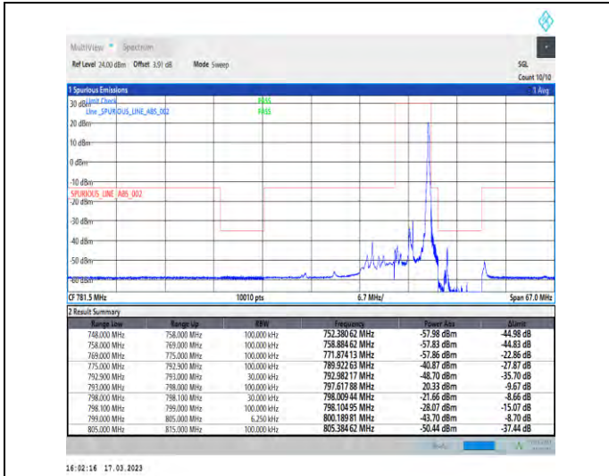
1-N14-PC3-15-5-H-2-DFT-PI2BPSK-Edge_1RB_Right-1@24-Ant1-1--PASS-see graph
