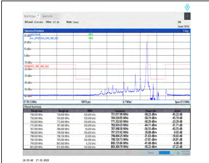
1-N14-PC3-15-10-H-2-DFT-PI2BPSK-Edge_1RB_Right-t-1@51-Ant1-1--PASS-see graph
