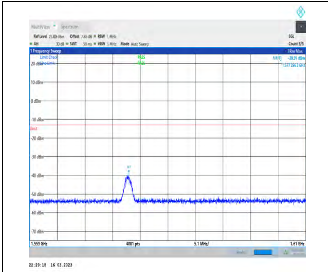
1-N14-PC3-15-10-H-1-DFT-PI2BPSK-Inner_1RB_L eft-1@1-1559-1610-Ant1-1577.30--38.91--13-PASS
