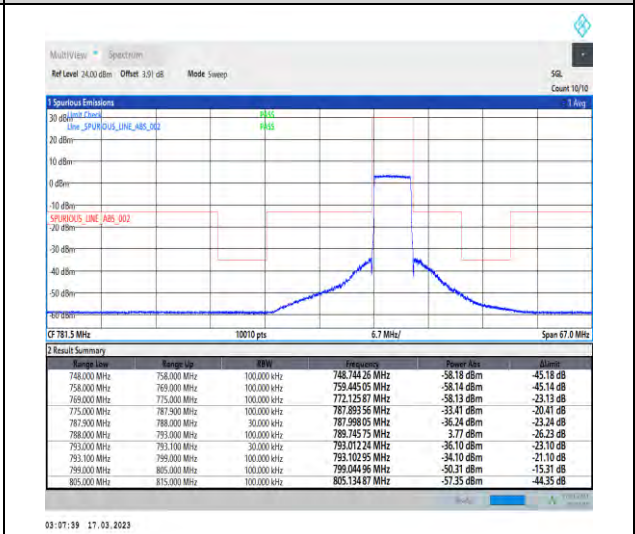
1-N14-PC3-15-5-L-6-CP-QPSK-Outer_Full-25@0-Ant1-1--PASS-see graph
