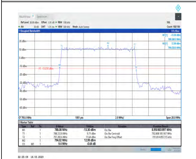
1-N14-PC3-15-10-H-2-DFT-PI2BPSK-Outer_Full-50 @0-Ant1-8.951-9.400-≤10-PASS
