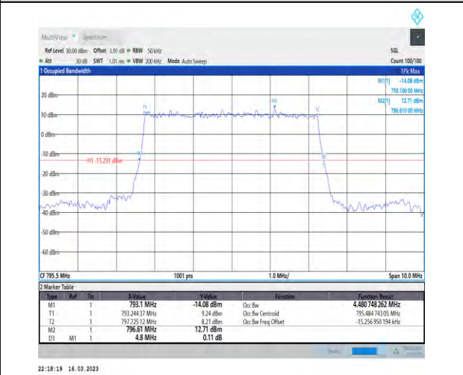
1-N14-PC3-15-5-H-2-DFT-PI2BPSK-Outer_Full-25@0-Ant1-4.481-4.800-≤5-PASS
