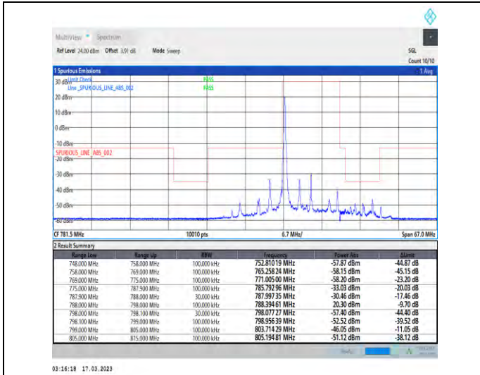
1-N14-PC3-15-10-L-1-DFT-PI2BPSK-Edge_1RB_Left-1@0-Ant1-1--PASS-see graph
