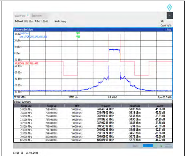
1-N14-PC3-15-5-L-3-DFT-PI2BPSK-Outer_Full-25 @0-Ant1-1--PASS-see graph
