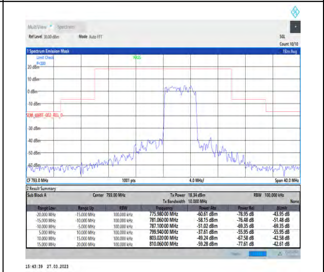
1-N14-PC3-15-5-H-6-CP-QPSK-Outer_Full-25@0-Ant1-1--PASS-see graph
