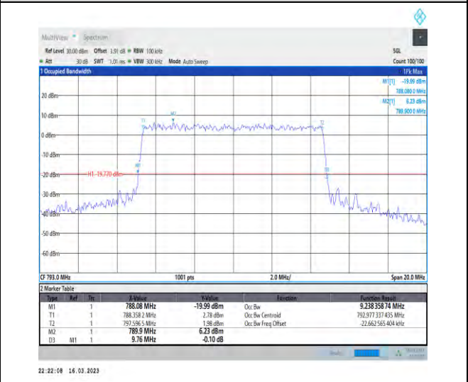
1-N14-PC3-15-10-L-9-CP-256QAM-Outer_Full-52@0-Ant1-9.238-9.760-≤10-PASS
