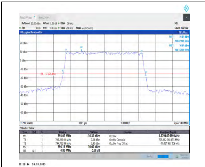
1-N14-PC3-15-5-H-3-DFT-16QAM-Outer_Full-25@0 -Ant1-4.48-4.860-≤5-PASS
