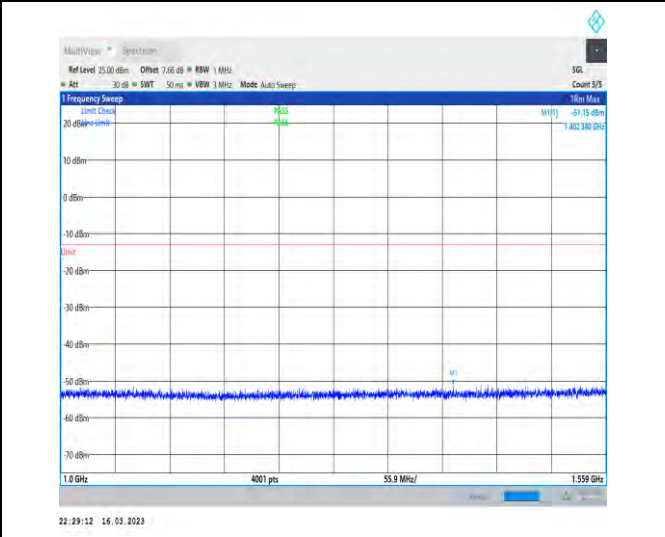
1-N14-PC3-15-10-H-1-DFT-PI2BPSK-Inner_1RB_Lef t-1@1-1000-1559-Ant1-1402.34--51.15--13-PASS
