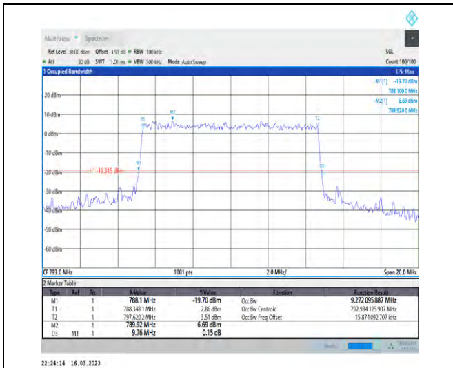
1-N14-PC3-15-10-M-9-CP-256QAM-Outer_Full-52@ 0-Ant1-9.272-9.760-≤10-PASS
