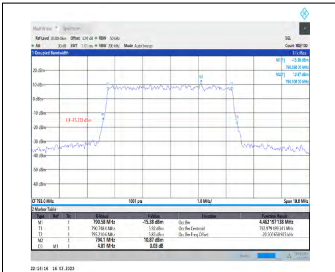
1-N14-PC3-15-5-M-4-DFT-64QAM-Outer_Full-25@0 -Ant1-4.462-4.810-≤5-PASS
