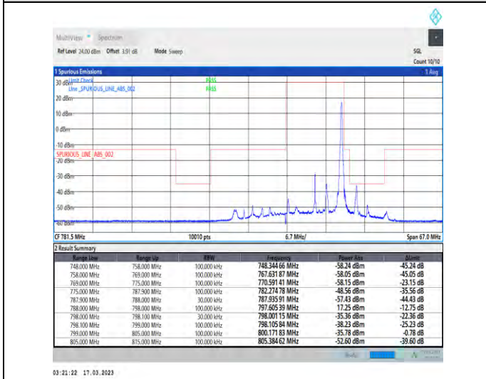
1-N14-PC3-15-10-H-5-CP-QPSK-Edge_1RB_Right-1@51-Ant1-1--PASS-see graph
