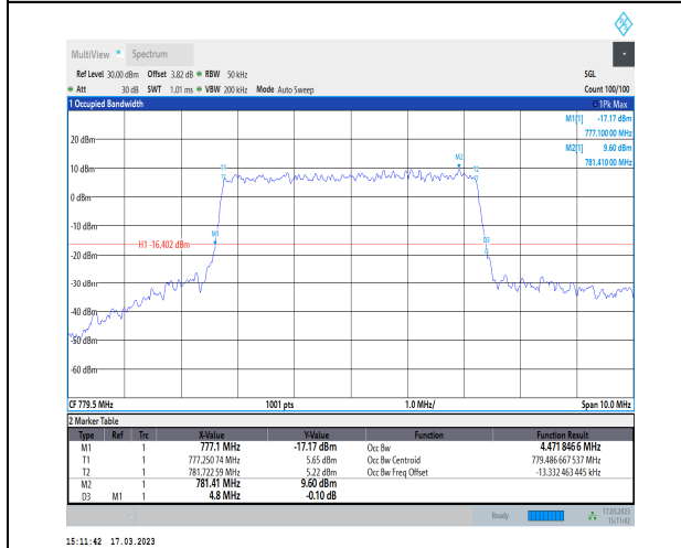
1-N13-PC3-15-5-L-7-CP-16QAM-Outer_Full-25@0-A nt1-4.472-4.800-<math>\leq 5</math>-PASS
