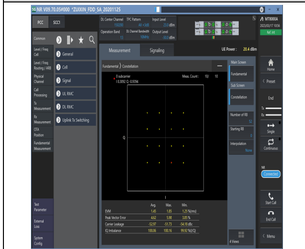
1-N13-PC3-15-10-M-7-CP-16QAM-Outer_Full-52@0-Ant1-see graph-PASS
