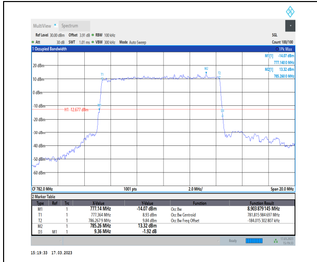
1-N13-PC3-15-10-M-2-DFT-PI2BPSK-Outer_Full-50 @0-Ant1-8.904-9.360-≤10-PASS
