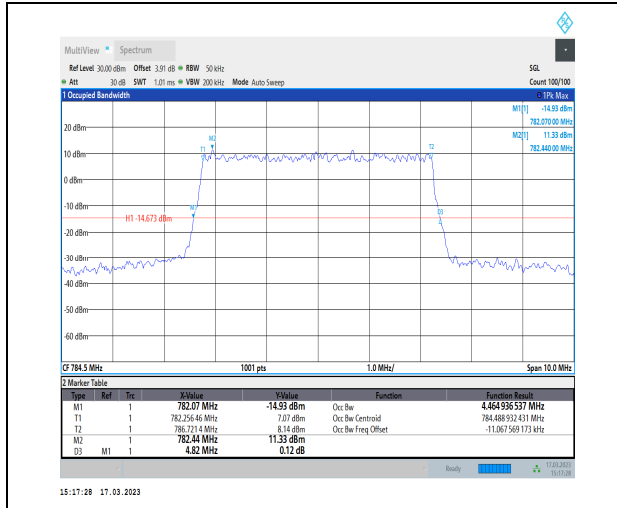
1-N13-PC3-15-5-H-3-DFT-16QAM-Outer_Full-25@0-Ant1-4.465-4.820-≤5-PASS
