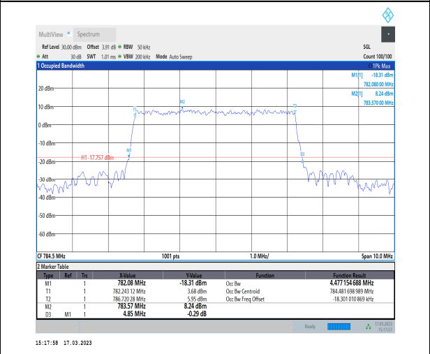
1-N13-PC3-15-5-H-6-CP-QPSK-Outer_Full-25@0-Ant1-4.477-4.850-≤5-PASS
