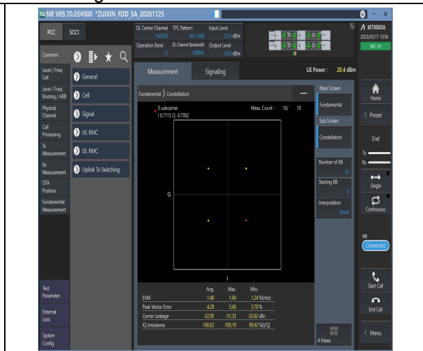
1-N13-PC3-15-10-M-6-CP-QPSK-Outer_Full-52@0-Ant1-see graph-PASS
