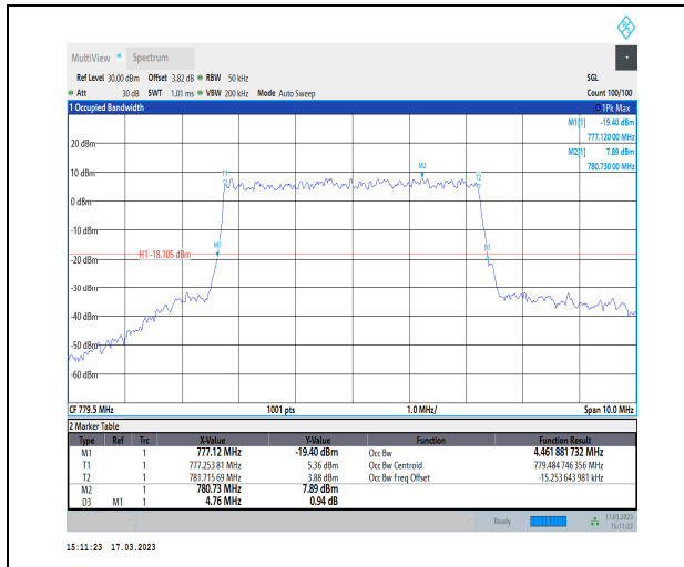
1-N13-PC3-15-5-L-5-DFT-256QAM-Outer_Full-25@ 0-Ant1-4.462-4.760-<math>\leq 5</math>-PASS
