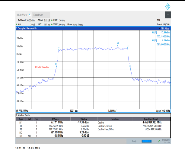
1-N13-PC3-15-5-L-8-CP-64QAM-Outer_Full-25@0- Ant1-4.459-4.800-<math>\leq 5</math>-PASS
