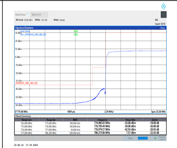
1-N13-PC3-15-10-L-6-CP-QPSK-Outer_Full-52@0-Ant1-1--PASS-see graph
