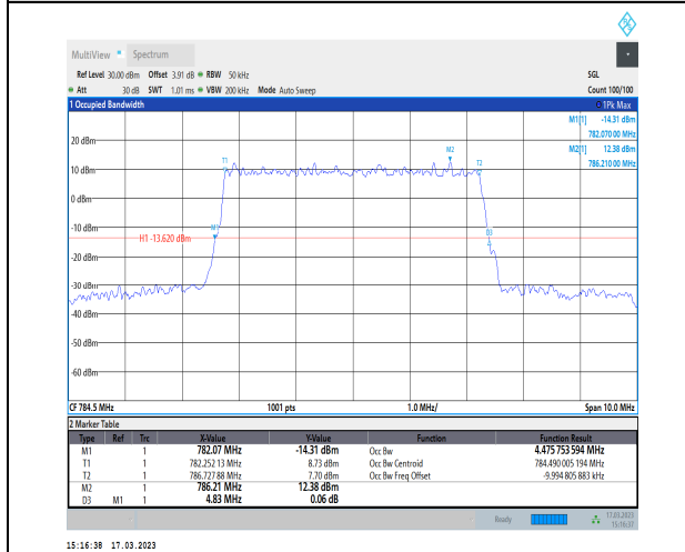
1-N13-PC3-15-5-H-1-DFT-QPSK-Outer_Full-25@0-Ant1-4.476-4.830-≤5-PASS
