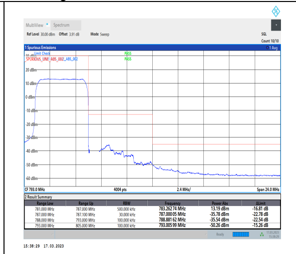
1-N13-PC3-15-5-H-3-DFT-PI2BPSK-Outer_Full-25@0-Ant1-1--PASS-see graph
