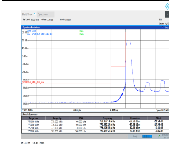
1-N13-PC3-15-10-L-4-CP-QPSK-Edge_1RB_Left-1@0-Ant1-1--PASS-see graph
