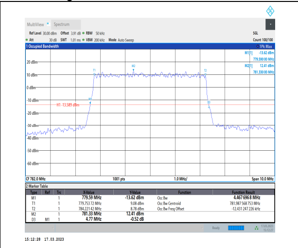
1-N13-PC3-15-5-M-1-DFT-QPSK-Outer_Full-25@0-Ant1-4.468-4.770-≤5-PASS
