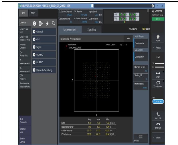
1-N13-PC3-15-10-M-5-DFT-256QAM-Outer_Full-50@0-Ant1-see graph-PASS
