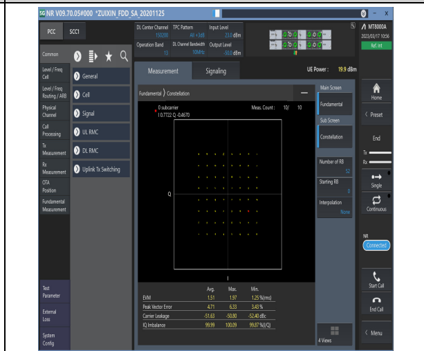
1-N13-PC3-15-10-M-8-CP-64QAM-Outer_Full-52@0-Ant1-see graph-PASS
