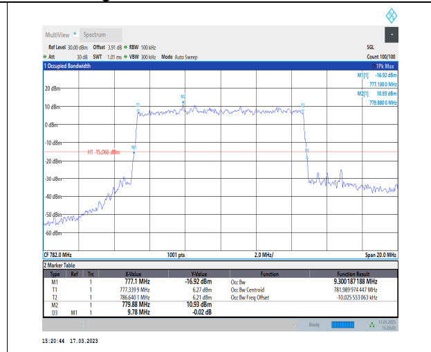
1-N13-PC3-15-10-M-7-CP-16QAM-Outer_Full-52@0-Ant1-9.3-9.780-≤10-PASS
