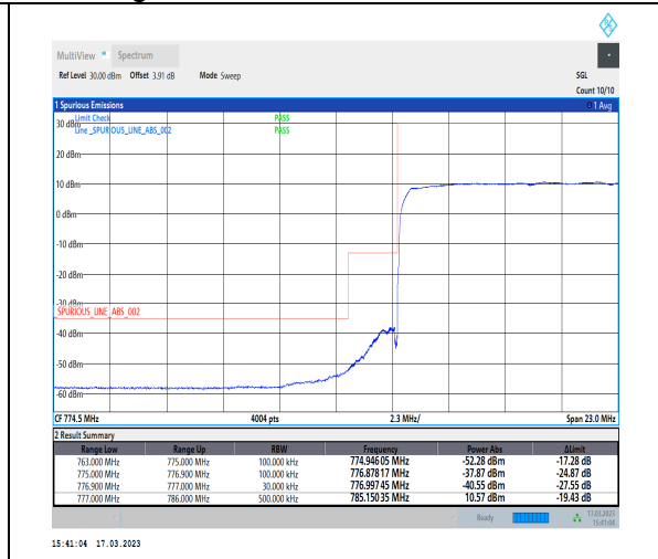
1-N13-PC3-15-10-L-3-DFT-PI2BPSK-Outer_Full-50@0-Ant1-1--PASS-see graph
