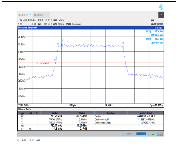
1-N13-PC3-15-5-M-4-DFT-64QAM-Outer_Full-25@0 -Ant1-4.461-4.800-≤5-PASS
