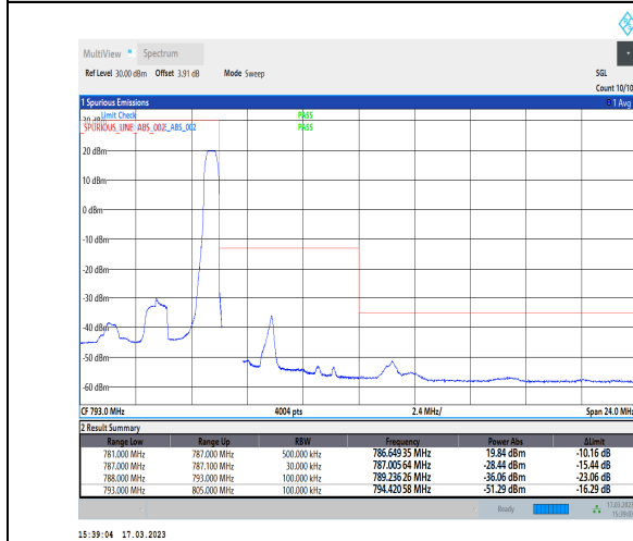
1-N13-PC3-15-5-H-5-CP-QPSK-Edge_1RB_Right-1@24-Ant1-1--PASS-see graph
