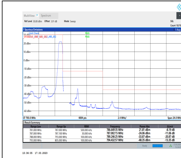
1-N13-PC3-15-5-H-2-DFT-PI2BPSK-Edge_1RB_Right-1@24-Ant1-1--PASS-see graph
