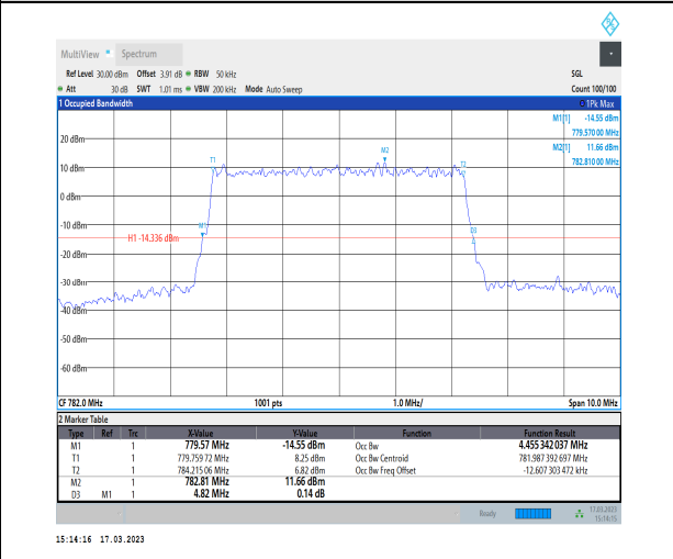
1-N13-PC3-15-5-M-3-DFT-16QAM-Outer_Full-25@0-Ant1-4.455-4.820-≤5-PASS
