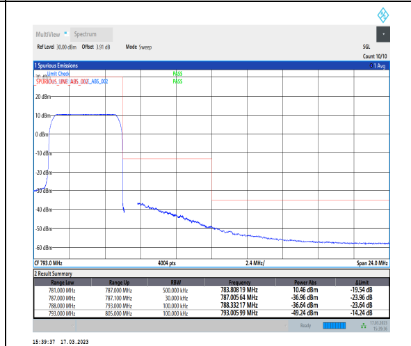
1-N13-PC3-15-5-H-6-CP-QPSK-Outer_Full-25@0-Ant1-1--PASS-see graph
