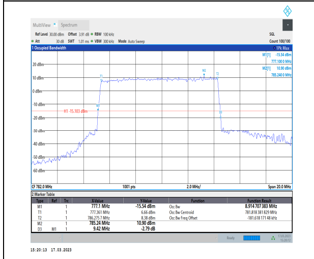
1-N13-PC3-15-10-M-4-DFT-64QAM-Outer_Full-50@ 0-Ant1-8.915-9.420-≤10-PASS
