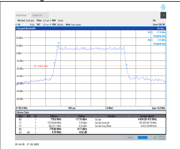
1-N13-PC3-15-5-M-5-DFT-256QAM-Outer_Full-25@0 -Ant1-4.454-4.790-≤5-PASS
