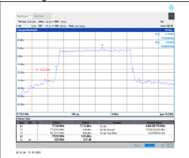
1-N13-PC3-15-5-L-6-CP-QPSK-Outer_Full-25@0-A nt1-4.464-4.830-<math>\leq 5</math>-PASS
