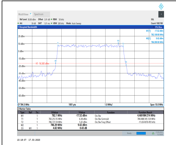
1-N13-PC3-15-5-H-7-CP-16QAM-Outer_Full-25@0-Ant1-4.47-4.820-≤5-PASS
