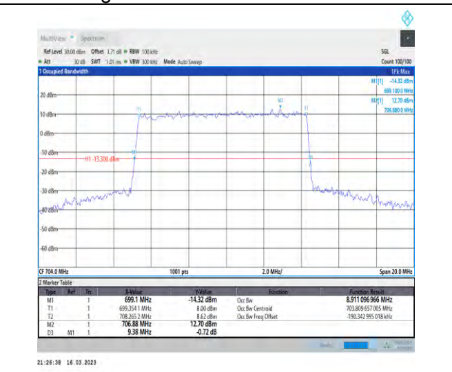
1-N12-PC3-15-10-L-3-DFT-16QAM-Outer_Full-50 @0-Ant1-8.911-9.380-≤10-PASS
