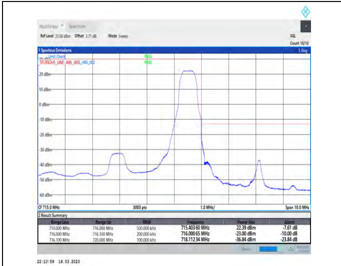
1-N12-PC3-15-15-H-2-DFT-PI2BPSK-Edge_1RB_Right-t-1@78-Ant1-1--PASS-see graph
