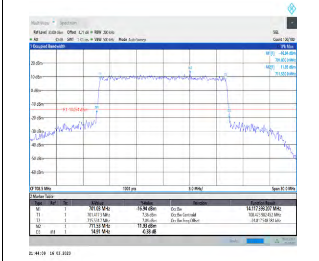
1-N12-PC3-15-15-H-7-CP-16QAM-Outer_Full-79@0 -Ant1-14.117-14.910-≤15-PASS
