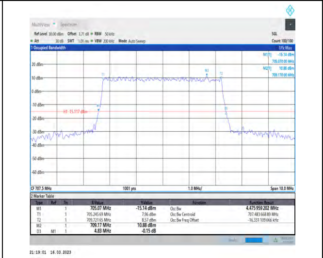
1-N12-PC3-15-5-M-3-DFT-16QAM-Outer_Full-25@0-Ant1-4.476-4.830-≤5-PASS
