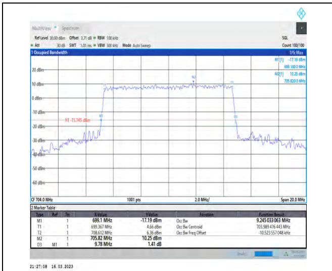
1-N12-PC3-15-10-L-6-CP-QPSK-Outer_Full-52@0-Ant1-9.245-9.780-≤10-PASS
