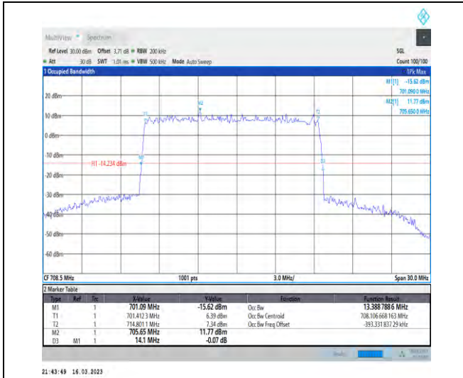
1-N12-PC3-15-15-H-5-DFT-256QAM-Outer_Full-75 @0-Ant1-13.389-14.100-≤15-PASS
