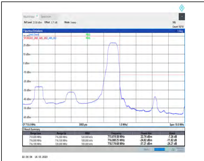
1-N12-PC3-15-10-H-2-DFT-PI2BPSK-Edge_1RB_Right-t-1@51-Ant1-1--PASS-see graph
