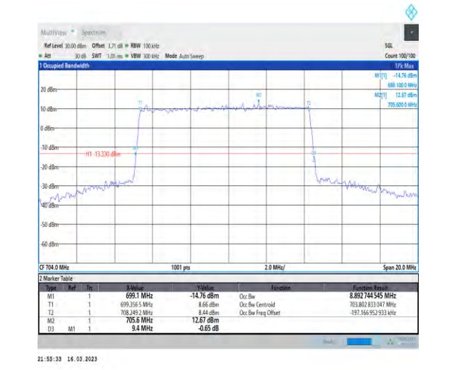
1-N12-PC3-15-10-L-1-DFT-QPSK-Outer_Full-50@0-Ant1-8.893-9.400-≤10-PASS
