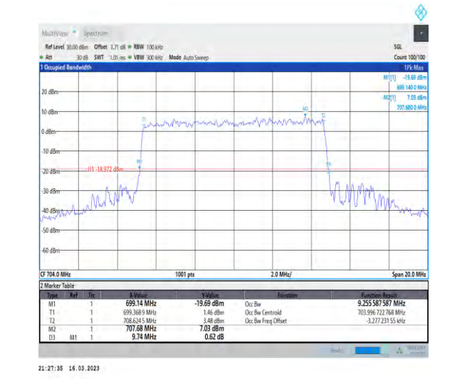
1-N12-PC3-15-10-L-9-CP-256QAM-Outer_Full-52@0-Ant1-9.256-9.740-≤10-PASS
