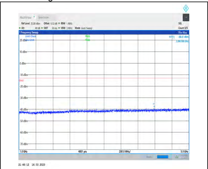
1-N12-PC3-15-15-M-1-DFT-PI2BPSK-Inner_1RB_Lef t-1@1-1000-3000-Ant1-2590.50--38.61--13-PASS
