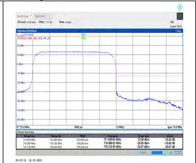
1-N12-PC3-15-5-H-3-DFT-PI2BPSK-Outer_Full-25@0-Ant1-1--PASS-see graph
