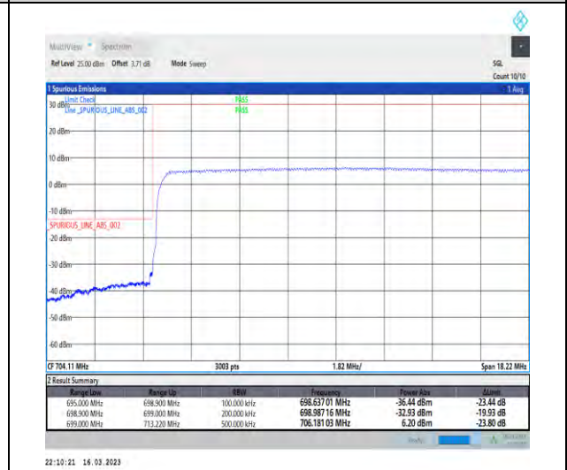
1-N12-PC3-15-15-L-6-CP-QPSK-Outer_Full-79@0-Ant1-1--PASS-see graph
