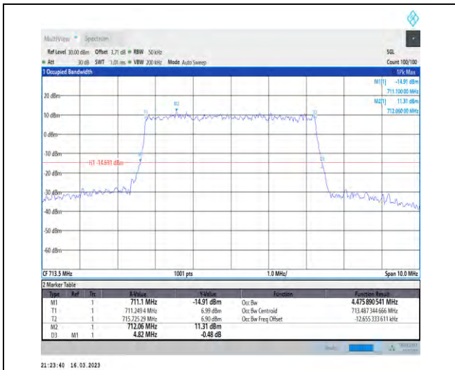
1-N12-PC3-15-5-H-3-DFT-16QAM-Outer_Full-25@0 -Ant1-4.476-4.820-≤5-PASS
