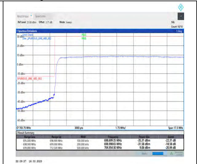
1-N12-PC3-15-15-L-3-DFT-PI2BPSK-Outer_Full-75@0-Ant1-1--PASS-see graph
