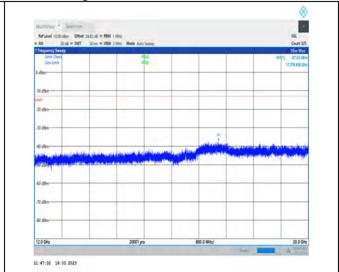
1-N12-PC3-15-15-H-1-DFT-PI2BPSK-Inner_1RB_Lef t-1@1-12000-20000-Ant1-17376.80--37.33--13-PASS
