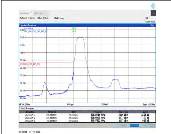
1-N12-PC3-15-15-L-4-CP-QPSK-Edge_1RB_Left-1@0-Ant1-1--PASS-see graph
