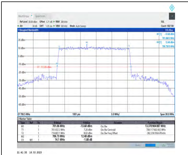
1-N12-PC3-15-15-H-1-DFT-QPSK-Outer_Full-75@0 -Ant1-13.371-14.100-≤15-PASS
