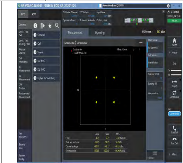
1-N12-PC3-15-15-M-6-CP-QPSK-Outer_Full-79@0- Ant1-see graph-PASS
