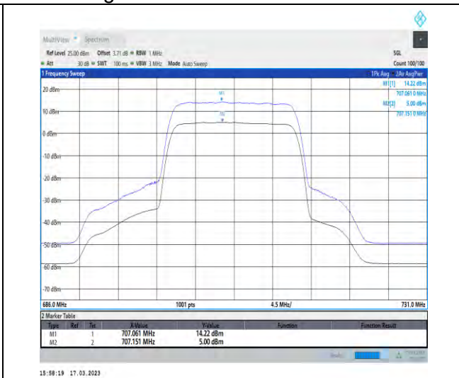
1-N12-PC3-15-15-H-2-CP-256QAM-Outer_Full-79@ 0-Ant1-9.22-100%-0.00-9.22-PASS-≤13
