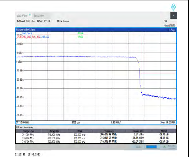
1-N12-PC3-15-15-H-6-CP-QPSK-Outer_Full-79@0-Ant1-1--PASS-see graph
