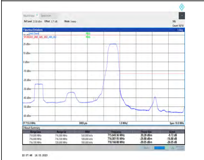
1-N12-PC3-15-10-H-5-CP-QPSK-Edge_1RB_Right-1@51-Ant1-1--PASS-see graph
