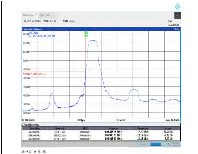
1-N12-PC3-15-15-L-1-DFT-PI2BPSK-Edge_1RB_Left-1@0-Ant1-1--PASS-see graph
