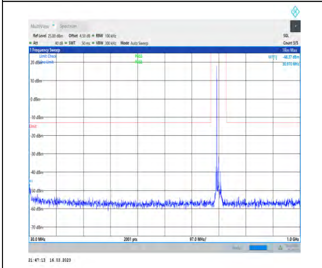
1-N12-PC3-15-15-H-1-DFT-PI2BPSK-Inner_1RB_L eft-1@1-30-1000-Ant1-30.97--48.37--13-PASS
