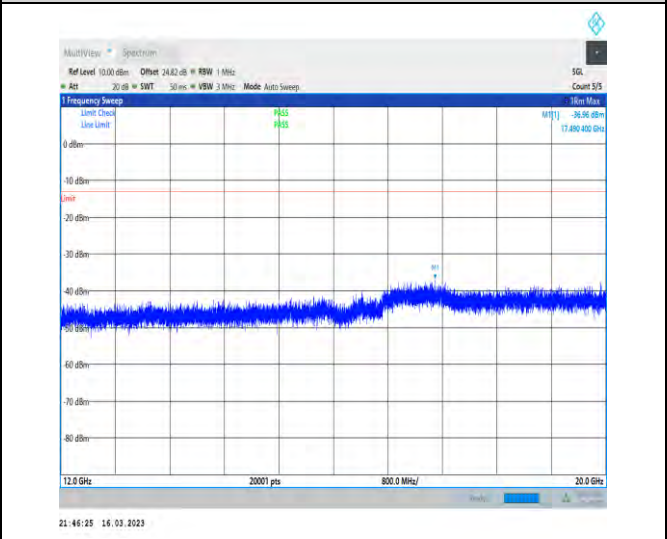
1-N12-PC3-15-15-M-1-DFT-PI2BPSK-Inner_1RB_Lef t-1@1-12000-20000-Ant1-17490.40--36.96--13-PASS
