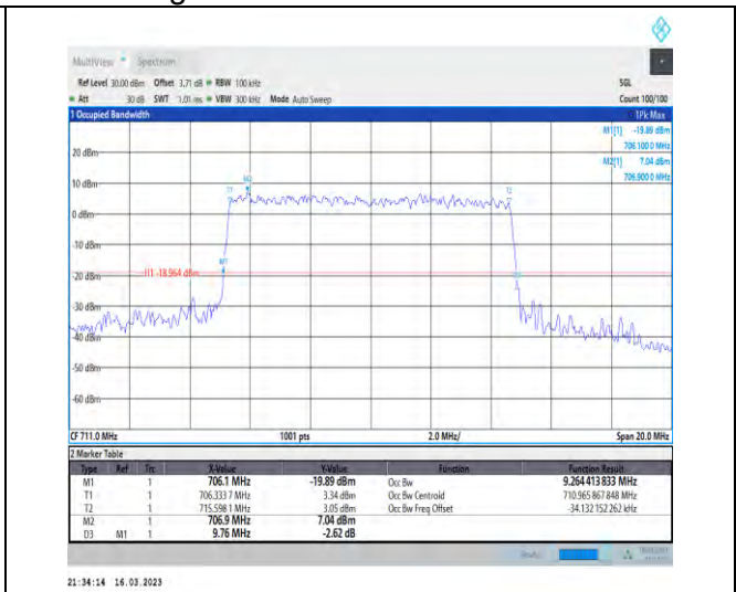
1-N12-PC3-15-10-H-9-CP-256QAM-Outer_Full-52@0 -Ant1-9.264-9.760-≤10-PASS
