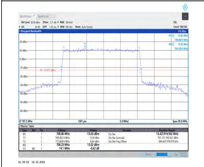
1-N12-PC3-15-15-M-4-DFT-64QAM-Outer_Full-75 @0-Ant1-13.426-14.100-≤15-PASS
