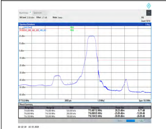
1-N12-PC3-15-15-H-5-CP-QPSK-Edge_1RB_Right-1@78-Ant1-1--PASS-see graph
