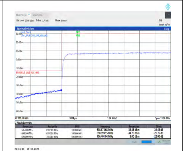
1-N12-PC3-15-10-L-6-CP-QPSK-Outer_Full-52@0-Ant1-1--PASS-see graph
