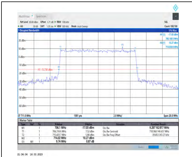
1-N12-PC3-15-10-H-8-CP-64QAM-Outer_Full-52@0 -Ant1-9.287-9.740-≤10-PASS
