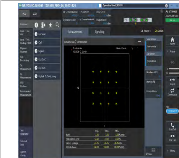
1-N12-PC3-15-15-M-7-CP-16QAM-Outer_Full-79@0- Ant1-see graph-PASS
