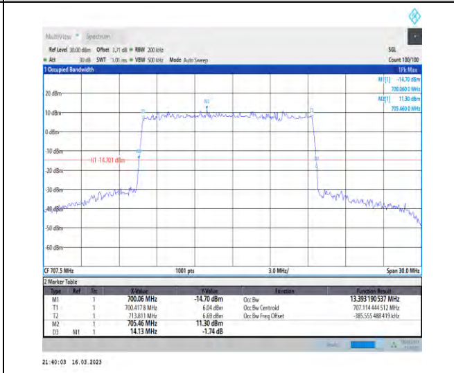
1-N12-PC3-15-15-M-5-DFT-256QAM-Outer_Full-75 @0-Ant1-13.393-14.130-≤15-PASS
