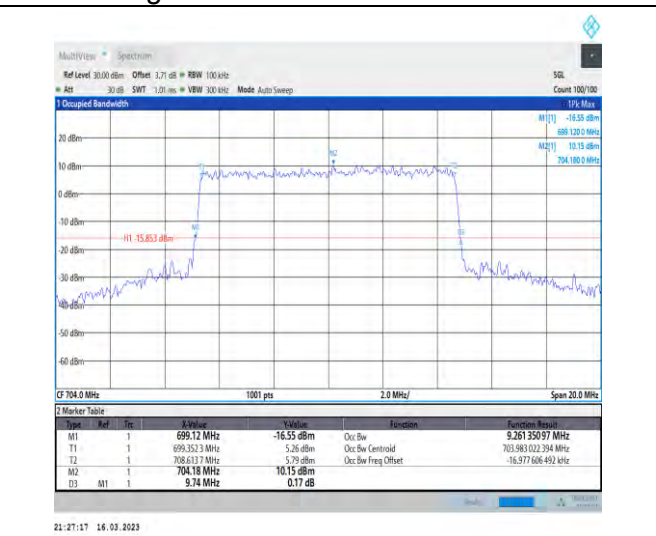
1-N12-PC3-15-10-L-7-CP-16QAM-Outer_Full-52@0-Ant1-9.261-9.740-≤10-PASS
