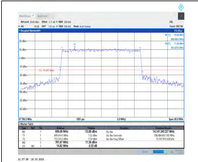
1-N12-PC3-15-15-L-7-CP-16QAM-Outer_Full-79@0-Ant1-14.141-14.820-≤15-PASS
