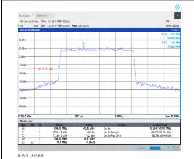
1-N12-PC3-15-15-L-5-DFT-256QAM-Outer_Full-75@0-Ant1-13.364-14.100-≤15-PASS
