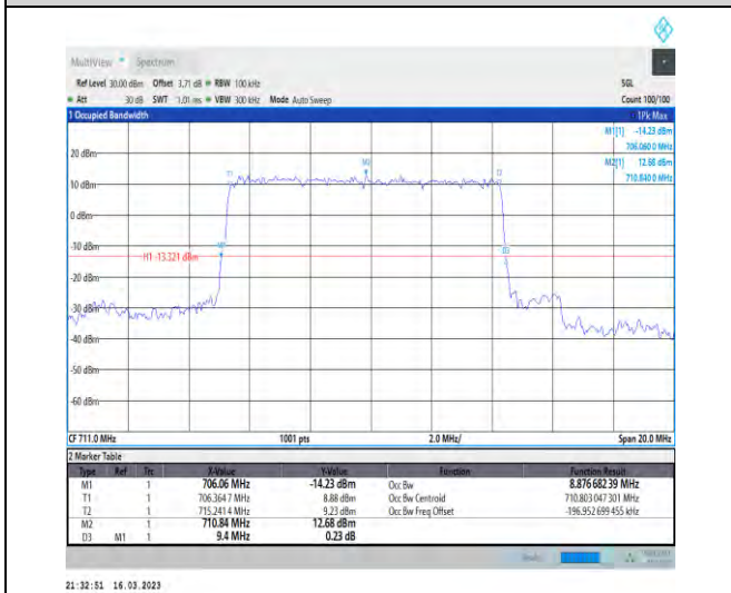
1-N12-PC3-15-10-H-2-DFT-PI2BPSK-Outer_Full-50 @0-Ant1-8.877-9.400-≤10-PASS
