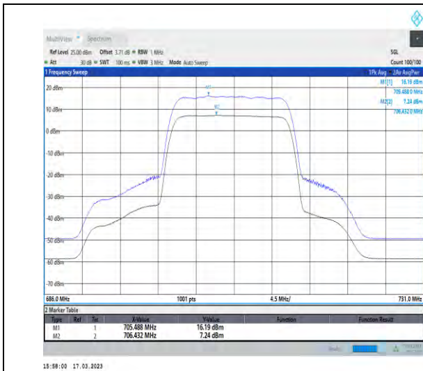
1-N12-PC3-15-15-H-1-DFT-256QAM-Outer_Full-75 @0-Ant1-8.95-100%-0.00-8.95-PASS-≤13
