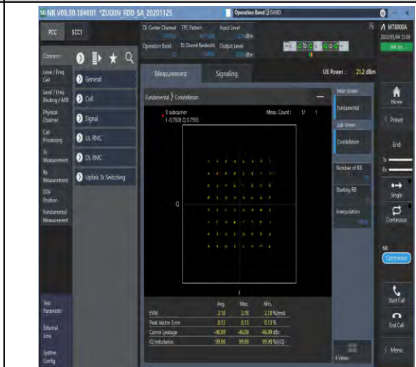
1-N12-PC3-15-15-M-8-CP-64QAM-Outer_Full-79@ 0-Ant1-see graph-PASS
