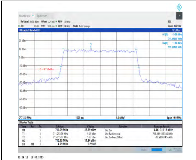
1-N12-PC3-15-5-H-7-CP-16QAM-Outer_Full-25@0-Ant1-4.461-4.790-≤5-PASS
