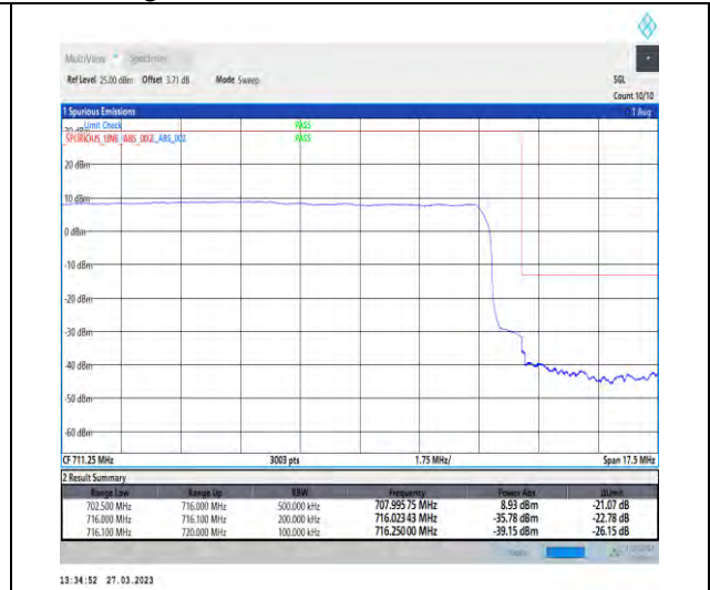
1-N12-PC3-15-15-H-3-DFT-PI2BPSK-Outer_Full-75@0-Ant1-1--PASS-see graph
