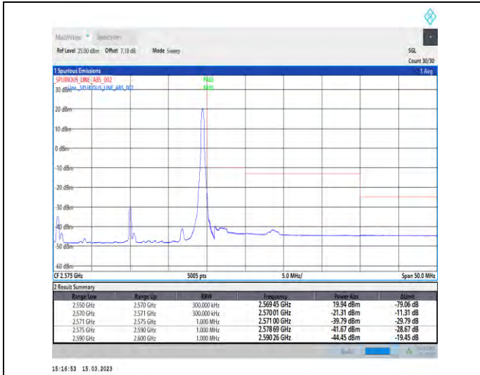
1-N7-PC3-15-20-H-2-DFT-PI2BPSK-Edge_1RB_Right-1@105-Ant1-1--PASS-see graph
