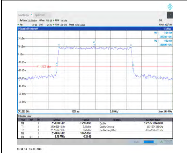
1-N7-PC3-15-10-M-7-CP-16QAM-Outer_Full-52@0-Ant1-9.296-9.780-≤10-PASS
