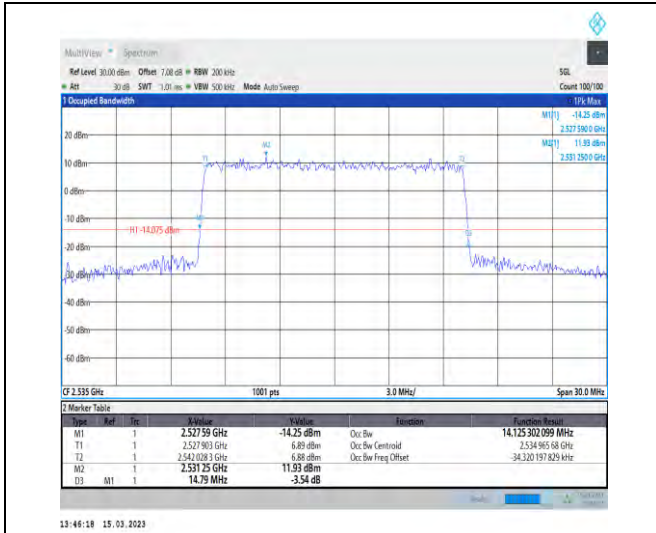
1-N7-PC3-15-15-M-6-CP-QPSK-Outer_Full-79@0-A Ant1-14.125-14.790-≤15-PASS
