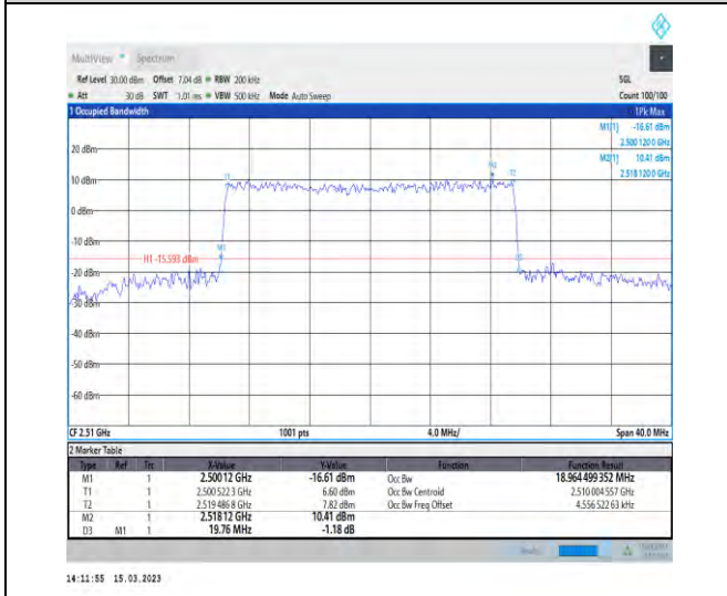
1-N7-PC3-15-20-L-6-CP-QPSK-Outer_Full-106@0- Ant1-18.964-19.760-≤20-PASS
