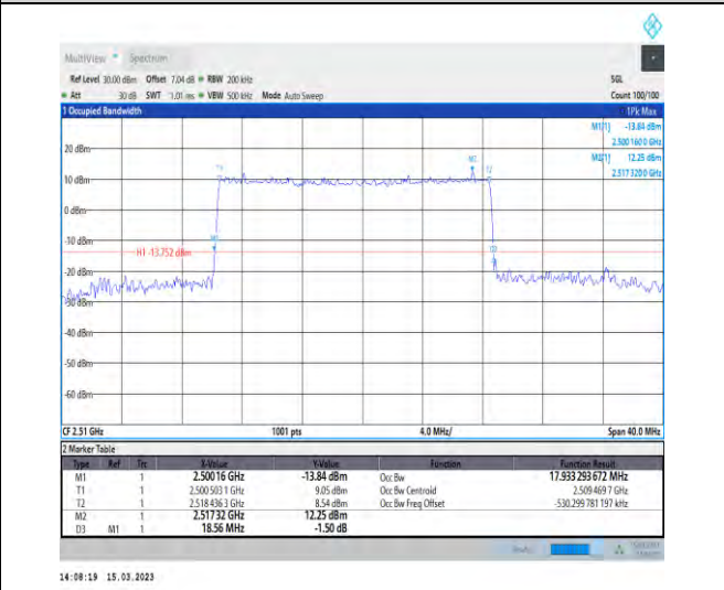
1-N7-PC3-15-20-L-3-DFT-16QAM-Outer_Full-100@ 0-Ant1-17.933-18.560-≤20-PASS
