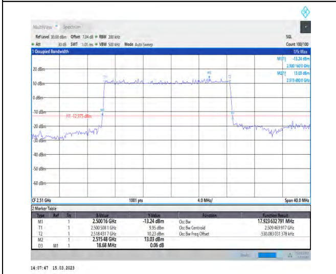
1-N7-PC3-15-20-L-2-DFT-PI2BPSK-Outer_Full-100 @0-Ant1-17.924-18.680-≤20-PASS
