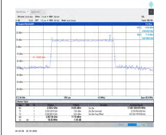
1-N7-PC3-15-20-H-4-DFT-64QAM-Outer_Full-100 @0-Ant1-17.852-18.560-≤20-PASS
