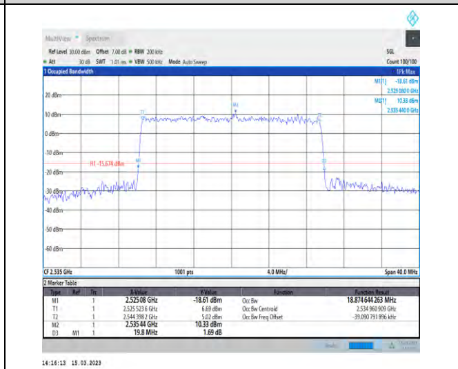
1-N7-PC3-15-20-M-6-CP-QPSK-Outer_Full-106@0- Ant1-18.875-19.800-≤20-PASS
