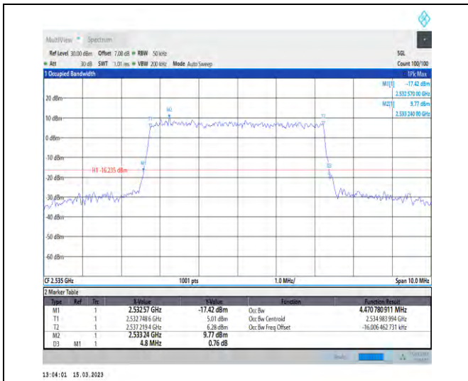
1-N7-PC3-15-5-M-8-CP-64QAM-Outer_Full-25@0-A nt1-4.471-4.800-≤5-PASS
