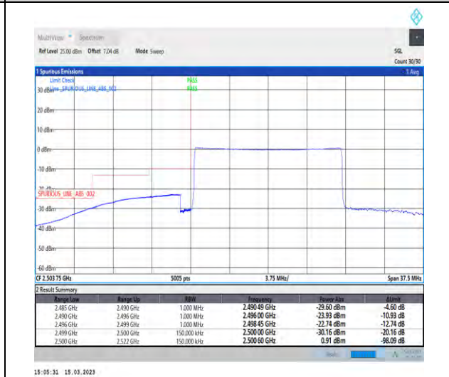
1-N7-PC3-15-15-L-6-CP-QPSK-Outer_Full-79@0-Ant1-1--PASS-see graph
