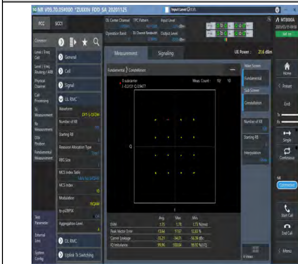
1-N7-PC3-15-20-M-3-DFT-16QAM-Outer_Full-100@ 0-Ant1-see graph-PASS
