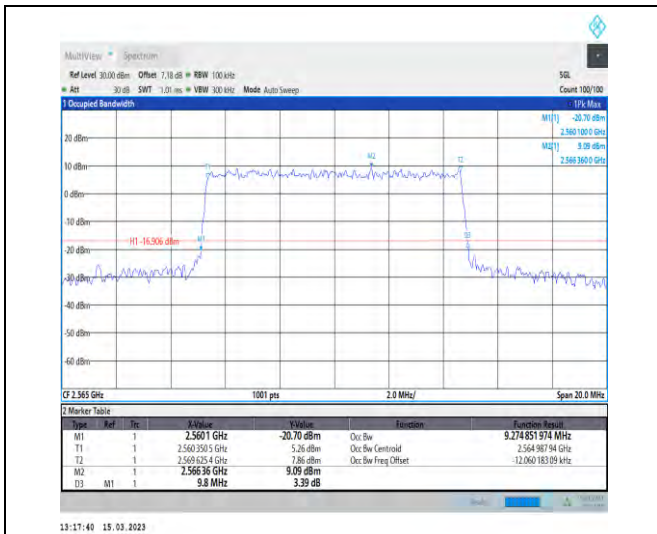
1-N7-PC3-15-10-H-8-CP-64QAM-Outer_Full-52@0-Ant1-9.275-9.800-≤10-PASS
