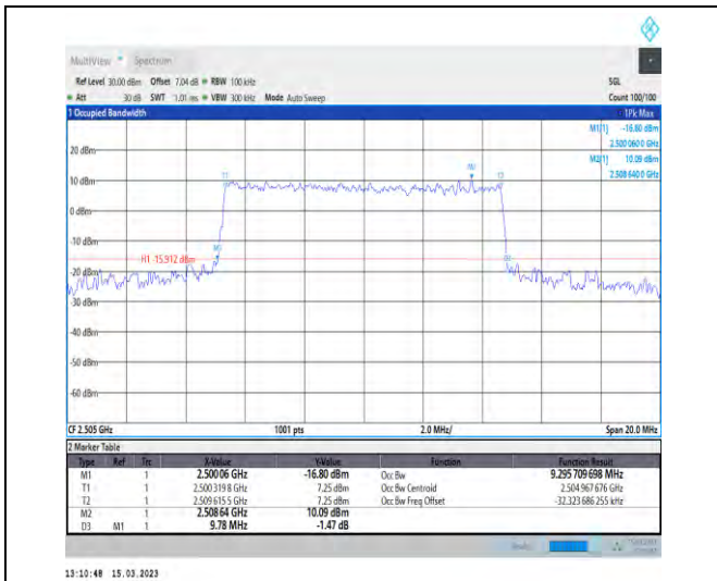
1-N7-PC3-15-10-L-6-CP-QPSK-Outer_Full-52@0-A nt1-9.296-9.780-≤10-PASS
