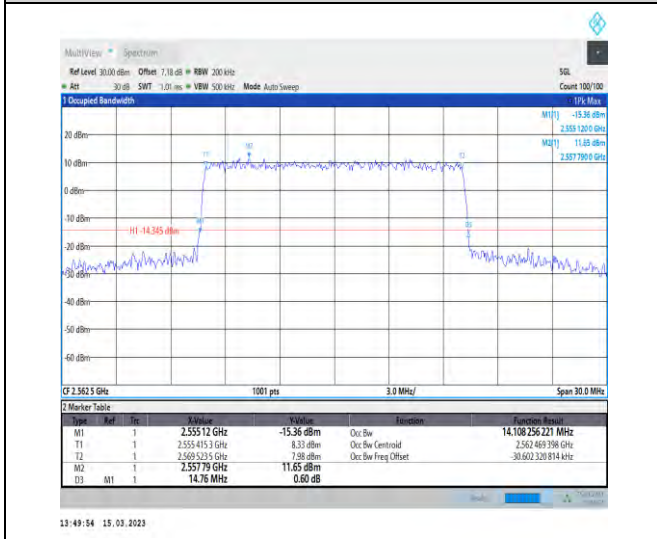
1-N7-PC3-15-15-H-7-CP-16QAM-Outer_Full-79@0- Ant1-14.108-14.760≤15-PASS
