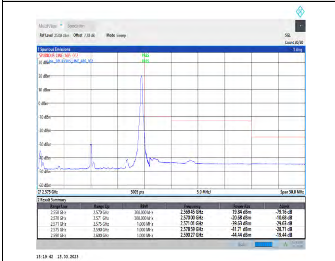
1-N7-PC3-15-20-H-5-CP-QPSK-Edge_1RB_Right-1@105-Ant1-1--PASS-see graph
