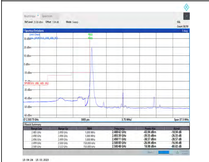
1-N7-PC3-15-15-L-4-CP-QPSK-Edge_1RB_Left-1@0-Ant1-1--PASS-see graph
