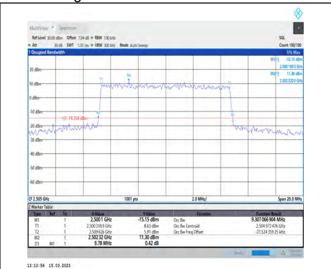
1-N7-PC3-15-10-L-7-CP-16QAM-Outer_Full-52@0-A nt1-9.307-9.780-≤10-PASS
