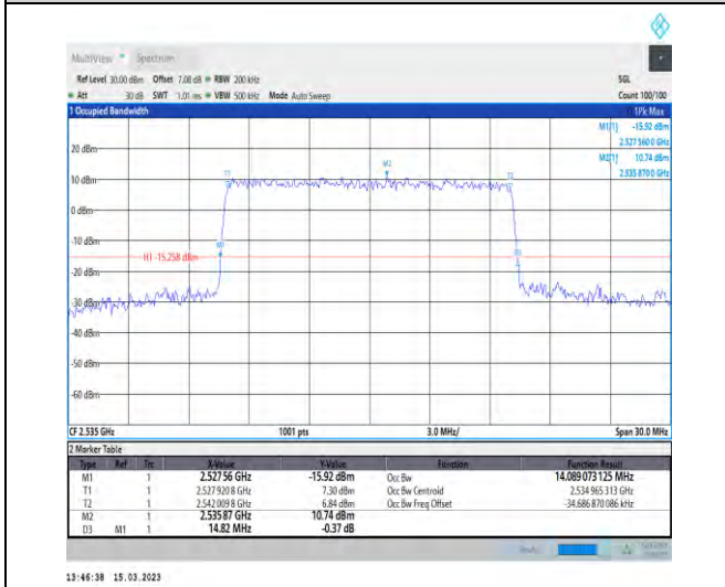
1-N7-PC3-15-15-M-8-CP-64QAM-Outer_Full-79@0- Ant1-14.089-14.820-≤15-PASS
