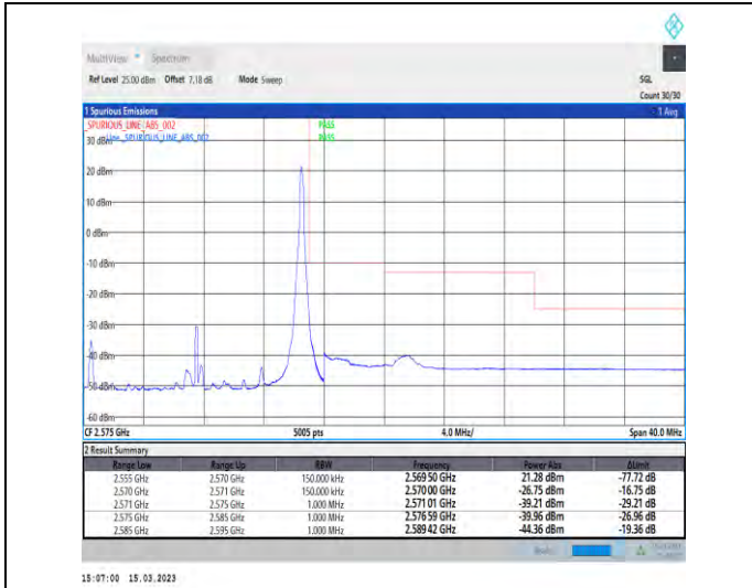
1-N7-PC3-15-15-H-2-DFT-PI2BPSK-Edge_1RB_Right-1@78-Ant1-1--PASS-see graph
