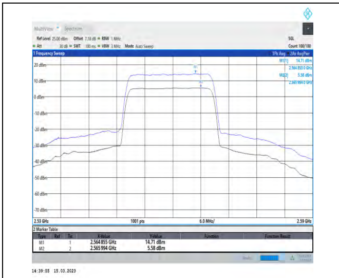
1-N7-PC3-15-20-H-1-DFT-256QAM-Outer_Full-100 @0-Ant1-9.13-100%-0.00-9.13-PASS-≤13
