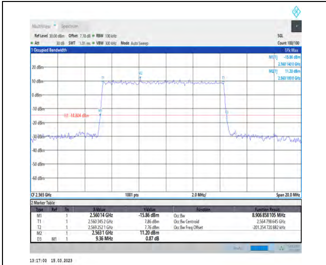
1-N7-PC3-15-10-H-4-DFT-64QAM-Outer_Full-50@0-Ant1-8.907-9.360-≤10-PASS
