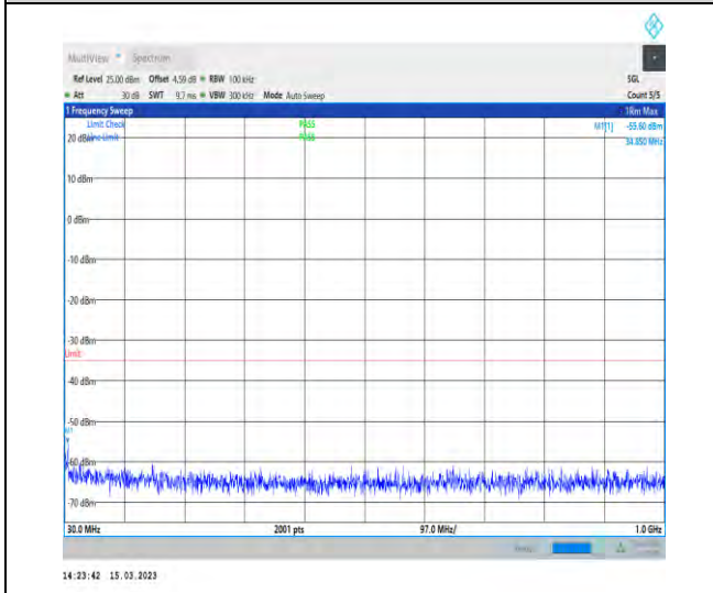
1-N7-PC3-15-20-H-1-DFT-PI2BPSK-Inner_1RB_Lef t-1@1-30-1000-Ant1-34.85--55.60--35-PASS
