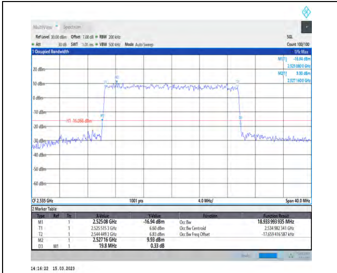
1-N7-PC3-15-20-M-7-CP-16QAM-Outer_Full-106@0 -Ant1-18.934-19.800-≤20-PASS
