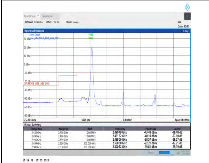
1-N7-PC3-15-20-L-4-CP-QPSK-Edge_1RB_Left-1@0-Ant1-1--PASS-see graph
