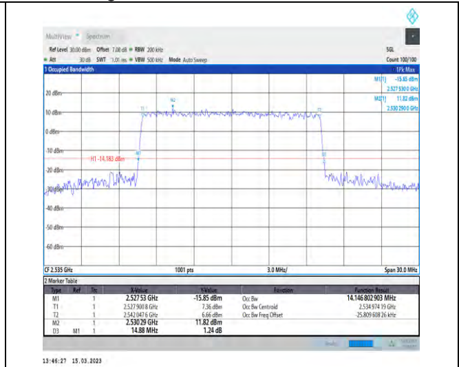
1-N7-PC3-15-15-M-7-CP-16QAM-Outer_Full-79@0- Ant1-14.147-14.880-≤15-PASS
