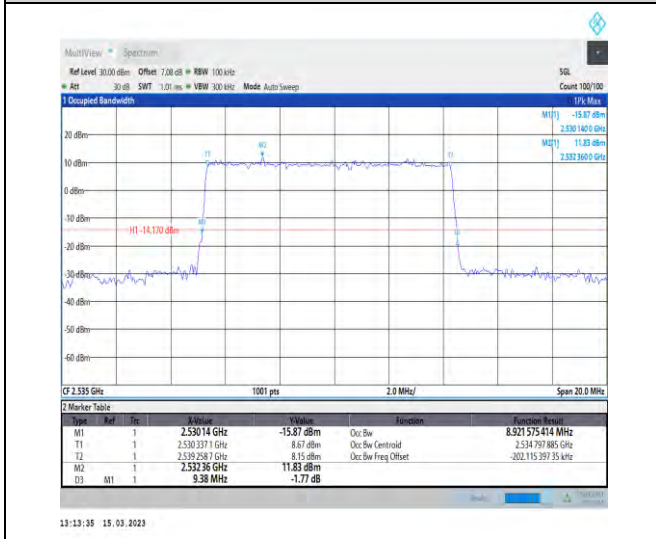
1-N7-PC3-15-10-M-3-DFT-16QAM-Outer_Full-50@0-Ant1-8.922-9.380-≤10-PASS
