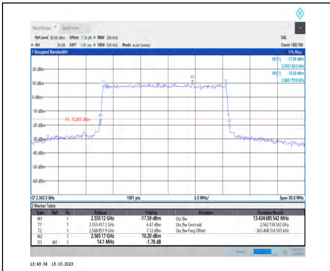
1-N7-PC3-15-15-H-5-DFT-256QAM-Outer_Full-75@ 0-Ant1-13.435-14.100≤15-PASS
