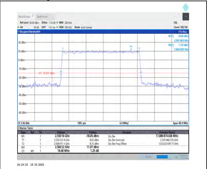
1-N7-PC3-15-20-H-3-DFT-16QAM-Outer_Full-100 @0-Ant1-17.89-18.680-≤20-PASS
