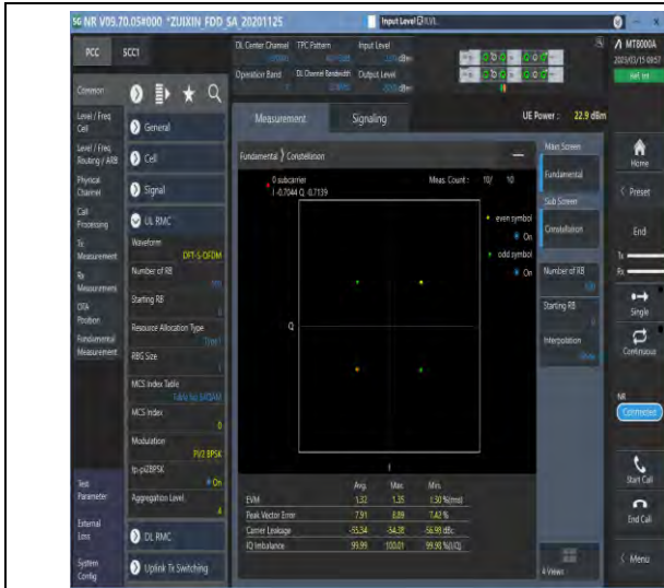
1-N7-PC3-15-20-M-1-DFT-PI2BPSK-Outer_Full-100 @0-Ant1-see graph-PASS
