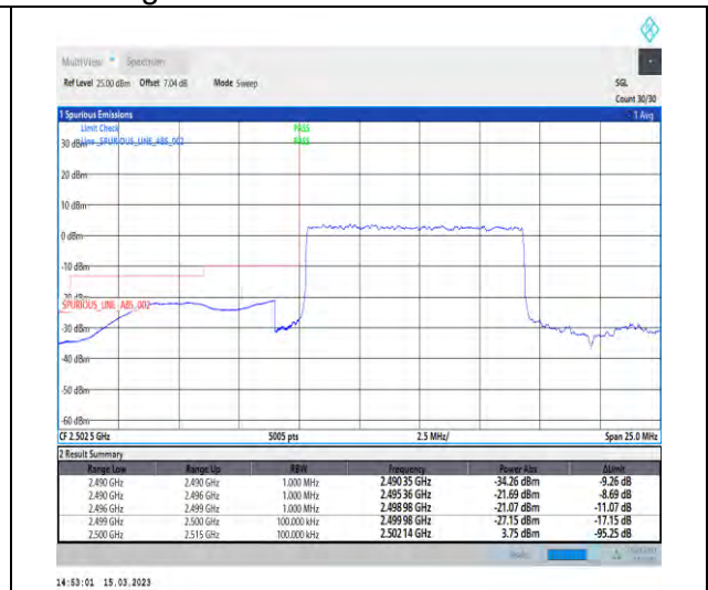
1-N7-PC3-15-10-L-3-DFT-PI2BPSK-Outer_Full-50 @0-Ant1-1--PASS-see graph
