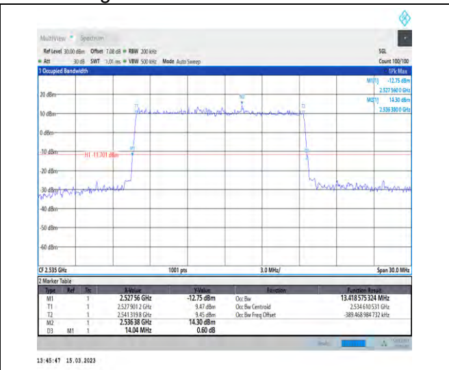
1-N7-PC3-15-15-M-3-DFT-16QAM-Outer_Full-75@0-Ant1-13.419-14.040-≤15-PASS
