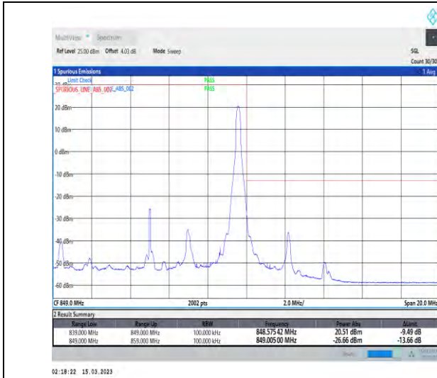
1-N5-PC3-15-10-H-2-DFT-PI2BPSK-Edge_1RB_Right-1@51-Ant1-1-seegraph-PASS-see graph
