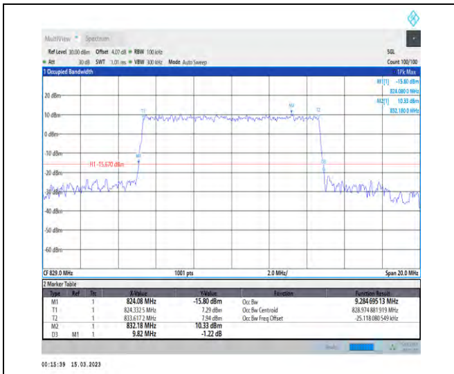
1-N5-PC3-15-10-L-6-CP-QPSK-Outer_Full-52@0-A nt1-9.285-9.820-≤10-PASS
