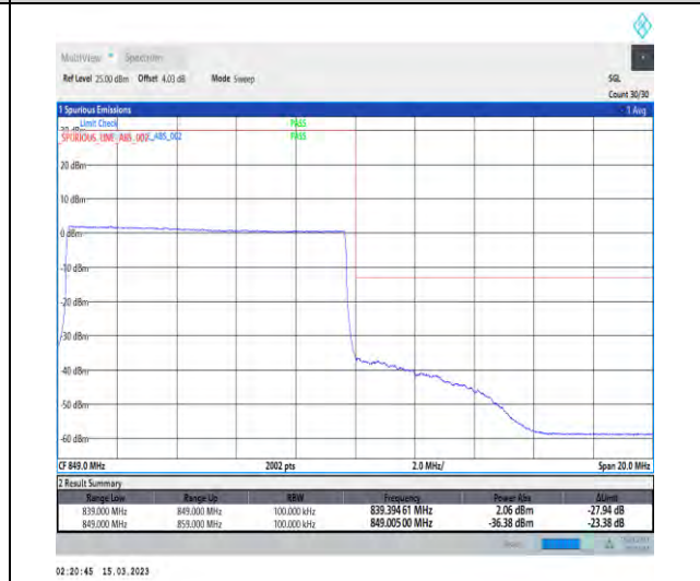
1-N5-PC3-15-10-H-6-CP-QPSK-Outer_Full-52@0-Ant1-1-seegraph-PASS-see graph
