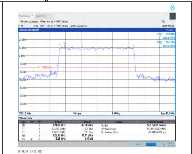
1-N5-PC3-15-15-L-8-CP-64QAM-Outer_Full-79@0-Ant1-14.175-14.880-≤15-PASS
