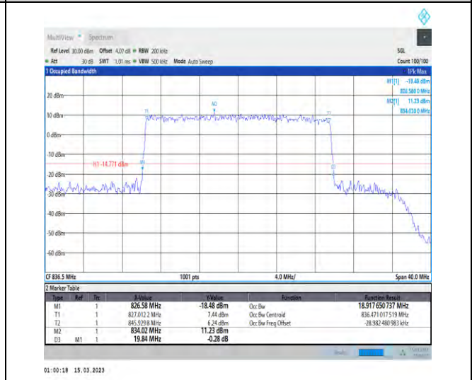
1-N5-PC3-15-20-M-6-CP-QPSK-Outer_Full-106@0- Ant1-18.918-19.840-≤20-PASS
