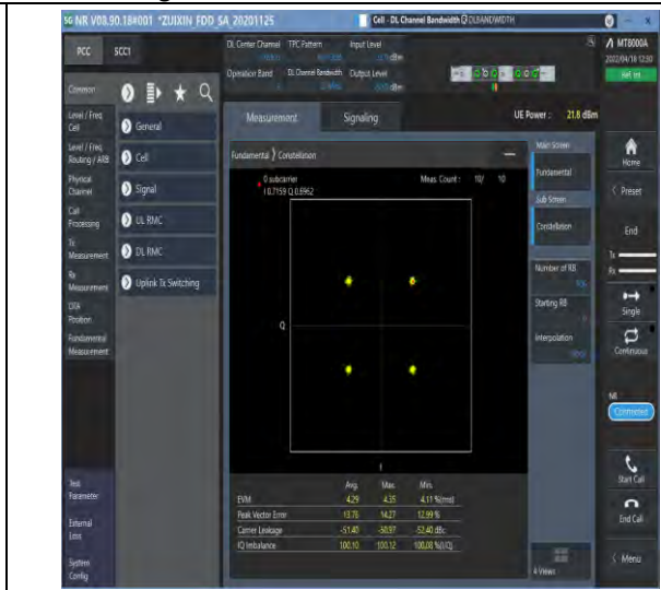
1-N5-PC3-15-20-M-6-CP-QPSK-Outer_Full-106@0-Ant1-see graph-PASS
