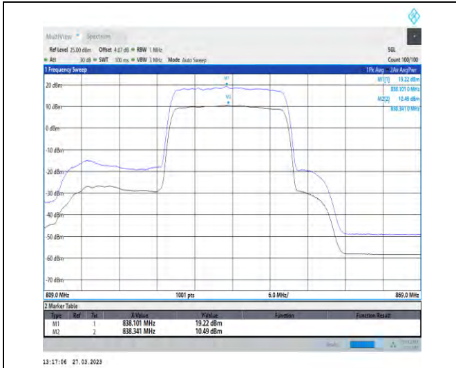
1-N5-PC3-15-20-H-1-DFT-256QAM-Outer_Full-100 @0-Ant1-8.73-100%-0.00-8.73-PASS≤13
