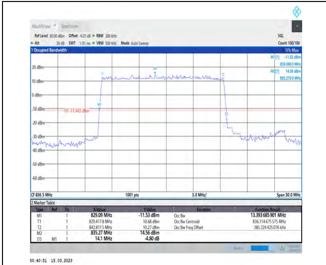
1-N5-PC3-15-15-M-2-DFT-PI2BPSK-Outer_Full-75 @0-Ant1-13.394-14.100-≤15-PASS
