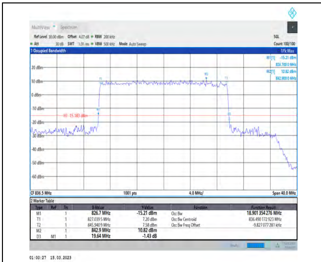
1-N5-PC3-15-20-M-7-CP-16QAM-Outer_Full-106@0 -Ant1-18.901-19.640-≤20-PASS
