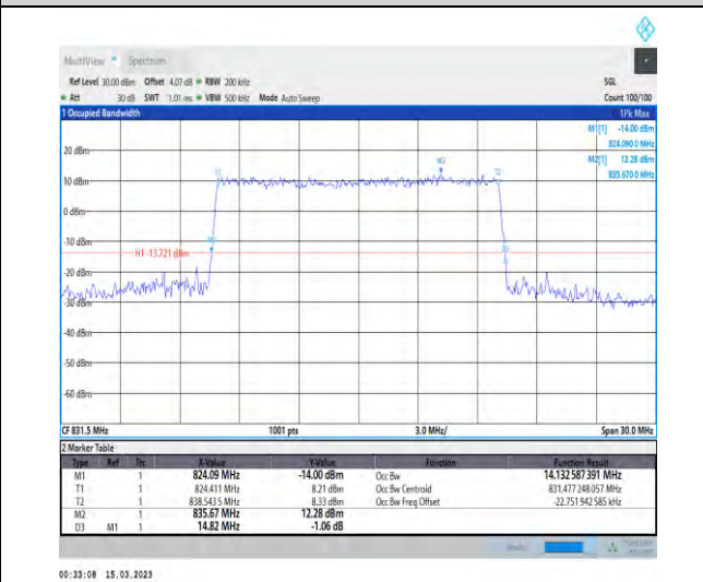
1-N5-PC3-15-15-L-6-CP-QPSK-Outer_Full-79@0-Ant1-14.133-14.820-≤15-PASS
