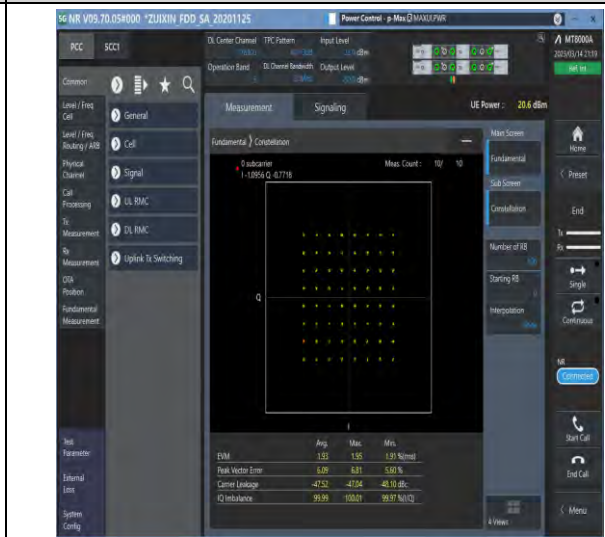
1-N5-PC3-15-20-M-8-CP-64QAM-Outer_Full-106@0-Ant1-see graph-PASS
