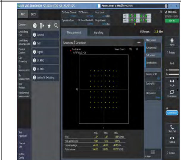
1-N5-PC3-15-20-M-4-DFT-64QAM-Outer_Full-100 @0-Ant1-see graph-PASS
