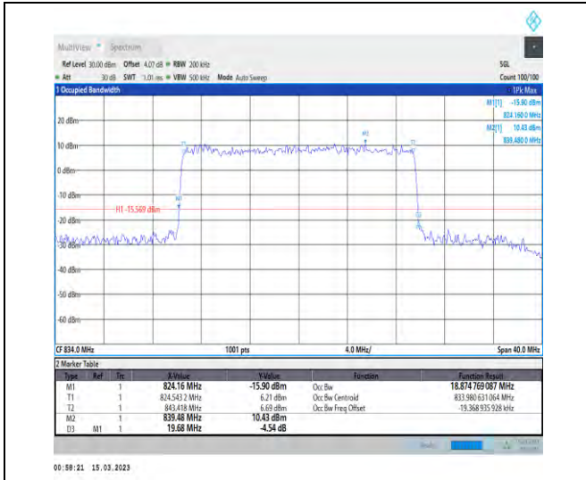
1-N5-PC3-15-20-L-8-CP-64QAM-Outer_Full-106@0-Ant1-18.875-19.680-≤20-PASS
