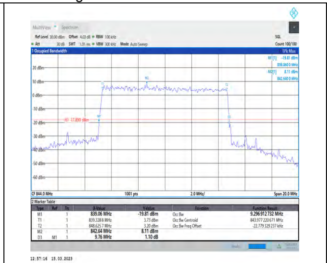
1-N5-PC3-15-10-H-9-CP-256QAM-Outer_Full-52@0-Ant1-9.297-9.760-≤10-PASS
