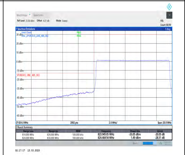
1-N5-PC3-15-10-L-6-CP-QPSK-Outer_Full-52@0-Ant1-1-seegraph-PASS-see graph
