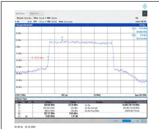
1-N5-PC3-15-15-H-9-CP-256QAM-Outer_Full-79@0 -Ant1-14.094-14.820-≤15-PASS
