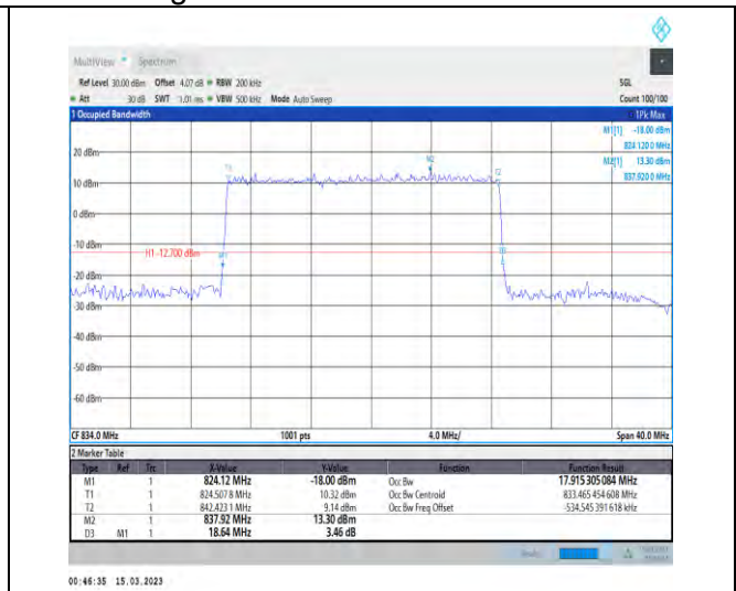
1-N5-PC3-15-20-L-1-DFT-QPSK-Outer_Full-100@0- Ant1-17.915-18.640-≤20-PASS
