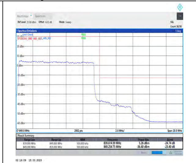
1-N5-PC3-15-10-H-3-DFT-PI2BPSK-Outer_Full-50@0-Ant1-1-seegraph-PASS-see graph
