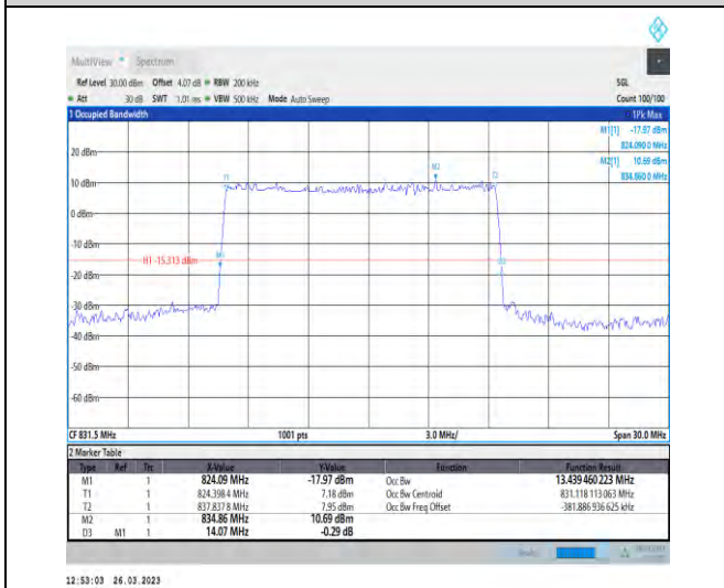
1-N5-PC3-15-15-L-5-DFT-256QAM-Outer_Full-75@0-Ant1-13.439-14.070-≤15-PASS
