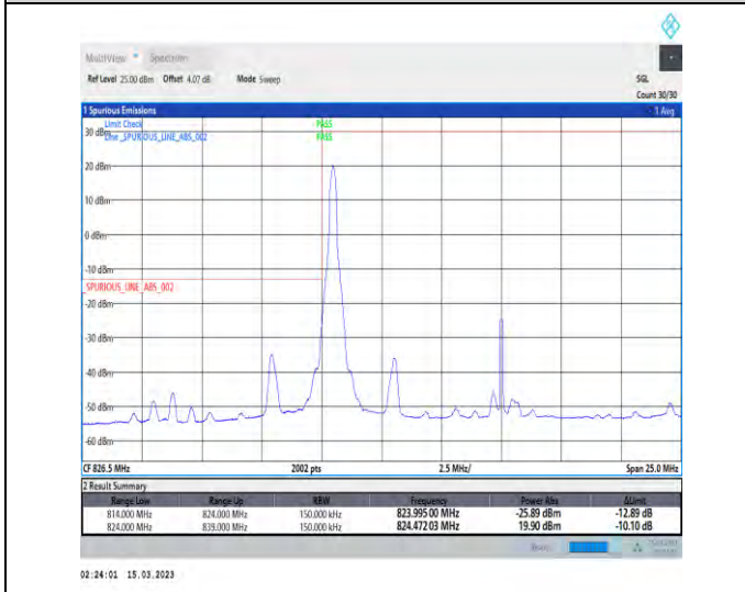
1-N5-PC3-15-15-L-4-CP-QPSK-Edge_1RB_Left-1@0-Ant1-1-seegraph-PASS-see graph
