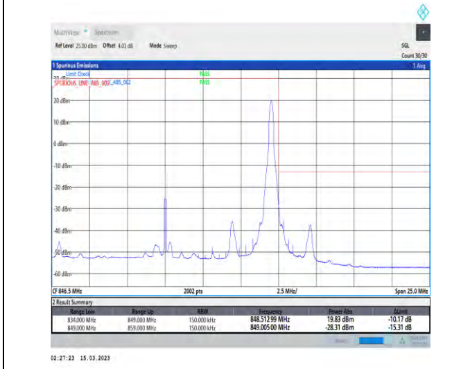
1-N5-PC3-15-15-H-5-CP-QPSK-Edge_1RB_Right-1@78-Ant1-1-seegraph-PASS-see graph
