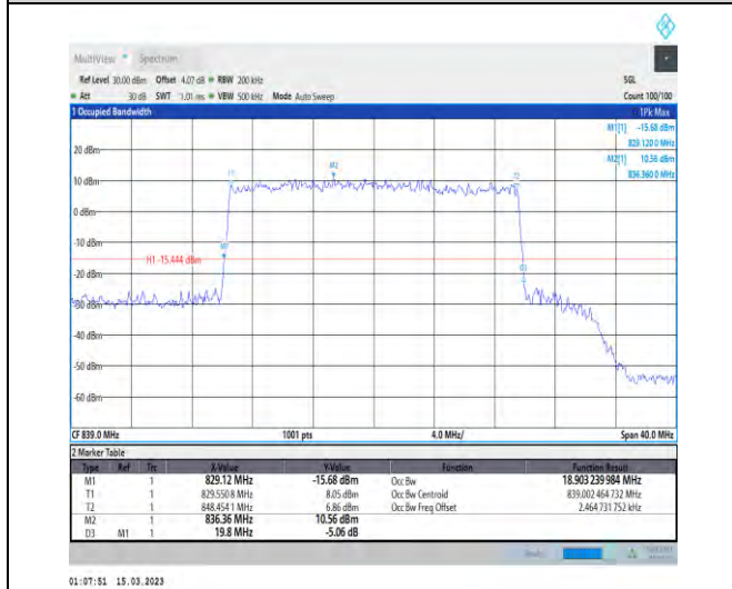
1-N5-PC3-15-20-H-8-CP-64QAM-Outer_Full-106@0-Ant1-18.903-19.800-≤20-PASS
