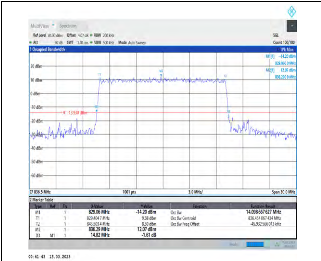
1-N5-PC3-15-15-M-6-CP-QPSK-Outer_Full-79@0-A Ant1-14.099-14.820-≤15-PASS
