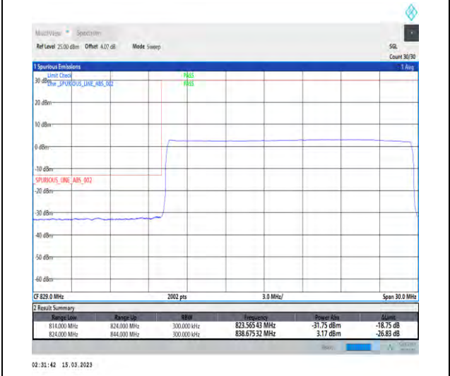
1-N5-PC3-15-20-L-6-CP-QPSK-Outer_Full-106@0-Ant1-1-seegraph-PASS-see graph
