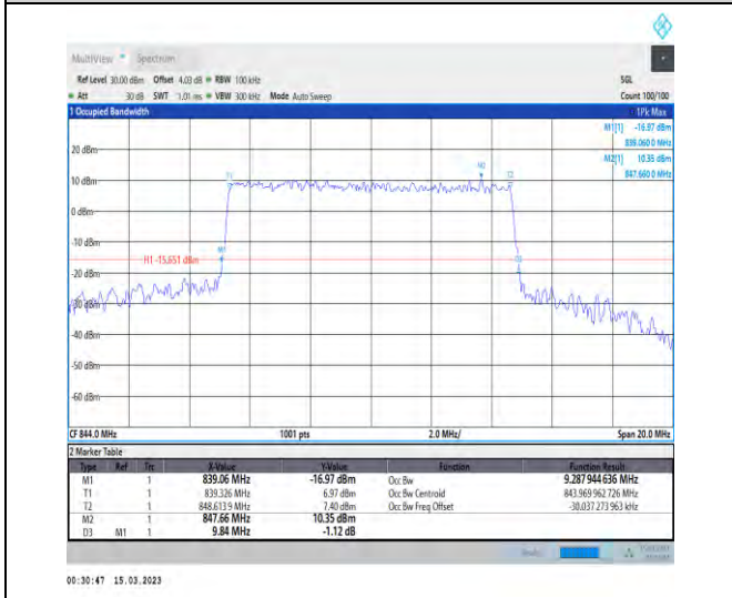
1-N5-PC3-15-10-H-6-CP-QPSK-Outer_Full-52@0-Ant1-9.288-9.840-≤10-PASS
