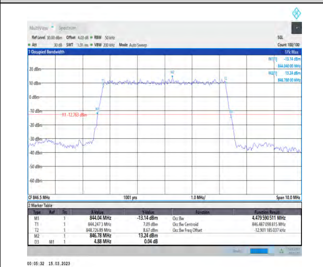
1-N5-PC3-15-5-H-2-DFT-PI2BPSK-Outer_Full-25@0- -Ant1-4.48-4.880-≤5-PASS
