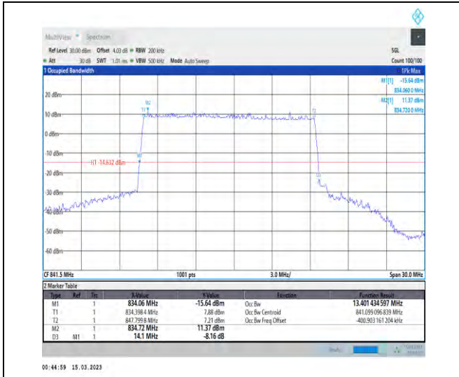
1-N5-PC3-15-15-H-5-DFT-256QAM-Outer_Full-75@0-Ant1-13.401-14.100-≤15-PASS
