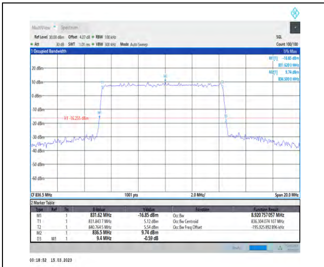
1-N5-PC3-15-10-M-5-DFT-256QAM-Outer_Full-50@0-Ant1-8.921-9.400-≤10-PASS
