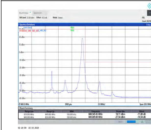
1-N5-PC3-15-10-H-5-CP-QPSK-Edge_1RB_Right-1@51-Ant1-1-seegraph-PASS-see graph
