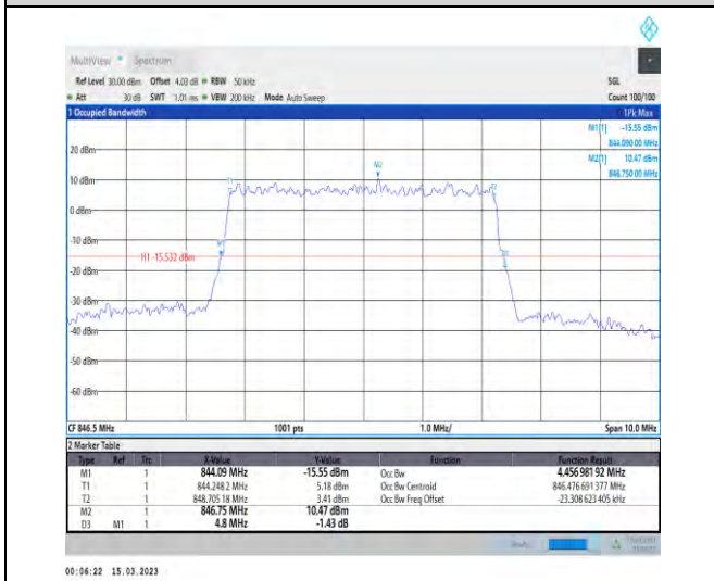
1-N5-PC3-15-5-H-5-DFT-256QAM-Outer_Full-25@0-Ant1-4.457-4.800-≤5-PASS
