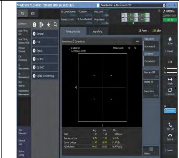
1-N5-PC3-15-20-M-2-DFT-QPSK-Outer_Full-100@ 0-Ant1-see graph-PASS
