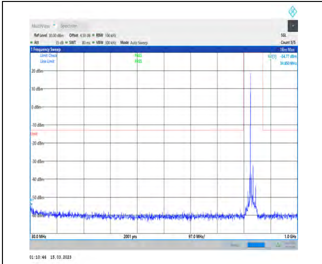
1-N5-PC3-15-20-H-1-DFT-PI2BPSK-Inner_1RB_Left -1@1-30-1000-Ant1-34.85--54.77--13-PASS
