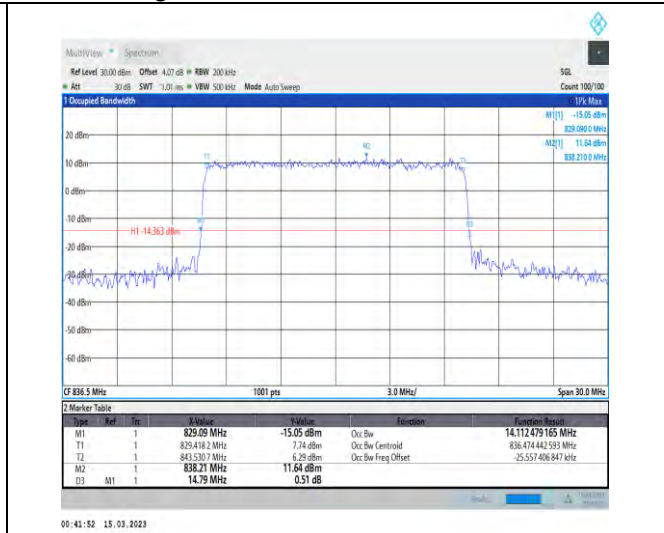
1-N5-PC3-15-15-M-7-CP-16QAM-Outer_Full-79@0- Ant1-14.112-14.790-≤15-PASS
