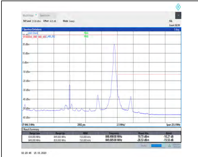
1-N5-PC3-15-15-H-2-DFT-PI2BPSK-Edge_1RB_Right-1@78-Ant1-1-seegraph-PASS-see graph
