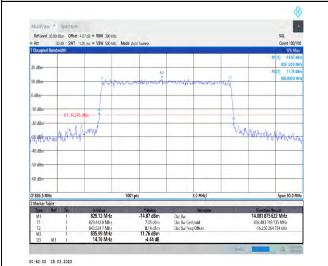
1-N5-PC3-15-15-M-8-CP-64QAM-Outer_Full-79@0- Ant1-14.082-14.760-≤15-PASS
