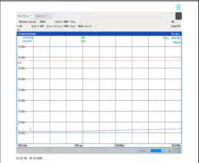
1-N5-PC3-15-20-H-1-DFT-PI2BPSK-Inner_1RB_Left -1@1-0.15-30-Ant1-0.15--84.87--23-PASS
