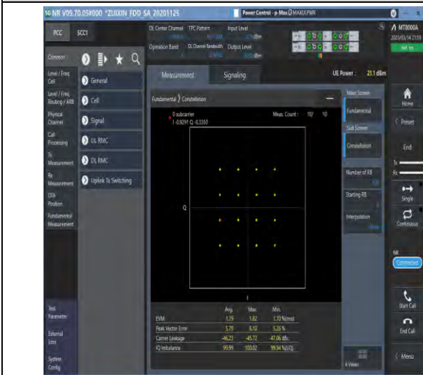
1-N5-PC3-15-20-M-7-CP-16QAM-Outer_Full-106@0-Ant1-see graph-PASS
