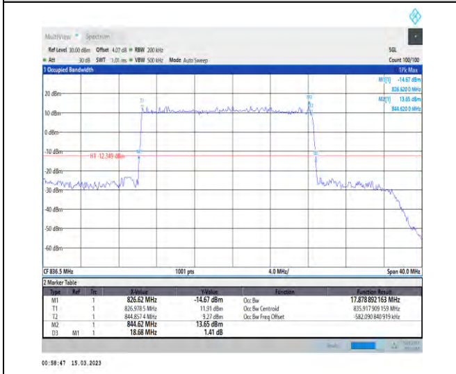
1-N5-PC3-15-20-M-1-DFT-QPSK-Outer_Full-100@0-Ant1-17.879-18.680-≤20-PASS
