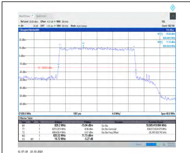
1-N5-PC3-15-20-H-6-CP-QPSK-Outer_Full-106@0-Ant1-18.905-19.720-≤20-PASS
