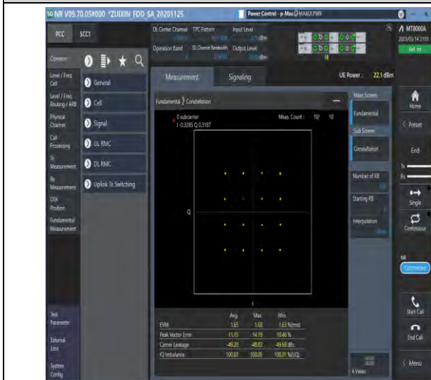
1-N5-PC3-15-20-M-3-DFT-16QAM-Outer_Full-100@ 0-Ant1-see graph-PASS
