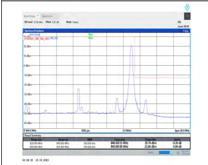
1-N5-PC3-15-20-H-5-CP-QPSK-Edge_1RB_Right-1@105-Ant1-1-seegraph-PASS-see graph
