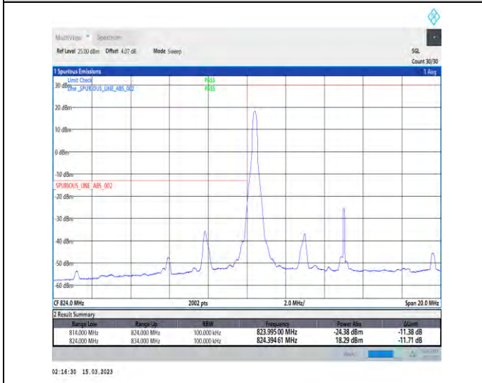
1-N5-PC3-15-10-L-4-CP-QPSK-Edge_1RB_Left-1@0-Ant1-1-seegraph-PASS-see graph
