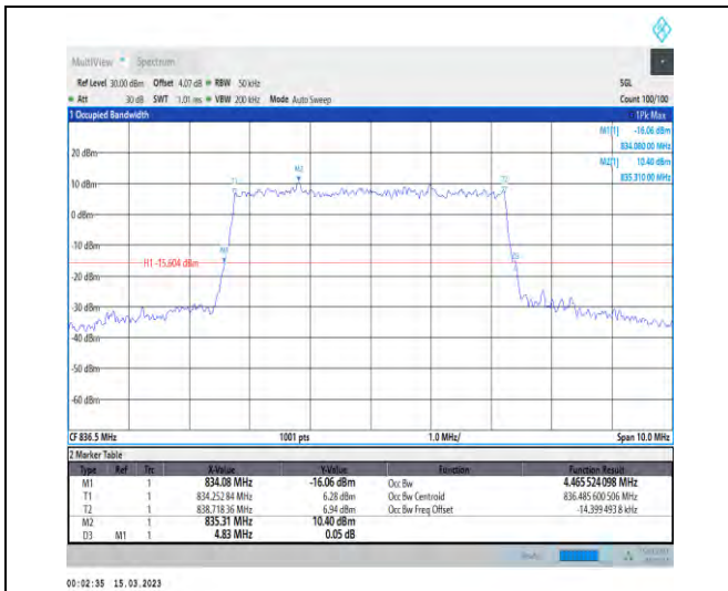
1-N5-PC3-15-5-M-8-CP-64QAM-Outer_Full-25@0-A nt1-4.466-4.830-≤5-PASS
