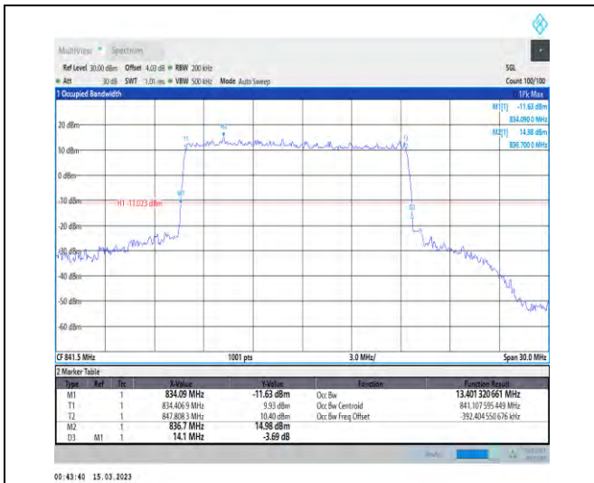
1-N5-PC3-15-15-H-1-DFT-QPSK-Outer_Full-75@0-Ant1-13.401-14.100-≤15-PASS
