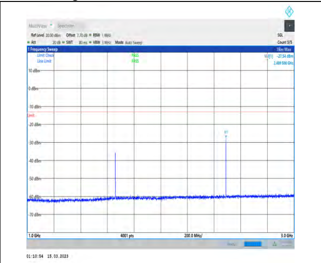
1-N5-PC3-15-20-H-1-DFT-PI2BPSK-Inner_1RB_Left -1@1-1000-3000-Ant1-2489.50--27.54--13-PASS
