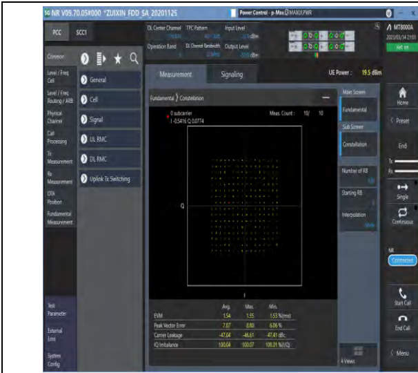
1-N5-PC3-15-20-M-5-DFT-256QAM-Outer_Full-100 @0-Ant1-see graph-PASS
