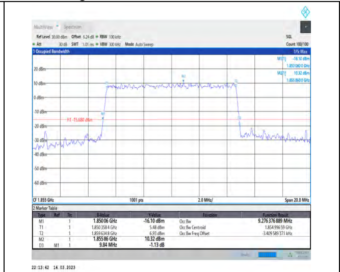
1-N2-PC3-15-10-L-7-CP-16QAM-Outer_Full-52@0-A nt1-9.276-9.840-≤10-PASS
