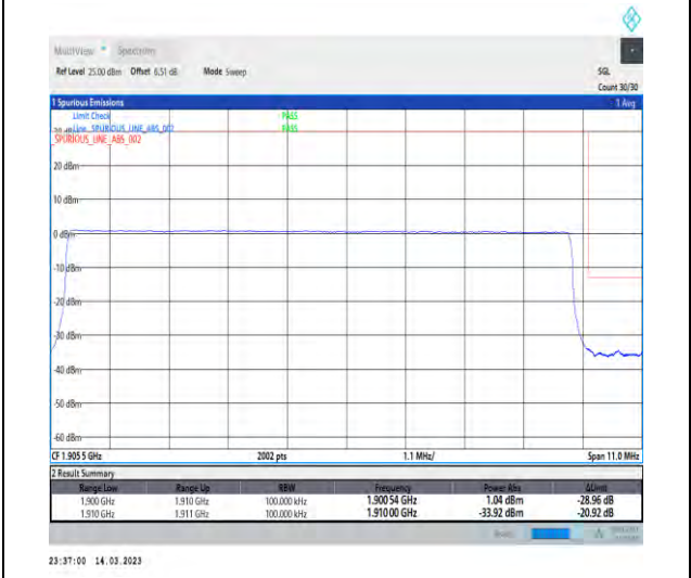
1-N2-PC3-15-10-H-6-CP-QPSK-Outer_Full-52@0-Ant1-1-seegraph-PASS-see graph
