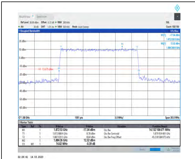
1-N2-PC3-15-15-M-6-CP-QPSK-Outer_Full-79@0-A Ant1-14.132-14.820-≤15-PASS
