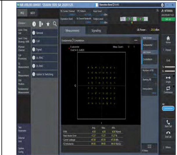
1-N2-PC3-15-20-M-8-CP-64QAM-Outer_Full-106@0-Ant1-see graph-PASS
