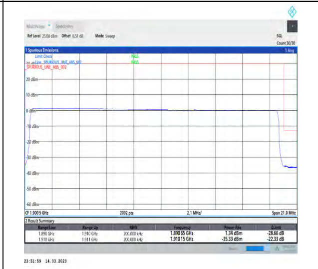
1-N2-PC3-15-20-H-6-CP-QPSK-Outer_Full-106@0-Ant1-1-seegraph-PASS-see graph
