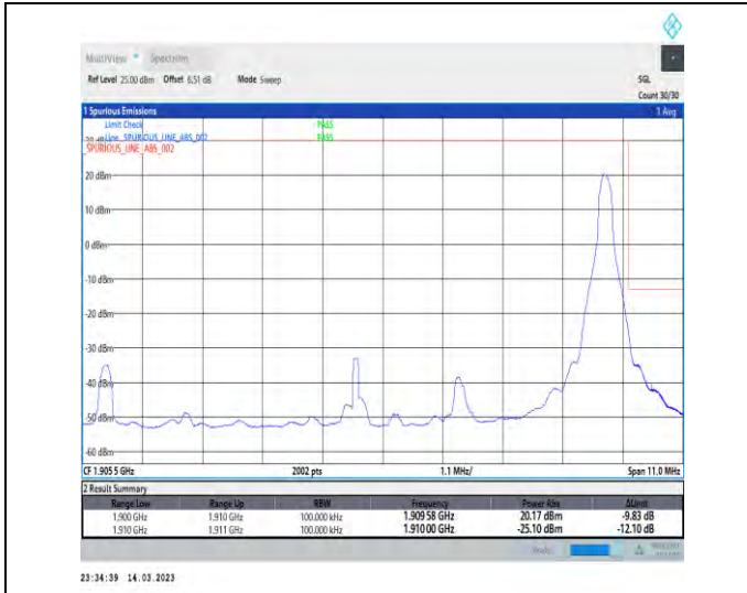
1-N2-PC3-15-10-H-2-DFT-PI2BPSK-Edge_1RB_Right-1@51-Ant1-1-seegraph-PASS-see graph
