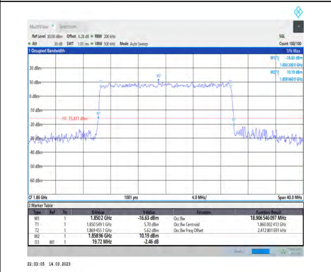
1-N2-PC3-15-20-L-7-CP-16QAM-Outer_Full-106@0-Ant1-18.907-19.720-≤20-PASS
