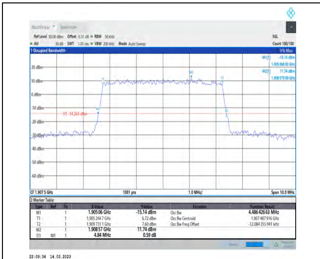
1-N2-PC3-15-5-H-3-DFT-16QAM-Outer_Full-25@0-Ant1-4.486-4.840-≤5-PASS
