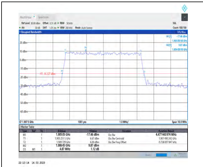
1-N2-PC3-15-5-H-7-CP-16QAM-Outer_Full-25@0-A nt1-4.477-4.870-≤5-PASS
