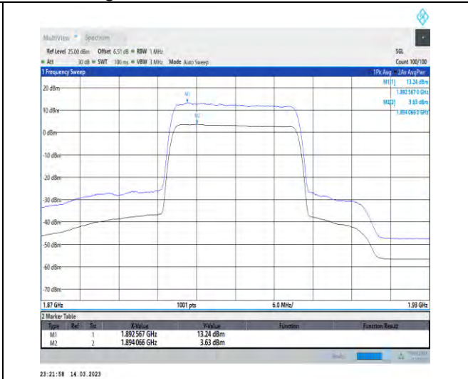
1-N2-PC3-15-20-H-2-CP-256QAM-Outer_Full-106 @0-Ant1-9.61-100%-0.00-9.61-PASS-≤13
