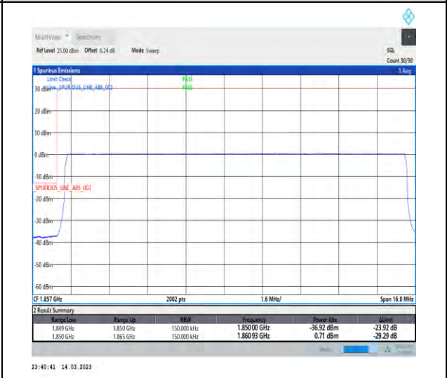
1-N2-PC3-15-15-L-6-CP-QPSK-Outer_Full-79@0-Ant1-1-seegraph-PASS-see graph
