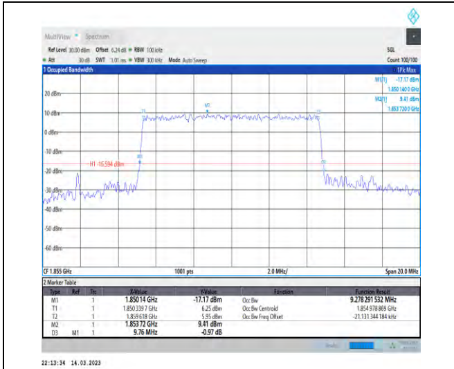
1-N2-PC3-15-10-L-6-CP-QPSK-Outer_Full-52@0-A nt1-9.278-9.760-≤10-PASS
