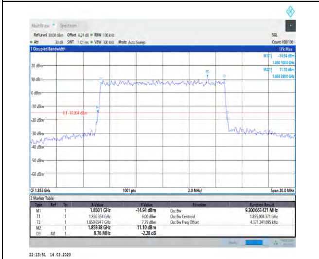
1-N2-PC3-15-10-L-8-CP-64QAM-Outer_Full-52@0-A Ant1-9.301-9.760-≤10-PASS
