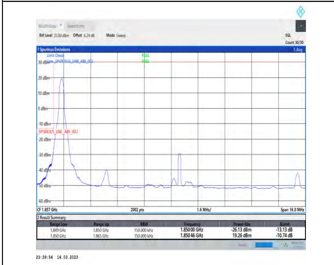
1-N2-PC3-15-15-L-4-CP-QPSK-Edge_1RB_Left-1@0-Ant1-1-seegraph-PASS-see graph
