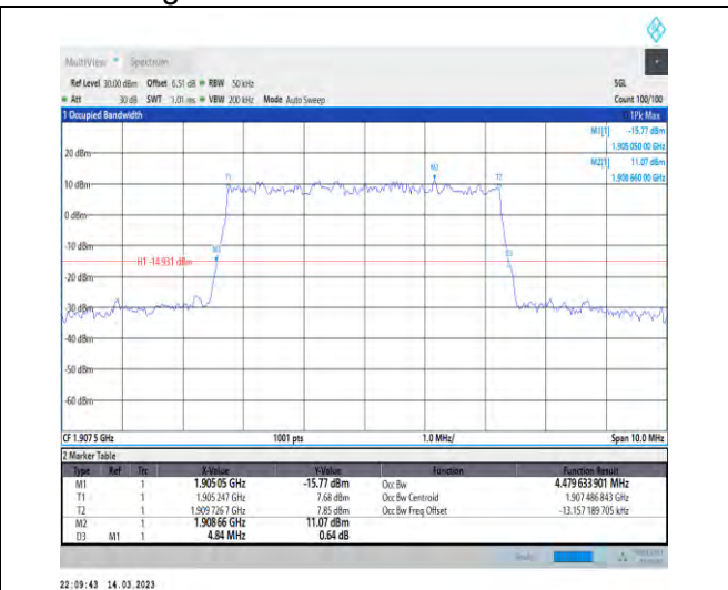
1-N2-PC3-15-5-H-4-DFT-64QAM-Outer_Full-25@0-Ant1-4.48-4.840-≤5-PASS
