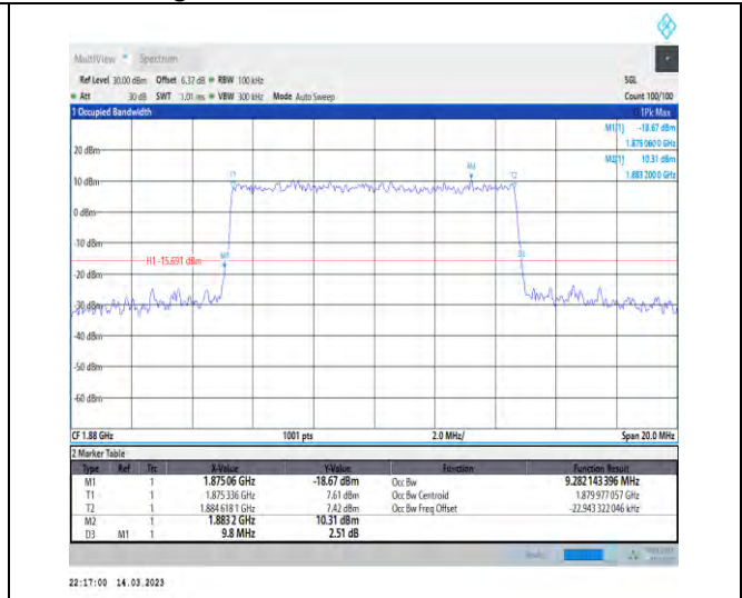
1-N2-PC3-15-10-M-6-CP-QPSK-Outer_Full-52@0-Ant1-9.282-9.800-≤10-PASS
