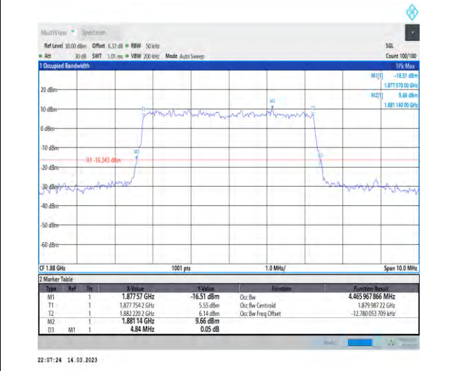
1-N2-PC3-15-5-M-7-CP-16QAM-Outer_Full-25@0-Ant1-4.466-4.840-≤5-PASS
