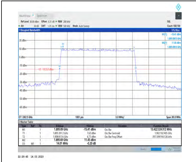
1-N2-PC3-15-15-H-5-DFT-256QAM-Outer_Full-75@ 0-Ant1-13.422-14.010-≤15-PASS
