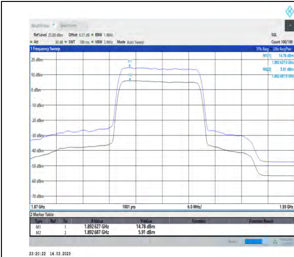
1-N2-PC3-15-20-H-1-DFT-256QAM-Outer_Full-100 @0-Ant1-8.87-100%-0.00-8.87-PASS-≤13
