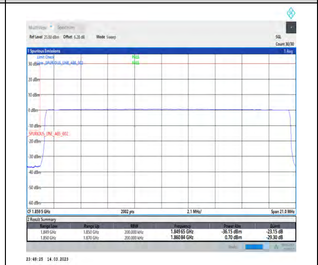
1-N2-PC3-15-20-L-6-CP-QPSK-Outer_Full-106@0-Ant1-1-seegraph-PASS-see graph
