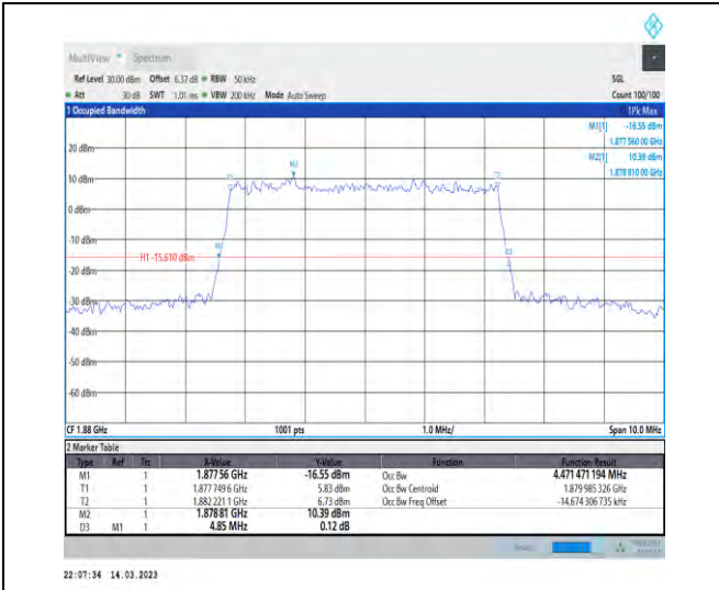
1-N2-PC3-15-5-M-8-CP-64QAM-Outer_Full-25@0-A nt1-4.471-4.850-≤5-PASS
