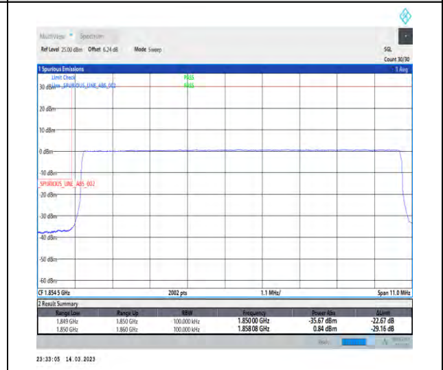
1-N2-PC3-15-10-L-6-CP-QPSK-Outer_Full-52@0-Ant1-1-seegraph-PASS-see graph
