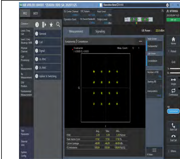
1-N2-PC3-15-20-M-7-CP-16QAM-Outer_Full-106@0-Ant1-see graph-PASS
