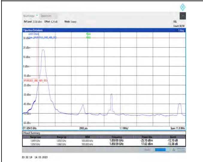
1-N2-PC3-15-10-L-4-CP-QPSK-Edge_1RB_Left-1@0-Ant1-1-seegraph-PASS-see graph
