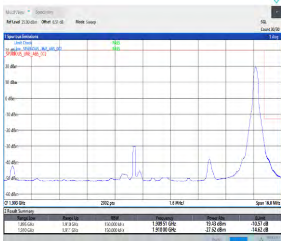
1-N2-PC3-15-15-H-5-CP-QPSK-Edge_1RB_Right-1@78-Ant1-1-seegraph-PASS-see graph
