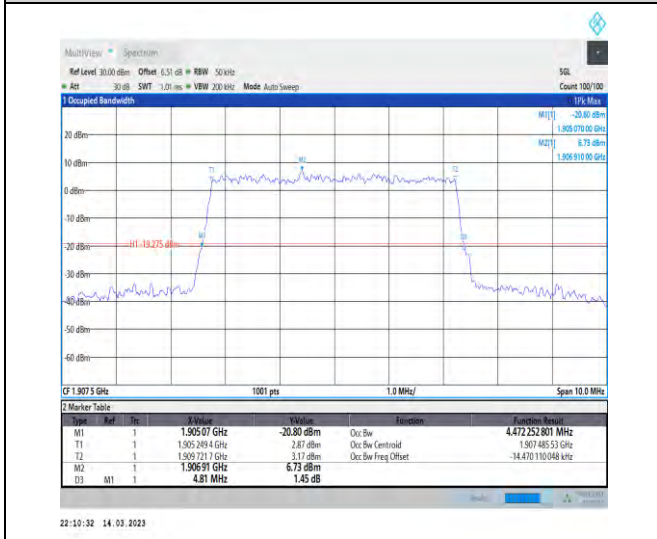
1-N2-PC3-15-5-H-9-CP-256QAM-Outer_Full-25@0-A Ant1-4.472-4.810-≤5-PASS
