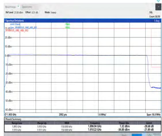
1-N2-PC3-15-15-H-6-CP-QPSK-Outer_Full-79@0-Ant1-1-seegraph-PASS-see graph
