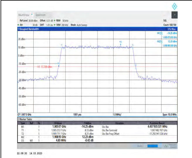
1-N2-PC3-15-5-H-1-DFT-QPSK-Outer_Full-25@0-A nt1-4.458-4.830-≤5-PASS
