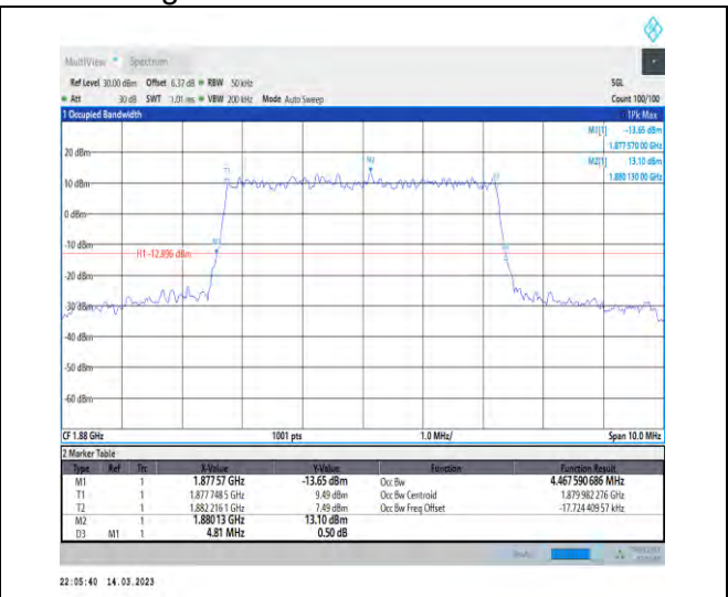
1-N2-PC3-15-5-M-1-DFT-QPSK-Outer_Full-25@0-Ant1-4.468-4.810-≤5-PASS
