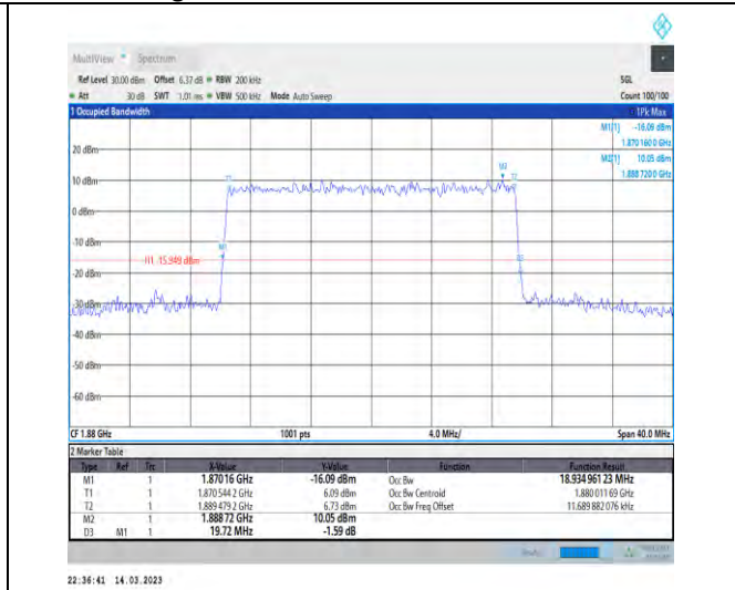
1-N2-PC3-15-20-M-8-CP-64QAM-Outer_Full-106@0 -Ant1-18.935-19.720-≤20-PASS
