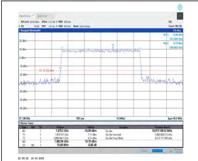
1-N2-PC3-15-20-M-7-CP-16QAM-Outer_Full-106@0 -Ant1-18.915-19.680-≤20-PASS
