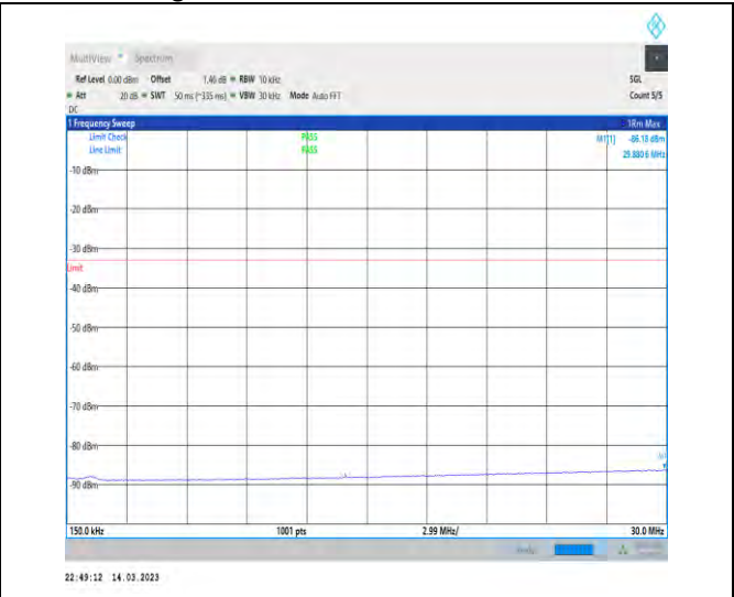
1-N2-PC3-15-20-H-1-DFT-PI2BPSK-Inner_1RB_Left- 1@1-0.15-30-Ant1-29.88--86.18--33-PASS
