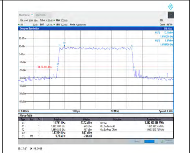
1-N2-PC3-15-10-M-8-CP-64QAM-Outer_Full-52@0-Ant1-9.283-9.780-≤10-PASS
