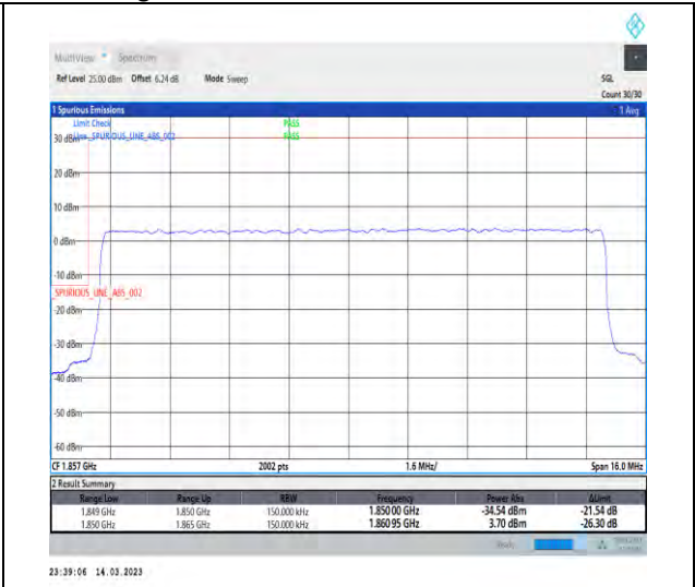
1-N2-PC3-15-15-L-3-DFT-PI2BPSK-Outer_Full-75 @0-Ant1-1-seegraph-PASS-see graph
