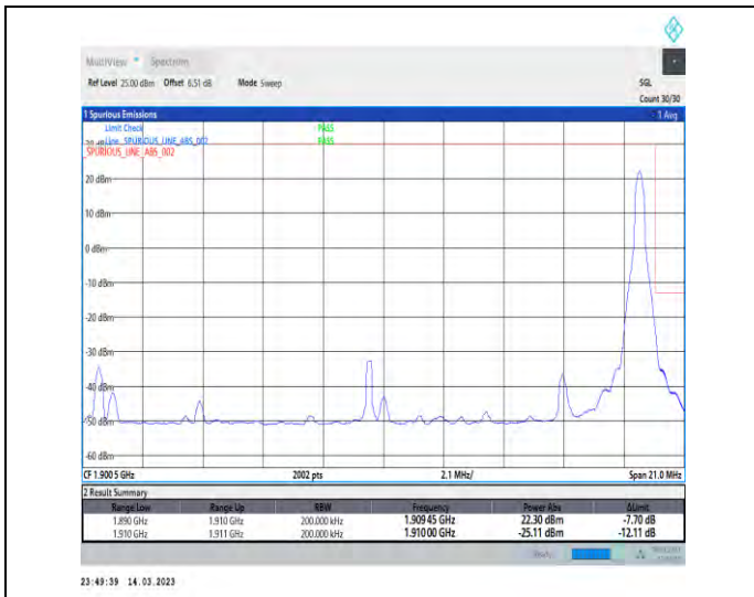
1-N2-PC3-15-20-H-2-DFT-PI2BPSK-Edge_1RB_Right-1@105-Ant1-1-seegraph-PASS-see graph
