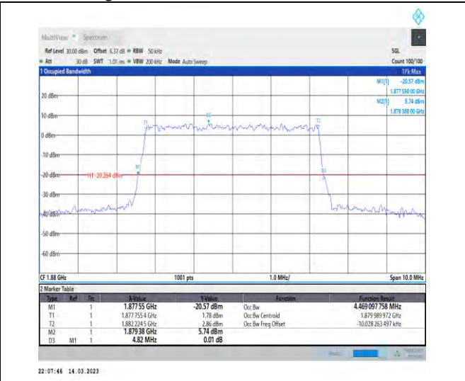
1-N2-PC3-15-5-M-9-CP-256QAM-Outer_Full-25@0-A Ant1-4.469-4.820-≤5-PASS
