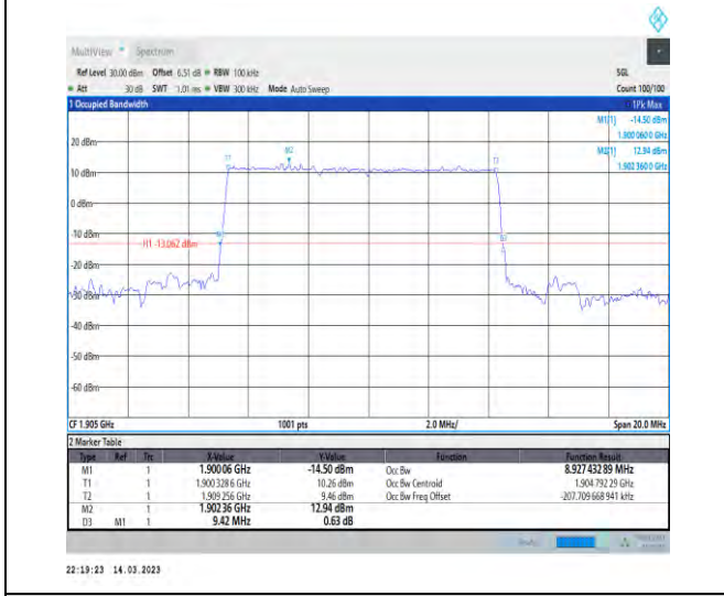
1-N2-PC3-15-10-H-2-DFT-PI2BPSK-Outer_Full-50@0- Ant1-8.927-9.420-≤10-PASS
