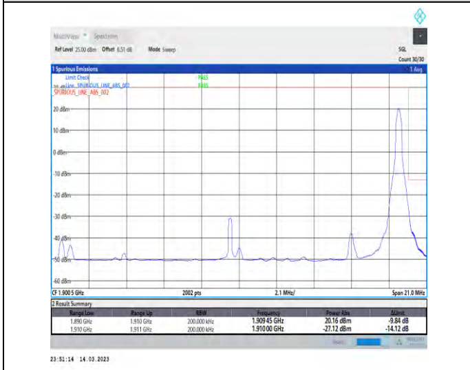
1-N2-PC3-15-20-H-5-CP-QPSK-Edge_1RB_Right-1@105-Ant1-1-seegraph-PASS-see graph
