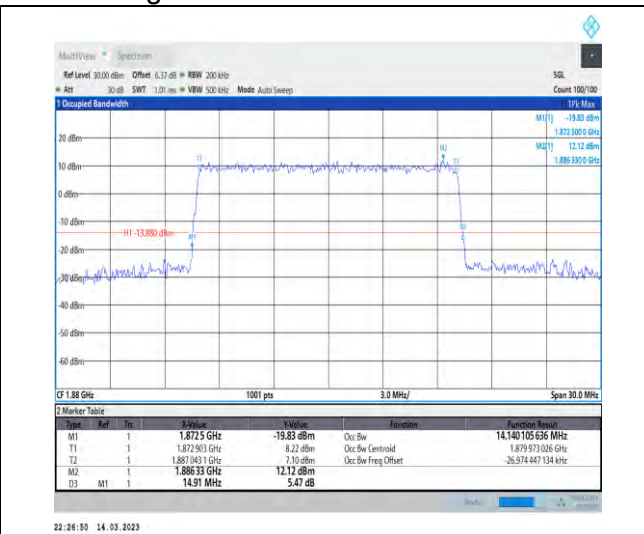
1-N2-PC3-15-15-M-7-CP-16QAM-Outer_Full-79@0- Ant1-14.14-14.910-≤15-PASS
