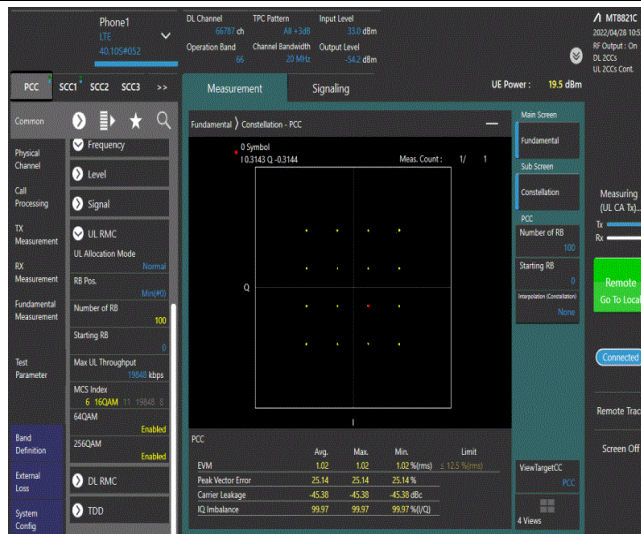
66-66-20MHz-20MHz-16QAM-16QAM -132323-132521-100RB#0-100RB#0
