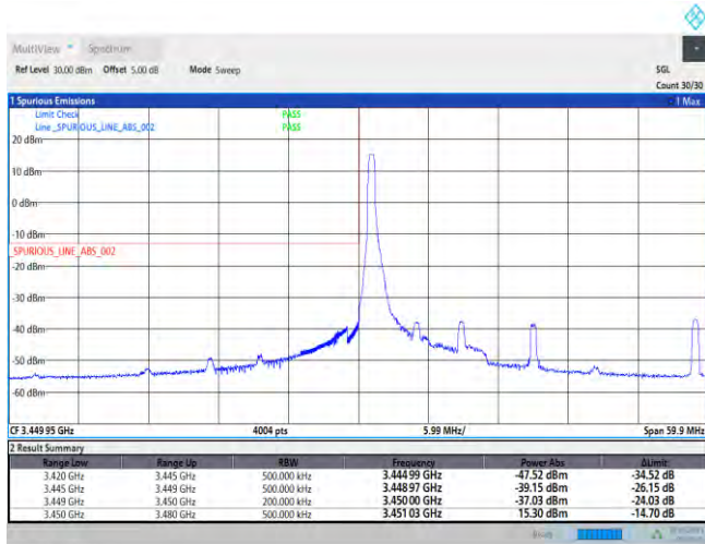
42-42-10MHz-20MHz-QPSK-QPSK-42145-42289-50RB#0-100RB#0
