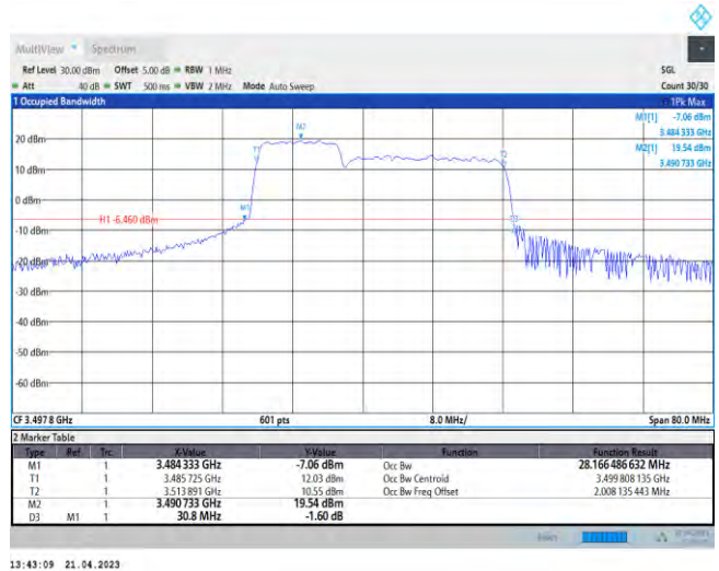
42-42-10MHz-20MHz-QPSK-QPSK-42496-42640-50RB#0-100RB#0
