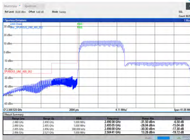
41-41-10MHz-15MHz-QPSK-QPSK-39703-39823-50RB#0-75RB#0
