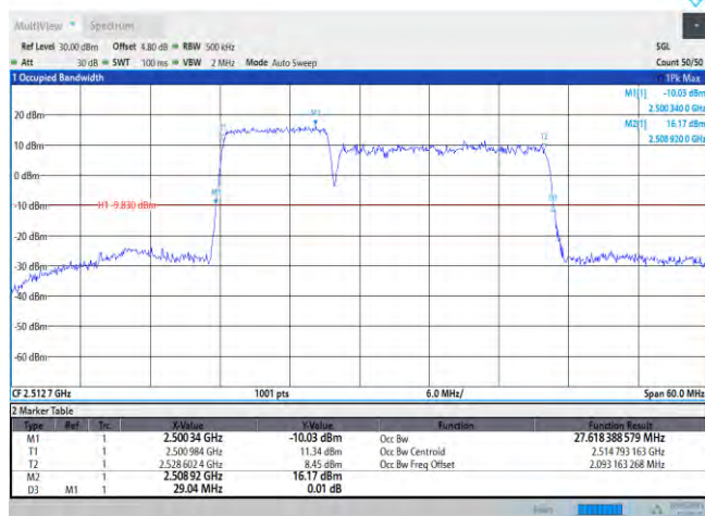
7-7-10MHz-20MHz-QPSK-QPSK-21006-21150-50RB#0-100RB#0
