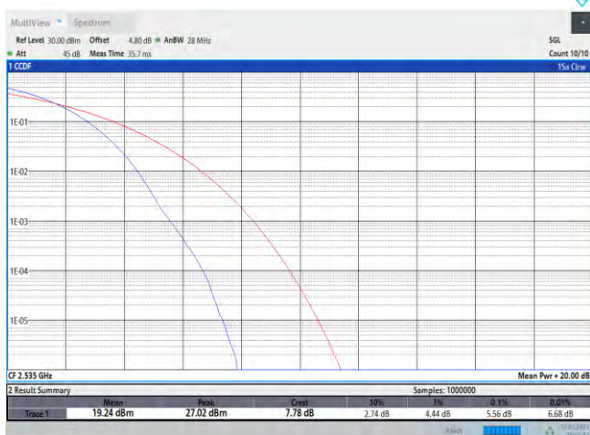
7-7-20MHz-20MHz-QPSK-QPSK-21001-21199-100RB#0-100RB#0
