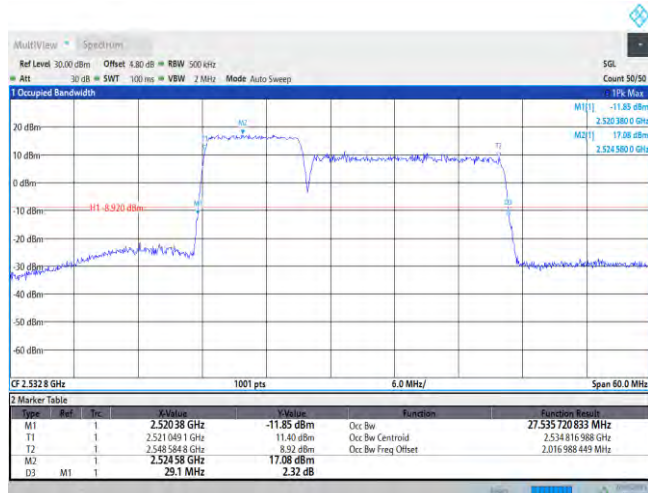
7-7-10MHz-20MHz-QPSK-QPSK-21006-21150-50RB#0-100RB#0
