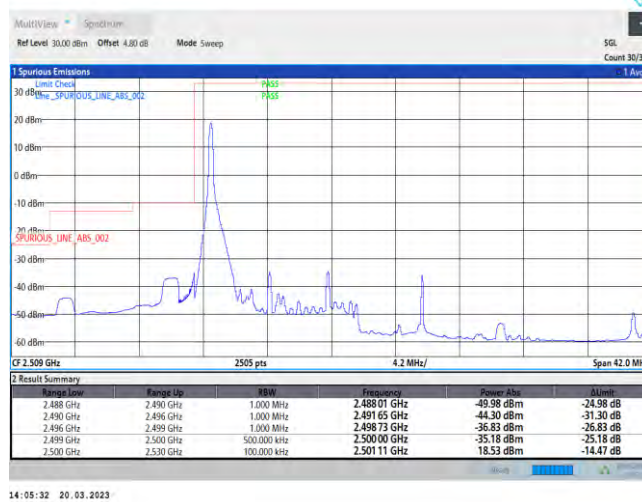
7-7-10MHz-20MHz-QPSK-QPSK-20805-20949-50RB#0-100RB#0
