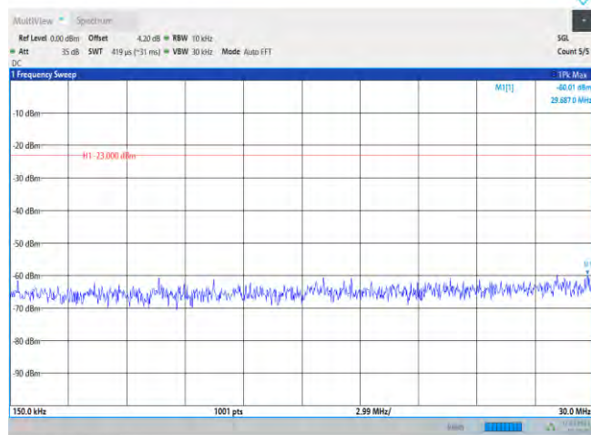
5-5-10MHz-10MHz-QPSK-QPSK-20450-20549-1RB#0-0RB#0-0.15~30MHz
