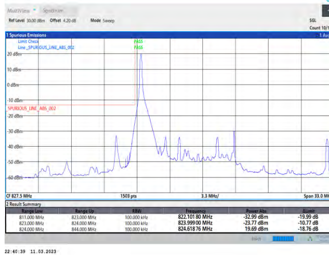
5-5-10MHz-10MHz-QPSK-QPSK-20450-20549-50RB#0-50RB#0
