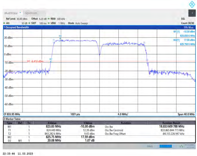
5-5-10MHz-10MHz-QPSK-QPSK-20476-20575-50RB#0-50RB#0
