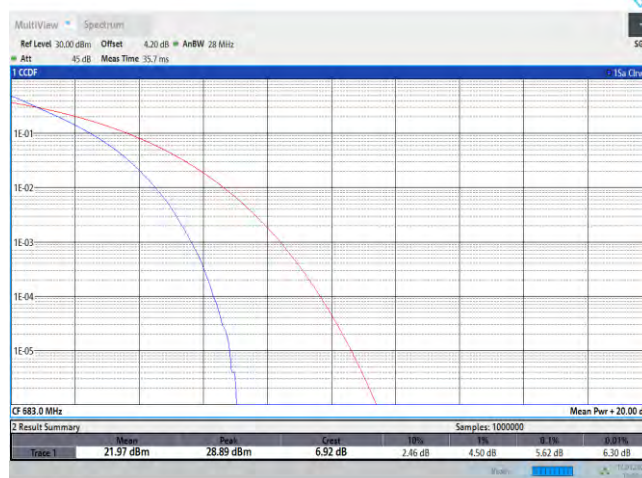
Band71-20MHz-QPSK-133322-100RB#0
