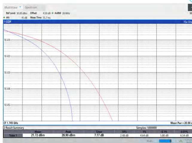
Band66-20MHz-QPSK-132322-100RB#0
