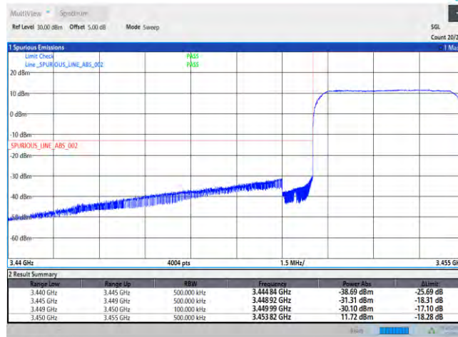
Band42-5MHz-QPSK-42115-25RB#0
