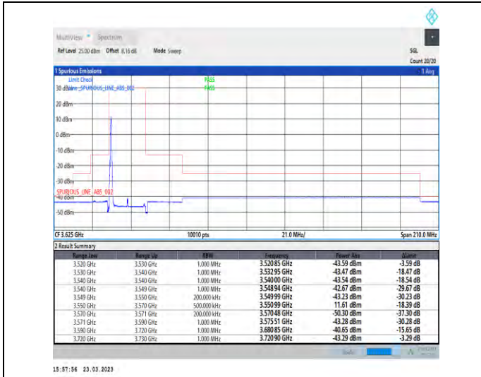
1-N48-PC3-30-20-L-1-CP-QPSK-Edge_1RB_Left-1@0-Ant1-1--PASS-see graph
