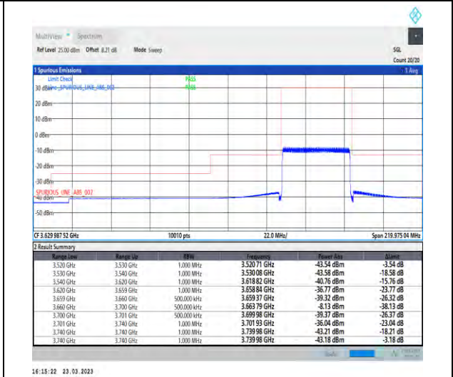
1-N48-PC3-30-40-H-3-CP-QPSK-Outer_Full-106@0-Ant1-1--PASS-see graph
