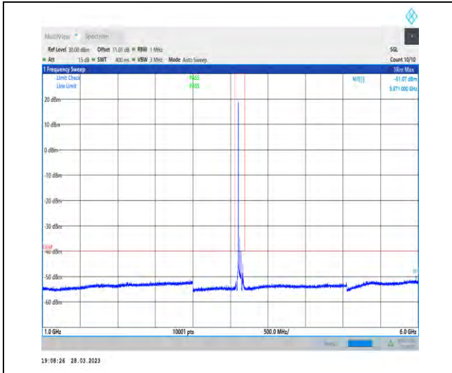
1-N48-PC3-30-40-M-1-CP-QPSK-Edge_1RB_Left-1 @0-1000-6000-Ant2-5971.00--51.07--40-PASS
