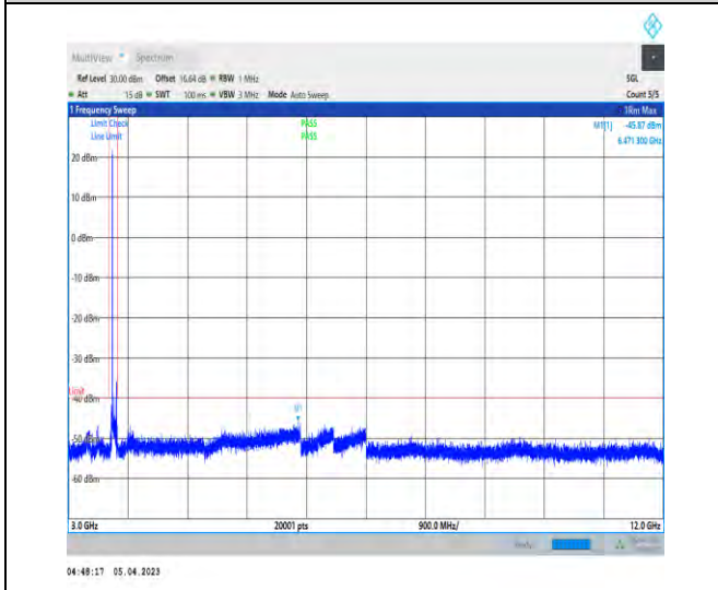
1-N48-PC3-30-40-H-1-DFT-PI2BPSK-Inner_1RB_Le ft-1@1-3000-12000-Ant1-3368.55--45.87--40-PASS
