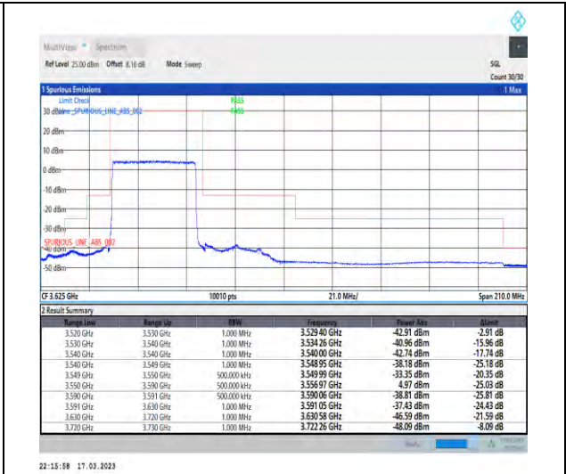
1-N48-PC3-30-40-L-3-DFT-PI2BPSK-Outer_Full-100@0-Ant1-1--PASS-see graph
