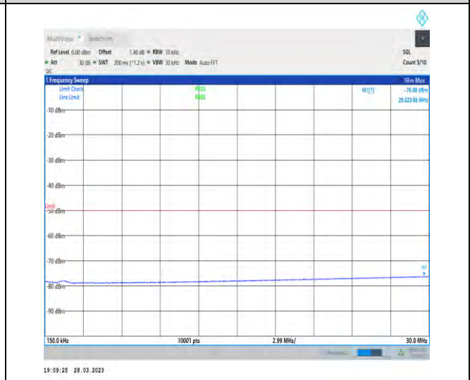
1-N48-PC3-30-40-H-1-CP-QPSK-Edge_1RB_Left-1 @0-0.15-30-Ant2-29.62--76.09--50-PASS
