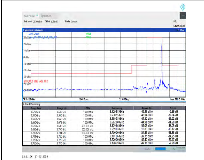
1-N48-PC3-30-20-H-5-CP-QPSK-Edge_1RB_Right-1@50-Ant1-1--PASS-see graph
