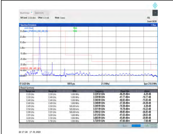
1-N48-PC3-30-40-L-4-CP-QPSK-Edge_1RB_Left-1@0-Ant1-1--PASS-see graph
