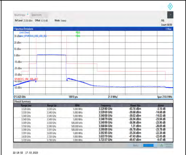
1-N48-PC3-30-40-L-6-CP-QPSK-Outer_Full-106@0-Ant1-1--PASS-see graph
