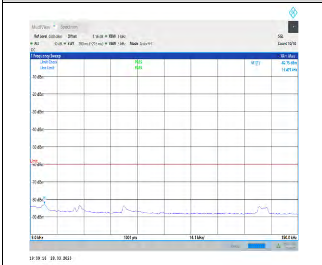
1-N48-PC3-30-40-H-1-CP-QPSK-Edge_1RB_Left-1 @0-0.009-0.15-Ant2-0.02--82.75--60-PASS
