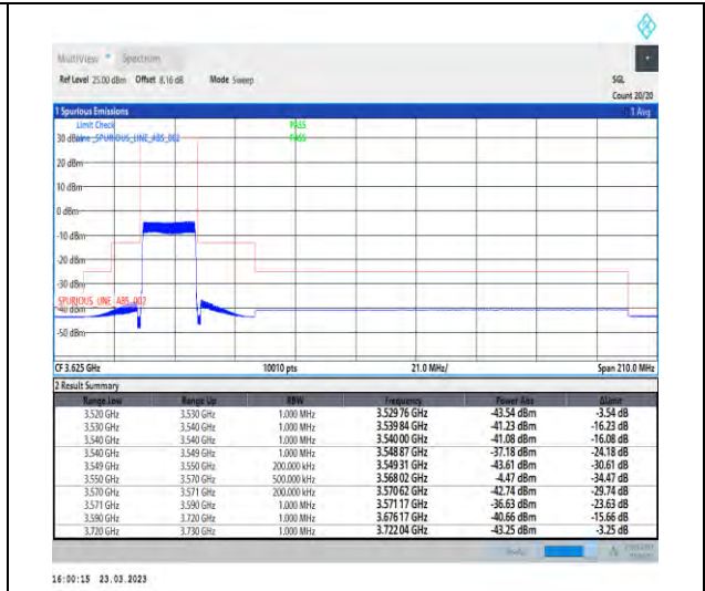
1-N48-PC3-30-20-L-3-CP-QPSK-Outer_Full-51@0-Ant1-1--PASS-see graph
