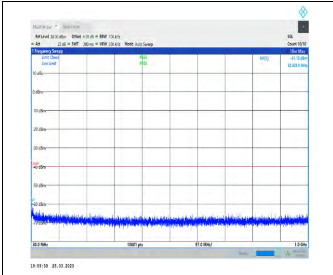
1-N48-PC3-30-40-H-1-CP-QPSK-Edge_1RB_Left-1 @0-30-1000-Ant2-32.43--61.13--40-PASS
