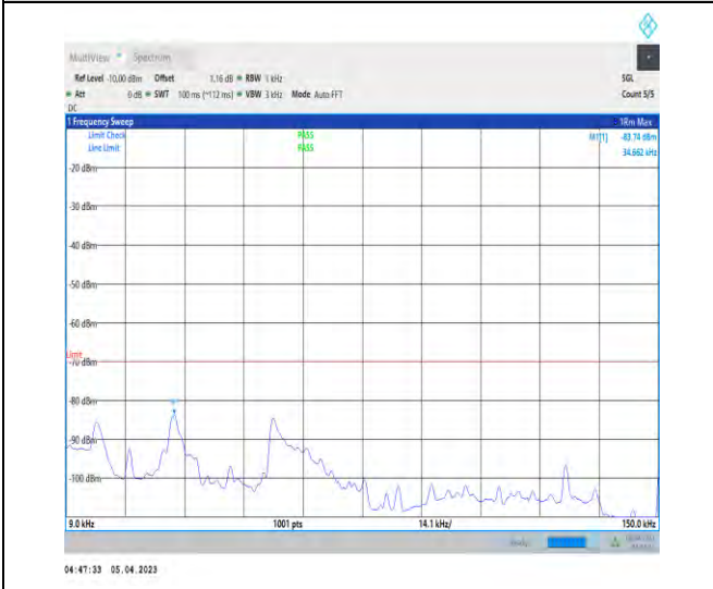
1-N48-PC3-30-40-H-1-DFT-PI2BPSK-Inner_1RB_Le ft-1@1-0.009-0.15-Ant1-0.06--83.74--70-PASS
