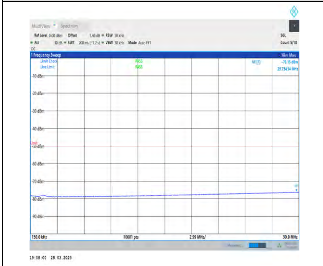
1-N48-PC3-30-40-M-1-CP-QPSK-Edge_1RB_Left-1 @0-0.15-30-Ant2-29.73--76.15--50-PASS
