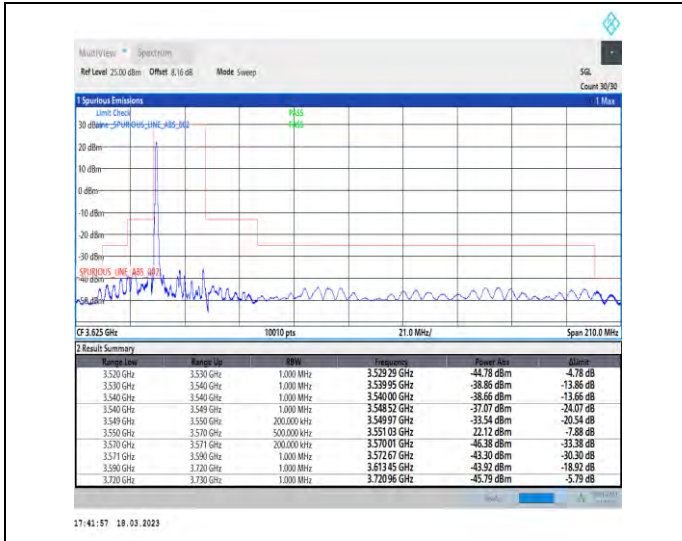
1-N48-PC3-30-20-L-1-DFT-PI2BPSK-Edge_1RB_Left-1@0-Ant1-1--PASS-see graph
