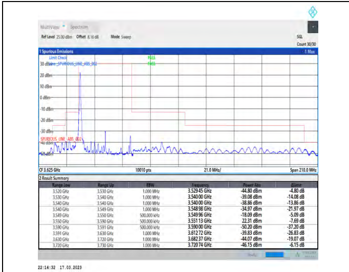
1-N48-PC3-30-40-L-1-DFT-PI2BPSK-Edge_1RB_Left-1@0-Ant1-1--PASS-see graph
