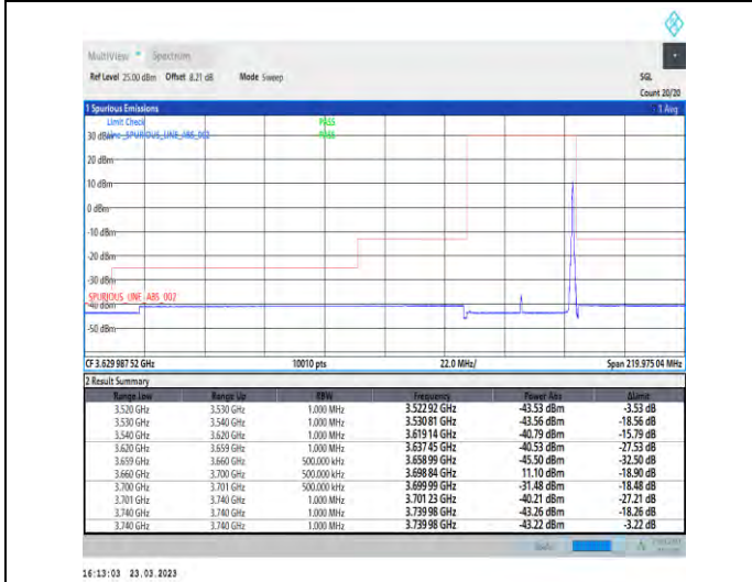
1-N48-PC3-30-40-H-2-CP-QPSK-Edge_1RB_Right-1@105-Ant1-1--PASS-see graph
