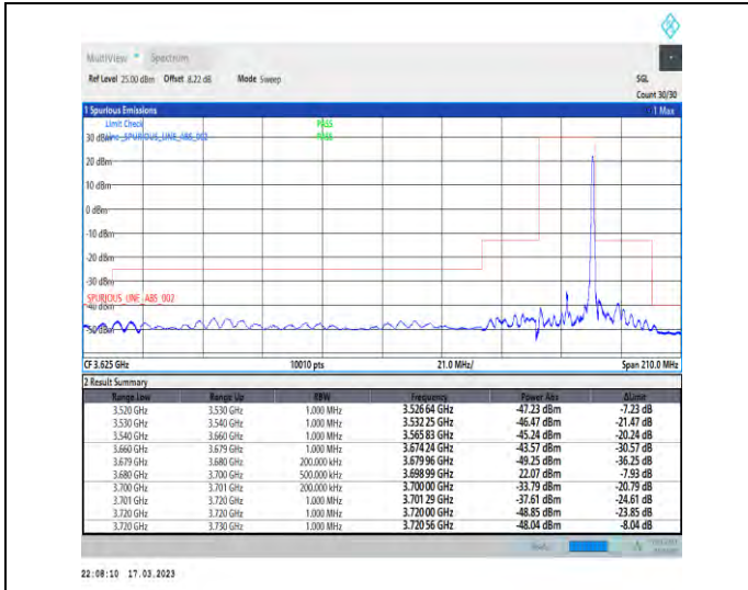
1-N48-PC3-30-20-H-2-DFT-PI2BPSK-Edge_1RB_Right-t-1@50-Ant1-1--PASS-see graph
