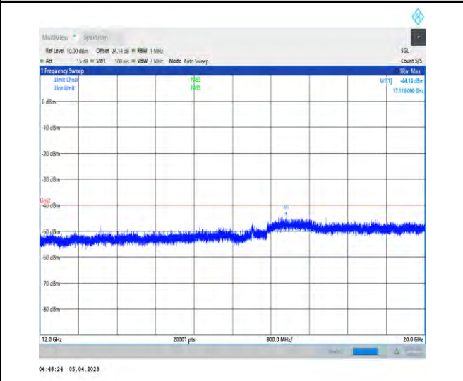
1-N48-PC3-30-40-H-1-DFT-PI2BPSK-Inner_1RB_Le ft-1@1-12000-20000-Ant1-17080.40--44.14--40-PASS
