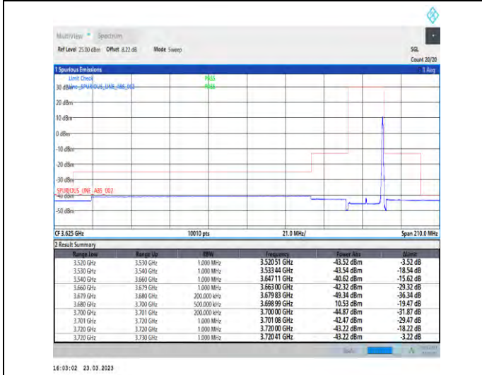
1-N48-PC3-30-20-H-2-CP-QPSK-Edge_1RB_Right-1@50-Ant1-1--PASS-see graph
