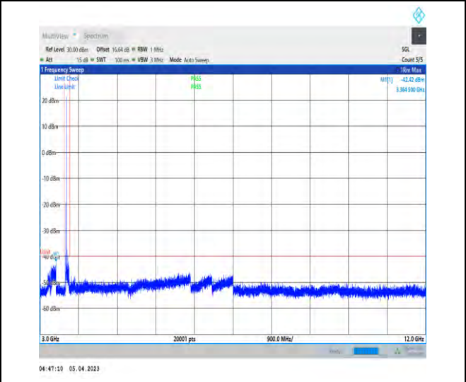
1-N48-PC3-30-40-M-1-DFT-PI2BPSK-Inner_1RB_Le ft-1@1-3000-12000-Ant1-3322.20--42.42--40-PASS
