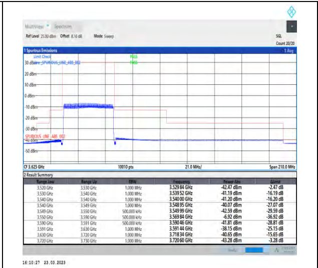
1-N48-PC3-30-40-L-3-CP-QPSK-Outer_Full-106@0-Ant1-1--PASS-see graph
