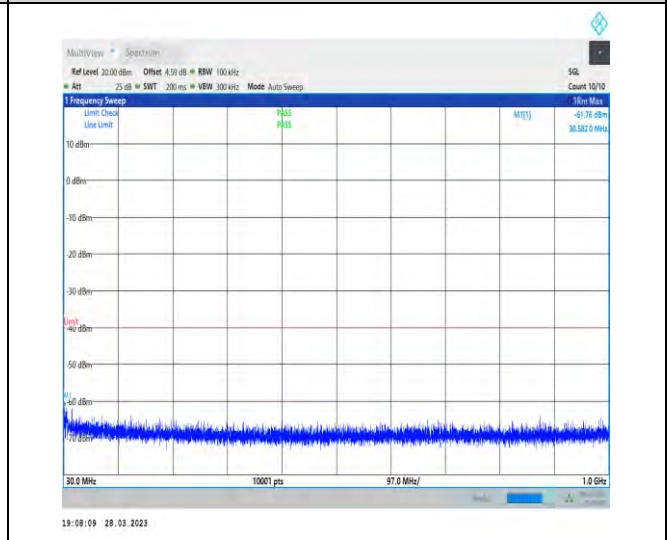
1-N48-PC3-30-40-M-1-CP-QPSK-Edge_1RB_Left-1 @0-30-1000-Ant2-30.58--61.76--40-PASS
