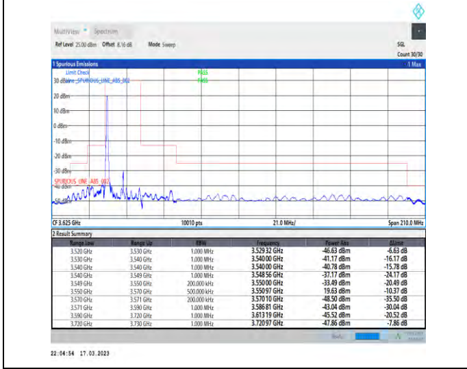
1-N48-PC3-30-20-L-4-CP-QPSK-Edge_1RB_Left-1@0-Ant1-1--PASS-see graph
