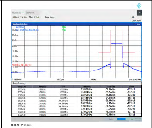
1-N48-PC3-30-20-H-6-CP-QPSK-Outer_Full-51@0-Ant1-1--PASS-see graph
