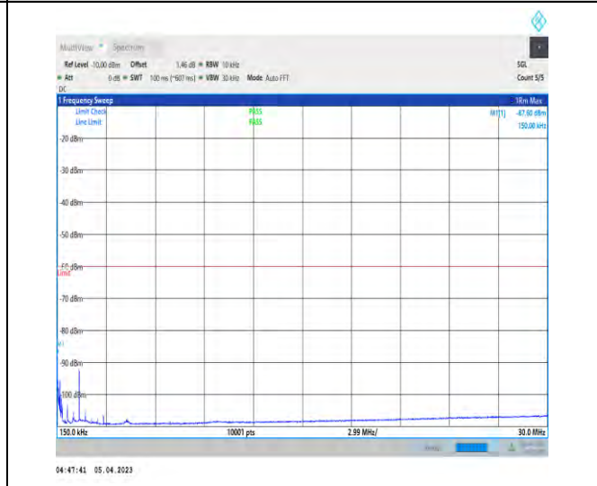
1-N48-PC3-30-40-H-1-DFT-PI2BPSK-Inner_1RB_Le ft-1@1-0.15-30-Ant1-0.15--87.60--60-PASS
