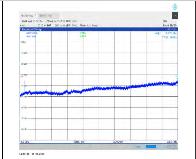
1-N48-PC3-30-40-M-1-CP-QPSK-Edge_1RB_Left-1 @0-6000-38000-Ant2-6000.00--44.27--40-PASS
