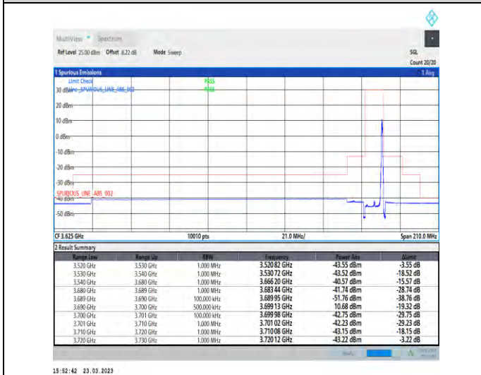
1-N48-PC3-30-10-H-2-CP-QPSK-Edge_1RB_Right-1@23-Ant1-1--PASS-see graph
