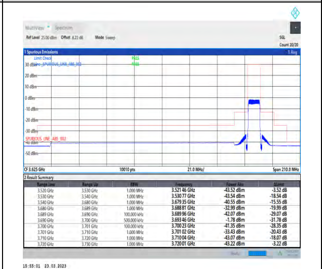
1-N48-PC3-30-10-H-3-CP-QPSK-Outer_Full-24@0-Ant1-1--PASS-see graph
