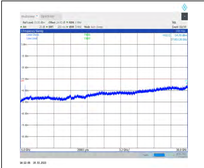
1-N48-PC3-30-40-L-1-CP-QPSK-Edge_1RB_Left-1 @0-6000-38000-Ant2-6000.00--39.36--40-PASS
