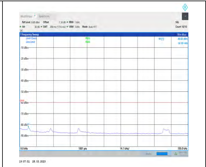
1-N48-PC3-30-40-M-1-CP-QPSK-Edge_1RB_Left-1 @0-0.009-0.15-Ant2-0.02--83.02--60-PASS
