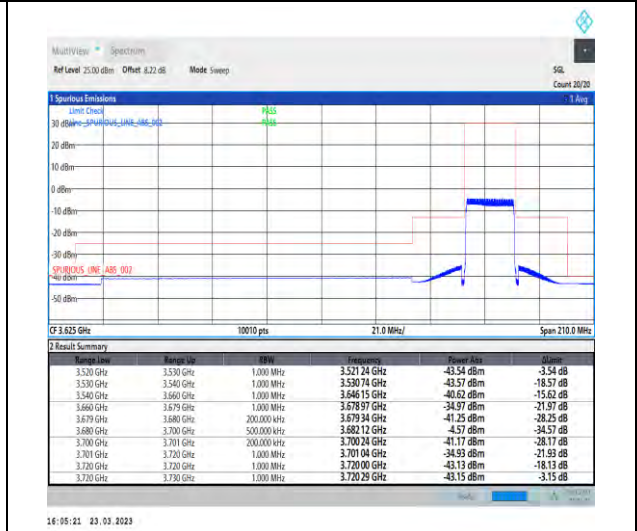
1-N48-PC3-30-20-H-3-CP-QPSK-Outer_Full-51@0-Ant1-1--PASS-see graph
