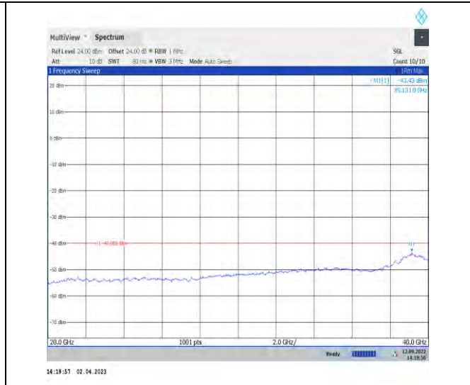
1-N48-PC3-30-40-H-1-DFT-PI2BPSK-Inner_1RB_Le ft-1@1-20000-40000-Ant1-61.62--54.53--50-PASS
