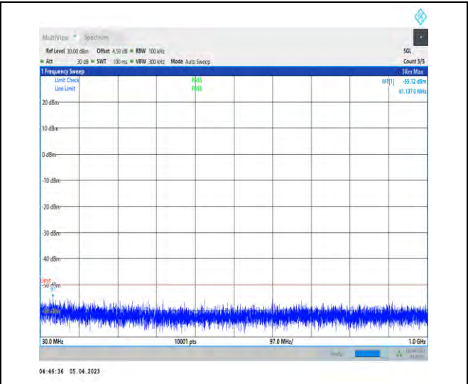
1-N48-PC3-30-40-M-1-DFT-PI2BPSK-Inner_1RB_Le ft-1@1-30-1000-Ant1-45.13--55.12--50-PASS
