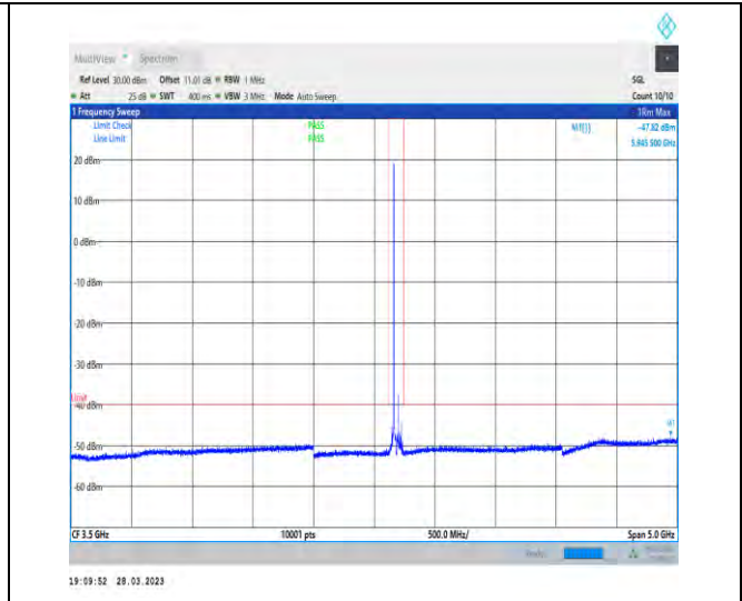
1-N48-PC3-30-40-H-1-CP-QPSK-Edge_1RB_Left-1 @0-1000-6000-Ant2-5945.50--47.82--40-PASS
