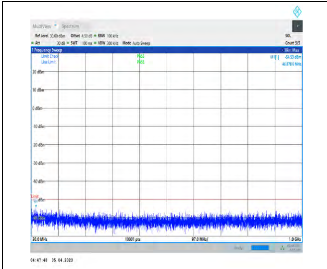
1-N48-PC3-30-40-H-1-DFT-PI2BPSK-Inner_1RB_Le ft-1@1-30-1000-Ant1-61.62--54.53--50-PASS
