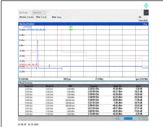
1-N48-PC3-30-40-L-1-CP-QPSK-Edge_1RB_Left-1@0-Ant1-1--PASS-see graph
