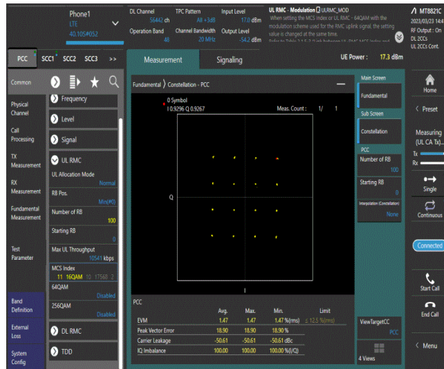
48-48-20MHz-20MHz-16QAM-16QAM-56442-56640-100RB#0-100RB#0
