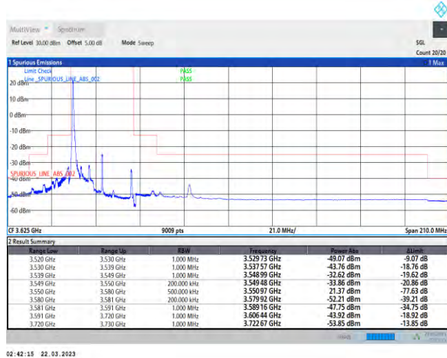
48-48-10MHz-20MHz-QPSK-QPSK-55295-55439-50RB#0-100RB#0
