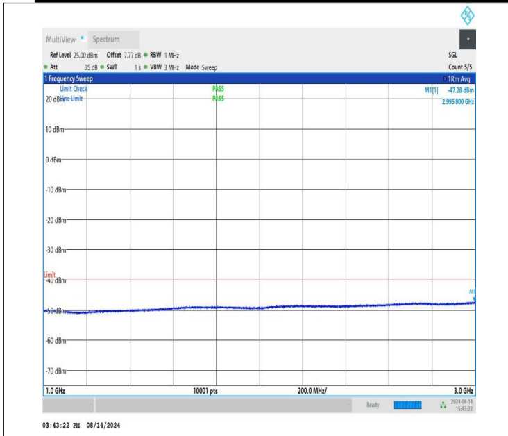
NTNV-n48-PC3-30-15-H-CP-QPSK-Edge_1RB_Right-1000-3000-PASS
