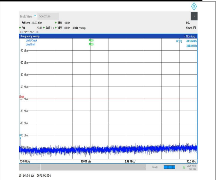
NTNV-n48-PC3-30-40-M-CP-QPSK-Edge_1RB_Left-0.15-30-PASS
