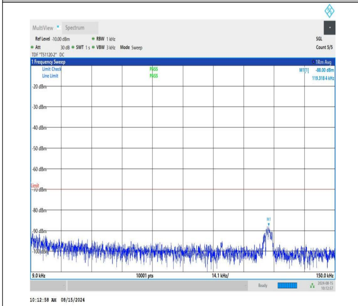
NTNV-n48-PC3-30-20-M-CP-QPSK-Edge_1RB_Left-0.009-0.15-P ASS
