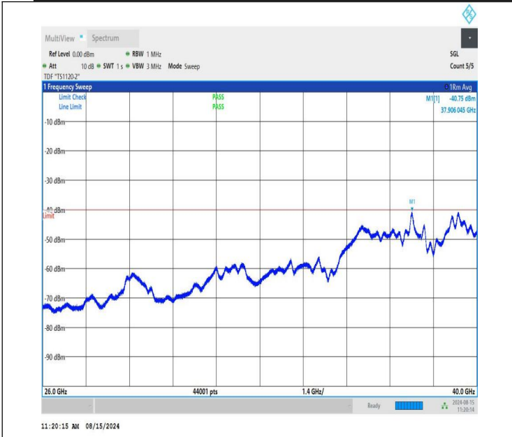
NTNV-n48-PC3-30-40-H-CP-QPSK-Edge_1RB_Left-26000-40000 -PASS
