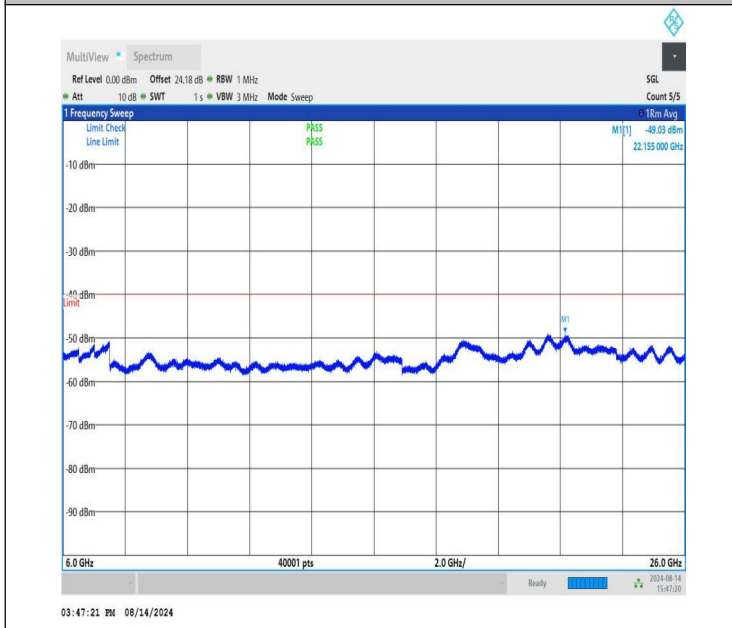
NTNV-n48-PC3-30-20-M-CP-QPSK-Edge_1RB_Right-6000-2600-0-PASS
