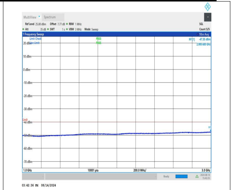
NTNV-n48-PC3-30-15-H-CP-QPSK-Edge_1RB_Left-1000-3000-PASS
