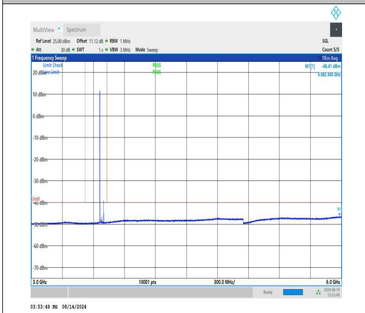
NTNV-n48-PC3-30-40-H-CP-QPSK-Edge_1RB_Left-3000-6000-P ASS
