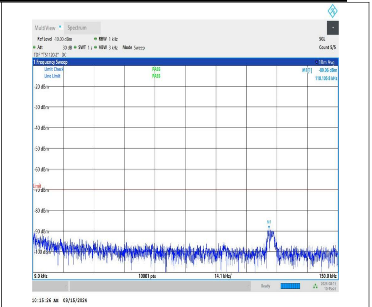
NTNV-n48-PC3-30-40-L-CP-QPSK-Edge_1RB_Right-0.009-0.15-P ASS
