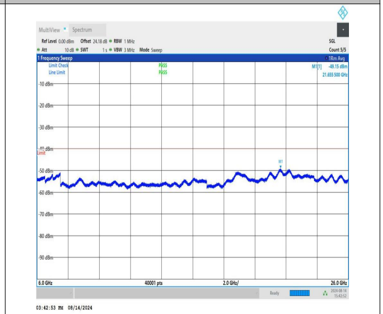
NTNV-n48-PC3-30-15-H-CP-QPSK-Edge_1RB_Left-6000-26000-PASS
