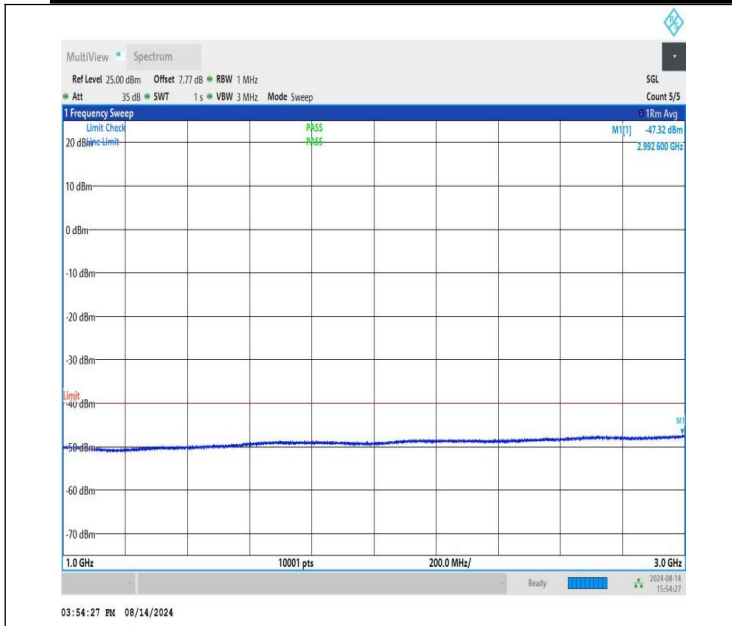
NTNV-n48-PC3-30-40-H-CP-QPSK-Edge_1RB_Right-1000-3000-PASS
