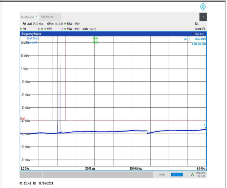
NTNV-n48-PC3-30-40-M-CP-QPSK-Edge_1RB_Right-3000-6000-P ASS
