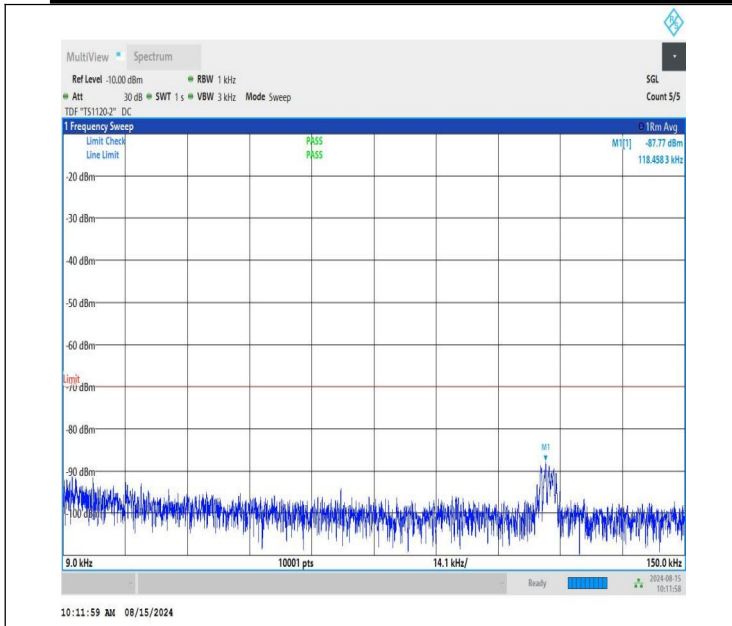
NTNV-n48-PC3-30-20-L-CP-QPSK-Edge_1RB_Left-0.009-0.15-P ASS
