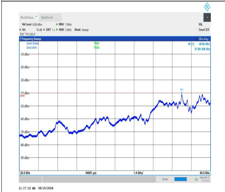
NTNV-n48-PC3-30-15-M-CP-QPSK-Edge_1RB_Left-26000-40000 -PASS
