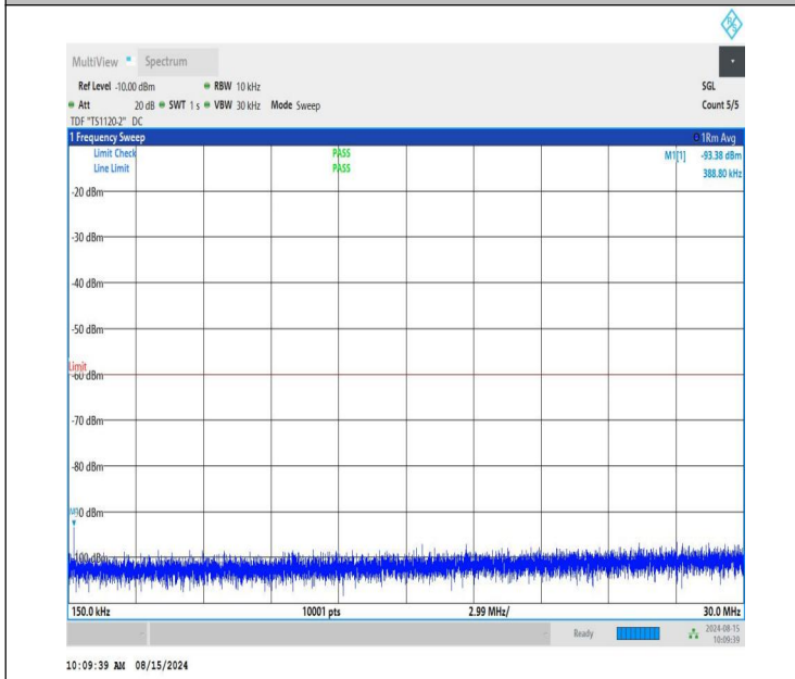
NTNV-n48-PC3-30-15-L-CP-QPSK-Edge_1RB_Right-0.15-30-PA SS
