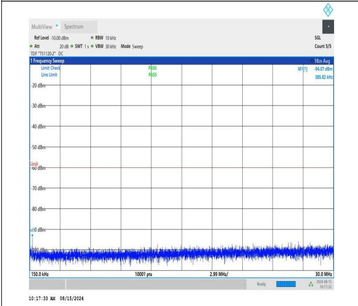
NTNV-n48-PC3-30-40-H-CP-QPSK-Edge_1RB_Right-0.15-30-PA SS
