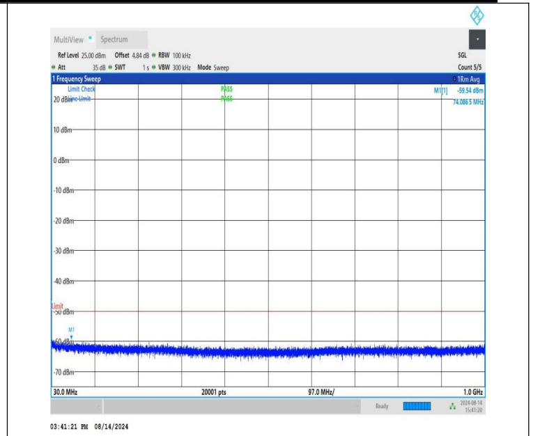
NTNV-n48-PC3-30-15-M-CP-QPSK-Edge_1RB_Right-30-1000-PA SS
