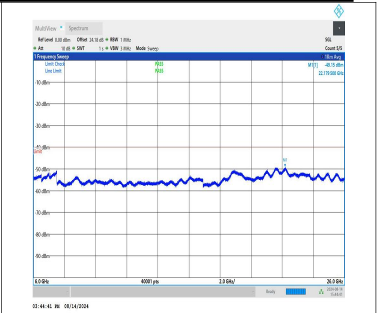
NTNV-n48-PC3-30-20-L-CP-QPSK-Edge_1RB_Left-6000-26000-P ASS
