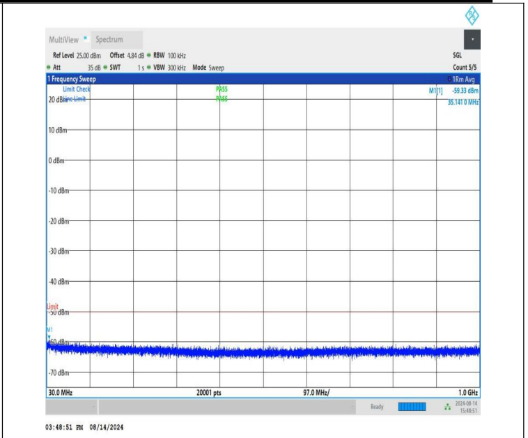
NTNV-n48-PC3-30-20-H-CP-QPSK-Edge_1RB_Right-30-1000-PA SS
