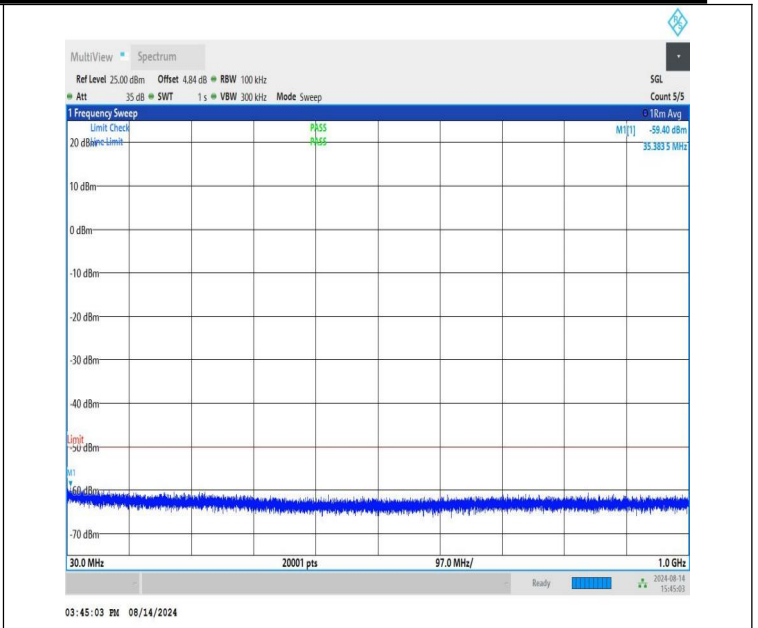
NTNV-n48-PC3-30-20-L-CP-QPSK-Edge_1RB_Right-30-1000-PAS S
