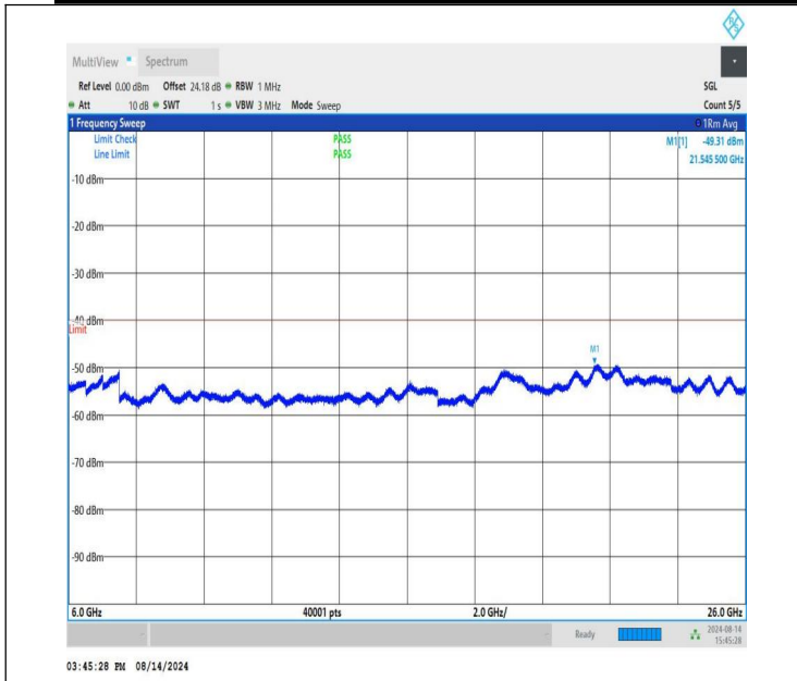
NTNV-n48-PC3-30-20-L-CP-QPSK-Edge_1RB_Right-6000-26000 -PASS
