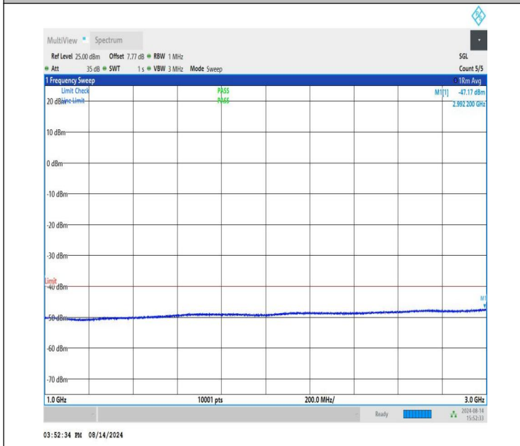
NTNV-n48-PC3-30-40-M-CP-QPSK-Edge_1RB_Right-1000-3000- PASS
