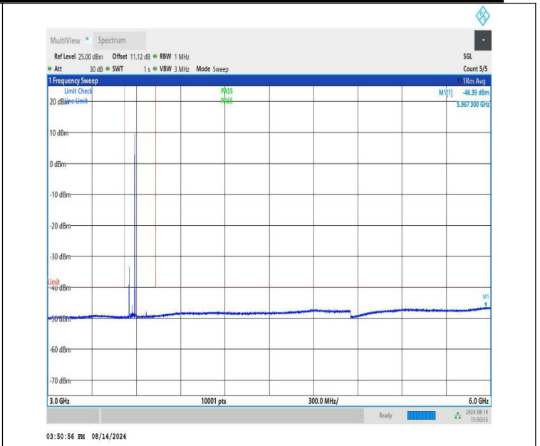
NTNV-n48-PC3-30-40-L-CP-QPSK-Edge_1RB_Right-3000-6000-PASS
