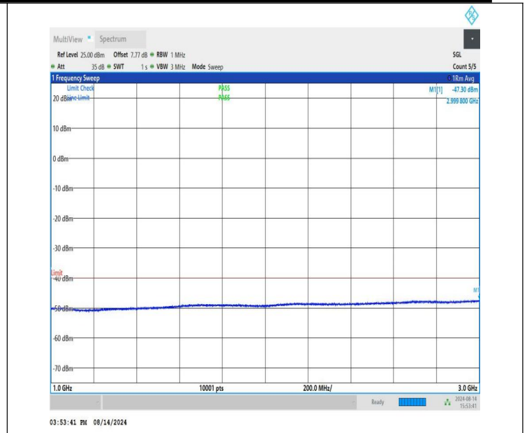
NTNV-n48-PC3-30-40-H-CP-QPSK-Edge_1RB_Left-1000-3000-PA SS
