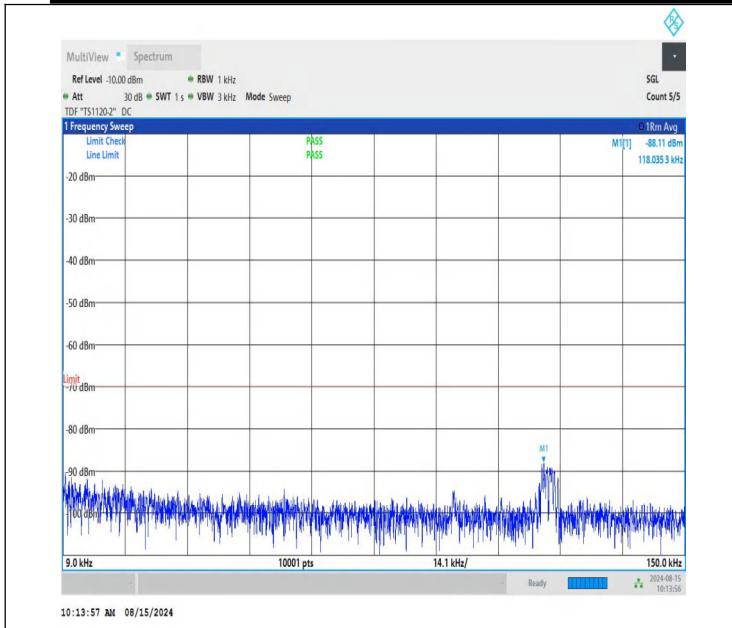
NTNV-n48-PC3-30-20-H-CP-QPSK-Edge_1RB_Left-0.009-0.15-P ASS
