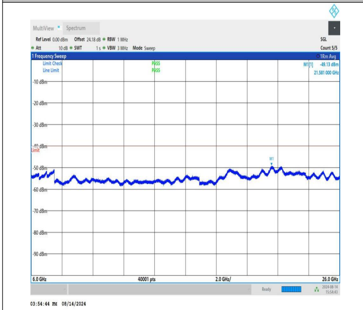
NTNV-n48-PC3-30-40-H-CP-QPSK-Edge_1RB_Right-6000-26000-PASS
