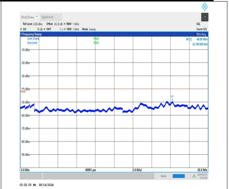
NTNV-n48-PC3-30-40-M-CP-QPSK-Edge_1RB_Left-6000-26000-P ASS
