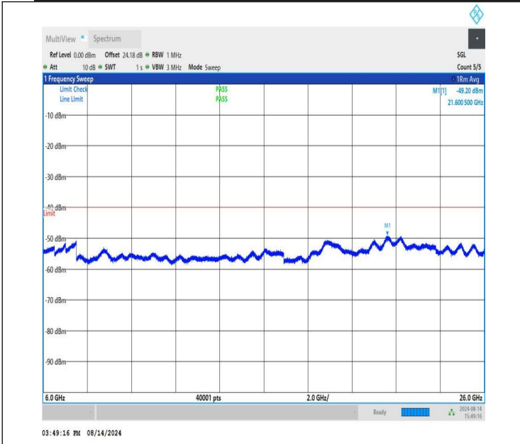
NTVN-n48-PC3-30-20-H-CP-QPSK-Edge_1RB_Right-6000-26000 -PASS
