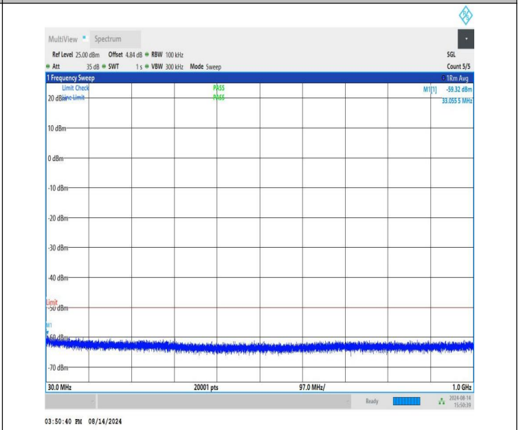
NTNV-n48-PC3-30-40-L-CP-QPSK-Edge_1RB_Right-30-1000-PAS S
