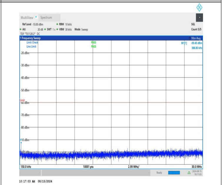
NTNV-n48-PC3-30-40-H-CP-QPSK-Edge_1RB_Left-0.15-30-PASS
