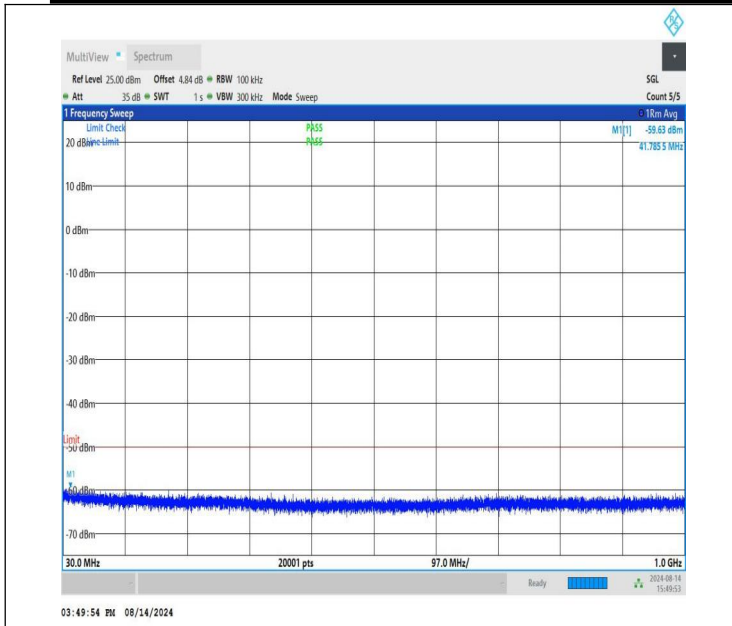
NTNV-n48-PC3-30-40-L-CP-QPSK-Edge_1RB_Left-30-1000-PAS S
