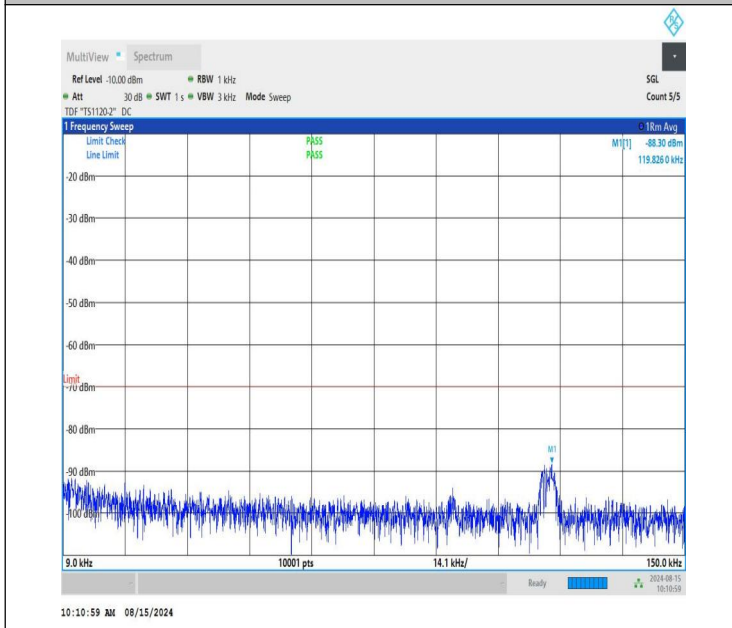
NTNV-n48-PC3-30-15-H-CP-QPSK-Edge_1RB_Left-0.009-0.15-P ASS
