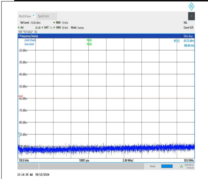
NTNV-n48-PC3-30-20-H-CP-QPSK-Edge_1RB_Right-0.15-30-PA SS
