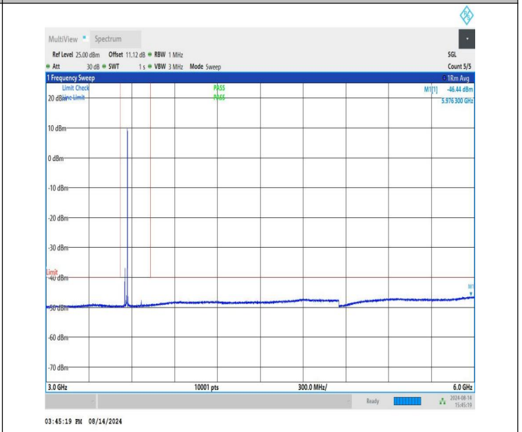
NTNV-n48-PC3-30-20-L-CP-QPSK-Edge_1RB_Right-3000-6000-P ASS
