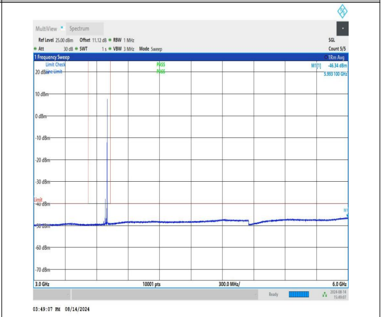
NTNV-n48-PC3-30-20-H-CP-QPSK-Edge_1RB_Right-3000-6000-P ASS
