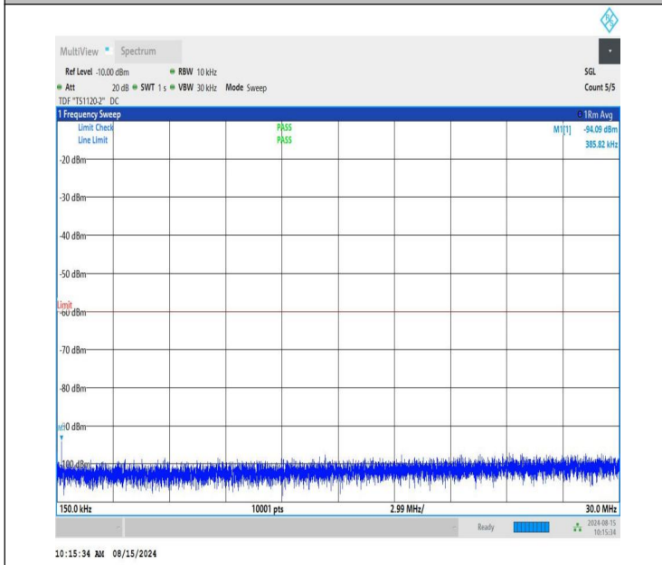
NTNV-n48-PC3-30-40-L-CP-QPSK-Edge_1RB_Right-0.15-30-PA SS
