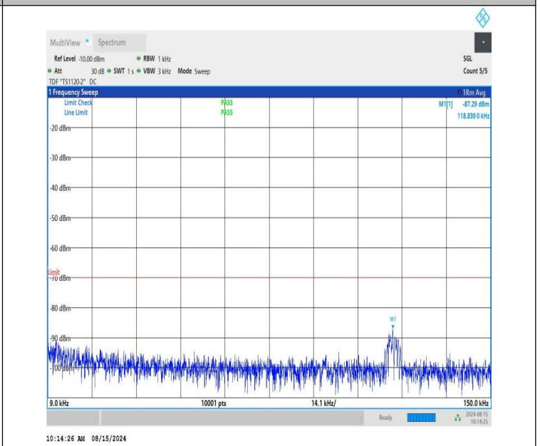
NTNV-n48-PC3-30-20-H-CP-QPSK-Edge_1RB_Right-0.009-0.15-P ASS
