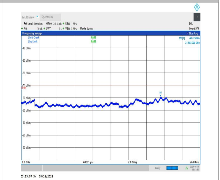
NTNV-n48-PC3-30-40-H-CP-QPSK-Edge_1RB_Left-6000-26000-P ASS
