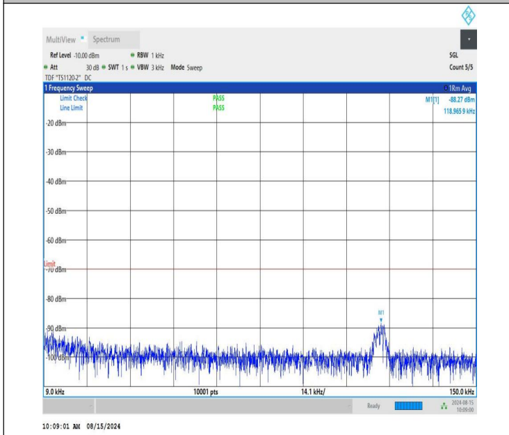
NTNV-n48-PC3-30-15-L-CP-QPSK-Edge_1RB_Left-0.009-0.15-P ASS
