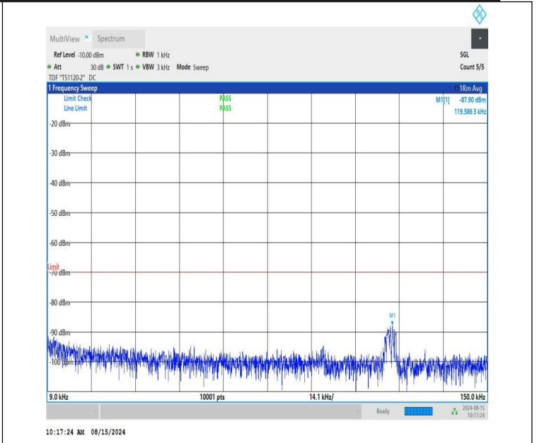
NTNV-n48-PC3-30-40-H-CP-QPSK-Edge_1RB_Right-0.009-0.15-P ASS
