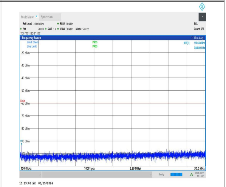
NTNV-n48-PC3-30-20-M-CP-QPSK-Edge_1RB_Left-0.15-30-PASS
