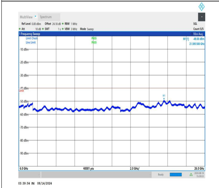
NTNV-n48-PC3-30-15-L-CP-QPSK-Edge_1RB_Right-6000-26000-PASS
