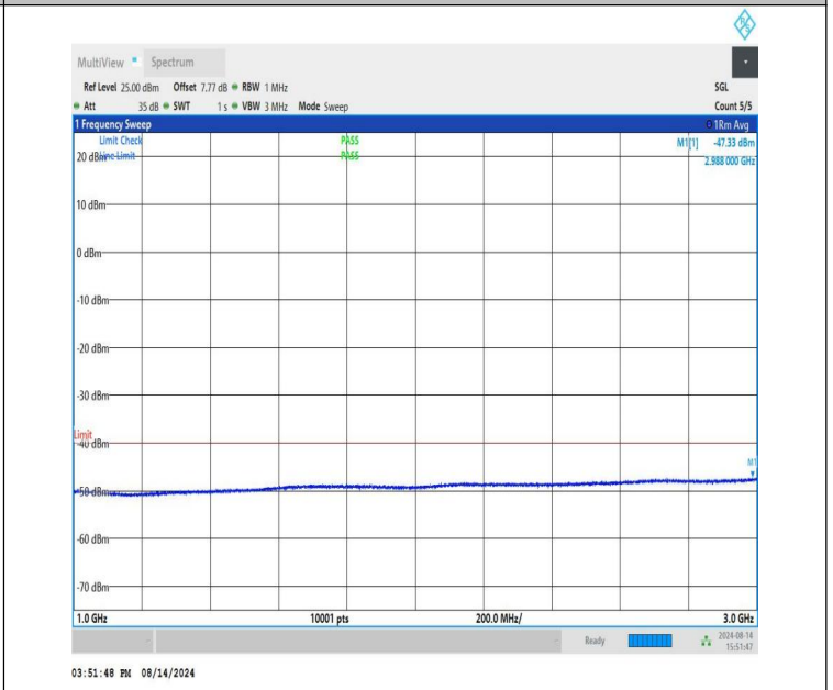
NTNV-n48-PC3-30-40-M-CP-QPSK-Edge_1RB_Left-1000-3000-PASS
