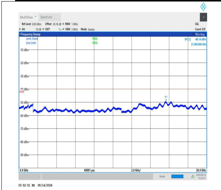
NTNV-n48-PC3-30-40-M-CP-QPSK-Edge_1RB_Right-6000-2600 0-PASS
