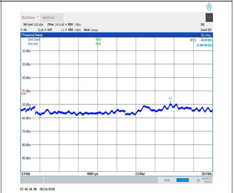
NTNV-n48-PC3-30-20-M-CP-QPSK-Edge_1RB_Left-6000-26000-P ASS
