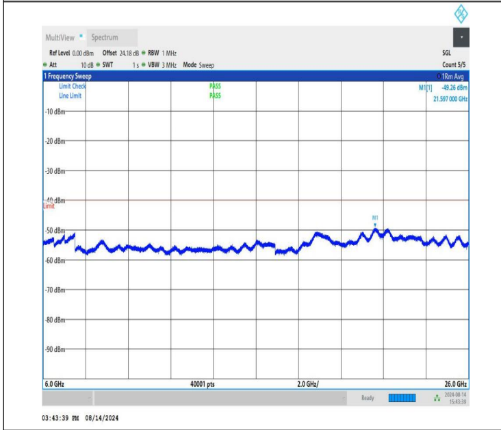
NTNV-n48-PC3-30-15-H-CP-QPSK-Edge_1RB_Right-6000-26000-PASS
