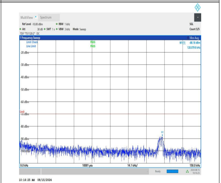
NTNV-n48-PC3-30-40-M-CP-QPSK-Edge_1RB_Right-0.009-0.15-P ASS
