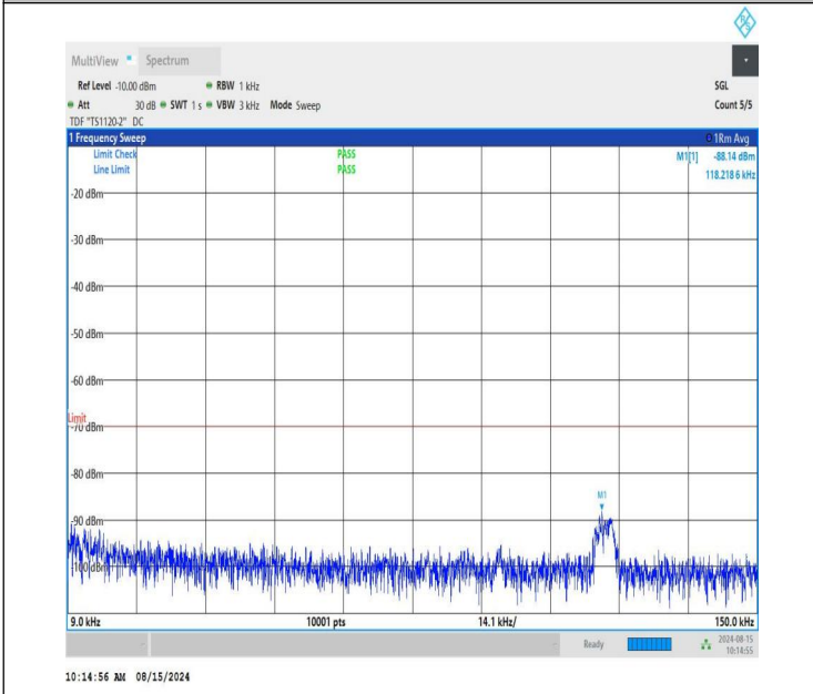
NTVN-n48-PC3-30-40-L-CP-QPSK-Edge_1RB_Left-0.009-0.15-P ASS
