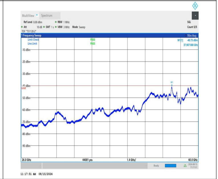
NTNV-n48-PC3-30-15-H-CP-QPSK-Edge_1RB_Right-26000-40000-PASS
