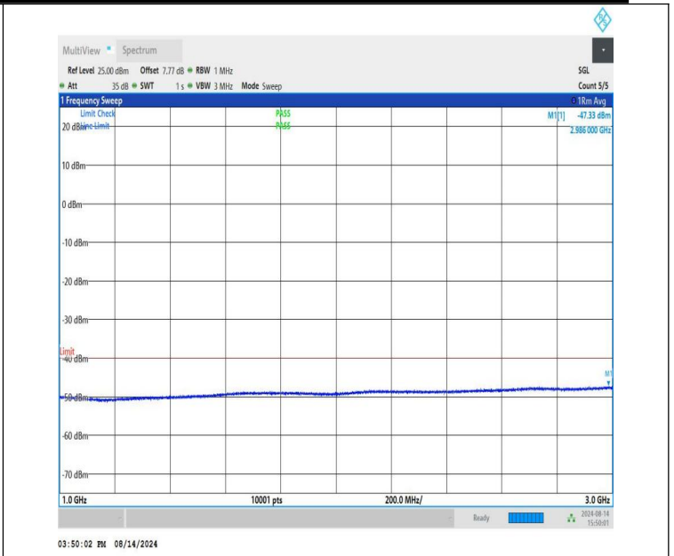
NTNV-n48-PC3-30-40-L-CP-QPSK-Edge_1RB_Left-1000-3000-PA SS
