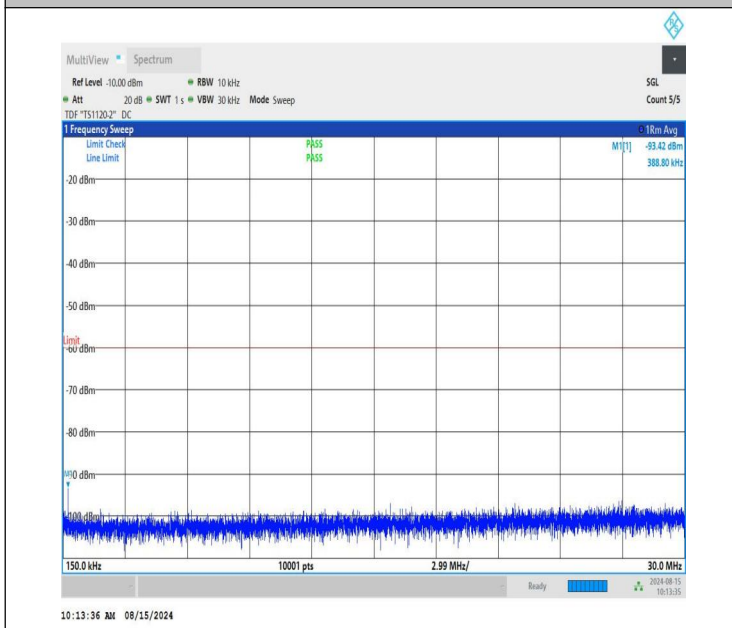
NTNV-n48-PC3-30-20-M-CP-QPSK-Edge_1RB_Right-0.15-30-PA SS
