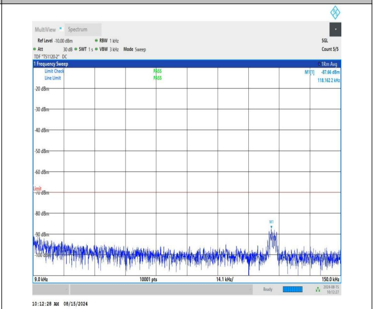
NTNV-n48-PC3-30-20-L-CP-QPSK-Edge_1RB_Right-0.009-0.15-P ASS
