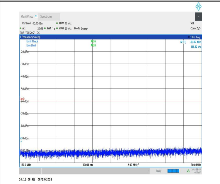
NTNV-n48-PC3-30-15-H-CP-QPSK-Edge_1RB_Left-0.15-30-PASS
