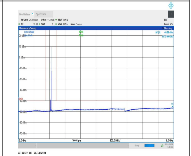
NTNV-n48-PC3-30-15-M-CP-QPSK-Edge_1RB_Right-3000-6000-P ASS
