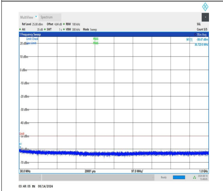
NTNV-n48-PC3-30-20-H-CP-QPSK-Edge_1RB_Left-30-1000-PAS S
