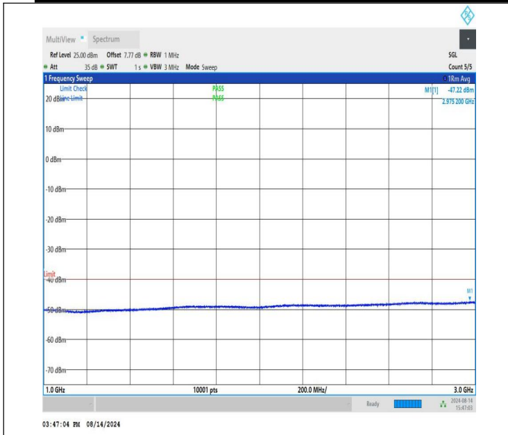
NTNV-n48-PC3-30-20-M-CP-QPSK-Edge_1RB_Right-1000-3000-PASS
