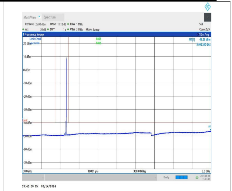
NTNV-n48-PC3-30-15-H-CP-QPSK-Edge_1RB_Right-3000-6000-PASS
