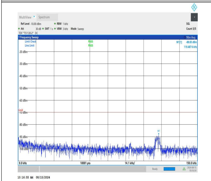
NTNV-n48-PC3-30-40-H-CP-QPSK-Edge_1RB_Left-0.009-0.15-P ASS
