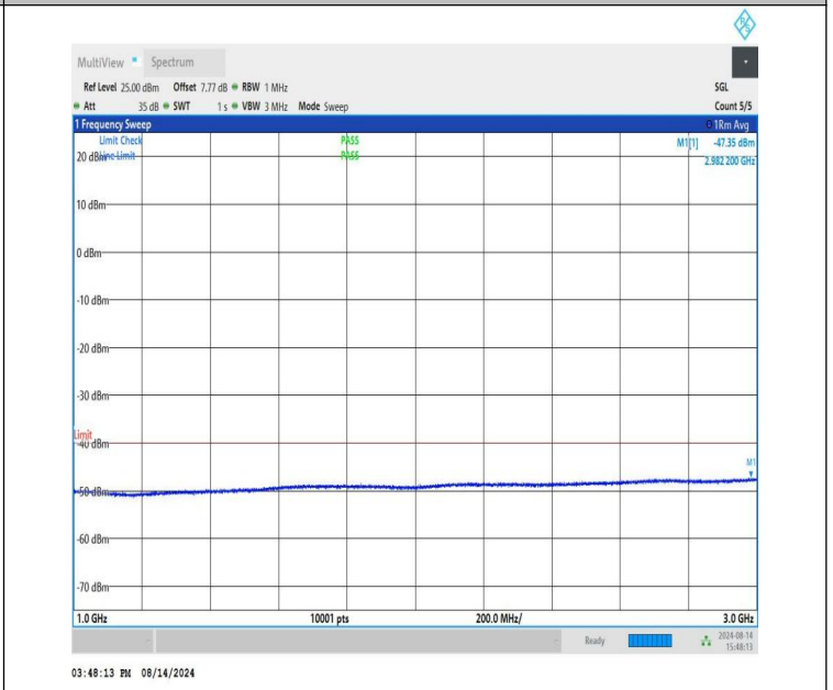
NTNV-n48-PC3-30-20-H-CP-QPSK-Edge_1RB_Left-1000-3000-PASS
