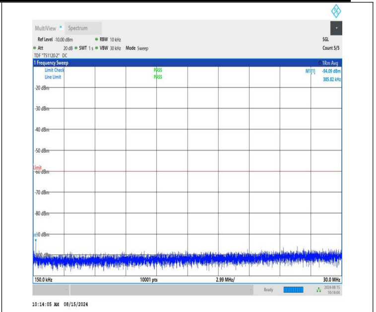
NTNV-n48-PC3-30-20-H-CP-QPSK-Edge_1RB_Left-0.15-30-PASS
