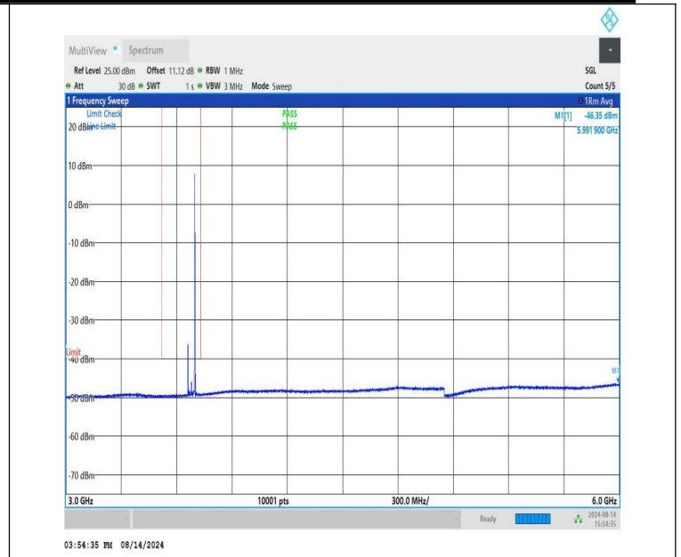
NTNV-n48-PC3-30-40-H-CP-QPSK-Edge_1RB_Right-3000-6000-PASS
