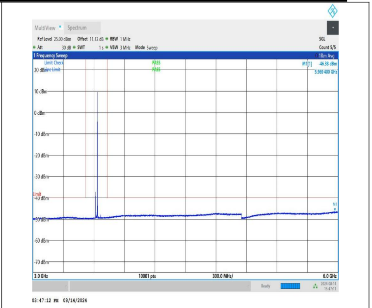
NTNV-n48-PC3-30-20-M-CP-QPSK-Edge_1RB_Right-3000-6000-PASS
