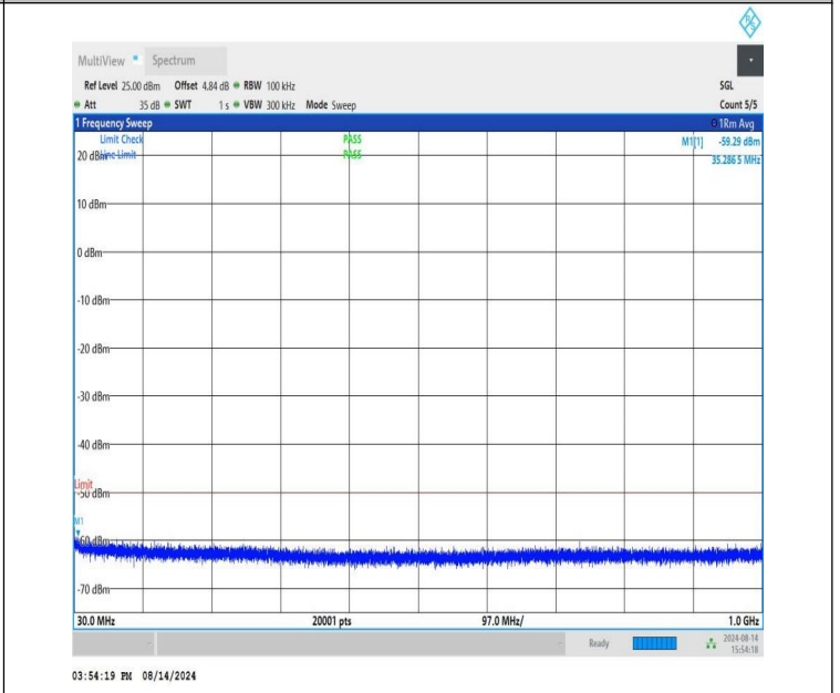
NTNV-n48-PC3-30-40-H-CP-QPSK-Edge_1RB_Right-30-1000-PA SS
