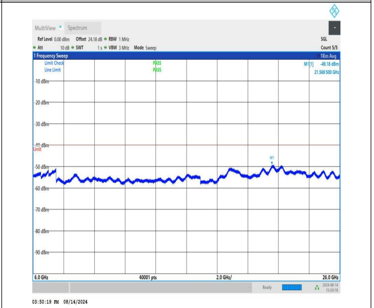
NTNV-n48-PC3-30-40-L-CP-QPSK-Edge_1RB_Left-6000-26000-P ASS
