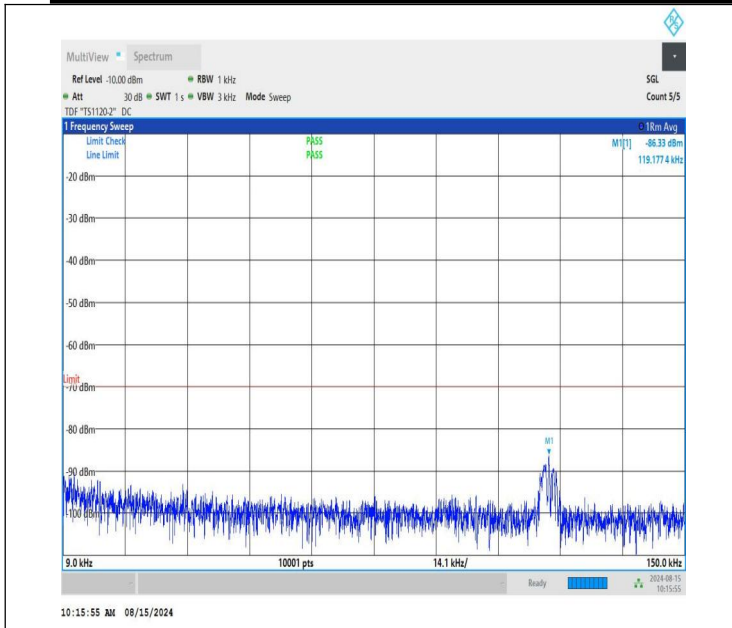
NTNV-n48-PC3-30-40-M-CP-QPSK-Edge_1RB_Left-0.009-0.15-P ASS
