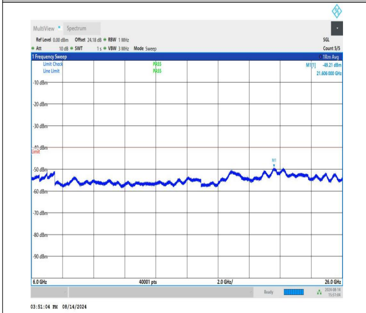
NTNV-n48-PC3-30-40-L-CP-QPSK-Edge_1RB_Right-6000-26000-PASS
