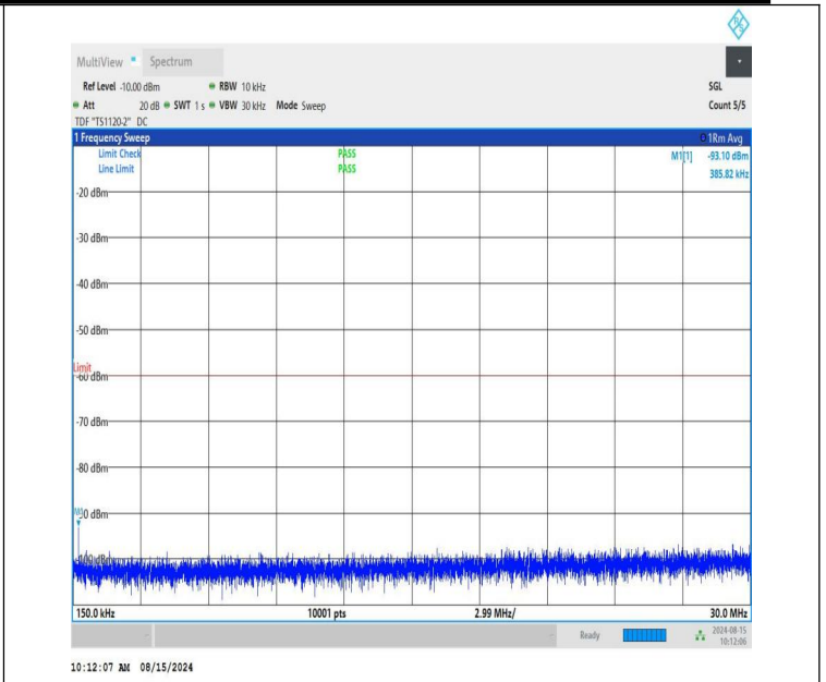
NTNV-n48-PC3-30-20-L-CP-QPSK-Edge_1RB_Left-0.15-30-PASS
