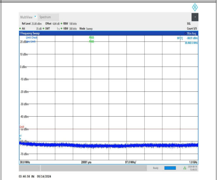
NTNV-n48-PC3-30-20-M-CP-QPSK-Edge_1RB_Right-30-1000-PA SS
