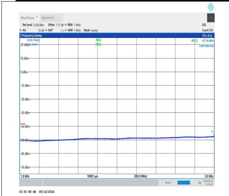
NTNV-n48-PC3-30-40-L-CP-QPSK-Edge_1RB_Right-1000-3000-PASS
