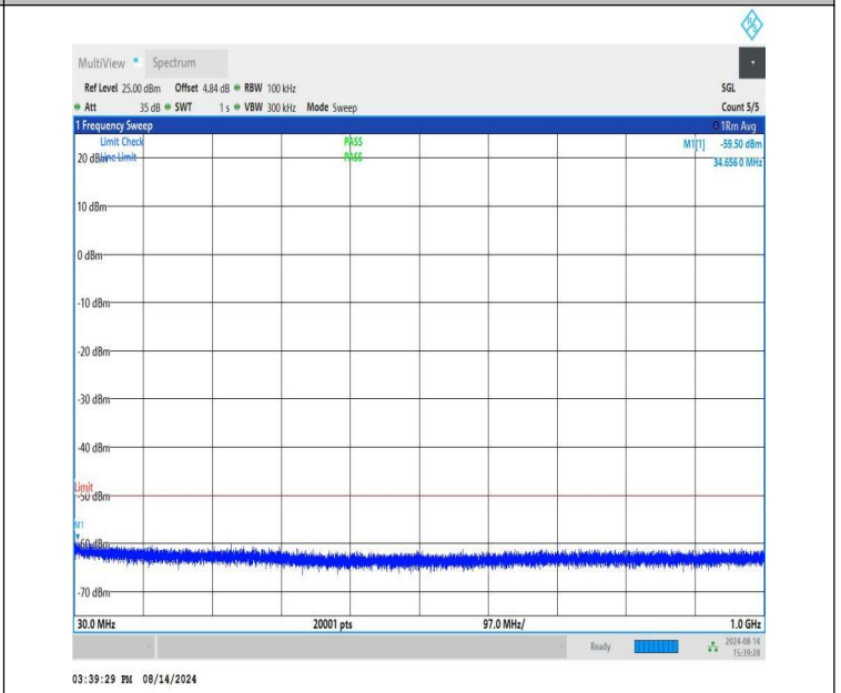
NTNV-n48-PC3-30-15-L-CP-QPSK-Edge_1RB_Right-30-1000-PAS S
