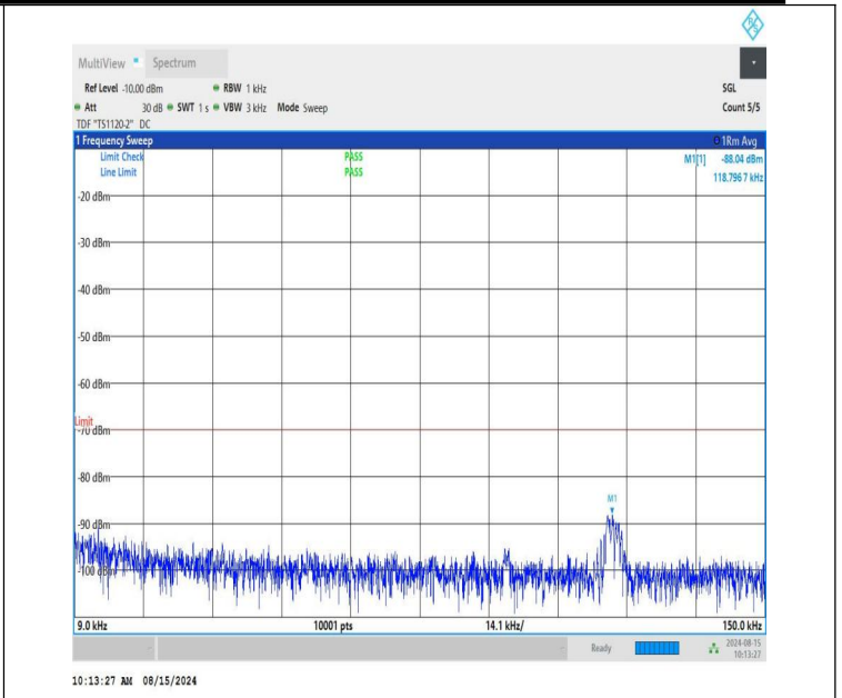
NTNV-n48-PC3-30-20-M-CP-QPSK-Edge_1RB_Right-0.009-0.15-P ASS
