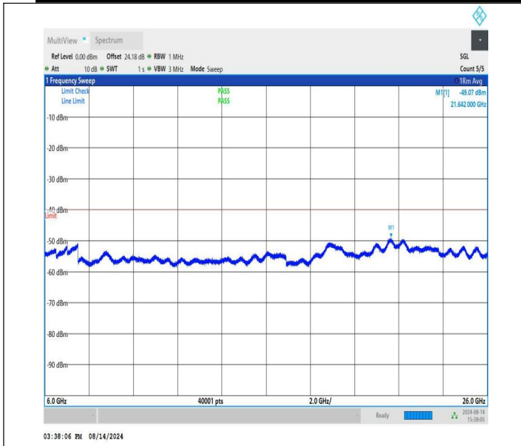
NTNV-n48-PC3-30-10-H-CP-QPSK-Edge_1RB_Right-6000-26000 -PASS
