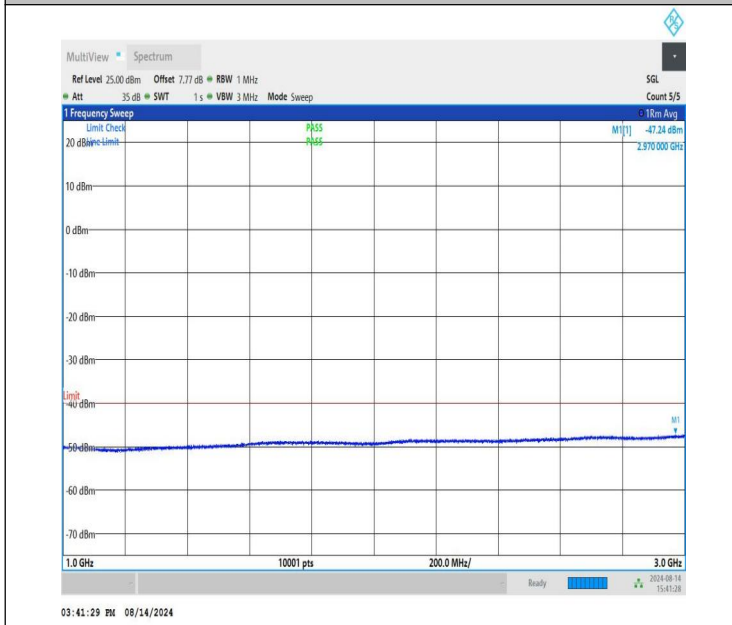
NTNV-n48-PC3-30-15-M-CP-QPSK-Edge_1RB_Right-1000-3000- PASS
