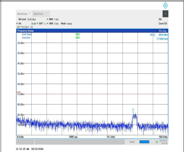
NTNV-n48-PC3-30-15-M-CP-QPSK-Edge_1RB_Right-0.009-0.15-P ASS
