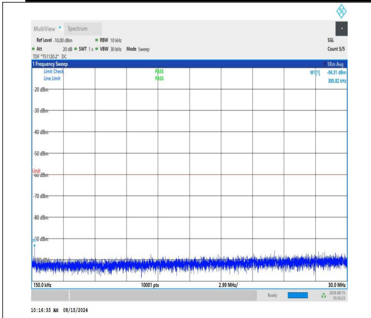
NTNV-n48-PC3-30-40-M-CP-QPSK-Edge_1RB_Right-0.15-30-PA SS
