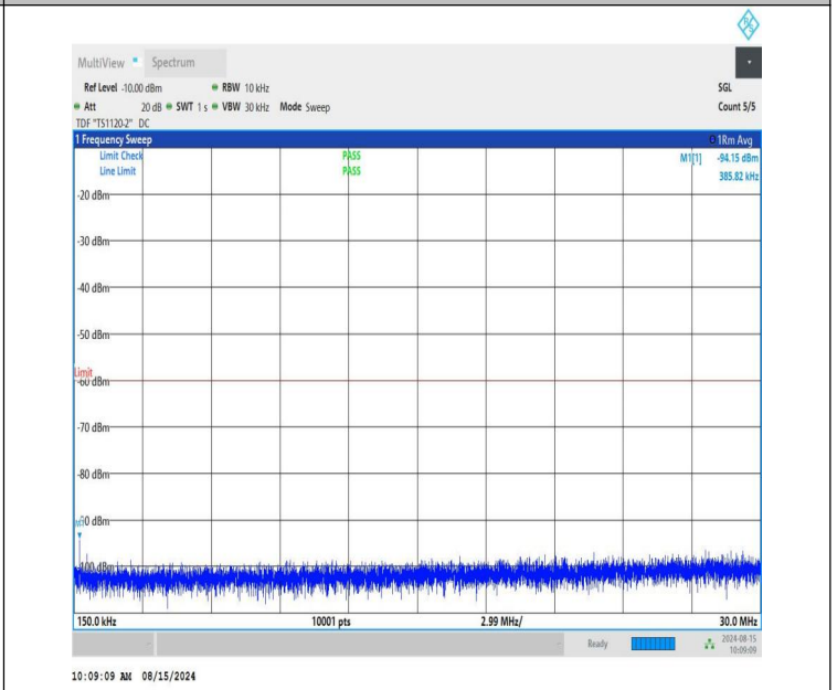
NTNV-n48-PC3-30-15-L-CP-QPSK-Edge_1RB_Left-0.15-30-PASS
