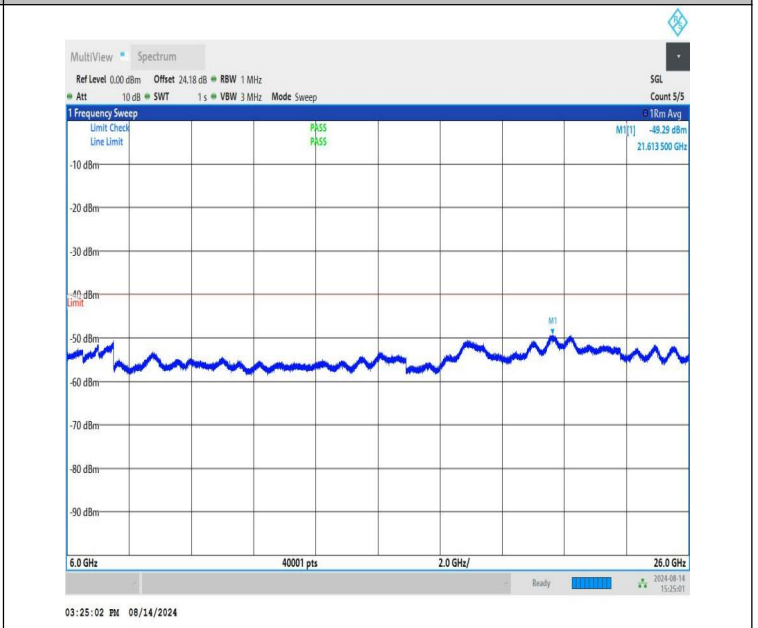
NTNV-n48-PC3-30-20-M-CP-QPSK-Edge_1RB_Left-6000-26000-P ASS
