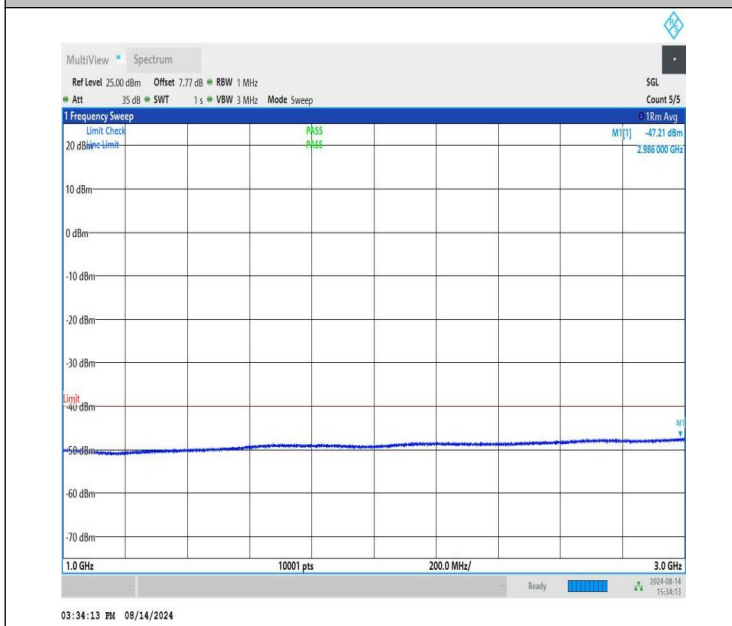
NTNV-n48-PC3-30-10-L-CP-QPSK-Edge_1RB_Right-1000-3000- PASS
