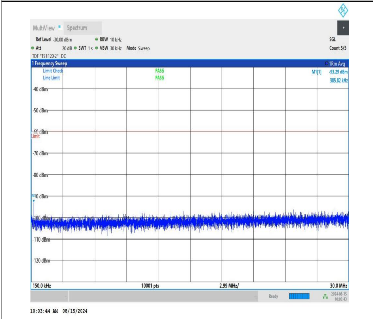
NTNV-n48-PC3-30-40-L-CP-QPSK-Edge_1RB_Right-0.15-30-PA SS
