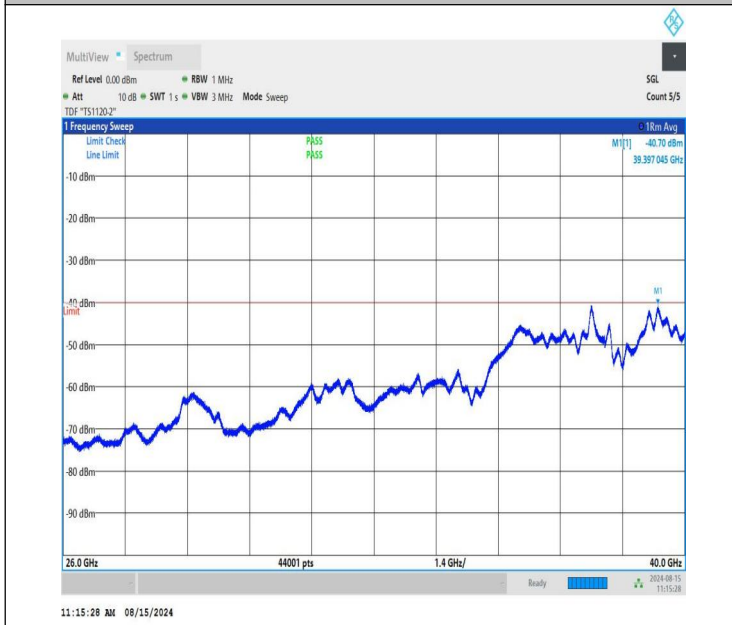
NTNV-n48-PC3-30-10-L-CP-QPSK-Edge_1RB_Left-26000-40000 -PASS
