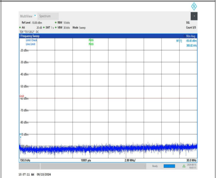
NTNV-n48-PC3-30-10-M-CP-QPSK-Edge_1RB_Left-0.15-30-PASS
