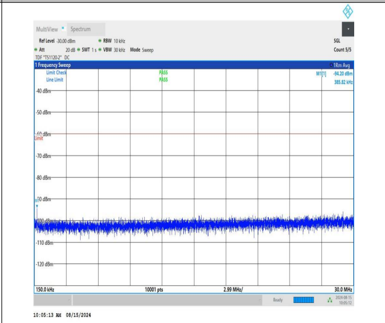
NTNV-n48-PC3-30-40-H-CP-QPSK-Edge_1RB_Left-0.15-30-PASS
