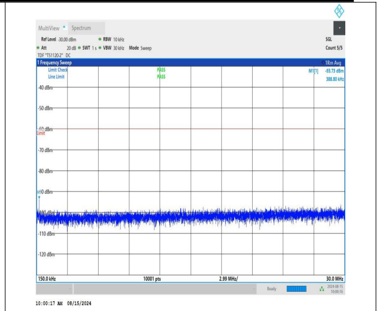
NTNV-n48-PC3-30-20-L-CP-QPSK-Edge_1RB_Left-0.15-30-PASS
