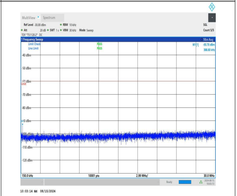
NTNV-n48-PC3-30-40-L-CP-QPSK-Edge_1RB_Left-0.15-30-PASS
