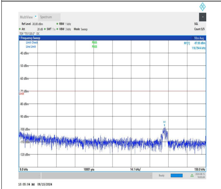
NTNV-n48-PC3-30-40-H-CP-QPSK-Edge_1RB_Left-0.009-0.15-P ASS
