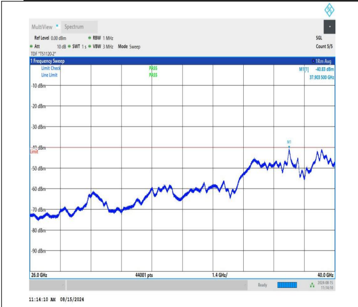
NTNV-n48-PC3-30-40-L-CP-QPSK-Edge_1RB_Left-26000-40000 -PASS
