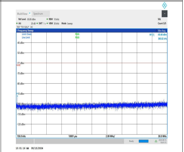
NTNV-n48-PC3-30-20-M-CP-QPSK-Edge_1RB_Left-0.15-30-PASS
