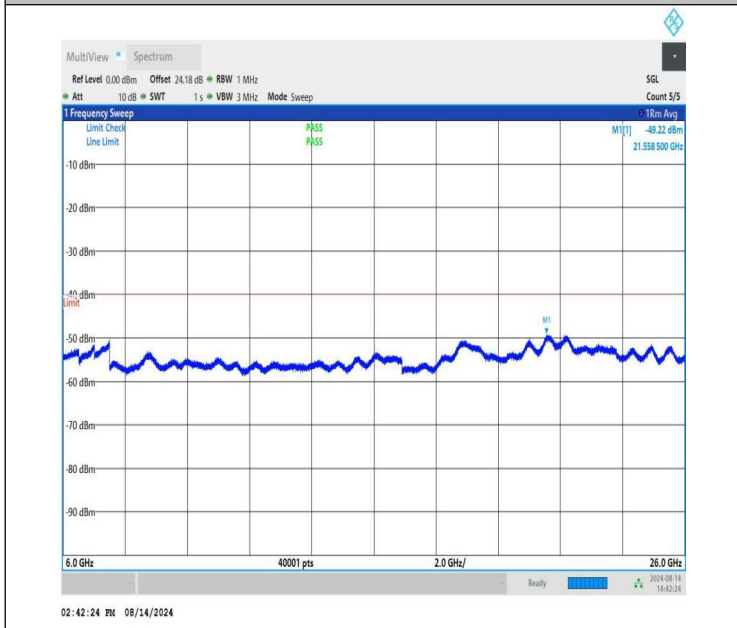
NTV-n48-PC3-30-15-H-CP-QPSK-Edge_1RB_Right-6000-26000 -PASS
