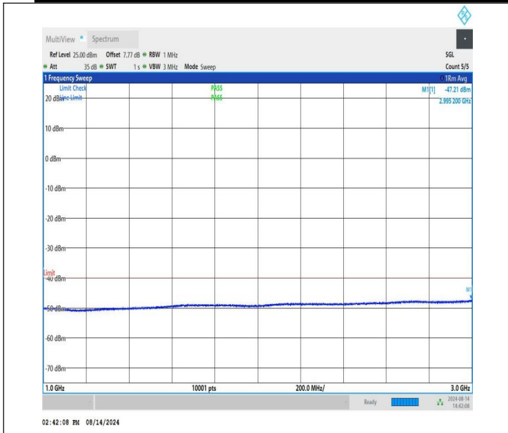
FNTNV-n48-PC3-30-15-H-CP-QPSK-Edge_1RB_Right-1000-300 0-PASS
