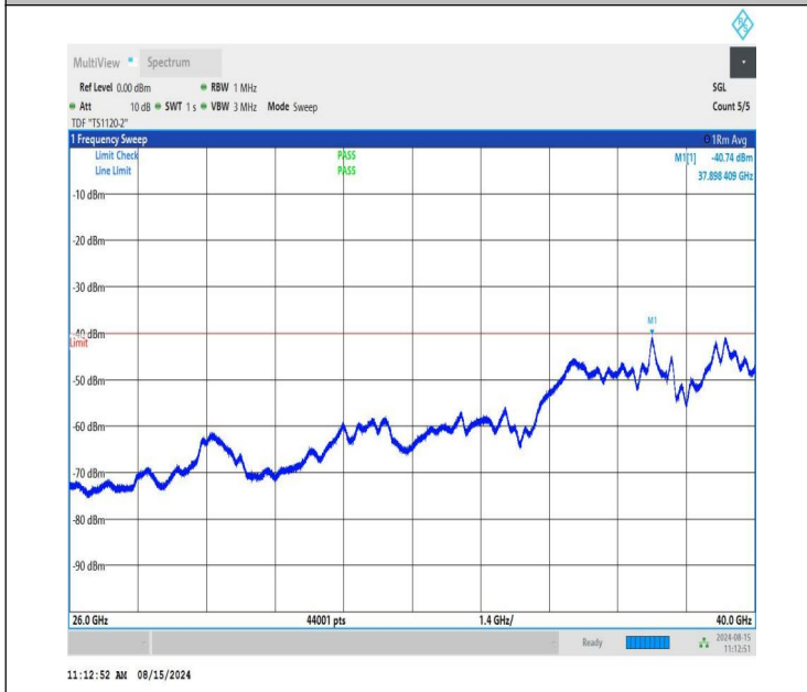
NTNV-n48-PC3-30-20-L-CP-QPSK-Edge_1RB_Left-26000-40000 -PASS
