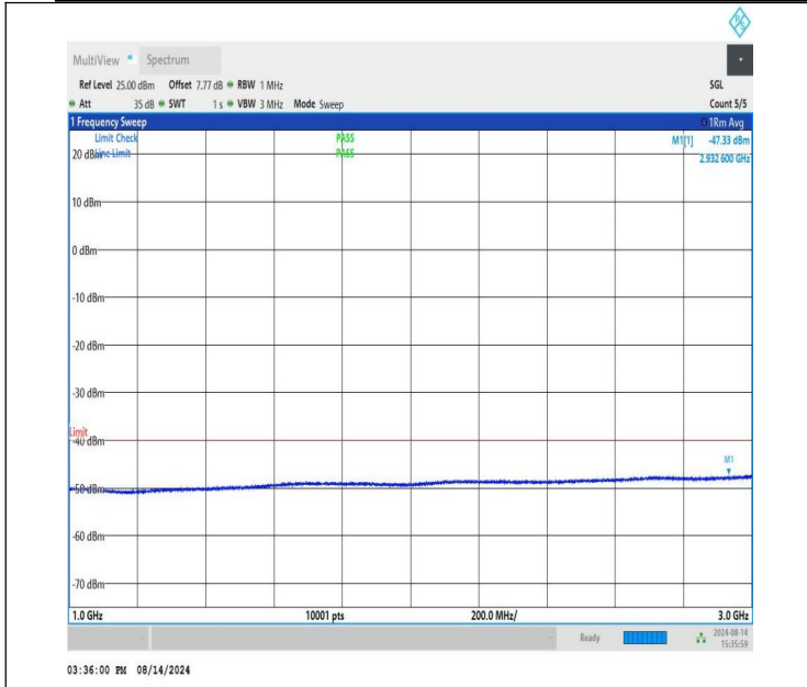
NTNV-n48-PC3-30-10-M-CP-QPSK-Edge_1RB_Right-1000-3000-PASS
