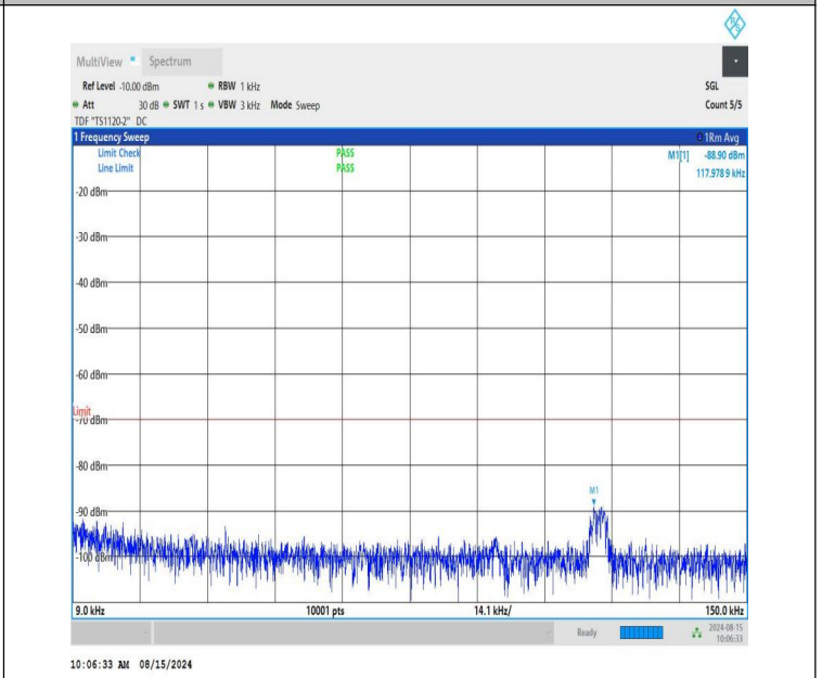
NTNV-n48-PC3-30-10-L-CP-QPSK-Edge_1RB_Right-0.009-0.15-P ASS
