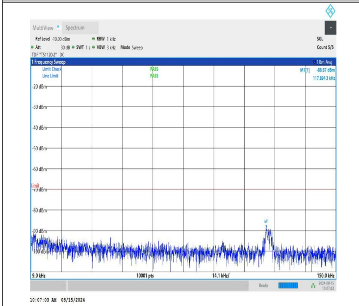
NTNV-n48-PC3-30-10-M-CP-QPSK-Edge_1RB_Left-0.009-0.15-P ASS
