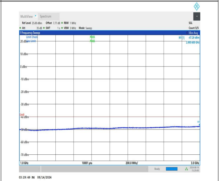
NTNV-n48-PC3-30-40-M-CP-QPSK-Edge_1RB_Left-1000-3000-PASS
