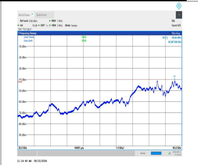
NTNV-n48-PC3-30-40-M-CP-QPSK-Edge_1RB_Right-26000-4000 0-PASS
