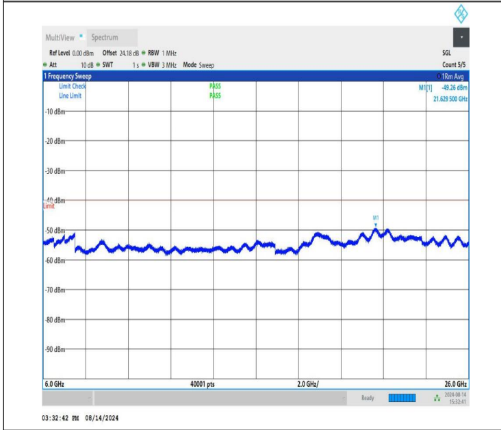
NTNV-n48-PC3-30-40-H-CP-QPSK-Edge_1RB_Right-6000-26000-PASS
