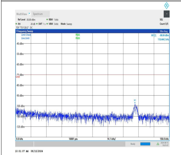
NTNV-n48-PC3-30-20-M-CP-QPSK-Edge_1RB_Left-0.009-0.15-P ASS
