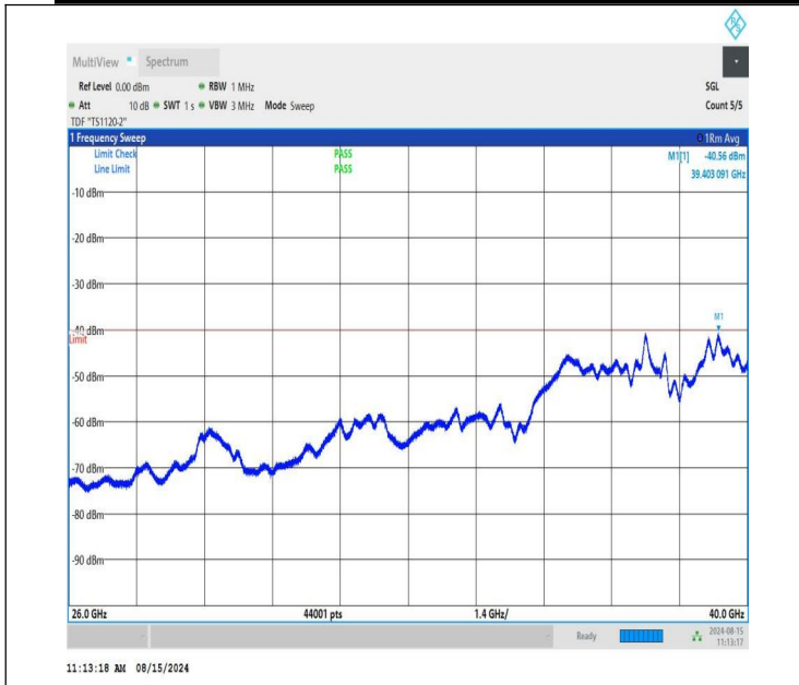
NTNV-n48-PC3-30-20-M-CP-QPSK-Edge_1RB_Left-26000-40000 -PASS
