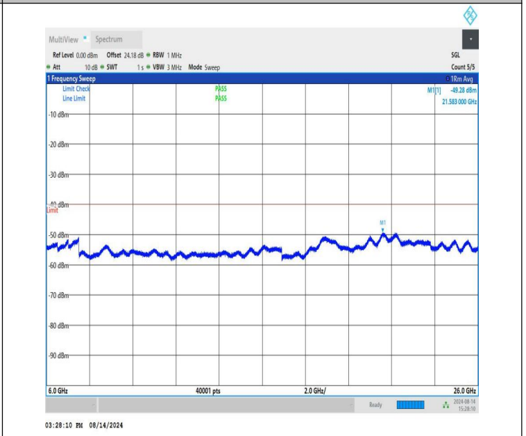
NTNV-n48-PC3-30-40-L-CP-QPSK-Edge_1RB_Left-6000-26000-P ASS
