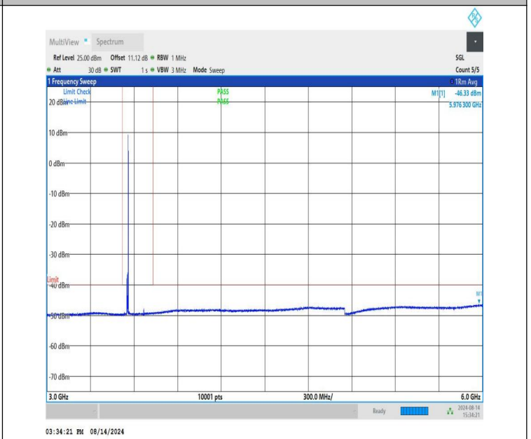
NTNV-n48-PC3-30-10-L-CP-QPSK-Edge_1RB_Right-3000-6000-P ASS
