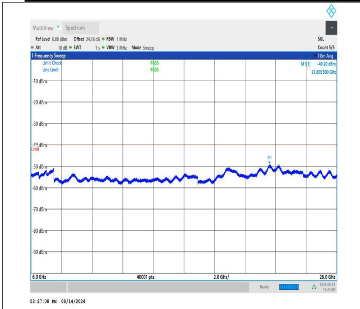
NTNV-n48-PC3-30-20-H-CP-QPSK-Edge_1RB_Right-6000-26000 -PASS
