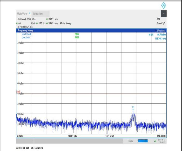
NTNV-n48-PC3-30-10-H-CP-QPSK-Edge_1RB_Right-0.009-0.15-P ASS
