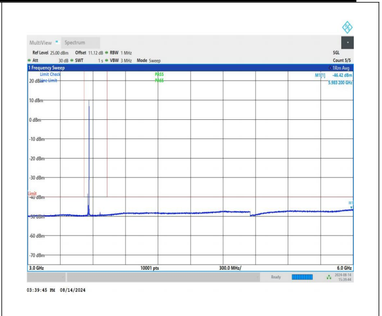
NTV-n48-PC3-30-15-H-CP-QPSK-Edge_1RB_Right-3000-6000-PASS
