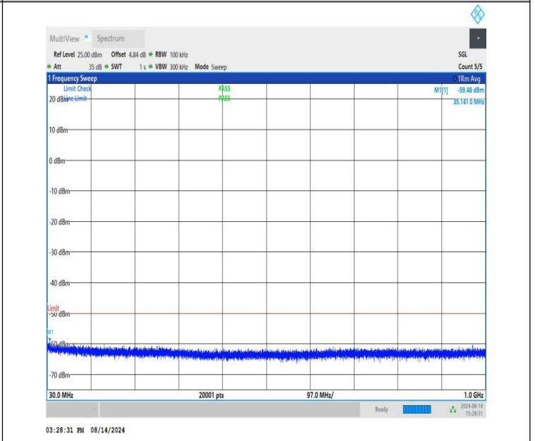
NTNV-n48-PC3-30-40-L-CP-QPSK-Edge_1RB_Right-30-1000-PAS S
