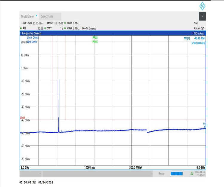
NTNV-n48-PC3-30-10-M-CP-QPSK-Edge_1RB_Right-3000-6000-PASS
