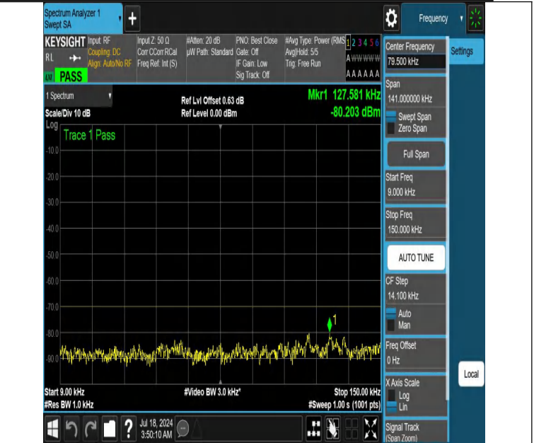
NTNV-DC_13A_n48A-PC3-30-5+20-M+M-N/A-N/A-DFT-QPSK-Edge_1RB_Right-0.009-0.15-PASS
