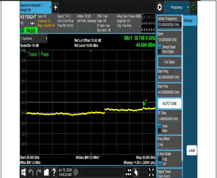
NTNV-DC_13A_n48A-PC3-30-5+20-M+M-N/A-N/A-DFT-PI2BPSK-E dge_1RB_Right-26000-40000-PASS
