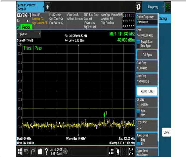
NTNV-DC_13A_n48A-PC3-30-5+20-M+H-N/A-N/A-DFT-QPSK-Edge_1RB_Left-0.009-0.15-PASS
