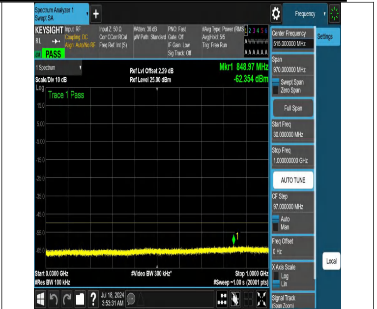
NTNV-DC_13A_n48A-PC3-30-5+20-M+H-N/A-N/A-DFT-PI2BPSK-E_dge_1RB_Right-30-1000-PASS
