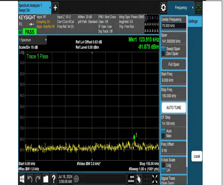
NTNV-DC_13A_n48A-PC3-30-5+20-M+H-N/A-N/A-DFT-QPSK-Edge e_1RB_Right-0.009-0.15-PASS
