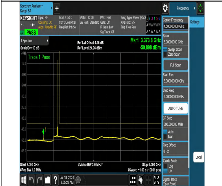
NTNV-DC_13A_n48A-PC3-30-5+20-M+H-N/A-N/A-DFT-QPSK-Edge e_1RB_Left-3000-6000-PASS
