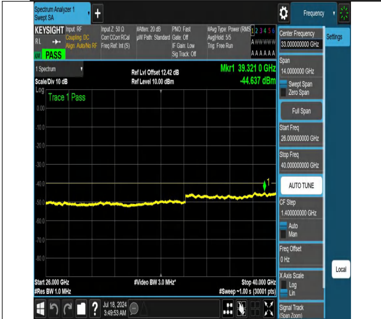
NTNV-DC_13A_n48A-PC3-30-5+20-M+M-N/A-N/A-DFT-QPSK-Edge_1RB_Left-26000-40000-PASS
