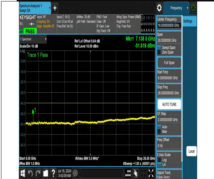
NTNV-DC_13A_n48A-PC3-30-5+20-M+L-N/A-N/A-DFT-PI2BPSK-Edge_1RB_Right-6000-26000-PASS
