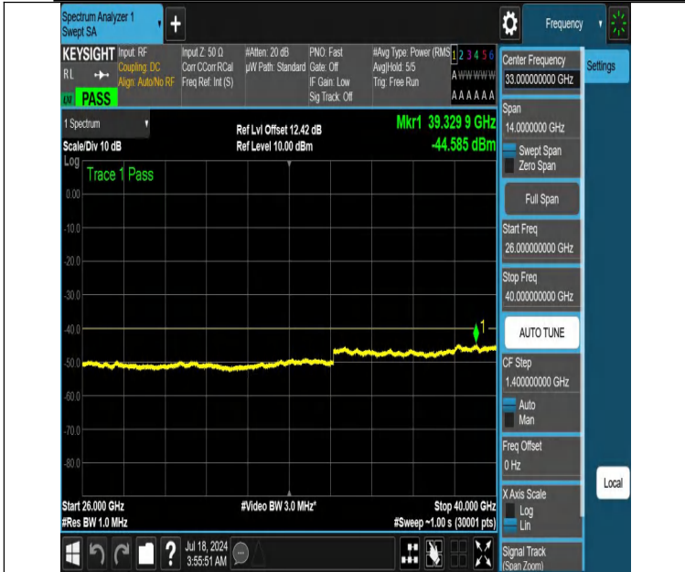
NTNV-DC_13A_n48A-PC3-30-5+20-M+H-N/A-N/A-DFT-QPSK-Edge e_1RB_Left-26000-40000-PASS
