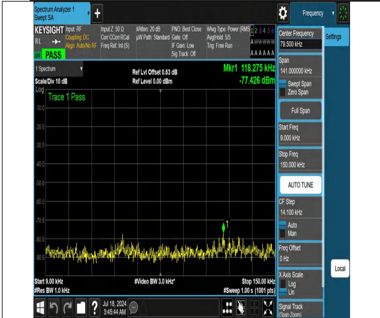
NTNV-DC_13A_n48A-PC3-30-5+20-M+M-N/A-N/A-DFT-PI2BPSK-Edge_1RB_Left-0.009-0.15-PASS
