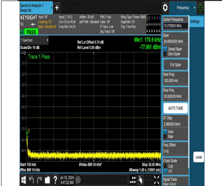
NTVN-DC_13A_n48A-PC3-30-5+20-M+M-N/A-N/A-DFT-PI2BPSK-Edge_1RB_Right-0.15-30-PASS
