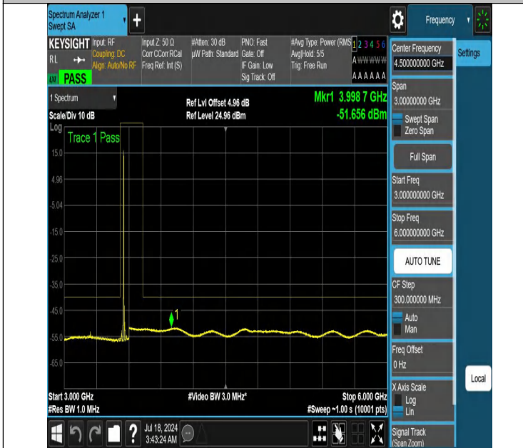
NTNV-DC_13A_n48A-PC3-30-5+20-M+L-N/A-N/A-DFT-QPSK-Edge e_1RB_Left-3000-6000-PASS
