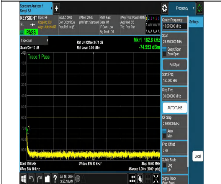
NTNV-DC_13A_n48A-PC3-30-5+20-M+H-N/A-N/A-DFT-QPSK-Edge e_1RB_Right-0.15-30-PASS
