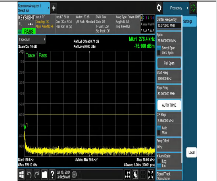
NTNV-DC_13A_n48A-PC3-30-5+20-M+H-N/A-N/A-DFT-QPSK-Edge_1RB_Left-0.15-30-PASS
