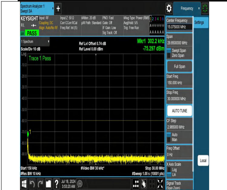
NTNV-DC_13A_n48A-PC3-30-5+20-M+H-N/A-N/A-DFT-PI2BPSK-Edge_1RB_Right-0.15-30-PASS
