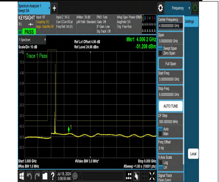
NTNV-DC_13A_n48A-PC3-30-5+20-M+H-N/A-N/A-DFT-QPSK-Edge_1RB_Right-3000-6000-PASS
