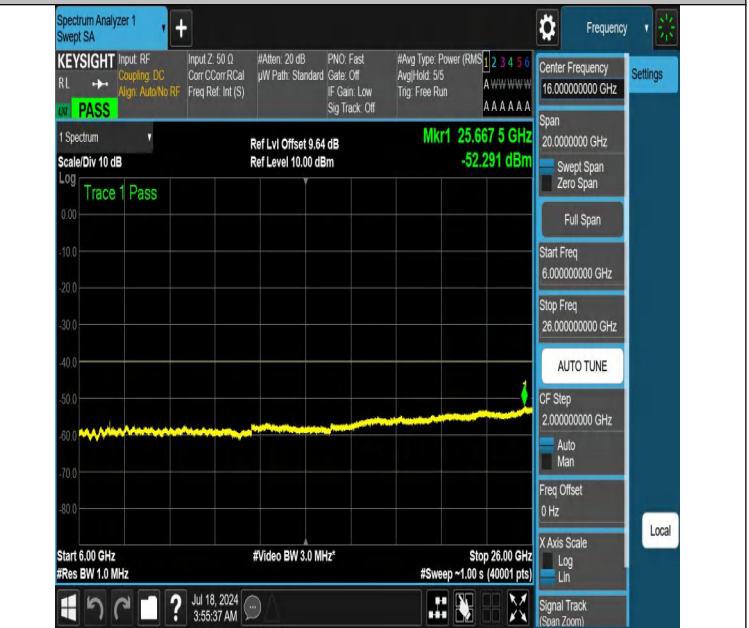
NTNV-DC_13A_n48A-PC3-30-5+20-M+H-N/A-N/A-DFT-QPSK-Edge e_1RB_Left-6000-26000-PASS
