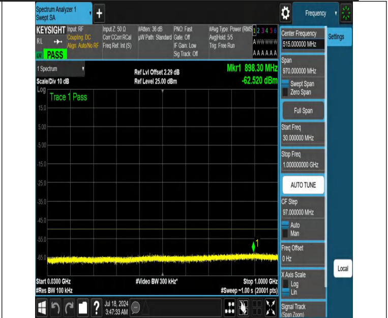
NTVN-DC_13A_n48A-PC3-30-5+20-M+M-N/A-N/A-DFT-PI2BPSK-E_dge_1RB_Right-30-1000-PASS
