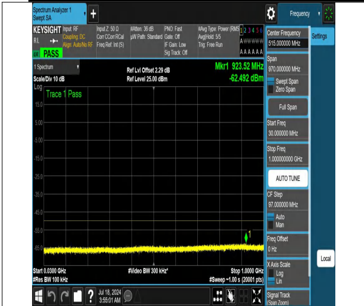
NTNV-DC_13A_n48A-PC3-30-5+20-M+H-N/A-N/A-DFT-QPSK-Edge e_1RB_Left-30-1000-PASS
