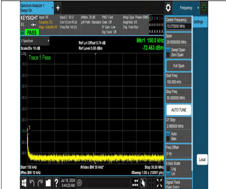
NTNV-DC_13A_n48A-PC3-30-5+20-M+L-N/A-N/A-DFT-QPSK-Edge e_1RB_Right-0.15-30-PASS
