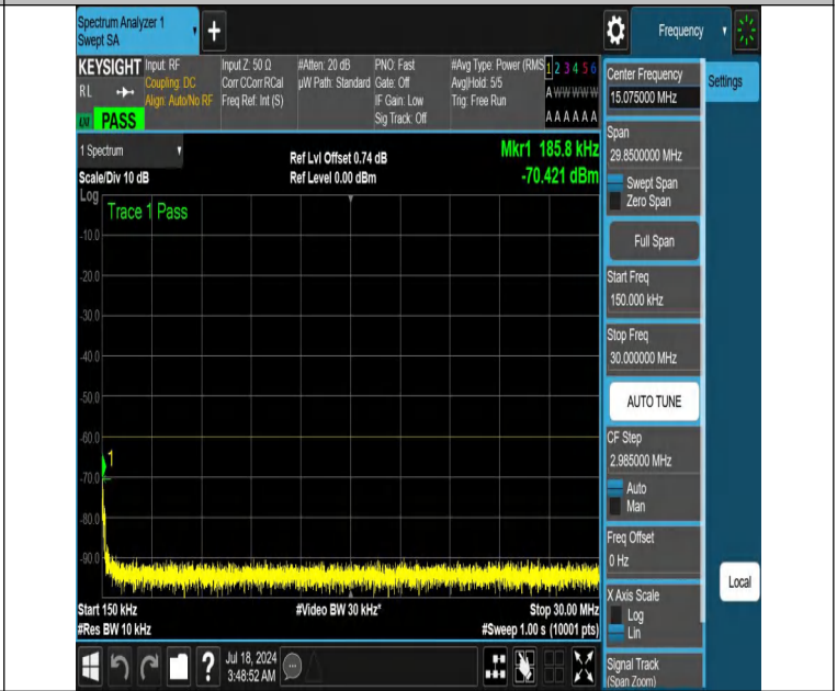
NTNV-DC_13A_n48A-PC3-30-5+20-M+M-N/A-N/A-DFT-QPSK-Edge_1RB_Left-0.15-30-PASS
