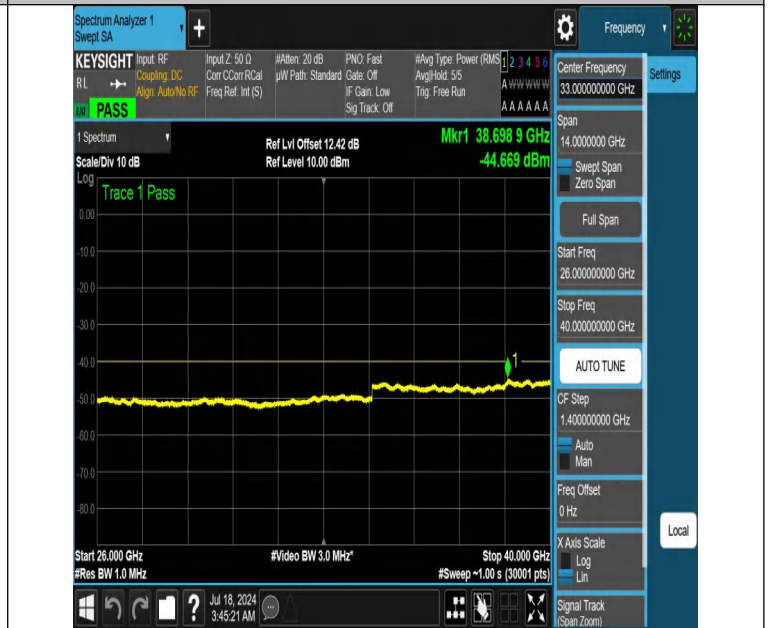
NTNV-DC_13A_n48A-PC3-30-5+20-M+L-N/A-N/A-DFT-QPSK-Edge _1RB_Right-26000-40000-PASS
