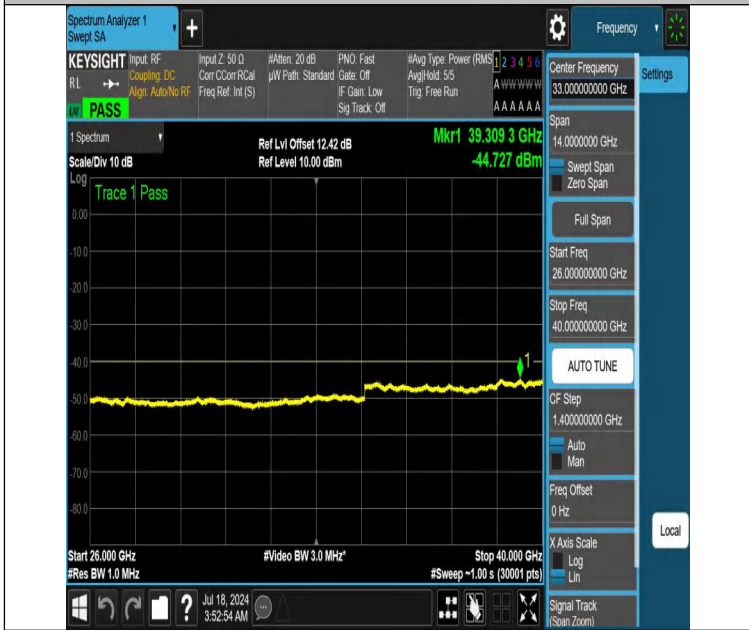
NTNV-DC_13A_n48A-PC3-30-5+20-M+H-N/A-N/A-DFT-PI2BPSK-Edge_1RB_Left-26000-40000-PASS
