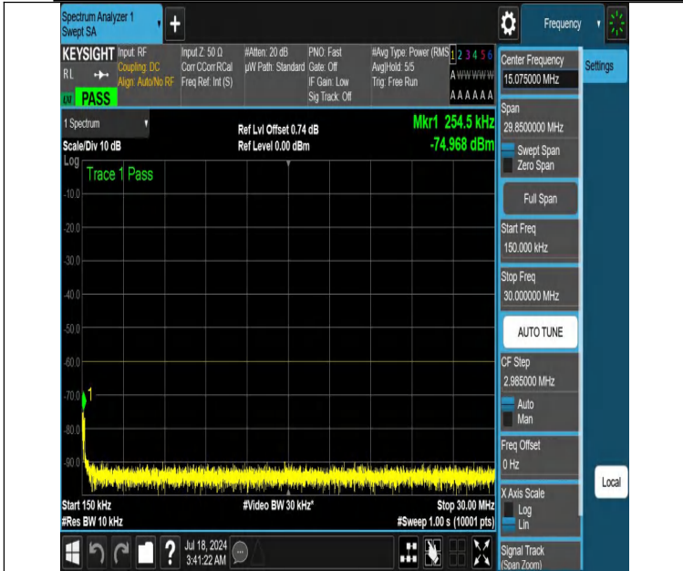
NTNV-DC_13A_n48A-PC3-30-5+20-M+L-N/A-N/A-DFT-PI2BPSK-Edge_1RB_Right-0.15-30-PASS
