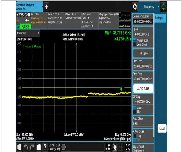
NTNV-DC_13A_n48A-PC3-30-5+20-M+L-N/A-N/A-DFT-PI2BPSK- Edge_1RB_Left-26000-40000-PASS
