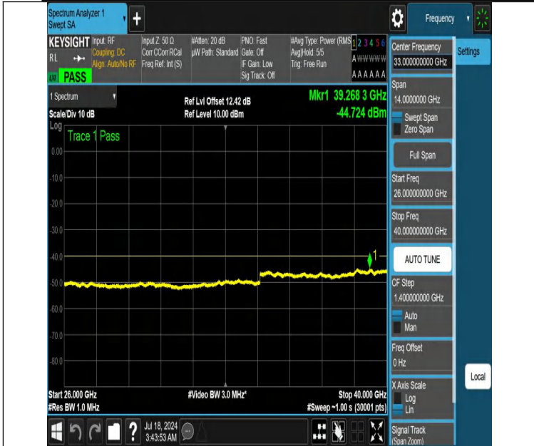
NTNV-DC_13A_n48A-PC3-30-5+20-M+L-N/A-N/A-DFT-QPSK-Edge e_1RB_Left-26000-40000-PASS
