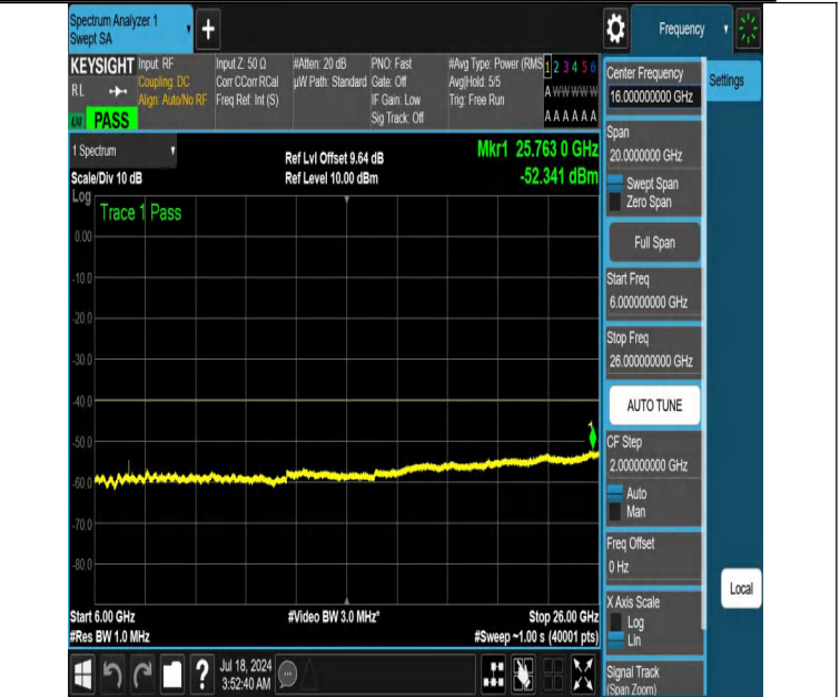
NTNV-DC_13A_n48A-PC3-30-5+20-M+H-N/A-N/A-DFT-PI2BPSK-E dge_1RB_Left-6000-26000-PASS
