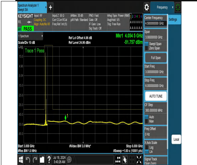
NTNV-DC_13A_n48A-PC3-30-5+20-M+L-N/A-N/A-DFT-PI2BPSK- Edge_1RB_Left-3000-6000-PASS
