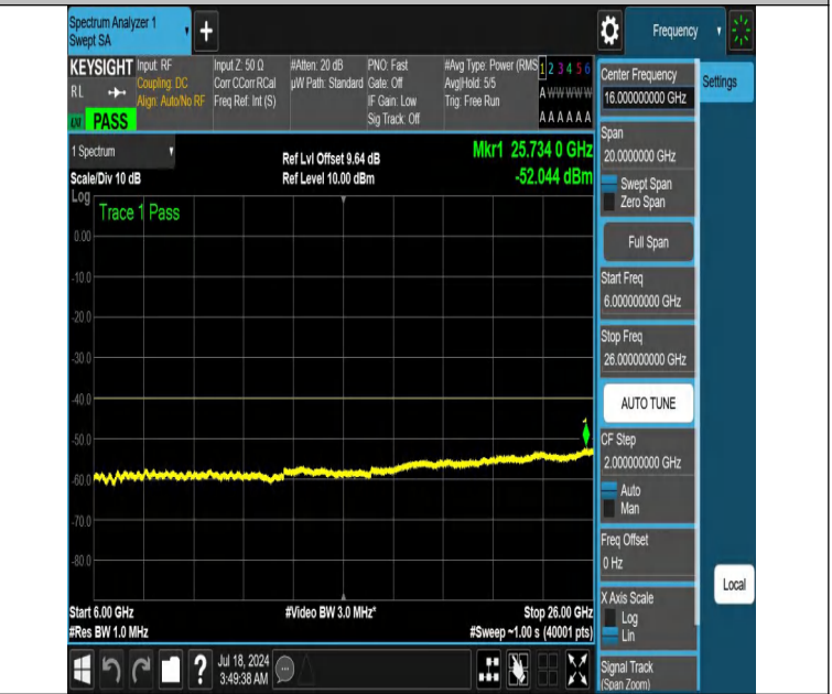
NTNV-DC_13A_n48A-PC3-30-5+20-M+M-N/A-N/A-DFT-QPSK-Edge_1RB_Left-6000-26000-PASS
