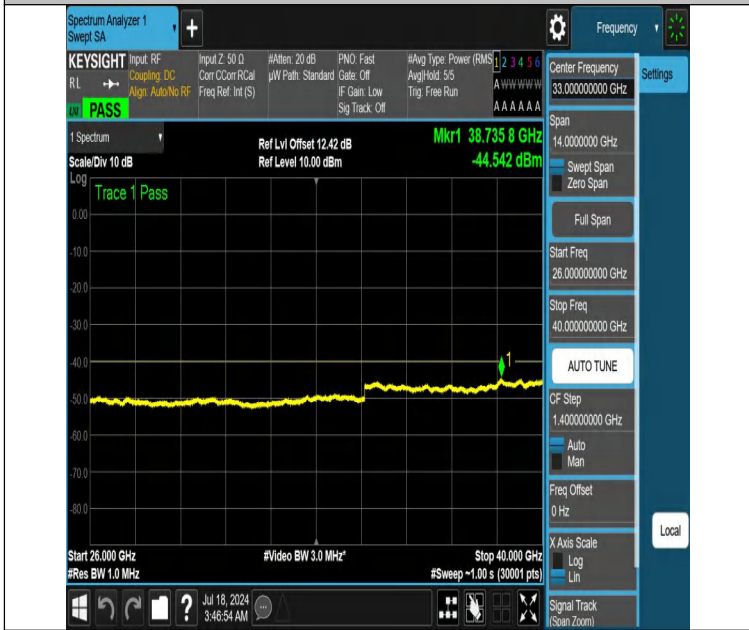
NTVN-DC_13A_n48A-PC3-30-5+20-M+M-N/A-N/A-DFT-PI2BPSK-Edge_1RB_Left-26000-40000-PASS
