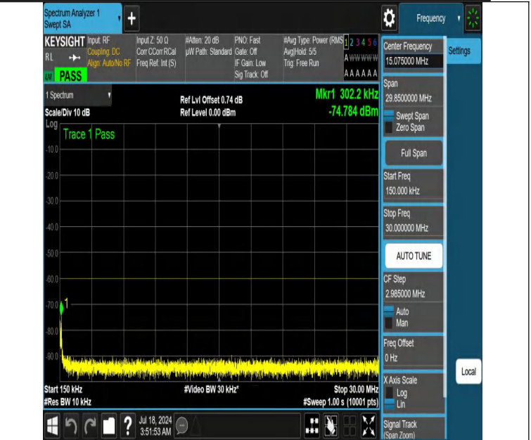
NTNV-DC_13A_n48A-PC3-30-5+20-M+H-N/A-N/A-DFT-PI2BPSK-E dge_1RB_Left-0.15-30-PASS
