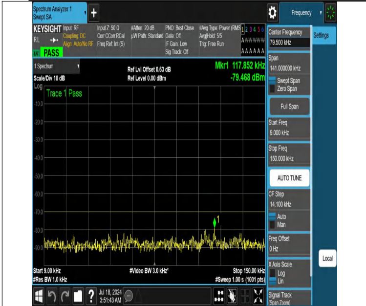
NTNV-DC_13A_n48A-PC3-30-5+20-M+H-N/A-N/A-DFT-PI2BPSK-Edge_1RB_Left-0.009-0.15-PASS
