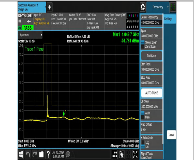
NTVN-DC_13A_n48A-PC3-30-5+20-M+M-N/A-N/A-DFT-PI2BPSK-E_dge_1RB_Right-3000-6000-PASS
