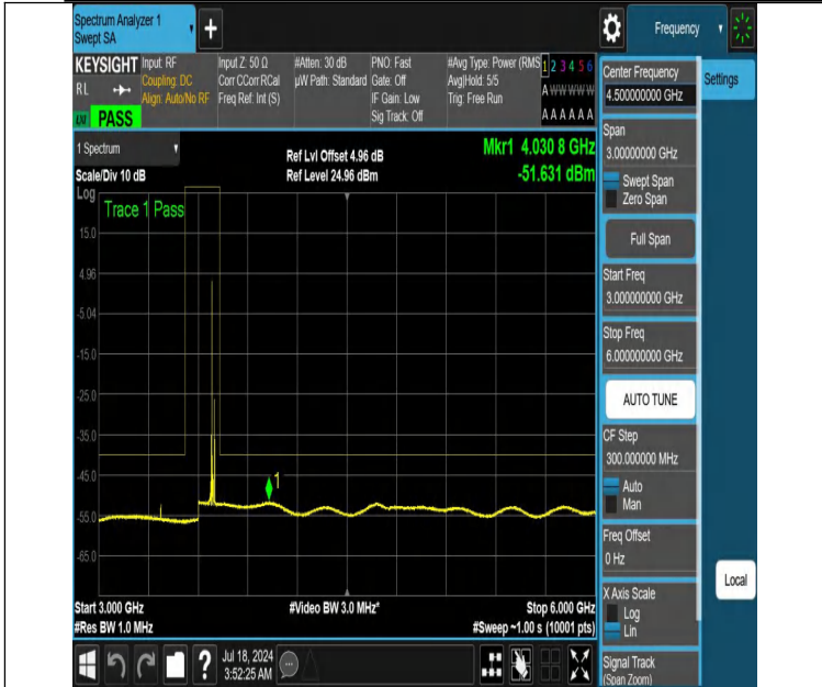
NTNV-DC_13A_n48A-PC3-30-5+20-M+H-N/A-N/A-DFT-PI2BPSK-Edge_1RB_Left-3000-6000-PASS
