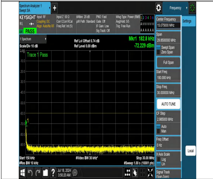
NTNV-DC_13A_n48A-PC3-30-5+20-M+M-N/A-N/A-DFT-QPSK-Edge_1RB_Right-0.15-30-PASS
