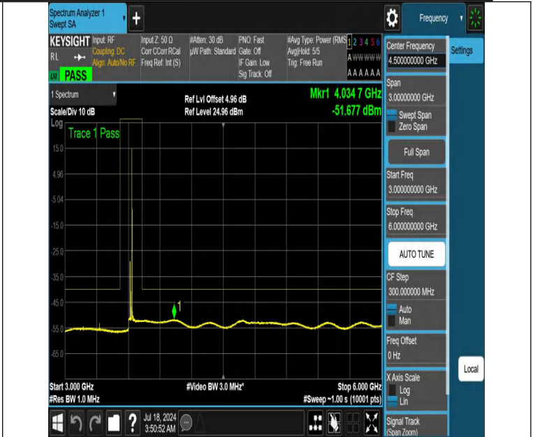
NTNV-DC_13A_n48A-PC3-30-5+20-M+M-N/A-N/A-DFT-QPSK-Edge_1RB_Right-3000-6000-PASS
