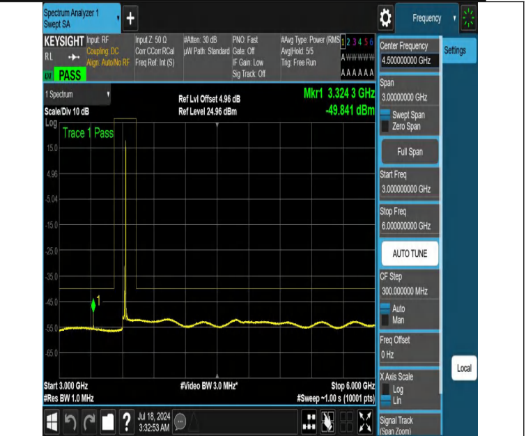
NTNV-DC_13A_n48A-PC3-30-5+15-M+M-N/A-N/A-DFT-QPSK-Edge_1RB_Right-3000-6000-PASS
