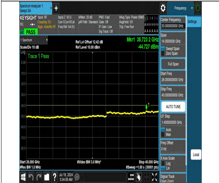
NTNV-DC_13A_n48A-PC3-30-5+15-M+H-N/A-N/A-DFT-PI2BPSK-Edge_1RB_Left-26000-40000-PASS
