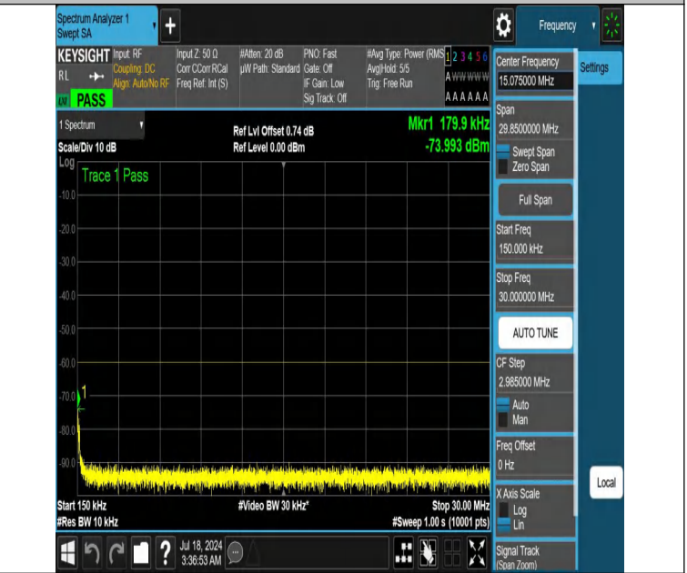
NTNV-DC_13A_n48A-PC3-30-5+15-M+H-N/A-N/A-DFT-QPSK-Edge_1RB_Left-0.15-30-PASS
