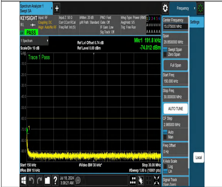
NTNV-DC_13A_n48A-PC3-30-5+15-M+H-N/A-N/A-DFT-QPSK-Edge_1RB_Right-0.15-30-PASS
