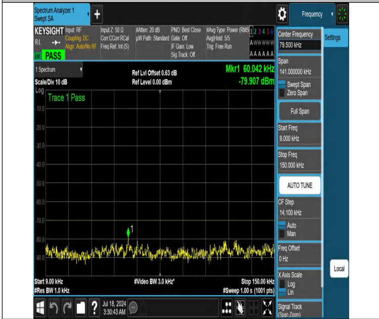
NTNV-DC_13A_n48A-PC3-30-5+15-M+M-N/A-N/A-DFT-QPSK-Edge_1RB_Left-0.009-0.15-PASS
