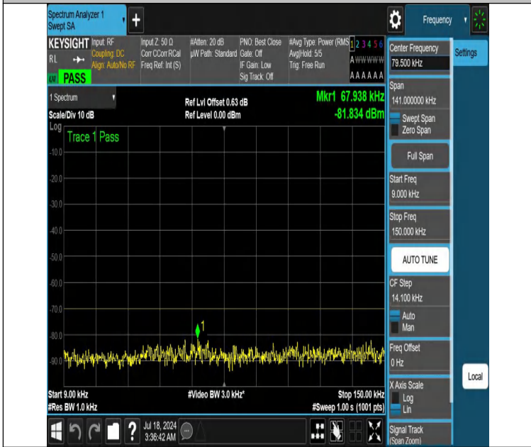
NTNV-DC_13A_n48A-PC3-30-5+15-M+H-N/A-N/A-DFT-QPSK-Edge_1RB_Left-0.009-0.15-PASS
