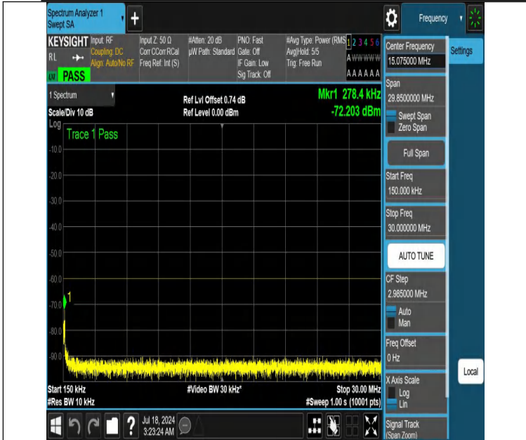
NTNV-DC_13A_n48A-PC3-30-5+15-M+L-N/A-N/A-DFT-PI2BPSK-Edge_1RB_Right-0.15-30-PASS
