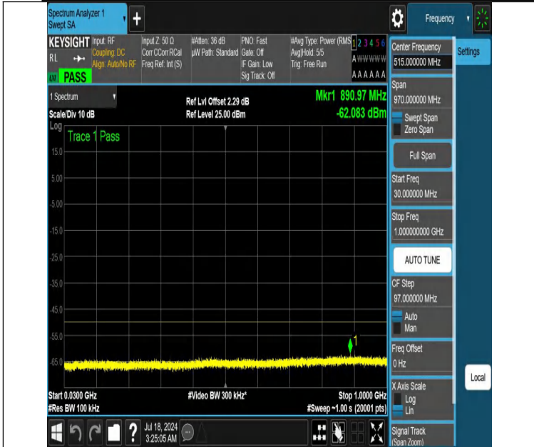
NTNV-DC_13A_n48A-PC3-30-5+15-M+L-N/A-N/A-DFT-QPSK-Edge e_1RB_Left-30-1000-PASS
