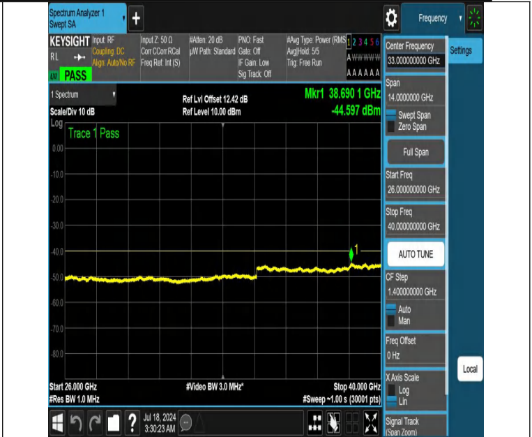
NTNV-DC_13A_n48A-PC3-30-5+15-M+M-N/A-N/A-DFT-PI2BPSK-E_dge_1RB_Right-26000-40000-PASS
