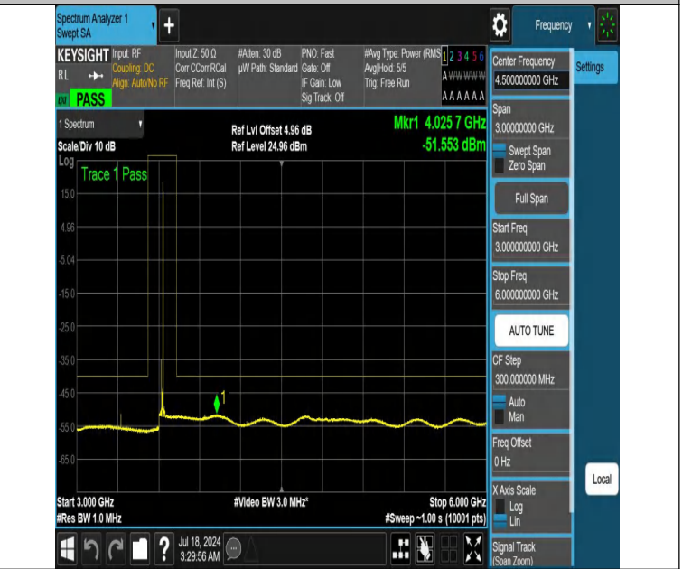
NTVN-DC_13A_n48A-PC3-30-5+15-M+M-N/A-N/A-DFT-PI2BPSK-E dge_1RB_Right-3000-6000-PASS
