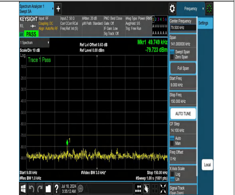
NTNV-DC_13A_n48A-PC3-30-5+15-M+H-N/A-N/A-DFT-PI2BPSK-E dge_1RB_Right-0.009-0.15-PASS
