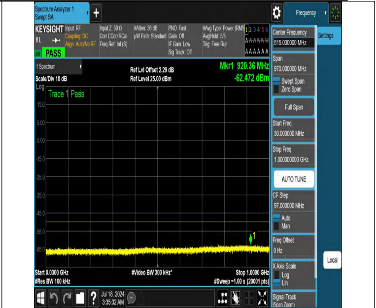
NTNV-DC_13A_n48A-PC3-30-5+15-M+H-N/A-N/A-DFT-PI2BPSK-E dge_1RB_Right-30-1000-PASS
