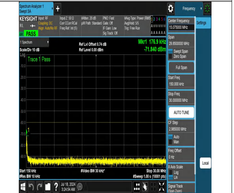
NTNV-DC_13A_n48A-PC3-30-5+15-M+L-N/A-N/A-DFT-QPSK-Edge_1RB_Left-0.15-30-PASS
