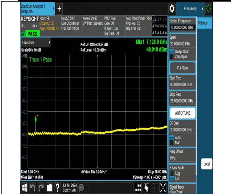
NTNV-DC_13A_n48A-PC3-30-5+15-M+L-N/A-N/A-DFT-PI2BPSK-Edge_1RB_Right-6000-26000-PASS
