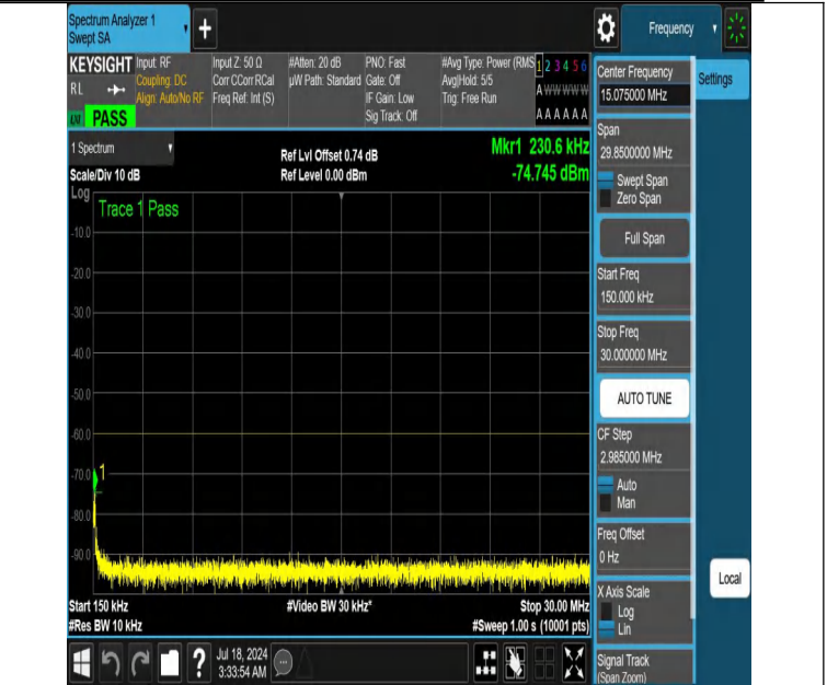
NTNV-DC_13A_n48A-PC3-30-5+15-M+H-N/A-N/A-DFT-PI2BPSK-E dge_1RB_Left-0.15-30-PASS
