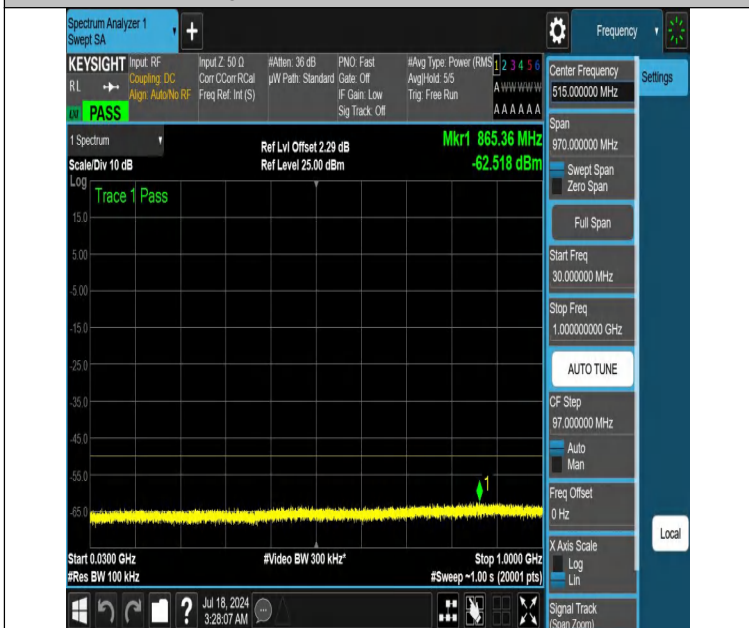
NTNV-DC_13A_n48A-PC3-30-5+15-M+M-N/A-N/A-DFT-PI2BPSK-Edge_1RB_Left-30-1000-PASS
