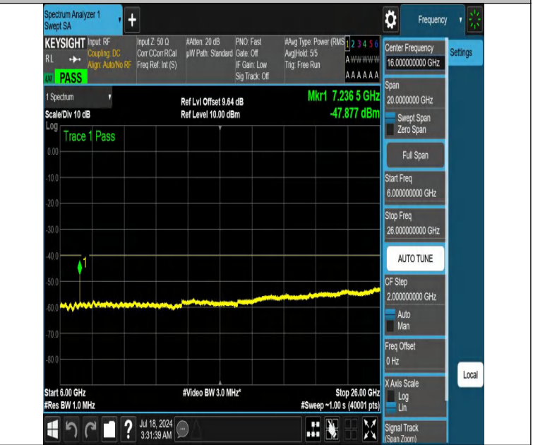
NTNV-DC_13A_n48A-PC3-30-5+15-M+M-N/A-N/A-DFT-QPSK-Edge_1RB_Left-6000-26000-PASS
