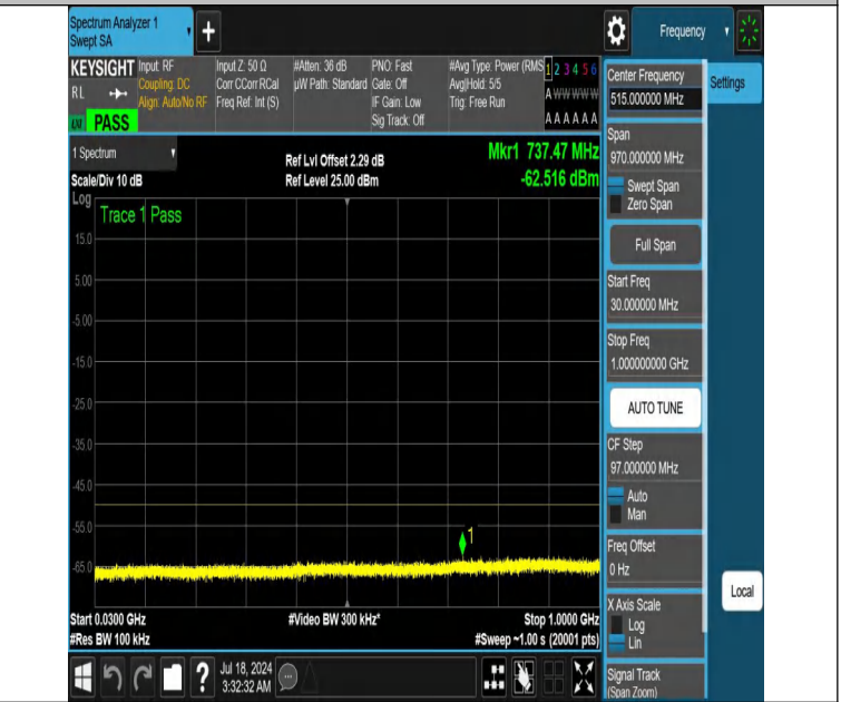
NTNV-DC_13A_n48A-PC3-30-5+15-M+M-N/A-N/A-DFT-QPSK-Edge_1RB_Right-30-1000-PASS
