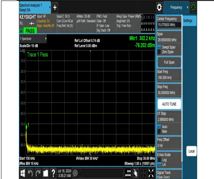
NTNV-DC_13A_n48A-PC3-30-5+15-M+H-N/A-N/A-DFT-PI2BPSK-Edge_1RB_Right-0.15-30-PASS
