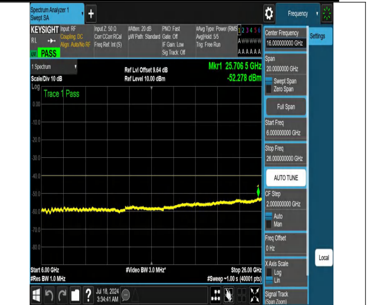
NTNV-DC_13A_n48A-PC3-30-5+15-M+H-N/A-N/A-DFT-PI2BPSK-E dge_1RB_Left-6000-26000-PASS
