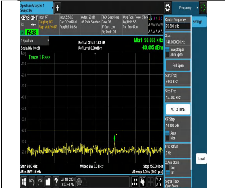
NTNV-DC_13A_n48A-PC3-30-5+15-M+H-N/A-N/A-DFT-PI2BPSK-Edge_1RB_Left-0.009-0.15-PASS
