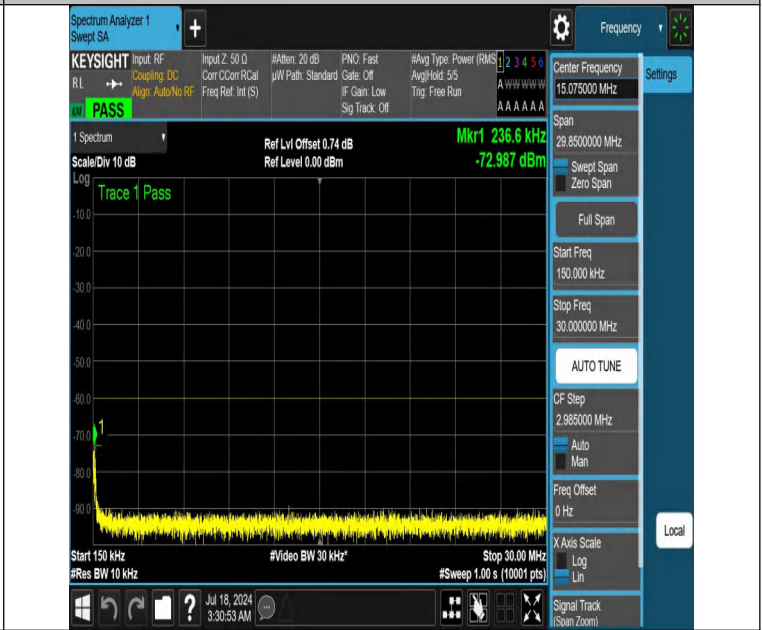
NTNV-DC_13A_n48A-PC3-30-5+15-M+M-N/A-N/A-DFT-QPSK-Edge_1RB_Left-0.15-30-PASS
