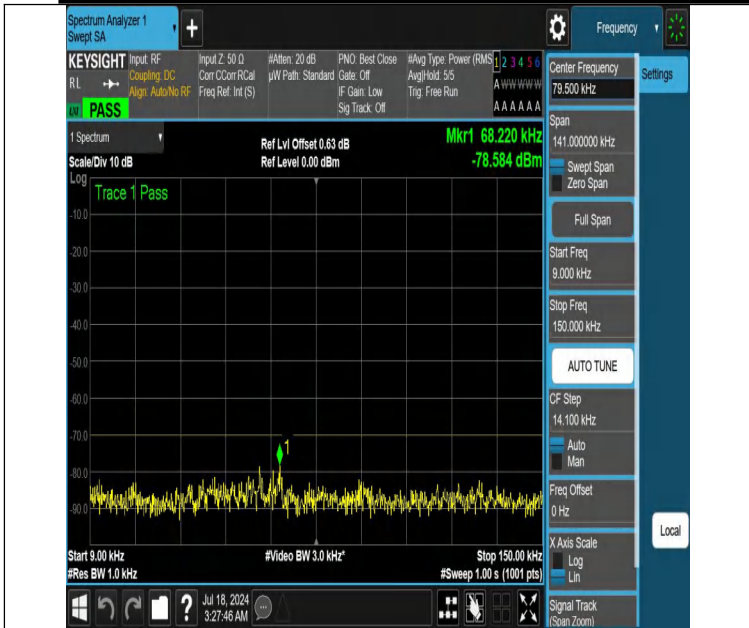
NTNV-DC_13A_n48A-PC3-30-5+15-M+M-N/A-N/A-DFT-PI2BPSK-Edge_1RB_Left-0.009-0.15-PASS
