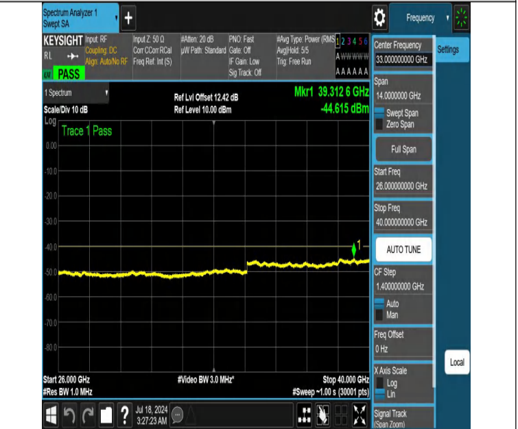
NTNV-DC_13A_n48A-PC3-30-5+15-M+L-N/A-N/A-DFT-QPSK-Edge _1RB_Right-26000-40000-PASS
