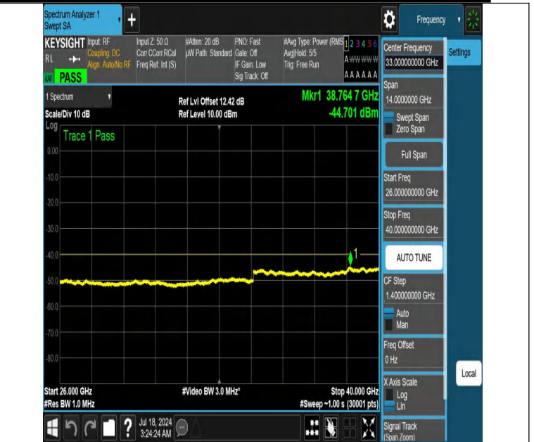
NTNV-DC_13A_n48A-PC3-30-5+15-M+L-N/A-N/A-DFT-PI2BPSK-E_dge_1RB_Right-26000-40000-PASS
