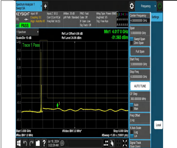
NTNV-DC_13A_n48A-PC3-30-5+15-M+L-N/A-N/A-DFT-PI2BPSK-Edge_1RB_Left-3000-6000-PASS
