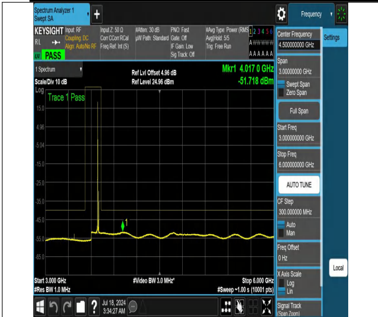
NTNV-DC_13A_n48A-PC3-30-5+15-M+H-N/A-N/A-DFT-PI2BPSK-Edge_1RB_Left-3000-6000-PASS
