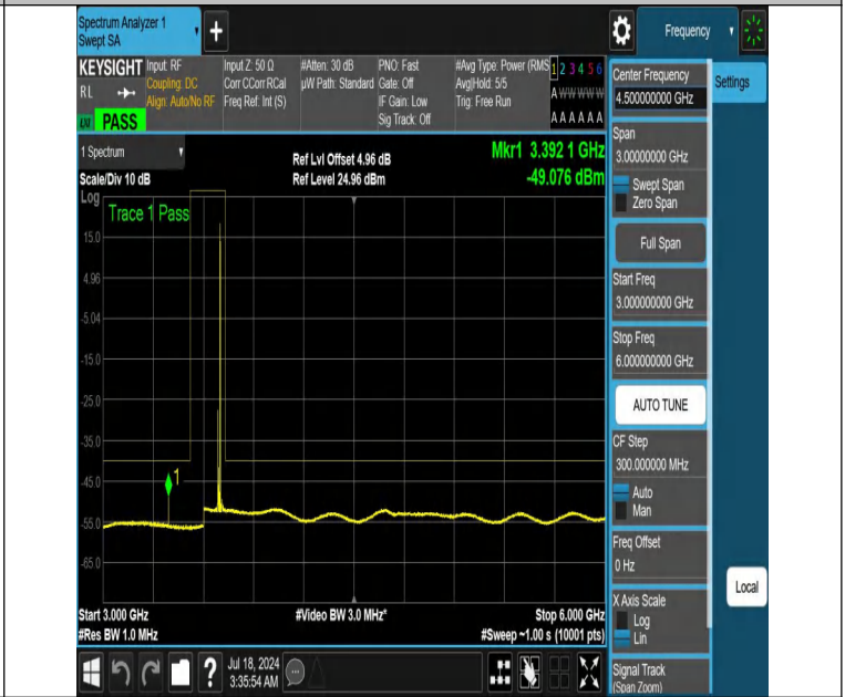
NTNV-DC_13A_n48A-PC3-30-5+15-M+H-N/A-N/A-DFT-PI2BPSK-E dge_1RB_Right-3000-6000-PASS
