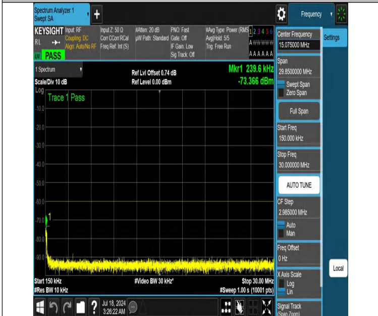
NTNV-DC_13A_n48A-PC3-30-5+15-M+L-N/A-N/A-DFT-QPSK-Edge e_1RB_Right-0.15-30-PASS
