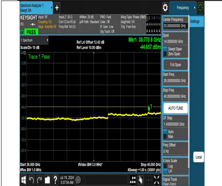
NTNV-DC_13A_n48A-PC3-30-5+15-M+H-N/A-N/A-DFT-QPSK-Edge_1RB_Left-26000-40000-PASS
