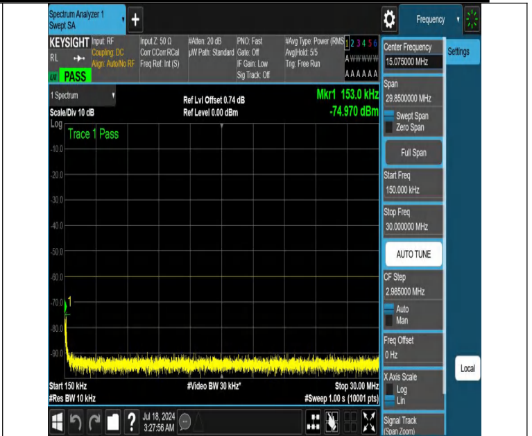
NTNV-DC_13A_n48A-PC3-30-5+15-M+M-N/A-N/A-DFT-PI2BPSK-E dge_1RB_Left-0.15-30-PASS
