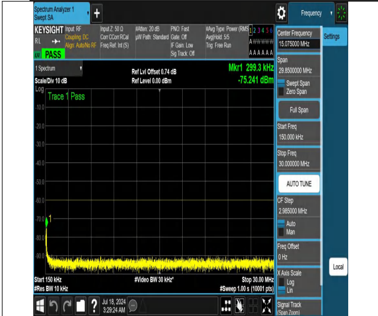
NTVN-DC_13A_n48A-PC3-30-5+15-M+M-N/A-N/A-DFT-PI2BPSK-Edge_1RB_Right-0.15-30-PASS
