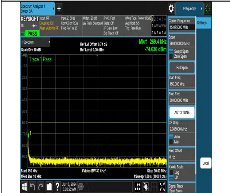
NTNV-DC_13A_n48A-PC3-30-5+10-M+H-N/A-N/A-DFT-QPSK-Edge e_1RB_Right-0.15-30-PASS
