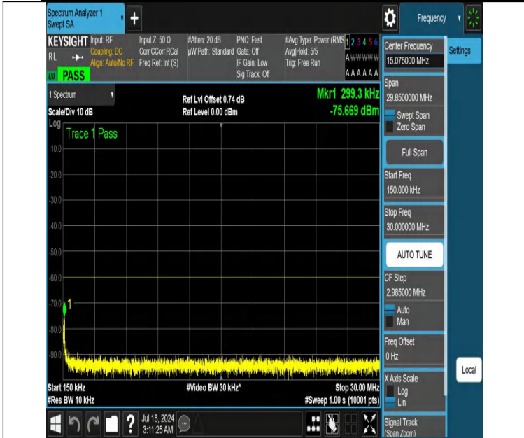
NTVN-DC_13A_n48A-PC3-30-5+10-M+M-N/A-N/A-DFT-PI2BPSK-Edge_1RB_Right-0.15-30-PASS
