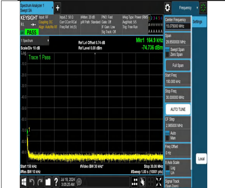
NTNV-DC_13A_n48A-PC3-30-5+10-M+L-N/A-N/A-DFT-PI2BPSK-Edge_1RB_Right-0.15-30-PASS
