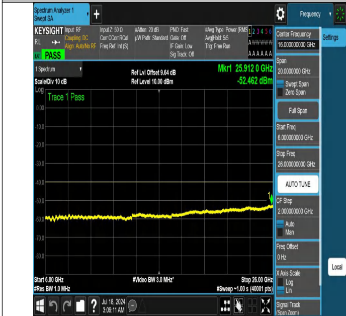
NTNV-DC_13A_n48A-PC3-30-5+10-M+L-N/A-N/A-DFT-QPSK-Edge e_1RB_Right-6000-26000-PASS
