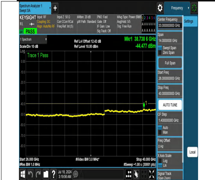
NTNV-DC_13A_n48A-PC3-30-5+10-M+H-N/A-N/A-DFT-QPSK-Edge e_1RB_Left-26000-40000-PASS
