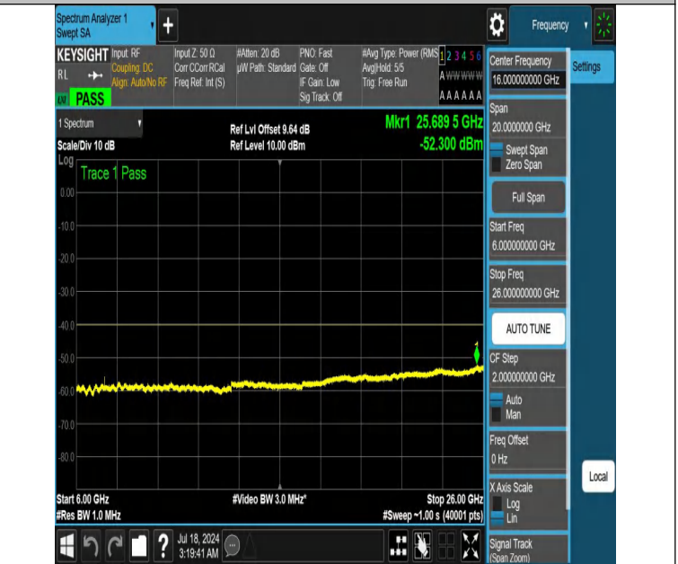
NTNV-DC_13A_n48A-PC3-30-5+10-M+H-N/A-N/A-DFT-QPSK-Edg e_1RB_Left-6000-26000-PASS
