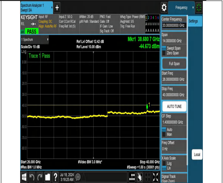
NTNV-DC_13A_n48A-PC3-30-5+10-M+H-N/A-N/A-DFT-PI2BPSK-E dge_1RB_Right-26000-40000-PASS
