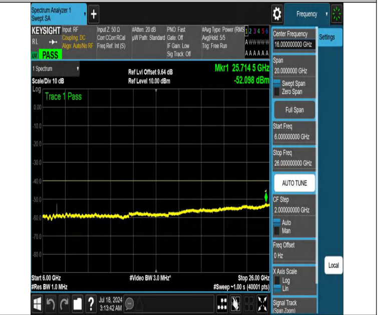
NTNV-DC_13A_n48A-PC3-30-5+10-M+M-N/A-N/A-DFT-QPSK-Edge_1RB_Left-6000-26000-PASS
