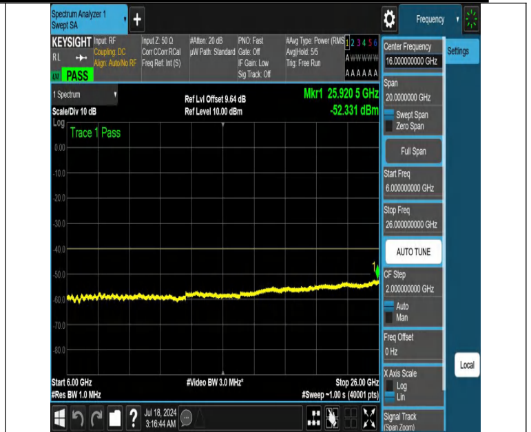
NTNV-DC_13A_n48A-PC3-30-5+10-M+H-N/A-N/A-DFT-PI2BPSK-E_dge_1RB_Left-6000-26000-PASS
