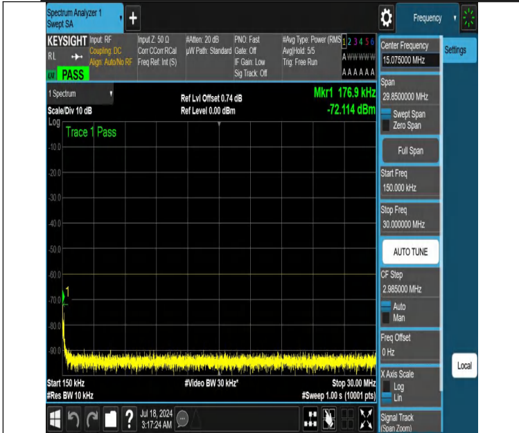
NTNV-DC_13A_n48A-PC3-30-5+10-M+H-N/A-N/A-DFT-PI2BPSK-Edge_1RB_Right-0.15-30-PASS
