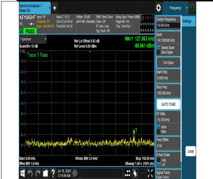
NTNV-DC_13A_n48A-PC3-30-5+10-M+H-N/A-N/A-DFT-PI2BPSK-Edge_1RB_Left-0.009-0.15-PASS
