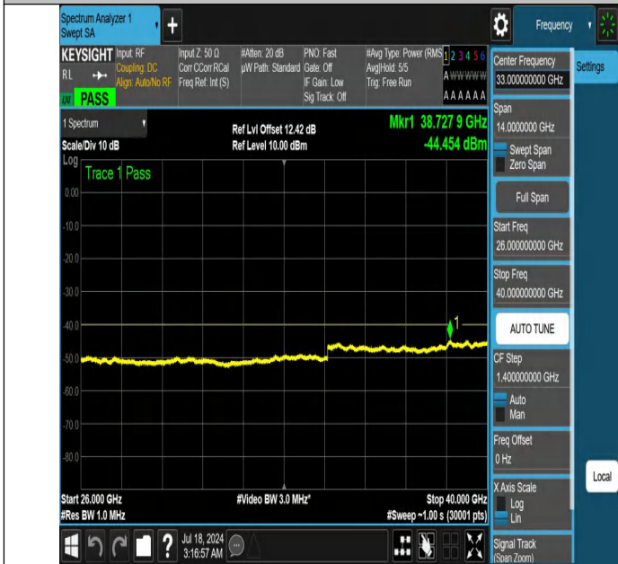
NTNV-DC_13A_n48A-PC3-30-5+10-M+H-N/A-N/A-DFT-PI2BPSK-Edge_1RB_Left-26000-40000-PASS
