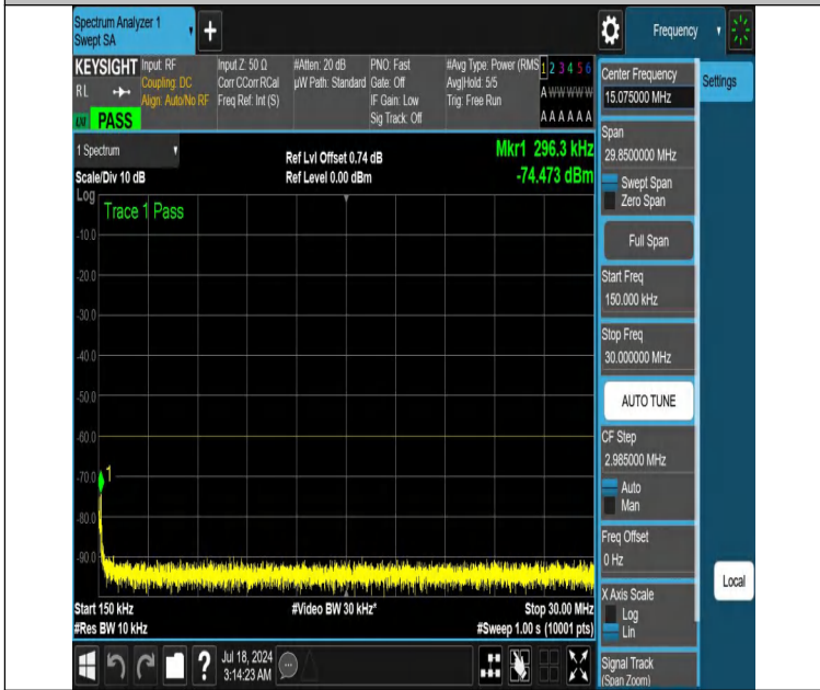
NTNV-DC_13A_n48A-PC3-30-5+10-M+M-N/A-N/A-DFT-QPSK-Edge_1RB_Right-0.15-30-PASS
