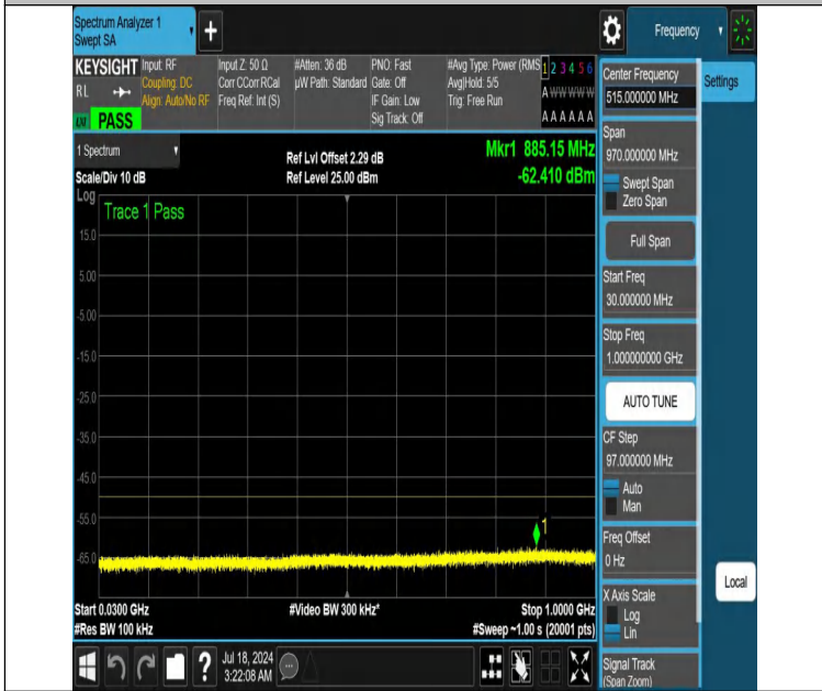
NTNV-DC_13A_n48A-PC3-30-5+15-M+L-N/A-N/A-DFT-PI2BPSK-Edge_1RB_Left-30-1000-PASS
