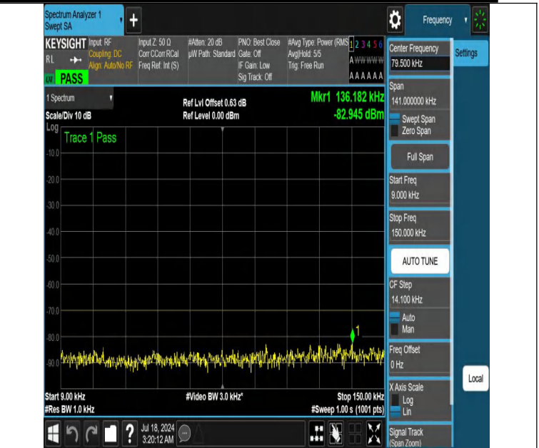
NTNV-DC_13A_n48A-PC3-30-5+10-M+H-N/A-N/A-DFT-QPSK-Edge e_1RB_Right-0.009-0.15-PASS
