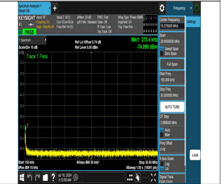
NTNV-DC_13A_n48A-PC3-30-5+10-M+M-N/A-N/A-DFT-QPSK-Edg e_1RB_Left-0.15-30-PASS
