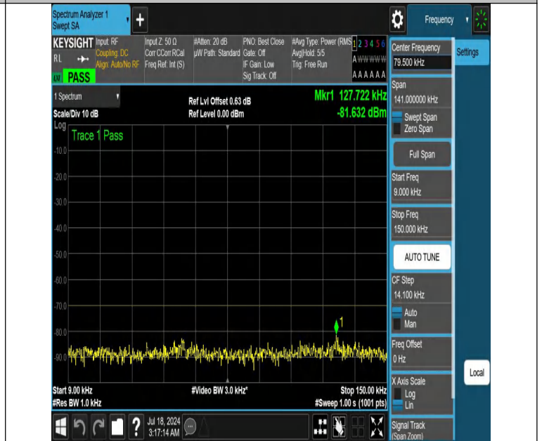
NTNV-DC_13A_n48A-PC3-30-5+10-M+H-N/A-N/A-DFT-PI2BPSK-E_dge_1RB_Right-0.009-0.15-PASS
