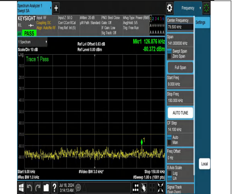
NTNV-DC_13A_n48A-PC3-30-5+10-M+M-N/A-N/A-DFT-QPSK-Edge_1RB_Right-0.009-0.15-PASS
