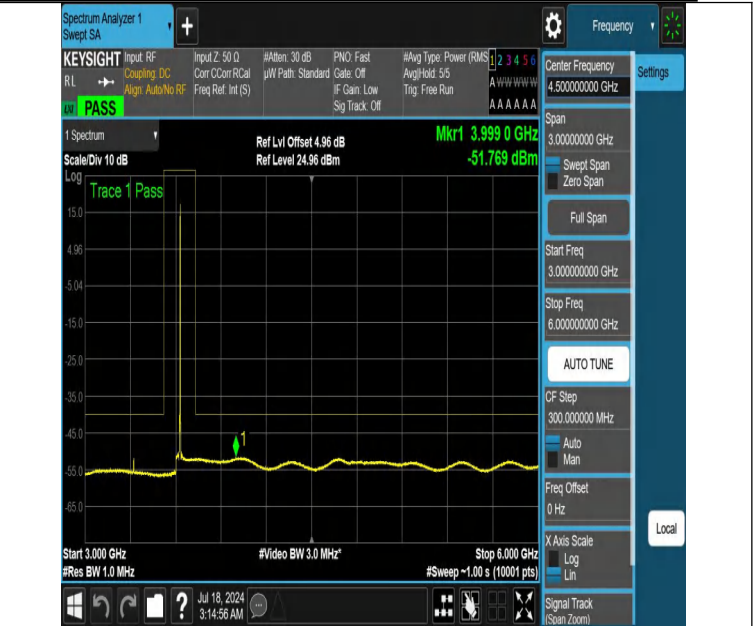
NTNV-DC_13A_n48A-PC3-30-5+10-M+M-N/A-N/A-DFT-QPSK-Edge_1RB_Right-3000-6000-PASS
