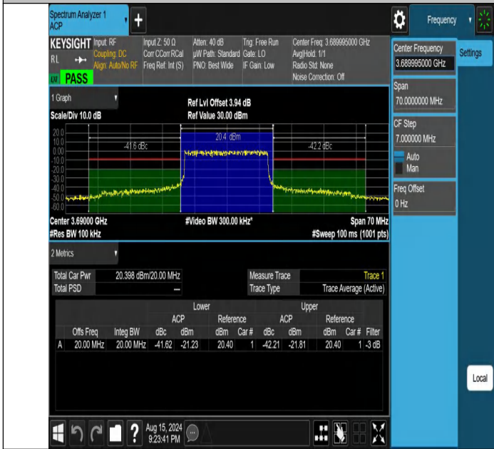
NTNV-DC_13A_n48A-PC3-30-5+20-M+H-N/A-N/A-DFT-QPSK-Out_er_Full-PASS
