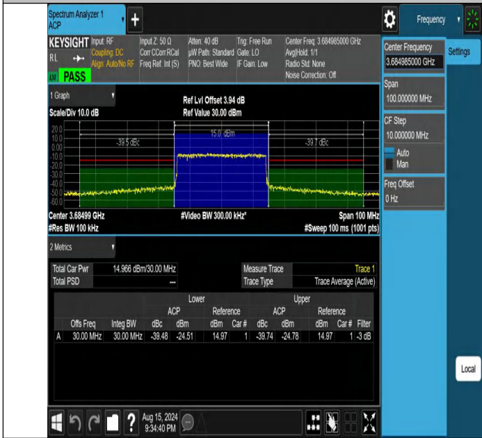
NTVN-DC_13A_n48A-PC3-30-5+30-M+H-N/A-N/A-CP-256QAM-Outer_Full-PASS
