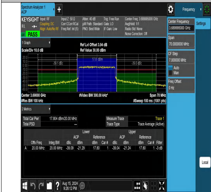
NTNV-DC_13A_n48A-PC3-30-5+20-M+H-N/A-N/A-CP-64QAM-Out_er_Full-PASS
