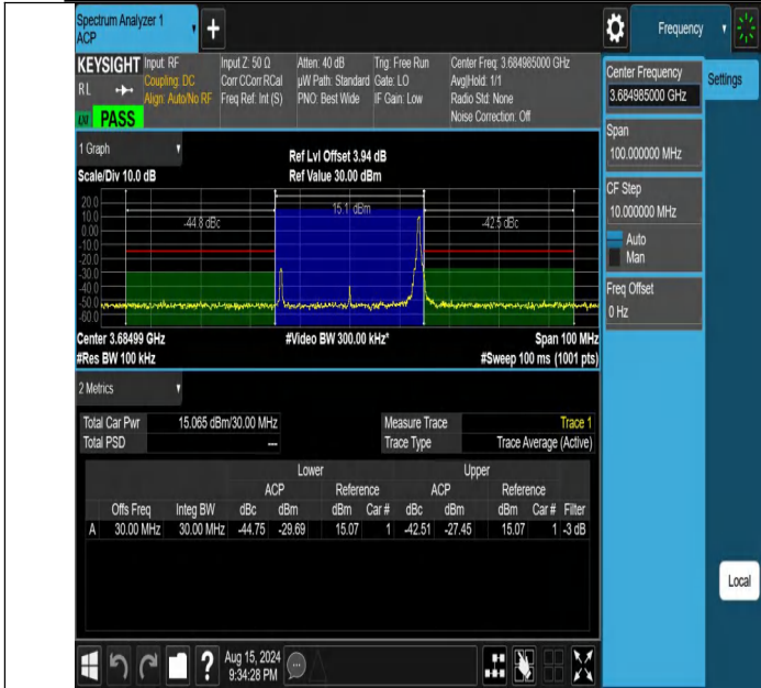
NTNV-DC_13A_n48A-PC3-30-5+30-M+H-N/A-N/A-CP-256QAM-Edge_1RB_Right-PASS
