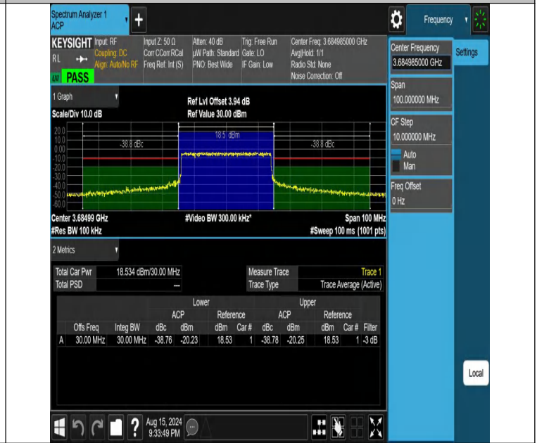
NTNV-DC_13A_n48A-PC3-30-5+30-M+H-N/A-N/A-CP-16QAM-Out er_Full-PASS
