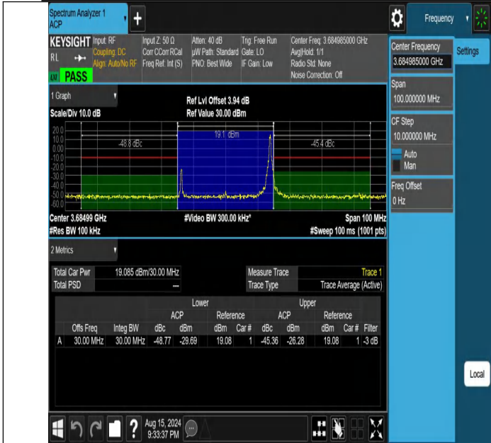
NTNV-DC_13A_n48A-PC3-30-5+30-M+H-N/A-N/A-CP-16QAM-Edge_1RB_Right-PASS
