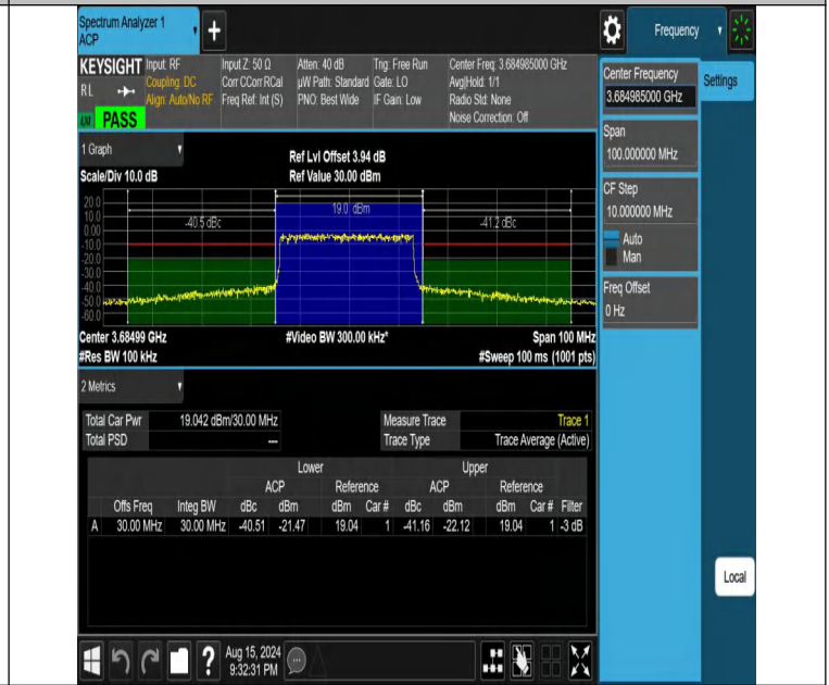
NTNV-DC_13A_n48A-PC3-30-5+30-M+H-N/A-N/A-DFT-64QAM-Outer_Full-PASS
