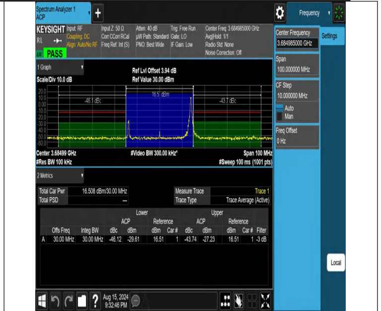
NTNV-DC_13A_n48A-PC3-30-5+30-M+H-N/A-N/A-DFT-256QAM-E dge_1RB_Right-PASS
