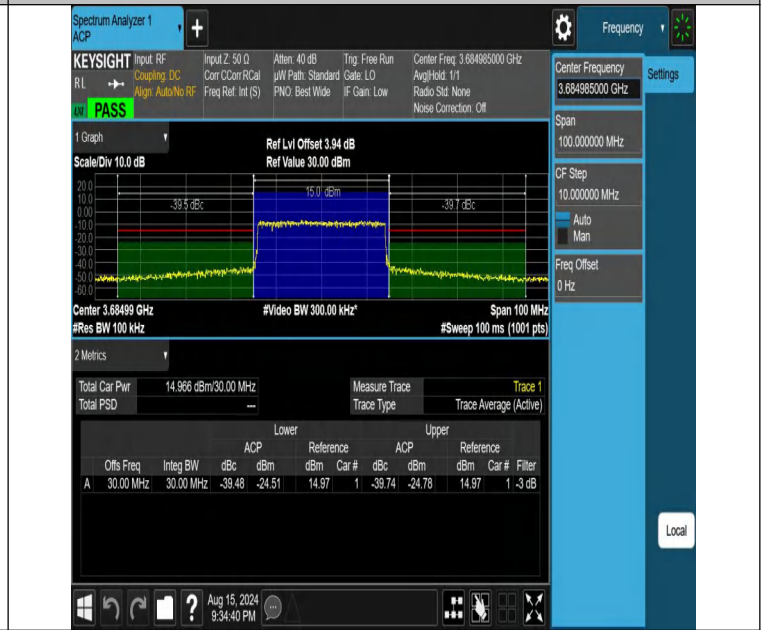
NTVN-DC_13A_n48A-PC3-30-5+30-M+H-N/A-N/A-CP-256QAM-Outer_Full-PASS
