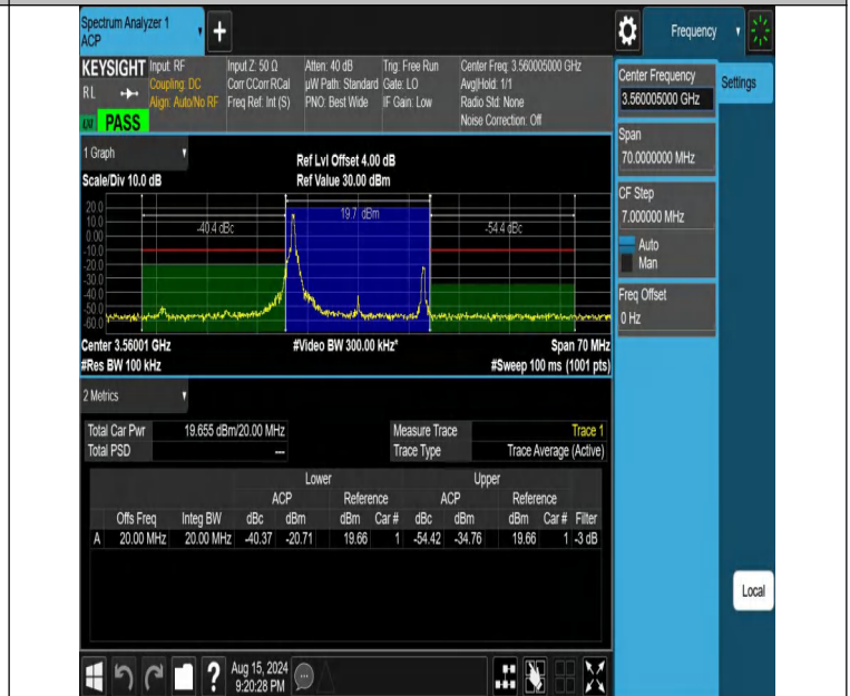
NTNV-DC_13A_n48A-PC3-30-5+20-M+L-N/A-N/A-DFT-64QAM-Ed ge_1RB_Left-PASS
