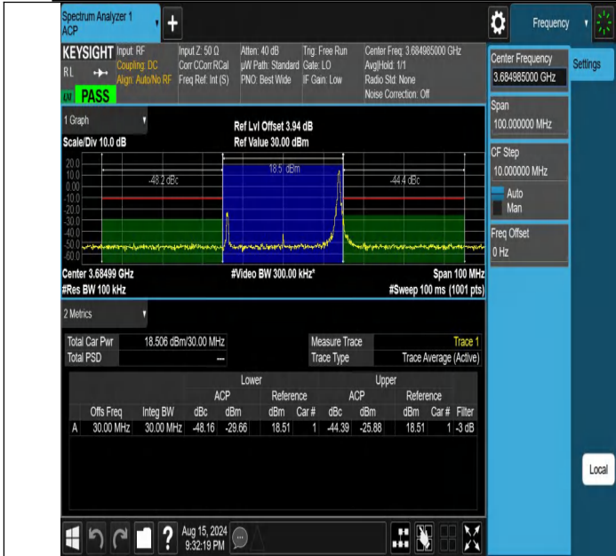
NTNV-DC_13A_n48A-PC3-30-5+30-M+H-N/A-N/A-DFT-64QAM-Edge_1RB_Right-PASS
