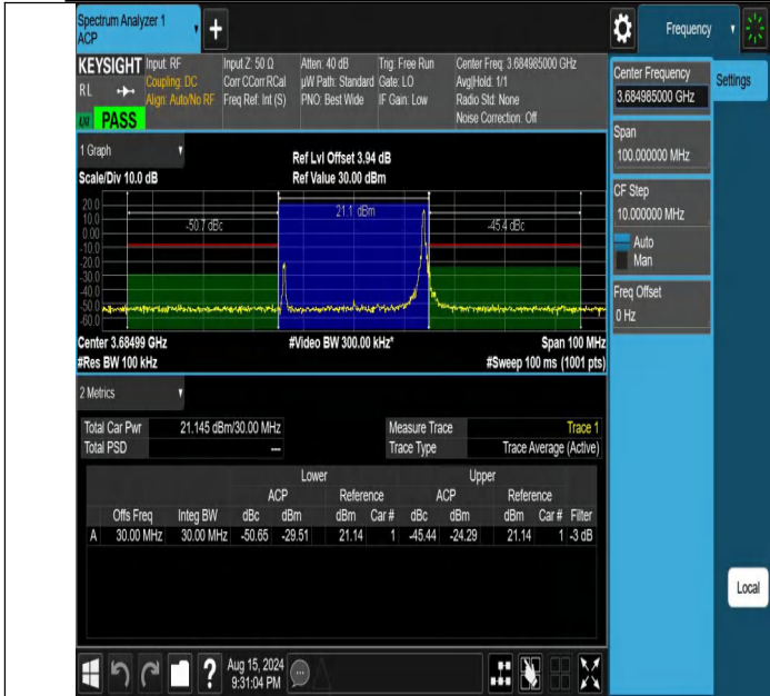
NTVN-DC_13A_n48A-PC3-30-5+30-M+H-N/A-N/A-DFT-PI2BPSK-Edge_1RB_Right-PASS
