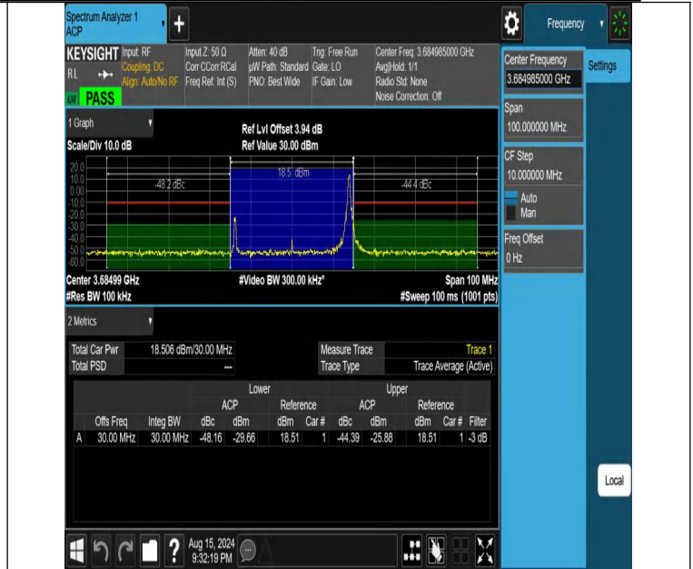
NTNV-DC_13A_n48A-PC3-30-5+30-M+H-N/A-N/A-DFT-64QAM-Edge_1RB_Right-PASS
