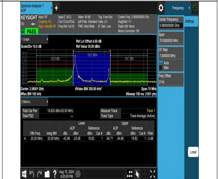
NTNV-DC_13A_n48A-PC3-30-5+20-M+L-N/A-N/A-DFT-16QAM-Edge_1RB_Left-PASS
