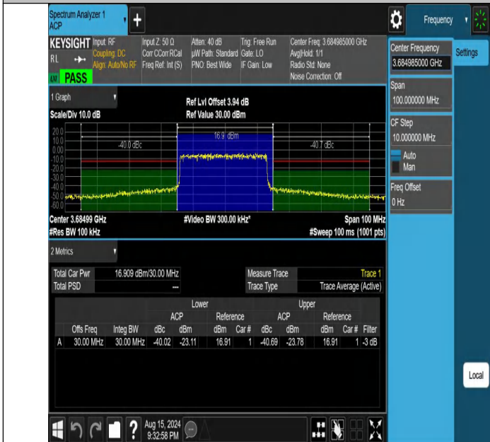
NTNV-DC_13A_n48A-PC3-30-5+30-M+H-N/A-N/A-DFT-256QAM-Outer_Full-PASS
