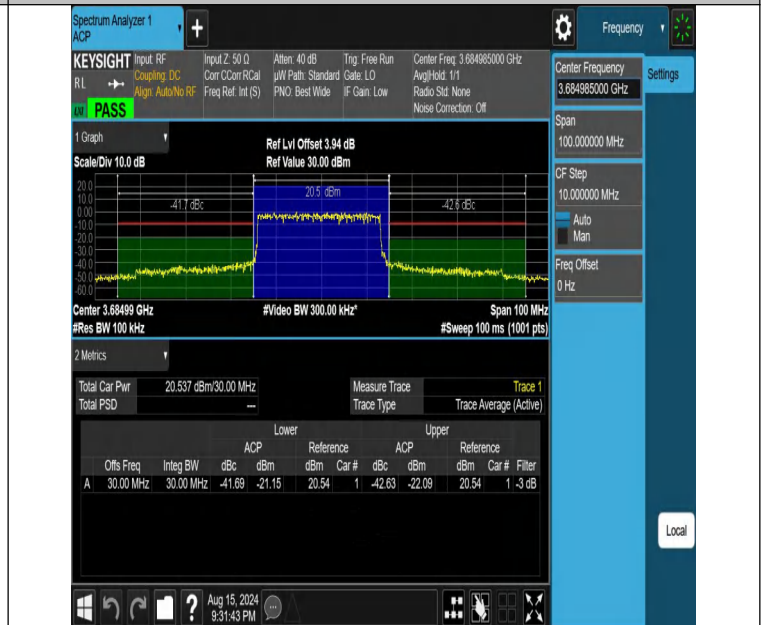
NTVN-DC_13A_n48A-PC3-30-5+30-M+H-N/A-N/A-DFT-QPSK-Out_er_Full-PASS
