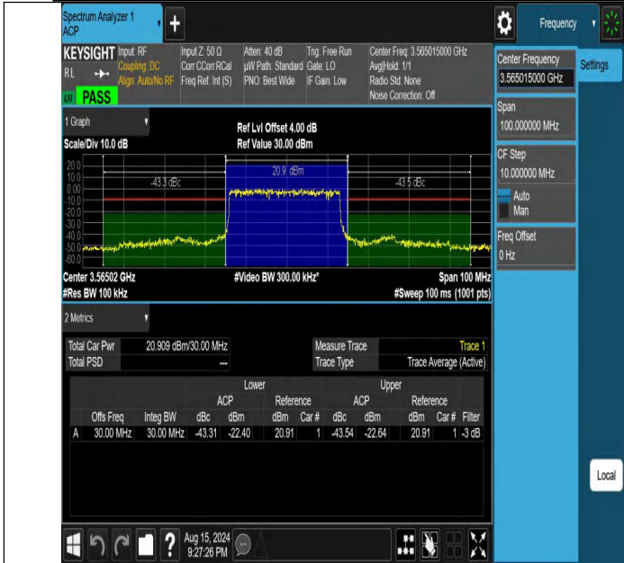
NTVN-DC_13A_n48A-PC3-30-5+30-M+L-N/A-N/A-DFT-PI2BPSK-Outer_Full-PASS
