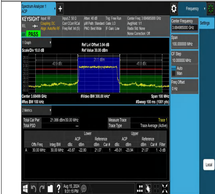
NTNV-DC_13A_n48A-PC3-30-5+30-M+H-N/A-N/A-DFT-PI2BPSK-Outer_Full-PASS
