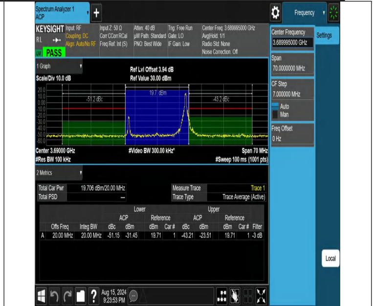
NTNV-DC_13A_n48A-PC3-30-5+20-M+H-N/A-N/A-DFT-16QAM-Edge_1RB_Right-PASS
