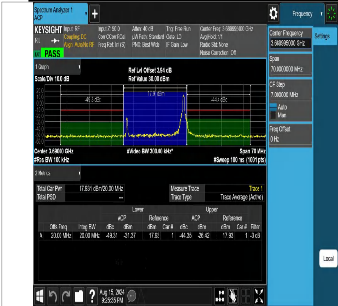
NTNV-DC_13A_n48A-PC3-30-5+20-M+H-N/A-N/A-CP-16QAM-Edge_1RB_Right-PASS
