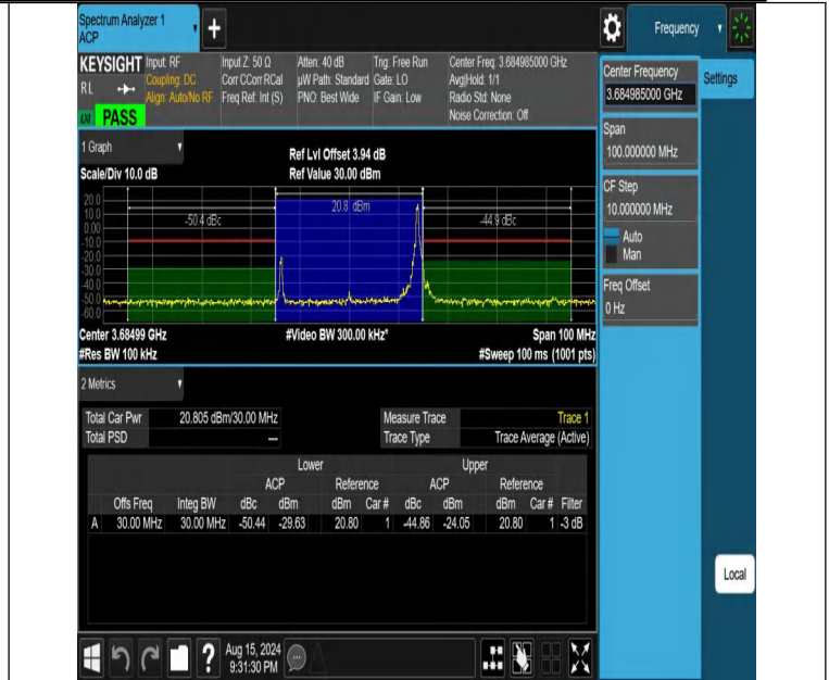
NTNV-DC_13A_n48A-PC3-30-5+30-M+H-N/A-N/A-DFT-QPSK-Edge_1RB_Right-PASS
