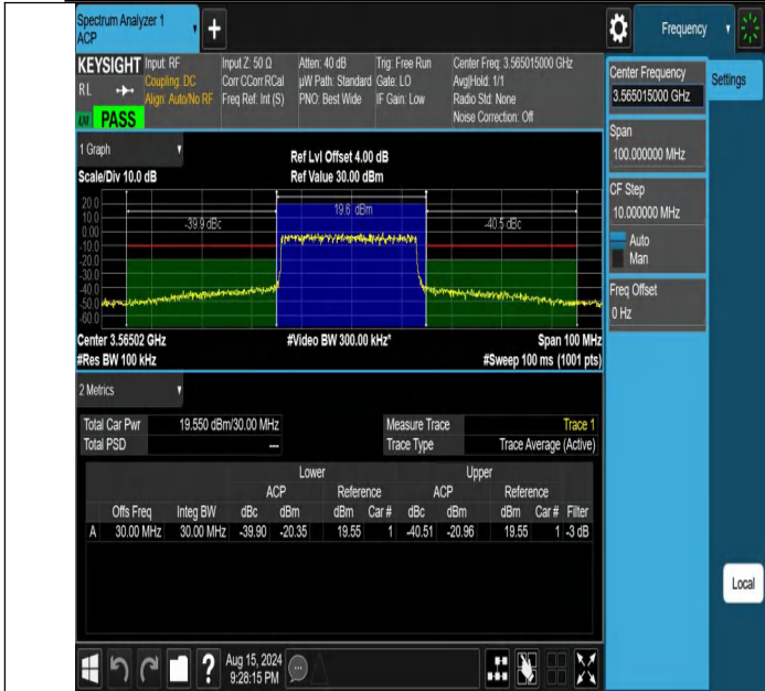
NTNV-DC_13A_n48A-PC3-30-5+30-M+L-N/A-N/A-DFT-16QAM-Ou ter_Full-PASS
