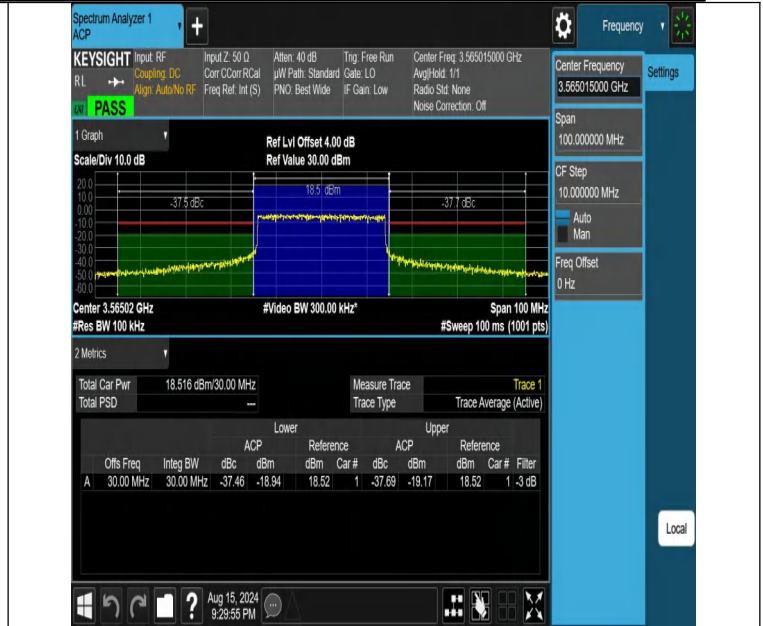
NTNV-DC_13A_n48A-PC3-30-5+30-M+L-N/A-N/A-CP-16QAM-Out er_Full-PASS
