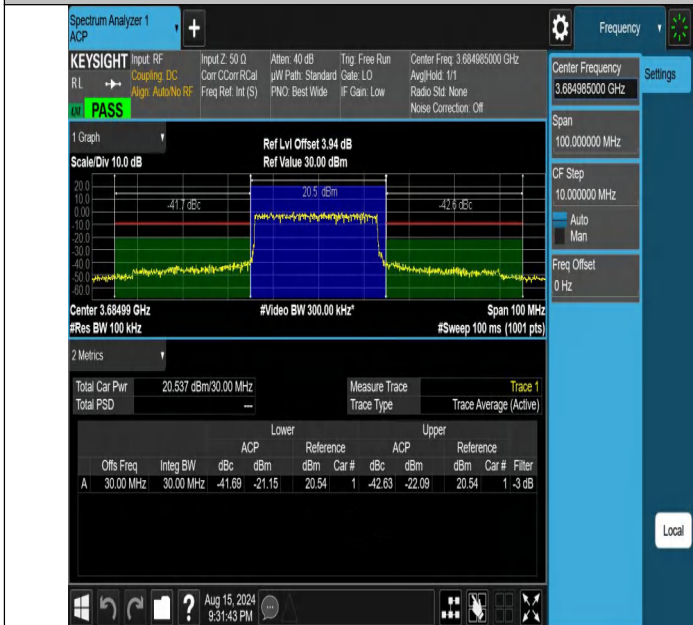
NTVN-DC_13A_n48A-PC3-30-5+30-M+H-N/A-N/A-DFT-QPSK-Out_er_Full-PASS
