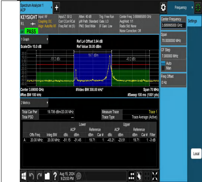
NTNV-DC_13A_n48A-PC3-30-5+20-M+H-N/A-N/A-DFT-16QAM-Edge_1RB_Right-PASS
