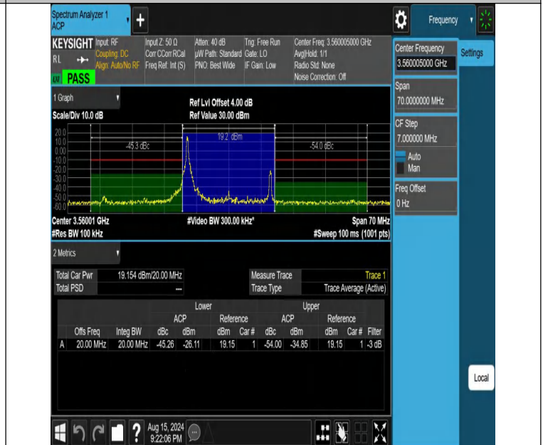
NTNV-DC_13A_n48A-PC3-30-5+20-M+L-N/A-N/A-CP-64QAM-Edge_1RB_Left-PASS
