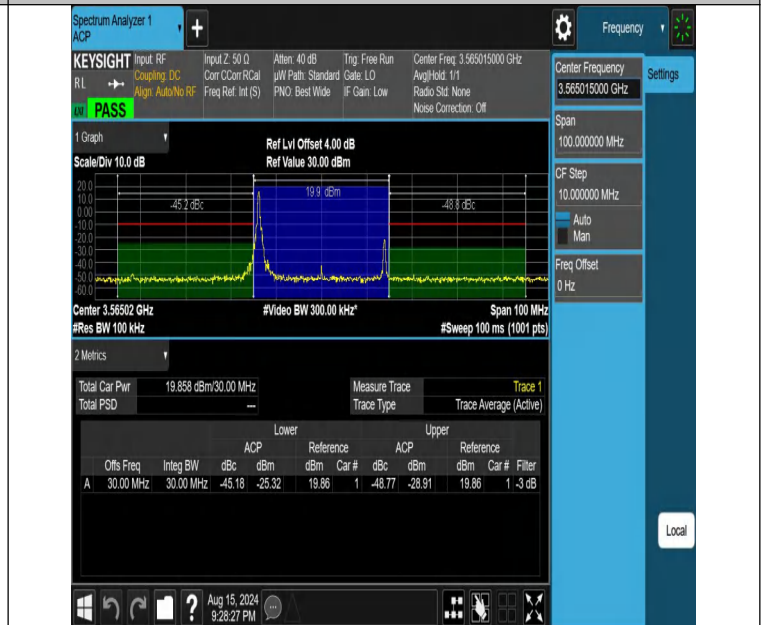
NTNV-DC_13A_n48A-PC3-30-5+30-M+L-N/A-N/A-DFT-64QAM-Ed ge_1RB_Left-PASS
