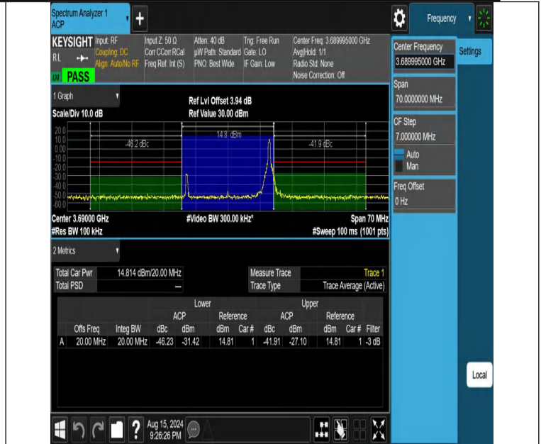
NTNV-DC_13A_n48A-PC3-30-5+20-M+H-N/A-N/A-CP-256QAM-Edge_1RB_Right-PASS
