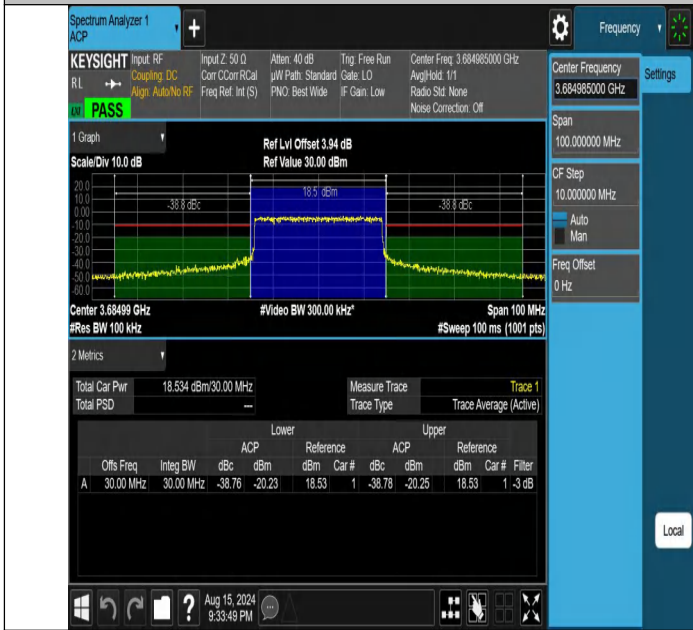
NTNV-DC_13A_n48A-PC3-30-5+30-M+H-N/A-N/A-CP-16QAM-Out er_Full-PASS
