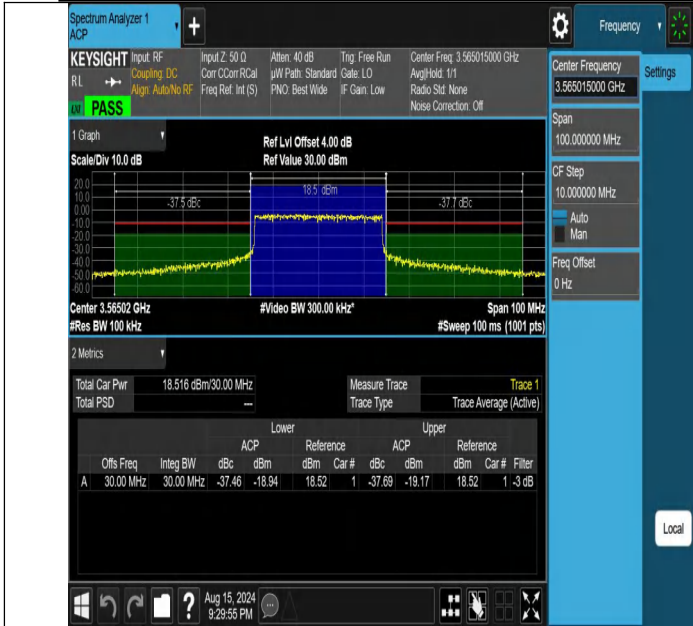
NTNV-DC_13A_n48A-PC3-30-5+30-M+L-N/A-N/A-CP-16QAM-Out er_Full-PASS
