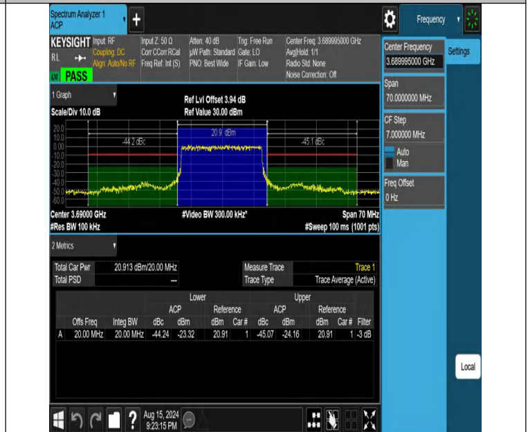
NTNV-DC_13A_n48A-PC3-30-5+20-M+H-N/A-N/A-DFT-PI2BPSK-Outer_Full-PASS
