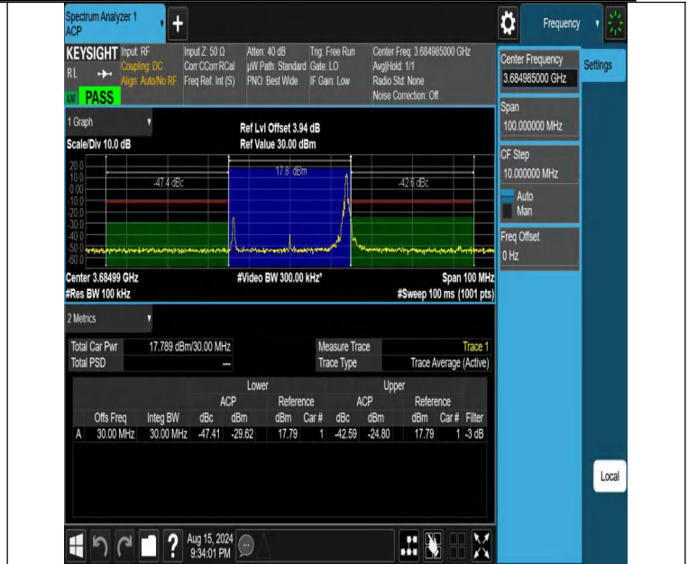
NTVN-DC_13A_n48A-PC3-30-5+30-M+H-N/A-N/A-CP-64QAM-Edge_1RB_Right-PASS
