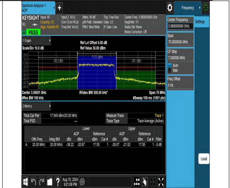
NTNV-DC_13A_n48A-PC3-30-5+20-M+L-N/A-N/A-DFT-256QAM-O uter_Full-PASS
