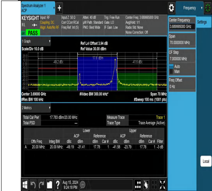
NTNV-DC_13A_n48A-PC3-30-5+20-M+H-N/A-N/A-DFT-64QAM-Edge_1RB_Right-PASS
