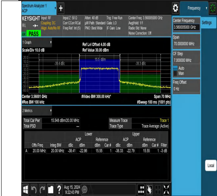
NTNV-DC_13A_n48A-PC3-30-5+20-M+L-N/A-N/A-CP-256QAM-Outer_Full-PASS
