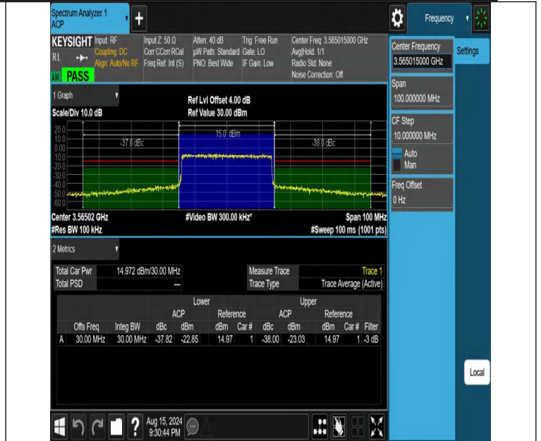
NTNV-DC_13A_n48A-PC3-30-5+30-M+L-N/A-N/A-CP-256QAM-Outer_Full-PASS
