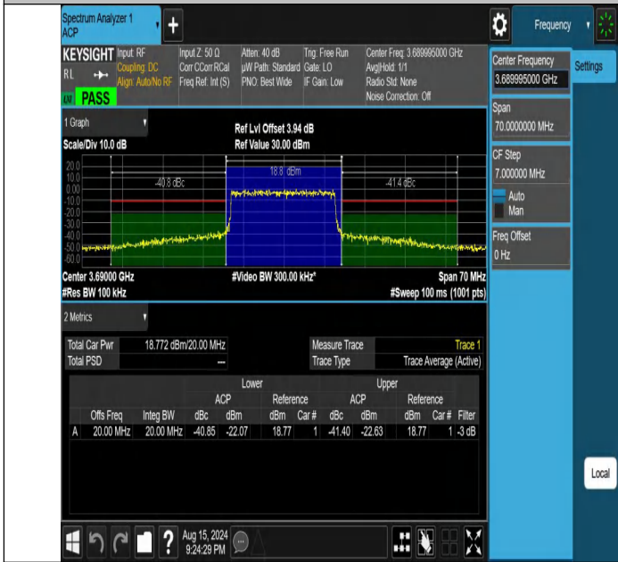
NTNV-DC_13A_n48A-PC3-30-5+20-M+H-N/A-N/A-DFT-64QAM-Outer_Full-PASS
