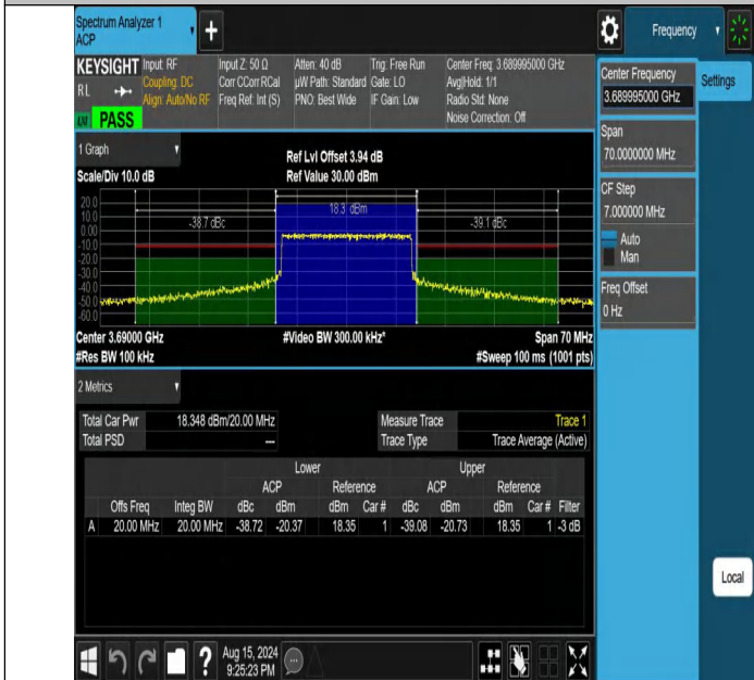
NTNV-DC_13A_n48A-PC3-30-5+20-M+H-N/A-N/A-CP-QPSK-Oute r_Full-PASS
