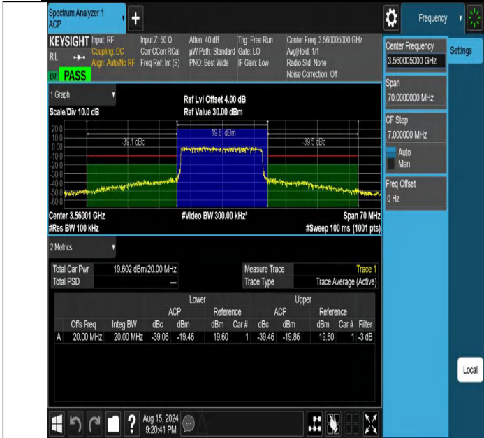
NTNV-DC_13A_n48A-PC3-30-5+20-M+L-N/A-N/A-DFT-64QAM-Ou ter_Full-PASS
