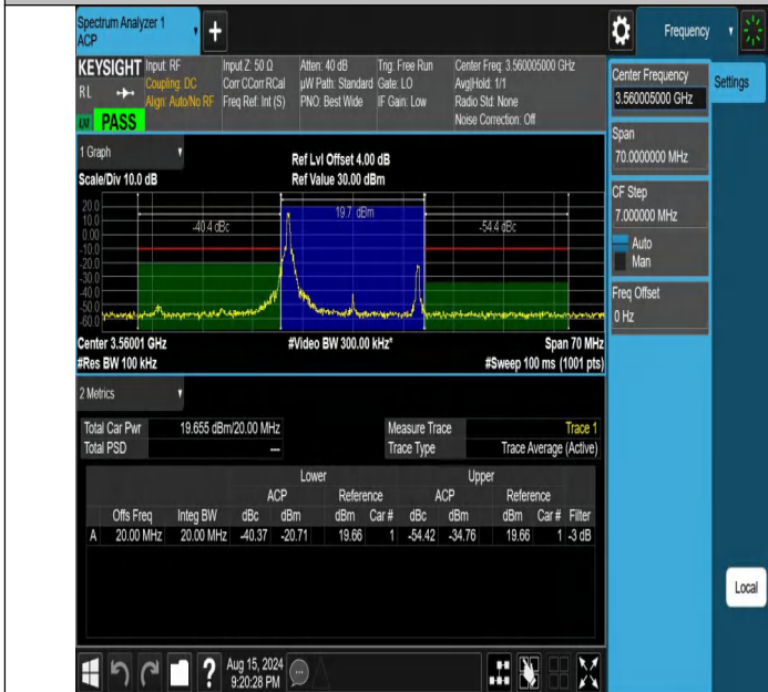
NTNV-DC_13A_n48A-PC3-30-5+20-M+L-N/A-N/A-DFT-64QAM-Ed ge_1RB_Left-PASS
