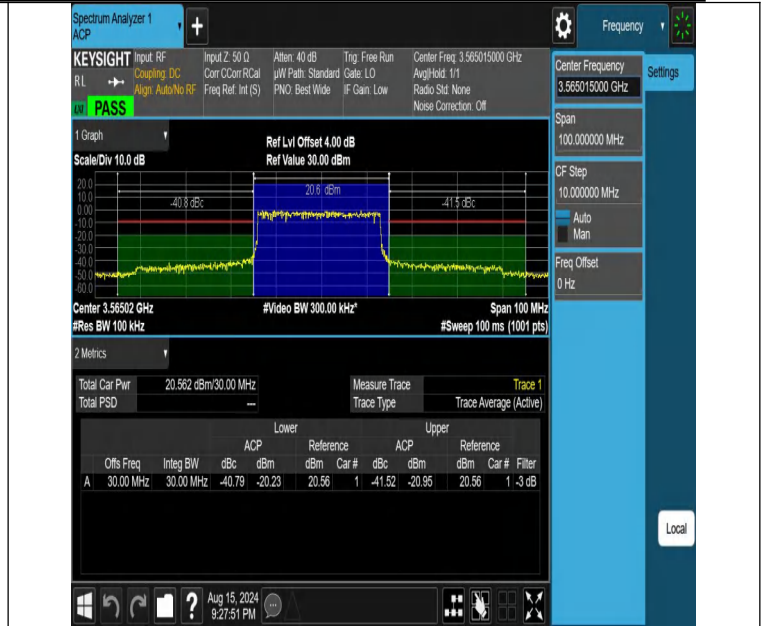
NTVN-DC_13A_n48A-PC3-30-5+30-M+L-N/A-N/A-DFT-QPSK-Out er_Full-PASS
