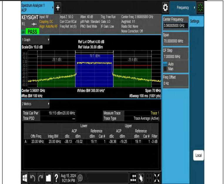
NTNV-DC_13A_n48A-PC3-30-5+20-M+L-N/A-N/A-CP-16QAM-Out er_Full-PASS
