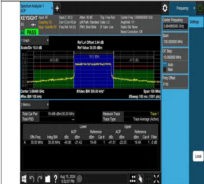
NTNV-DC_13A_n48A-PC3-30-5+30-M+H-N/A-N/A-DFT-16QAM-Ou ter_Full-PASS
