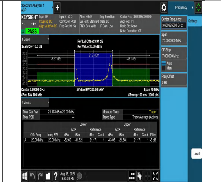
NTNV-DC_13A_n48A-PC3-30-5+20-M+H-N/A-N/A-DFT-PI2BPSK-Edge_1RB_Right-PASS
