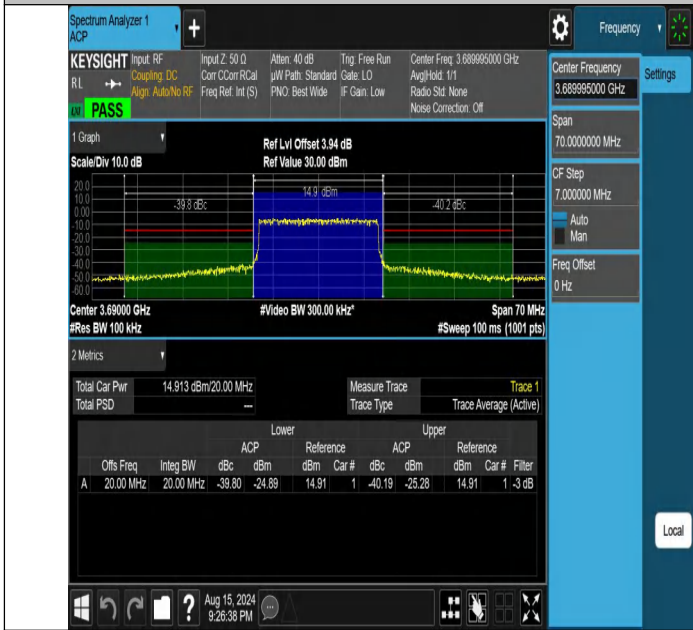
NTNV-DC_13A_n48A-PC3-30-5+20-M+H-N/A-N/A-CP-256QAM-Outer_Full-PASS
