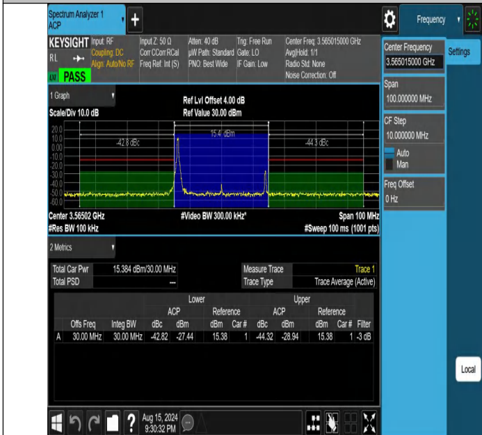
NTNV-DC_13A_n48A-PC3-30-5+30-M+L-N/A-N/A-CP-256QAM-Edge_1RB_Left-PASS
