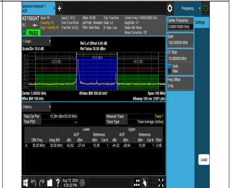
NTNV-DC_13A_n48A-PC3-30-5+30-M+L-N/A-N/A-CP-256QAM-Edge_1RB_Left-PASS
