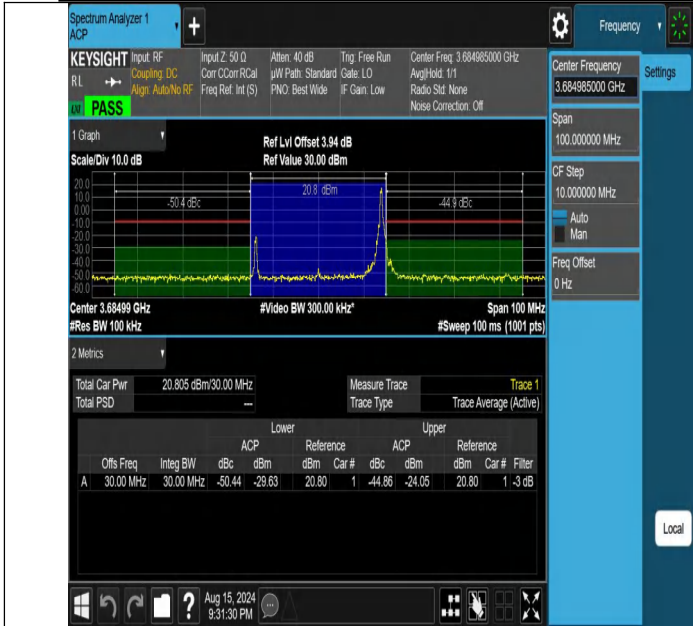
NTNV-DC_13A_n48A-PC3-30-5+30-M+H-N/A-N/A-DFT-QPSK-Edge_1RB_Right-PASS
