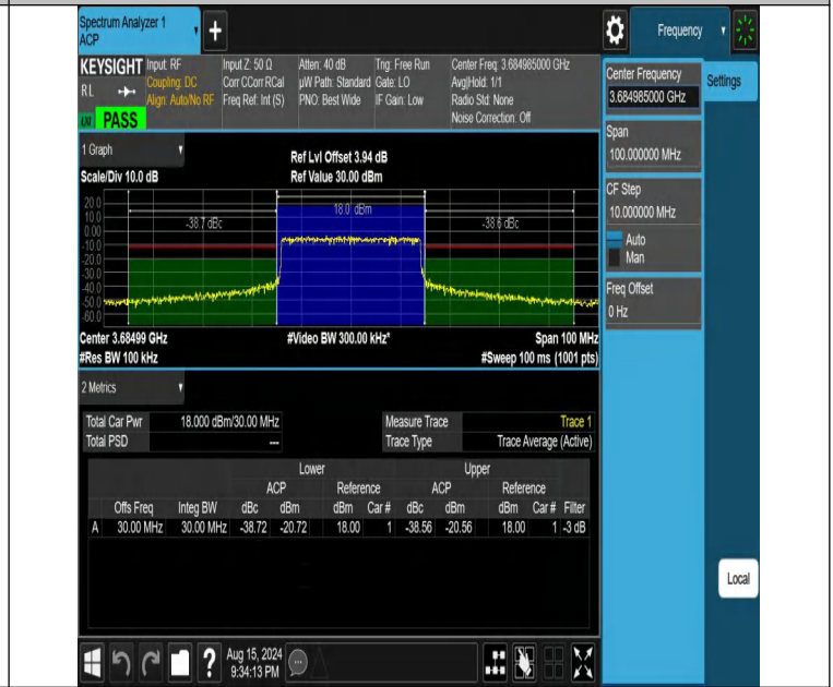
NTNV-DC_13A_n48A-PC3-30-5+30-M+H-N/A-N/A-CP-64QAM-Out_er_Full-PASS
