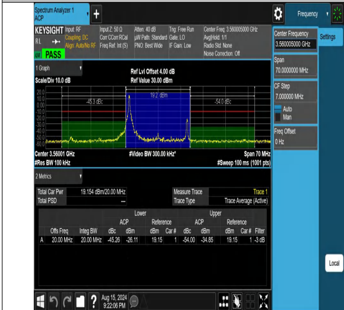
NTNV-DC_13A_n48A-PC3-30-5+20-M+L-N/A-N/A-CP-64QAM-Edge_1RB_Left-PASS
