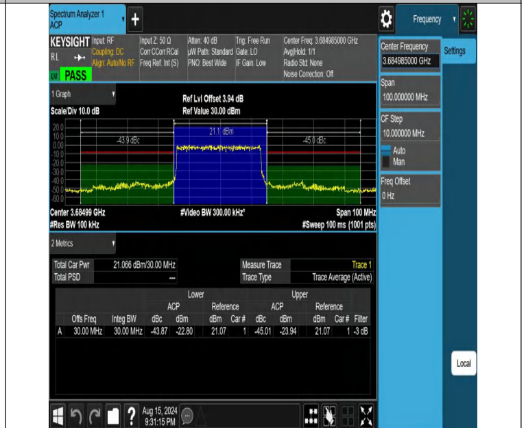
NTNV-DC_13A_n48A-PC3-30-5+30-M+H-N/A-N/A-DFT-PI2BPSK-Outer_Full-PASS
