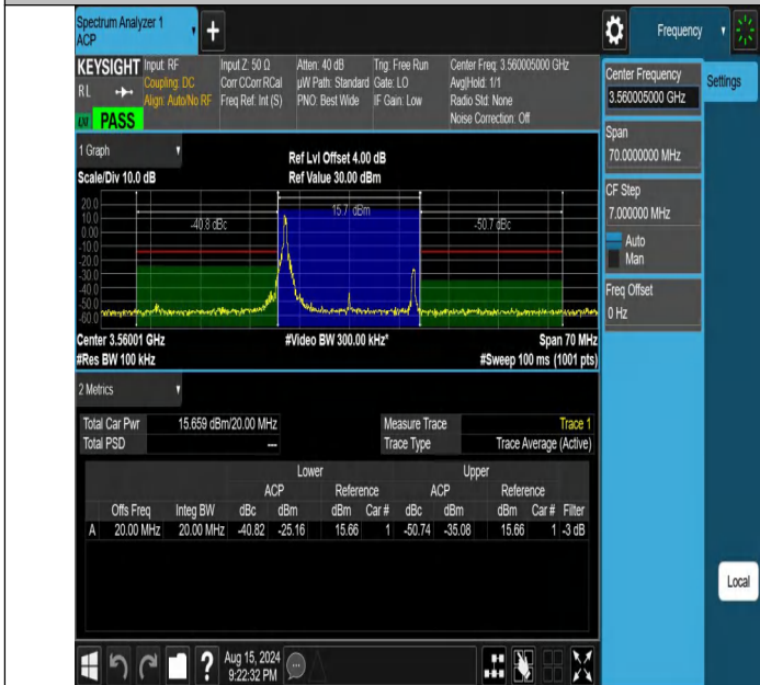
NTNV-DC_13A_n48A-PC3-30-5+20-M+L-N/A-N/A-CP-256QAM-Edge_1RB_Left-PASS
