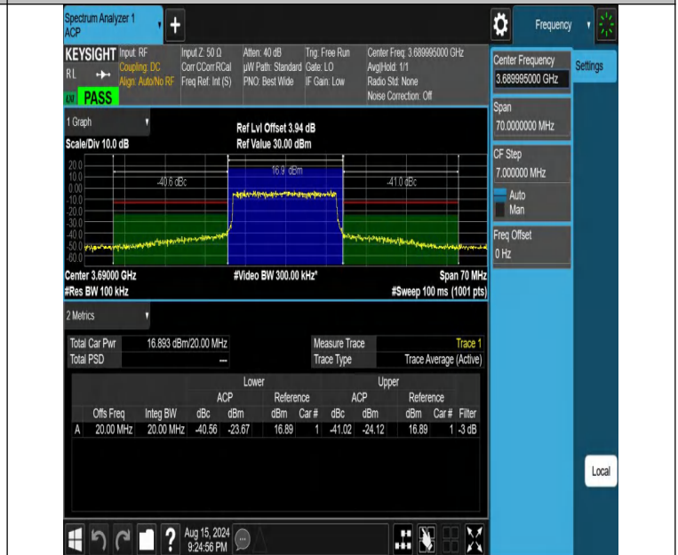
NTNV-DC_13A_n48A-PC3-30-5+20-M+H-N/A-N/A-DFT-256QAM-Outer_Full-PASS
