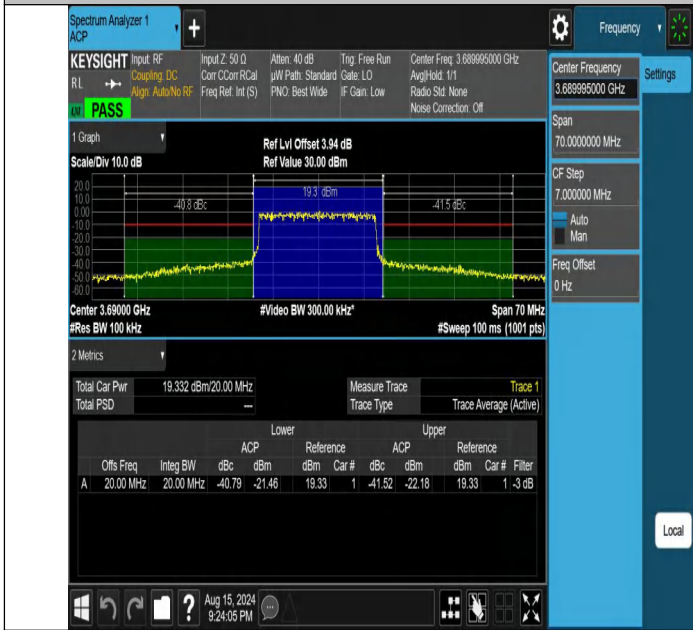
NTNV-DC_13A_n48A-PC3-30-5+20-M+H-N/A-N/A-DFT-16QAM-Outer_Full-PASS
