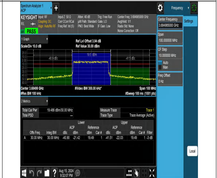
NTNV-DC_13A_n48A-PC3-30-5+30-M+H-N/A-N/A-DFT-16QAM-Ou ter_Full-PASS
