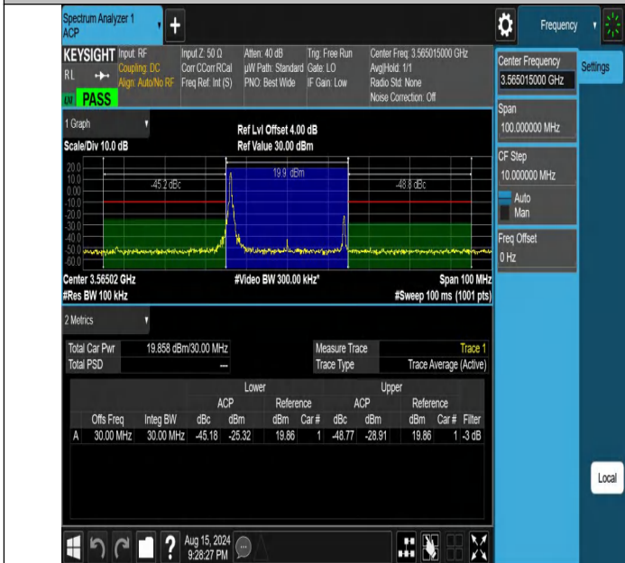
NTNV-DC_13A_n48A-PC3-30-5+30-M+L-N/A-N/A-DFT-64QAM-Ed ge_1RB_Left-PASS
