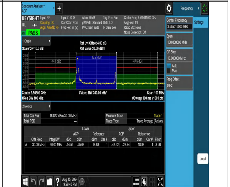
NTNV-DC_13A_n48A-PC3-30-5+30-M+L-N/A-N/A-CP-16QAM-Edg e_1RB_Left-PASS
