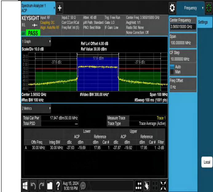
NTNV-DC_13A_n48A-PC3-30-5+30-M+L-N/A-N/A-CP-64QAM-Out er_Full-PASS
