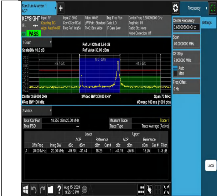
NTNV-DC_13A_n48A-PC3-30-5+20-M+H-N/A-N/A-CP-QPSK-Edge_1RB_Right-PASS
