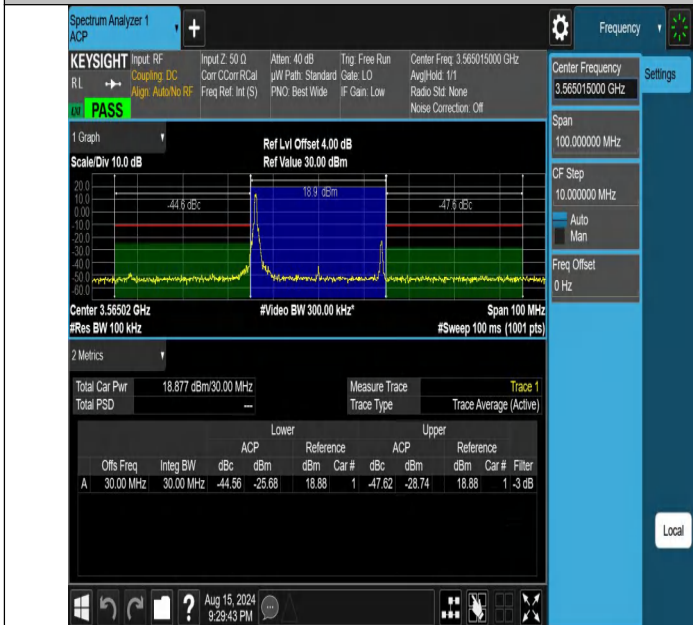
NTNV-DC_13A_n48A-PC3-30-5+30-M+L-N/A-N/A-CP-16QAM-Edg e_1RB_Left-PASS
