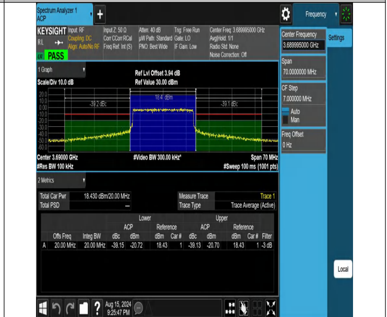
NTNV-DC_13A_n48A-PC3-30-5+20-M+H-N/A-N/A-CP-16QAM-Out_er_Full-PASS
