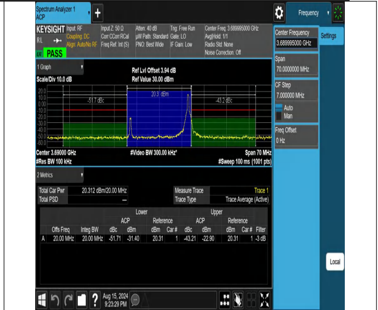
NTNV-DC_13A_n48A-PC3-30-5+20-M+H-N/A-N/A-DFT-QPSK-Edge_1RB_Right-PASS
