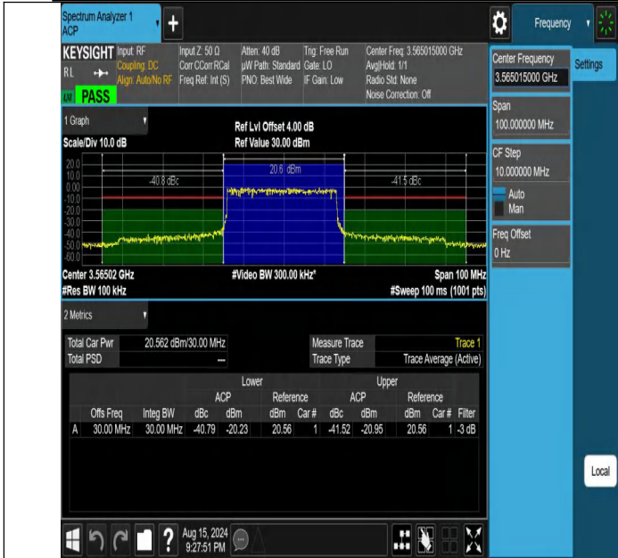
NTVN-DC_13A_n48A-PC3-30-5+30-M+L-N/A-N/A-DFT-QPSK-Out er_Full-PASS
