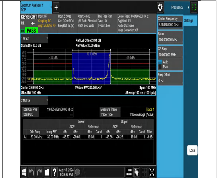
NTNV-DC_13A_n48A-PC3-30-5+30-M+H-N/A-N/A-CP-16QAM-Edge_1RB_Right-PASS
