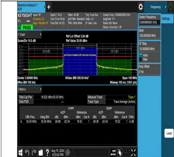
NTNV-DC_13A_n48A-PC3-30-5+30-M+H-N/A-N/A-CP-QPSK-Oute r_Full-PASS
