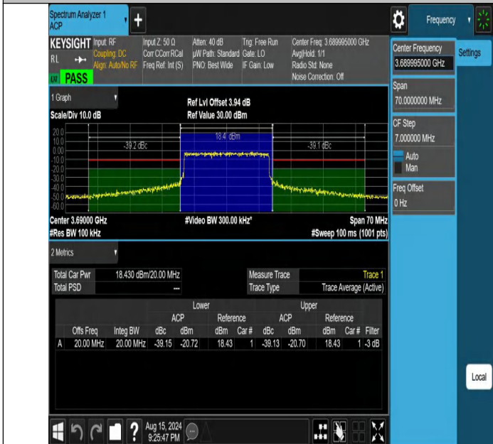
NTNV-DC_13A_n48A-PC3-30-5+20-M+H-N/A-N/A-CP-16QAM-Out_er_Full-PASS
