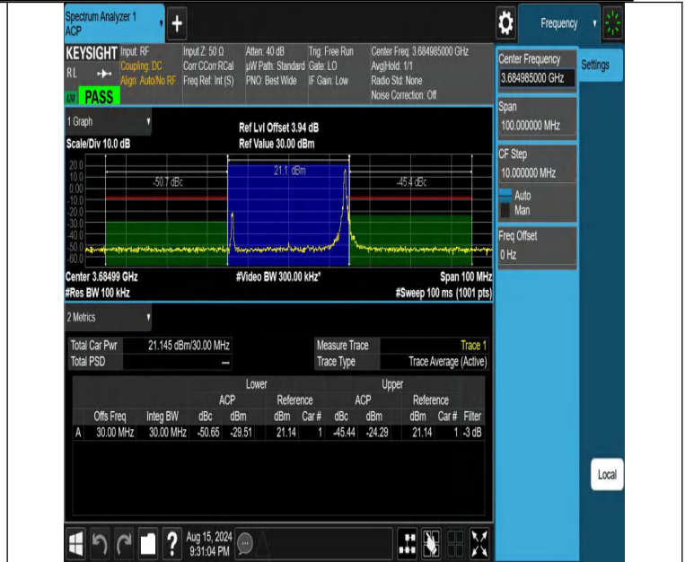
NTVN-DC_13A_n48A-PC3-30-5+30-M+H-N/A-N/A-DFT-PI2BPSK-Edge_1RB_Right-PASS
