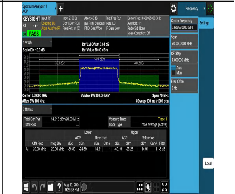
NTNV-DC_13A_n48A-PC3-30-5+20-M+H-N/A-N/A-CP-256QAM-Outer_Full-PASS
