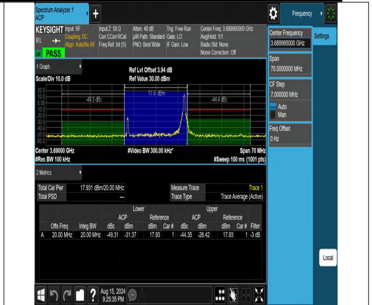
NTNV-DC_13A_n48A-PC3-30-5+20-M+H-N/A-N/A-CP-16QAM-Edge_1RB_Right-PASS
