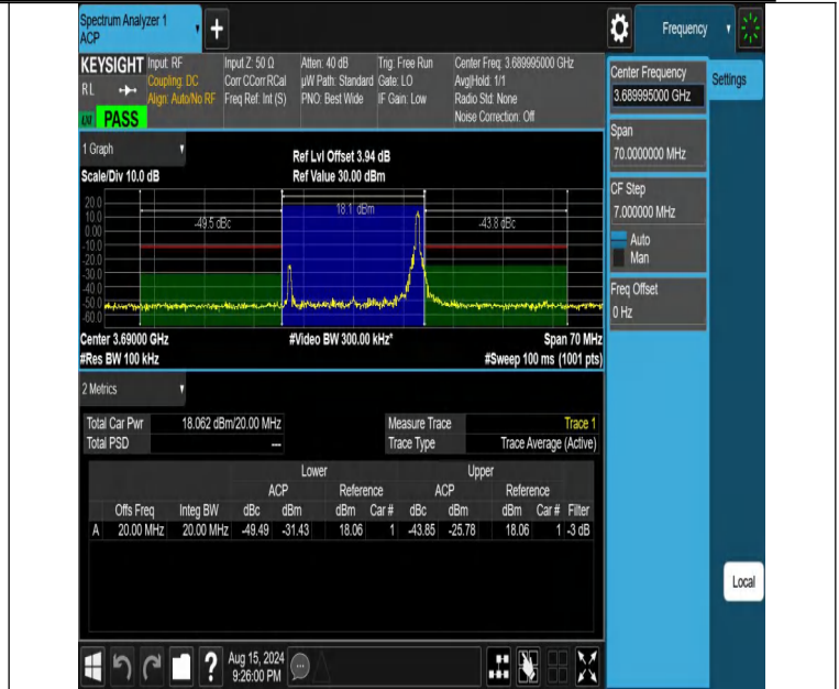
NTNV-DC_13A_n48A-PC3-30-5+20-M+H-N/A-N/A-CP-64QAM-Edge_1RB_Right-PASS
