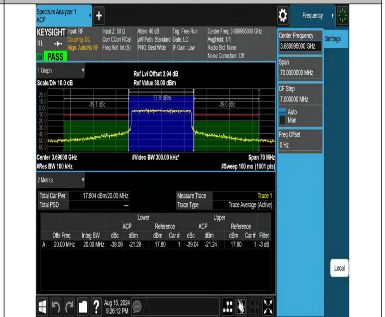
NTNV-DC_13A_n48A-PC3-30-5+20-M+H-N/A-N/A-CP-64QAM-Out_er_Full-PASS
