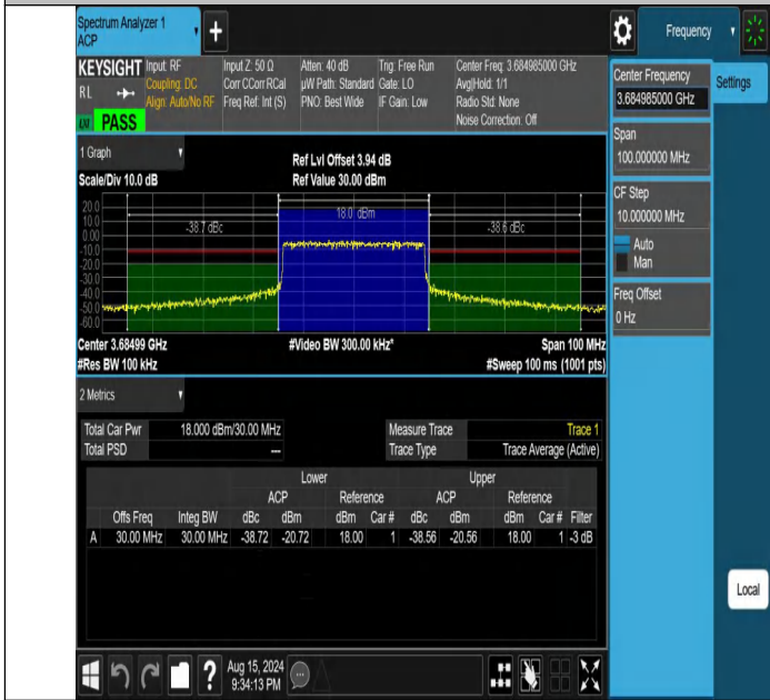
NTNV-DC_13A_n48A-PC3-30-5+30-M+H-N/A-N/A-CP-64QAM-Out_er_Full-PASS
