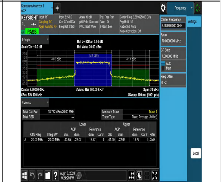
NTNV-DC_13A_n48A-PC3-30-5+20-M+H-N/A-N/A-DFT-64QAM-Outer_Full-PASS
