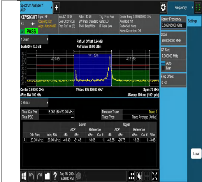
NTNV-DC_13A_n48A-PC3-30-5+20-M+H-N/A-N/A-CP-64QAM-Edge_1RB_Right-PASS
