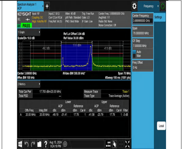
NTNV-DC_13A_n48A-PC3-30-5+20-M+H-N/A-N/A-DFT-64QAM-Edge_1RB_Right-PASS
