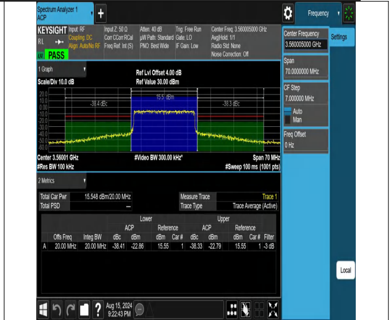
NTNV-DC_13A_n48A-PC3-30-5+20-M+L-N/A-N/A-CP-256QAM-Outer_Full-PASS
