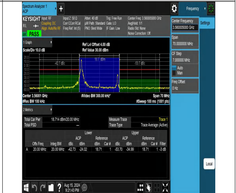
NTNV-DC_13A_n48A-PC3-30-5+20-M+L-N/A-N/A-CP-16QAM-Edg e_1RB_Left-PASS
