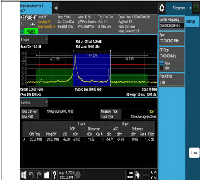
NTNV-DC_13A_n48A-PC3-30-5+20-M+L-N/A-N/A-DFT-16QAM-Edge_1RB_Left-PASS
