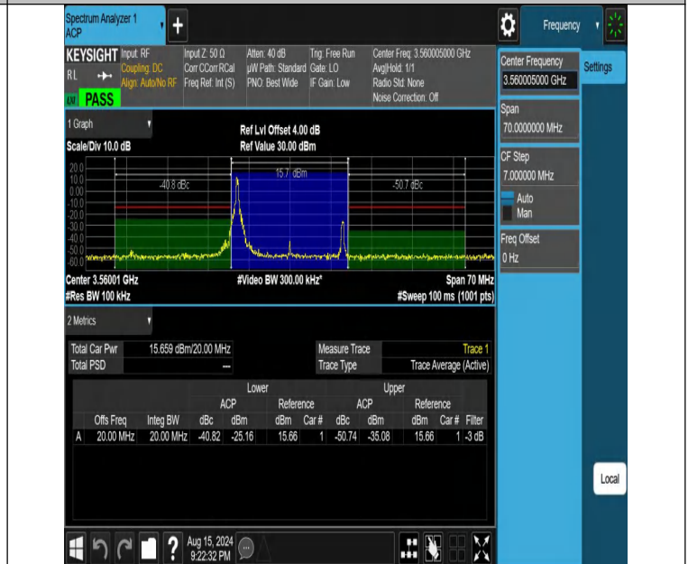
NTNV-DC_13A_n48A-PC3-30-5+20-M+L-N/A-N/A-CP-256QAM-Edge_1RB_Left-PASS
