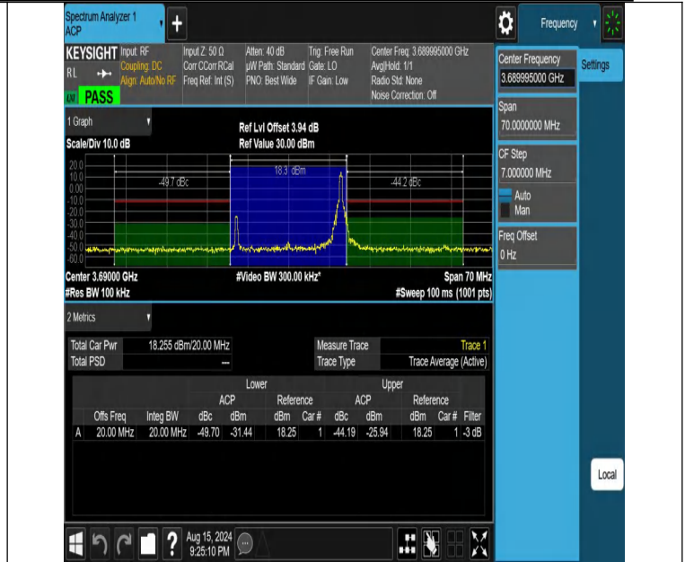
NTNV-DC_13A_n48A-PC3-30-5+20-M+H-N/A-N/A-CP-QPSK-Edge_1RB_Right-PASS
