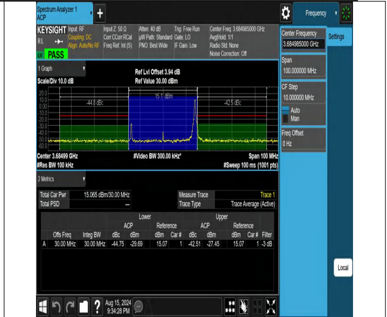
NTNV-DC_13A_n48A-PC3-30-5+30-M+H-N/A-N/A-CP-256QAM-Edge_1RB_Right-PASS
