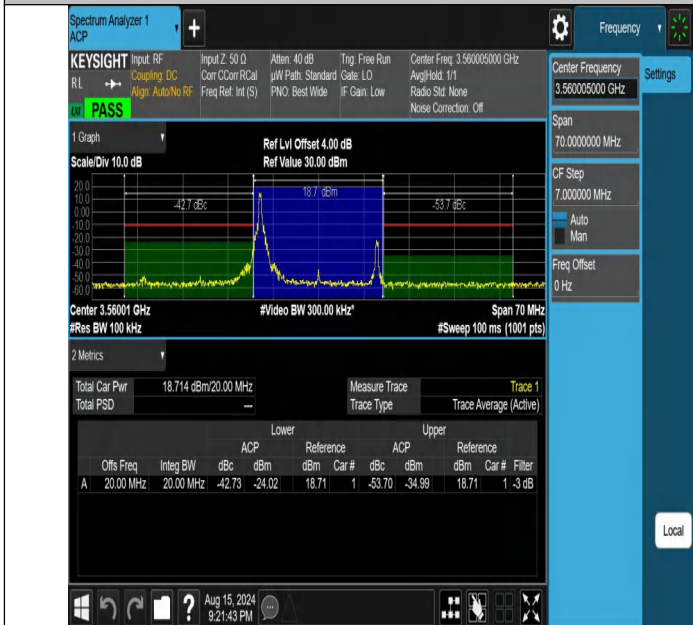
NTNV-DC_13A_n48A-PC3-30-5+20-M+L-N/A-N/A-CP-16QAM-Edg e_1RB_Left-PASS
