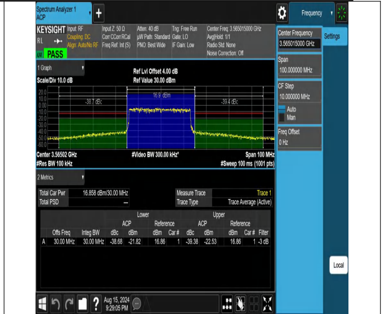
NTNV-DC_13A_n48A-PC3-30-5+30-M+L-N/A-N/A-DFT-256QAM-O uter_Full-PASS
