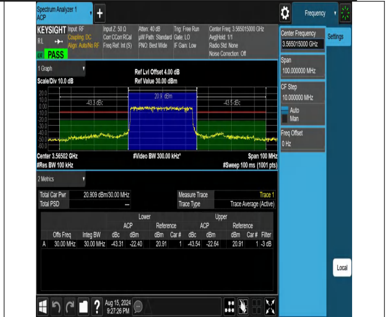
NTVN-DC_13A_n48A-PC3-30-5+30-M+L-N/A-N/A-DFT-PI2BPSK-Outer_Full-PASS
