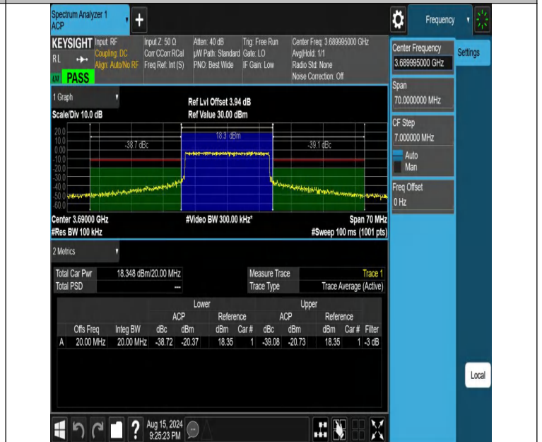
NTNV-DC_13A_n48A-PC3-30-5+20-M+H-N/A-N/A-CP-QPSK-Oute r_Full-PASS
