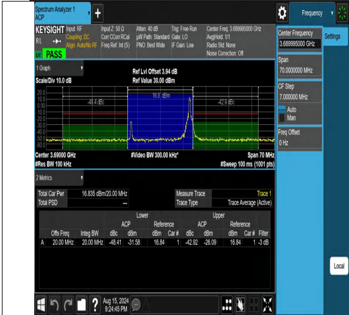
NTNV-DC_13A_n48A-PC3-30-5+20-M+H-N/A-N/A-DFT-256QAM-E dge_1RB_Right-PASS
