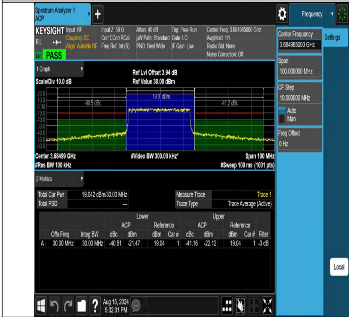
NTNV-DC_13A_n48A-PC3-30-5+30-M+H-N/A-N/A-DFT-64QAM-Outer_Full-PASS
