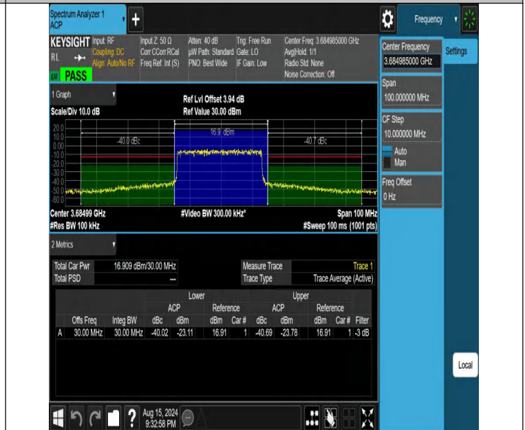
NTNV-DC_13A_n48A-PC3-30-5+30-M+H-N/A-N/A-DFT-256QAM-Outer_Full-PASS
