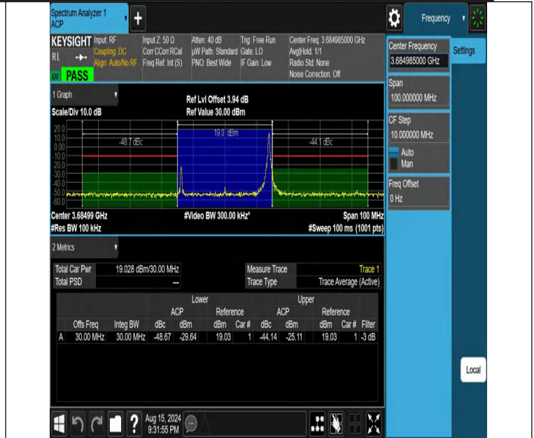
NTNV-DC_13A_n48A-PC3-30-5+30-M+H-N/A-N/A-DFT-16QAM-Edge_1RB_Right-PASS
