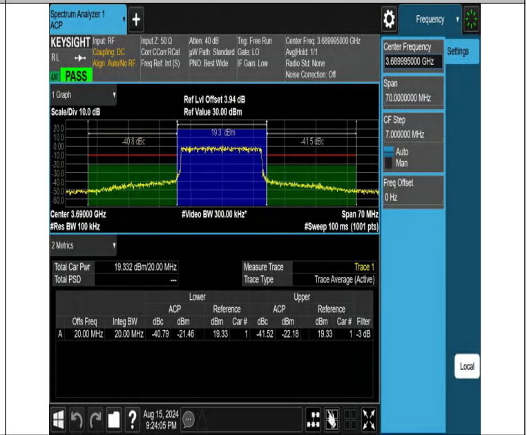
NTNV-DC_13A_n48A-PC3-30-5+20-M+H-N/A-N/A-DFT-16QAM-Outer_Full-PASS
