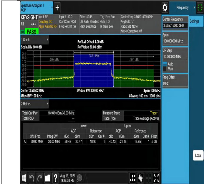
NTNV-DC_13A_n48A-PC3-30-5+30-M+L-N/A-N/A-DFT-64QAM-Ou ter_Full-PASS
