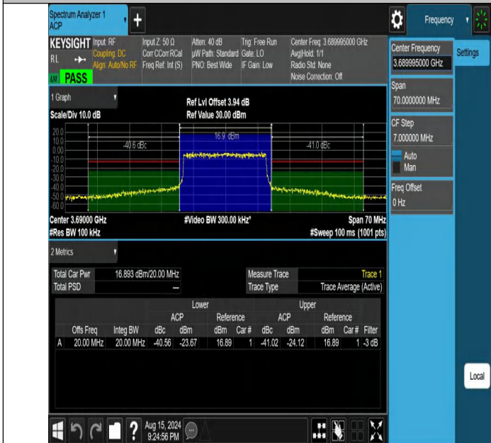
NTNV-DC_13A_n48A-PC3-30-5+20-M+H-N/A-N/A-DFT-256QAM-Outer_Full-PASS
