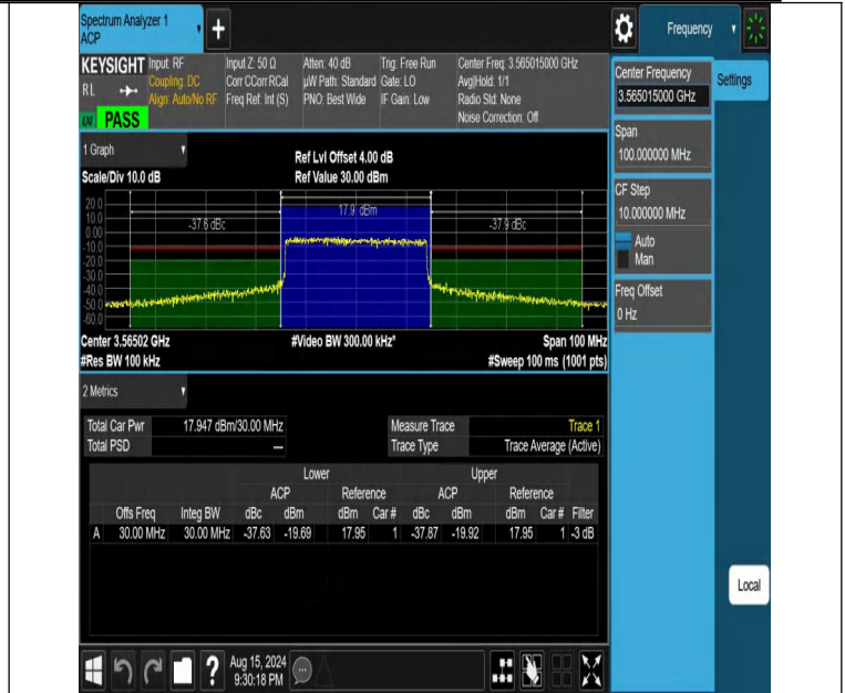
NTNV-DC_13A_n48A-PC3-30-5+30-M+L-N/A-N/A-CP-64QAM-Out er_Full-PASS
