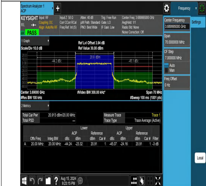
NTNV-DC_13A_n48A-PC3-30-5+20-M+H-N/A-N/A-DFT-PI2BPSK-Outer_Full-PASS
