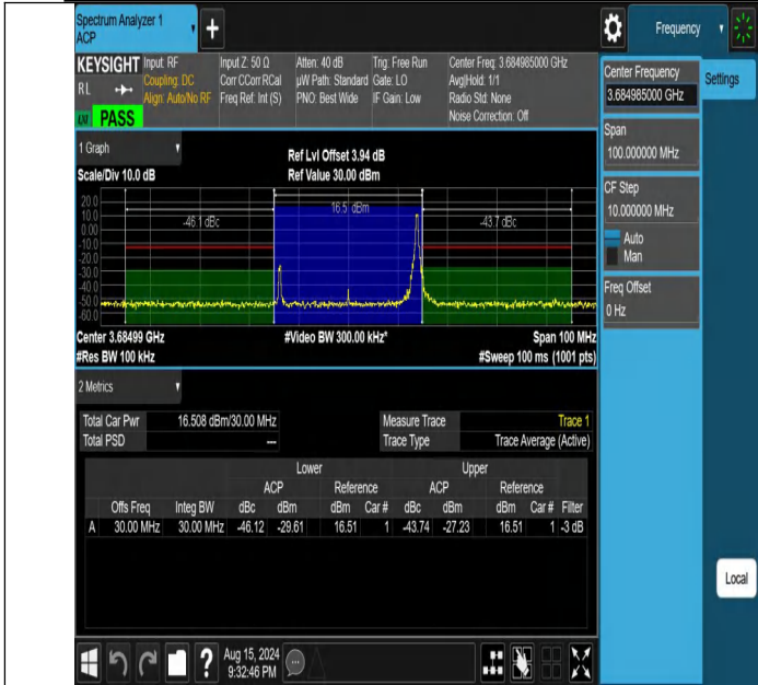
NTNV-DC_13A_n48A-PC3-30-5+30-M+H-N/A-N/A-DFT-256QAM-E dge_1RB_Right-PASS
