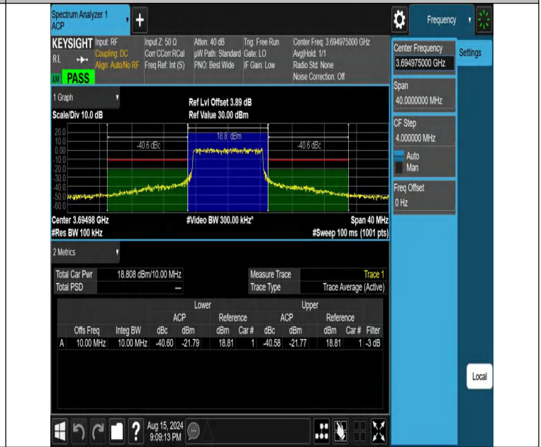
NTNV-DC_13A_n48A-PC3-30-5+10-M+H-N/A-N/A-DFT-64QAM-Outer_Full-PASS
