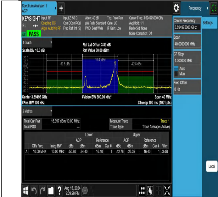
NTNV-DC_13A_n48A-PC3-30-5+10-M+H-N/A-N/A-DFT-256QAM-E dge_1RB_Right-PASS
