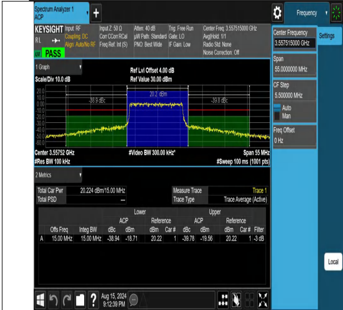
NTNV-DC_13A_n48A-PC3-30-5+15-M+L-N/A-N/A-DFT-16QAM-Outer_Full-PASS
