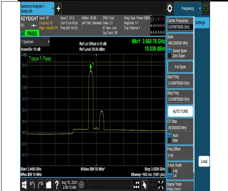
NTNV-DC_13A_n48A-PC3-30-5+40-M+H-N/A-N/A-CP-256QAM-E dge_1RB_Left-3439.975-3919.975-PASS
