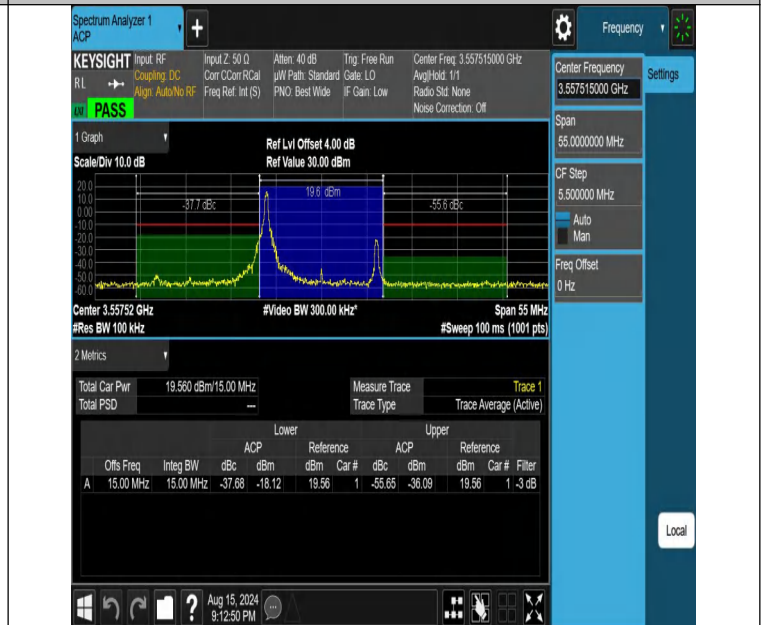
NTNV-DC_13A_n48A-PC3-30-5+15-M+L-N/A-N/A-DFT-64QAM-Edge_1RB_Left-PASS
