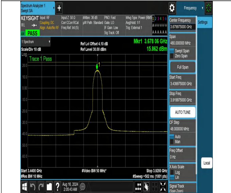
NTNV-DC_13A_n48A-PC3-30-5+40-M+H-N/A-N/A-CP-64QAM-Inner_Full-3439.975-3919.975-PASS
