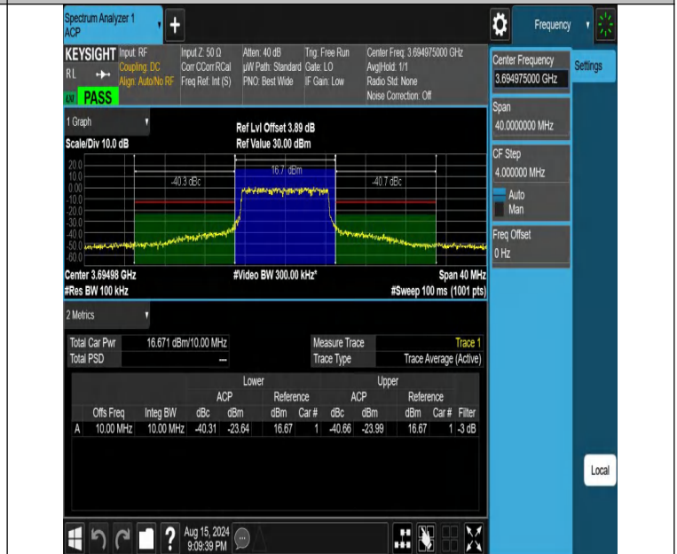
NTNV-DC_13A_n48A-PC3-30-5+10-M+H-N/A-N/A-DFT-256QAM-Outer_Full-PASS
