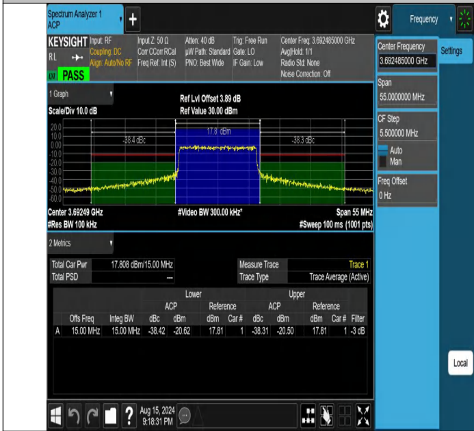
NTNV-DC_13A_n48A-PC3-30-5+15-M+H-N/A-N/A-CP-64QAM-Out_er_Full-PASS
