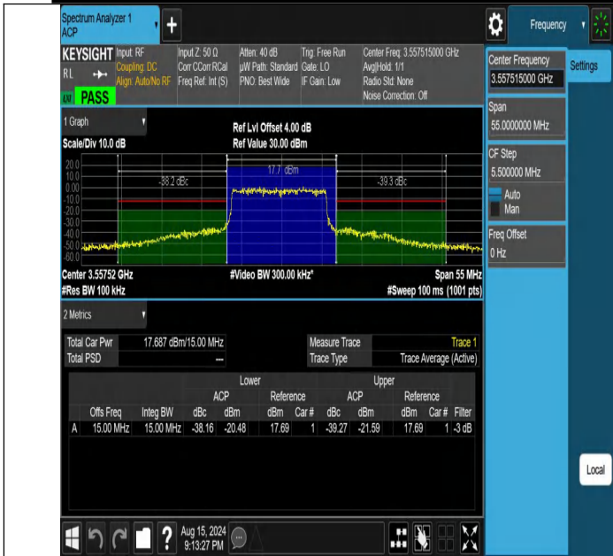
NTNV-DC_13A_n48A-PC3-30-5+15-M+L-N/A-N/A-DFT-256QAM-Outer_Full-PASS
