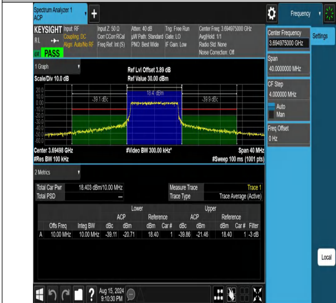
NTNV-DC_13A_n48A-PC3-30-5+10-M+H-N/A-N/A-CP-16QAM-Out er_Full-PASS
