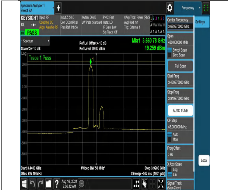
NTNV-DC_13A_n48A-PC3-30-5+40-M+H-N/A-N/A-CP-64QAM-Edge_1RB_Left-3439.975-3919.975-PASS
