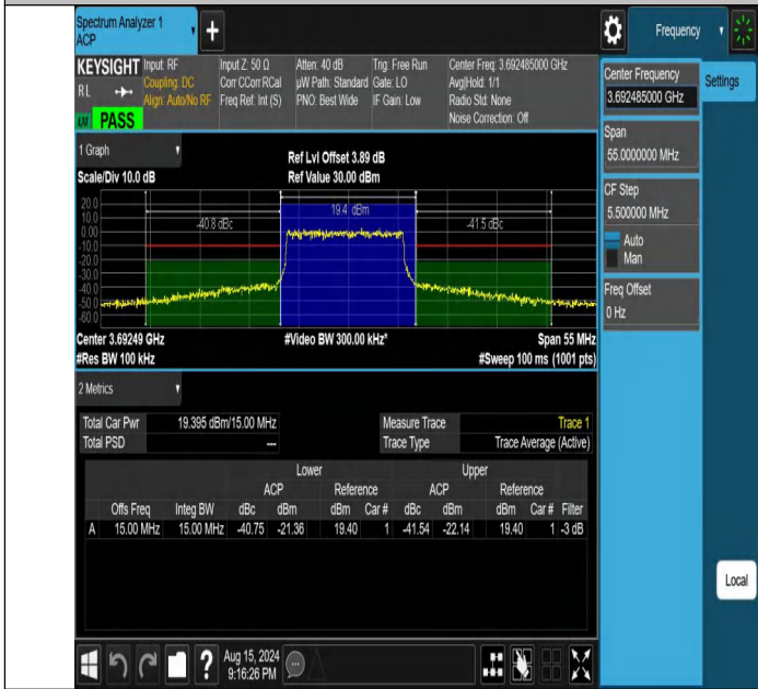
NTNV-DC_13A_n48A-PC3-30-5+15-M+H-N/A-N/A-DFT-16QAM-Outer_Full-PASS
