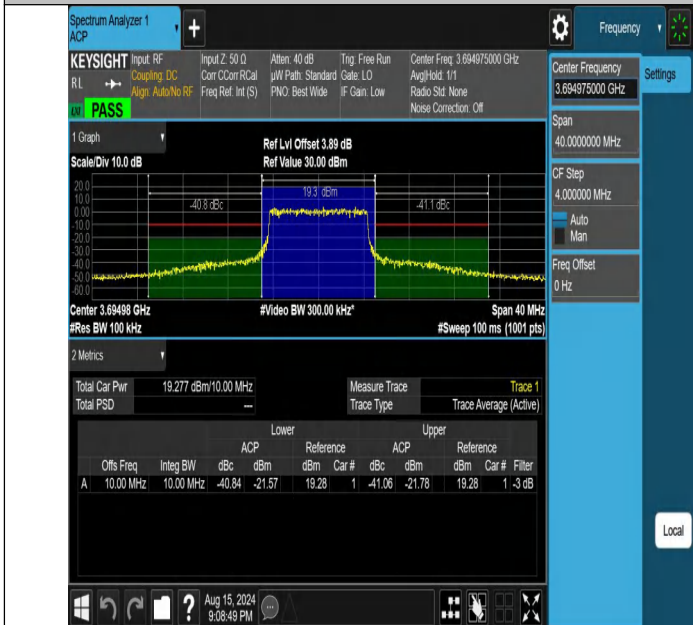
NTNV-DC_13A_n48A-PC3-30-5+10-M+H-N/A-N/A-DFT-16QAM-Outer_Full-PASS
