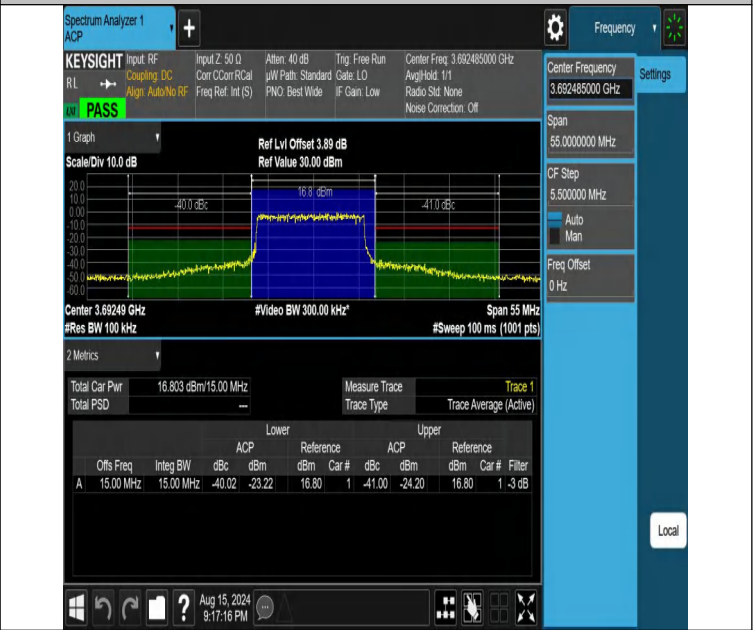
NTNV-DC_13A_n48A-PC3-30-5+15-M+H-N/A-N/A-DFT-256QAM-Outer_Full-PASS
