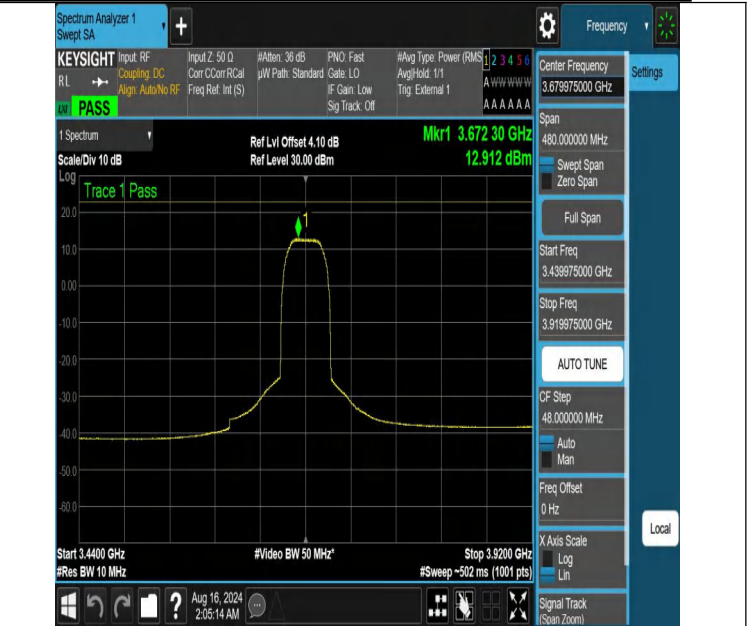
NTNV-DC_13A_n48A-PC3-30-5+40-M+H-N/A-N/A-CP-64QAM-Outer_Full-3439.975-3919.975-PASS
