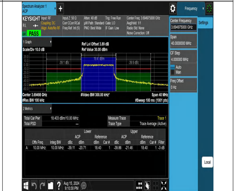
NTNV-DC_13A_n48A-PC3-30-5+10-M+H-N/A-N/A-CP-16QAM-Out er_Full-PASS
