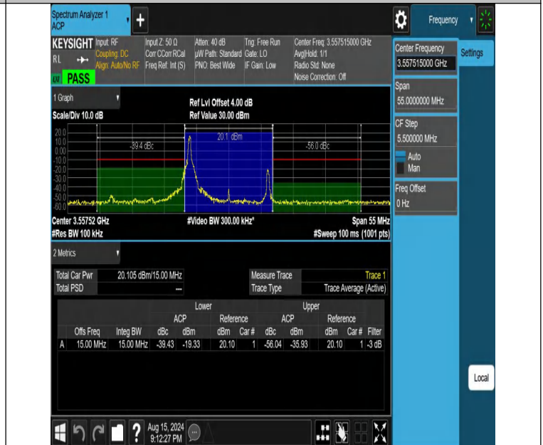
NTNV-DC_13A_n48A-PC3-30-5+15-M+L-N/A-N/A-DFT-16QAM-Ed ge_1RB_Left-PASS
