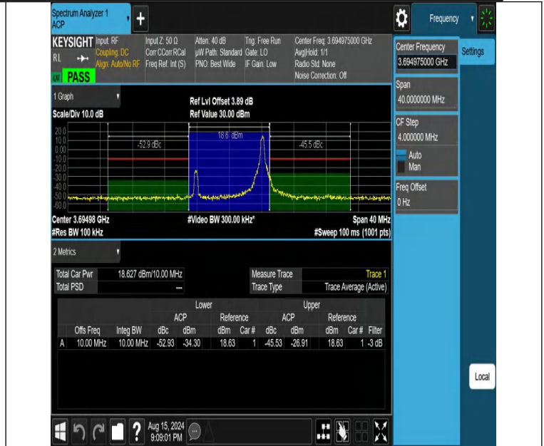
NTNV-DC_13A_n48A-PC3-30-5+10-M+H-N/A-N/A-DFT-64QAM-Edge_1RB_Right-PASS
