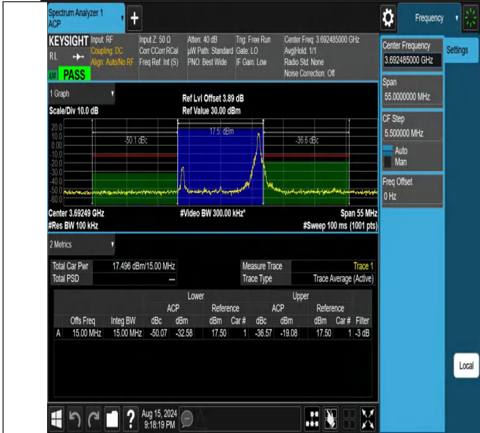
NTNV-DC_13A_n48A-PC3-30-5+15-M+H-N/A-N/A-CP-64QAM-Edge_1RB_Right-PASS
