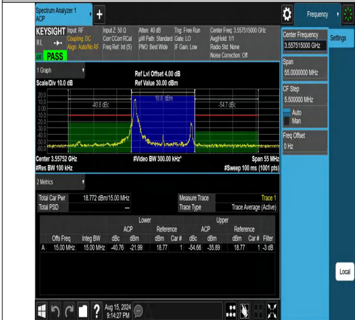
NTNV-DC_13A_n48A-PC3-30-5+15-M+L-N/A-N/A-CP-64QAM-Edge_1RB_Left-PASS
