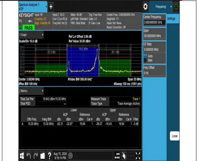
NTNV-DC_13A_n48A-PC3-30-5+15-M+H-N/A-N/A-DFT-16QAM-Edge_1RB_Right-PASS
