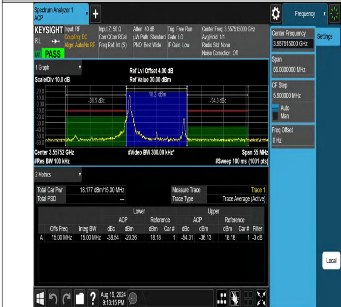
NTNV-DC_13A_n48A-PC3-30-5+15-M+L-N/A-N/A-DFT-256QAM-E dge_1RB_Left-PASS
