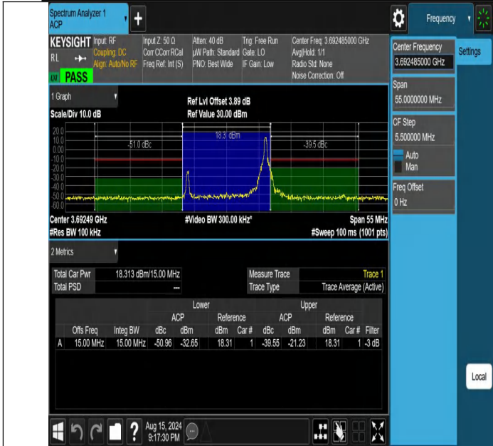
NTNV-DC_13A_n48A-PC3-30-5+15-M+H-N/A-N/A-CP-QPSK-Edge_1RB_Right-PASS
