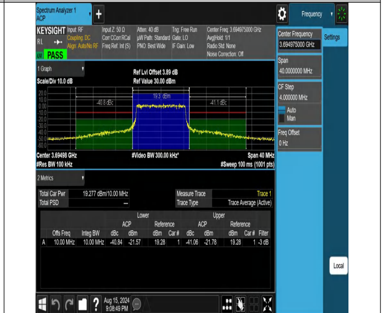
NTNV-DC_13A_n48A-PC3-30-5+10-M+H-N/A-N/A-DFT-16QAM-Outer_Full-PASS
