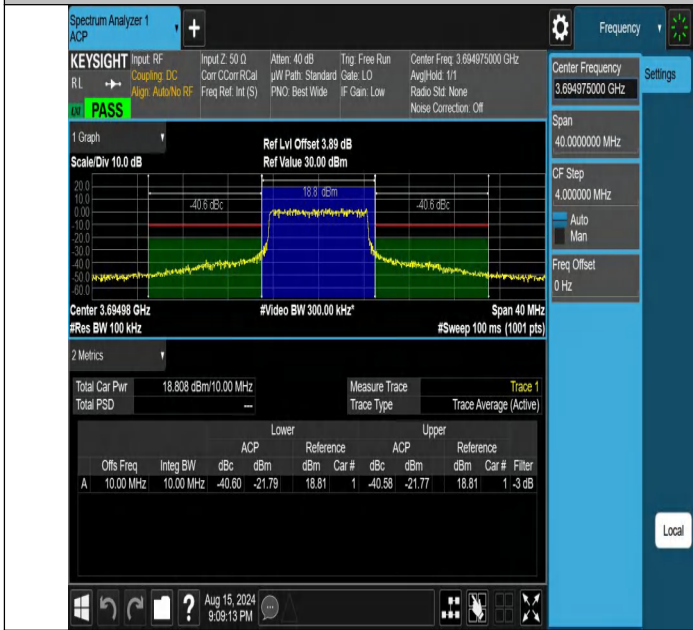
NTNV-DC_13A_n48A-PC3-30-5+10-M+H-N/A-N/A-DFT-64QAM-Outer_Full-PASS
