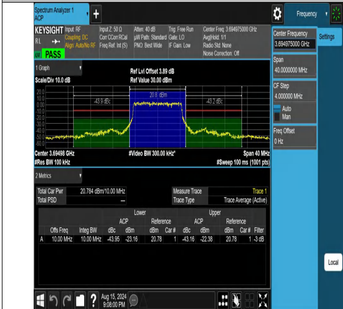
NTNV-DC_13A_n48A-PC3-30-5+10-M+H-N/A-N/A-DFT-PI2BPSK-Outer_Full-PASS
