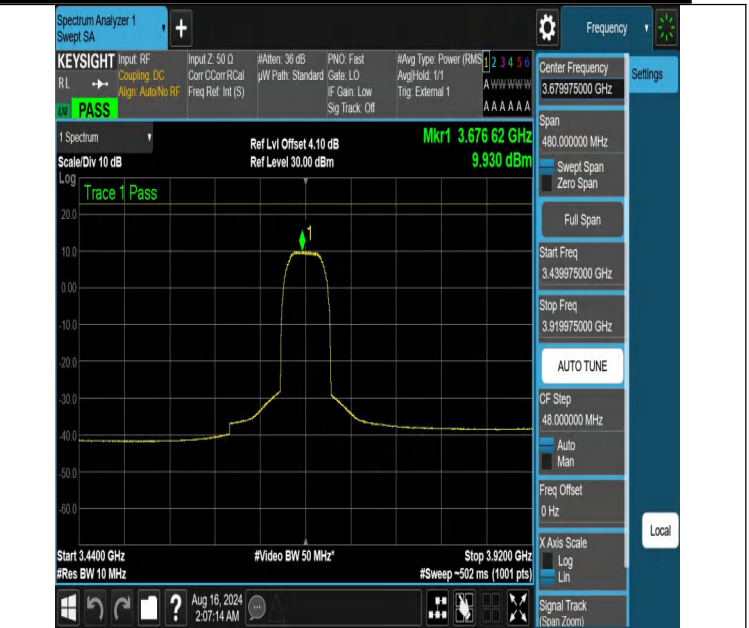
NTNV-DC_13A_n48A-PC3-30-5+40-M+H-N/A-N/A-CP-256QAM-Ou ter_Full-3439.975-3919.975-PASS
