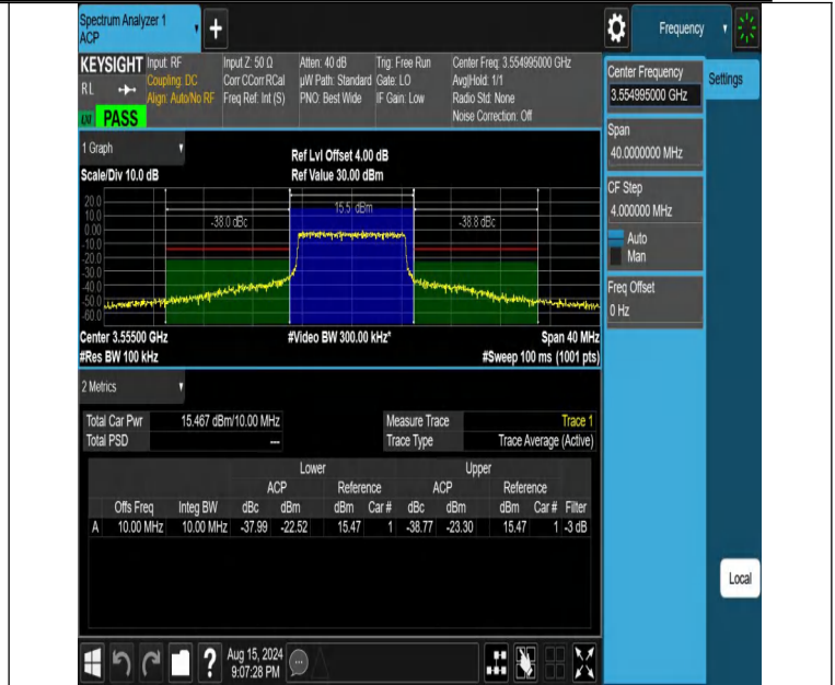
NTNV-DC_13A_n48A-PC3-30-5+10-M+L-N/A-N/A-CP-256QAM-Outer_Full-PASS
