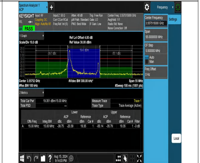
NTNV-DC_13A_n48A-PC3-30-5+15-M+L-N/A-N/A-CP-16QAM-Edg e_1RB_Left-PASS
