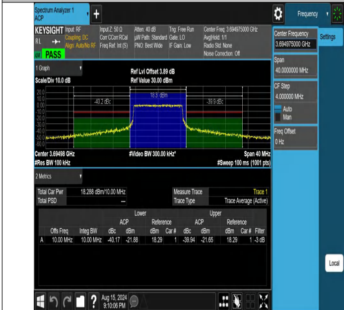
NTNV-DC_13A_n48A-PC3-30-5+10-M+H-N/A-N/A-CP-QPSK-Oute r_Full-PASS
