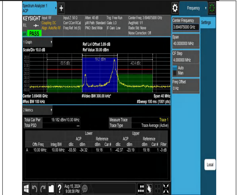
NTNV-DC_13A_n48A-PC3-30-5+10-M+H-N/A-N/A-DFT-16QAM-Edge_1RB_Right-PASS
