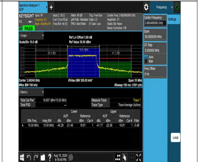
NTNV-DC_13A_n48A-PC3-30-5+15-M+H-N/A-N/A-DFT-64QAM-Outer_Full-PASS
