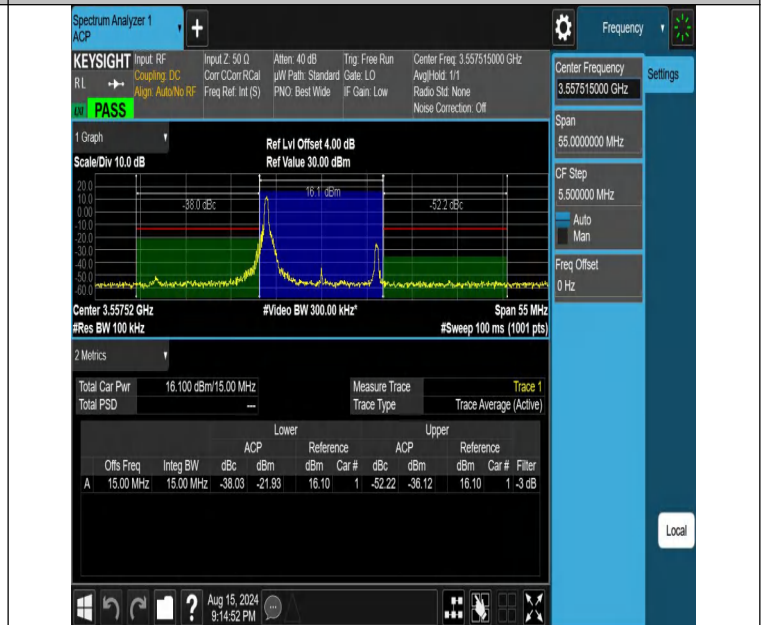
NTNV-DC_13A_n48A-PC3-30-5+15-M+L-N/A-N/A-CP-256QAM-Edge_1RB_Left-PASS
