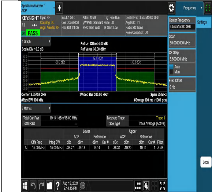
NTNV-DC_13A_n48A-PC3-30-5+15-M+L-N/A-N/A-CP-16QAM-Out er_Full-PASS
