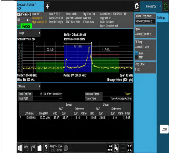
NTNV-DC_13A_n48A-PC3-30-5+10-M+H-N/A-N/A-CP-16QAM-Edge_1RB_Right-PASS
