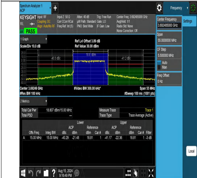
NTNV-DC_13A_n48A-PC3-30-5+15-M+H-N/A-N/A-DFT-64QAM-Outer_Full-PASS
