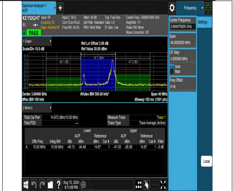
NTNV-DC_13A_n48A-PC3-30-5+10-M+H-N/A-N/A-CP-256QAM-Edge_1RB_Right-PASS
