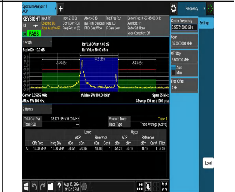
NTNV-DC_13A_n48A-PC3-30-5+15-M+L-N/A-N/A-DFT-256QAM-E dge_1RB_Left-PASS
