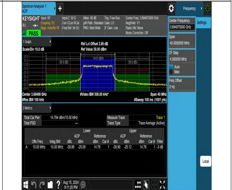
NTNV-DC_13A_n48A-PC3-30-5+10-M+H-N/A-N/A-CP-256QAM-Outer_Full-PASS
