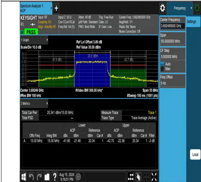
NTNV-DC_13A_n48A-PC3-30-5+15-M+H-N/A-N/A-DFT-QPSK-Out_er_Full-PASS
