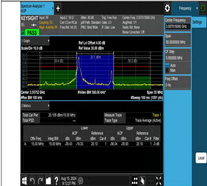
NTNV-DC_13A_n48A-PC3-30-5+15-M+L-N/A-N/A-DFT-16QAM-Ed ge_1RB_Left-PASS
