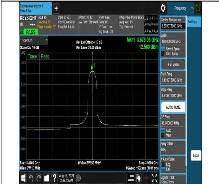
NTNV-DC_13A_n48A-PC3-30-5+40-M+H-N/A-N/A-CP-256QAM-In ner_Full-3439.975-3919.975-PASS
