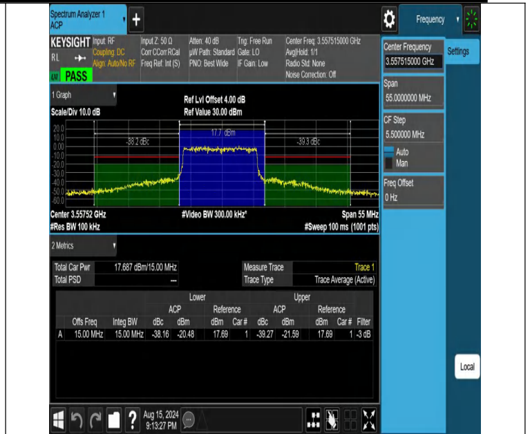
NTNV-DC_13A_n48A-PC3-30-5+15-M+L-N/A-N/A-DFT-256QAM-Outer_Full-PASS
