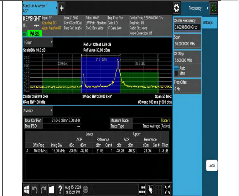
NTNV-DC_13A_n48A-PC3-30-5+15-M+H-N/A-N/A-DFT-PI2BPSK-Edge_1RB_Right-PASS
