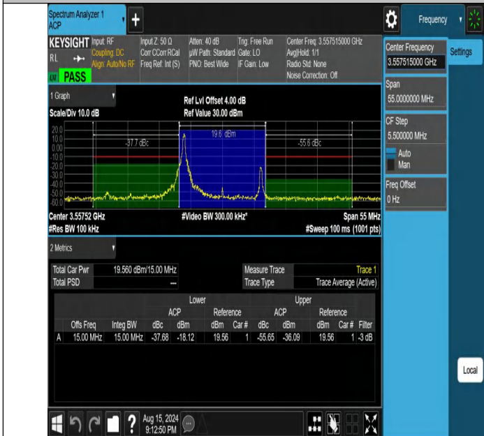
NTNV-DC_13A_n48A-PC3-30-5+15-M+L-N/A-N/A-DFT-64QAM-Edge_1RB_Left-PASS
