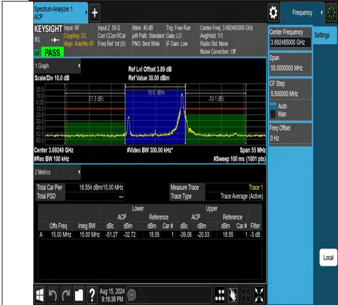
NTNV-DC_13A_n48A-PC3-30-5+15-M+H-N/A-N/A-DFT-64QAM-Edge_1RB_Right-PASS
