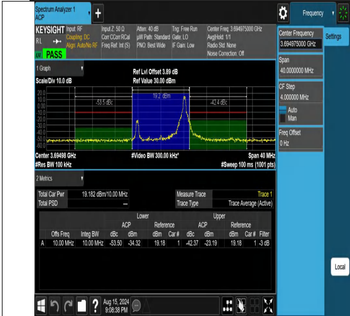
NTNV-DC_13A_n48A-PC3-30-5+10-M+H-N/A-N/A-DFT-16QAM-Edge_1RB_Right-PASS
