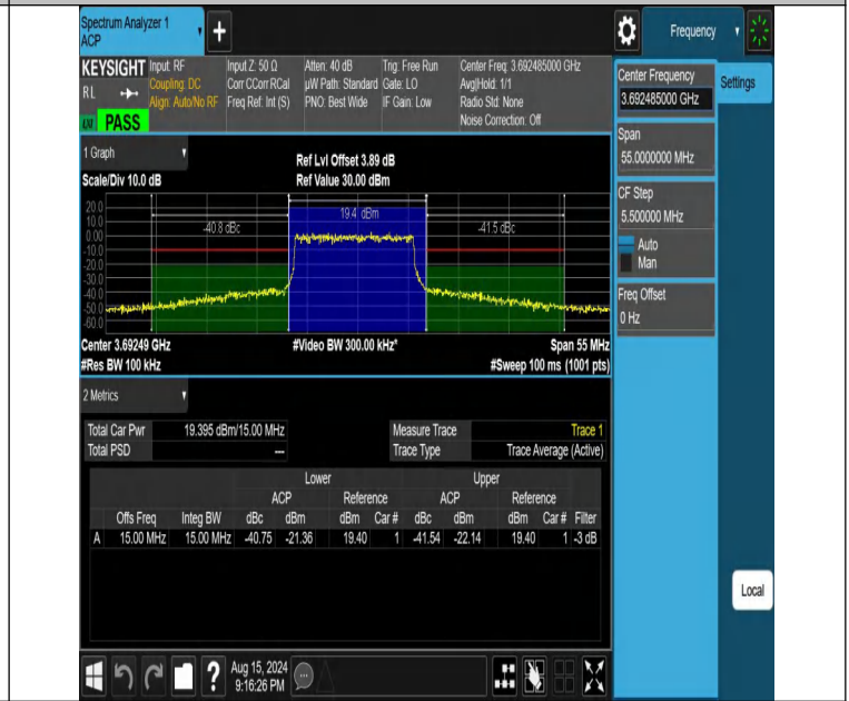
NTNV-DC_13A_n48A-PC3-30-5+15-M+H-N/A-N/A-DFT-16QAM-Outer_Full-PASS
