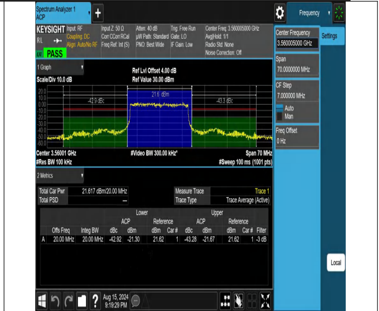
NTNV-DC_13A_n48A-PC3-30-5+20-M+L-N/A-N/A-DFT-PI2BPSK-Outer_Full-PASS
