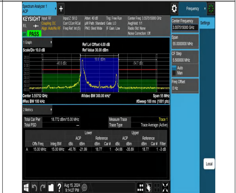
NTNV-DC_13A_n48A-PC3-30-5+15-M+L-N/A-N/A-CP-64QAM-Edge_1RB_Left-PASS
