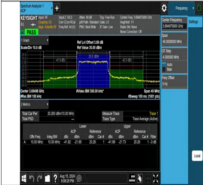
NTNV-DC_13A_n48A-PC3-30-5+10-M+H-N/A-N/A-DFT-QPSK-Out_er_Full-PASS
