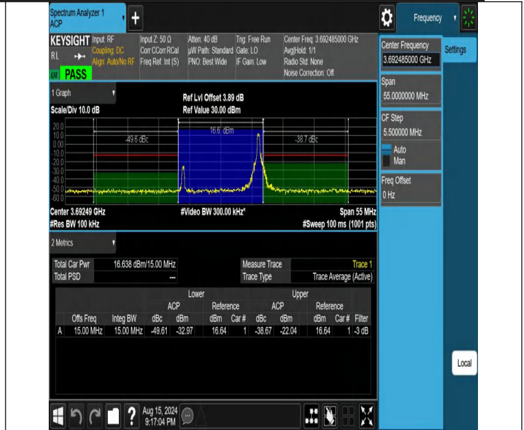
NTNV-DC_13A_n48A-PC3-30-5+15-M+H-N/A-N/A-DFT-256QAM-E dge_1RB_Right-PASS
