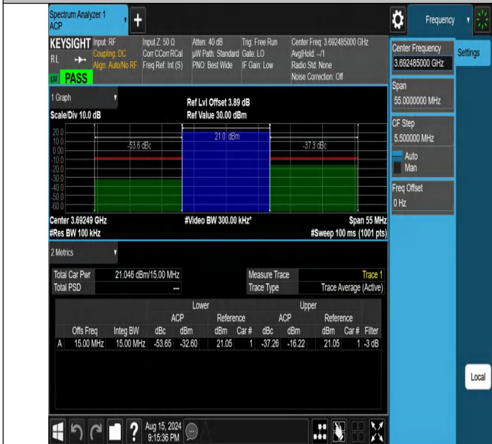
NTNV-DC_13A_n48A-PC3-30-5+15-M+H-N/A-N/A-DFT-PI2BPSK-Outer_Full-PASS
