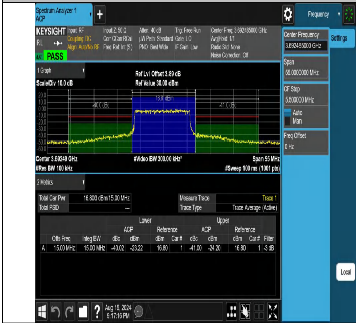
NTNV-DC_13A_n48A-PC3-30-5+15-M+H-N/A-N/A-DFT-256QAM-Outer_Full-PASS
