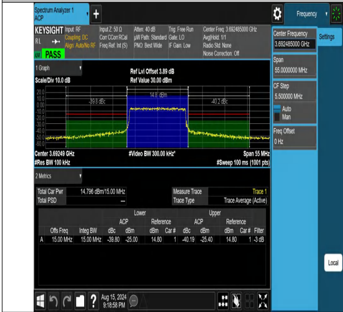
NTNV-DC_13A_n48A-PC3-30-5+15-M+H-N/A-N/A-CP-256QAM-Outer_Full-PASS
