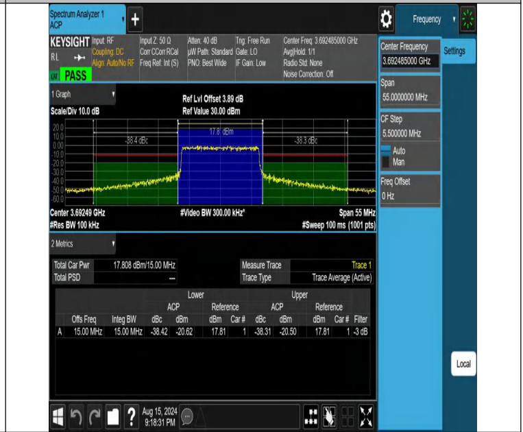
NTNV-DC_13A_n48A-PC3-30-5+15-M+H-N/A-N/A-CP-64QAM-Out_er_Full-PASS
