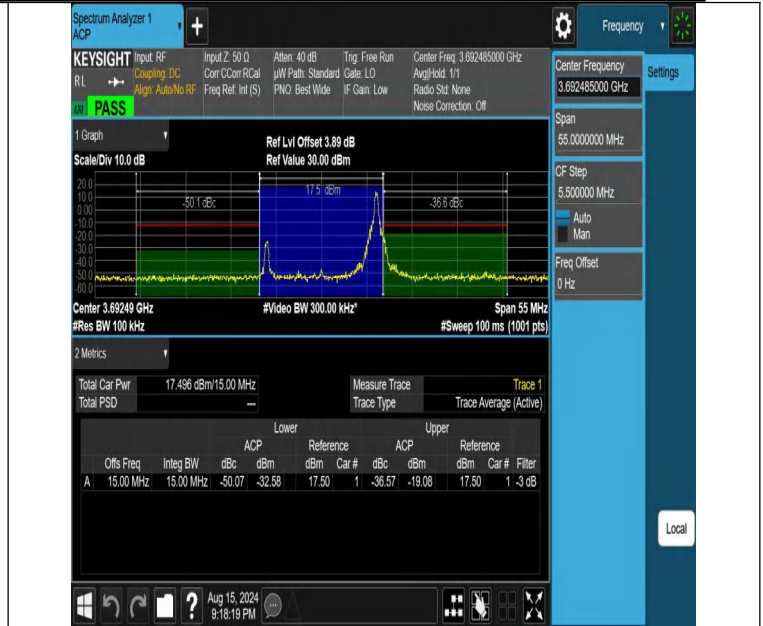
NTNV-DC_13A_n48A-PC3-30-5+15-M+H-N/A-N/A-CP-64QAM-Edge_1RB_Right-PASS
