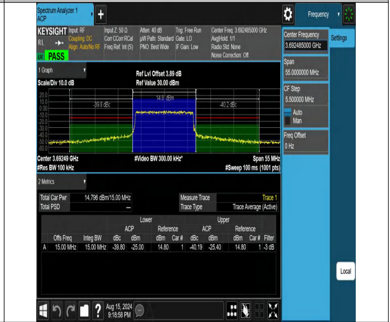
NTNV-DC_13A_n48A-PC3-30-5+15-M+H-N/A-N/A-CP-256QAM-Outer_Full-PASS
