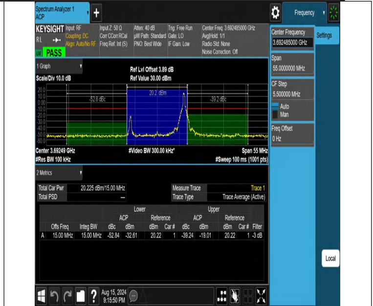
NTNV-DC_13A_n48A-PC3-30-5+15-M+H-N/A-N/A-DFT-QPSK-Edge_1RB_Right-PASS
