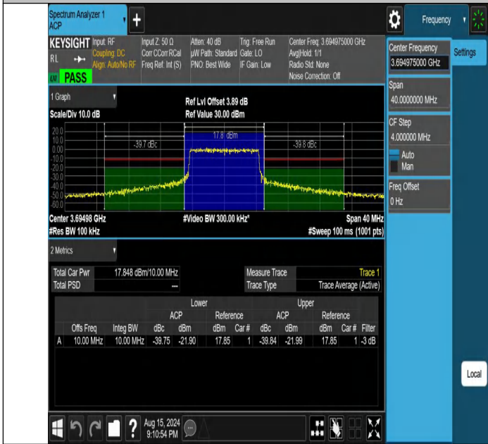
NTNV-DC_13A_n48A-PC3-30-5+10-M+H-N/A-N/A-CP-64QAM-Out_er_Full-PASS
