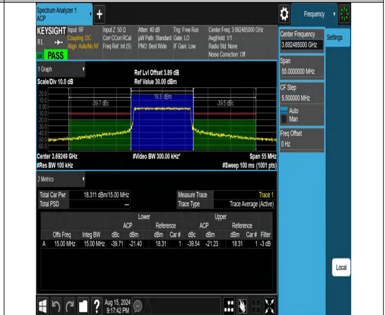
NTNV-DC_13A_n48A-PC3-30-5+15-M+H-N/A-N/A-CP-QPSK-Oute r_Full-PASS
