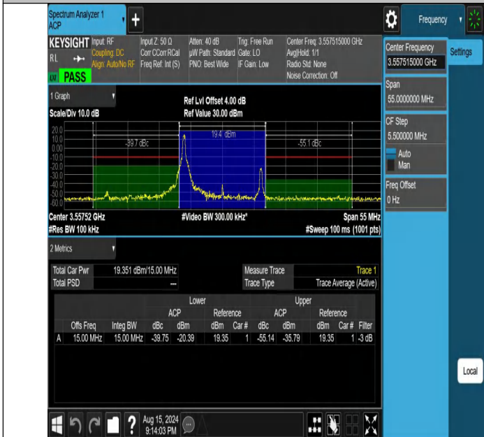
NTNV-DC_13A_n48A-PC3-30-5+15-M+L-N/A-N/A-CP-16QAM-Edg e_1RB_Left-PASS
