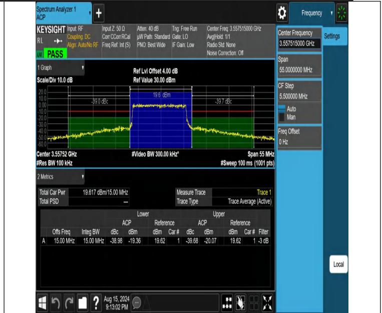
NTNV-DC_13A_n48A-PC3-30-5+15-M+L-N/A-N/A-DFT-64QAM-Ou ter_Full-PASS
