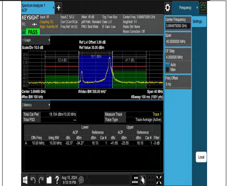
NTNV-DC_13A_n48A-PC3-30-5+10-M+H-N/A-N/A-CP-16QAM-Edge_1RB_Right-PASS
