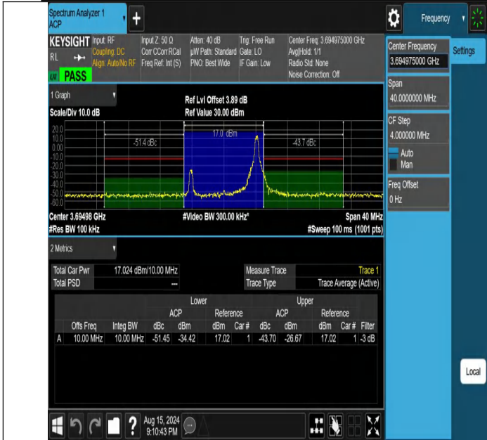
NTNV-DC_13A_n48A-PC3-30-5+10-M+H-N/A-N/A-CP-64QAM-Edge_1RB_Right-PASS
