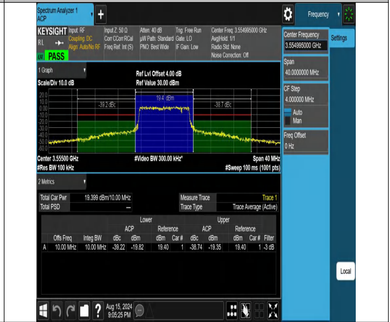
NTNV-DC_13A_n48A-PC3-30-5+10-M+L-N/A-N/A-DFT-64QAM-Outer_Full-PASS
