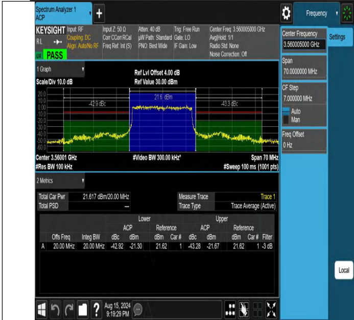
NTNV-DC_13A_n48A-PC3-30-5+20-M+L-N/A-N/A-DFT-PI2BPSK-Outer_Full-PASS
