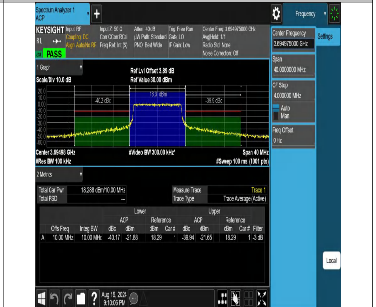
NTNV-DC_13A_n48A-PC3-30-5+10-M+H-N/A-N/A-CP-QPSK-Oute r_Full-PASS
