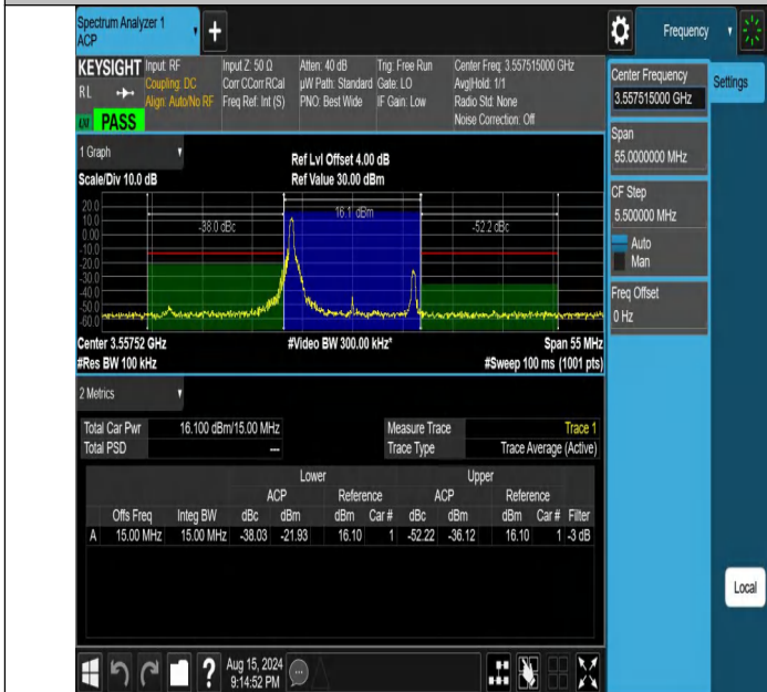
NTNV-DC_13A_n48A-PC3-30-5+15-M+L-N/A-N/A-CP-256QAM-Edge_1RB_Left-PASS
