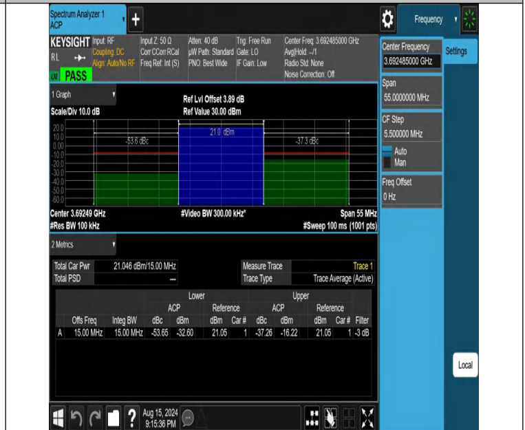
NTNV-DC_13A_n48A-PC3-30-5+15-M+H-N/A-N/A-DFT-PI2BPSK-Outer_Full-PASS
