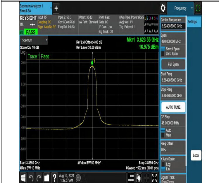
NTNV-DC_13A_n48A-PC3-30-5+40-M+M-N/A-N/A-DFT-64QAM-In ner_Full-3384.985-3864.985-PASS
