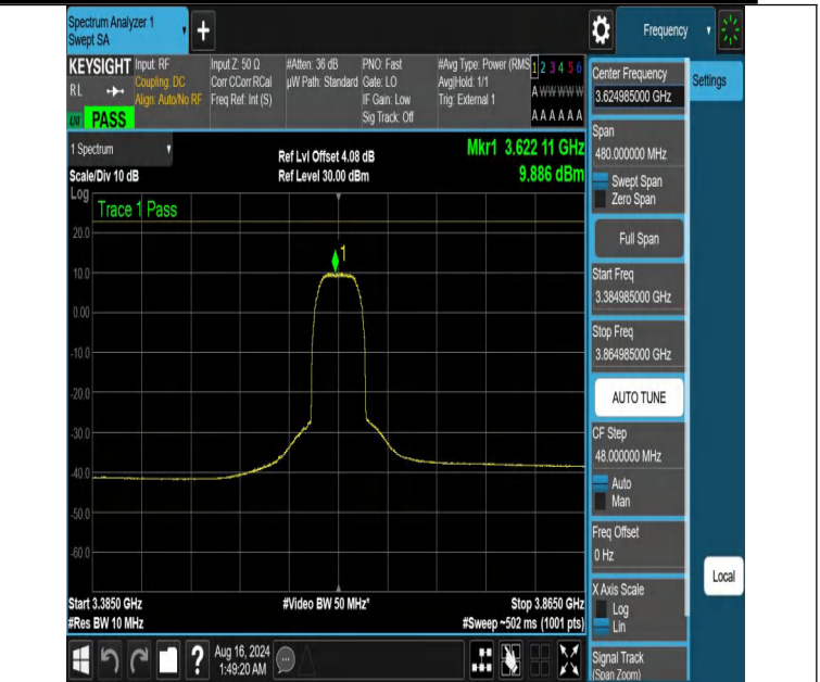
NTNV-DC_13A_n48A-PC3-30-5+40-M+M-N/A-N/A-CP-256QAM-Ou ter_Full-3384.985-3864.985-PASS
