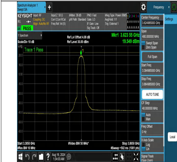
NTNV-DC_13A_n48A-PC3-30-5+40-M+M-N/A-N/A-DFT-PI2BPSK-I nner_Full-3384.985-3864.985-PASS
