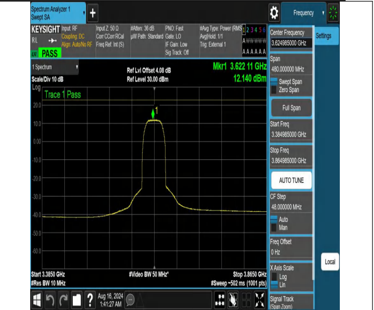
NTNV-DC_13A_n48A-PC3-30-5+40-M+M-N/A-N/A-DFT-256QAM-Outer_Full-3384.985-3864.985-PASS
