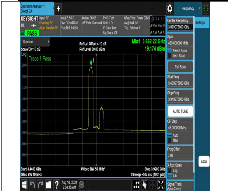
NTNV-DC_13A_n48A-PC3-30-5+40-M+H-N/A-N/A-CP-16QAM-Edge_1RB_Left-3439.975-3919.975-PASS
