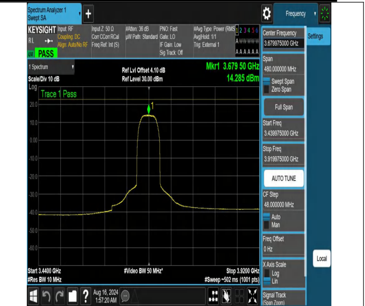
NTNV-DC_13A_n48A-PC3-30-5+40-M+H-N/A-N/A-DFT-64QAM-Ou ter_Full-3439.975-3919.975-PASS
