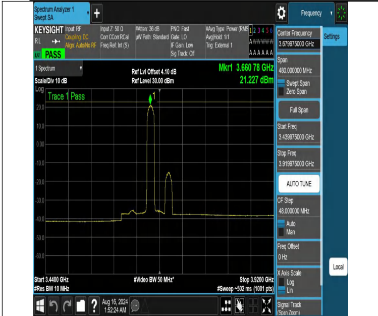
NTVN-DC_13A_n48A-PC3-30-5+40-M+H-N/A-N/A-DFT-PI2BPSK-Edge_1RB_Left-3439.975-3919.975-PASS
