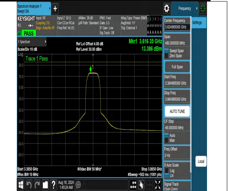
NTNV-DC_13A_n48A-PC3-30-5+40-M+M-N/A-N/A-CP-16QAM-Outer_Full-3384.985-3864.985-PASS
