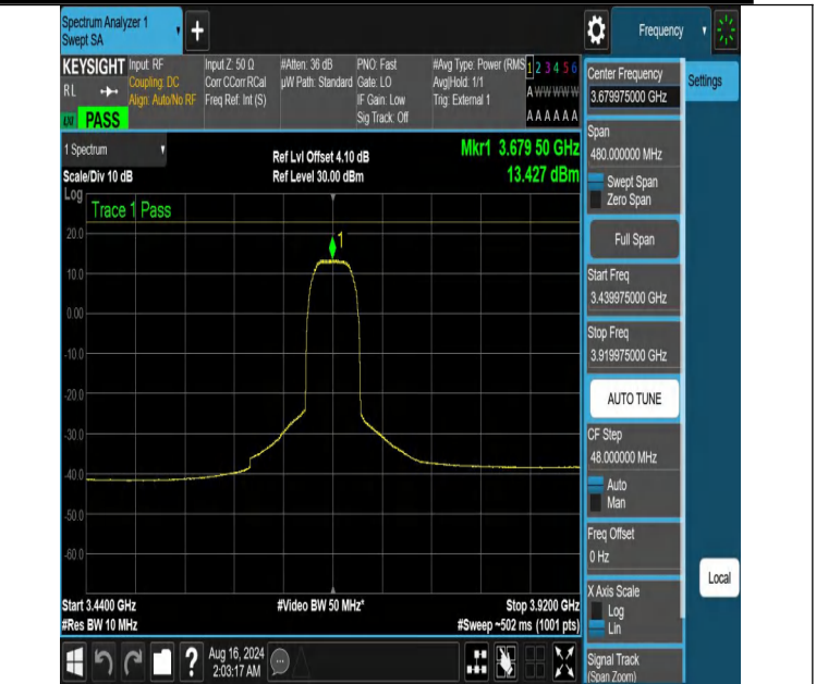
NTNV-DC_13A_n48A-PC3-30-5+40-M+H-N/A-N/A-CP-16QAM-Outer_Full-3439.975-3919.975-PASS
