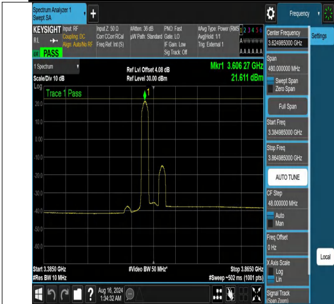
NTNV-DC_13A_n48A-PC3-30-5+40-M+M-N/A-N/A-DFT-PI2BPSK-Edge_1RB_Left-3384.985-3864.985-PASS
