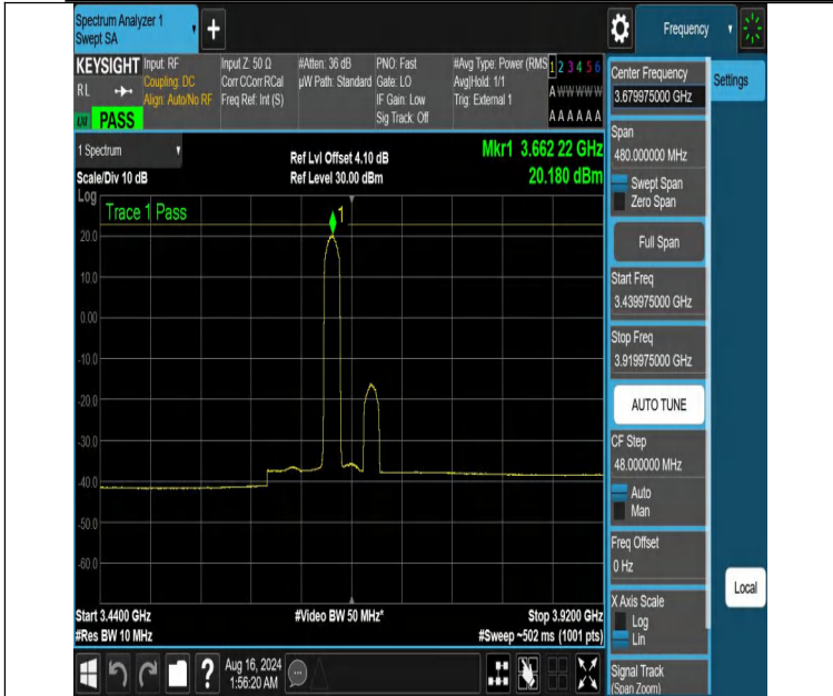
NTNV-DC_13A_n48A-PC3-30-5+40-M+H-N/A-N/A-DFT-16QAM-E dge_1RB_Left-3439.975-3919.975-PASS
