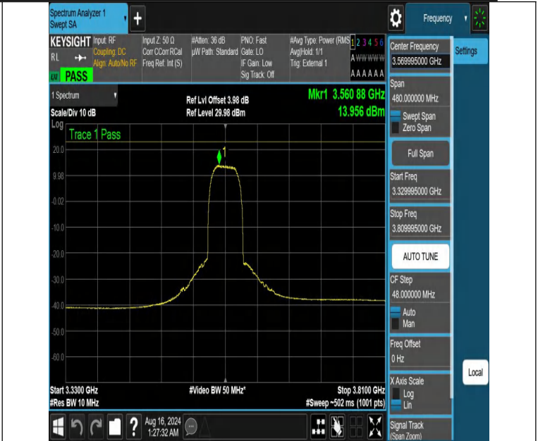
NTVN-DC_13A_n48A-PC3-30-5+40-M+L-N/A-N/A-CP-16QAM-Outer_Full-3329.995-3809.995-PASS
