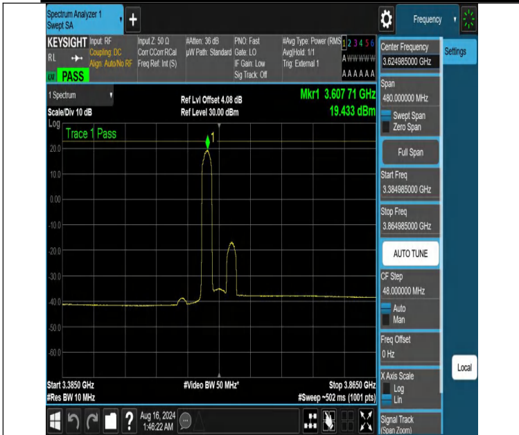
NTNV-DC_13A_n48A-PC3-30-5+40-M+M-N/A-N/A-CP-16QAM-Edge_1RB_Left-3384.985-3864.985-PASS
