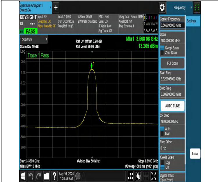
NTNV-DC_13A_n48A-PC3-30-5+40-M+L-N/A-N/A-CP-256QAM-Inner_Full-3329.995-3809.995-PASS
