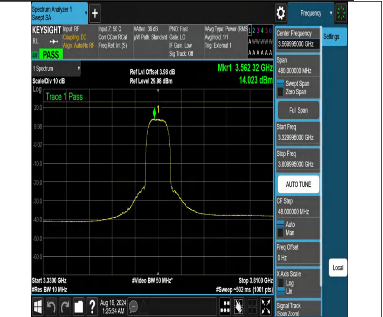
NTNV-DC_13A_n48A-PC3-30-5+40-M+L-N/A-N/A-CP-QPSK-Outer_Full-3329.995-3809.995-PASS
