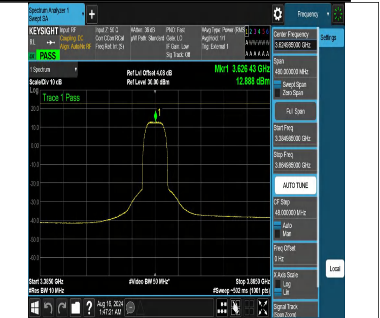
NTNV-DC_13A_n48A-PC3-30-5+40-M+M-N/A-N/A-CP-64QAM-Outer_Full-3384.985-3864.985-PASS
