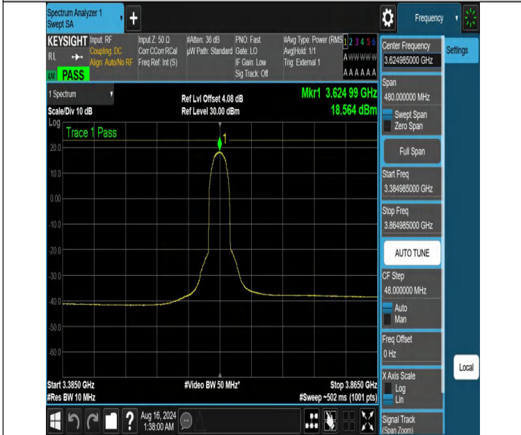
NTVN-DC_13A_n48A-PC3-30-5+40-M+M-N/A-N/A-DFT-16QAM-In ner_Full-3384.985-3864.985-PASS
