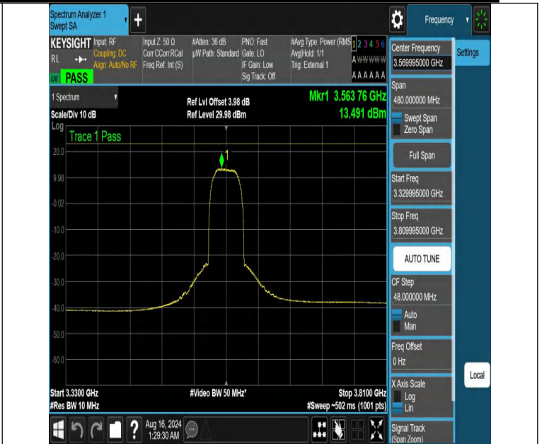
NTVN-DC_13A_n48A-PC3-30-5+40-M+L-N/A-N/A-CP-64QAM-Outer_Full-3329.995-3809.995-PASS
