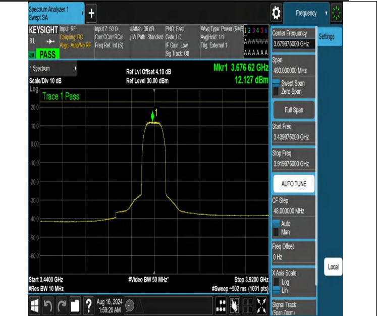
NTNV-DC_13A_n48A-PC3-30-5+40-M+H-N/A-N/A-DFT-256QAM-Outer_Full-3439.975-3919.975-PASS
