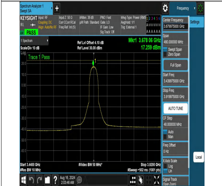
NTNV-DC_13A_n48A-PC3-30-5+40-M+H-N/A-N/A-CP-16QAM-Inner_Full-3439.975-3919.975-PASS
