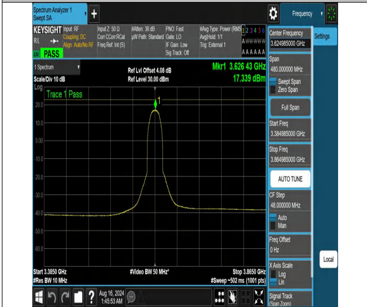
NTNV-DC_13A_n48A-PC3-30-5+40-M+M-N/A-N/A-CP-16QAM-Inner_Full-3384.985-3864.985-PASS
