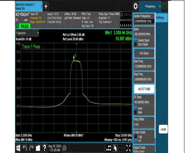
NTNV-DC_13A_n48A-PC3-30-5+40-M+L-N/A-N/A-CP-256QAM-Outer_Full-3329.995-3809.995-PASS
