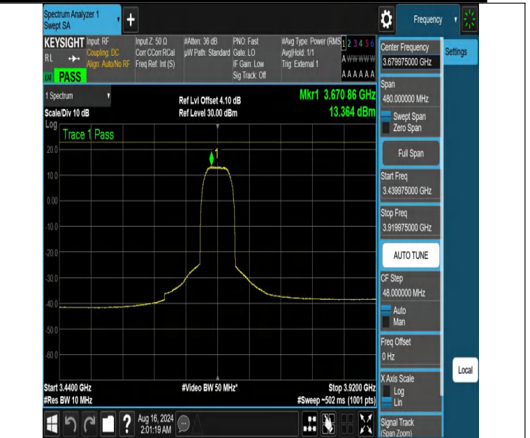
NTVN-DC_13A_n48A-PC3-30-5+40-M+H-N/A-N/A-CP-QPSK-Outer_Full-3439.975-3919.975-PASS
