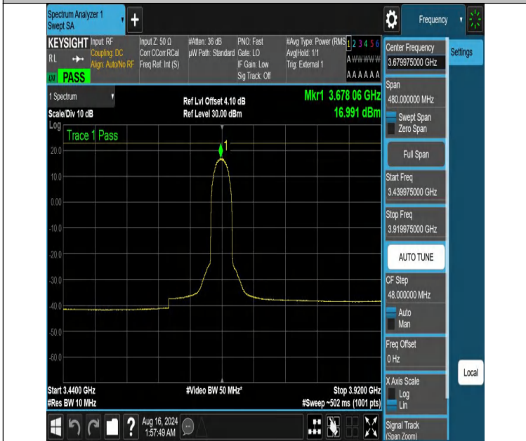
NTNV-DC_13A_n48A-PC3-30-5+40-M+H-N/A-N/A-DFT-64QAM-In ner_Full-3439.975-3919.975-PASS
