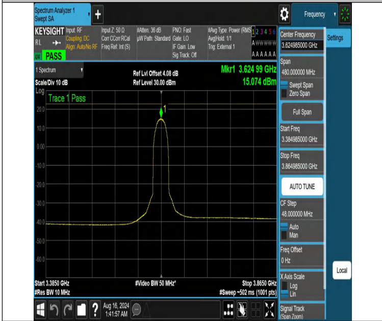
NTNV-DC_13A_n48A-PC3-30-5+40-M+M-N/A-N/A-DFT-256QAM-Inner_Full-3384.985-3864.985-PASS
