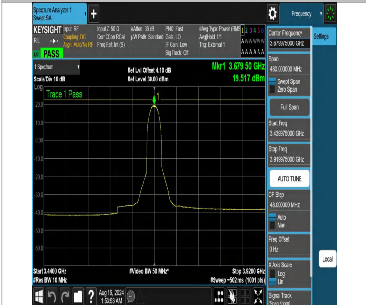
NTNV-DC_13A_n48A-PC3-30-5+40-M+H-N/A-N/A-DFT-QPSK-Inner_Full-3439.975-3919.975-PASS
