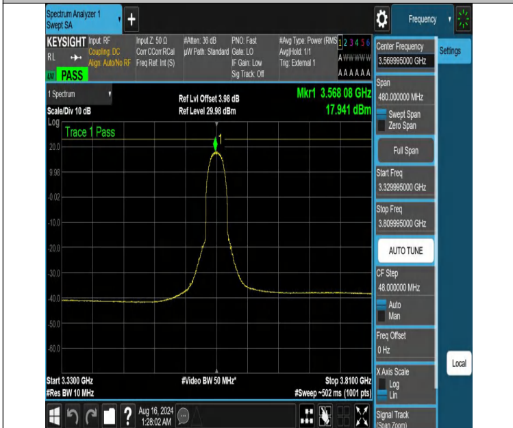
NTVN-DC_13A_n48A-PC3-30-5+40-M+L-N/A-N/A-CP-16QAM-Inner_Full-3329.995-3809.995-PASS
