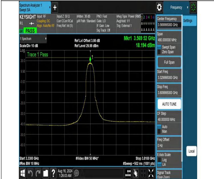
NTNV-DC_13A_n48A-PC3-30-5+40-M+L-N/A-N/A-CP-QPSK-Inner_Full-3329.995-3809.995-PASS
