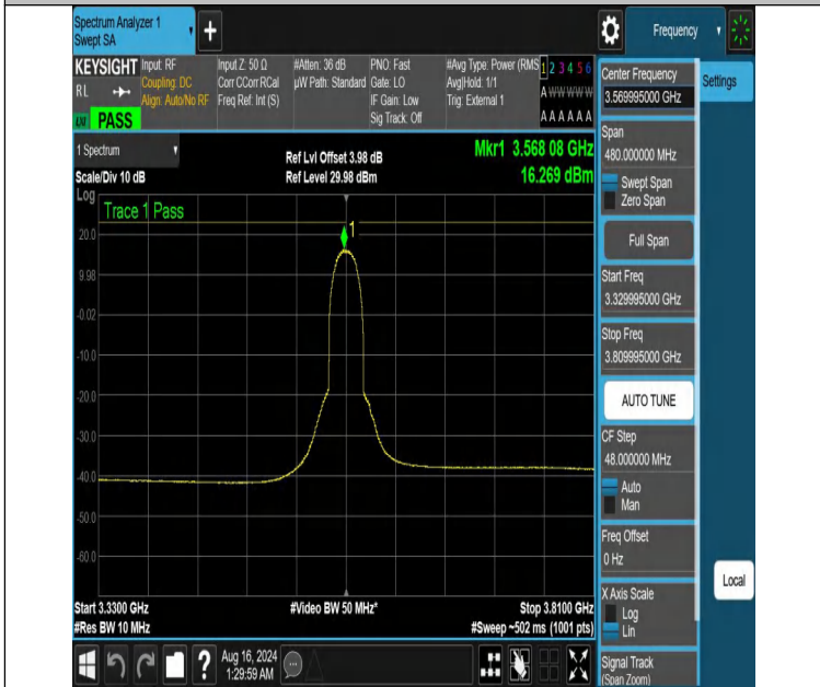
NTVN-DC_13A_n48A-PC3-30-5+40-M+L-N/A-N/A-CP-64QAM-Inner_Full-3329.995-3809.995-PASS
