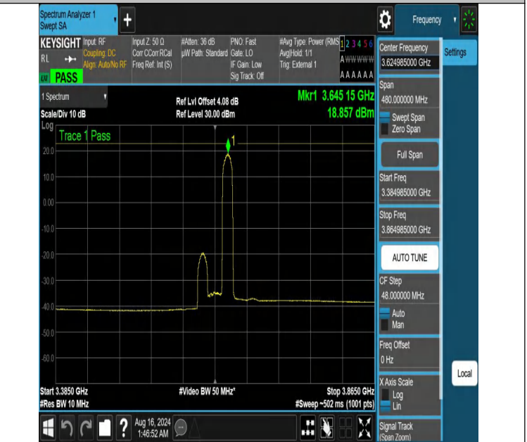
NTNV-DC_13A_n48A-PC3-30-5+40-M+M-N/A-N/A-CP-16QAM-Edge_1RB_Right-3384.985-3864.985-PASS
