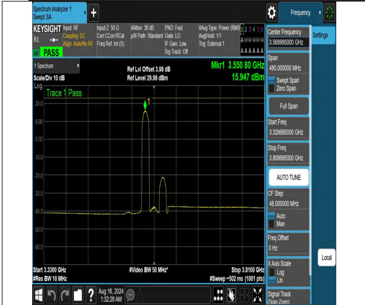
NTNV-DC_13A_n48A-PC3-30-5+40-M+L-N/A-N/A-CP-256QAM-Edge_1RB_Left-3329.995-3809.995-PASS
