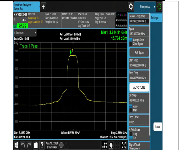
NTNV-DC_13A_n48A-PC3-30-5+40-M+M-N/A-N/A-DFT-QPSK-Outer_Full-3384.985-3864.985-PASS
