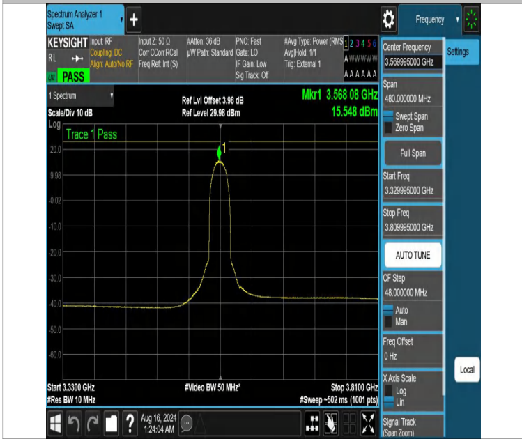
NTNV-DC_13A_n48A-PC3-30-5+40-M+L-N/A-N/A-DFT-256QAM-I nner_Full-3329.995-3809.995-PASS
