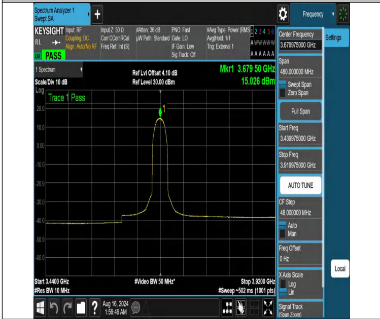
NTNV-DC_13A_n48A-PC3-30-5+40-M+H-N/A-N/A-DFT-256QAM-Inner_Full-3439.975-3919.975-PASS
