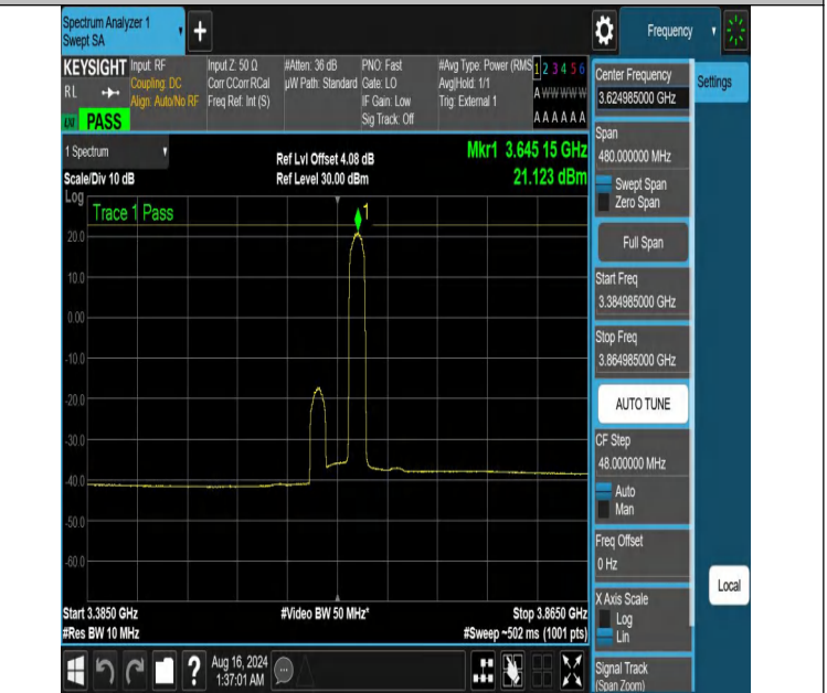
NTNV-DC_13A_n48A-PC3-30-5+40-M+M-N/A-N/A-DFT-QPSK-Edge_1RB_Right-3384.985-3864.985-PASS
