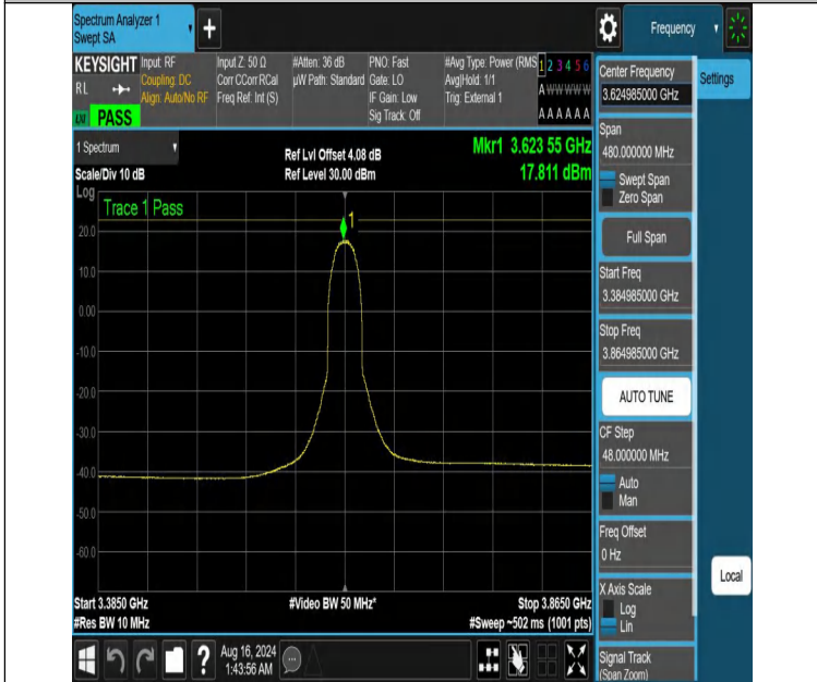
NTVN-DC_13A_n48A-PC3-30-5+40-M+M-N/A-N/A-CP-QPSK-Inner_Full-3384.985-3864.985-PASS
