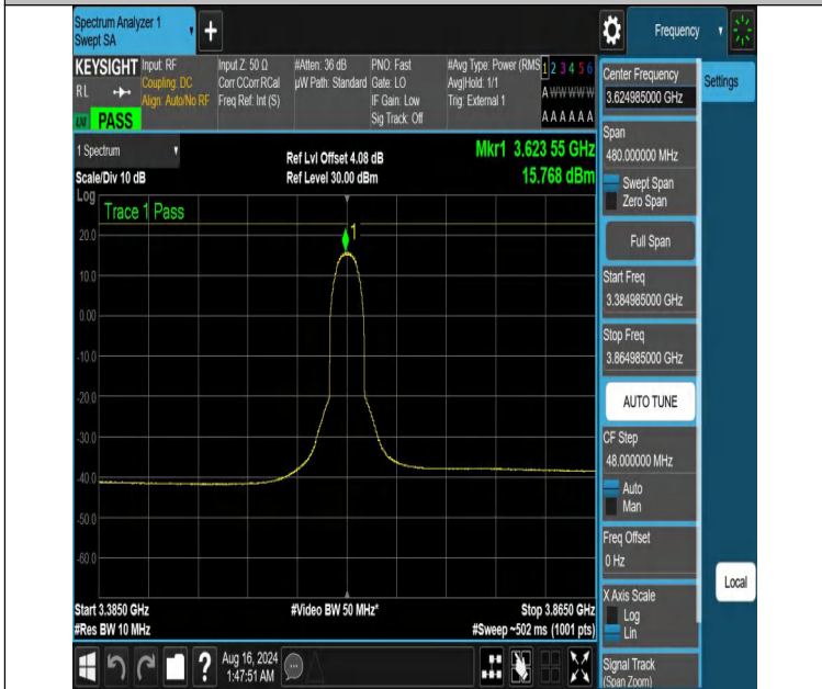
NTNV-DC_13A_n48A-PC3-30-5+40-M+M-N/A-N/A-CP-64QAM-Inner_Full-3384.985-3864.985-PASS
