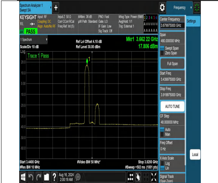
NTNV-DC_13A_n48A-PC3-30-5+40-M+H-N/A-N/A-DFT-256QAM-Edge_1RB_Left-3439.975-3919.975-PASS
