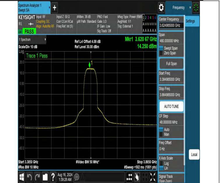
NTNV-DC_13A_n48A-PC3-30-5+40-M+M-N/A-N/A-DFT-64QAM-Ou ter_Full-3384.985-3864.985-PASS
