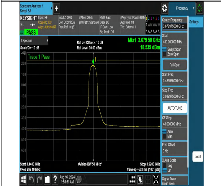
NTNV-DC_13A_n48A-PC3-30-5+40-M+H-N/A-N/A-DFT-16QAM-In ner_Full-3439.975-3919.975-PASS
