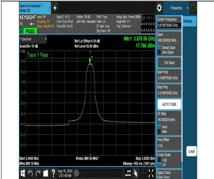
NTVN-DC_13A_n48A-PC3-30-5+40-M+H-N/A-N/A-CP-QPSK-Inner_Full-3439.975-3919.975-PASS
