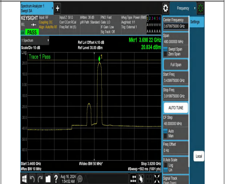
NTNV-DC_13A_n48A-PC3-30-5+40-M+H-N/A-N/A-DFT-QPSK-Edge_1RB_Right-3439.975-3919.975-PASS
