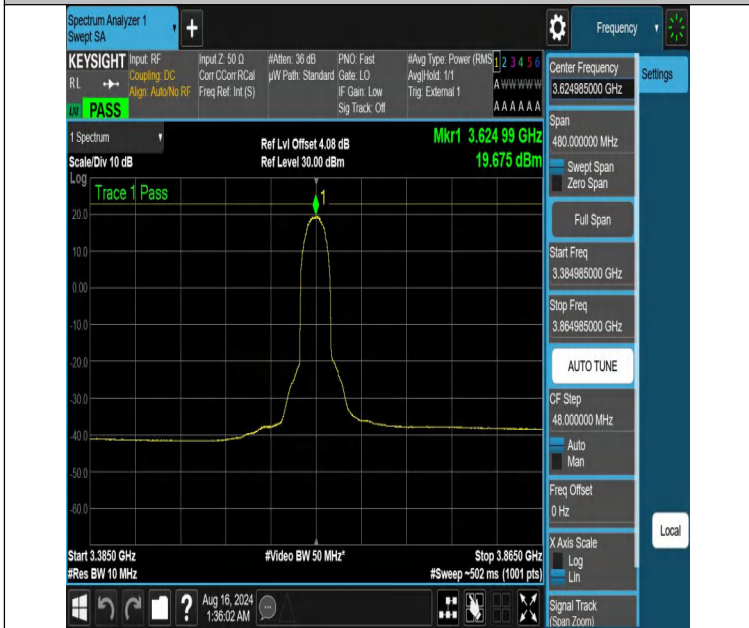
NTNV-DC_13A_n48A-PC3-30-5+40-M+M-N/A-N/A-DFT-QPSK-Inner_Full-3384.985-3864.985-PASS
