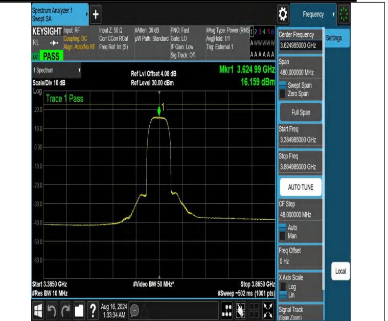
NTNV-DC_13A_n48A-PC3-30-5+40-M+M-N/A-N/A-DFT-PI2BPSK-Outer_Full-3384.985-3864.985-PASS
