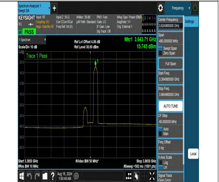
NTNV-DC_13A_n48A-PC3-30-5+40-M+M-N/A-N/A-CP-256QAM-Ed ge_1RB_Right-3384.985-3864.985-PASS
