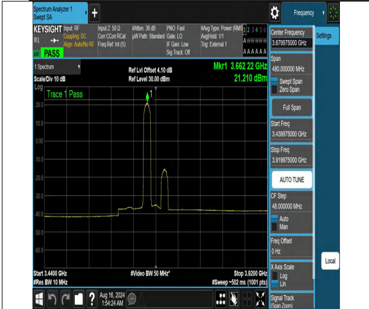
NTNV-DC_13A_n48A-PC3-30-5+40-M+H-N/A-N/A-DFT-QPSK-Edge_1RB_Left-3439.975-3919.975-PASS
