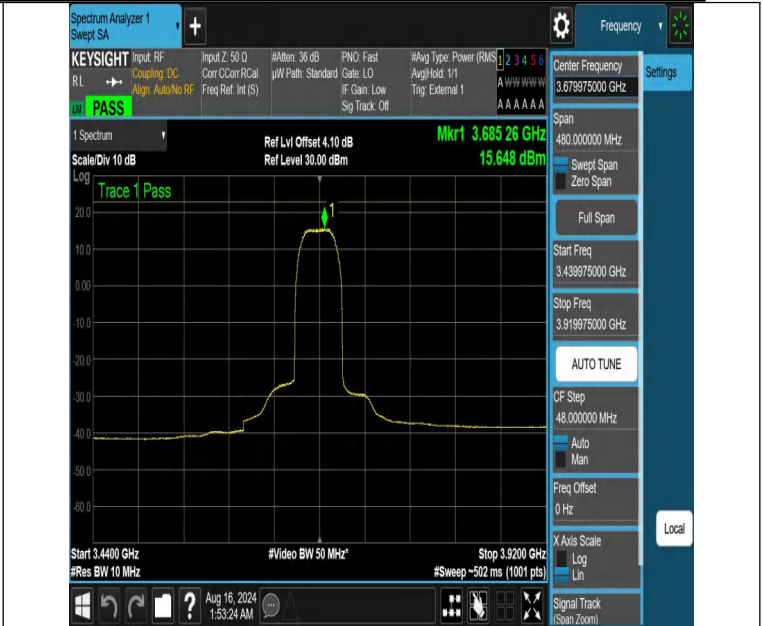
NTNV-DC_13A_n48A-PC3-30-5+40-M+H-N/A-N/A-DFT-QPSK-Outer_Full-3439.975-3919.975-PASS
