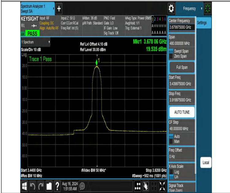
NTVN-DC_13A_n48A-PC3-30-5+40-M+H-N/A-N/A-DFT-PI2BPSK-Inner_Full-3439.975-3919.975-PASS
