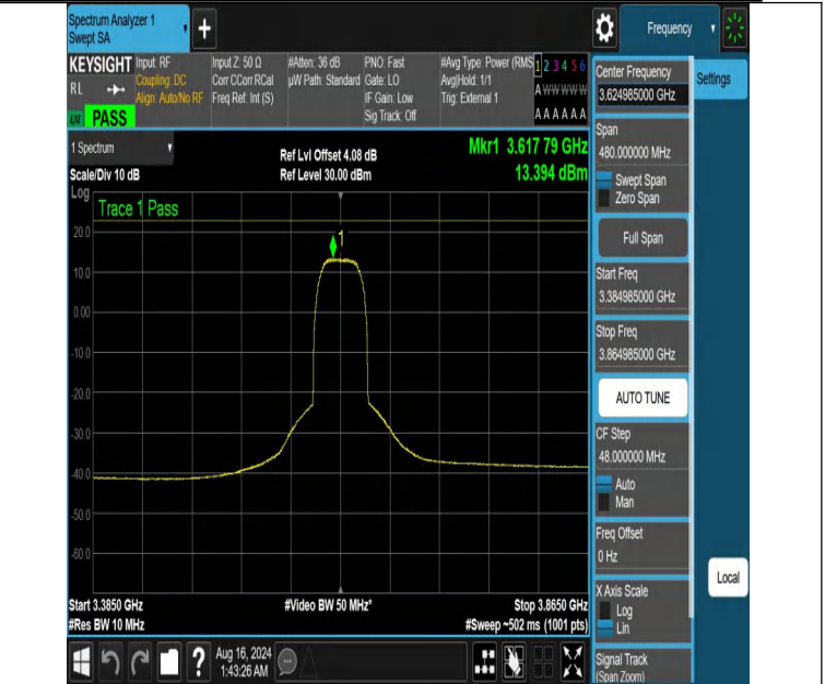
NTVN-DC_13A_n48A-PC3-30-5+40-M+M-N/A-N/A-CP-QPSK-Outer_Full-3384.985-3864.985-PASS
