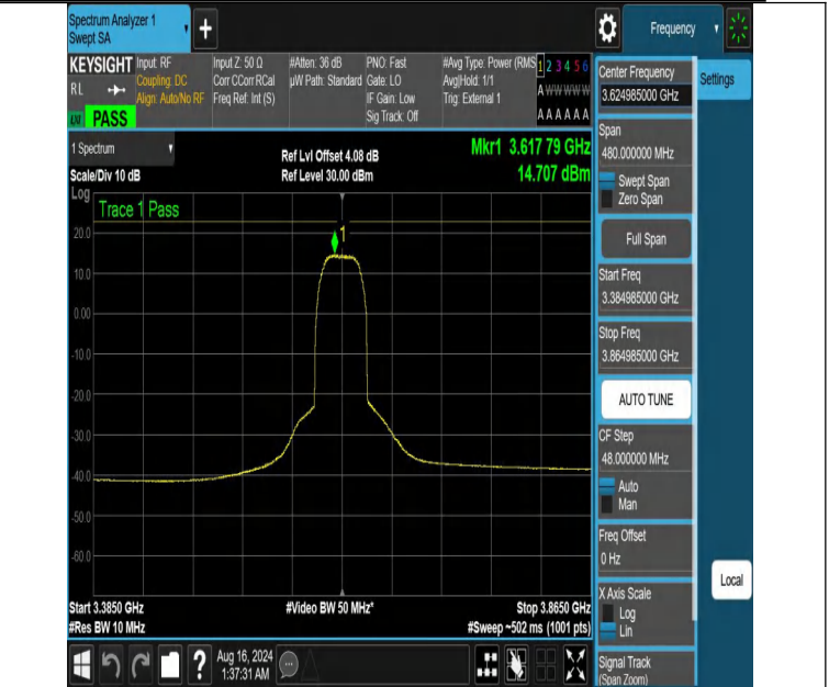
NTVN-DC_13A_n48A-PC3-30-5+40-M+M-N/A-N/A-DFT-16QAM-Ou ter_Full-3384.985-3864.985-PASS
