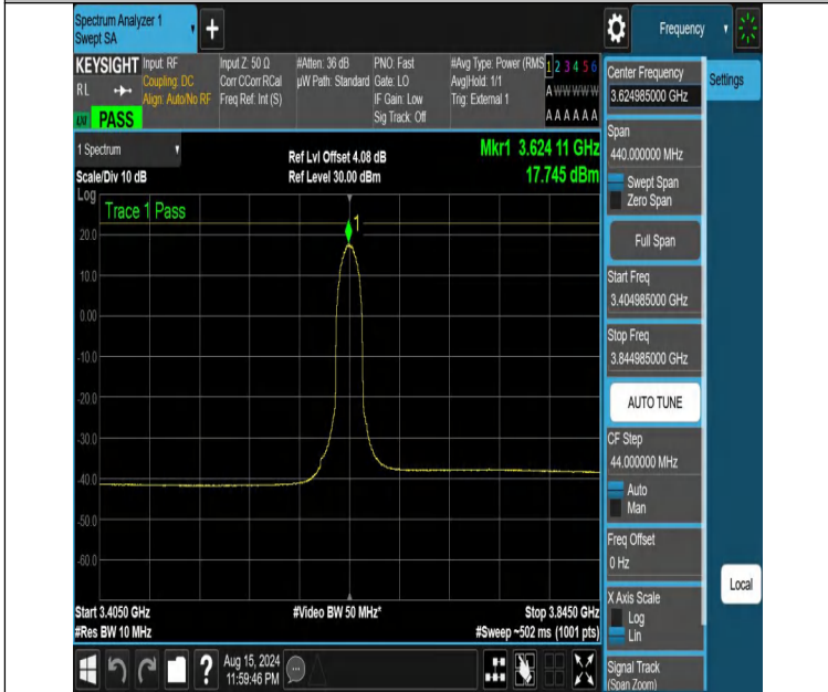
NTNV-DC_13A_n48A-PC3-30-5+20-M+M-N/A-N/A-CP-64QAM-Inner_Full-3404.985-3844.985-PASS
