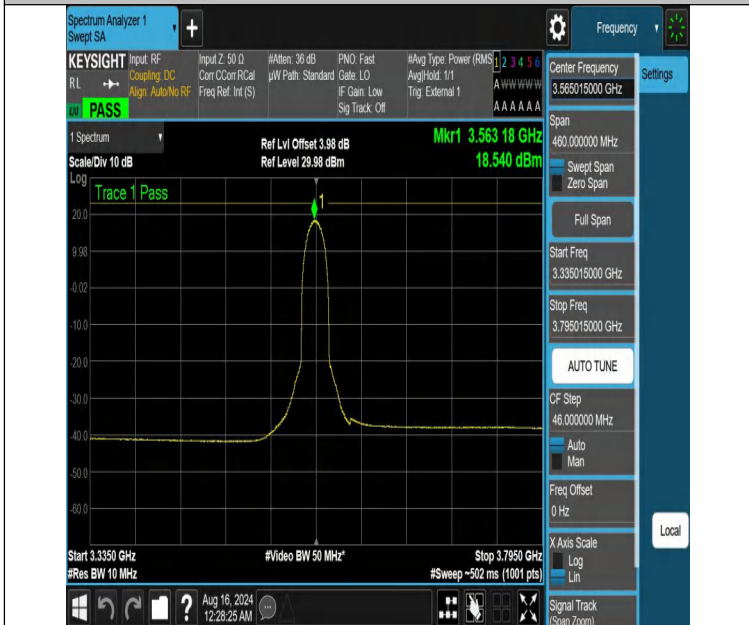
NTNV-DC_13A_n48A-PC3-30-5+30-M+L-N/A-N/A-DFT-64QAM-Inner_Full-3335.015-3795.015-PASS
