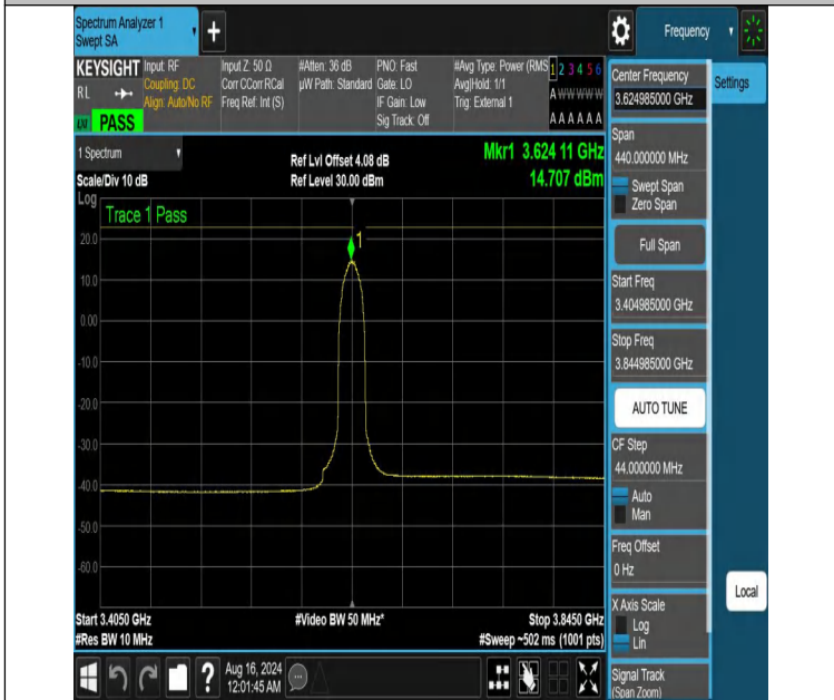
NTVN-DC_13A_n48A-PC3-30-5+20-M+M-N/A-N/A-CP-256QAM-In ner_Full-3404.985-3844.985-PASS
