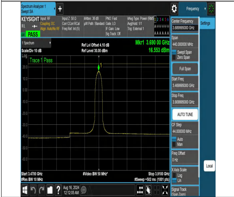
NTNV-DC_13A_n48A-PC3-30-5+20-M+H-N/A-N/A-DFT-256QAM-Inner_Full-3469.995-3909.995-PASS
