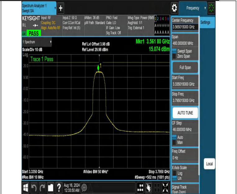
NTNV-DC_13A_n48A-PC3-30-5+30-M+L-N/A-N/A-CP-16QAM-Outer_Full-3335.015-3795.015-PASS
