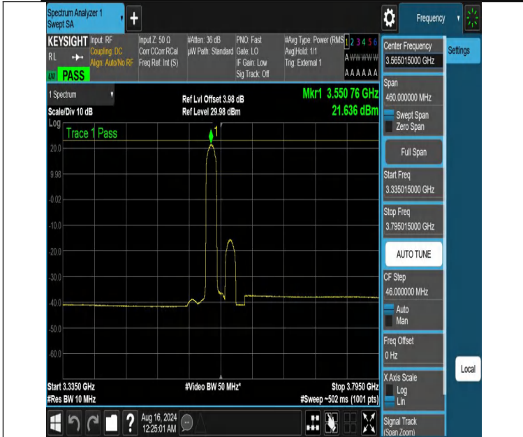
NTNV-DC_13A_n48A-PC3-30-5+30-M+L-N/A-N/A-DFT-QPSK-Edge e_1RB_Left-3335.015-3795.015-PASS
