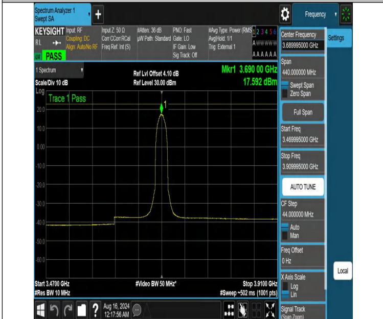
NTNV-DC_13A_n48A-PC3-30-5+20-M+H-N/A-N/A-CP-64QAM-Inner_Full-3469.995-3909.995-PASS
