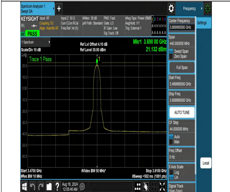
NTNV-DC_13A_n48A-PC3-30-5+20-M+H-N/A-N/A-DFT-QPSK-Inner_Full-3469.995-3909.995-PASS
