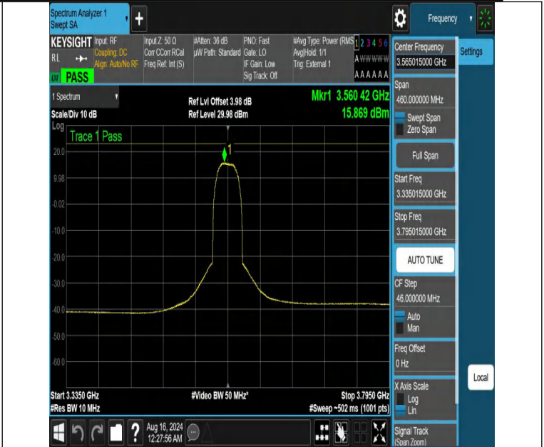
NTNV-DC_13A_n48A-PC3-30-5+30-M+L-N/A-N/A-DFT-64QAM-Outer_Full-3335.015-3795.015-PASS
