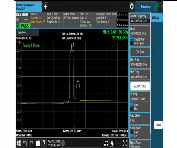
NTNV-DC_13A_n48A-PC3-30-5+30-M+M-N/A-N/A-DFT-PI2BPSK-Edge_1RB_Left-3394.985-3854.985-PASS
