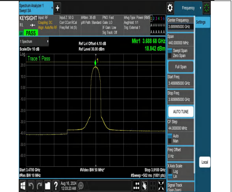
NTVN-DC_13A_n48A-PC3-30-5+20-M+H-N/A-N/A-DFT-PI2BPSK-Outer_Full-3469.995-3909.995-PASS
