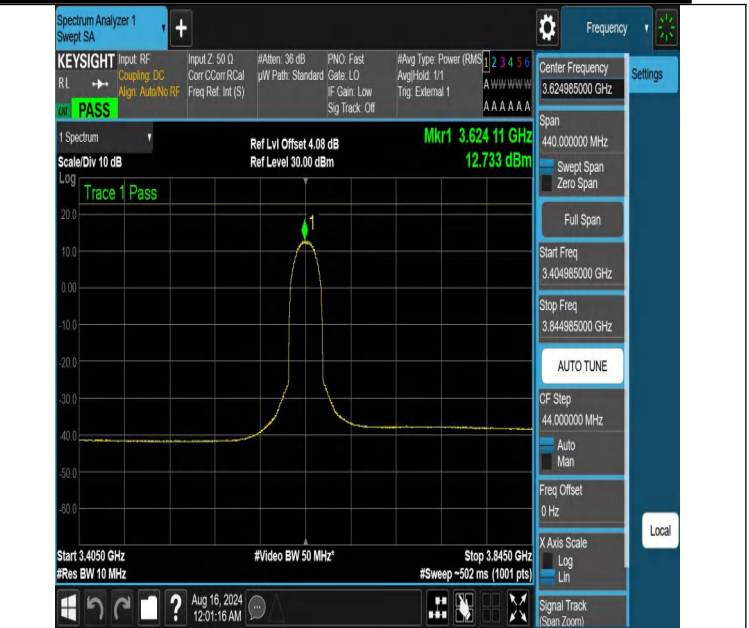
NTVN-DC_13A_n48A-PC3-30-5+20-M+M-N/A-N/A-CP-256QAM-Ou ter_Full-3404.985-3844.985-PASS
