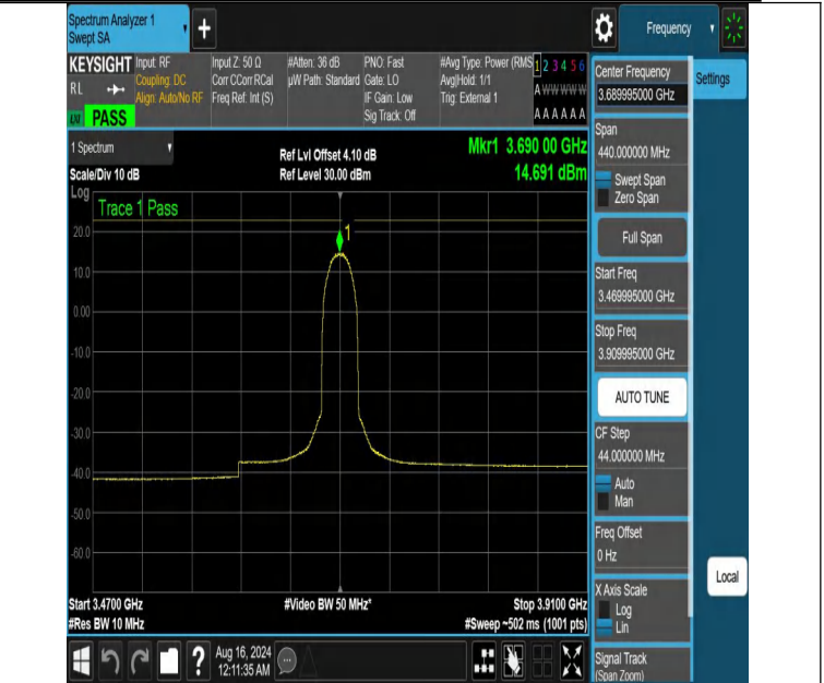
NTNV-DC_13A_n48A-PC3-30-5+20-M+H-N/A-N/A-DFT-256QAM-Outer_Full-3469.995-3909.995-PASS
