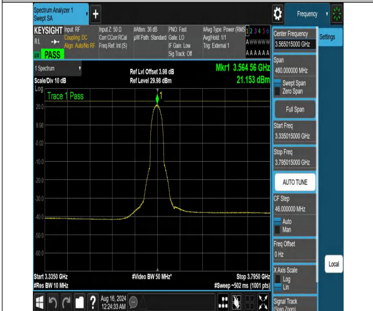
NTNV-DC_13A_n48A-PC3-30-5+30-M+L-N/A-N/A-DFT-QPSK-Inne r_Full-3335.015-3795.015-PASS
