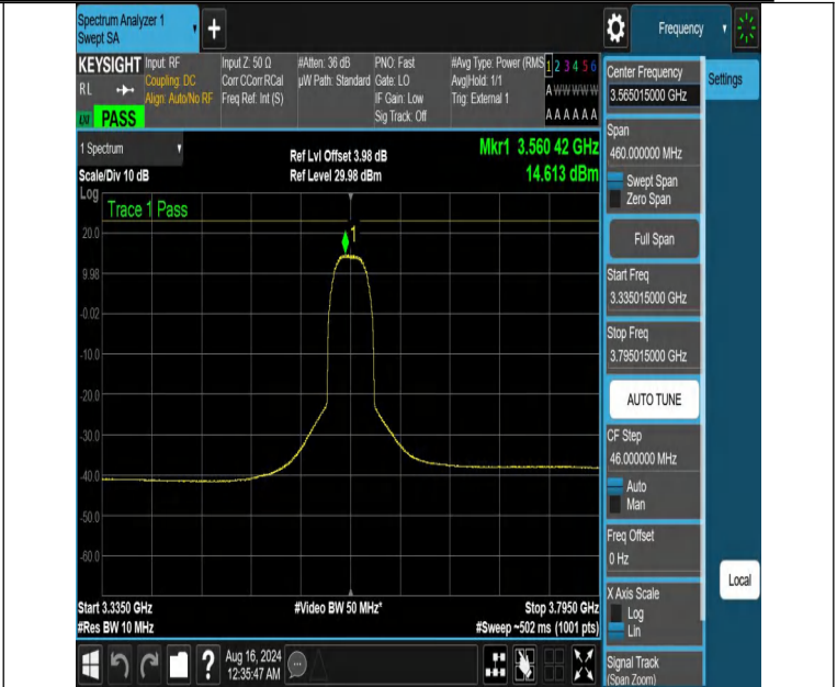
NTVN-DC_13A_n48A-PC3-30-5+30-M+L-N/A-N/A-CP-64QAM-Outer_Full-3335.015-3795.015-PASS
