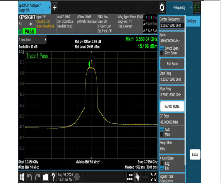
NTNV-DC_13A_n48A-PC3-30-5+30-M+L-N/A-N/A-CP-QPSK-Outer _Full-3335.015-3795.015-PASS
