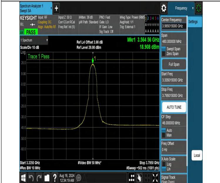
NTNV-DC_13A_n48A-PC3-30-5+30-M+L-N/A-N/A-CP-16QAM-Inner_Full-3335.015-3795.015-PASS
