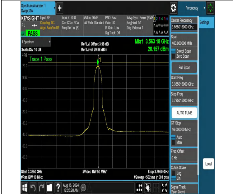
NTNV-DC_13A_n48A-PC3-30-5+30-M+L-N/A-N/A-DFT-16QAM-Inner_Full-3335.015-3795.015-PASS
