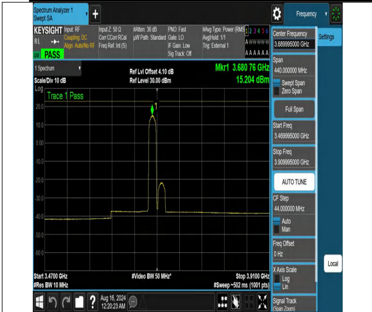
NTNV-DC_13A_n48A-PC3-30-5+20-M+H-N/A-N/A-CP-256QAM-E dge_1RB_Left-3469.995-3909.995-PASS
