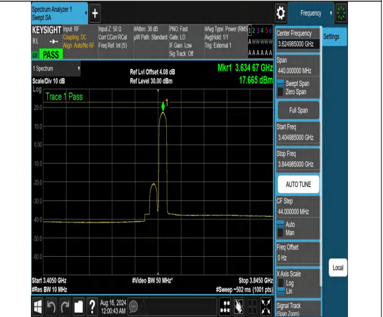
NTNV-DC_13A_n48A-PC3-30-5+20-M+M-N/A-N/A-CP-64QAM-Edge_1RB_Right-3404.985-3844.985-PASS
