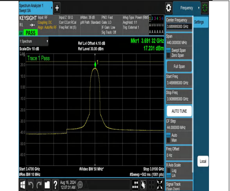
NTNV-DC_13A_n48A-PC3-30-5+20-M+H-N/A-N/A-DFT-16QAM-Ou ter_Full-3469.995-3909.995-PASS
