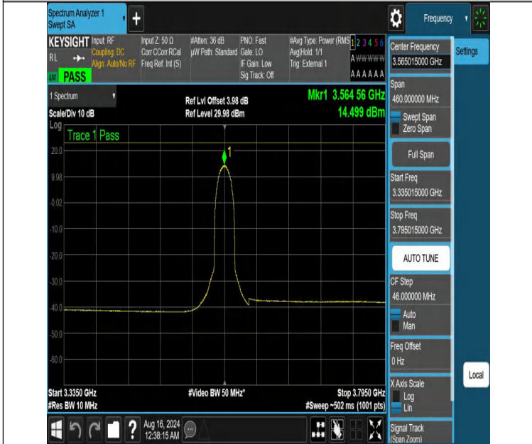
NTNV-DC_13A_n48A-PC3-30-5+30-M+L-N/A-N/A-CP-256QAM-Inner_Full-3335.015-3795.015-PASS
