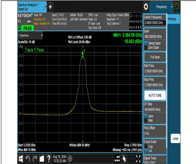
NTNV-DC_13A_n48A-PC3-30-5+30-M+L-N/A-N/A-CP-QPSK-Inner _Full-3335.015-3795.015-PASS
