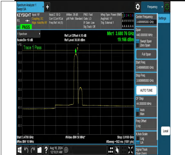
NTNV-DC_13A_n48A-PC3-30-5+20-M+H-N/A-N/A-DFT-64QAM-E dge_1RB_Left-3469.995-3909.995-PASS
