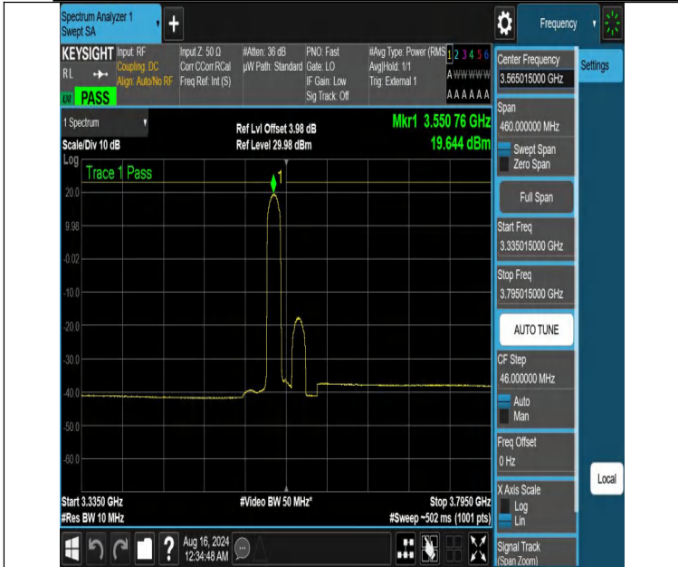
NTNV-DC_13A_n48A-PC3-30-5+30-M+L-N/A-N/A-CP-16QAM-Edge_1RB_Left-3335.015-3795.015-PASS
