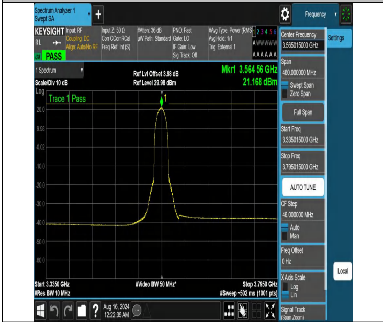
NTNV-DC_13A_n48A-PC3-30-5+30-M+L-N/A-N/A-DFT-PI2BPSK-IInner_Full-3335.015-3795.015-PASS
