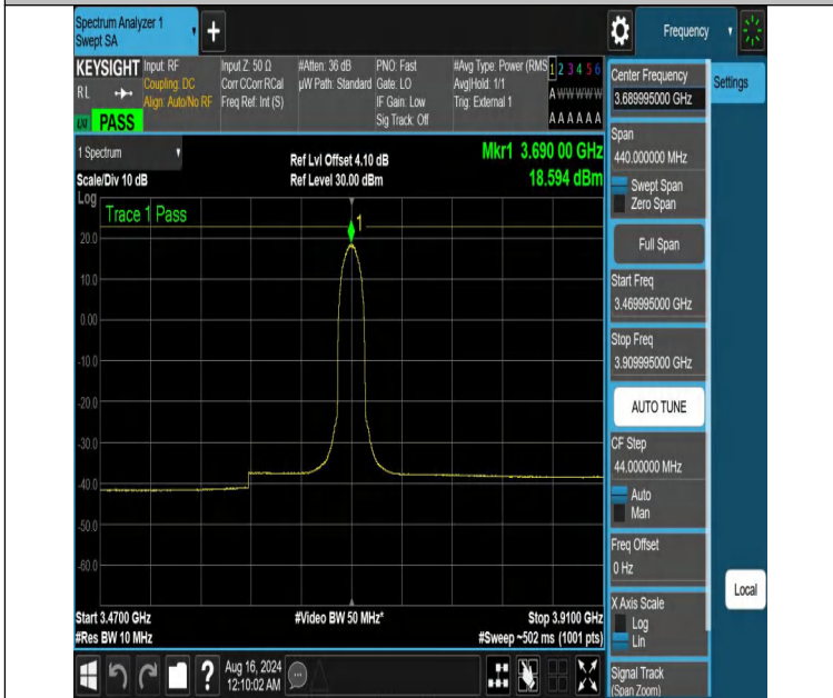
NTNV-DC_13A_n48A-PC3-30-5+20-M+H-N/A-N/A-DFT-64QAM-In ner_Full-3469.995-3909.995-PASS
