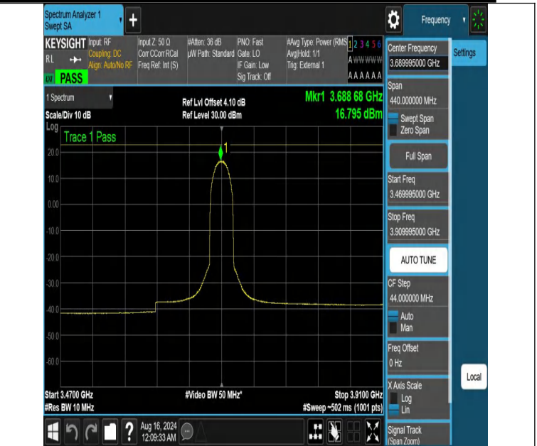
NTNV-DC_13A_n48A-PC3-30-5+20-M+H-N/A-N/A-DFT-64QAM-Ou ter_Full-3469.995-3909.995-PASS
