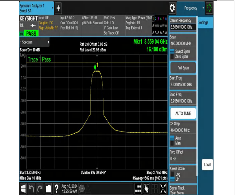
NTNV-DC_13A_n48A-PC3-30-5+30-M+L-N/A-N/A-DFT-16QAM-Outer_Full-3335.015-3795.015-PASS
