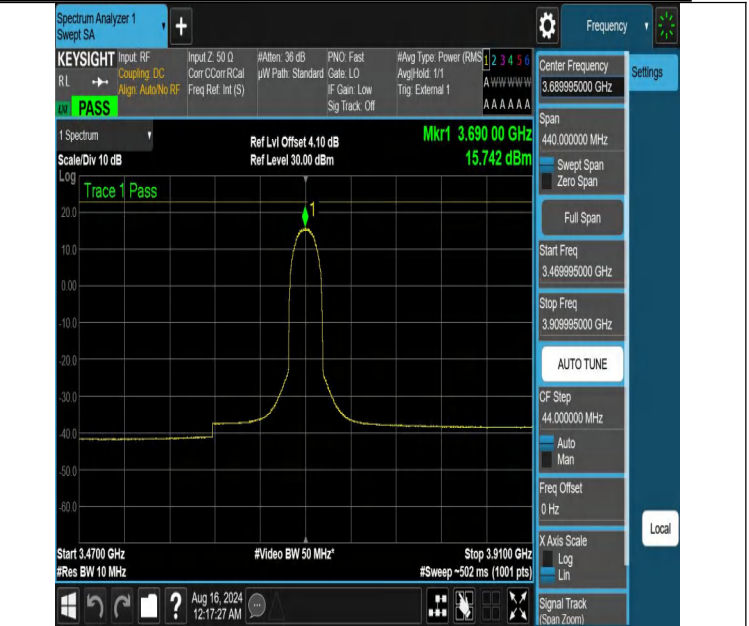
NTNV-DC_13A_n48A-PC3-30-5+20-M+H-N/A-N/A-CP-64QAM-Outer_Full-3469.995-3909.995-PASS
