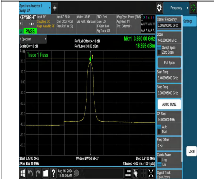
NTNV-DC_13A_n48A-PC3-30-5+20-M+H-N/A-N/A-CP-16QAM-Inner_Full-3469.995-3909.995-PASS
