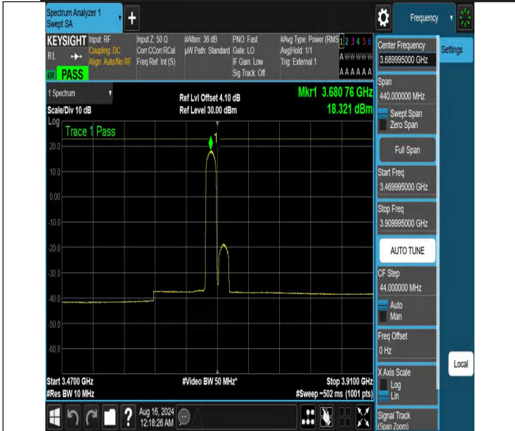
NTNV-DC_13A_n48A-PC3-30-5+20-M+H-N/A-N/A-CP-64QAM-Edge_1RB_Left-3469.995-3909.995-PASS
