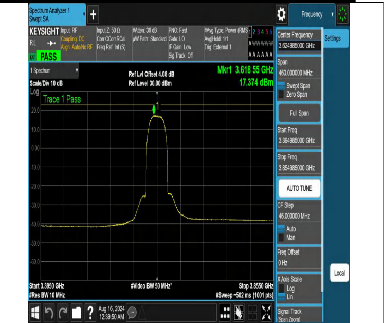
NTNV-DC_13A_n48A-PC3-30-5+30-M+M-N/A-N/A-DFT-PI2BPSK-Outer_Full-3394.985-3854.985-PASS
