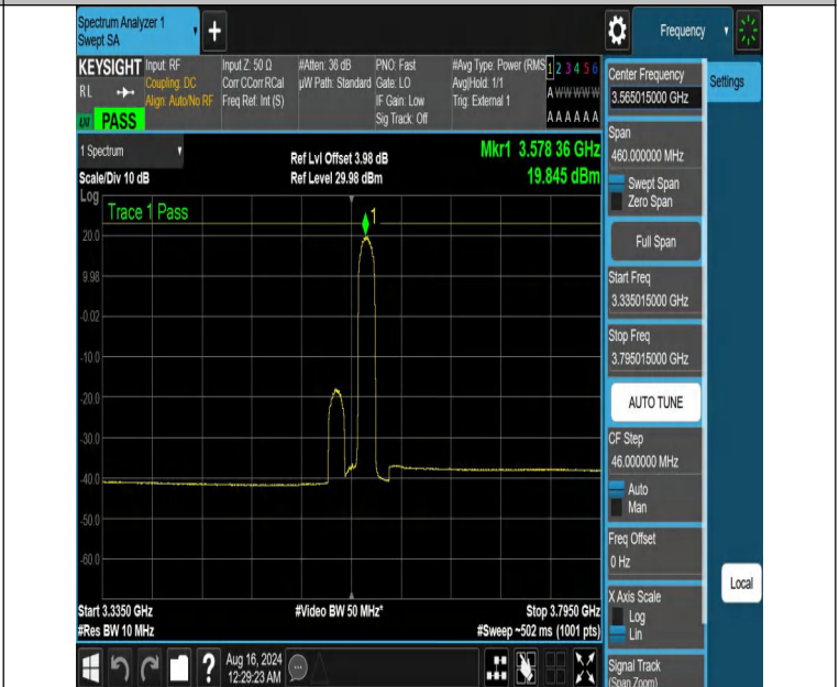
NTNV-DC_13A_n48A-PC3-30-5+30-M+L-N/A-N/A-DFT-64QAM-Edge_1RB_Right-3335.015-3795.015-PASS
