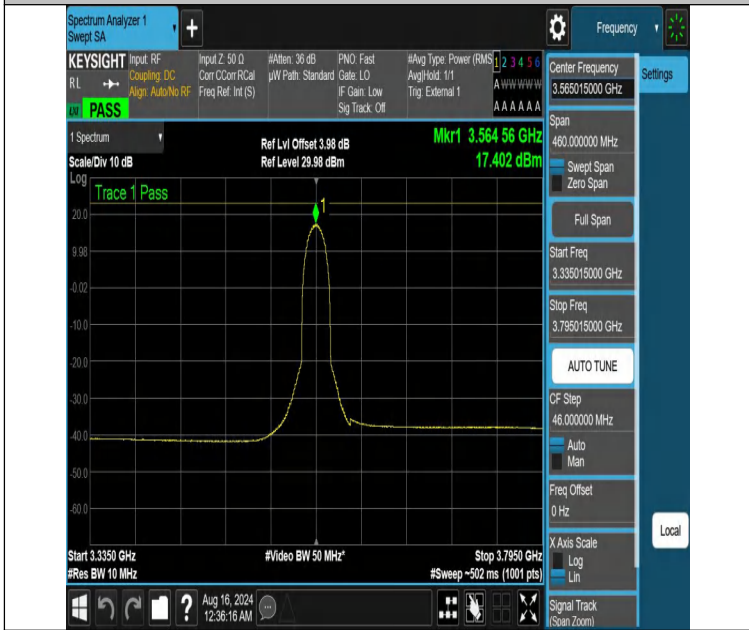
NTVN-DC_13A_n48A-PC3-30-5+30-M+L-N/A-N/A-CP-64QAM-Inner_Full-3335.015-3795.015-PASS
