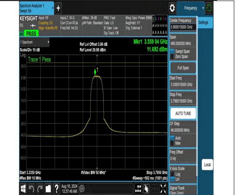
NTNV-DC_13A_n48A-PC3-30-5+30-M+L-N/A-N/A-CP-256QAM-Outer_Full-3335.015-3795.015-PASS
