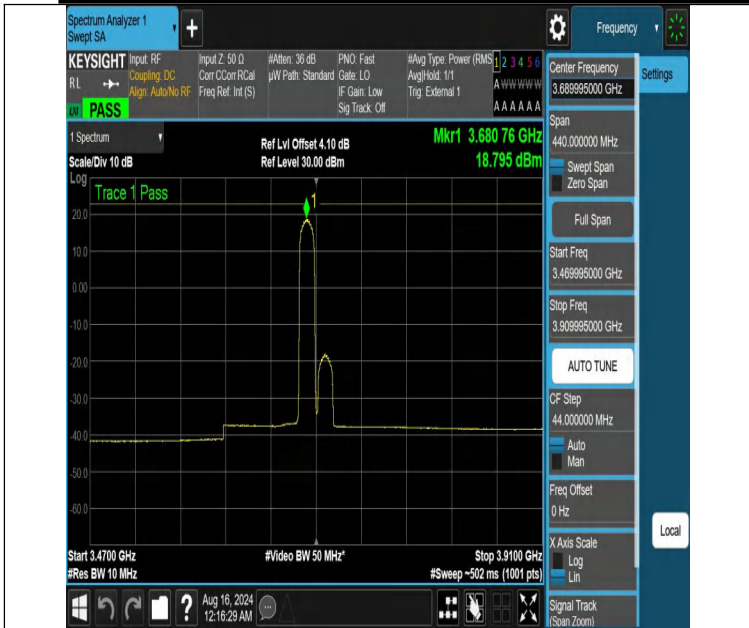
NTNV-DC_13A_n48A-PC3-30-5+20-M+H-N/A-N/A-CP-16QAM-Edge_1RB_Left-3469.995-3909.995-PASS
