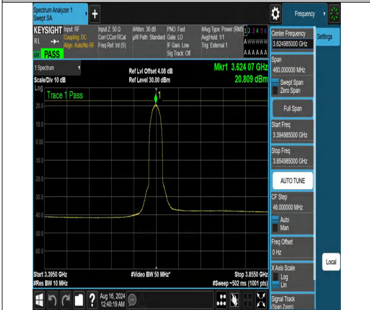
NTNV-DC_13A_n48A-PC3-30-5+30-M+M-N/A-N/A-DFT-PI2BPSK-I nner_Full-3394.985-3854.985-PASS
