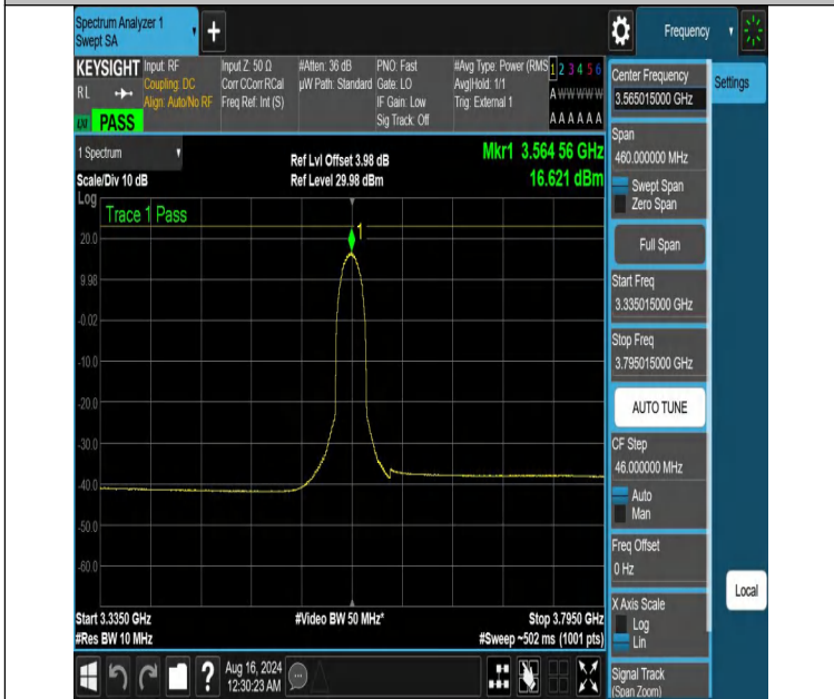
NTNV-DC_13A_n48A-PC3-30-5+30-M+L-N/A-N/A-DFT-256QAM-I nner_Full-3335.015-3795.015-PASS
