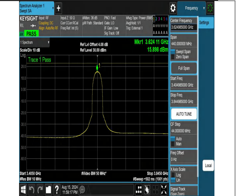
NTNV-DC_13A_n48A-PC3-30-5+20-M+M-N/A-N/A-CP-64QAM-Outer_Full-3404.985-3844.985-PASS
