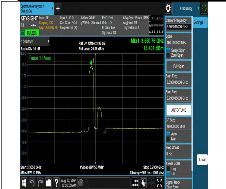
NTNV-DC_13A_n48A-PC3-30-5+30-M+L-N/A-N/A-DFT-256QAM-E dge_1RB_Left-3335.015-3795.015-PASS
