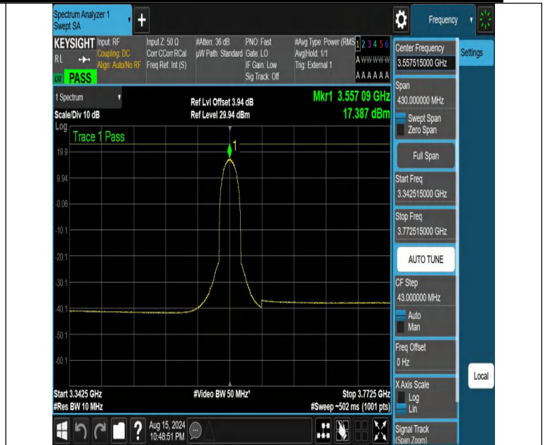
NTVN-DC_13A_n48A-PC3-30-5+15-M+L-N/A-N/A-CP-64QAM-Outer_Full-3342.515-3772.515-PASS
