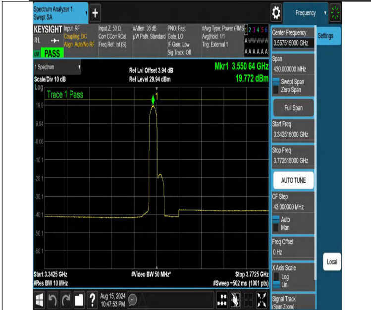
NTVN-DC_13A_n48A-PC3-30-5+15-M+L-N/A-N/A-CP-16QAM-Edge_1RB_Left-3342.515-3772.515-PASS
