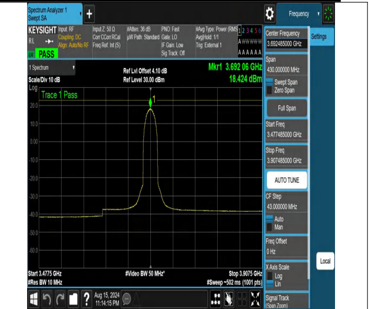
NTNV-DC_13A_n48A-PC3-30-5+15-M+H-N/A-N/A-DFT-16QAM-Ou ter_Full-3477.485-3907.485-PASS
