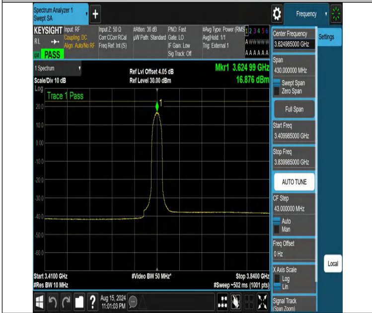
NTVN-DC_13A_n48A-PC3-30-5+15-M+M-N/A-N/A-DFT-256QAM-Inner_Full-3409.985-3839.985-PASS
