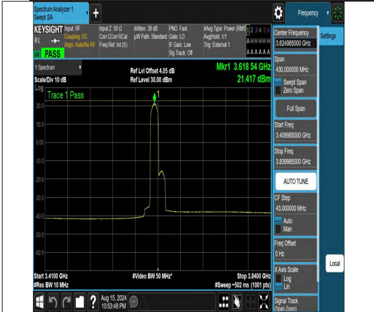
NTNV-DC_13A_n48A-PC3-30-5+15-M+M-N/A-N/A-DFT-PI2BPSK-Edge_1RB_Left-3409.985-3839.985-PASS
