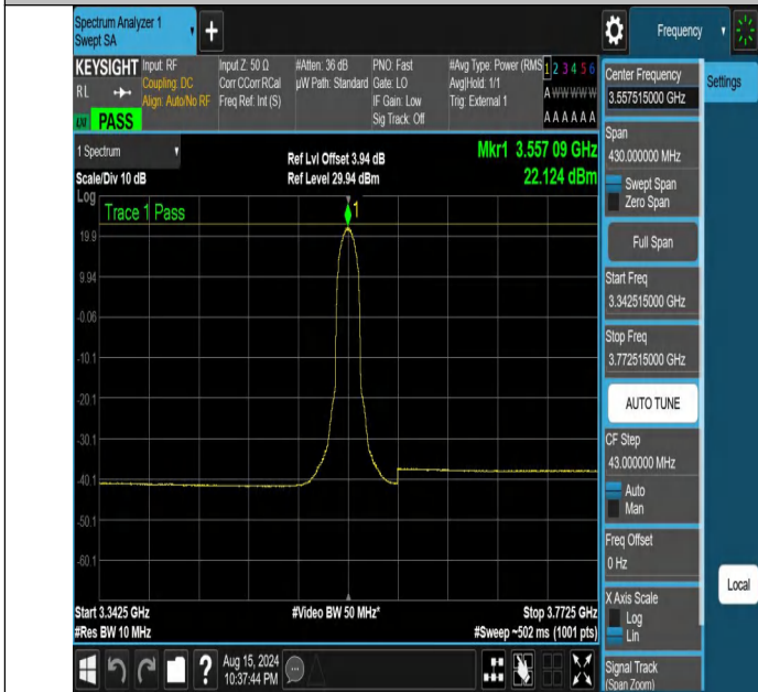
NTNV-DC_13A_n48A-PC3-30-5+15-M+L-N/A-N/A-DFT-QPSK-Inner_Full-3342.515-3772.515-PASS
