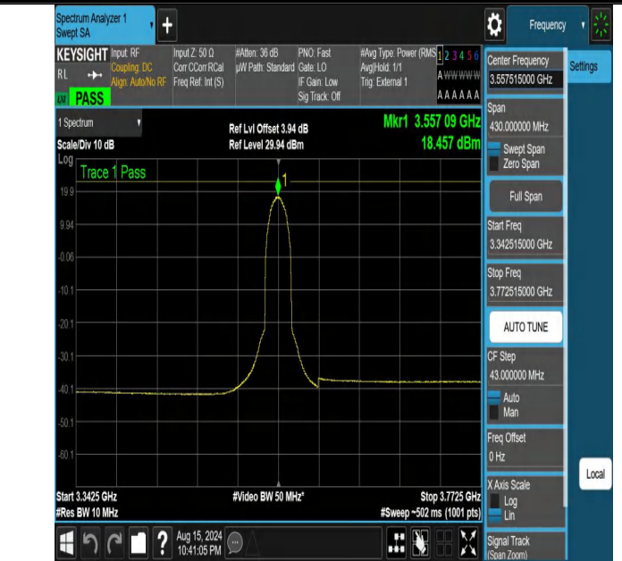
NTNV-DC_13A_n48A-PC3-30-5+15-M+L-N/A-N/A-DFT-64QAM-Outer_Full-3342.515-3772.515-PASS
