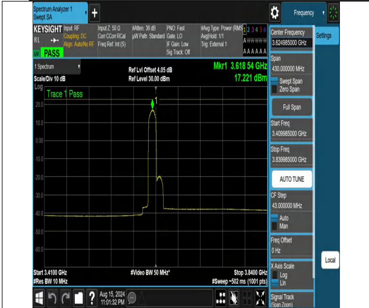
NTVN-DC_13A_n48A-PC3-30-5+15-M+M-N/A-N/A-DFT-256QAM-Edge_1RB_Left-3409.985-3839.985-PASS
