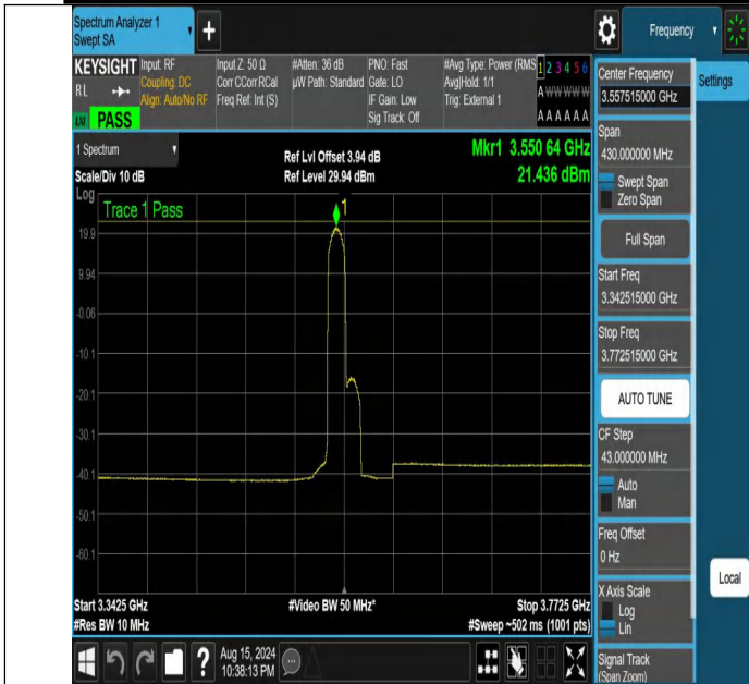
NTNV-DC_13A_n48A-PC3-30-5+15-M+L-N/A-N/A-DFT-QPSK-Edge e_1RB_Left-3342.515-3772.515-PASS
