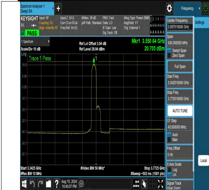
NTNV-DC_13A_n48A-PC3-30-5+15-M+L-N/A-N/A-DFT-16QAM-Edge_1RB_Left-3342.515-3772.515-PASS
