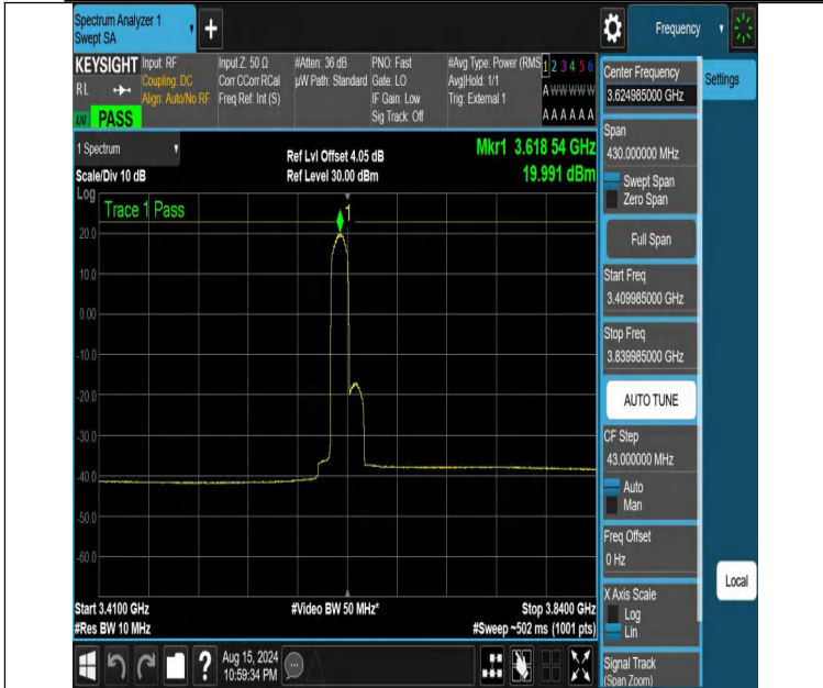
NTNV-DC_13A_n48A-PC3-30-5+15-M+M-N/A-N/A-DFT-64QAM-E dge_1RB_Left-3409.985-3839.985-PASS
