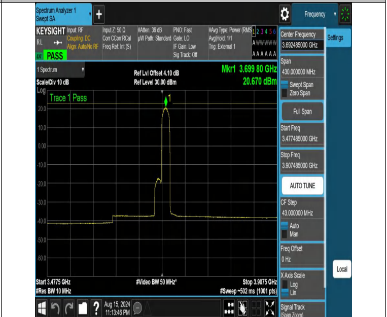
NTNV-DC_13A_n48A-PC3-30-5+15-M+H-N/A-N/A-DFT-QPSK-Edge_1RB_Right-3477.485-3907.485-PASS
