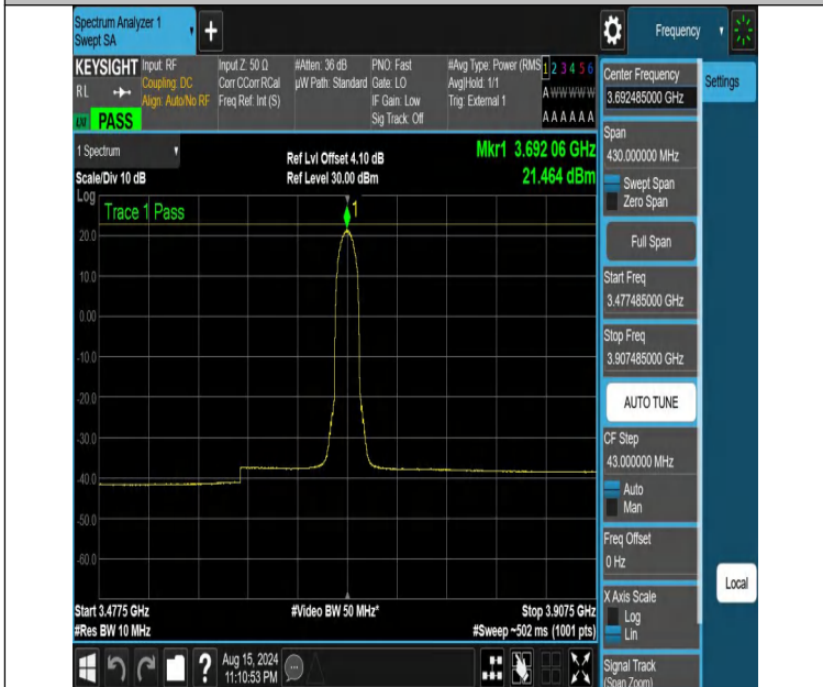
NTVN-DC_13A_n48A-PC3-30-5+15-M+H-N/A-N/A-DFT-PI2BPSK-I_nner_Full-3477.485-3907.485-PASS
