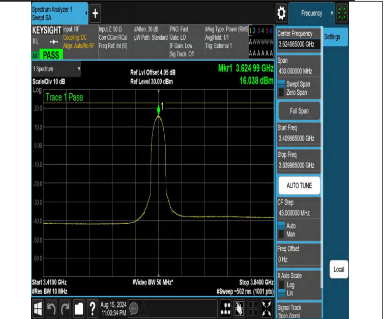
NTVN-DC_13A_n48A-PC3-30-5+15-M+M-N/A-N/A-DFT-256QAM-Outer_Full-3409.985-3839.985-PASS
