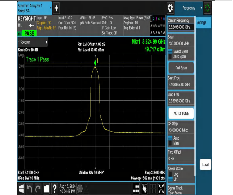
NTNV-DC_13A_n48A-PC3-30-5+15-M+M-N/A-N/A-DFT-QPSK-Outer_Full-3409.985-3839.985-PASS
