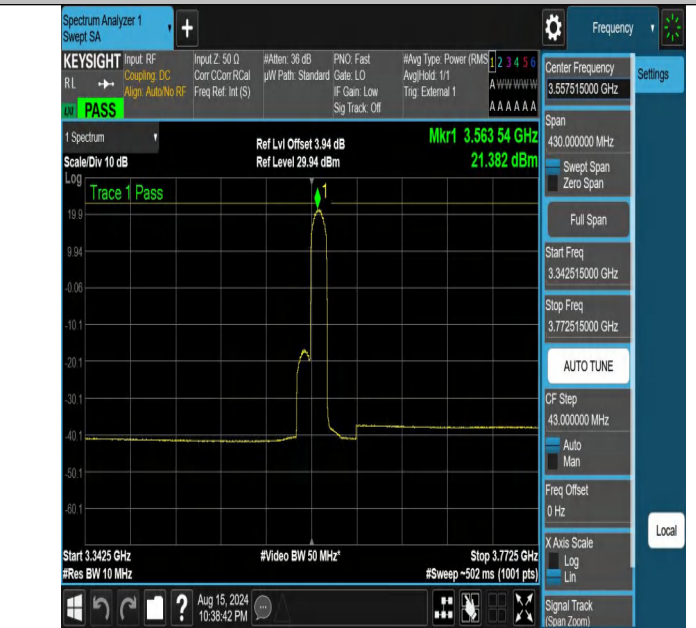
NTNV-DC_13A_n48A-PC3-30-5+15-M+L-N/A-N/A-DFT-QPSK-Edge_1RB_Right-3342.515-3772.515-PASS
