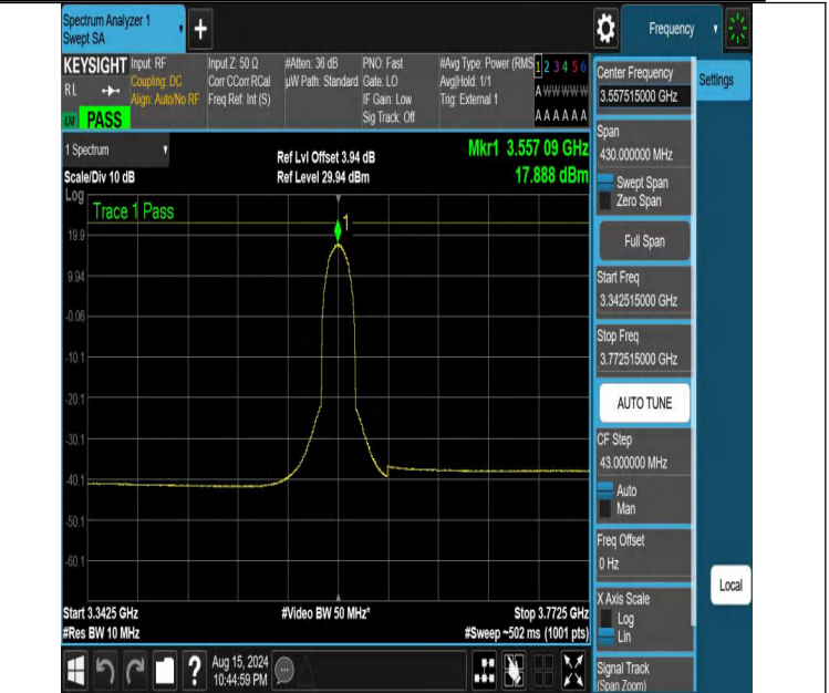
NTNV-DC_13A_n48A-PC3-30-5+15-M+L-N/A-N/A-CP-QPSK-Outer_Full-3342.515-3772.515-PASS
