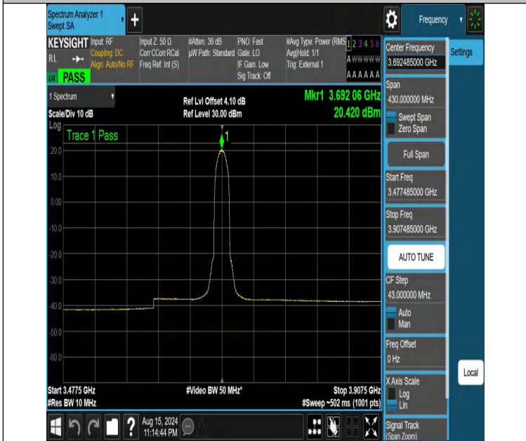
NTNV-DC_13A_n48A-PC3-30-5+15-M+H-N/A-N/A-DFT-16QAM-In ner_Full-3477.485-3907.485-PASS
