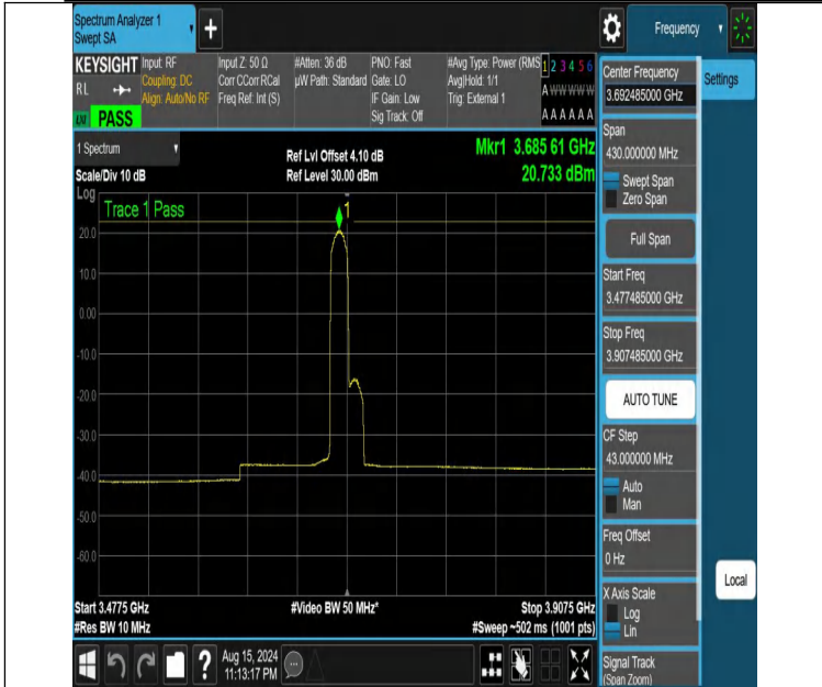
NTNV-DC_13A_n48A-PC3-30-5+15-M+H-N/A-N/A-DFT-QPSK-Edge_1RB_Left-3477.485-3907.485-PASS
