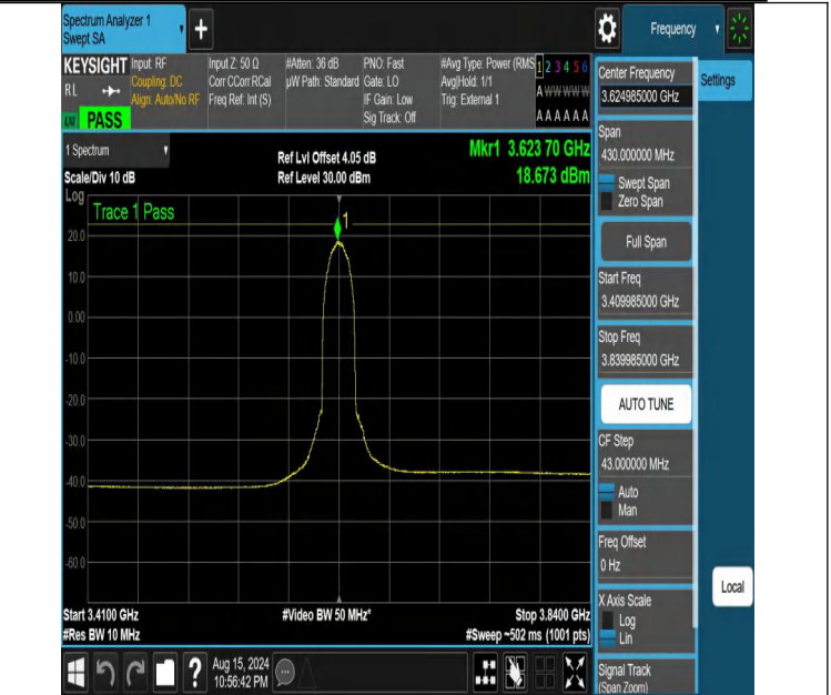
NTVN-DC_13A_n48A-PC3-30-5+15-M+M-N/A-N/A-DFT-16QAM-Ou ter_Full-3409.985-3839.985-PASS
