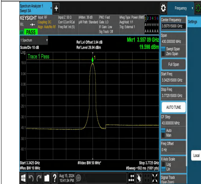
NTNV-DC_13A_n48A-PC3-30-5+15-M+L-N/A-N/A-DFT-64QAM-Inner_Full-3342.515-3772.515-PASS
