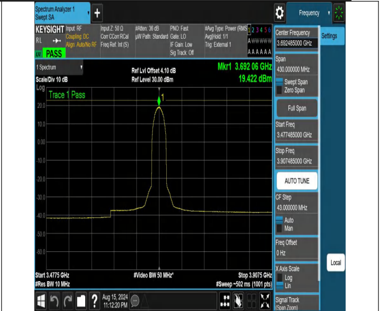
NTNV-DC_13A_n48A-PC3-30-5+15-M+H-N/A-N/A-DFT-QPSK-Outer_Full-3477.485-3907.485-PASS
