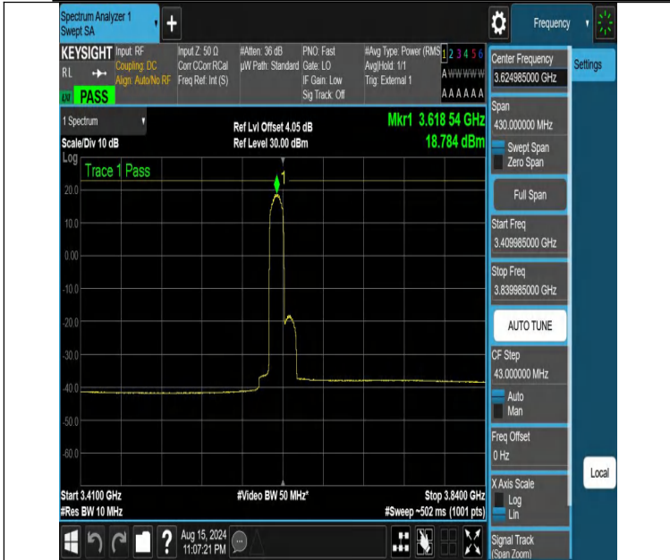
NTNV-DC_13A_n48A-PC3-30-5+15-M+M-N/A-N/A-CP-64QAM-Edge_1RB_Left-3409.985-3839.985-PASS
