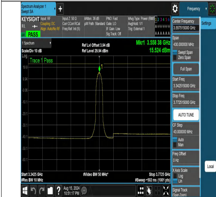
NTNV-DC_13A_n48A-PC3-30-5+15-M+L-N/A-N/A-CP-256QAM-Inner_Full-3342.515-3772.515-PASS
