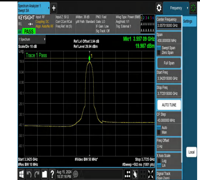
NTNV-DC_13A_n48A-PC3-30-5+15-M+L-N/A-N/A-DFT-QPSK-Outer_Full-3342.515-3772.515-PASS
