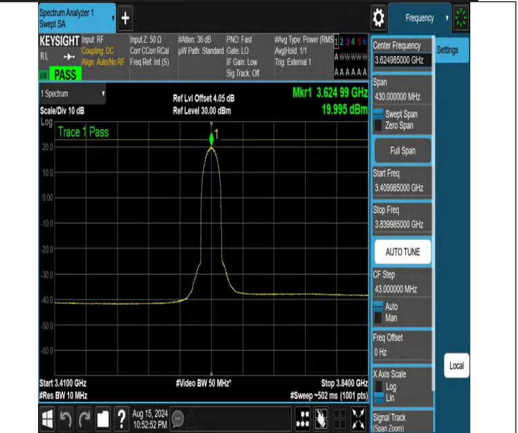
NTNV-DC_13A_n48A-PC3-30-5+15-M+M-N/A-N/A-DFT-PI2BPSK-Outer_Full-3409.985-3839.985-PASS
