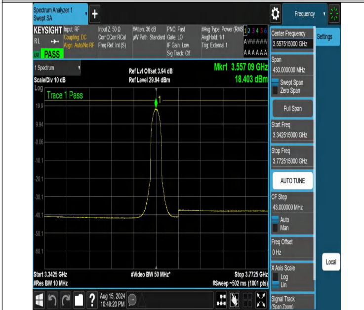
NTVN-DC_13A_n48A-PC3-30-5+15-M+L-N/A-N/A-CP-64QAM-Inner_Full-3342.515-3772.515-PASS
