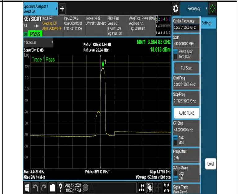
NTVN-DC_13A_n48A-PC3-30-5+15-M+L-N/A-N/A-CP-64QAM-Edge_1RB_Right-3342.515-3772.515-PASS
