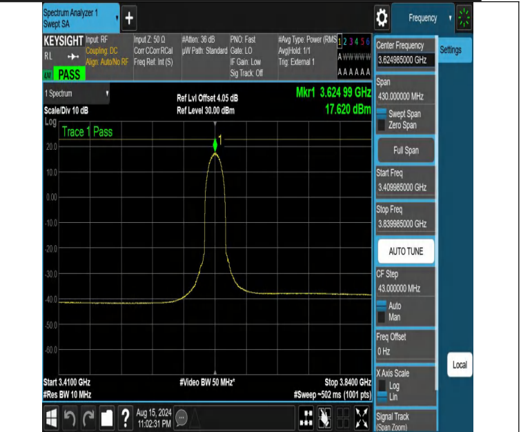
NTVN-DC_13A_n48A-PC3-30-5+15-M+M-N/A-N/A-CP-QPSK-Outer_Full-3409.985-3839.985-PASS
