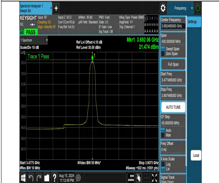
NTNV-DC_13A_n48A-PC3-30-5+15-M+H-N/A-N/A-DFT-QPSK-Inner_Full-3477.485-3907.485-PASS
