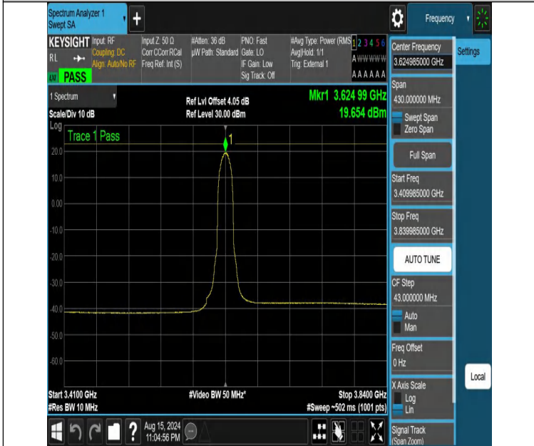
NTNV-DC_13A_n48A-PC3-30-5+15-M+M-N/A-N/A-CP-16QAM-Inner_Full-3409.985-3839.985-PASS
