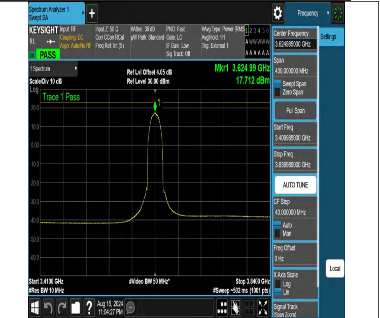
NTNV-DC_13A_n48A-PC3-30-5+15-M+M-N/A-N/A-CP-16QAM-Outer_Full-3409.985-3839.985-PASS
