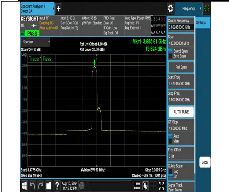
NTNV-DC_13A_n48A-PC3-30-5+15-M+H-N/A-N/A-DFT-16QAM-E dge_1RB_Left-3477.485-3907.485-PASS
