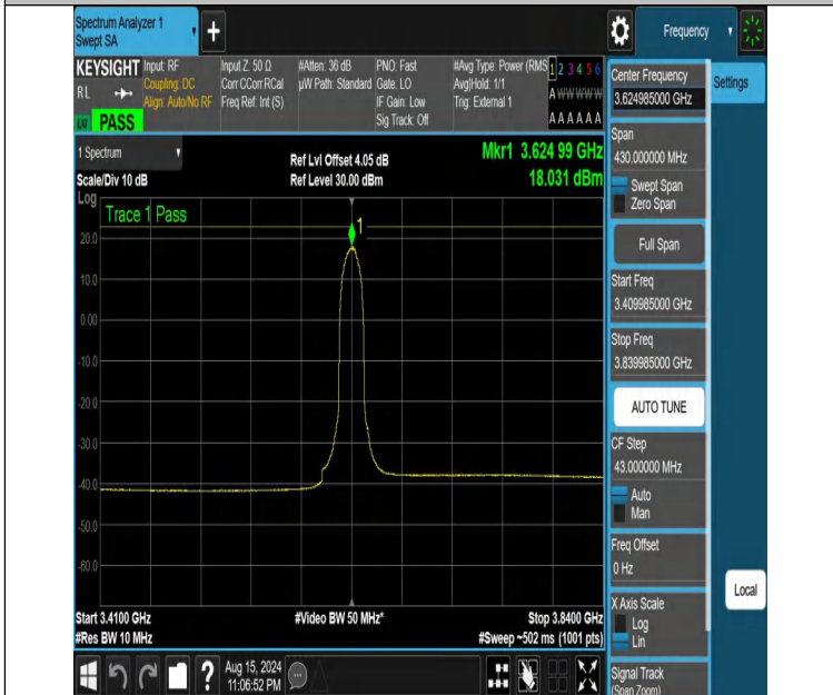
NTNV-DC_13A_n48A-PC3-30-5+15-M+M-N/A-N/A-CP-64QAM-Inner_Full-3409.985-3839.985-PASS
