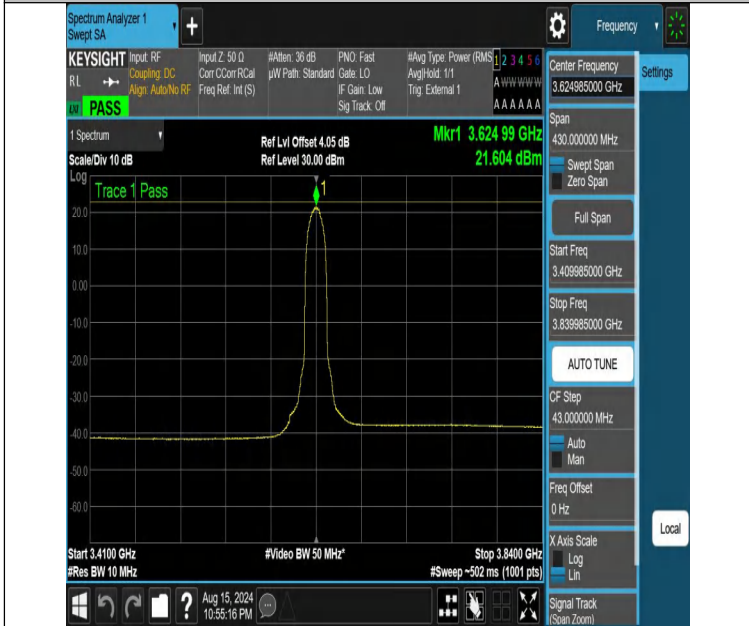
NTNV-DC_13A_n48A-PC3-30-5+15-M+M-N/A-N/A-DFT-QPSK-Inner_Full-3409.985-3839.985-PASS
