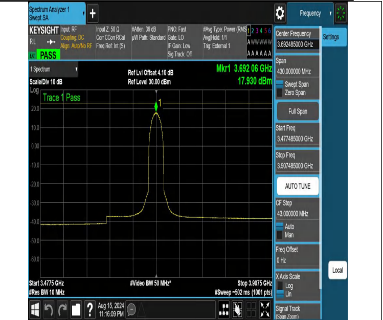
NTNV-DC_13A_n48A-PC3-30-5+15-M+H-N/A-N/A-DFT-64QAM-Ou ter_Full-3477.485-3907.485-PASS
