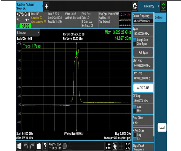
NTVN-DC_13A_n48A-PC3-30-5+15-M+M-N/A-N/A-CP-256QAM-In ner_Full-3409.985-3839.985-PASS
