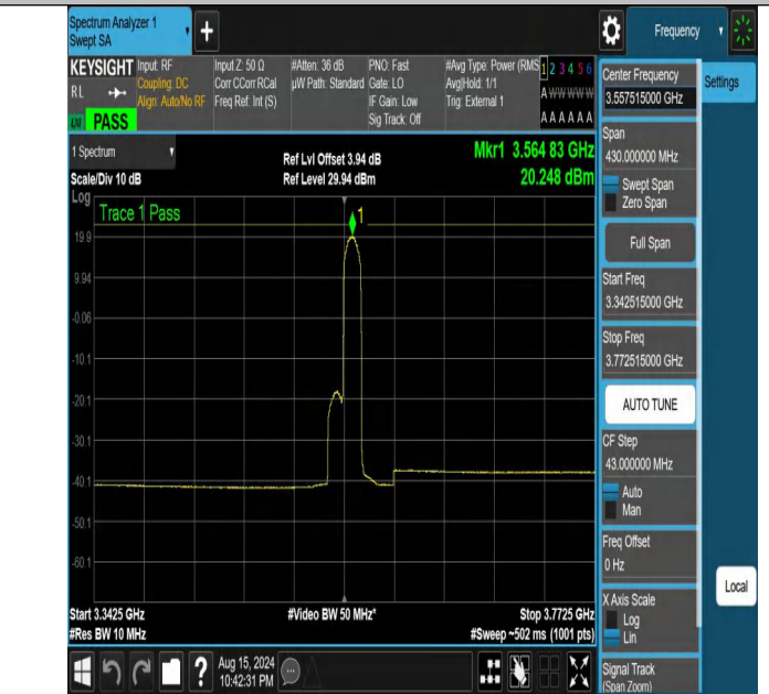
NTNV-DC_13A_n48A-PC3-30-5+15-M+L-N/A-N/A-DFT-64QAM-Edge_1RB_Right-3342.515-3772.515-PASS
