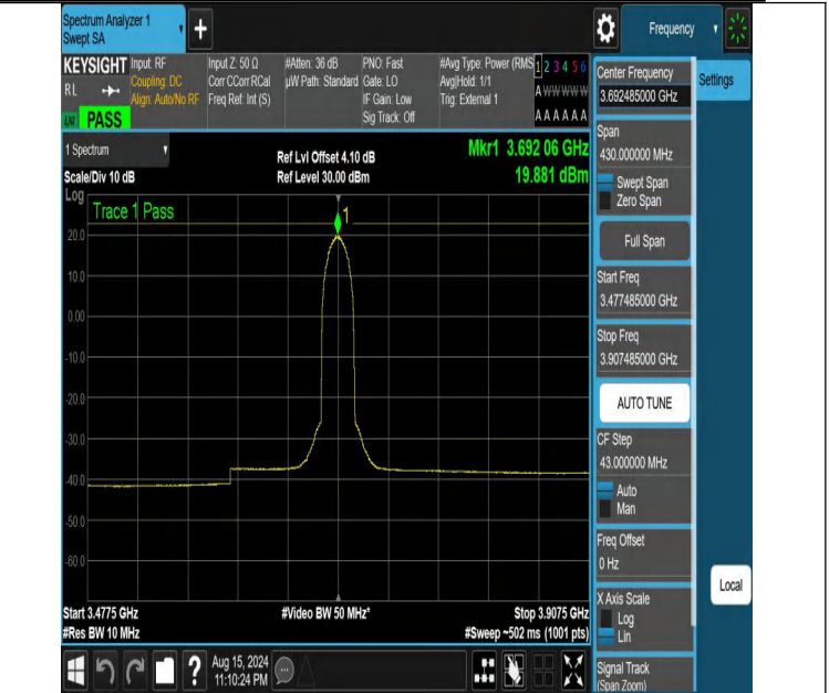
NTVN-DC_13A_n48A-PC3-30-5+15-M+H-N/A-N/A-DFT-PI2BPSK-Outer_Full-3477.485-3907.485-PASS
