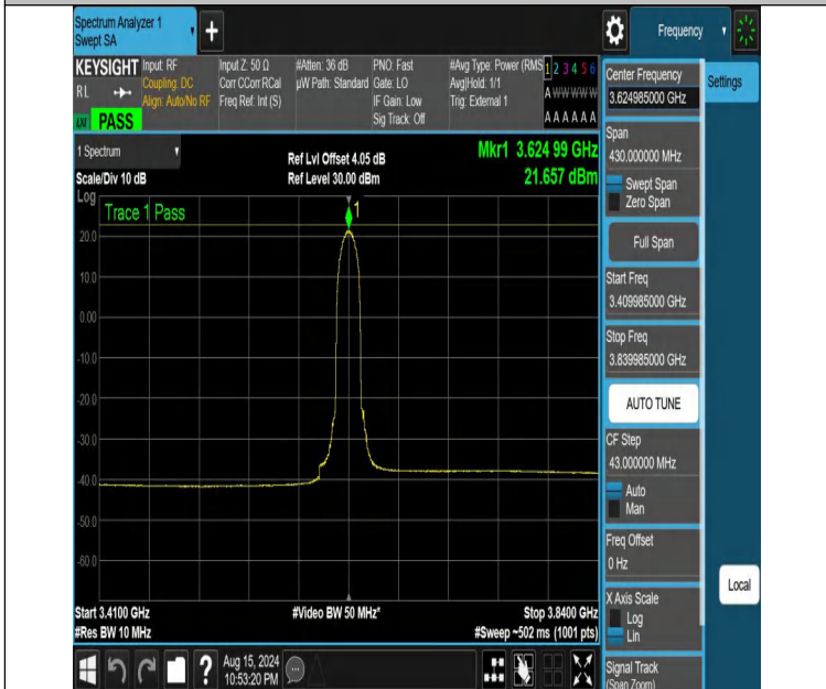
NTNV-DC_13A_n48A-PC3-30-5+15-M+M-N/A-N/A-DFT-PI2BPSK-I nner_Full-3409.985-3839.985-PASS
