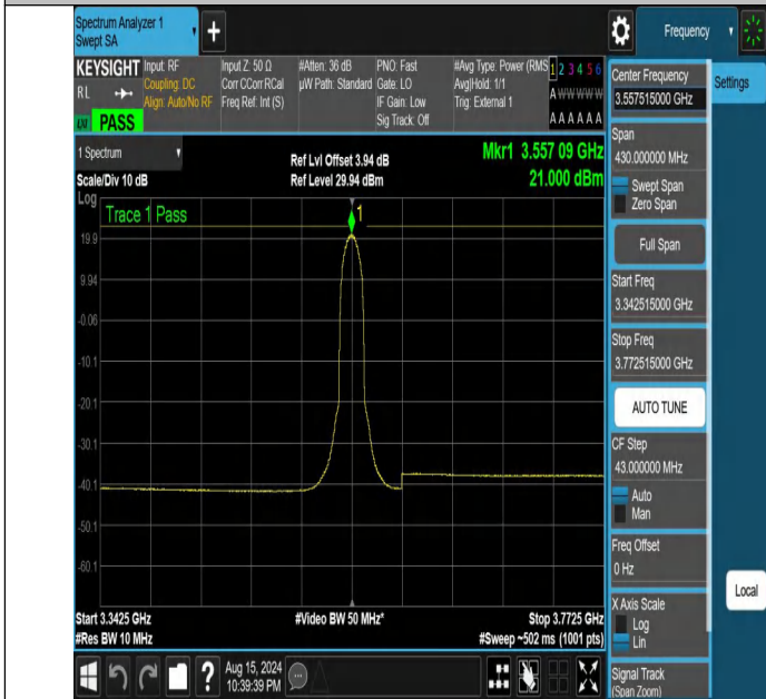
NTNV-DC_13A_n48A-PC3-30-5+15-M+L-N/A-N/A-DFT-16QAM-Inner_Full-3342.515-3772.515-PASS
