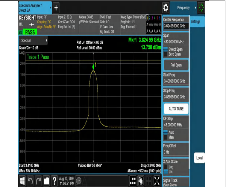
NTVN-DC_13A_n48A-PC3-30-5+15-M+M-N/A-N/A-CP-256QAM-Ou ter_Full-3409.985-3839.985-PASS
