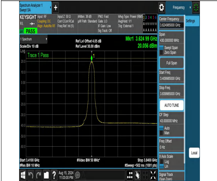
NTVN-DC_13A_n48A-PC3-30-5+15-M+M-N/A-N/A-CP-QPSK-Inner_Full-3409.985-3839.985-PASS
