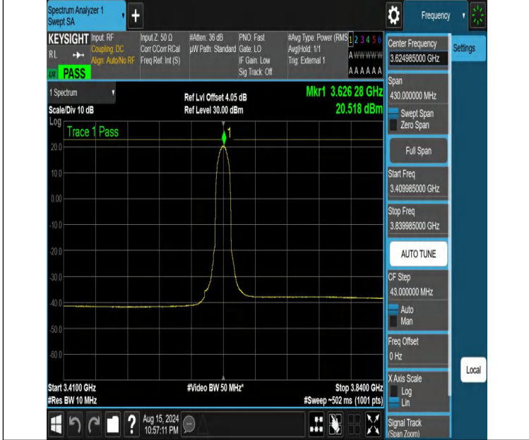
NTVN-DC_13A_n48A-PC3-30-5+15-M+M-N/A-N/A-DFT-16QAM-In ner_Full-3409.985-3839.985-PASS
