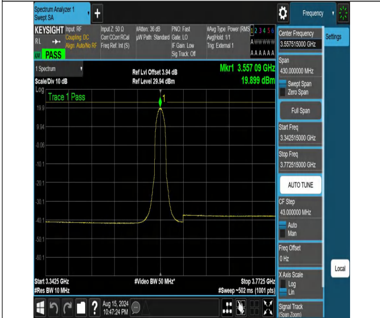
NTVN-DC_13A_n48A-PC3-30-5+15-M+L-N/A-N/A-CP-16QAM-Inner_Full-3342.515-3772.515-PASS
