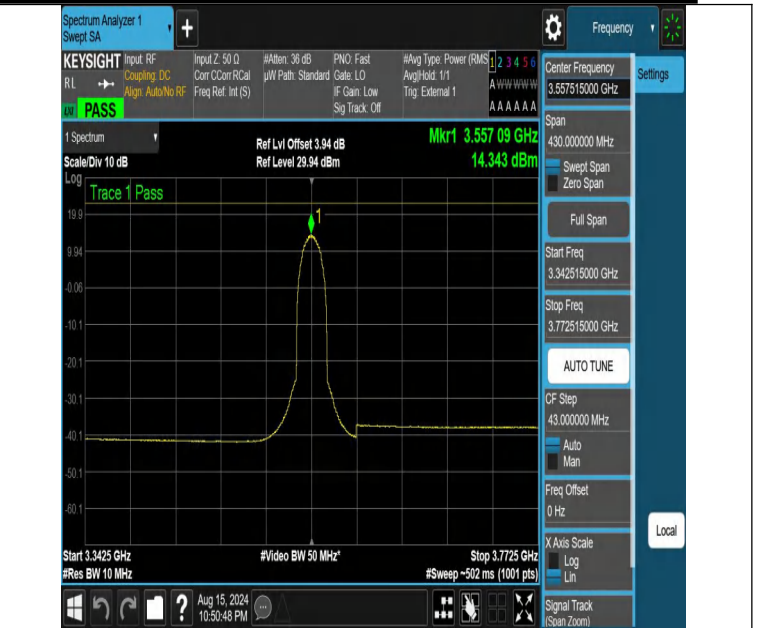
NTNV-DC_13A_n48A-PC3-30-5+15-M+L-N/A-N/A-CP-256QAM-Outer_Full-3342.515-3772.515-PASS
