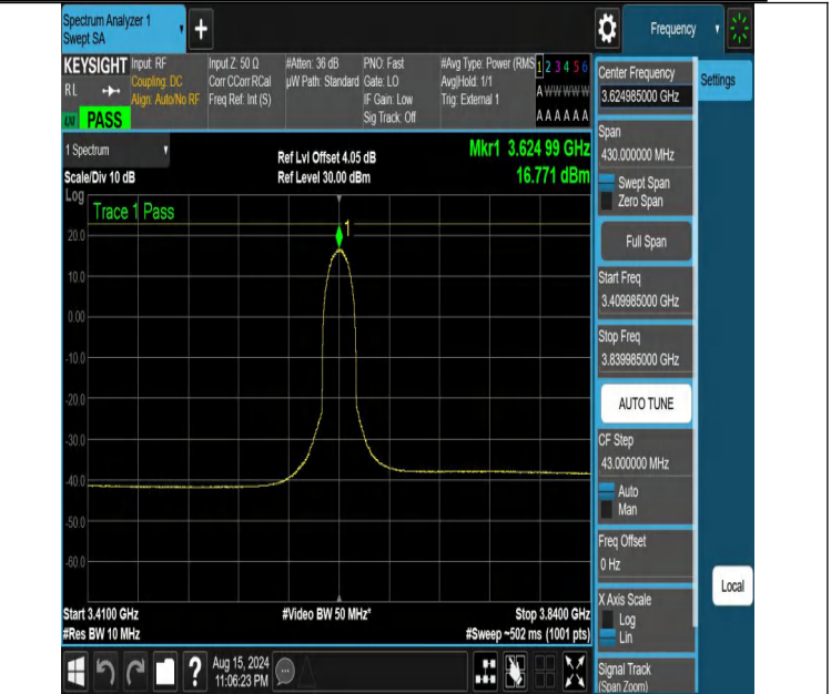
NTNV-DC_13A_n48A-PC3-30-5+15-M+M-N/A-N/A-CP-64QAM-Outer_Full-3409.985-3839.985-PASS
