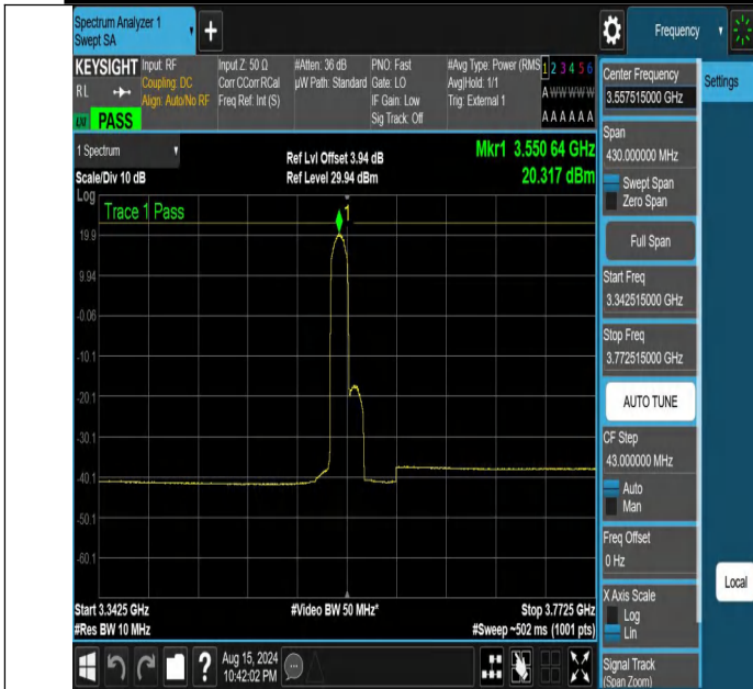
NTNV-DC_13A_n48A-PC3-30-5+15-M+L-N/A-N/A-DFT-64QAM-Edge_1RB_Left-3342.515-3772.515-PASS
