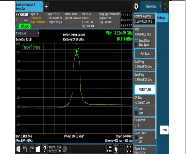
NTNV-DC_13A_n48A-PC3-30-5+15-M+M-N/A-N/A-DFT-64QAM-Ou ter_Full-3409.985-3839.985-PASS
