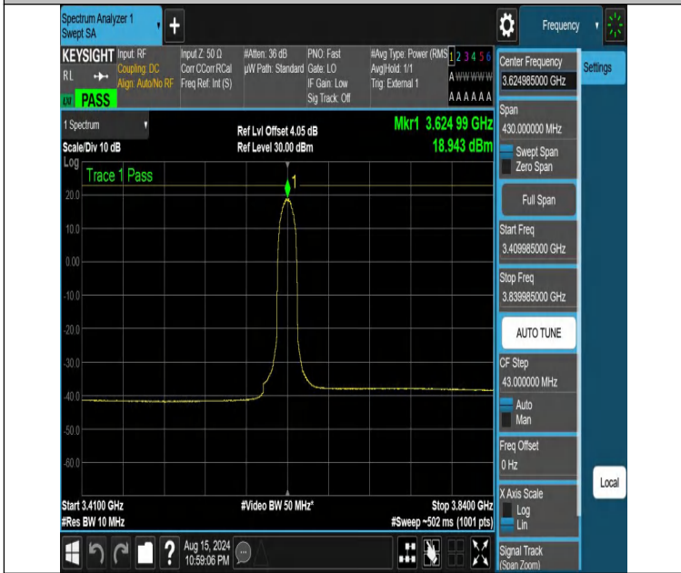
NTNV-DC_13A_n48A-PC3-30-5+15-M+M-N/A-N/A-DFT-64QAM-In ner_Full-3409.985-3839.985-PASS
