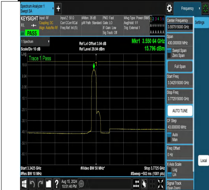
NTNV-DC_13A_n48A-PC3-30-5+15-M+L-N/A-N/A-CP-256QAM-Edge_1RB_Left-3342.515-3772.515-PASS
