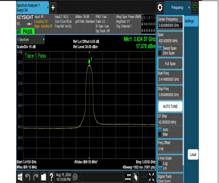
NTNV-DC_13A_n48A-PC3-30-5+10-M+M-N/A-N/A-CP-64QAM-Outer_Full-3414.985-3834.985-PASS
