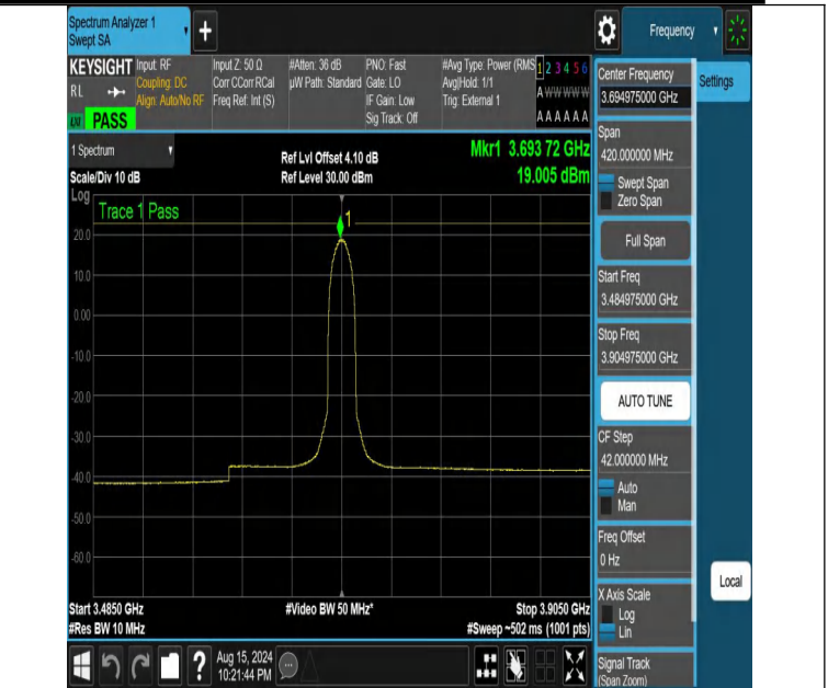
NTNV-DC_13A_n48A-PC3-30-5+10-M+H-N/A-N/A-DFT-16QAM-Ou ter_Full-3484.975-3904.975-PASS
