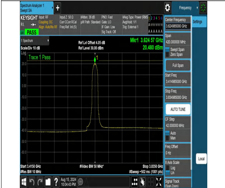
NTNV-DC_13A_n48A-PC3-30-5+10-M+M-N/A-N/A-DFT-16QAM-In ner_Full-3414.985-3834.985-PASS
