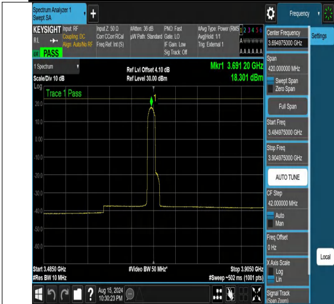
NTNV-DC_13A_n48A-PC3-30-5+10-M+H-N/A-N/A-CP-16QAM-Edge_1RB_Left-3484.975-3904.975-PASS
