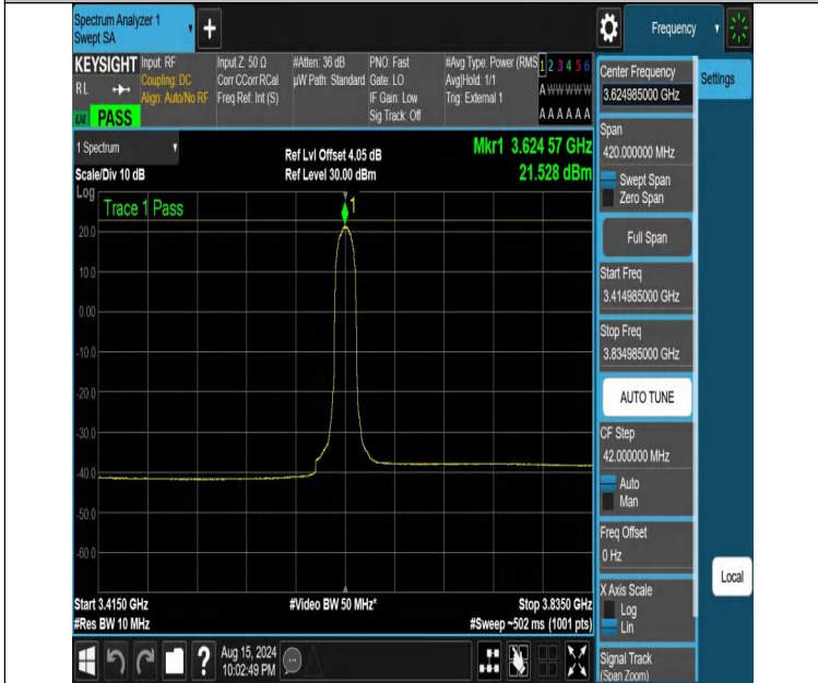
NTNV-DC_13A_n48A-PC3-30-5+10-M+M-N/A-N/A-DFT-QPSK-Inner_Full-3414.985-3834.985-PASS
