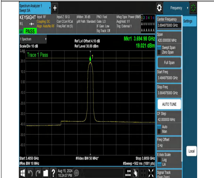
NTNV-DC_13A_n48A-PC3-30-5+10-M+H-N/A-N/A-DFT-64QAM-In ner_Full-3484.975-3904.975-PASS
