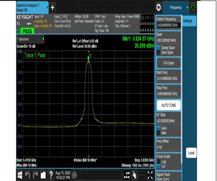
NTNV-DC_13A_n48A-PC3-30-5+10-M+M-N/A-N/A-DFT-QPSK-Outer_Full-3414.985-3834.985-PASS
