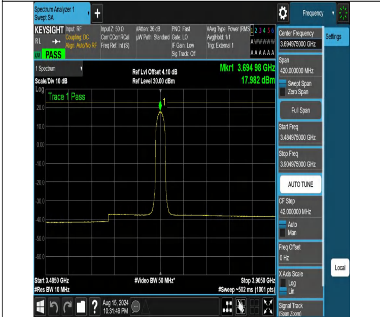
NTNV-DC_13A_n48A-PC3-30-5+10-M+H-N/A-N/A-CP-64QAM-Inner_Full-3484.975-3904.975-PASS
