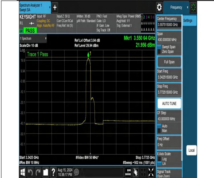
NTNV-DC_13A_n48A-PC3-30-5+15-M+L-N/A-N/A-DFT-PI2BPSK-Edge_1RB_Left-3342.515-3772.515-PASS
