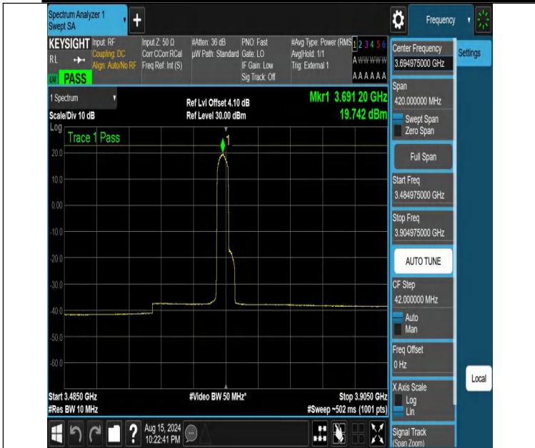
NTNV-DC_13A_n48A-PC3-30-5+10-M+H-N/A-N/A-DFT-16QAM-E dge_1RB_Left-3484.975-3904.975-PASS
