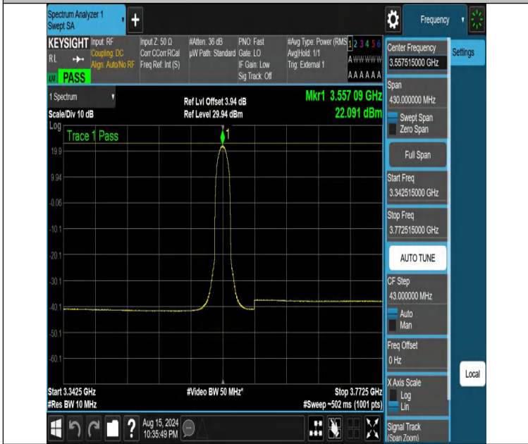
NTNV-DC_13A_n48A-PC3-30-5+15-M+L-N/A-N/A-DFT-PI2BPSK-I_nner_Full-3342.515-3772.515-PASS
