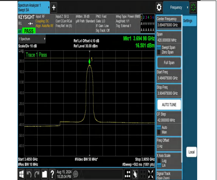
NTNV-DC_13A_n48A-PC3-30-5+10-M+H-N/A-N/A-DFT-256QAM-Outer_Full-3484.975-3904.975-PASS
