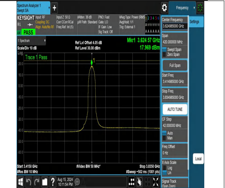
NTNV-DC_13A_n48A-PC3-30-5+10-M+M-N/A-N/A-CP-16QAM-Outer_Full-3414.985-3834.985-PASS
