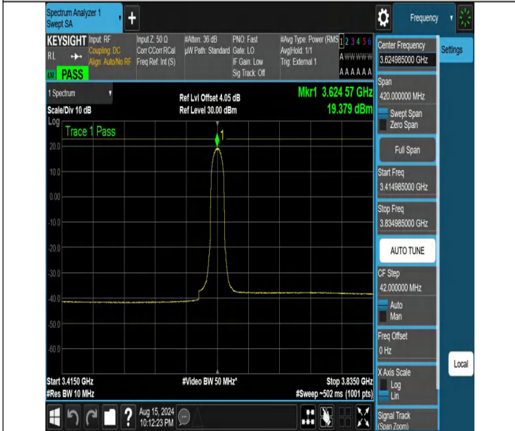
NTNV-DC_13A_n48A-PC3-30-5+10-M+M-N/A-N/A-CP-16QAM-Inner_Full-3414.985-3834.985-PASS
