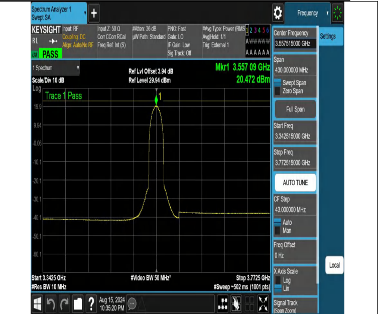
NTNV-DC_13A_n48A-PC3-30-5+15-M+L-N/A-N/A-DFT-PI2BPSK-Outer_Full-3342.515-3772.515-PASS
