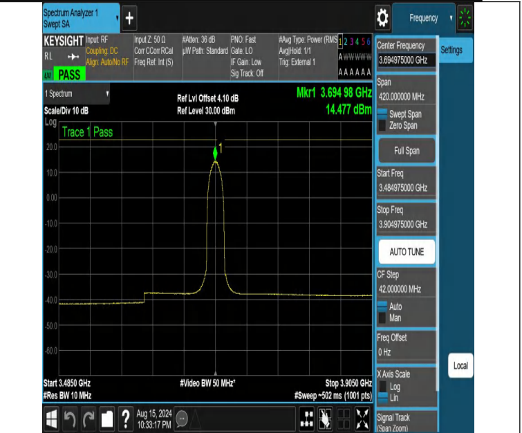
NTNV-DC_13A_n48A-PC3-30-5+10-M+H-N/A-N/A-CP-256QAM-Ou ter_Full-3484.975-3904.975-PASS
