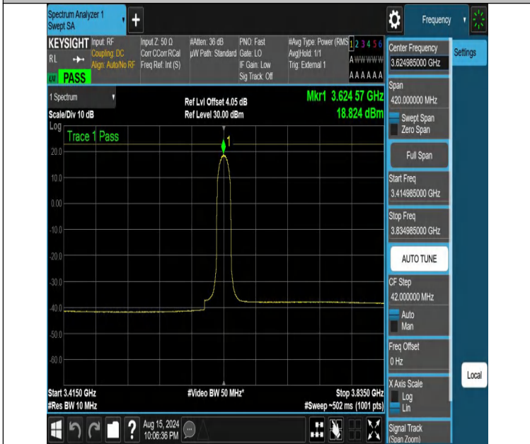
NTNV-DC_13A_n48A-PC3-30-5+10-M+M-N/A-N/A-DFT-64QAM-In ner_Full-3414.985-3834.985-PASS
