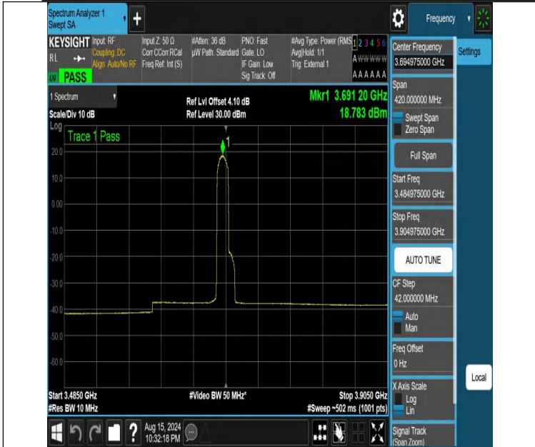
NTNV-DC_13A_n48A-PC3-30-5+10-M+H-N/A-N/A-CP-64QAM-Edge_1RB_Left-3484.975-3904.975-PASS
