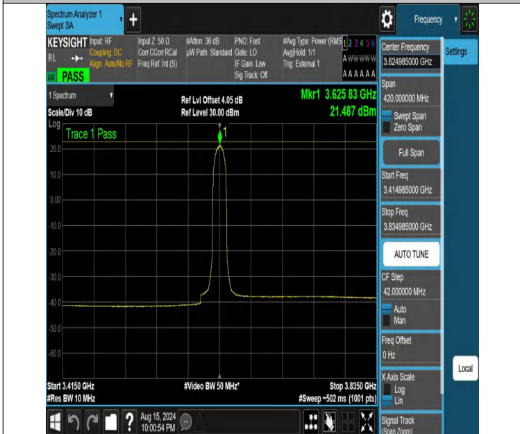
NTNV-DC_13A_n48A-PC3-30-5+10-M+M-N/A-N/A-DFT-PI2BPSK-I nner_Full-3414.985-3834.985-PASS
