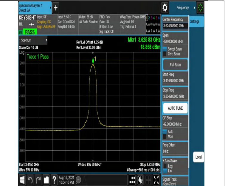
NTNV-DC_13A_n48A-PC3-30-5+10-M+M-N/A-N/A-DFT-16QAM-Ou ter_Full-3414.985-3834.985-PASS
