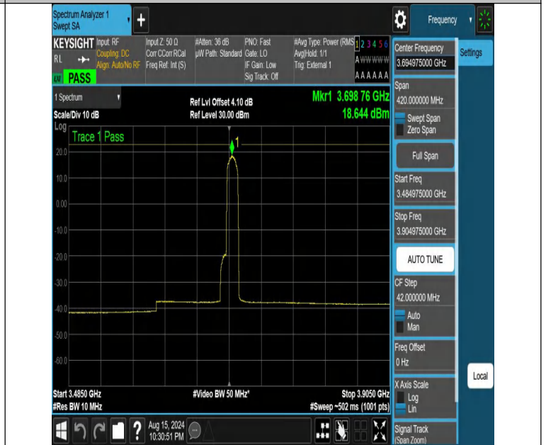
NTNV-DC_13A_n48A-PC3-30-5+10-M+H-N/A-N/A-CP-16QAM-Edge_1RB_Right-3484.975-3904.975-PASS
