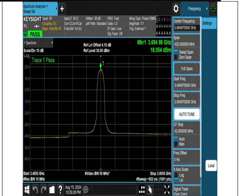
NTNV-DC_13A_n48A-PC3-30-5+10-M+H-N/A-N/A-CP-16QAM-Outer_Full-3484.975-3904.975-PASS
