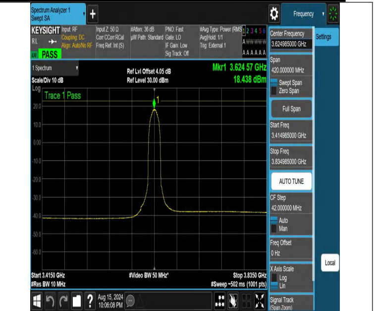
NTNV-DC_13A_n48A-PC3-30-5+10-M+M-N/A-N/A-DFT-64QAM-Ou ter_Full-3414.985-3834.985-PASS
