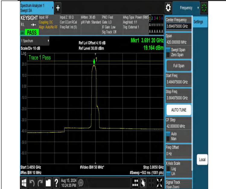
NTNV-DC_13A_n48A-PC3-30-5+10-M+H-N/A-N/A-DFT-64QAM-E dge_1RB_Left-3484.975-3904.975-PASS
