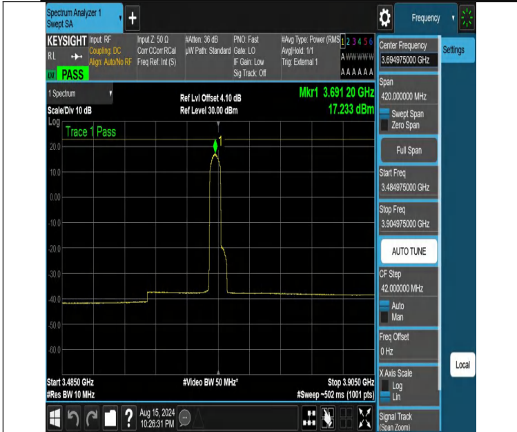
NTNV-DC_13A_n48A-PC3-30-5+10-M+H-N/A-N/A-DFT-256QAM-Edge_1RB_Left-3484.975-3904.975-PASS
