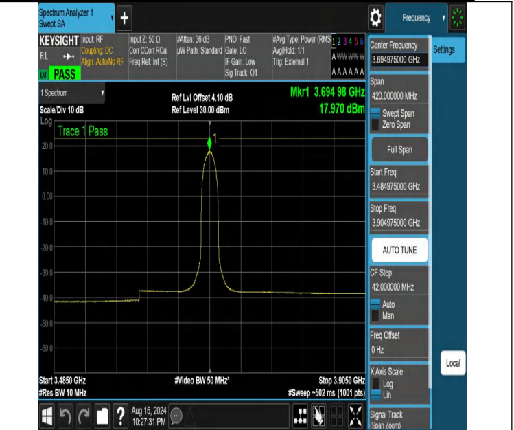
NTVN-DC_13A_n48A-PC3-30-5+10-M+H-N/A-N/A-CP-QPSK-Outer_Full-3484.975-3904.975-PASS
