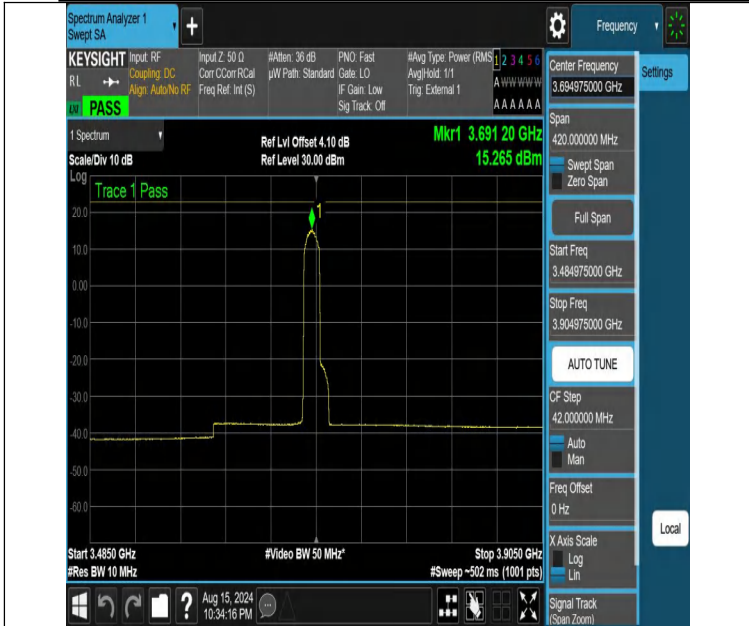
NTNV-DC_13A_n48A-PC3-30-5+10-M+H-N/A-N/A-CP-256QAM-E dge_1RB_Left-3484.975-3904.975-PASS
