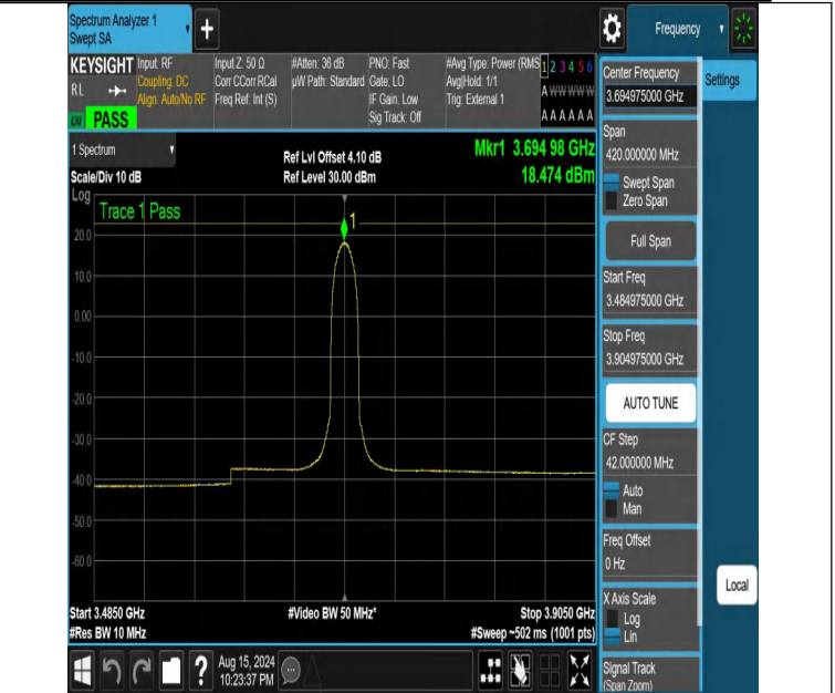
NTNV-DC_13A_n48A-PC3-30-5+10-M+H-N/A-N/A-DFT-64QAM-Ou ter_Full-3484.975-3904.975-PASS
