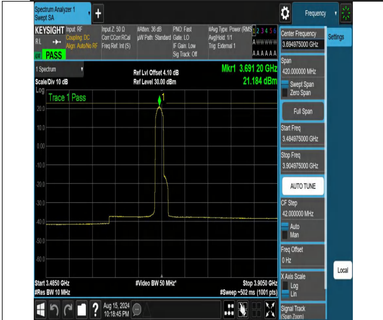
NTNV-DC_13A_n48A-PC3-30-5+10-M+H-N/A-N/A-DFT-PI2BPSK-Edge_1RB_Left-3484.975-3904.975-PASS
