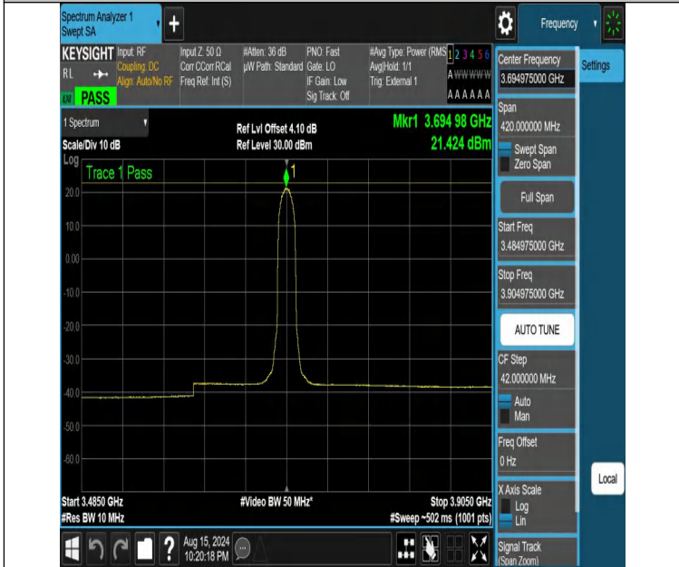
NTNV-DC_13A_n48A-PC3-30-5+10-M+H-N/A-N/A-DFT-QPSK-Inner_Full-3484.975-3904.975-PASS
