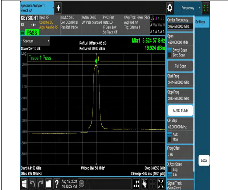
NTVN-DC_13A_n48A-PC3-30-5+10-M+M-N/A-N/A-CP-QPSK-Inner_Full-3414.985-3834.985-PASS
