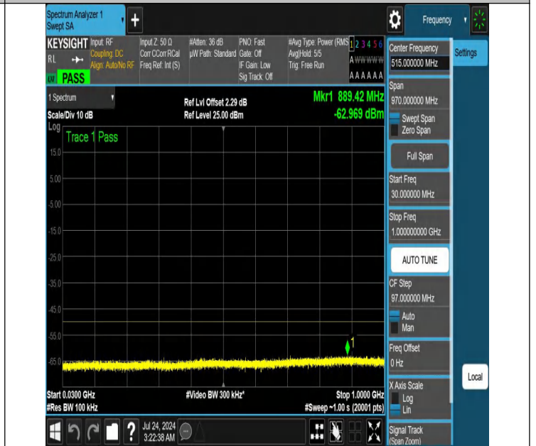
NTNV-N48-PC3-30-30-H-DFT-QPSK-Edge_1RB_Right-30-1000-Ant1-PASS
