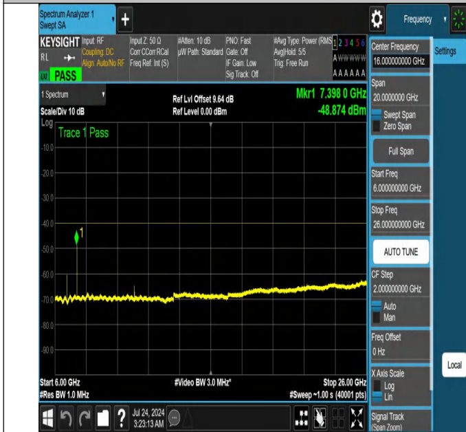
NTNV-N48-PC3-30-30-H-DFT-QPSK-Edge_1RB_Right-6000-260 00-Ant1-PASS
