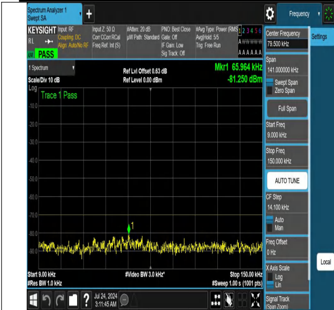
NTNV-N48-PC3-30-30-M-DFT-PI2BPSK-Edge_1RB_Left-0.009-0.15-Ant1-PASS
