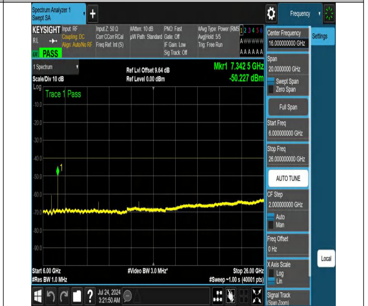
NTNV-N48-PC3-30-30-H-DFT-QPSK-Edge_1RB_Left-6000-26000 -Ant1-PASS
