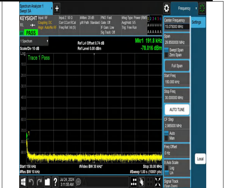
NTNV-N48-PC3-30-30-M-DFT-PI2BPSK-Edge_1RB_Left-0.15-30-Ant1-PASS
