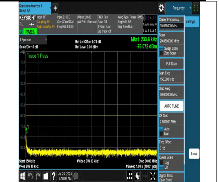
NTNV-N48-PC3-30-30-H-DFT-PI2BPSK-Edge_1RB_Left-0.15-30-Ant1-PASS
