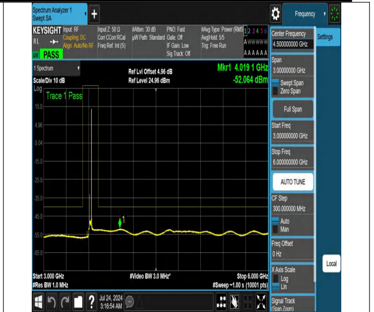
NTNV-N48-PC3-30-30-M-DFT-QPSK-Edge_1RB_Right-3000-600 0-Ant1-PASS
