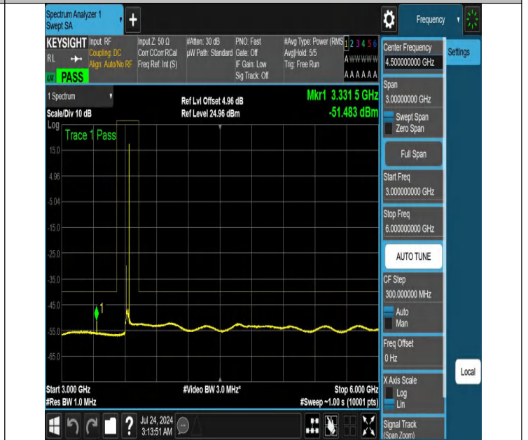
NTNV-N48-PC3-30-30-M-DFT-PI2BPSK-Edge_1RB_Right-3000-6000-Ant1-PASS
