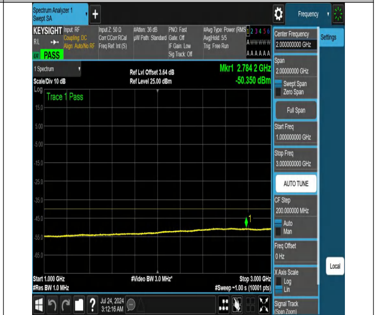
NTNV-N48-PC3-30-30-M-DFT-PI2BPSK-Edge_1RB_Left-1000-3000-Ant1-PASS
