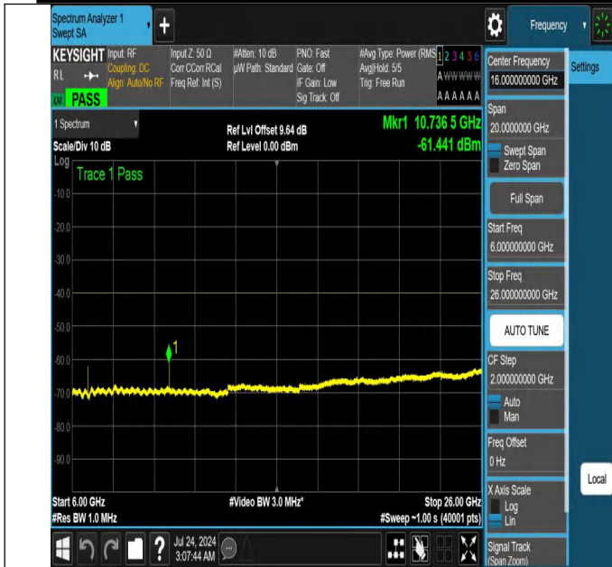
NTNV-N48-PC3-30-30-L-DFT-PI2BPSK-Edge_1RB_Right-6000-26000-Ant1-PASS
