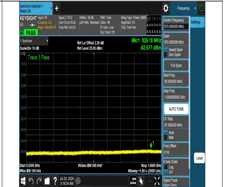
NTNV-N48-PC3-30-30-M-DFT-QPSK-Edge_1RB_Right-30-1000.000-Ant1-PASS
