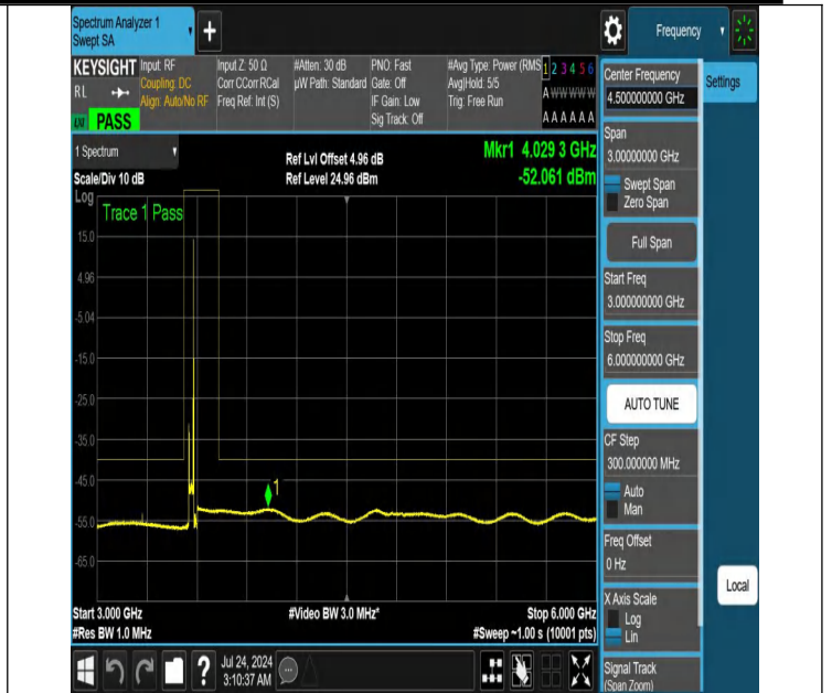
NTNV-N48-PC3-30-30-L-DFT-QPSK-Edge_1RB_Right-3000-6000 -Ant1-PASS
