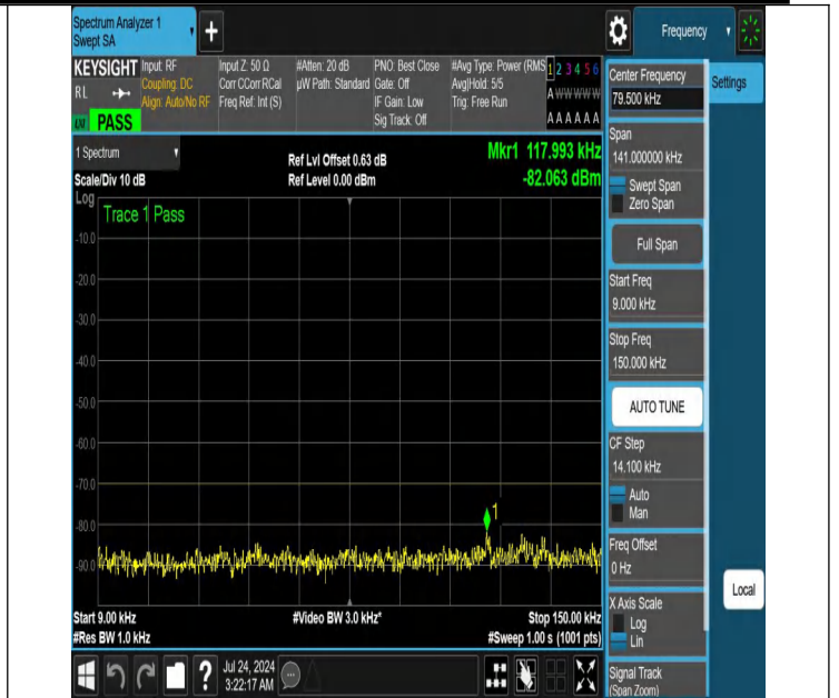
NTNV-N48-PC3-30-30-H-DFT-QPSK-Edge_1RB_Right-0.009-0.150-Ant1-PASS
