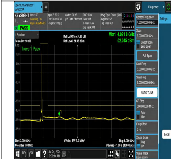
NTNV-N48-PC3-30-30-L-DFT-QPSK-Edge_1RB_Left-3000-6000-Ant1-PASS
