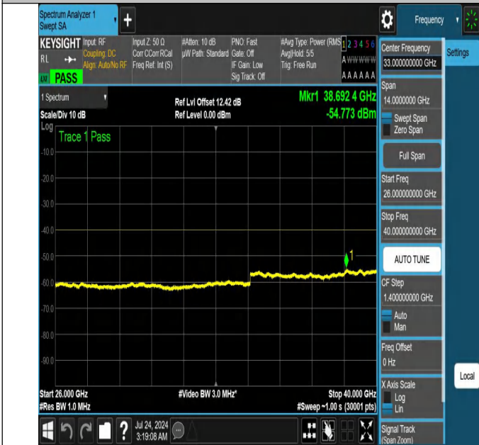
NTNV-N48-PC3-30-30-H-DFT-PI2BPSK-Edge_1RB_Left-26000-40000-Ant1-PASS
