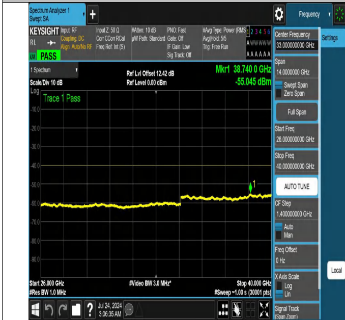
NTNV-N48-PC3-30-30-L-DFT-PI2BPSK-Edge_1RB_Left-26000-4 0000-Ant1-PASS
