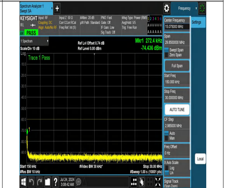
NTNV-N48-PC3-30-30-L-DFT-QPSK-Edge_1RB_Left-0.15-30-Ant1-PASS
