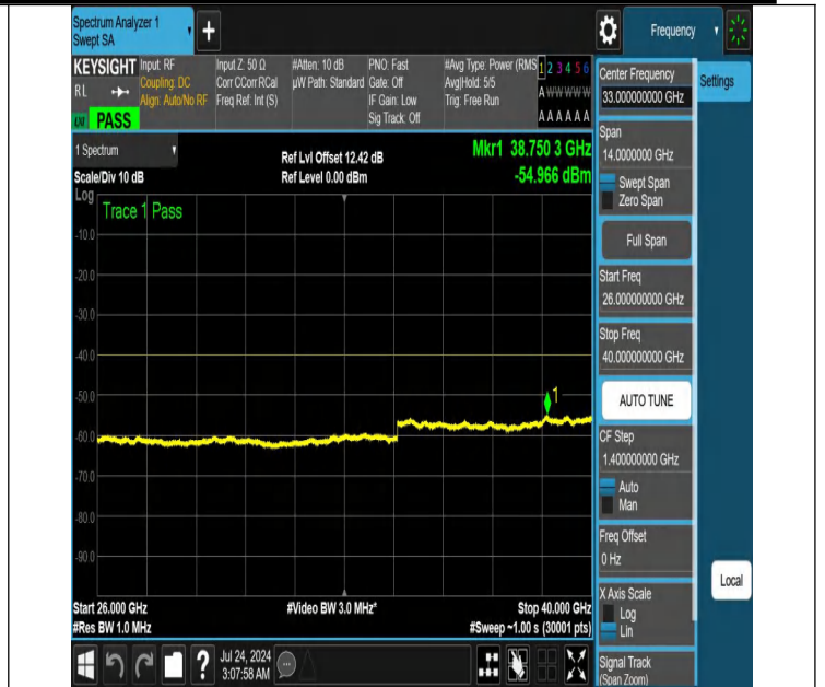
NTNV-N48-PC3-30-30-L-DFT-PI2BPSK-Edge_1RB_Right-26000-40000-Ant1-PASS
