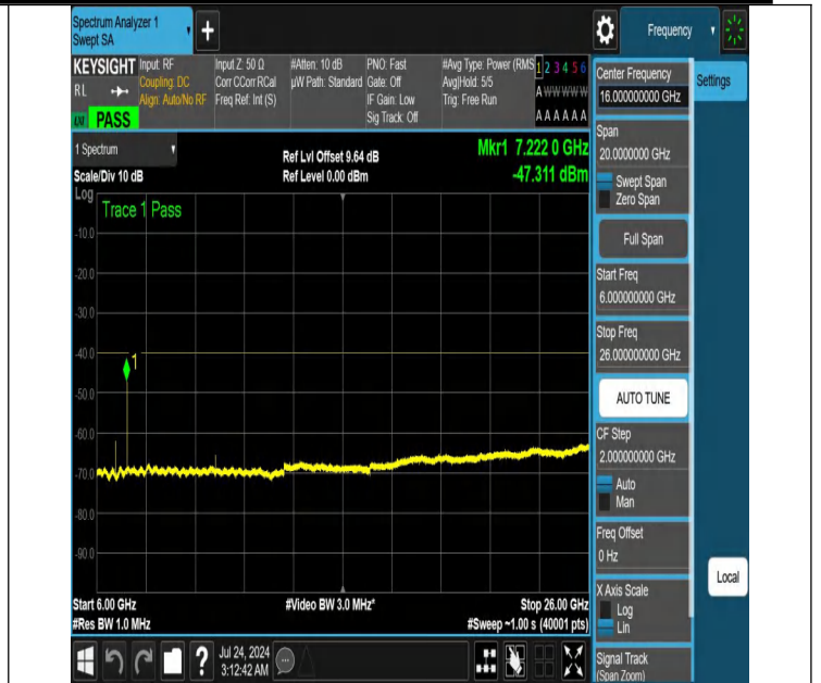
NTNV-N48-PC3-30-30-M-DFT-PI2BPSK-Edge_1RB_Left-6000-26000-Ant1-PASS
