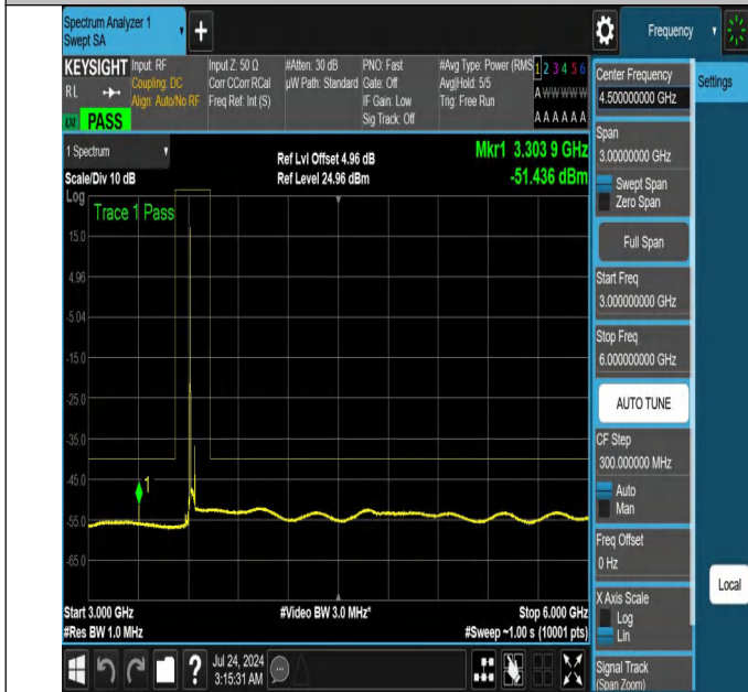
NTNV-N48-PC3-30-30-M-DFT-QPSK-Edge_1RB_Left-3000-6000-Ant1-PASS
