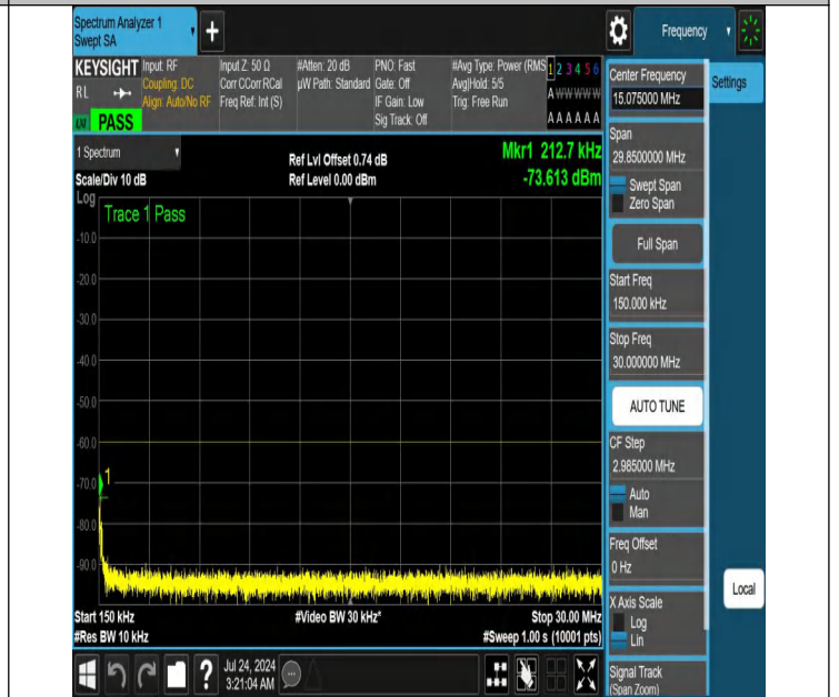
NTNV-N48-PC3-30-30-H-DFT-QPSK-Edge_1RB_Left-0.15-30-Ant1-PASS
