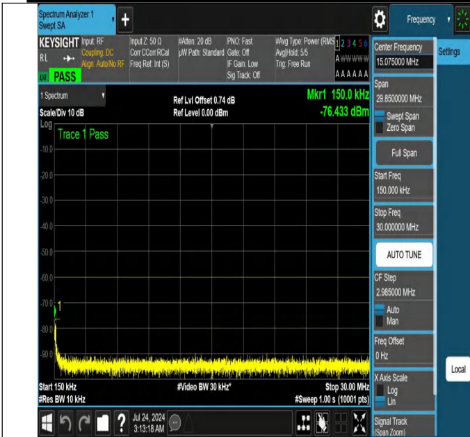
NTNV-N48-PC3-30-30-M-DFT-PI2BPSK-Edge_1RB_Right-0.15-30-Ant1-PASS
