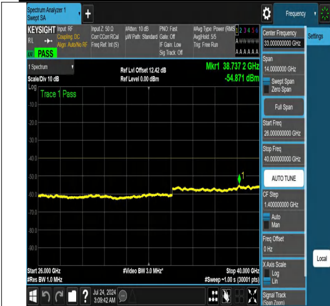
NTNV-N48-PC3-30-30-L-DFT-QPSK-Edge_1RB_Left-26000-40000-Ant1-PASS
