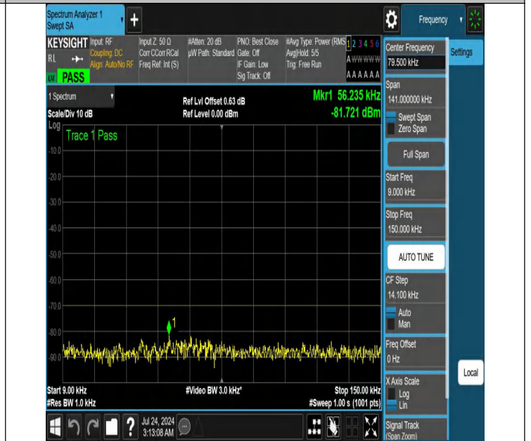
NTNV-N48-PC3-30-30-M-DFT-PI2BPSK-Edge_1RB_Right-0.009-0.15-Ant1-PASS
