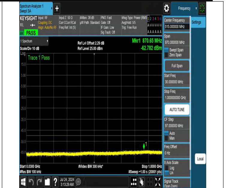
NTNV-N48-PC3-30-30-M-DFT-PI2BPSK-Edge_1RB_Right-30-100-0-Ant1-PASS
