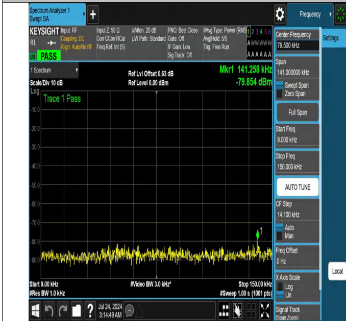
NTNV-N48-PC3-30-30-M-DFT-QPSK-Edge_1RB_Left-0.009-0.15-Ant1-PASS
