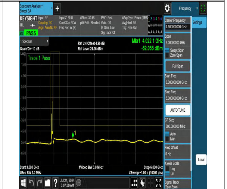
NTNV-N48-PC3-30-30-L-DFT-PI2BPSK-Edge_1RB_Right-3000-6000-Ant1-PASS
