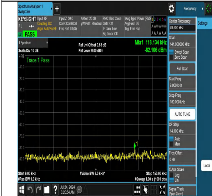
NTNV-N48-PC3-30-30-H-DFT-QPSK-Edge_1RB_Left-0.009-0.15-Ant1-PASS
