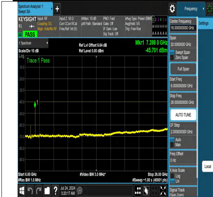
NTNV-N48-PC3-30-30-H-DFT-PI2BPSK-Edge_1RB_Right-6000-26000-Ant1-PASS
