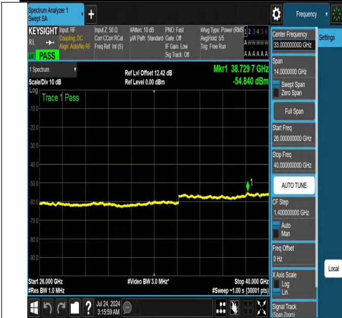
NTNV-N48-PC3-30-30-M-DFT-QPSK-Edge_1RB_Left-26000-40000-Ant1-PASS
