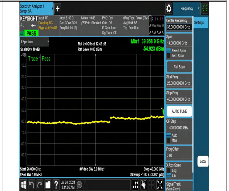
NTNV-N48-PC3-30-30-L-DFT-QPSK-Edge_1RB_Right-26000-400 00-Ant1-PASS
