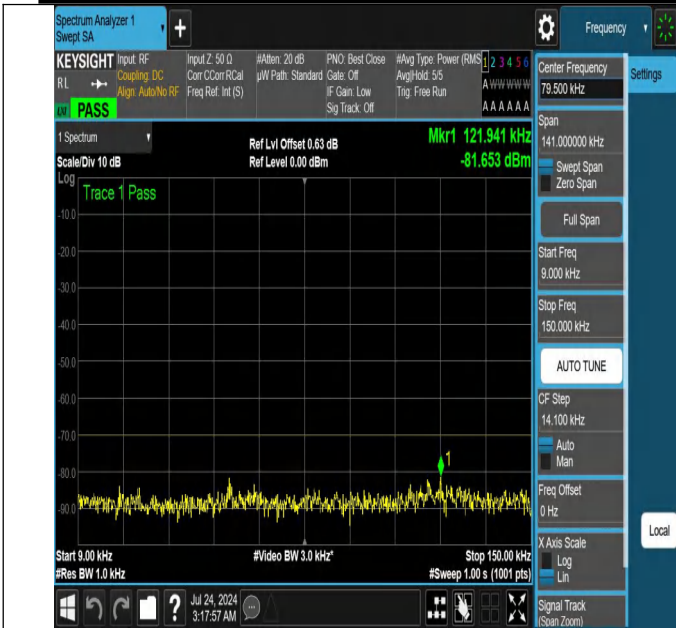
NTNV-N48-PC3-30-30-H-DFT-PI2BPSK-Edge_1RB_Left-0.009-0.15-Ant1-PASS
