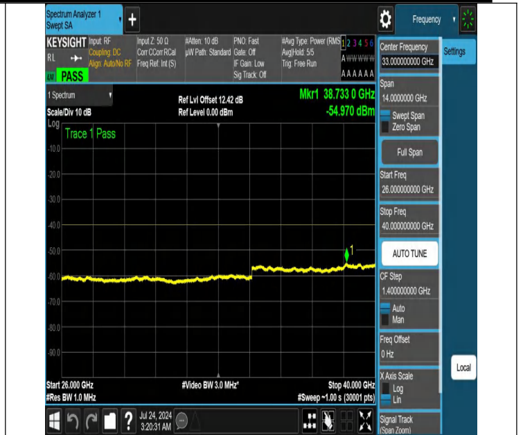
NTNV-N48-PC3-30-30-H-DFT-PI2BPSK-Edge_1RB_Right-26000-40000-Ant1-PASS
