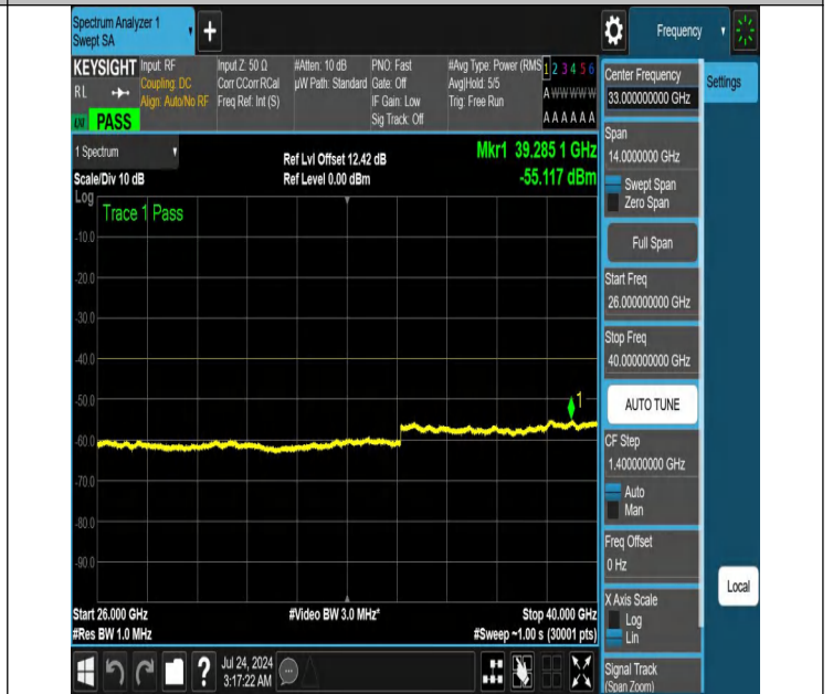
NTNV-N48-PC3-30-30-M-DFT-QPSK-Edge_1RB_Right-26000-40 000-Ant1-PASS
