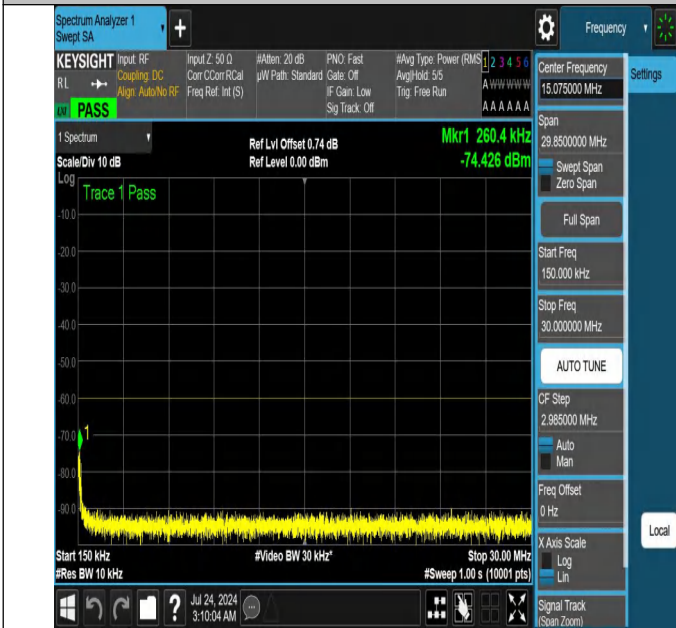
NTNV-N48-PC3-30-30-L-DFT-QPSK-Edge_1RB_Right-0.150-30.0-Ant1-PASS
