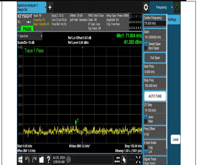
NTNV-N48-PC3-30-30-L-DFT-QPSK-Edge_1RB_Right-0.009-0.150-Ant1-PASS
