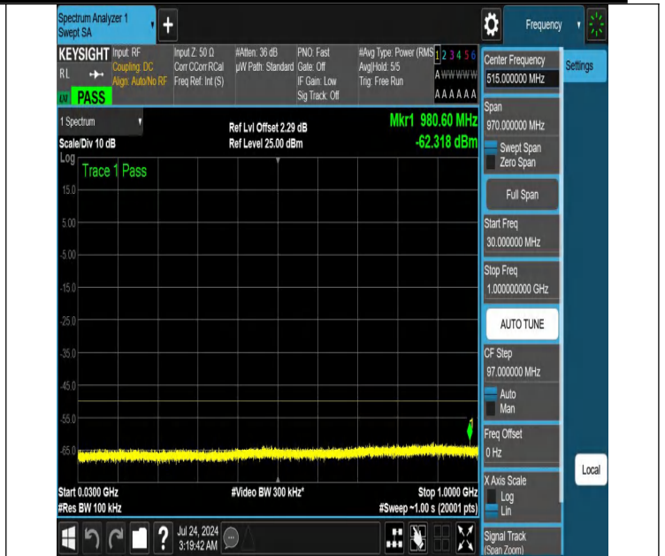
NTNV-N48-PC3-30-30-H-DFT-PI2BPSK-Edge_1RB_Right-30-100 0-Ant1-PASS
