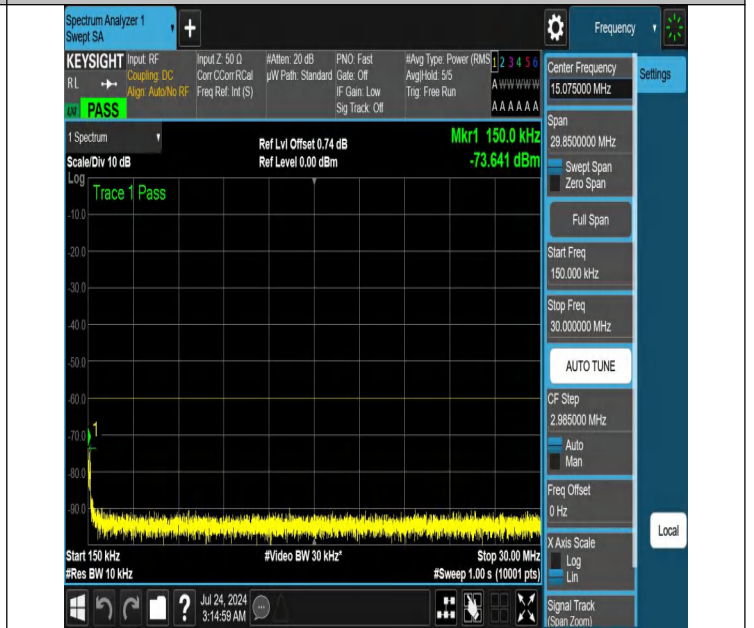
NTNV-N48-PC3-30-30-M-DFT-QPSK-Edge_1RB_Left-0.15-30-Ant1-PASS
