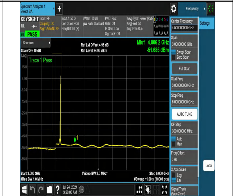
NTNV-N48-PC3-30-30-H-DFT-PI2BPSK-Edge_1RB_Right-3000-6000-Ant1-PASS
