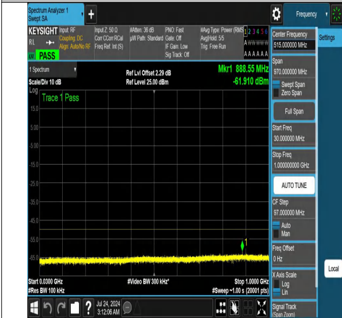
NTNV-N48-PC3-30-30-M-DFT-PI2BPSK-Edge_1RB_Left-30-1000-Ant1-PASS
