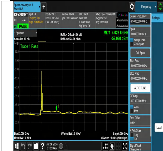
NTNV-N48-PC3-30-30-M-DFT-PI2BPSK-Edge_1RB_Left-3000-6000-Ant1-PASS
