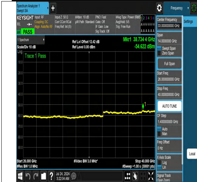
NTNV-N48-PC3-30-30-H-DFT-QPSK-Edge_1RB_Left-26000-40000-Ant1-PASS
