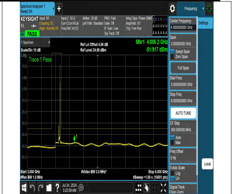
NTNV-N48-PC3-30-30-H-DFT-QPSK-Edge_1RB_Right-3000-600 0-Ant1-PASS
