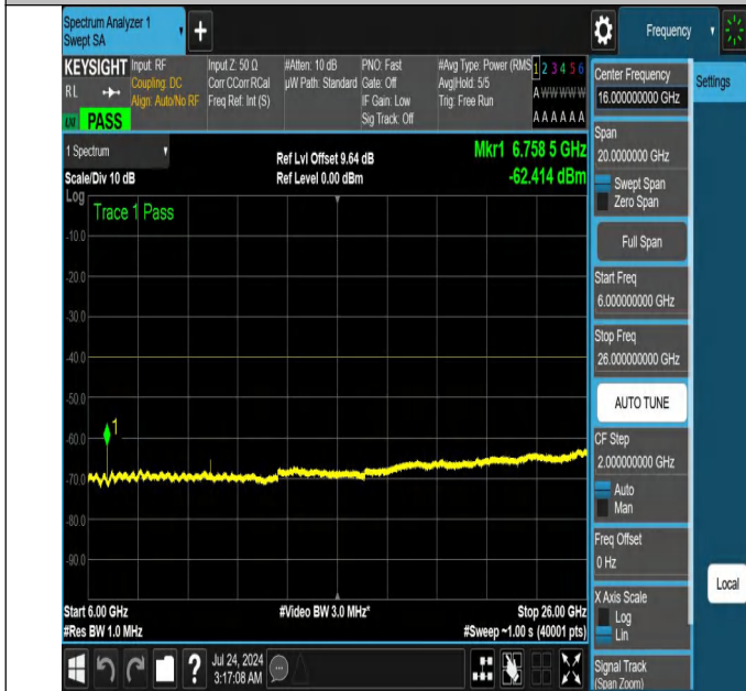
NTNV-N48-PC3-30-30-M-DFT-QPSK-Edge_1RB_Right-6000-26 000-Ant1-PASS
