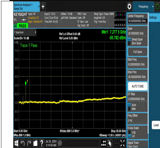
NTNV-N48-PC3-30-30-M-DFT-PI2BPSK-Edge_1RB_Right-6000-26000-Ant1-PASS
