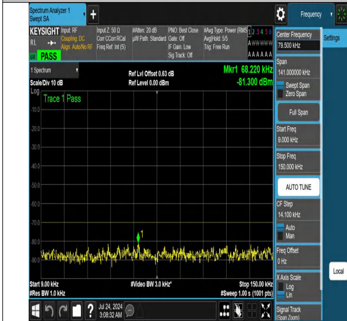
NTNV-N48-PC3-30-30-L-DFT-QPSK-Edge_1RB_Left-0.009-0.15-Ant1-PASS
