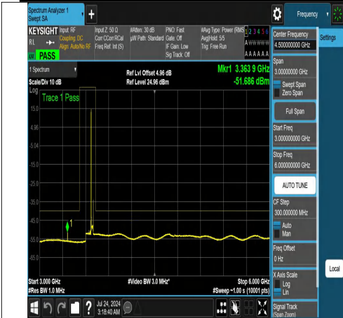
NTNV-N48-PC3-30-30-H-DFT-PI2BPSK-Edge_1RB_Left-3000-6000-Ant1-PASS
