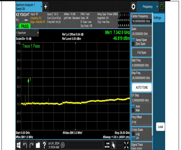
NTNV-N48-PC3-30-30-H-DFT-PI2BPSK-Edge_1RB_Left-6000-26000-Ant1-PASS
