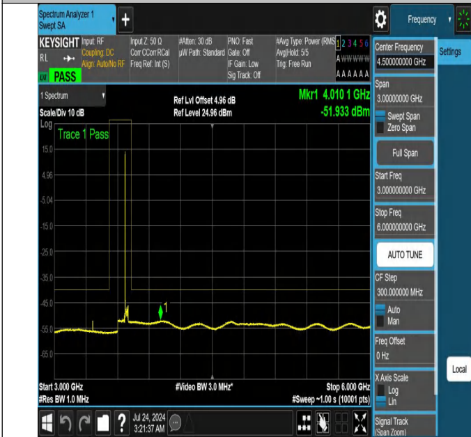
NTNV-N48-PC3-30-30-H-DFT-QPSK-Edge_1RB_Left-3000-6000 -Ant1-PASS
