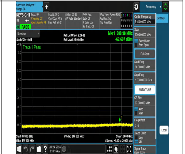
NTNV-N48-PC3-30-30-L-DFT-QPSK-Edge_1RB_Right-30-1000-Ant1-PASS
