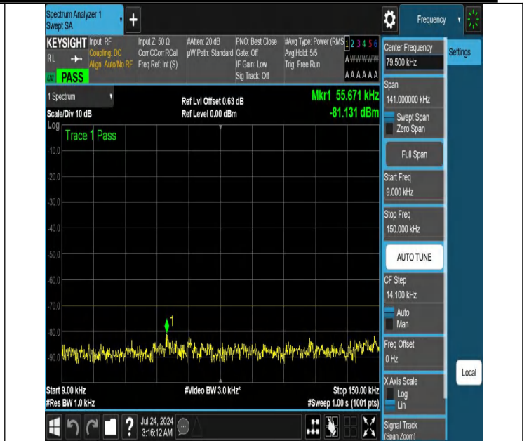
NTNV-N48-PC3-30-30-M-DFT-QPSK-Edge_1RB_Right-0.009-0.150-Ant1-PASS
