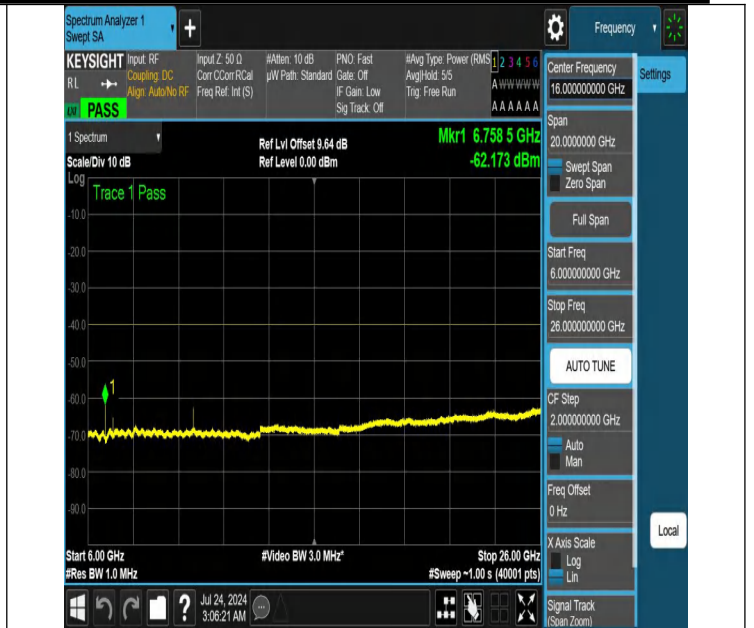
NTNV-N48-PC3-30-30-L-DFT-PI2BPSK-Edge_1RB_Left-6000-26 000-Ant1-PASS
