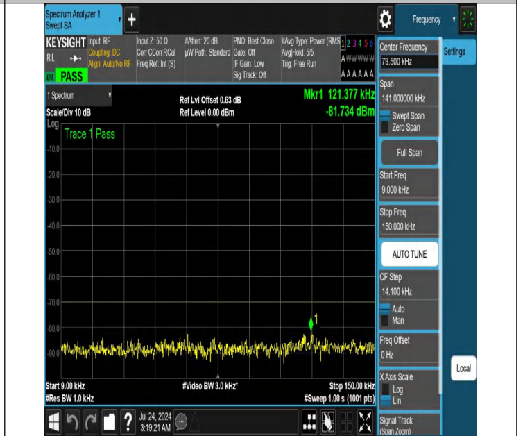
NTNV-N48-PC3-30-30-H-DFT-PI2BPSK-Edge_1RB_Right-0.009-0.15-Ant1-PASS
