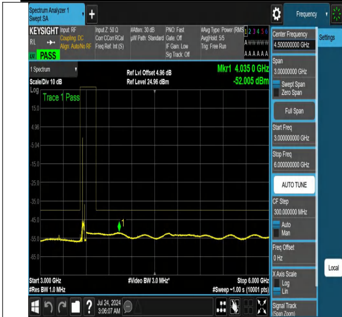
NTNV-N48-PC3-30-30-L-DFT-PI2BPSK-Edge_1RB_Left-3000-60 00-Ant1-PASS
