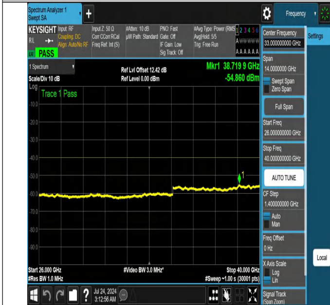
NTNV-N48-PC3-30-30-M-DFT-PI2BPSK-Edge_1RB_Left-26000-40000-Ant1-PASS
