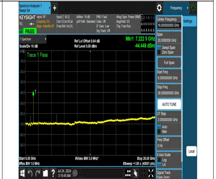
NTNV-N48-PC3-30-30-M-DFT-QPSK-Edge_1RB_Left-6000-2600-0-Ant1-PASS
