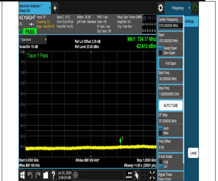
NTNV-N48-PC3-30-20-L-DFT-PI2BPSK-Edge_1RB_Right-30-100 0-Ant1-PASS
