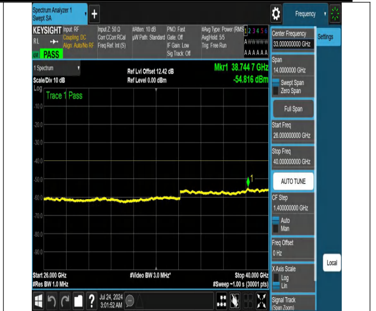
NTNV-N48-PC3-30-20-H-DFT-PI2BPSK-Edge_1RB_Right-26000-40000-Ant1-PASS
