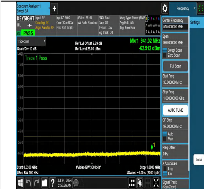
NTNV-N48-PC3-30-20-M-DFT-PI2BPSK-Edge_1RB_Left-30-1000-Ant1-PASS
