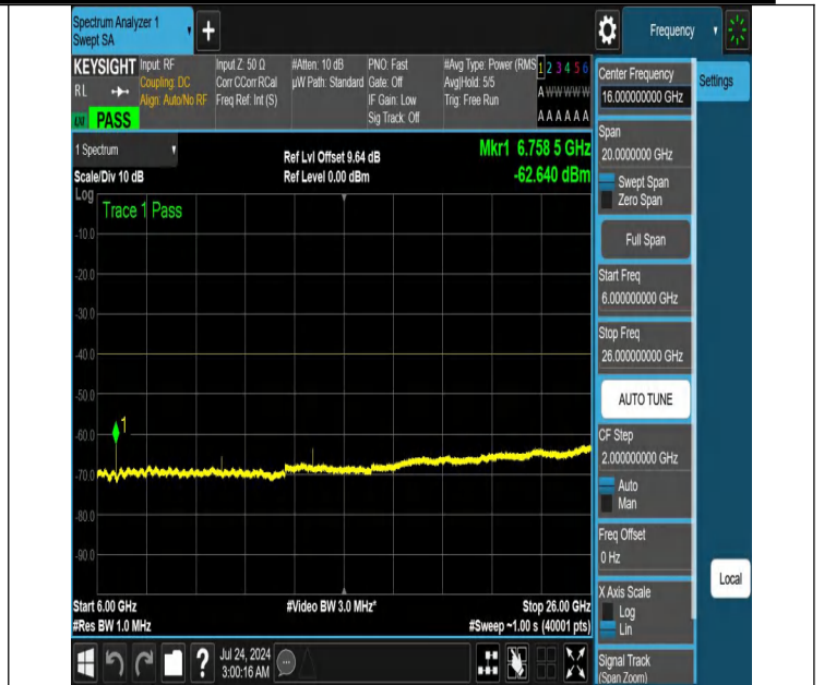
NTNV-N48-PC3-30-20-H-DFT-PI2BPSK-Edge_1RB_Left-6000-26000-Ant1-PASS
