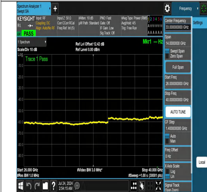
NTNV-N48-PC3-30-20-M-DFT-PI2BPSK-Edge_1RB_Left-26000-40000-Ant1-PASS
