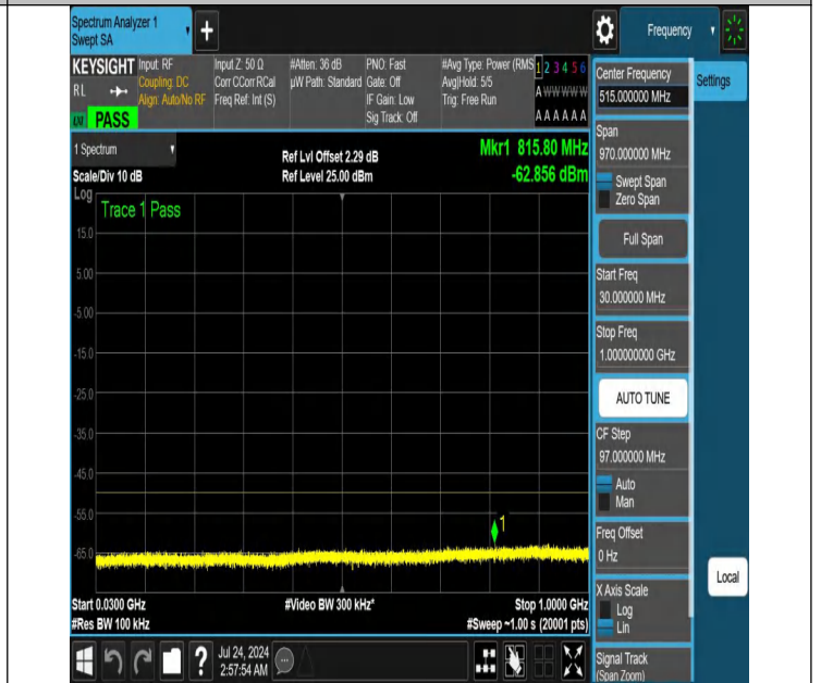
NTNV-N48-PC3-30-20-M-DFT-QPSK-Edge_1RB_Right-30-1000-Ant1-PASS
