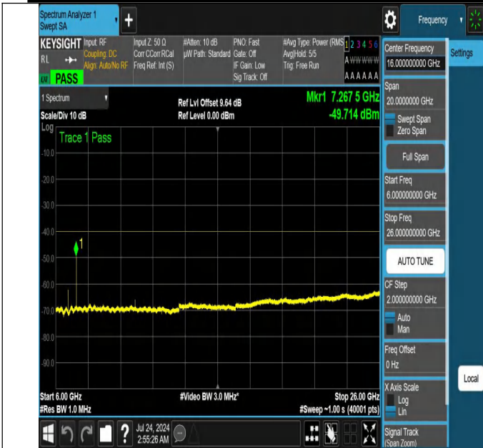
NTNV-N48-PC3-30-20-M-DFT-PI2BPSK-Edge_1RB_Right-6000-26000-Ant1-PASS
