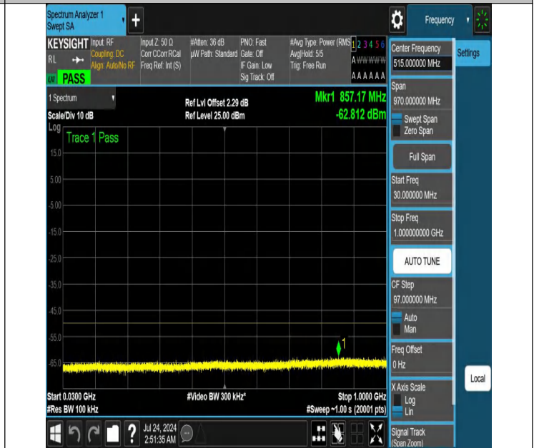
NTNV-N48-PC3-30-20-L-DFT-QPSK-Edge_1RB_Right-30.000-1000.000-Ant1-PASS
