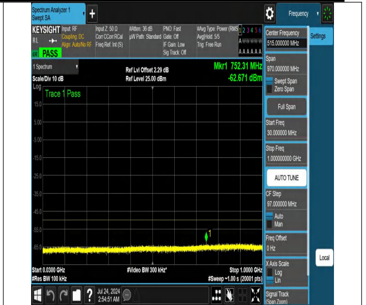
NTNV-N48-PC3-30-20-M-DFT-PI2BPSK-Edge_1RB_Right-30-100-0-Ant1-PASS
