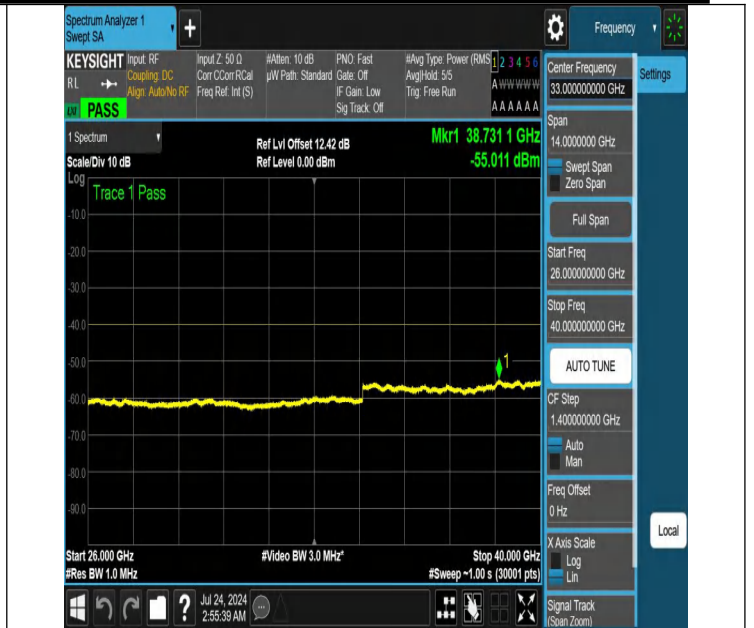
NTNV-N48-PC3-30-20-M-DFT-PI2BPSK-Edge_1RB_Right-26000-40000-Ant1-PASS
