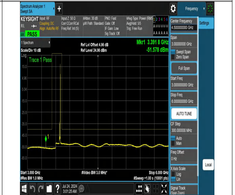
NTNV-N48-PC3-30-20-H-DFT-PI2BPSK-Edge_1RB_Right-3000-6000-Ant1-PASS
