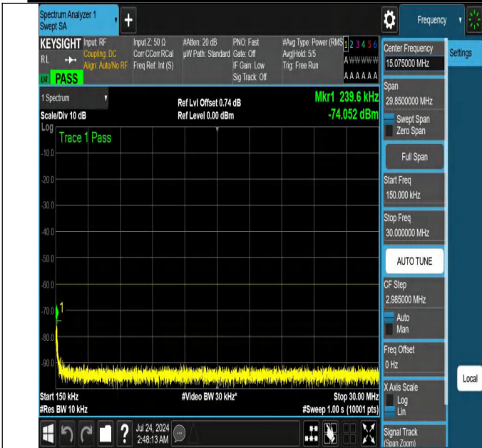
NTNV-N48-PC3-30-20-L-DFT-PI2BPSK-Edge_1RB_Right-0.15-3 0-Ant1-PASS
