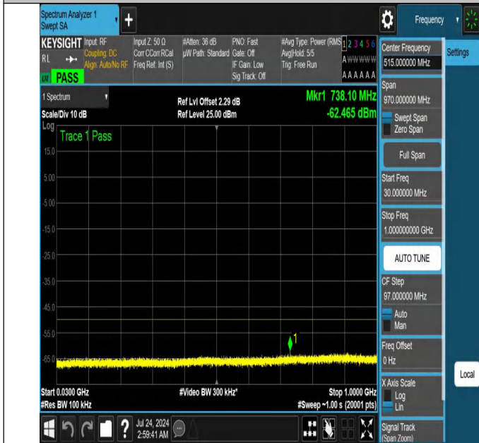
NTNV-N48-PC3-30-20-H-DFT-PI2BPSK-Edge_1RB_Left-30-1000-Ant1-PASS
