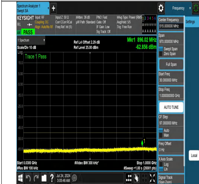
NTNV-N48-PC3-30-30-L-DFT-PI2BPSK-Edge_1RB_Left-30-1000-Ant1-PASS
