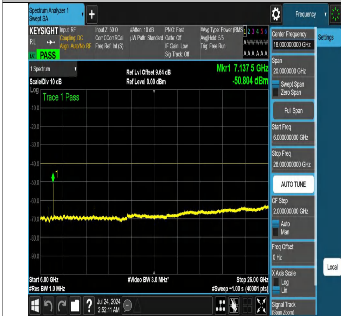
NTNV-N48-PC3-30-20-L-DFT-QPSK-Edge_1RB_Right-6000-260 00-Ant1-PASS
