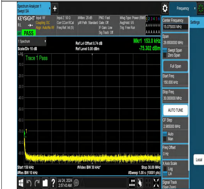
NTNV-N48-PC3-30-20-M-DFT-QPSK-Edge_1RB_Right-0.150-30.000-Ant1-PASS
