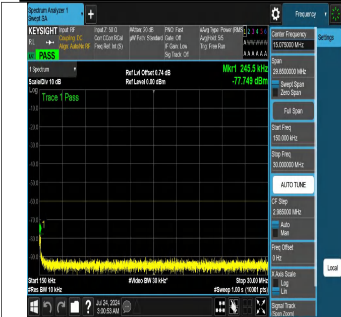
NTNV-N48-PC3-30-20-H-DFT-PI2BPSK-Edge_1RB_Right-0.15-3 0-Ant1-PASS
