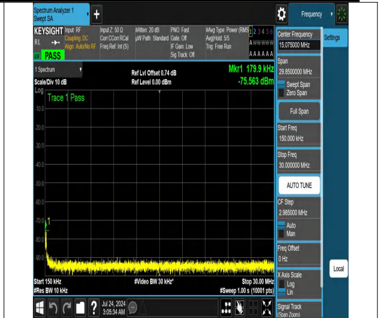
NTNV-N48-PC3-30-30-L-DFT-PI2BPSK-Edge_1RB_Left-0.15-30-Ant1-PASS
