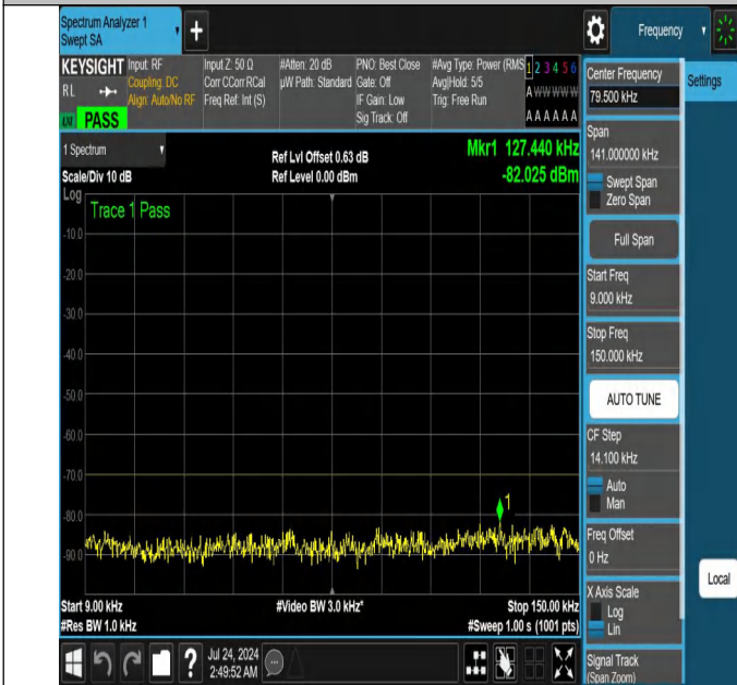
NTNV-N48-PC3-30-20-L-DFT-QPSK-Edge_1RB_Left-0.009-0.15-Ant1-PASS
