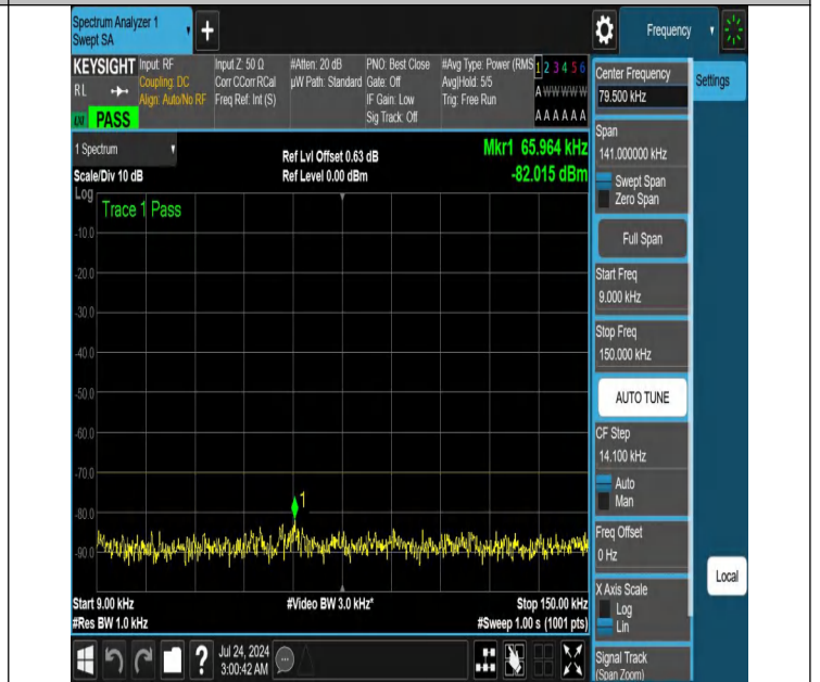
NTNV-N48-PC3-30-20-H-DFT-PI2BPSK-Edge_1RB_Right-0.009-0.15-Ant1-PASS
