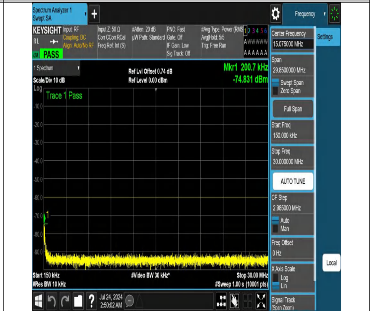
NTNV-N48-PC3-30-20-L-DFT-QPSK-Edge_1RB_Left-0.15-30-Ant1-PASS
