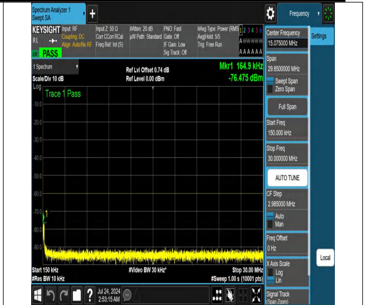
NTNV-N48-PC3-30-20-M-DFT-PI2BPSK-Edge_1RB_Left-0.15-30-Ant1-PASS
