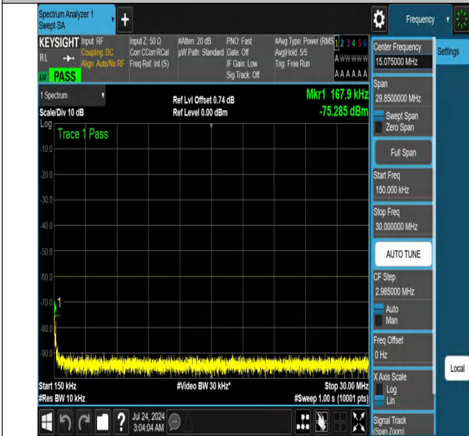
NTNV-N48-PC3-30-20-H-DFT-QPSK-Edge_1RB_Right-0.150-30.000-Ant1-PASS
