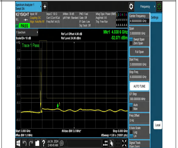
NTNV-N48-PC3-30-20-L-DFT-PI2BPSK-Edge_1RB_Right-3000-6000-Ant1-PASS
