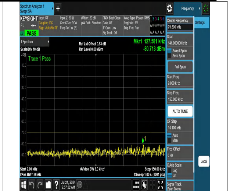
NTNV-N48-PC3-30-20-M-DFT-QPSK-Edge_1RB_Right-0.009-0.150-Ant1-PASS
