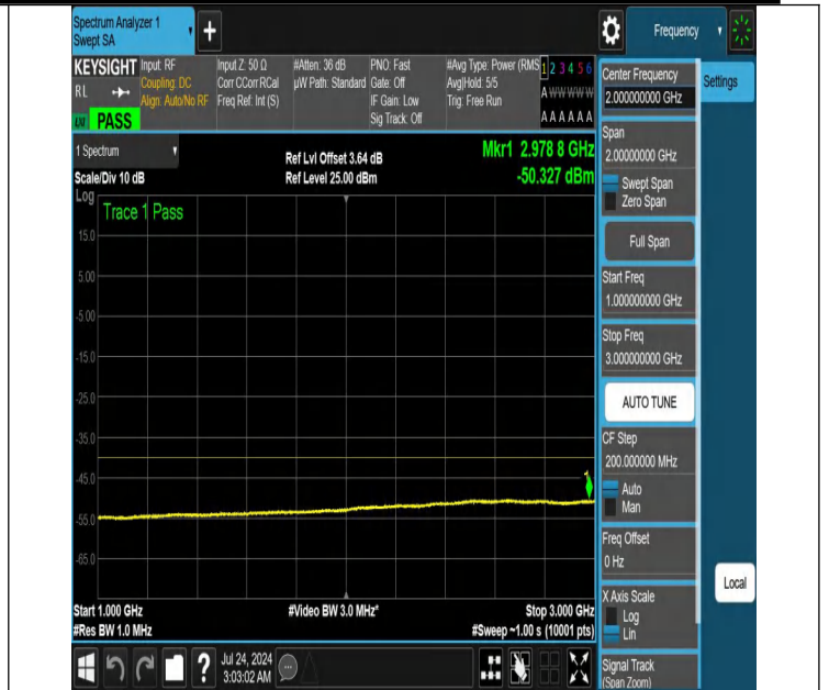
NTNV-N48-PC3-30-20-H-DFT-QPSK-Edge_1RB_Left-1000-3000-Ant1-PASS
