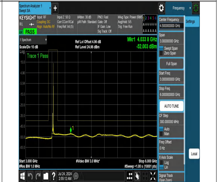
NTNV-N48-PC3-30-20-M-DFT-PI2BPSK-Edge_1RB_Right-3000-6000-Ant1-PASS
