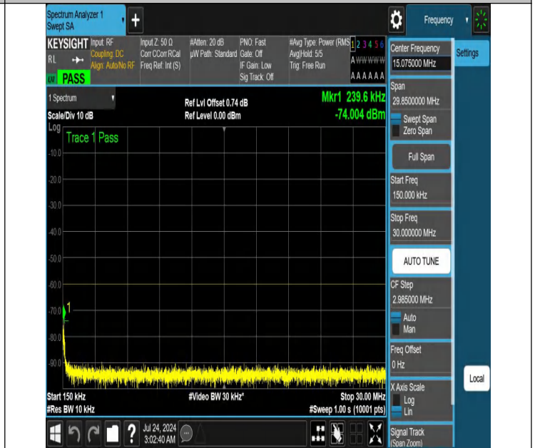
NTNV-N48-PC3-30-20-H-DFT-QPSK-Edge_1RB_Left-0.15-30-Ant1-PASS
