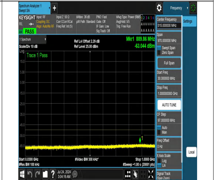
NTNV-N48-PC3-30-20-H-DFT-QPSK-Edge_1RB_Right-30-1000-Ant1-PASS
