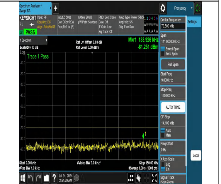
NTNV-N48-PC3-30-20-M-DFT-PI2BPSK-Edge_1RB_Right-0.009-0.15-Ant1-PASS
