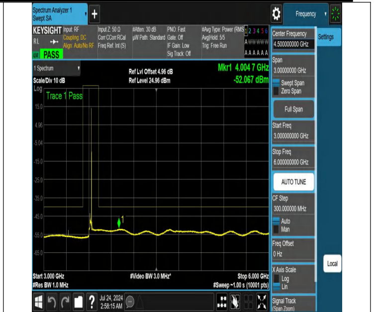
NTNV-N48-PC3-30-20-M-DFT-QPSK-Edge_1RB_Right-3000-600 0-Ant1-PASS
