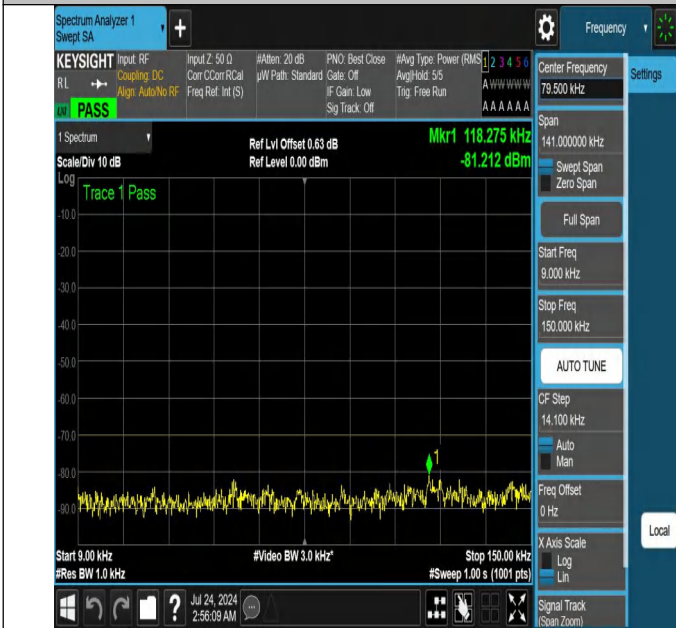
NTNV-N48-PC3-30-20-M-DFT-QPSK-Edge_1RB_Left-0.009-0.15-Ant1-PASS
