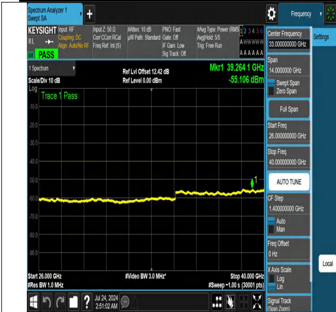
NTNV-N48-PC3-30-20-L-DFT-QPSK-Edge_1RB_Left-26000-40000-Ant1-PASS
