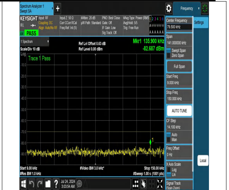
NTNV-N48-PC3-30-20-H-DFT-QPSK-Edge_1RB_Right-0.009-0.150-Ant1-PASS
