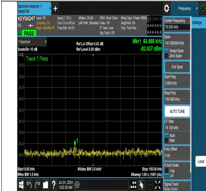
NTNV-N48-PC3-30-20-H-DFT-QPSK-Edge_1RB_Left-0.009-0.15-Ant1-PASS
