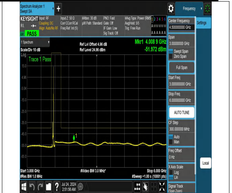
NTNV-N48-PC3-30-20-L-DFT-QPSK-Edge_1RB_Right-3000-6000 -Ant1-PASS
