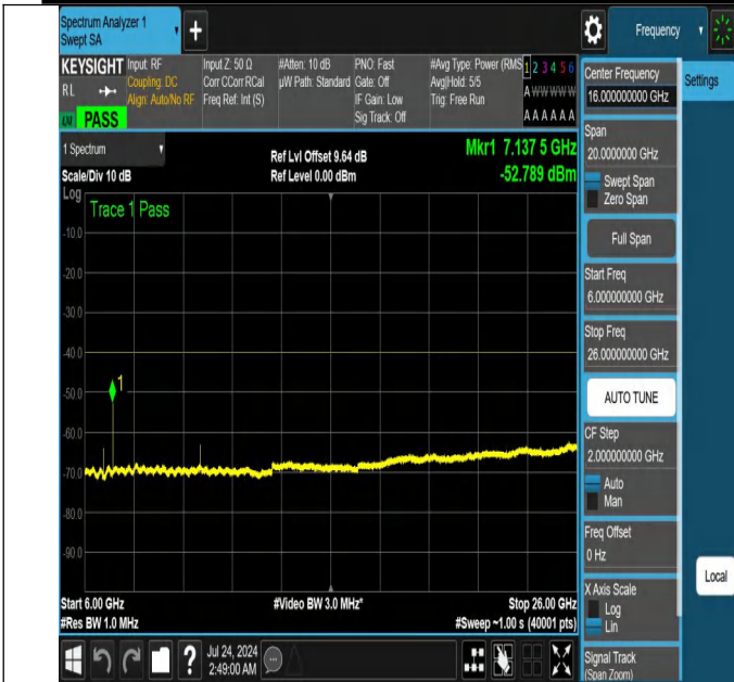
NTNV-N48-PC3-30-20-L-DFT-PI2BPSK-Edge_1RB_Right-6000-26000-Ant1-PASS
