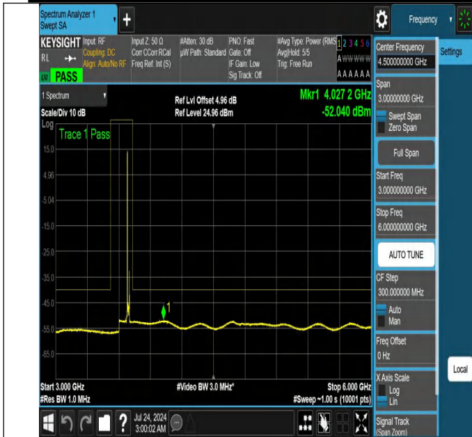
NTNV-N48-PC3-30-20-H-DFT-PI2BPSK-Edge_1RB_Left-3000-6000-Ant1-PASS
