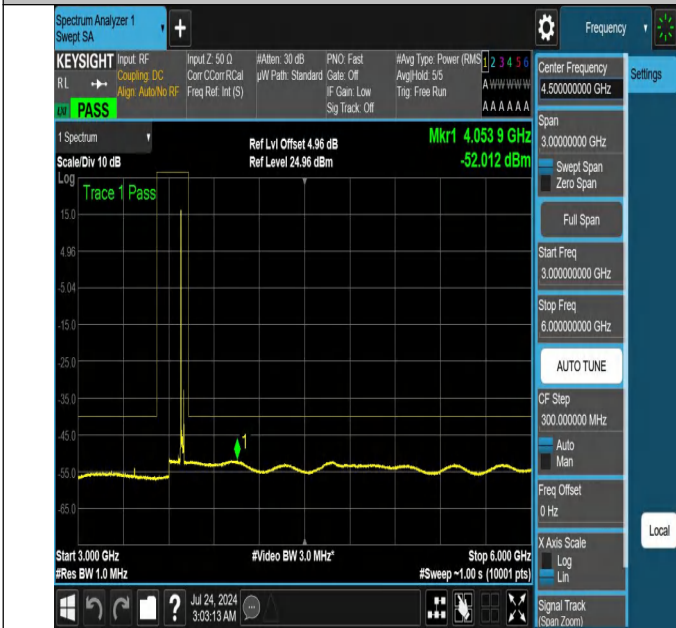
NTNV-N48-PC3-30-20-H-DFT-QPSK-Edge_1RB_Left-3000-6000-Ant1-PASS
