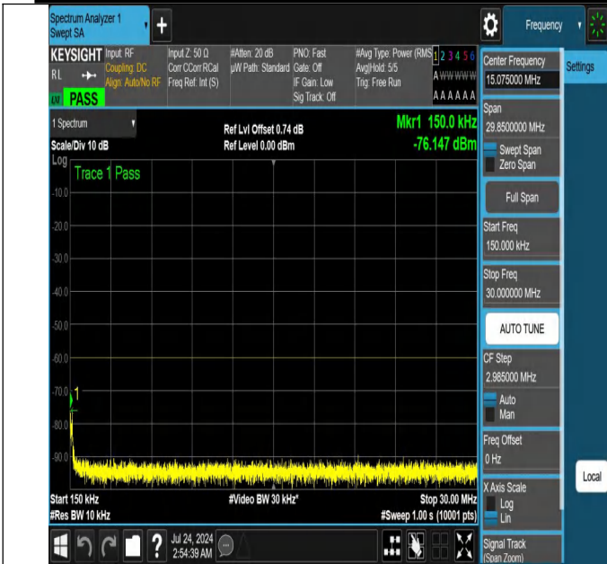
NTNV-N48-PC3-30-20-M-DFT-PI2BPSK-Edge_1RB_Right-0.15-30-Ant1-PASS
