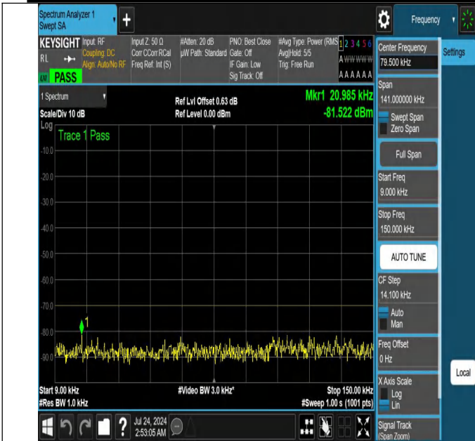
NTNV-N48-PC3-30-20-M-DFT-PI2BPSK-Edge_1RB_Left-0.009-0.15-Ant1-PASS
