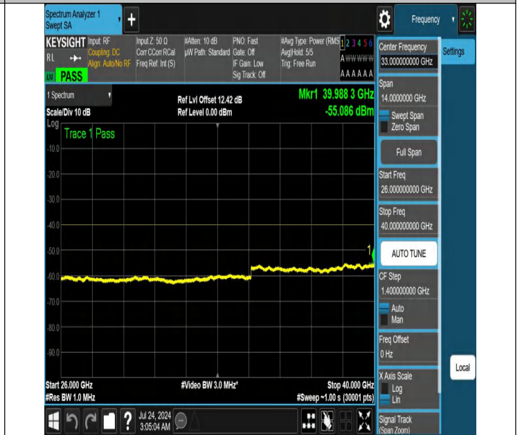
NTNV-N48-PC3-30-20-H-DFT-QPSK-Edge_1RB_Right-26000-40 000-Ant1-PASS
