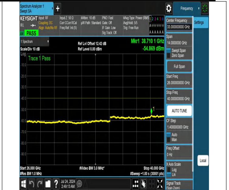
NTNV-N48-PC3-30-20-L-DFT-PI2BPSK-Edge_1RB_Right-26000-40000-Ant1-PASS
