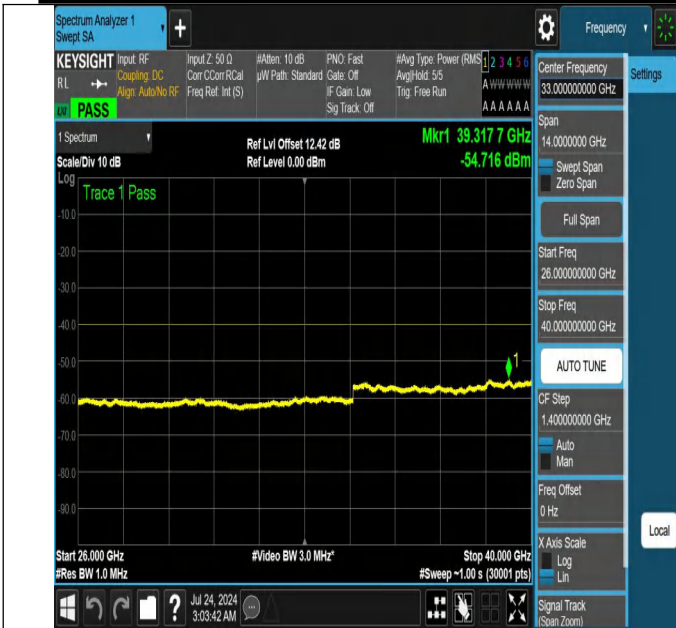
NTNV-N48-PC3-30-20-H-DFT-QPSK-Edge_1RB_Left-26000-40000-Ant1-PASS
