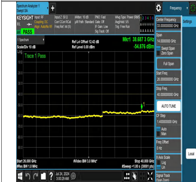
NTNV-N48-PC3-30-20-H-DFT-PI2BPSK-Edge_1RB_Left-26000-40000-Ant1-PASS
