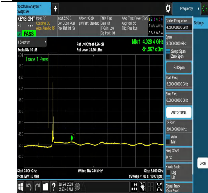
NTNV-N48-PC3-30-20-M-DFT-PI2BPSK-Edge_1RB_Left-3000-6000-Ant1-PASS
