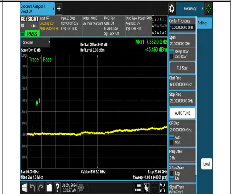
NTNV-N48-PC3-30-20-H-DFT-QPSK-Edge_1RB_Left-6000-26000-Ant1-PASS
