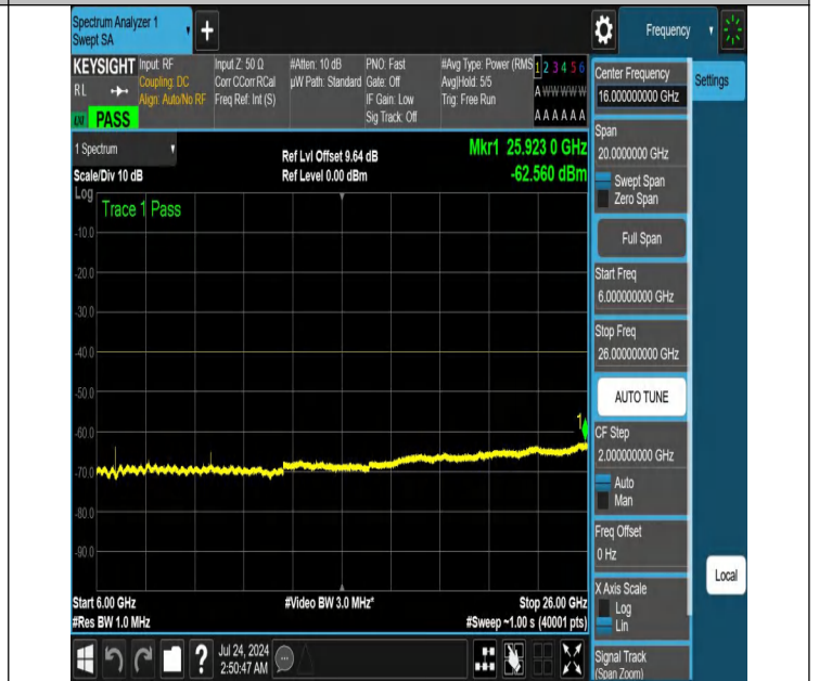
NTNV-N48-PC3-30-20-L-DFT-QPSK-Edge_1RB_Left-6000-26000-Ant1-PASS
