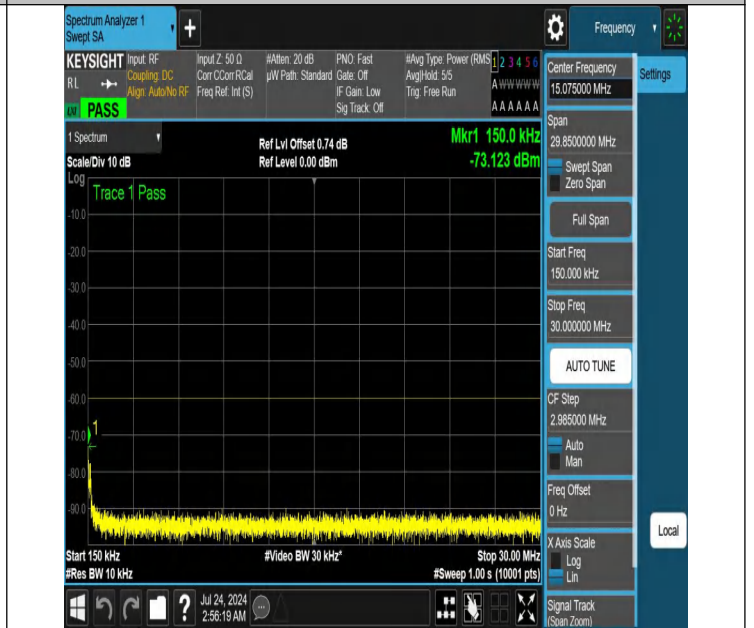
NTNV-N48-PC3-30-20-M-DFT-QPSK-Edge_1RB_Left-0.15-30-Ant1-PASS
