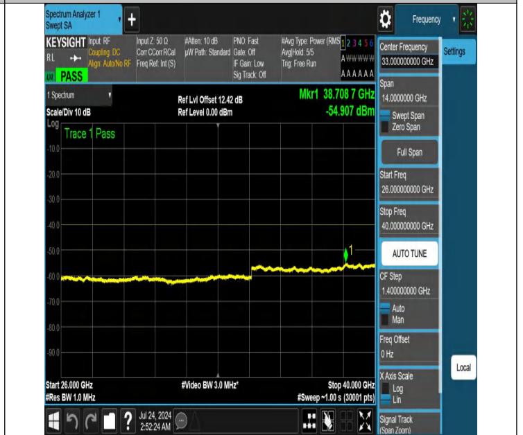
NTNV-N48-PC3-30-20-L-DFT-QPSK-Edge_1RB_Right-26000-400 00-Ant1-PASS
