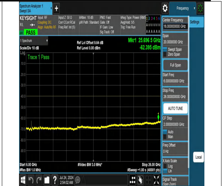
NTNV-N48-PC3-30-20-M-DFT-PI2BPSK-Edge_1RB_Left-6000-26000-Ant1-PASS
