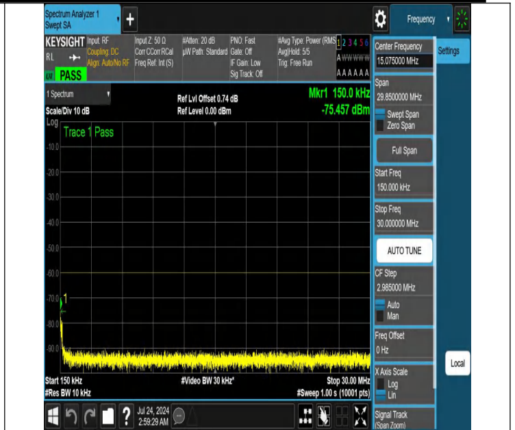
NTNV-N48-PC3-30-20-H-DFT-PI2BPSK-Edge_1RB_Left-0.15-30-Ant1-PASS
