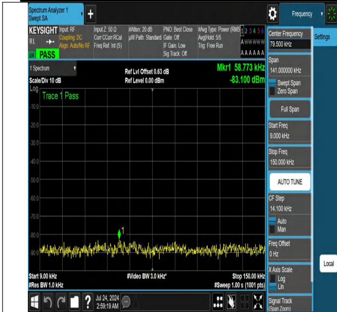
NTNV-N48-PC3-30-20-H-DFT-PI2BPSK-Edge_1RB_Left-0.009-0.15-Ant1-PASS
