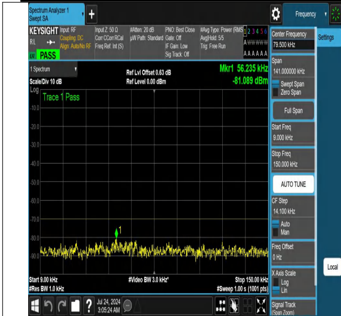
NTNV-N48-PC3-30-30-L-DFT-PI2BPSK-Edge_1RB_Left-0.009-0.15-Ant1-PASS
