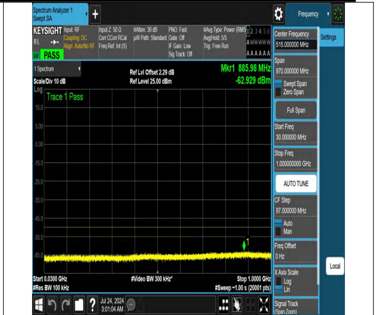
NTNV-N48-PC3-30-20-H-DFT-PI2BPSK-Edge_1RB_Right-30-100 0-Ant1-PASS
