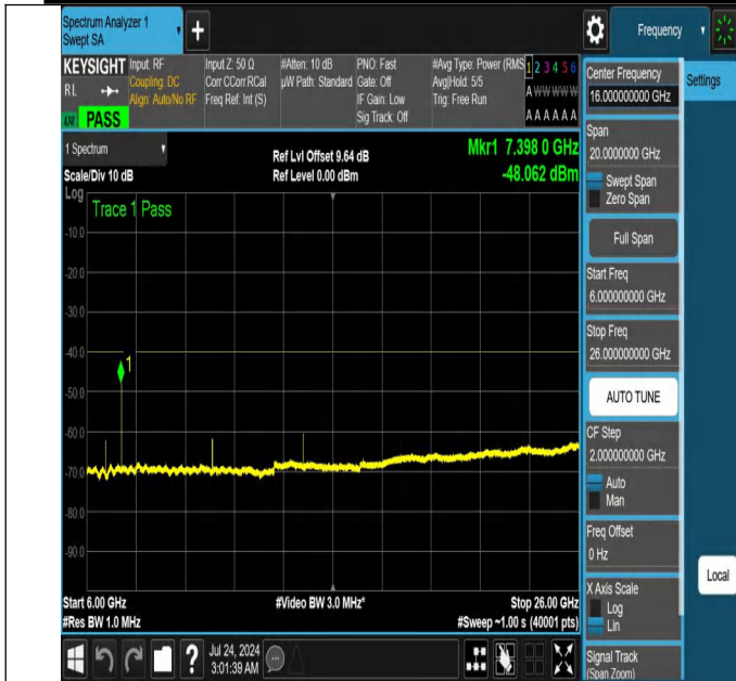
NTNV-N48-PC3-30-20-H-DFT-PI2BPSK-Edge_1RB_Right-6000-26000-Ant1-PASS
