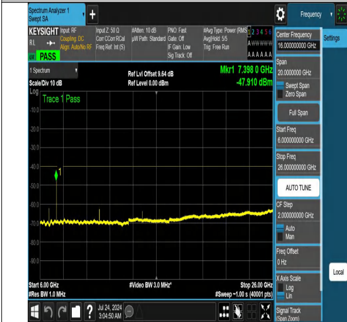
NTNV-N48-PC3-30-20-H-DFT-QPSK-Edge_1RB_Right-6000-260 00-Ant1-PASS
