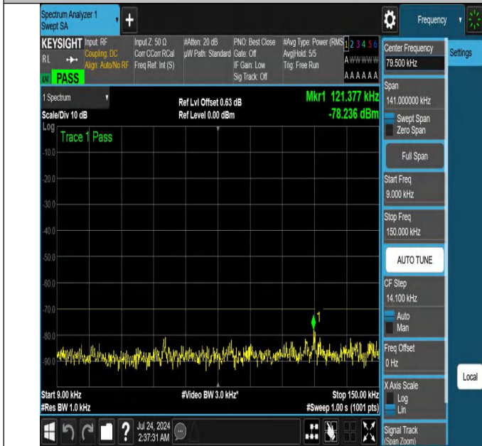
NTNV-N48-PC3-30-15-M-DFT-QPSK-Edge_1RB_Left-0.009-0.15-Ant1-PASS
