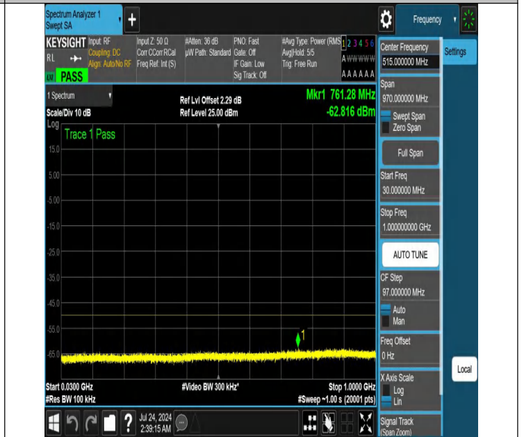
NTNV-N48-PC3-30-15-M-DFT-QPSK-Edge_1RB_Right-30-1000-Ant1-PASS
