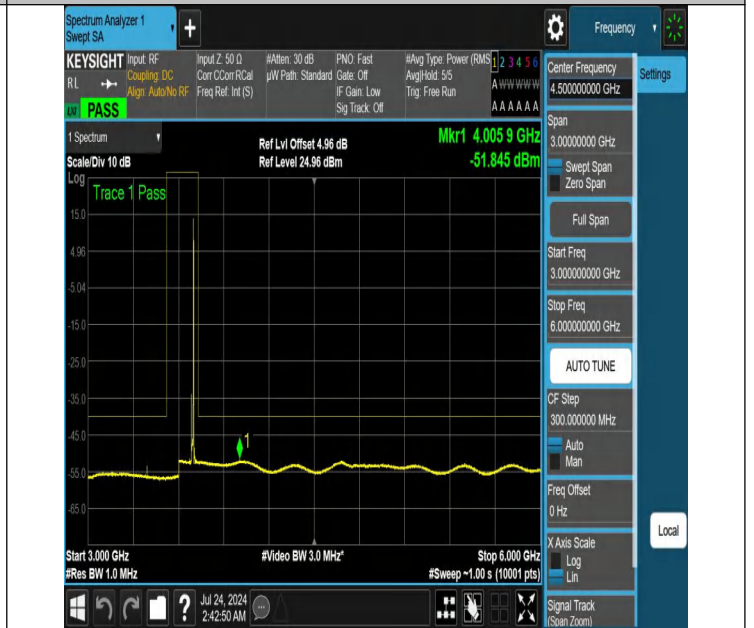
NTNV-N48-PC3-30-15-H-DFT-PI2BPSK-Edge_1RB_Right-3000-6000-Ant1-PASS
