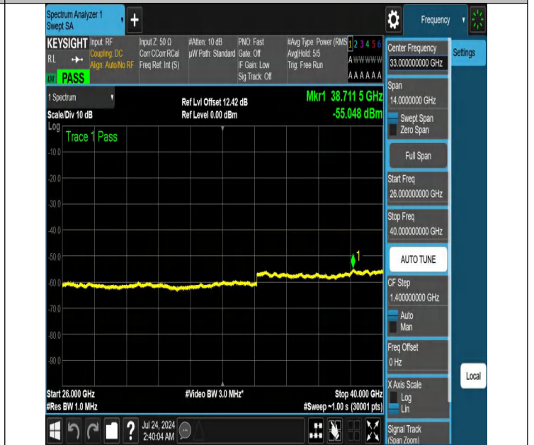
NTNV-N48-PC3-30-15-M-DFT-QPSK-Edge_1RB_Right-26000-40 000-Ant1-PASS
