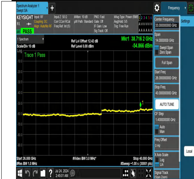
NTNV-N48-PC3-30-15-H-DFT-QPSK-Edge_1RB_Left-26000-40000-Ant1-PASS
