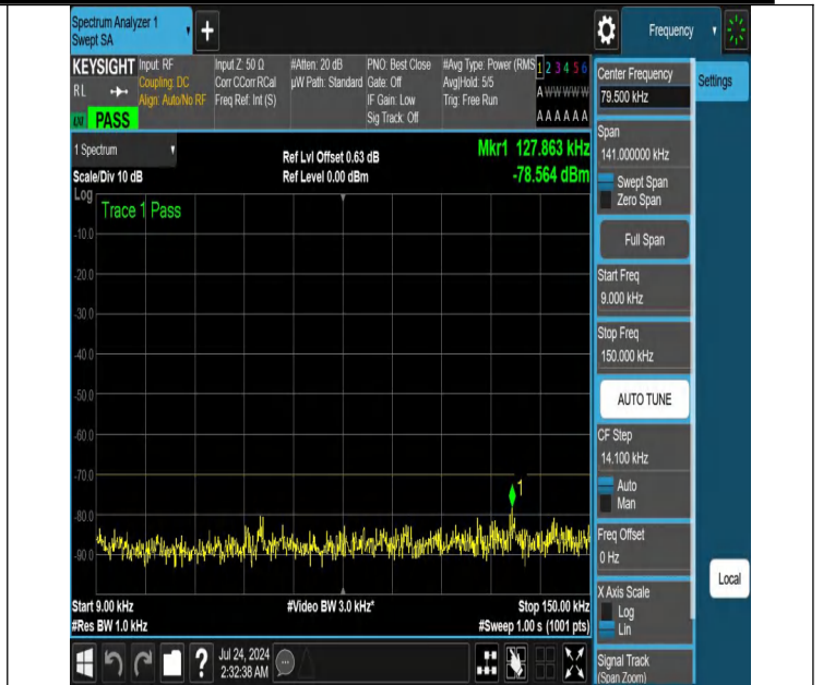
NTNV-N48-PC3-30-15-L-DFT-QPSK-Edge_1RB_Right-0.009-0.150-Ant1-PASS
