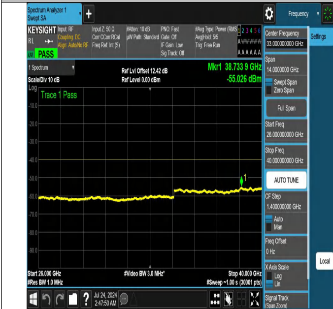
NTNV-N48-PC3-30-20-L-DFT-PI2BPSK-Edge_1RB_Left-26000-4 0000-Ant1-PASS
