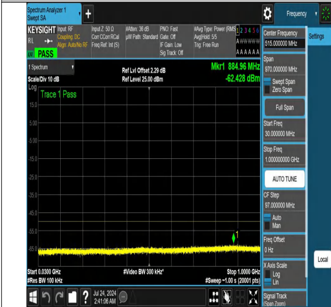
NTNV-N48-PC3-30-15-H-DFT-PI2BPSK-Edge_1RB_Left-30-1000-Ant1-PASS
