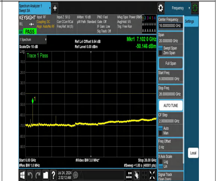
NTNV-N48-PC3-30-15-L-DFT-QPSK-Edge_1RB_Left-6000-26000-Ant1-PASS
