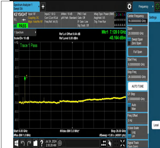
NTNV-N48-PC3-30-15-L-DFT-PI2BPSK-Edge_1RB_Right-6000-26000-Ant1-PASS
