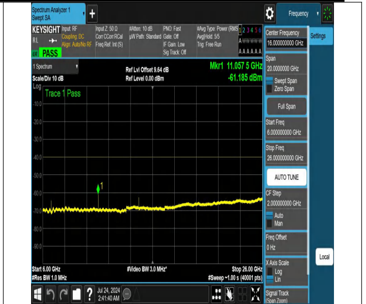
NTNV-N48-PC3-30-15-H-DFT-PI2BPSK-Edge_1RB_Left-6000-26000-Ant1-PASS
