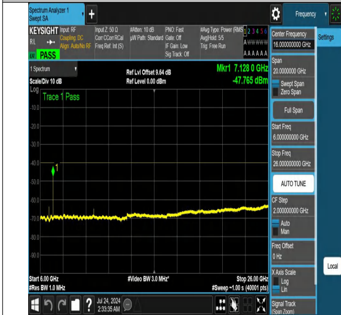
NTNV-N48-PC3-30-15-L-DFT-QPSK-Edge_1RB_Right-6000-260 00-Ant1-PASS
