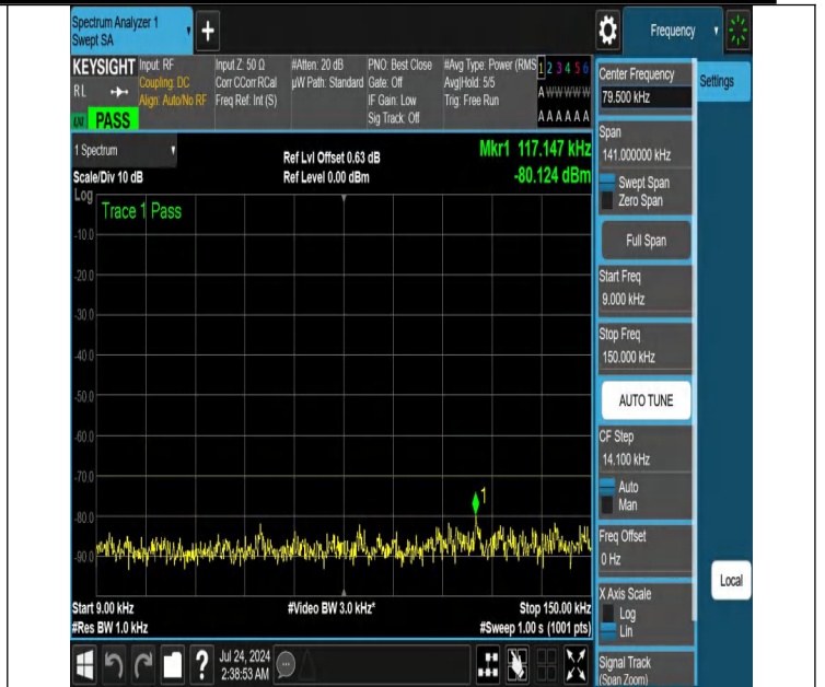
NTNV-N48-PC3-30-15-M-DFT-QPSK-Edge_1RB_Right-0.009-0.150-Ant1-PASS
