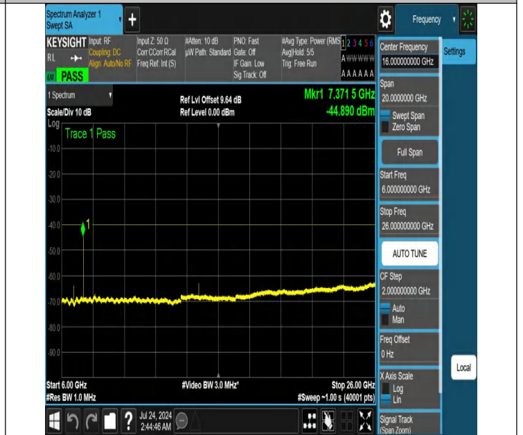
NTNV-N48-PC3-30-15-H-DFT-QPSK-Edge_1RB_Left-6000-26000 -Ant1-PASS
