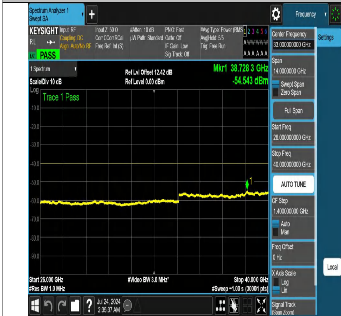
NTNV-N48-PC3-30-15-M-DFT-PI2BPSK-Edge_1RB_Left-26000-40000-Ant1-PASS
