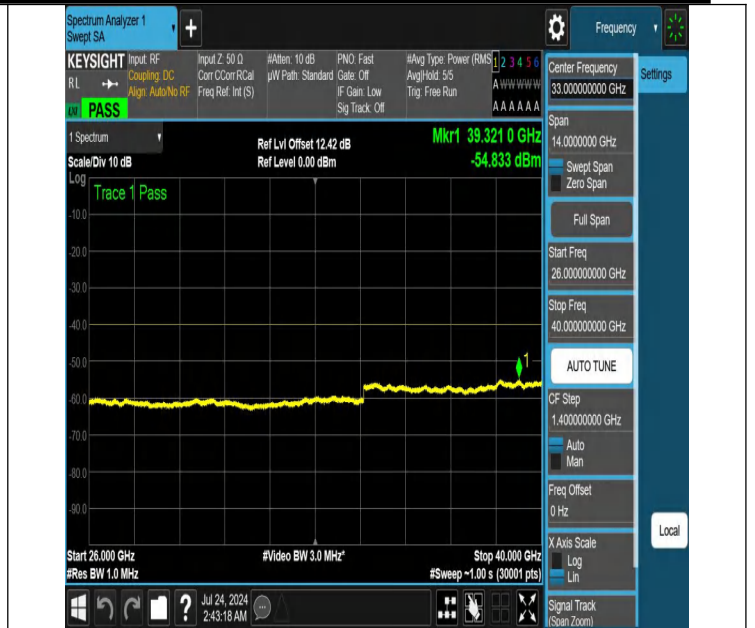
NTNV-N48-PC3-30-15-H-DFT-PI2BPSK-Edge_1RB_Right-26000-40000-Ant1-PASS
