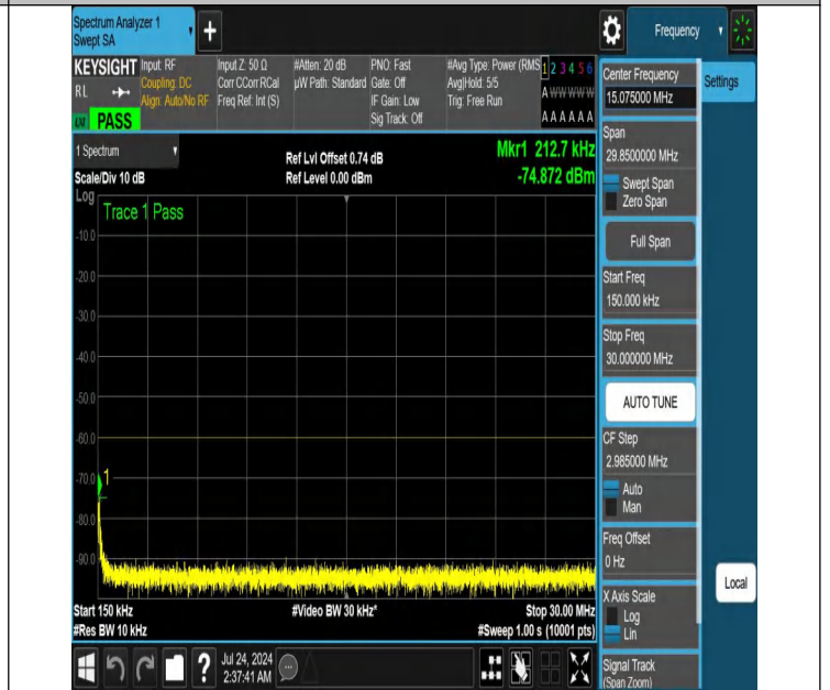
NTNV-N48-PC3-30-15-M-DFT-QPSK-Edge_1RB_Left-0.15-30-Ant1-PASS
