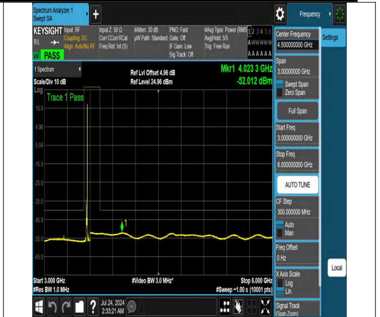
NTNV-N48-PC3-30-15-L-DFT-QPSK-Edge_1RB_Right-3000-6000 -Ant1-PASS
