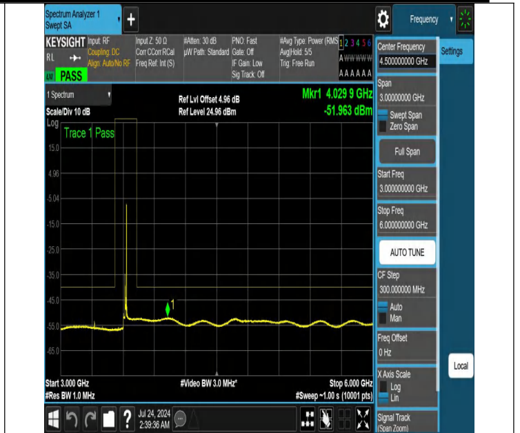
NTNV-N48-PC3-30-15-M-DFT-QPSK-Edge_1RB_Right-3000-600 0-Ant1-PASS
