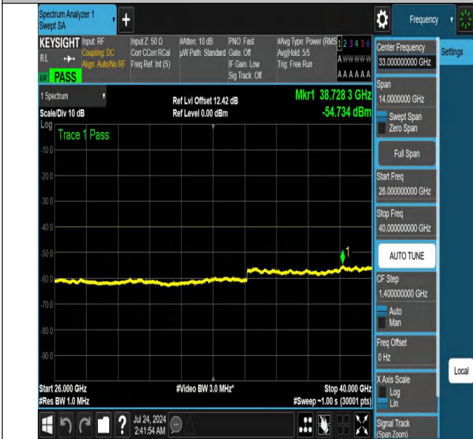
NTNV-N48-PC3-30-15-H-DFT-PI2BPSK-Edge_1RB_Left-26000-40000-Ant1-PASS
