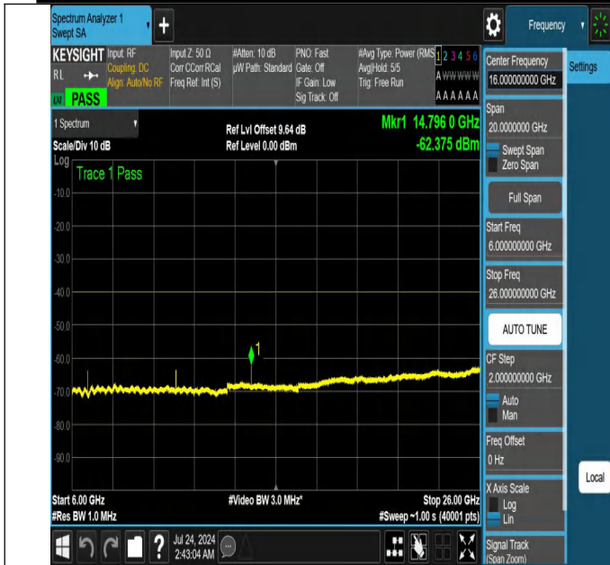
NTNV-N48-PC3-30-15-H-DFT-PI2BPSK-Edge_1RB_Right-6000-26000-Ant1-PASS
