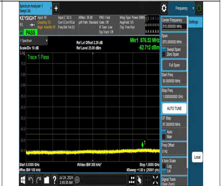
NTNV-N48-PC3-30-15-H-DFT-QPSK-Edge_1RB_Right-30-1000-Ant1-PASS
