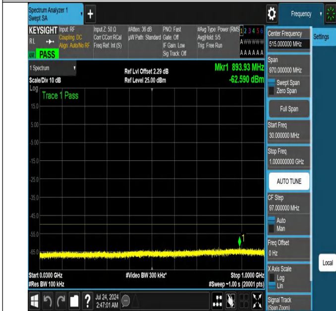
NTNV-N48-PC3-30-20-L-DFT-PI2BPSK-Edge_1RB_Left-30-1000-Ant1-PASS
