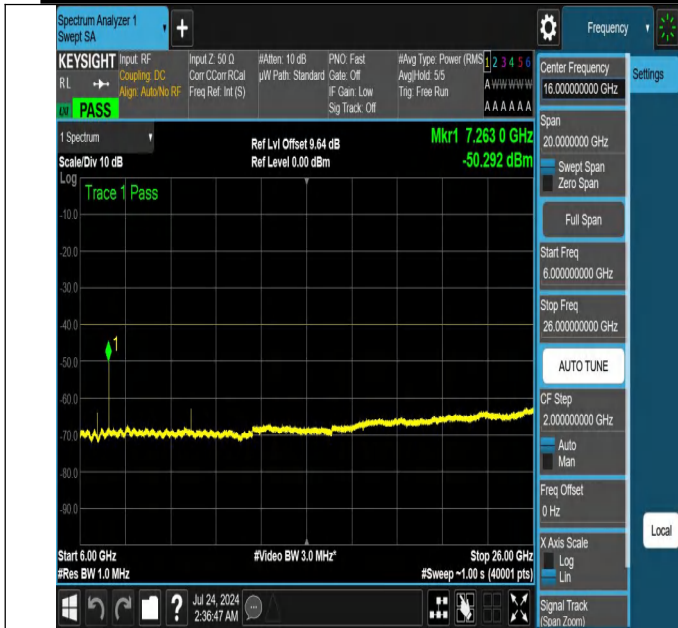
NTNV-N48-PC3-30-15-M-DFT-PI2BPSK-Edge_1RB_Right-6000-26000-Ant1-PASS
