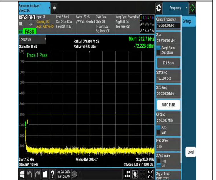
NTNV-N48-PC3-30-15-L-DFT-QPSK-Edge_1RB_Left-0.15-30-Ant1-PASS
