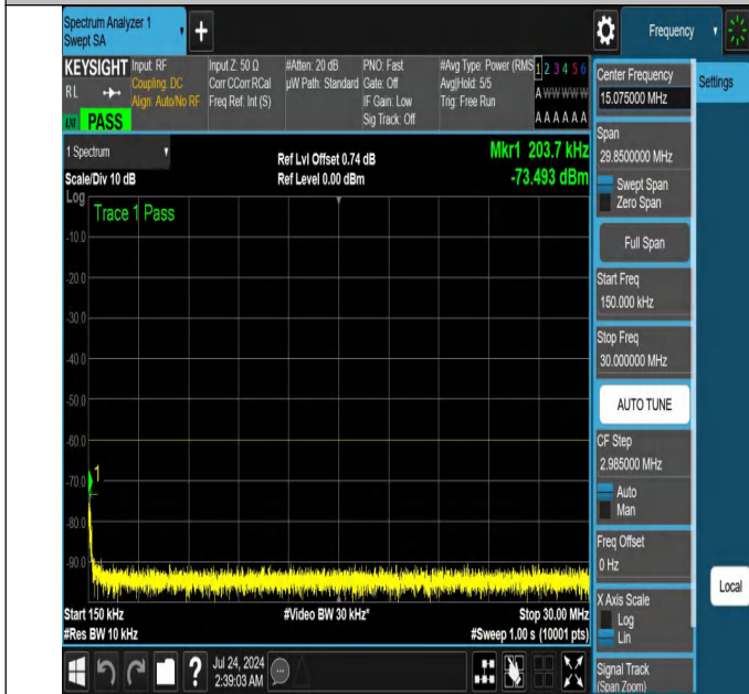
NTNV-N48-PC3-30-15-M-DFT-QPSK-Edge_1RB_Right-0.150-30.000-Ant1-PASS
