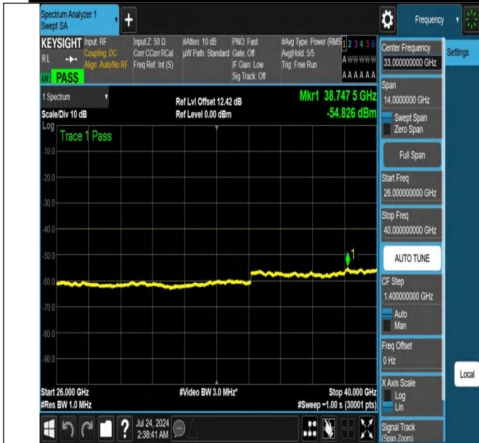
NTNV-N48-PC3-30-15-M-DFT-QPSK-Edge_1RB_Left-26000-40000-Ant1-PASS
