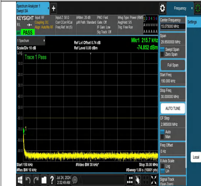
NTNV-N48-PC3-30-15-L-DFT-QPSK-Edge_1RB_Right-0.15-30-Ant1-PASS
