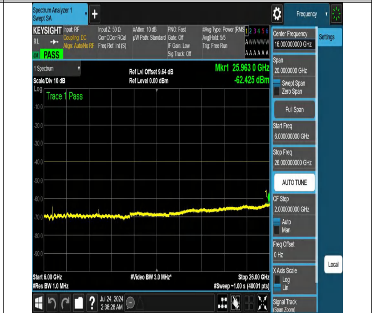
NTNV-N48-PC3-30-15-M-DFT-QPSK-Edge_1RB_Left-6000-2600-0-Ant1-PASS
