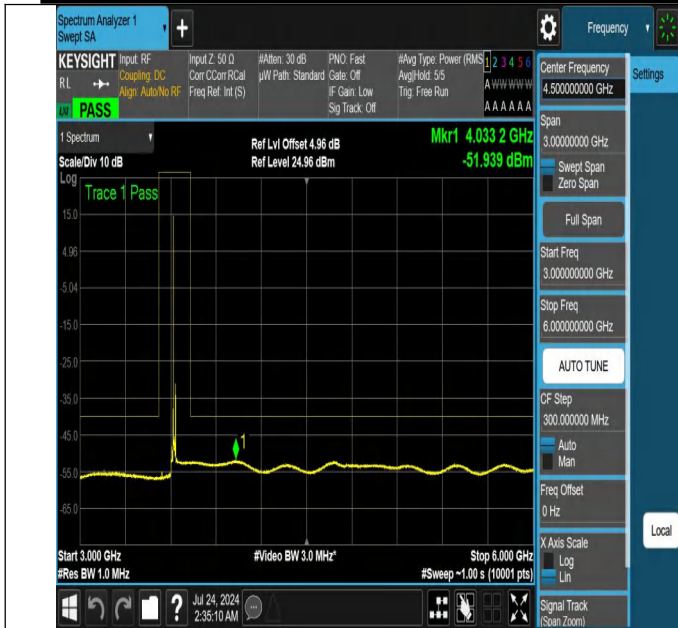
NTNV-N48-PC3-30-15-M-DFT-PI2BPSK-Edge_1RB_Left-3000-6000-Ant1-PASS
