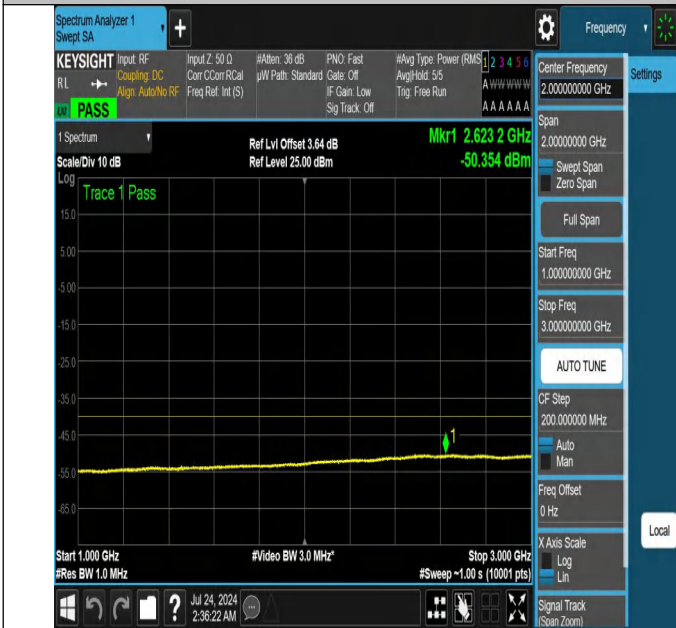
NTNV-N48-PC3-30-15-M-DFT-PI2BPSK-Edge_1RB_Right-1000-3000-Ant1-PASS
