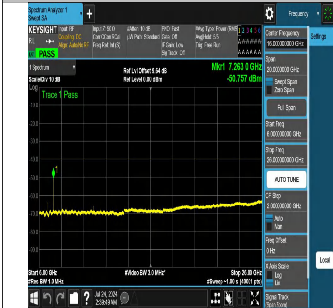
NTNV-N48-PC3-30-15-M-DFT-QPSK-Edge_1RB_Right-6000-26 000-Ant1-PASS
