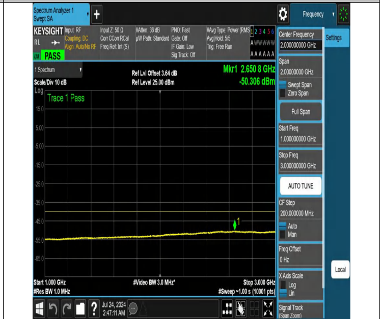
NTNV-N48-PC3-30-20-L-DFT-PI2BPSK-Edge_1RB_Left-1000-3000-Ant1-PASS
