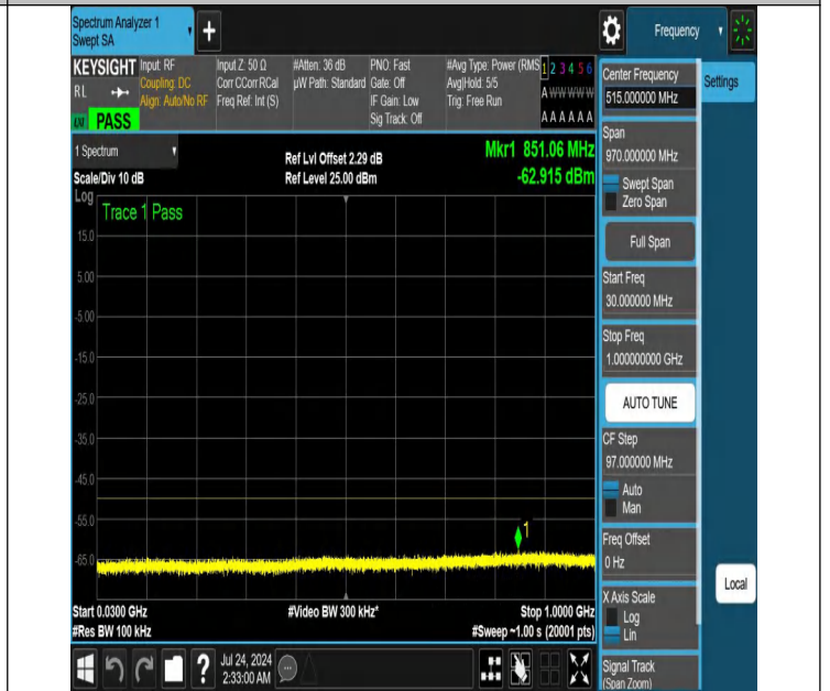
NTNV-N48-PC3-30-15-L-DFT-QPSK-Edge_1RB_Right-30-1000-Ant1-PASS
