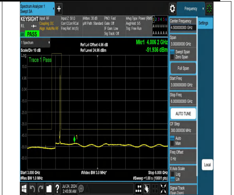
NTNV-N48-PC3-30-15-H-DFT-QPSK-Edge_1RB_Right-3000-600 0-Ant1-PASS
