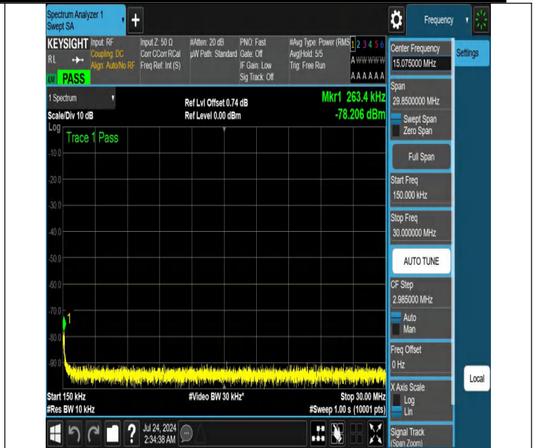
NTNV-N48-PC3-30-15-M-DFT-PI2BPSK-Edge_1RB_Left-0.15-30-Ant1-PASS
