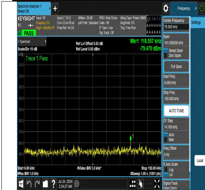
NTNV-N48-PC3-30-15-M-DFT-PI2BPSK-Edge_1RB_Left-0.009-0.15-Ant1-PASS
