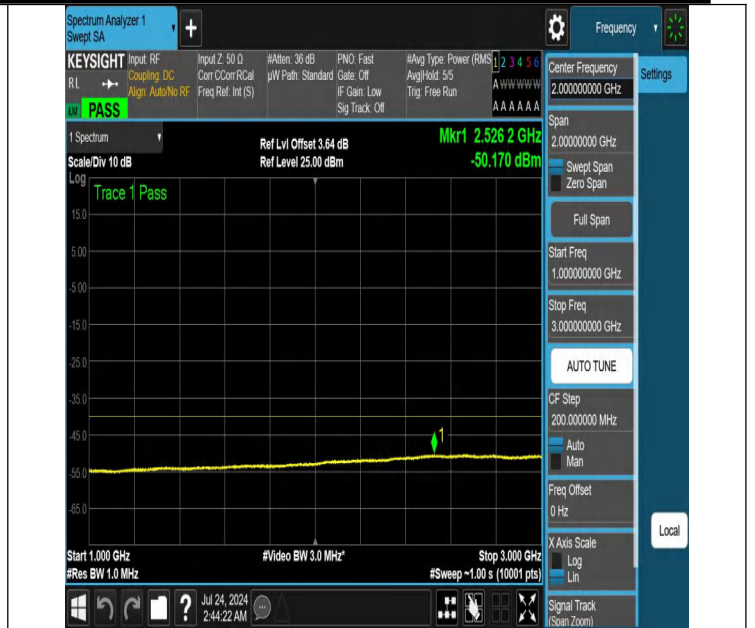
NTNV-N48-PC3-30-15-H-DFT-QPSK-Edge_1RB_Left-1000-3000-Ant1-PASS
