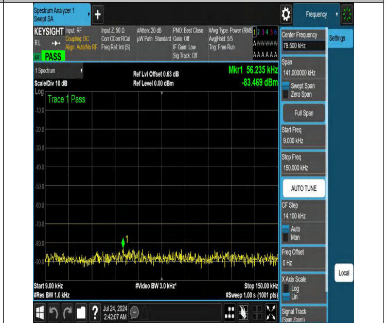
NTNV-N48-PC3-30-15-H-DFT-PI2BPSK-Edge_1RB_Right-0.009-0.15-Ant1-PASS
