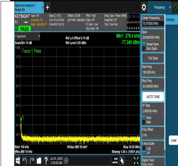
NTNV-N48-PC3-30-15-M-DFT-PI2BPSK-Edge_1RB_Right-0.15-30-Ant1-PASS
