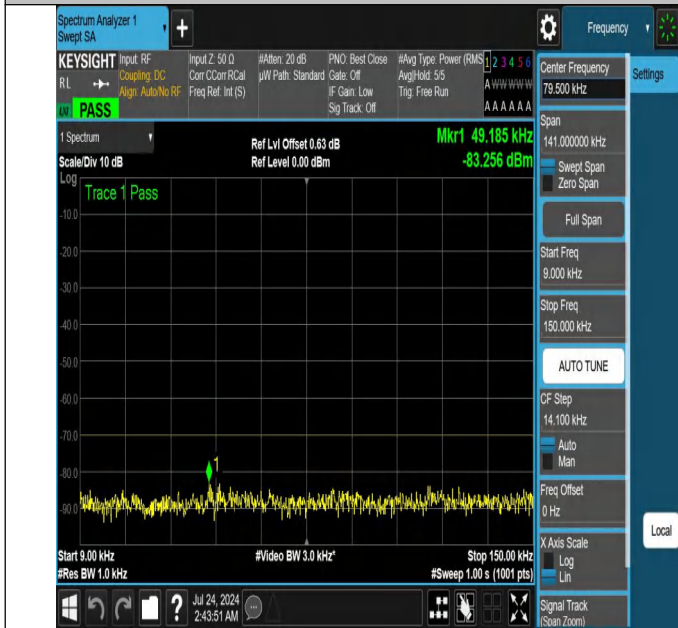
NTNV-N48-PC3-30-15-H-DFT-QPSK-Edge_1RB_Left-0.009-0.15-Ant1-PASS
