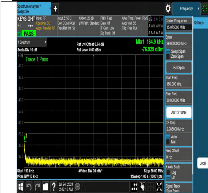
NTNV-N48-PC3-30-15-H-DFT-PI2BPSK-Edge_1RB_Right-0.15-3 0-Ant1-PASS
