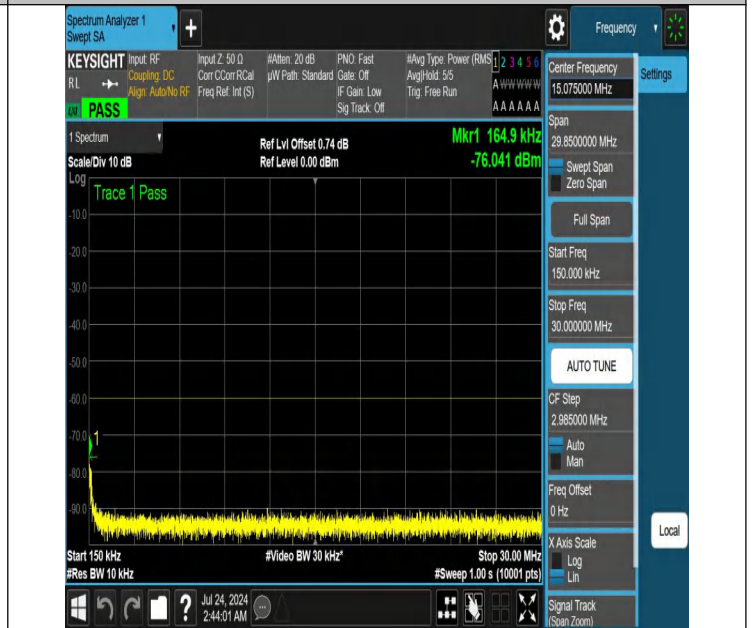
NTNV-N48-PC3-30-15-H-DFT-QPSK-Edge_1RB_Left-0.15-30-Ant1-PASS
