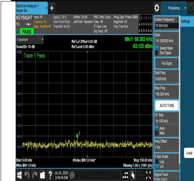
NTNV-N48-PC3-30-15-H-DFT-PI2BPSK-Edge_1RB_Left-0.009-0.15-Ant1-PASS
