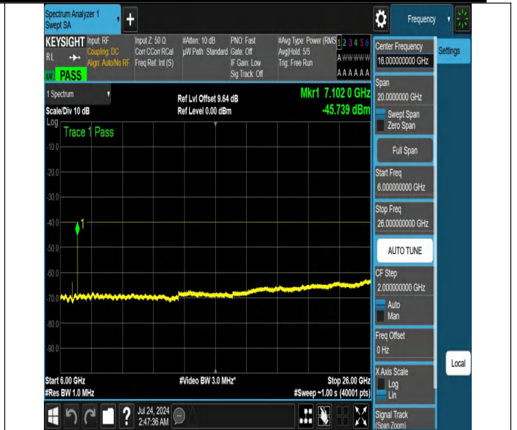
NTNV-N48-PC3-30-20-L-DFT-PI2BPSK-Edge_1RB_Left-6000-26 000-Ant1-PASS
