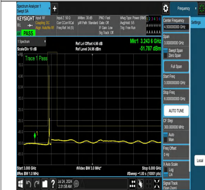
NTNV-N48-PC3-30-15-L-DFT-QPSK-Edge_1RB_Left-3000-6000-Ant1-PASS
