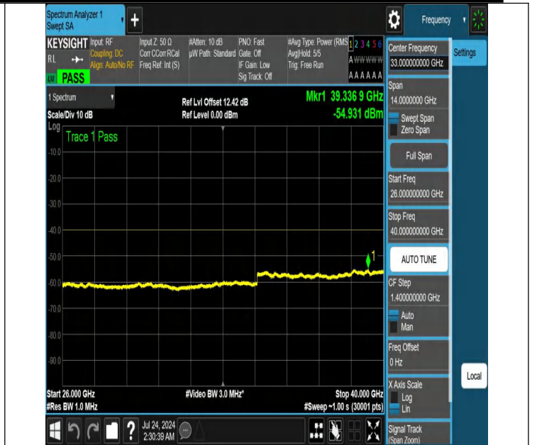
NTNV-N48-PC3-30-15-L-DFT-PI2BPSK-Edge_1RB_Right-26000-40000-Ant1-PASS
