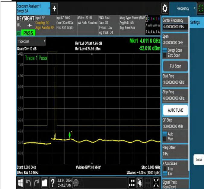
NTNV-N48-PC3-30-15-H-DFT-PI2BPSK-Edge_1RB_Left-3000-6000-Ant1-PASS
