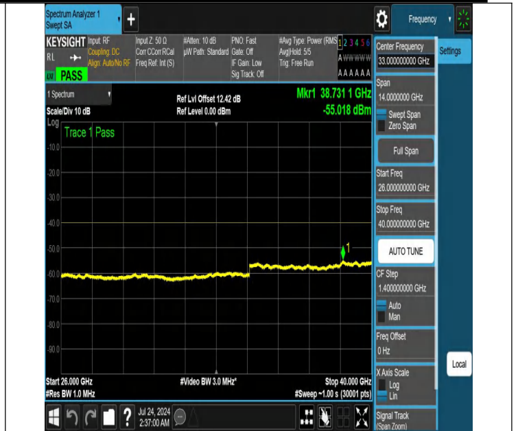
NTNV-N48-PC3-30-15-M-DFT-PI2BPSK-Edge_1RB_Right-26000-40000-Ant1-PASS
