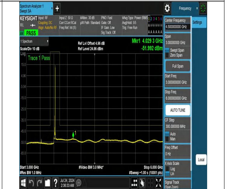
NTNV-N48-PC3-30-15-M-DFT-PI2BPSK-Edge_1RB_Right-3000-6000-Ant1-PASS
