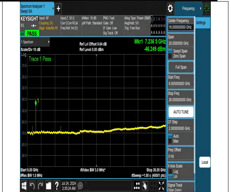
NTNV-N48-PC3-30-15-M-DFT-PI2BPSK-Edge_1RB_Left-6000-26000-Ant1-PASS
