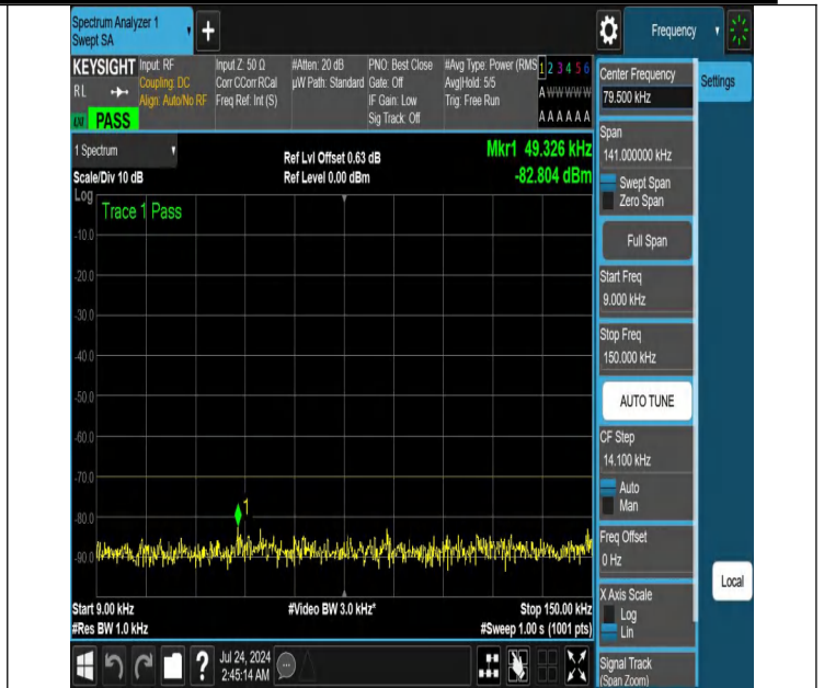
NTNV-N48-PC3-30-15-H-DFT-QPSK-Edge_1RB_Right-0.009-0.150-Ant1-PASS
