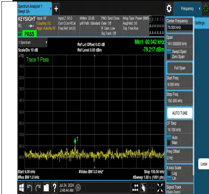
NTNV-N48-PC3-30-20-L-DFT-PI2BPSK-Edge_1RB_Left-0.009-0.15-Ant1-PASS
