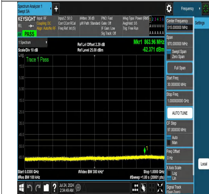
NTNV-N48-PC3-30-15-M-DFT-PI2BPSK-Edge_1RB_Left-30-1000-Ant1-PASS
