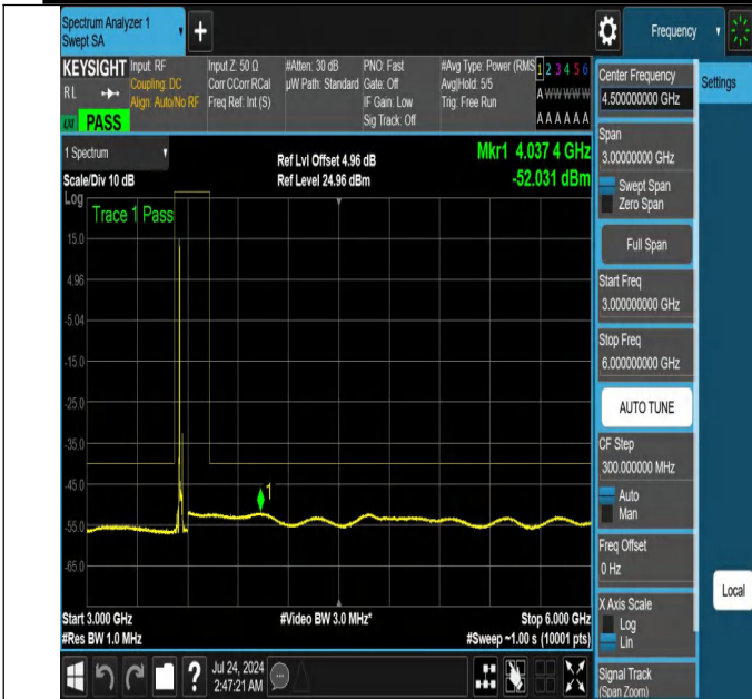
NTNV-N48-PC3-30-20-L-DFT-PI2BPSK-Edge_1RB_Left-3000-60 00-Ant1-PASS
