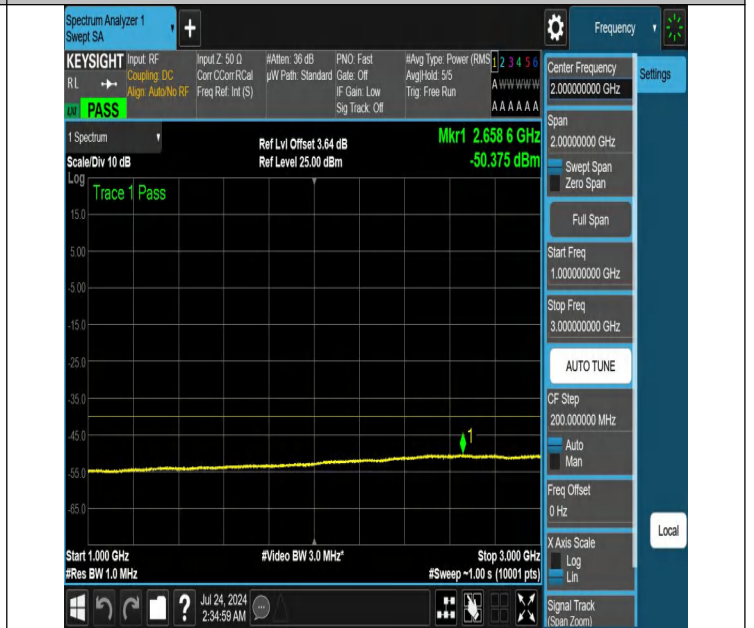
NTNV-N48-PC3-30-15-M-DFT-PI2BPSK-Edge_1RB_Left-1000-3000-Ant1-PASS
