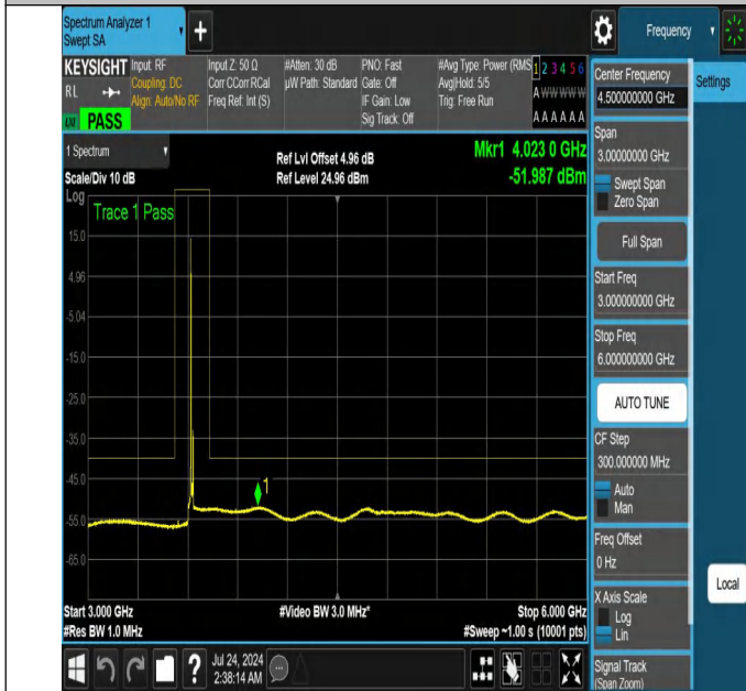
NTNV-N48-PC3-30-15-M-DFT-QPSK-Edge_1RB_Left-3000-6000-Ant1-PASS
