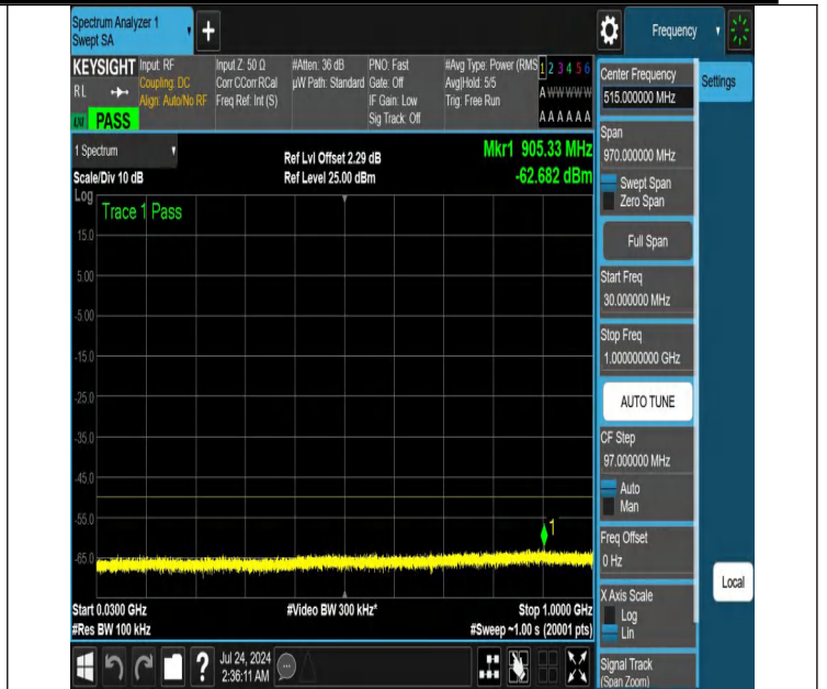
NTNV-N48-PC3-30-15-M-DFT-PI2BPSK-Edge_1RB_Right-30-100-0-Ant1-PASS
