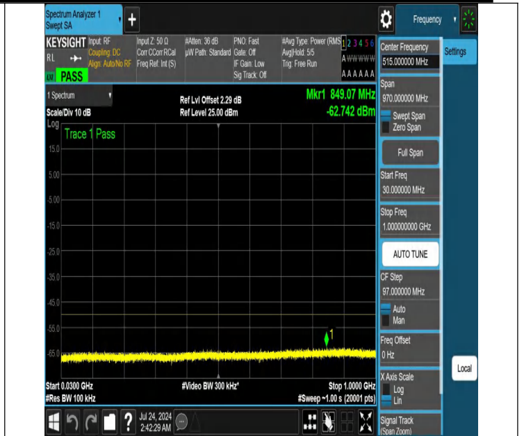
NTNV-N48-PC3-30-15-H-DFT-PI2BPSK-Edge_1RB_Right-30-100 0-Ant1-PASS
