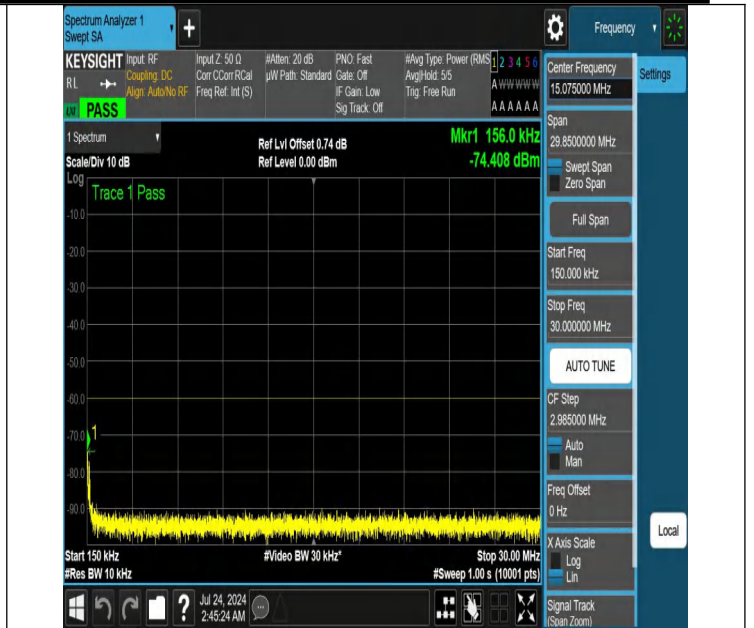
NTNV-N48-PC3-30-20-L-DFT-PI2BPSK-Edge_1RB_Left-0.15-30-Ant1-PASS
